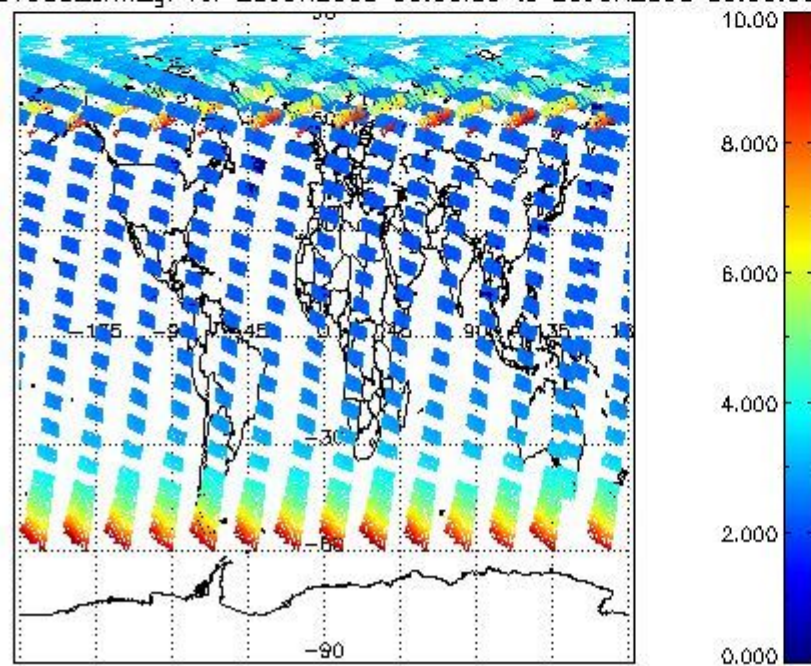
SCIOL2P_NADUV003_amf_gr for 25JUN2008 00:00:00 to 26JUN2008 00:00:00
