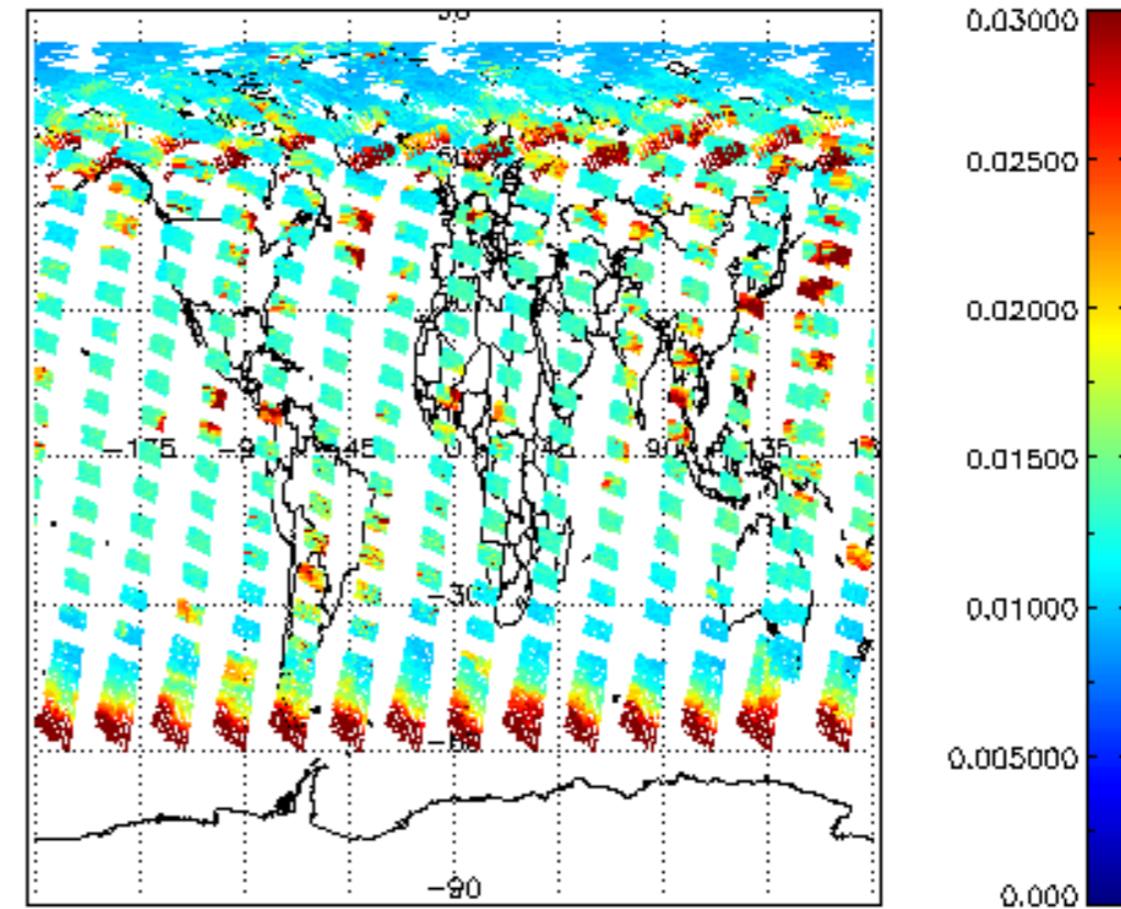
SCIOL2P_NADUV003_vcd_err for 25JUN2008 00:00:00 to 26JUN2008 00:00:00
