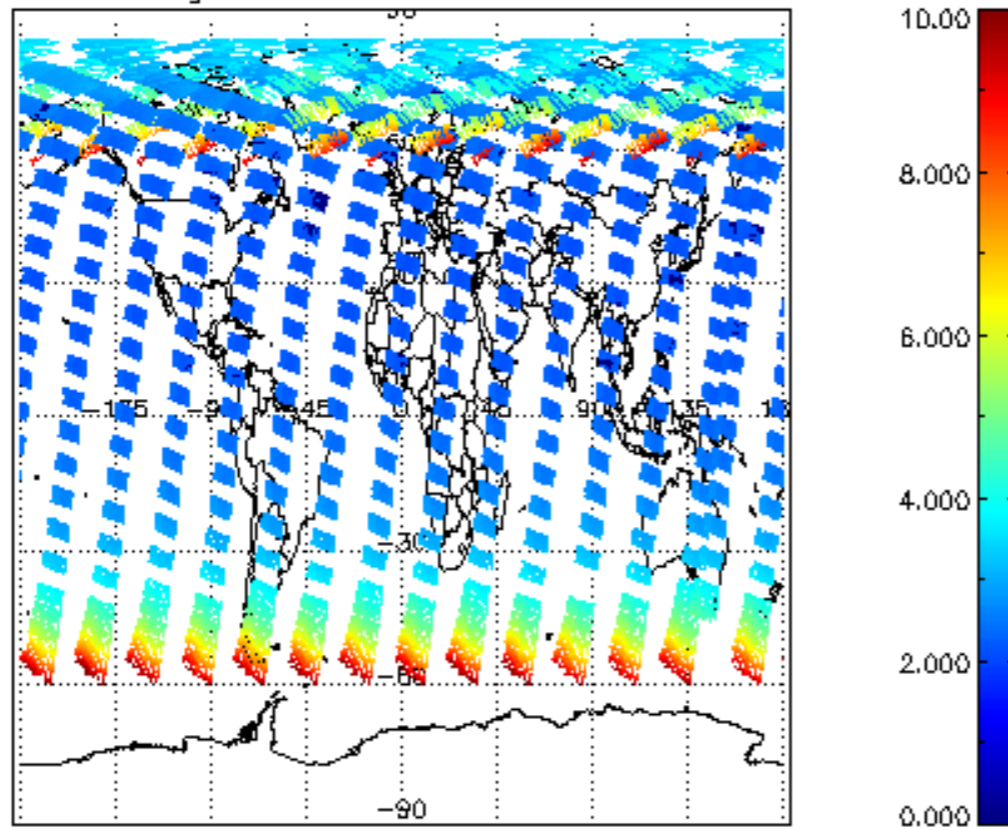
SCIOL2P_NADUV003_amf_gr for 25JUN2008 00:00:00 to 26JUN2008 00:00:00
