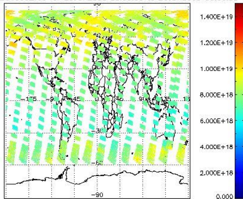
SCIOL2P_NADUV003_vcd for 25JUN2008 00:00:00 to 26JUN2008 00:00:00
