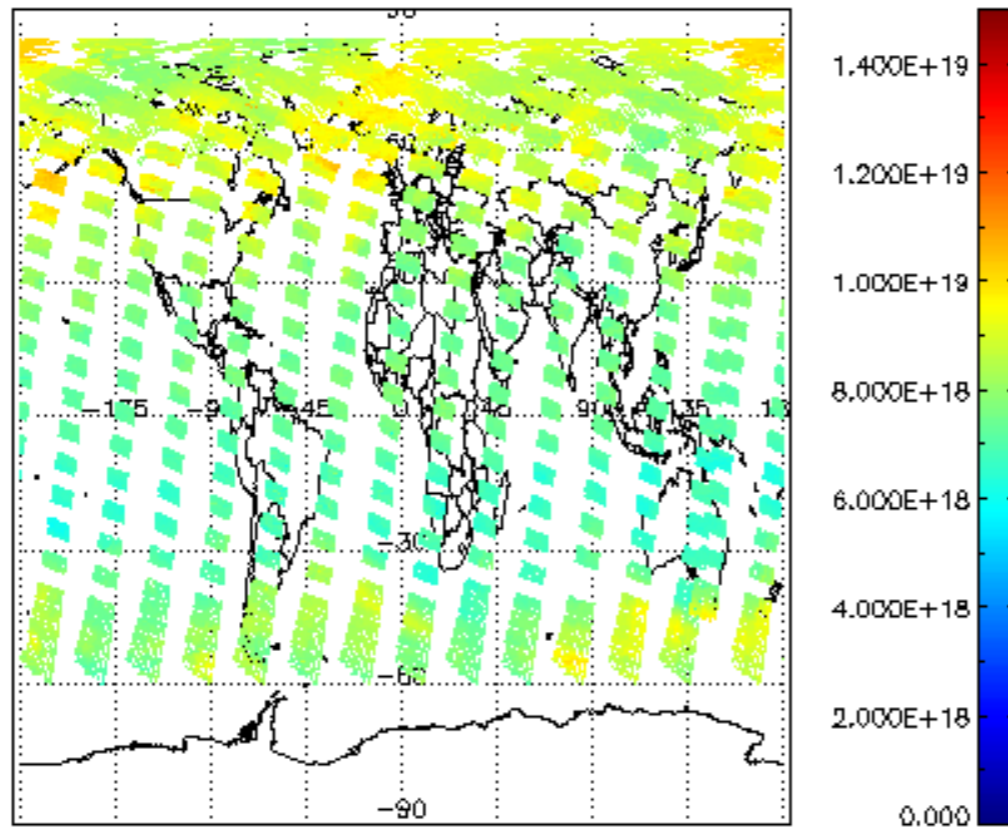
SCIOL2P_NADUV003_vcd for 25JUN2008 00:00:00 to 26JUN2008 00:00:00
