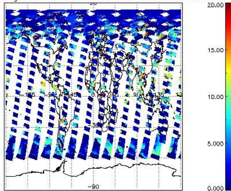
cL_top_height for 25JUN2008 00:00:00 to 26JUN2008 00:00:00
