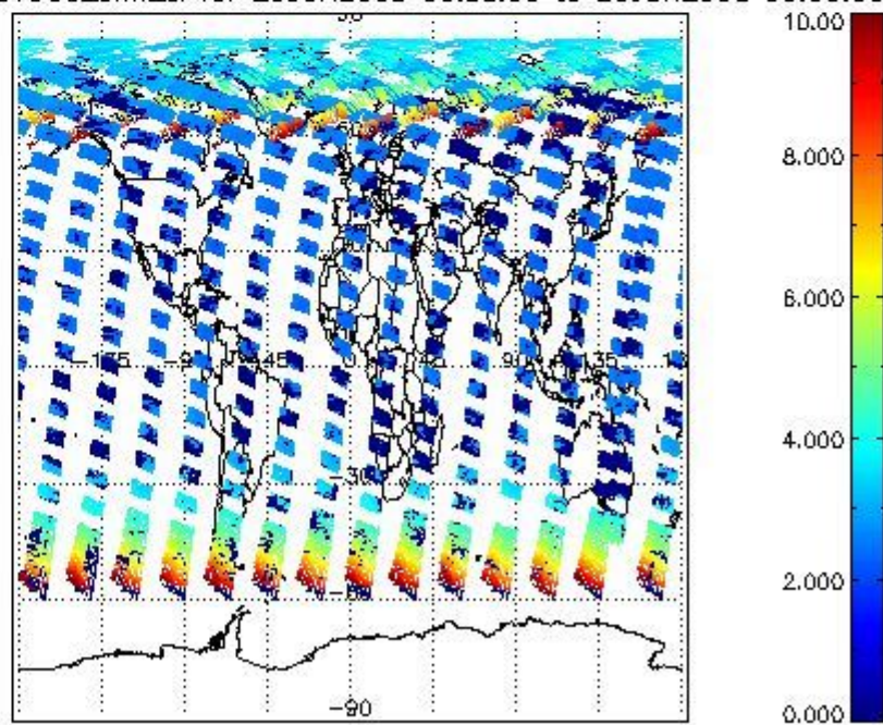
SCIOL2P_NADUV003_amf_cl for 25JUN2008 00:00:00 to 26JUN2008 00:00:00
