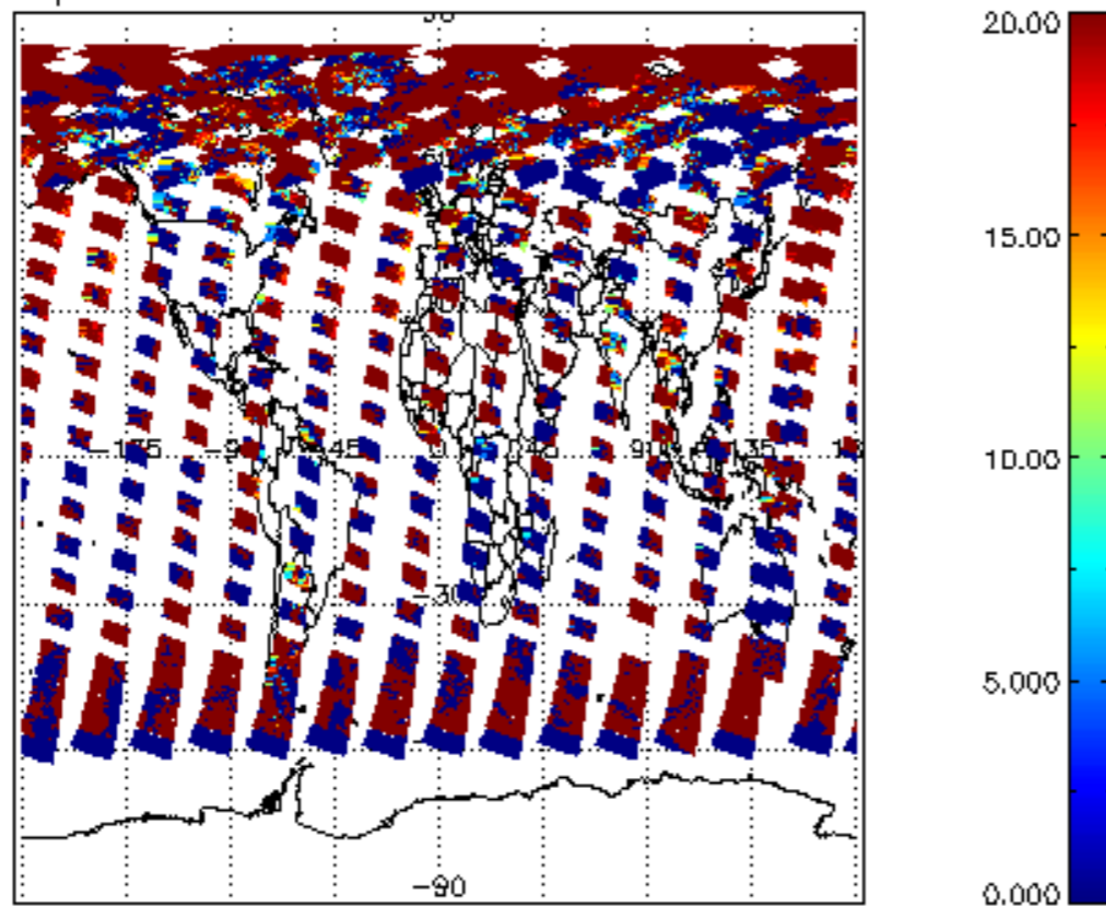
cl_opt_depth for 25JUN2008 00:00:00 to 26JUN2008 00:00:00
