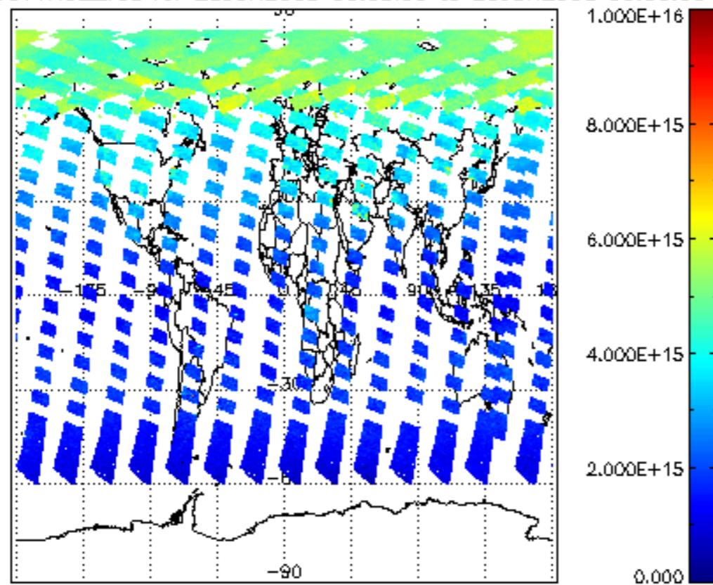
SCIOL2P_NADUV1NO2_vcd for 25JUN2008 00:00:00 to 26JUN2008 00:00:00
