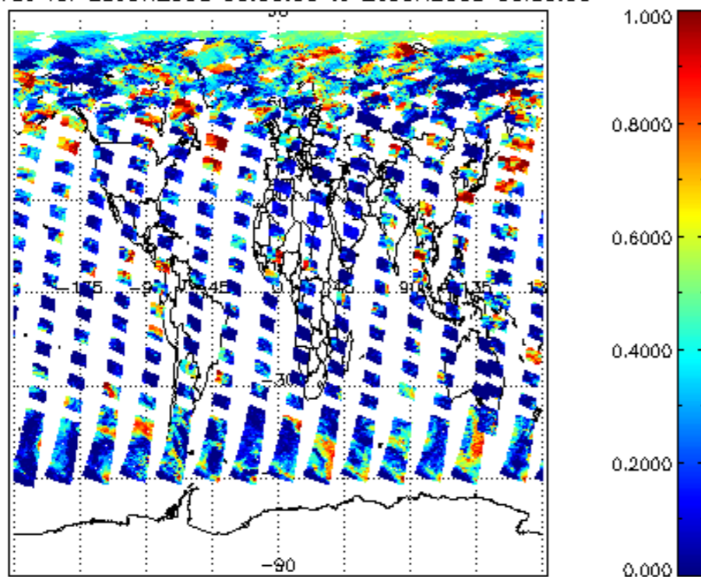
cl_frac for 25JUN2008 00:00:00 to 26JUN2008 00:00:00
