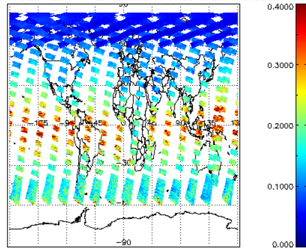
iCIOL2P_NADUV1NO2_vcd_err for 25JUN2008 00:00:00 to 26JUN2008 00:00:00
