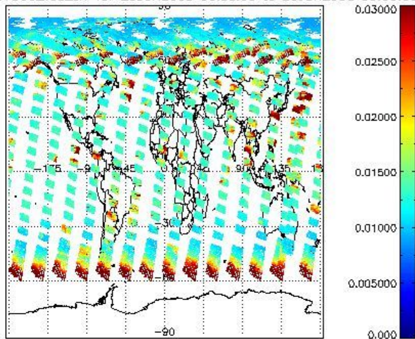
SCIOL2P_NADUV003_vcd_err for 25JUN2008 00:00:00 to 26JUN2008 00:00:00
