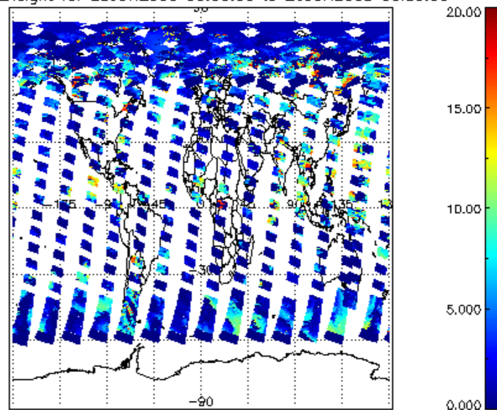
cl_top_height for 25JUN2008 00:00:00 to 26JUN2008 00:00:00
