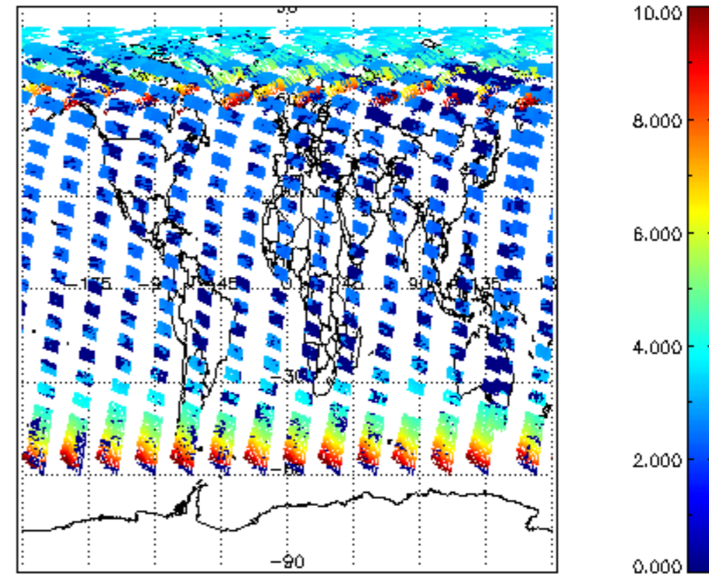
SCIOL2P_NADUV003_amf_cl for 25JUN2008 00:00:00 to 26JUN2008 00:00:00
