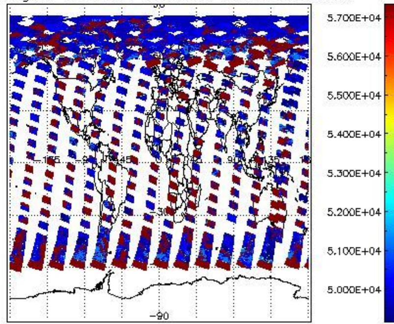
cloud_flags for 25JUN2008 00:00:00 to 26JUN2008 00:00:00
