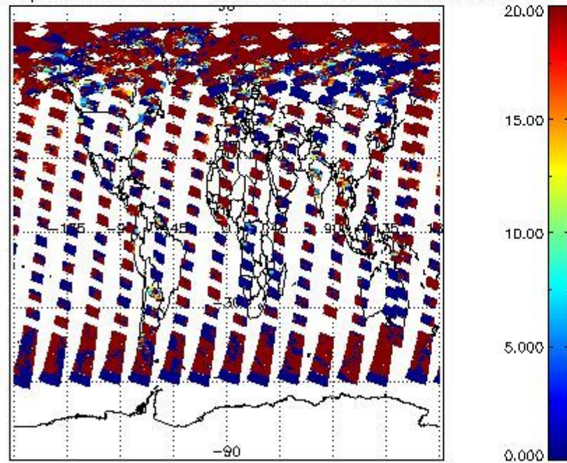
cL_opt_depth for 25JUN2008 00:00:00 to 26JUN2008 00:00:00
