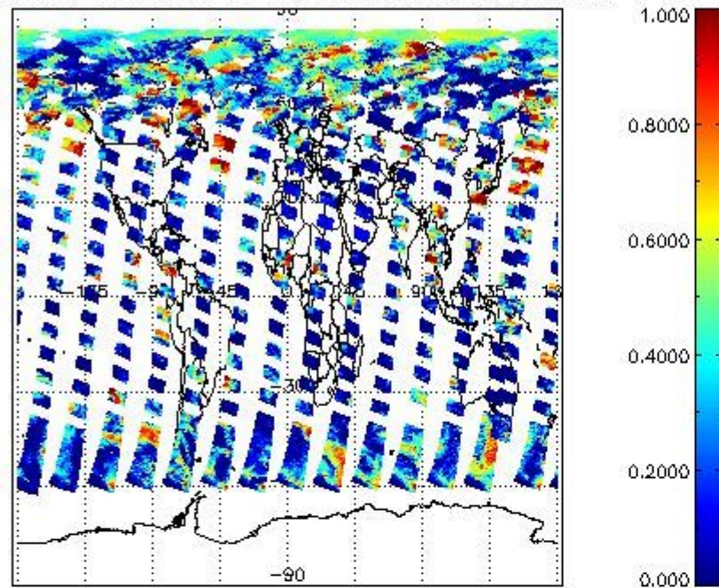
cL_frac for 25JUN2008 00:00:00 to 26JUN2008 00:00:00
