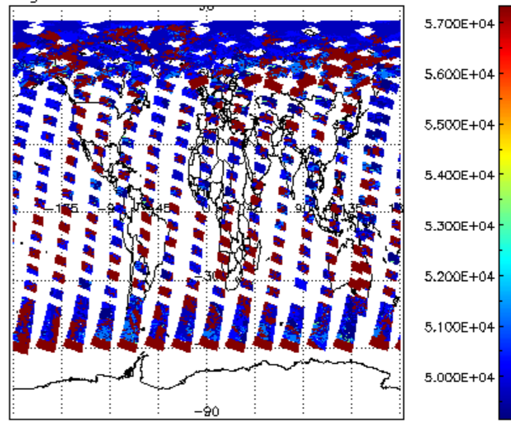
cloud_flags for 25JUN2008 00:00:00 to 26JUN2008 00:00:00
