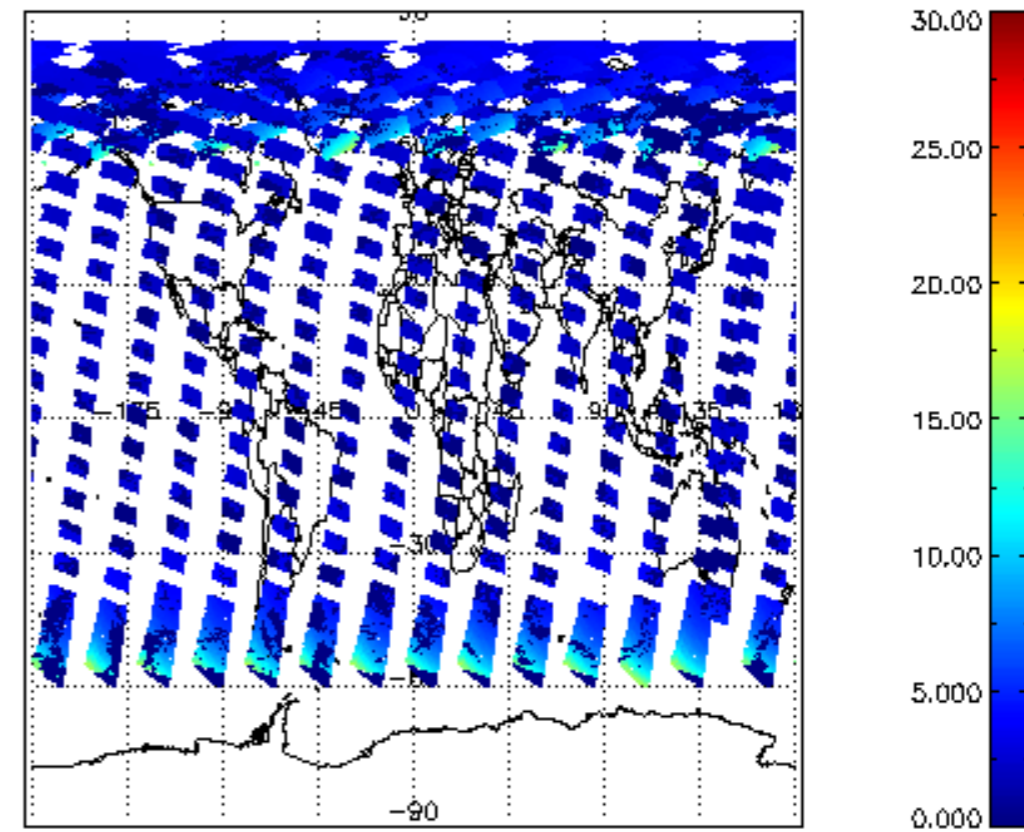
iCIOL2P_NADUV1NO2_amf_cl for 25JUN2008 00:00:00 to 26JUN2008 00:00:00
