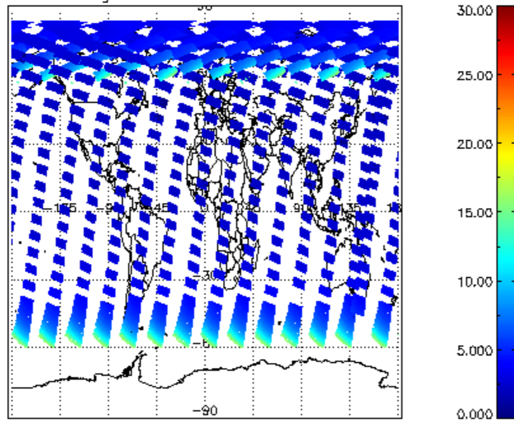
iCIOL2P_NADUV1NO2_amf_gr for 25JUN2008 00:00:00 to 26JUN2008 00:00:00
