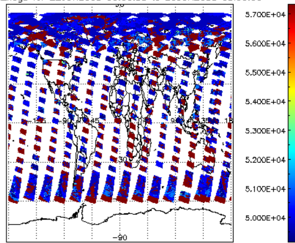
cloud_flags for 22JUN2008 00:00:00 to 23JUN2008 00:00:00
