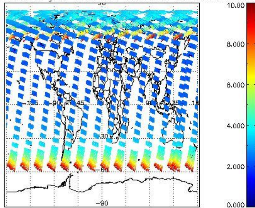
SCIOL2P_NADUV003_amf_gr for 22JUN2008 00:00:00 to 23JUN2008 00:00:00
