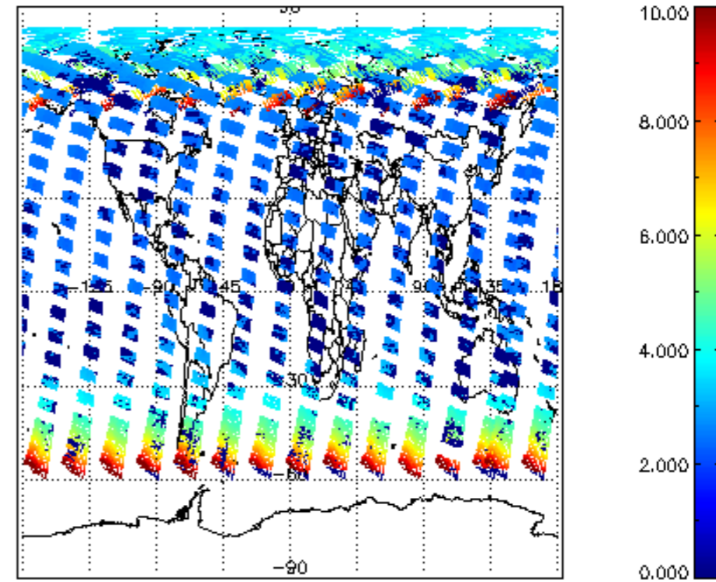
SCIOL2P_NADUV003_amf_cl for 22JUN2008 00:00:00 to 23JUN2008 00:00:00
