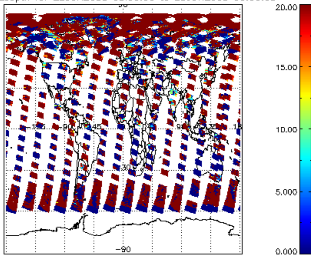
cl_opt_depth for 22JUN2008 00:00:00 to 23JUN2008 00:00:00
