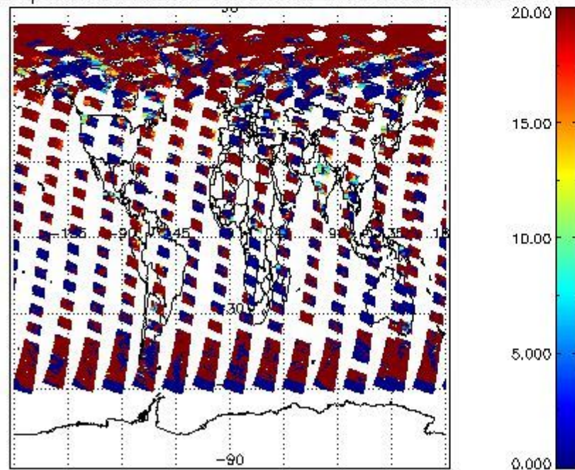
cL_opt_depth for 22JUN2008 00:00:00 to 23JUN2008 00:00:00
