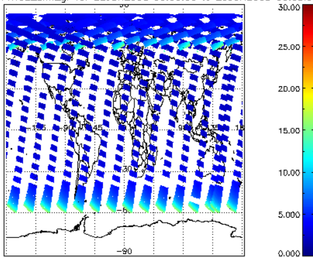
iCIOL2P_NADUV1NO2_amf_gr for 22JUN2008 00:00:00 to 23JUN2008 00:00:00
