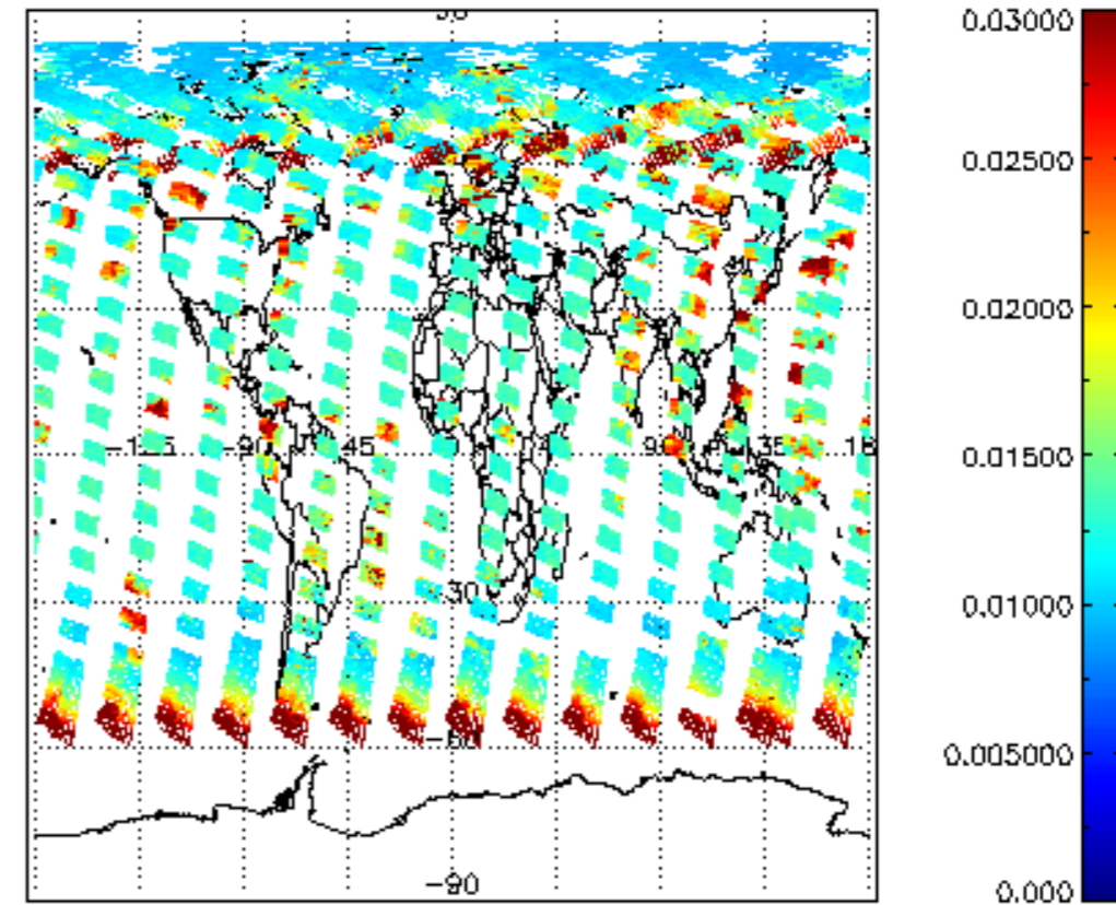
SCIOL2P_NADUV003_vcd_err for 22JUN2008 00:00:00 to 23JUN2008 00:00:00
