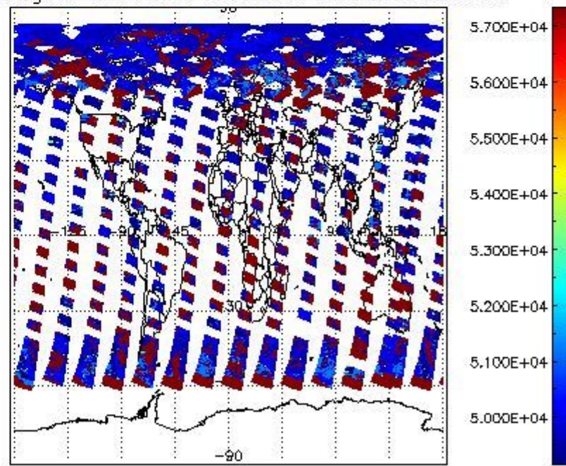
cloud_flags for 22JUN2008 00:00:00 to 23JUN2008 00:00:00
