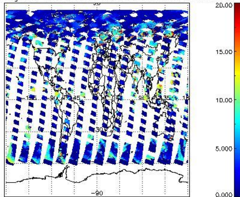
cL_top_height for 22JUN2008 00:00:00 to 23JUN2008 00:00:00
