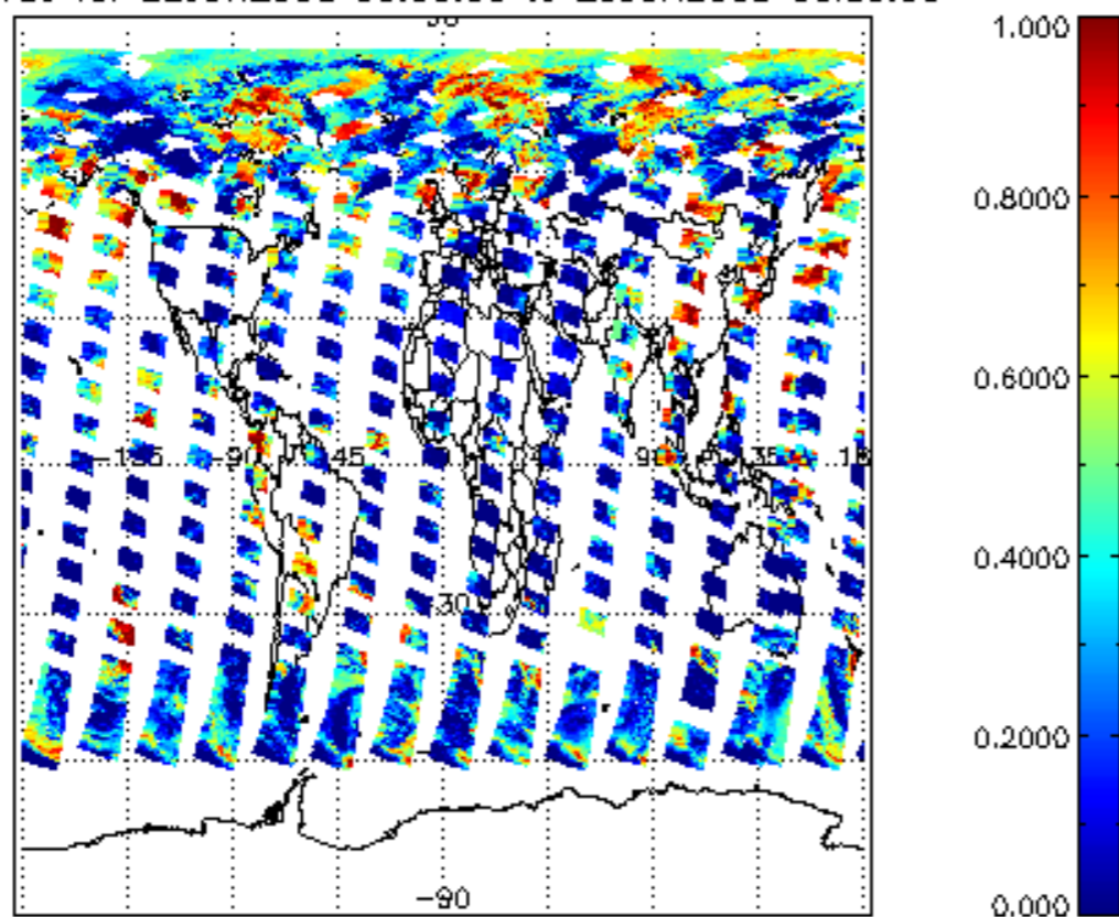
cl_frac for 22JUN2008 00:00:00 to 23JUN2008 00:00:00
