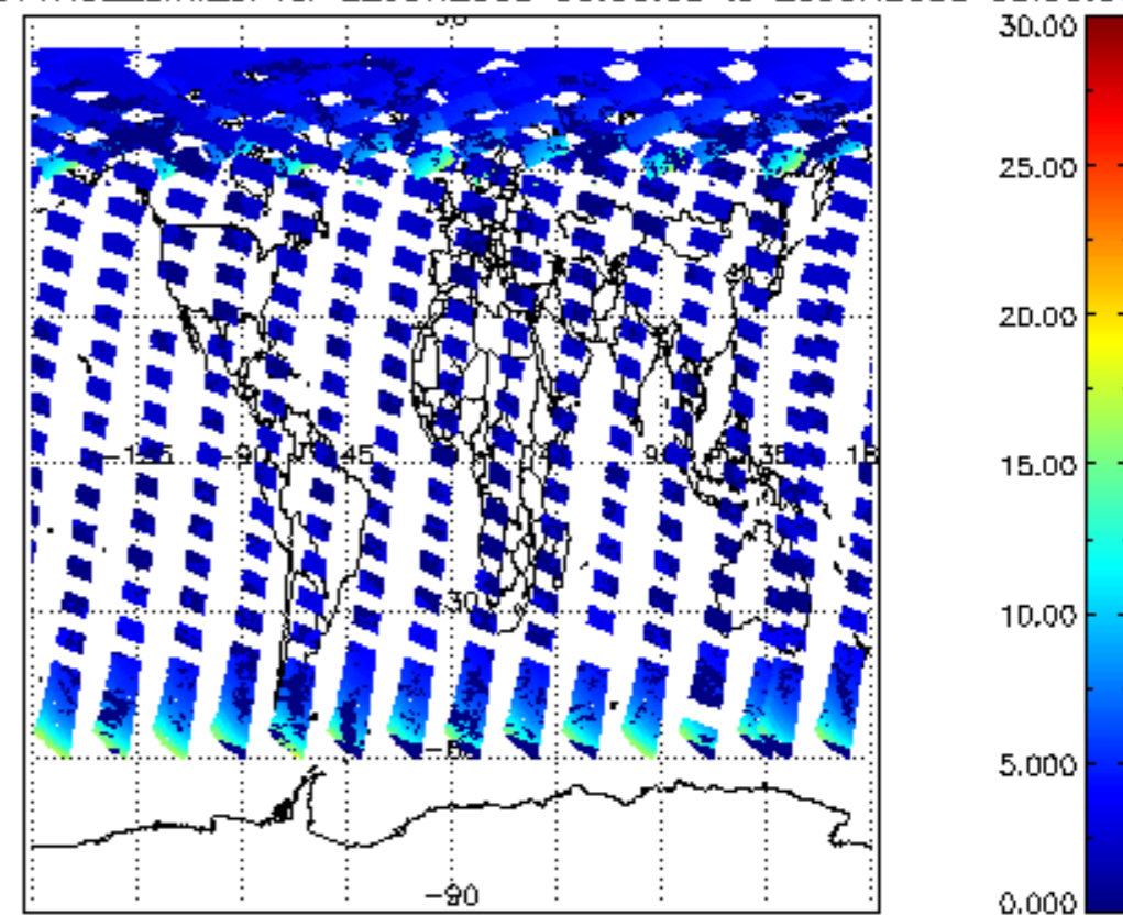
iCIOL2P_NADUV1NO2_amf_cl for 22JUN2008 00:00:00 to 23JUN2008 00:00:00
