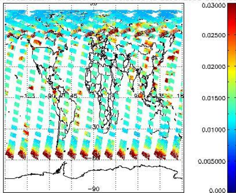
SCIOL2P_NADUV003_vcd_err for 22JUN2008 00:00:00 to 23JUN2008 00:00:00
