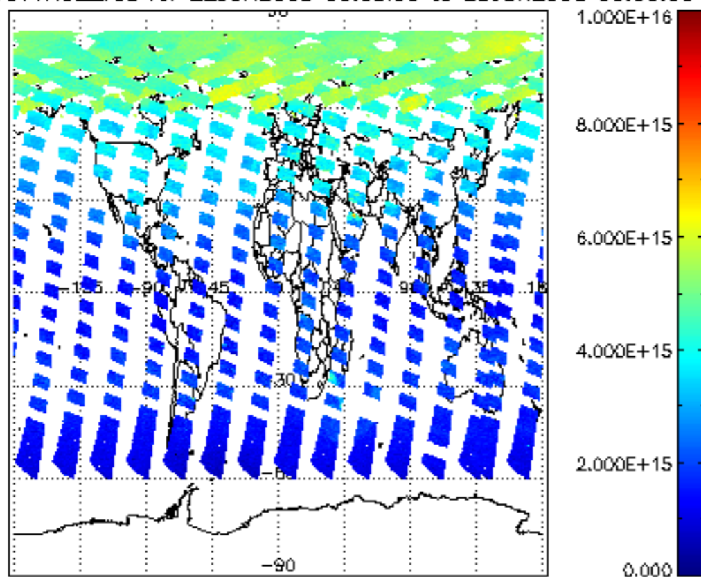
SCIOL2P_NADUV1NO2_vcd for 22JUN2008 00:00:00 to 23JUN2008 00:00:00
