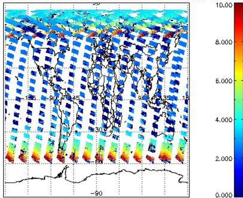
SCIOL2P_NADUV003_amf_cl for 22JUN2008 00:00:00 to 23JUN2008 00:00:00
