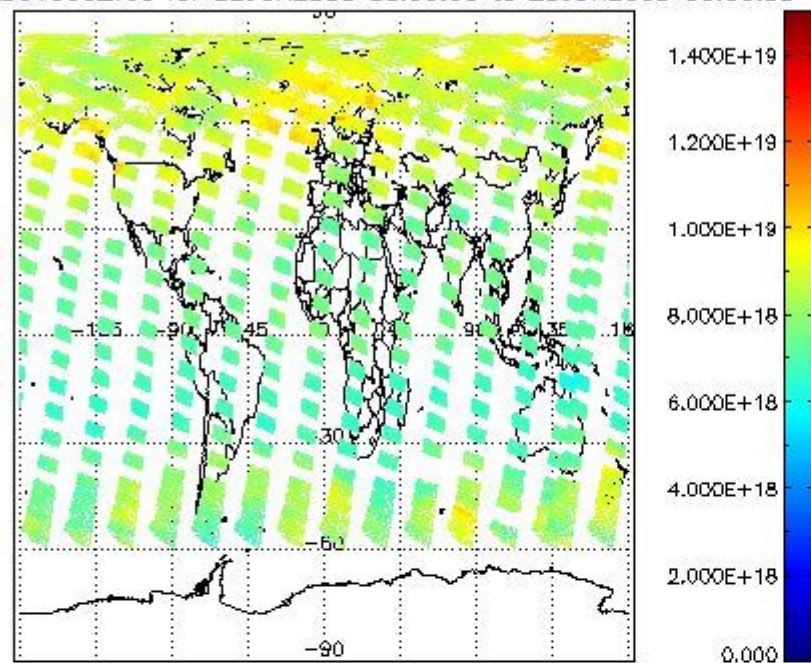
SCIOL2P_NADUV003_vcd for 22JUN2008 00:00:00 to 23JUN2008 00:00:00
