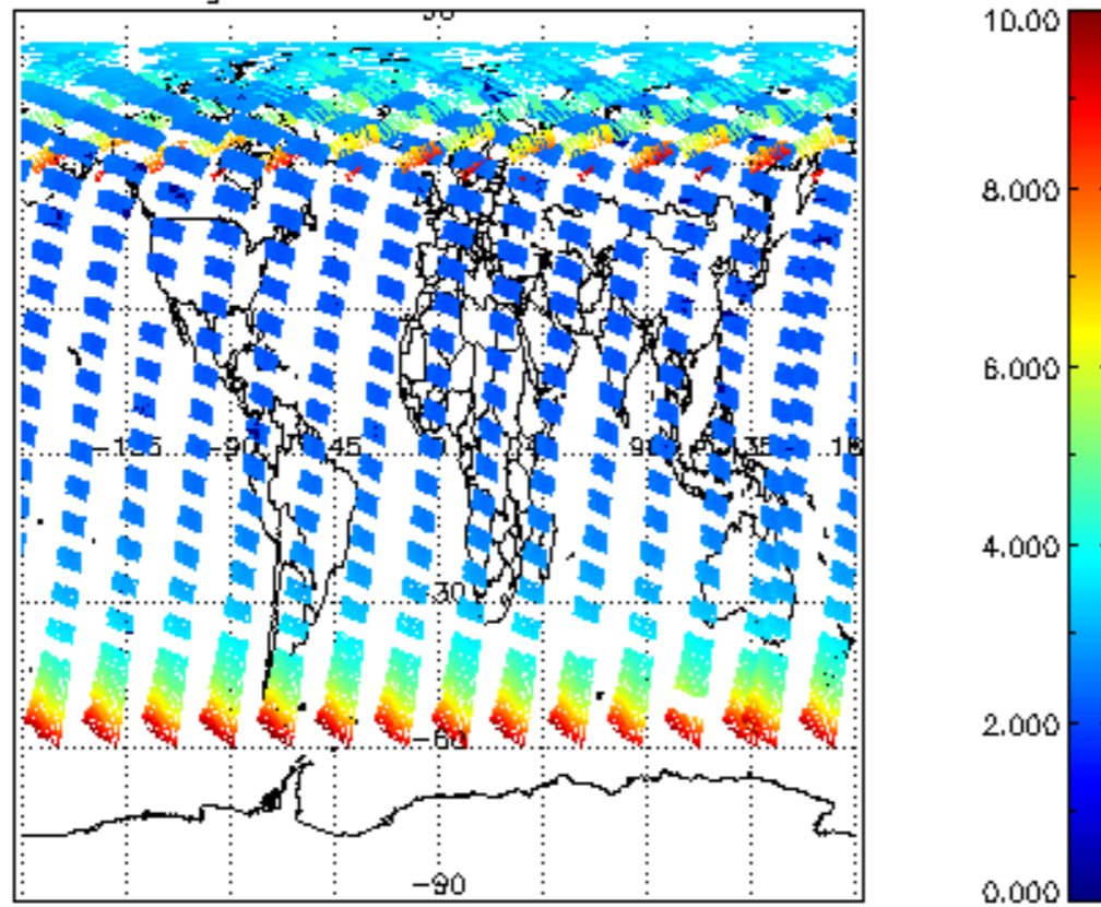
SCIOL2P_NADUV003_amf_gr for 22JUN2008 00:00:00 to 23JUN2008 00:00:00
