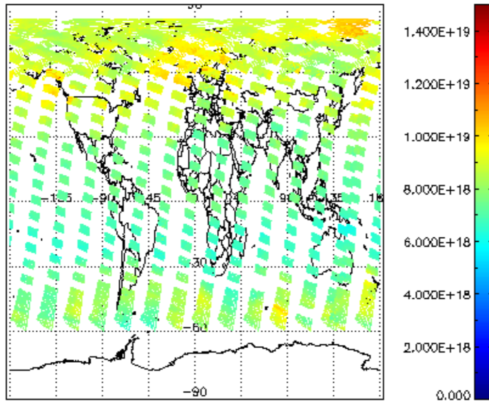
SCIOL2P_NADUV003_vcd for 22JUN2008 00:00:00 to 23JUN2008 00:00:00
