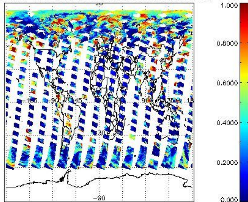
cL_frac for 22JUN2008 00:00:00 to 23JUN2008 00:00:00
