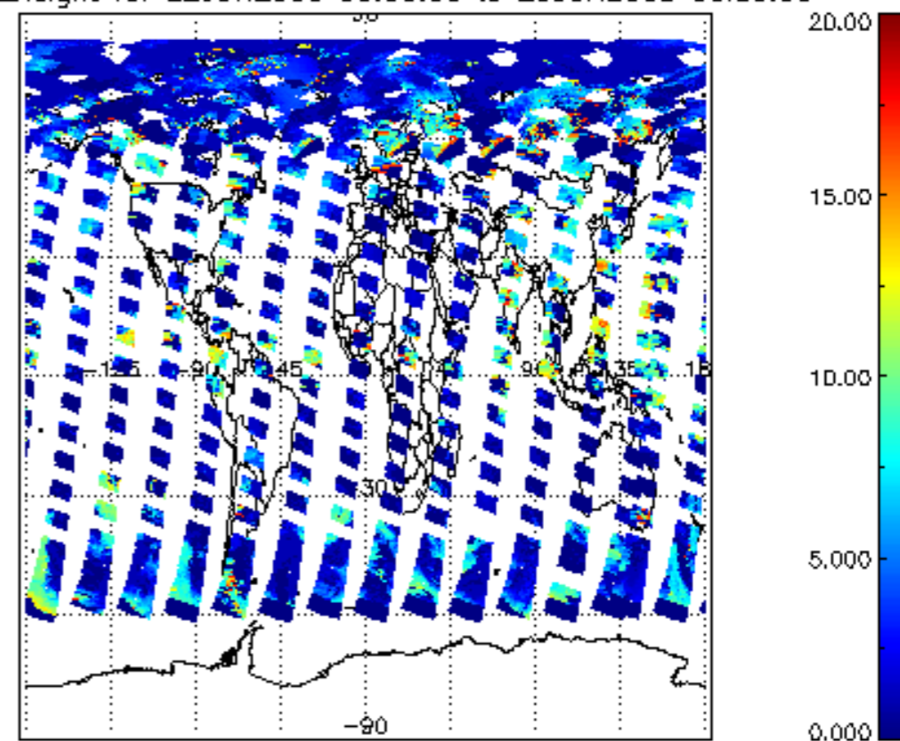
cl_top_height for 22JUN2008 00:00:00 to 23JUN2008 00:00:00
