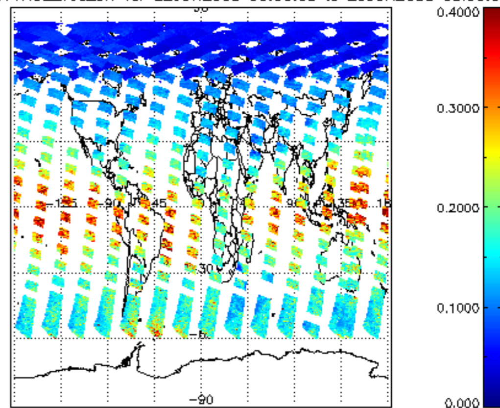
iCIOL2P_NADUV1NO2_vcd_err for 22JUN2008 00:00:00 to 23JUN2008 00:00:00
