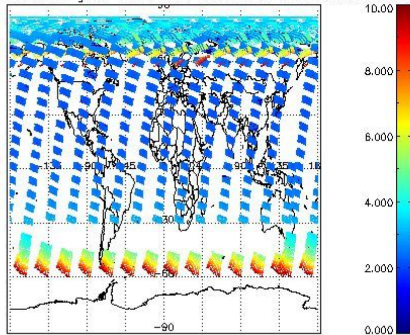
SCIOL2P_NADUV003_amf_gr for 16JUN2008 00:00:00 to 17JUN2008 00:00:00
