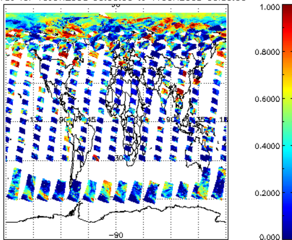
cl_frac for 16JUN2008 00:00:00 to 17JUN2008 00:00:00
