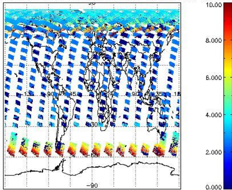
SCIOL2P_NADUV003_amf_cl for 16JUN2008 00:00:00 to 17JUN2008 00:00:00
