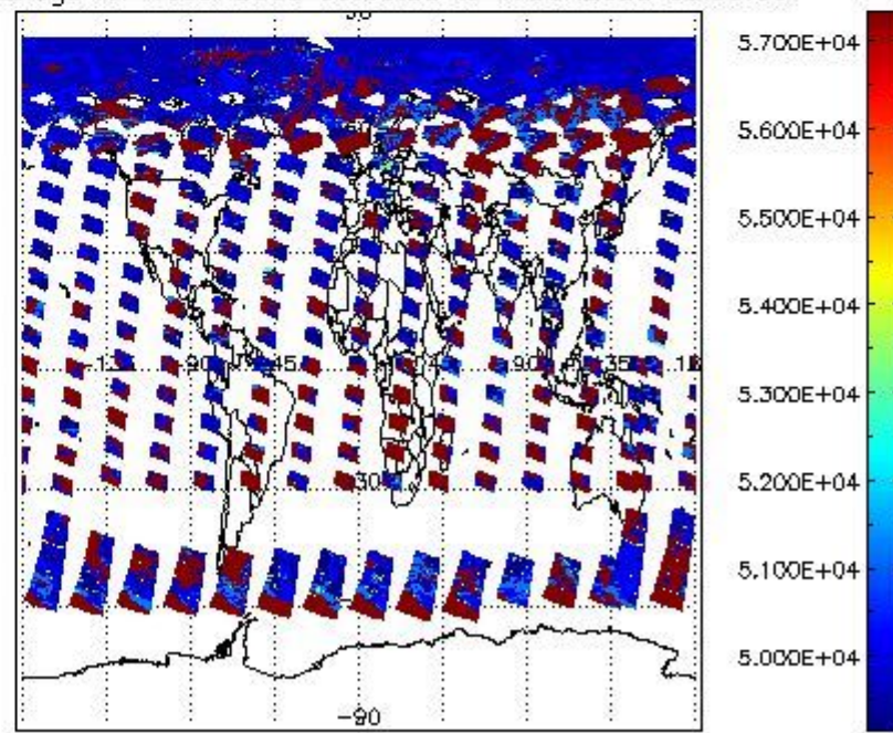
cloud_flags for 16JUN2008 00:00:00 to 17JUN2008 00:00:00
