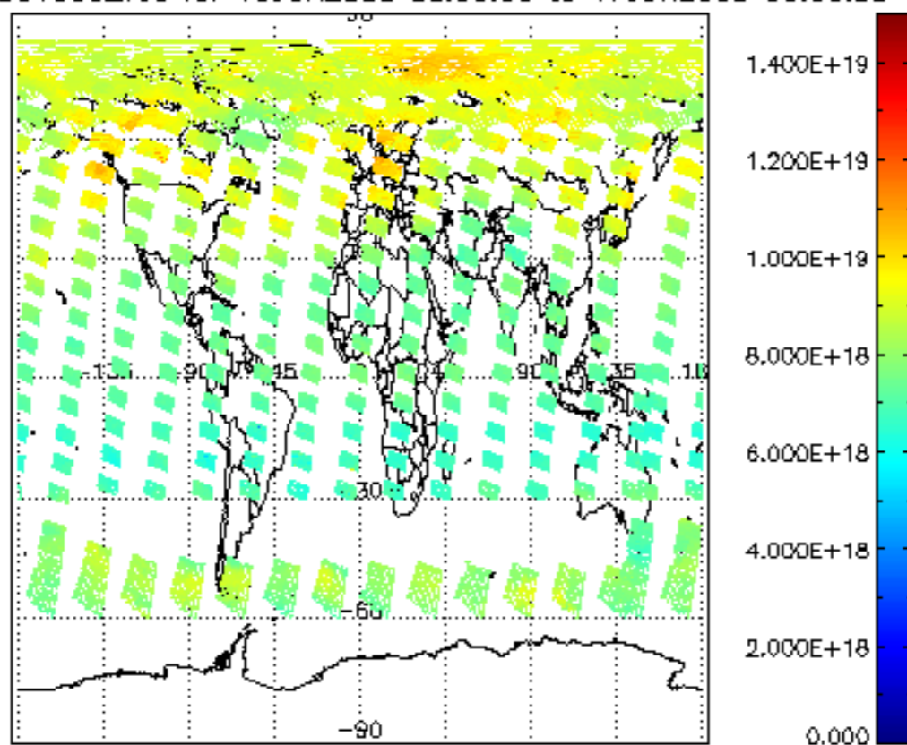
SCIOL2P_NADUV003_vcd for 16JUN2008 00:00:00 to 17JUN2008 00:00:00
