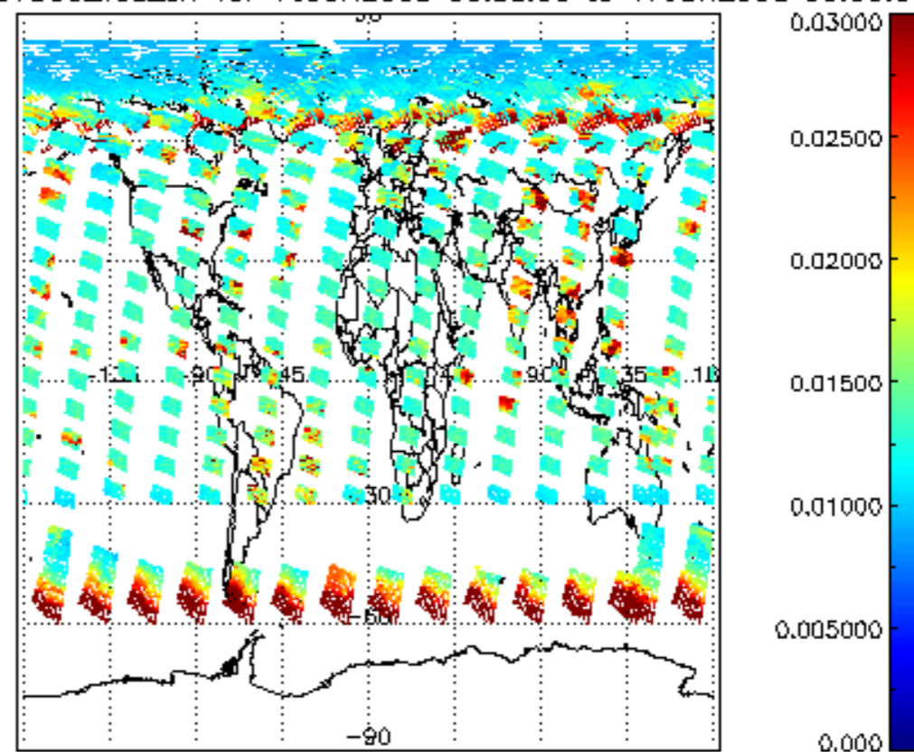
SCIOL2P_NADUV003_vcd_err for 16JUN2008 00:00:00 to 17JUN2008 00:00:00
