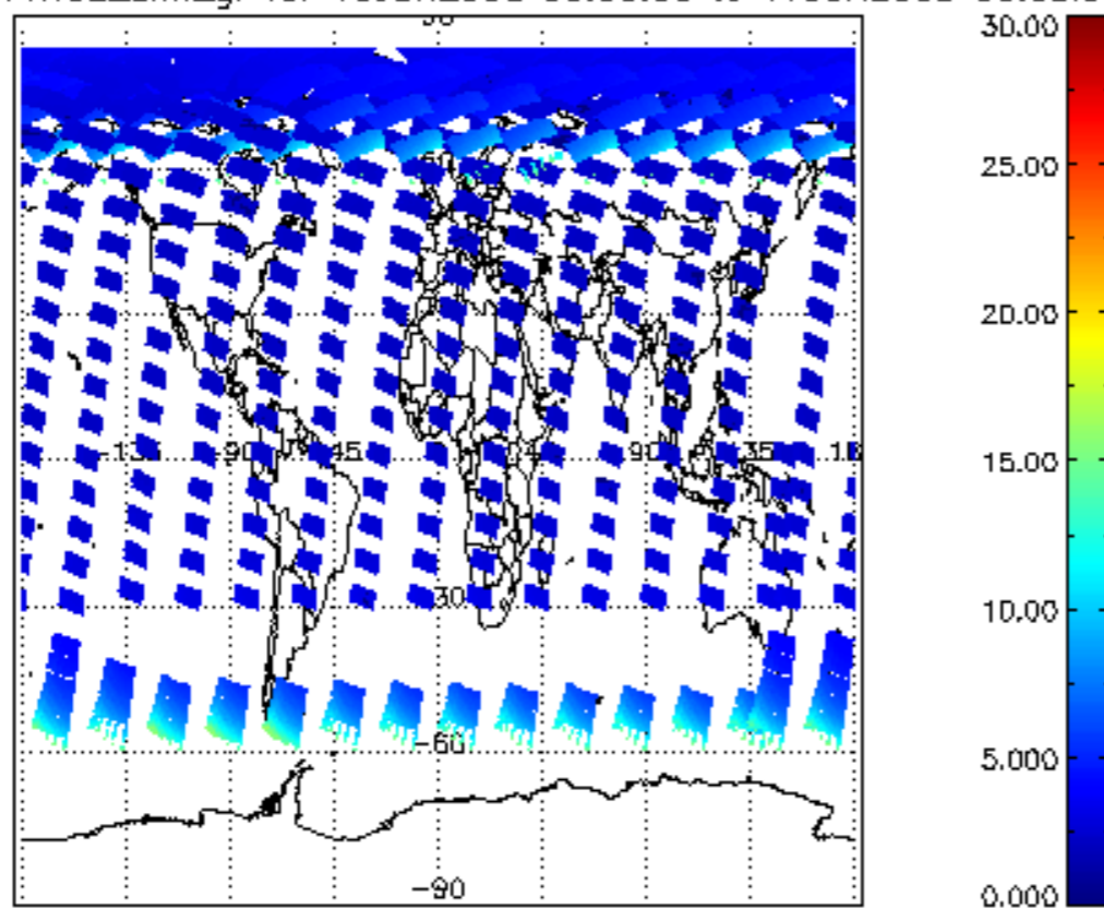
iCIOL2P_NADUV1NO2_amf_gr for 16JUN2008 00:00:00 to 17JUN2008 00:00:00
