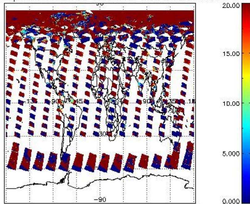
cL_opt_depth for 16JUN2008 00:00:00 to 17JUN2008 00:00:00
