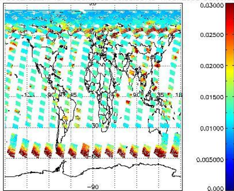
SCIOL2P_NADUV003_vcd_err for 16JUN2008 00:00:00 to 17JUN2008 00:00:00
