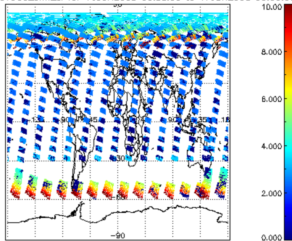
SCIOL2P_NADUV003_amf_cl for 16JUN2008 00:00:00 to 17JUN2008 00:00:00
