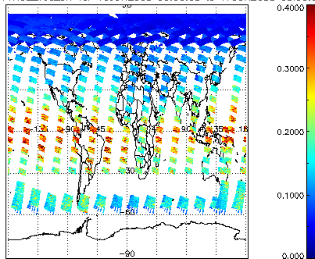
iCIOL2P_NADUV1NO2_vcd_err for 16JUN2008 00:00:00 to 17JUN2008 00:00:00
