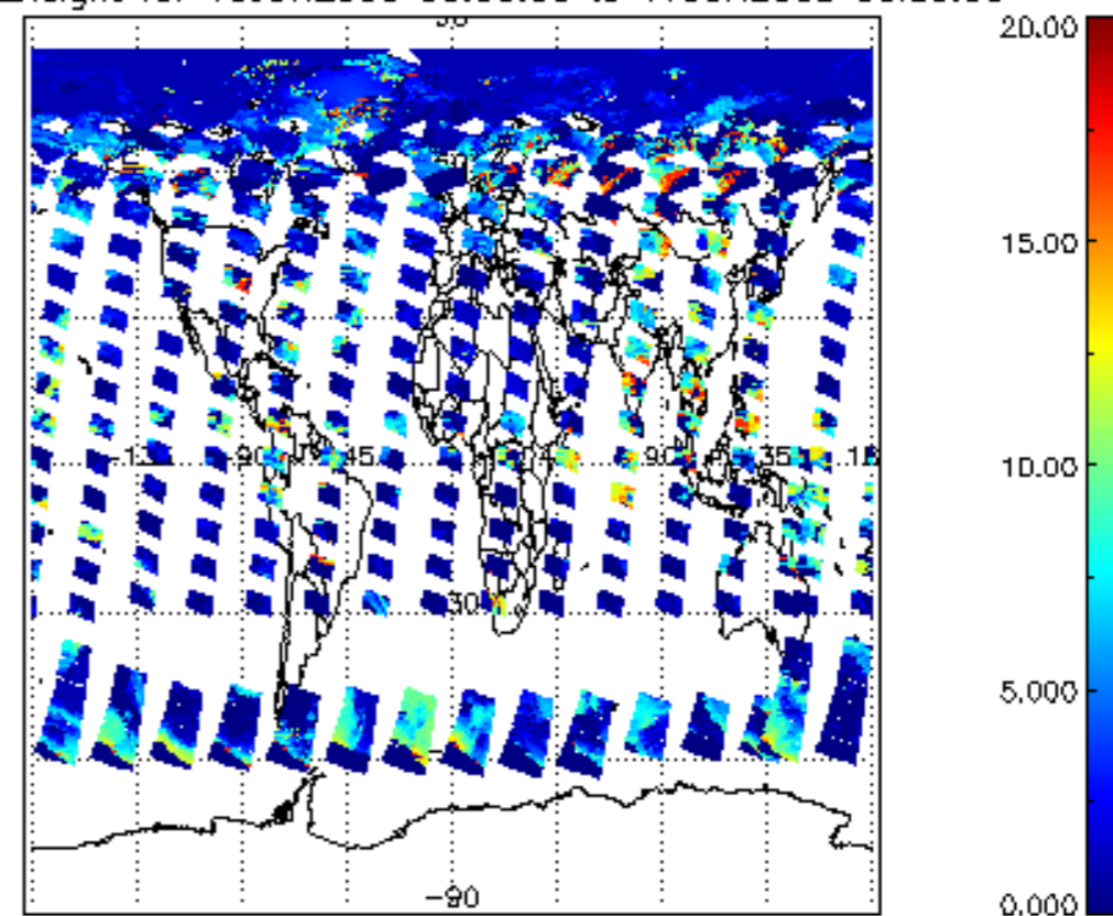
cl_top_height for 16JUN2008 00:00:00 to 17JUN2008 00:00:00
