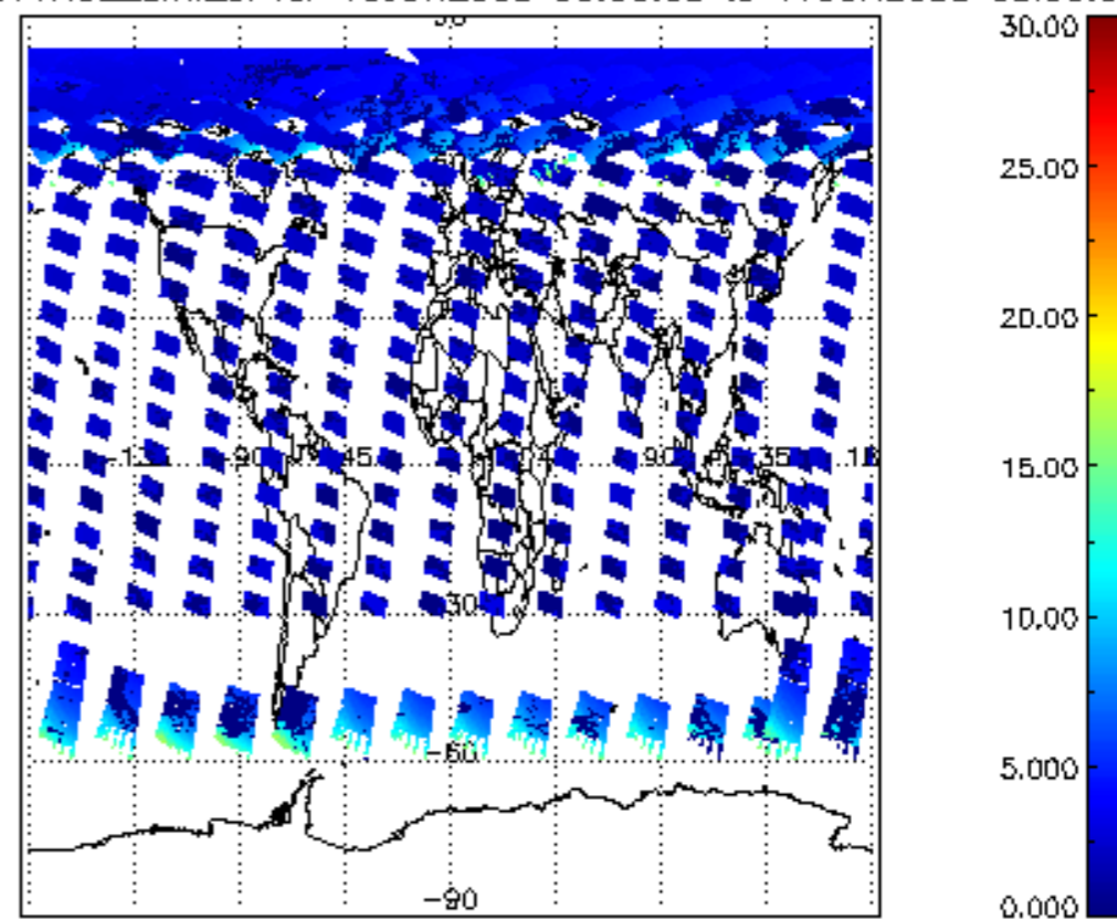
iCIOL2P_NADUV1NO2_amf_cl for 16JUN2008 00:00:00 to 17JUN2008 00:00:00
