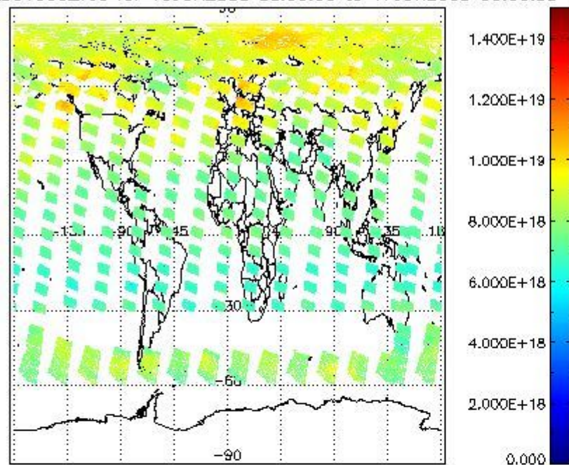
SCIOL2P_NADUV003_vcd for 16JUN2008 00:00:00 to 17JUN2008 00:00:00
