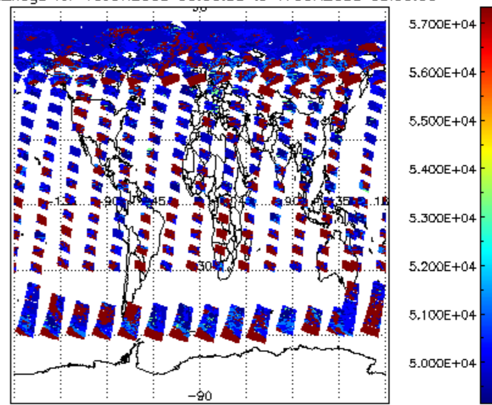
cloud_flags for 16JUN2008 00:00:00 to 17JUN2008 00:00:00
