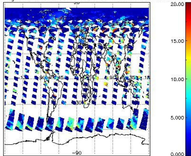
cL_top_height for 16JUN2008 00:00:00 to 17JUN2008 00:00:00
