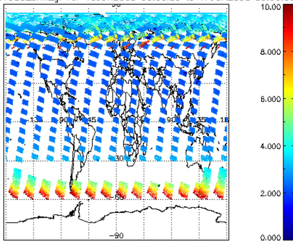
SCIOL2P_NADUV003_amf_gr for 16JUN2008 00:00:00 to 17JUN2008 00:00:00
