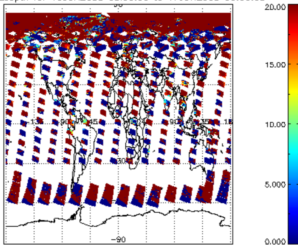
cl_opt_depth for 16JUN2008 00:00:00 to 17JUN2008 00:00:00
