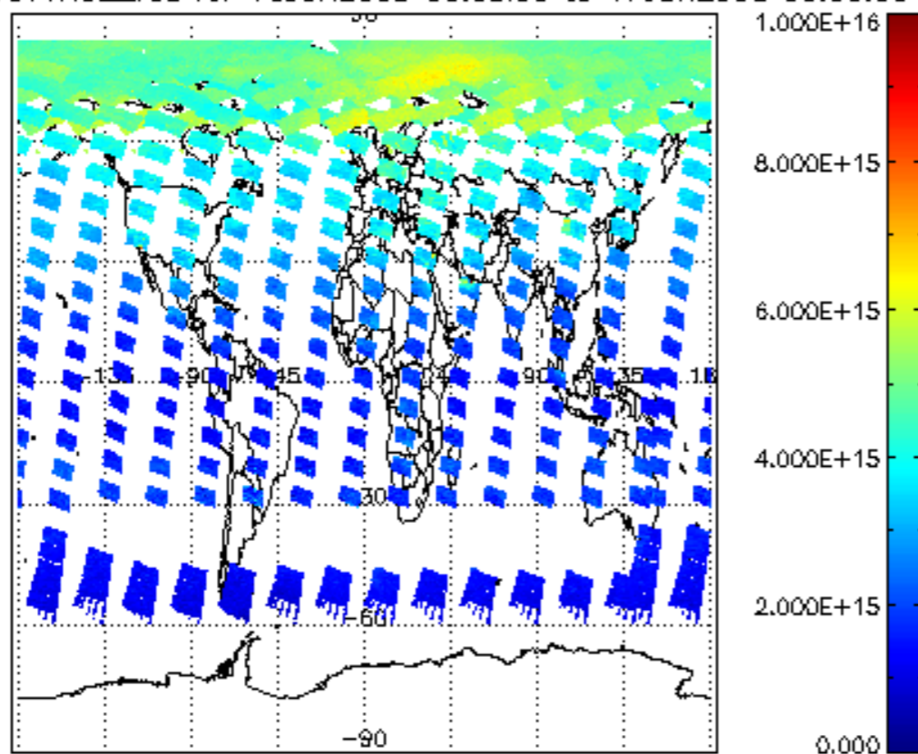
SCIOL2P_NADUV1NO2_vcd for 16JUN2008 00:00:00 to 17JUN2008 00:00:00
