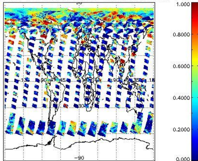
cL_frac for 16JUN2008 00:00:00 to 17JUN2008 00:00:00
