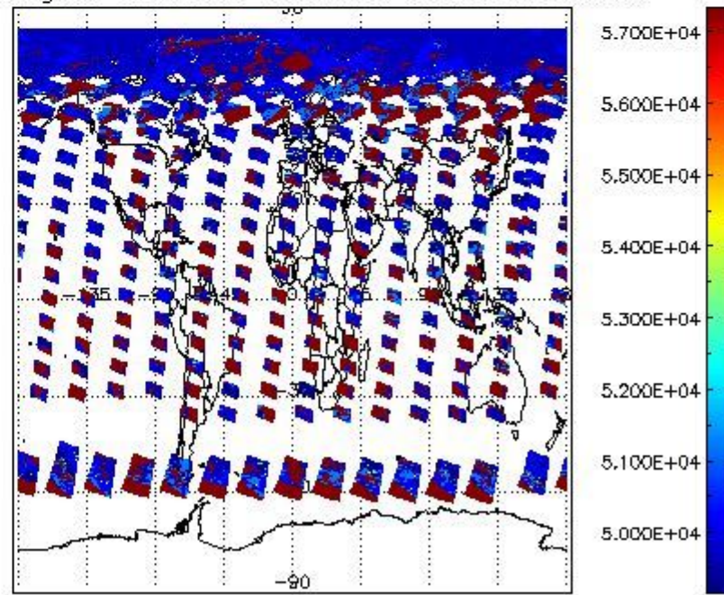
cloud_flags for 15JUN2008 00:00:00 to 16JUN2008 00:00:00
