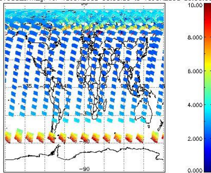
SCIOL2P_NADUV003_amf_gr for 15JUN2008 00:00:00 to 16JUN2008 00:00:00
