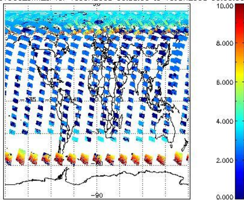
SCIOL2P_NADUV003_amf_cl for 15JUN2008 00:00:00 to 16JUN2008 00:00:00
