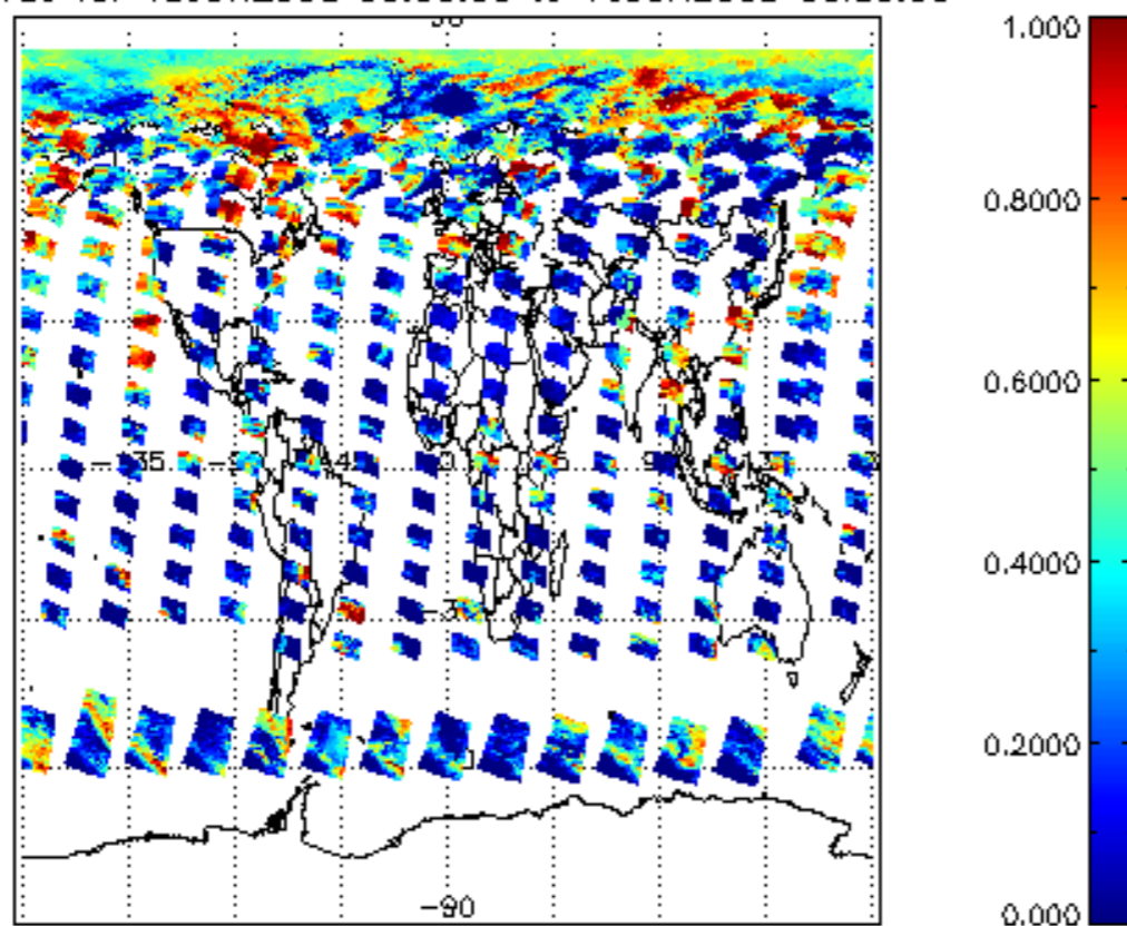
cl_frac for 15JUN2008 00:00:00 to 16JUN2008 00:00:00
