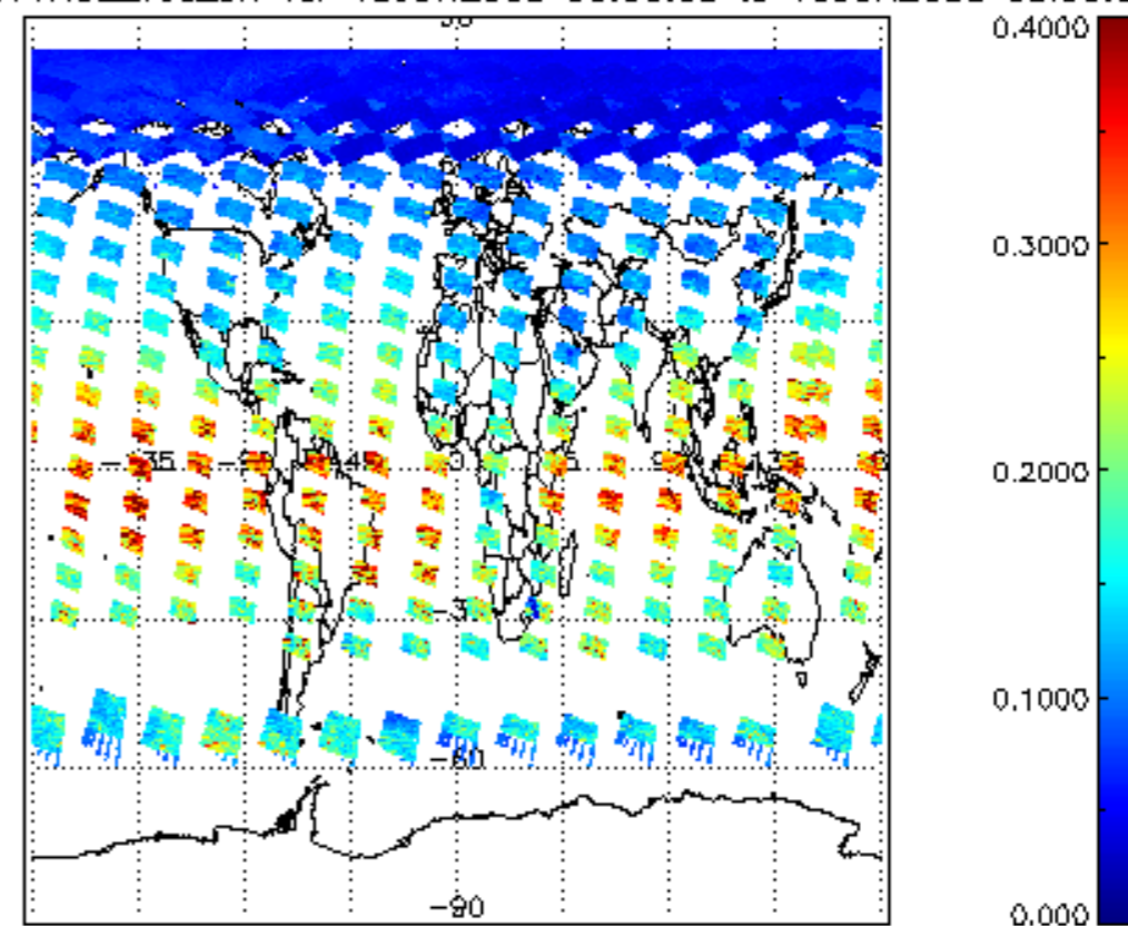
iCIOL2P_NADUV1NO2_vcd_err for 15JUN2008 00:00:00 to 16JUN2008 00:00:00
