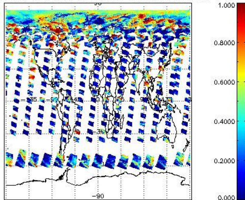
cL_frac for 15JUN2008 00:00:00 to 16JUN2008 00:00:00
