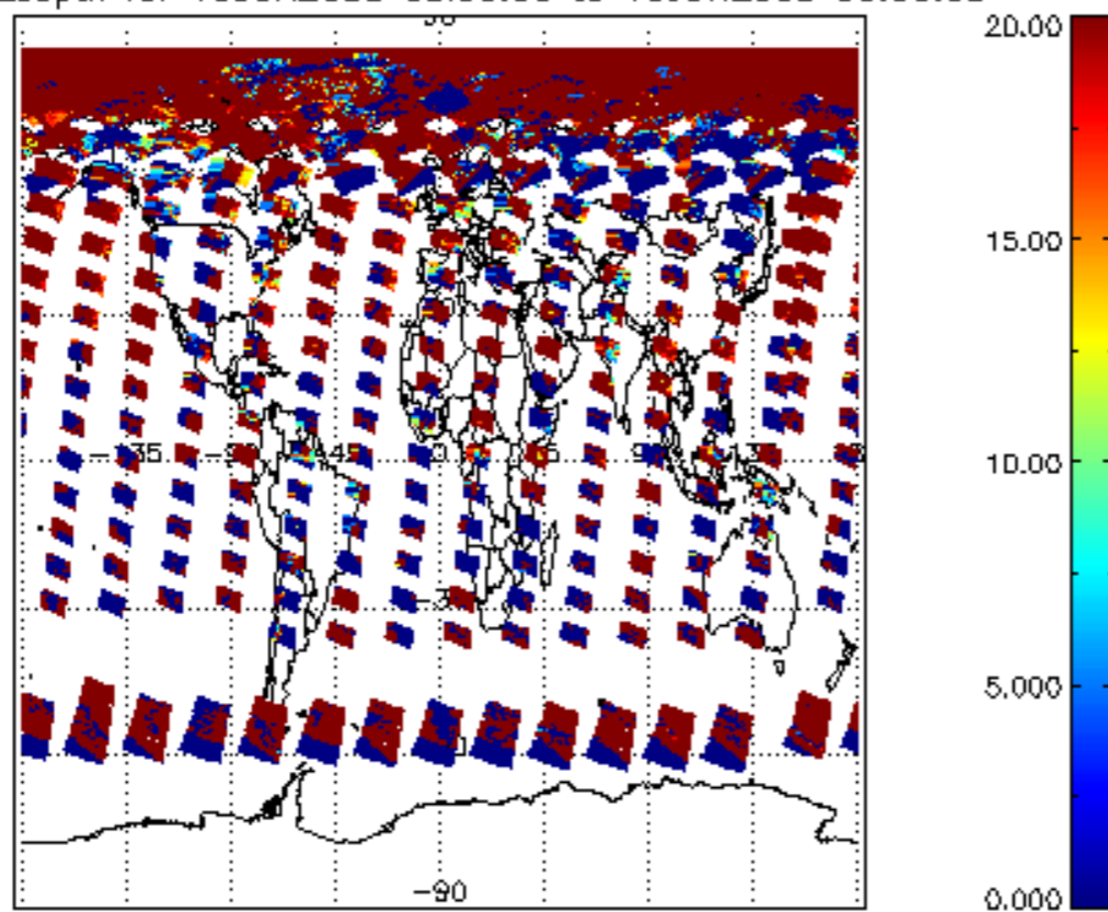
cl_opt_depth for 15JUN2008 00:00:00 to 16JUN2008 00:00:00
