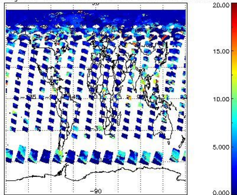
cL_top_height for 15JUN2008 00:00:00 to 16JUN2008 00:00:00
