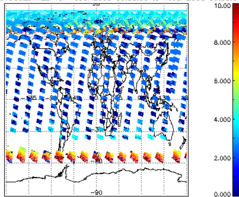
SCIOL2P_NADUV003_amf_cl for 15JUN2008 00:00:00 to 16JUN2008 00:00:00
