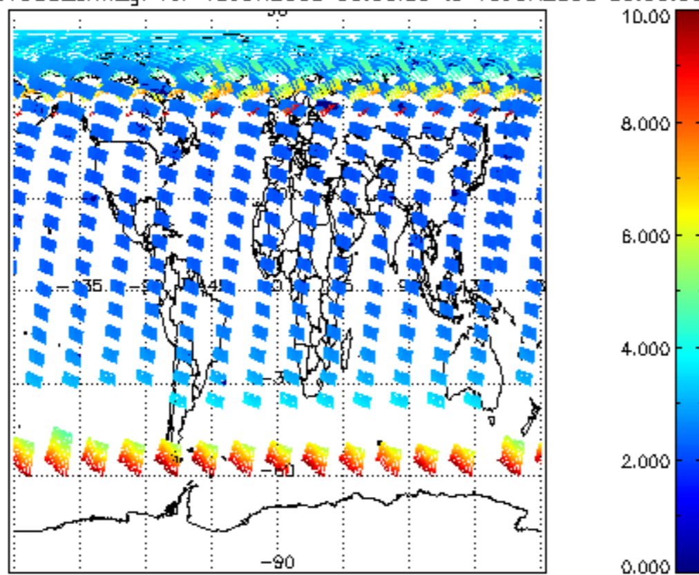
SCIOL2P_NADUV003_amf_gr for 15JUN2008 00:00:00 to 16JUN2008 00:00:00
