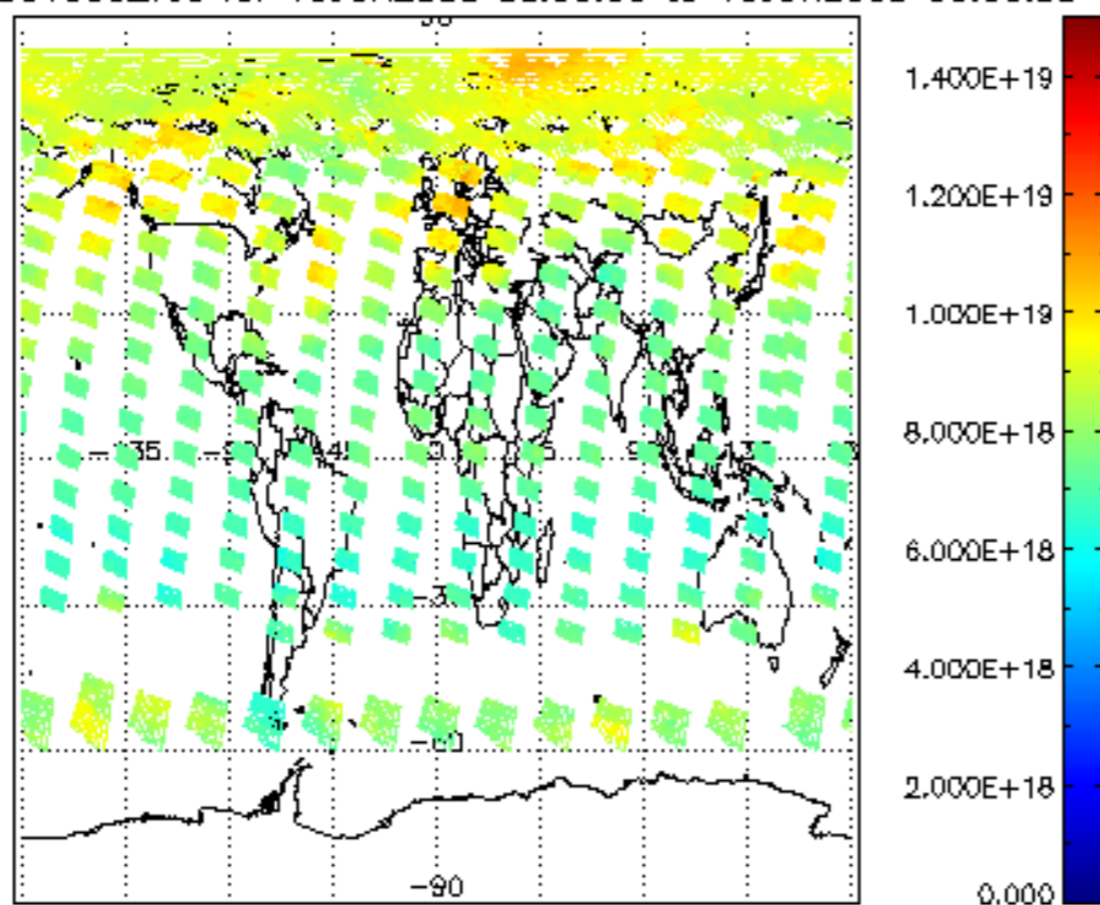
SCIOL2P_NADUV003_vcd for 15JUN2008 00:00:00 to 16JUN2008 00:00:00
