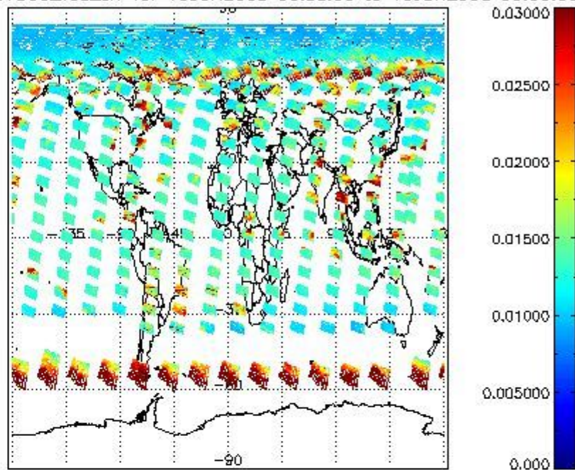
SCIOL2P_NADUV003_vcd_err for 15JUN2008 00:00:00 to 16JUN2008 00:00:00
