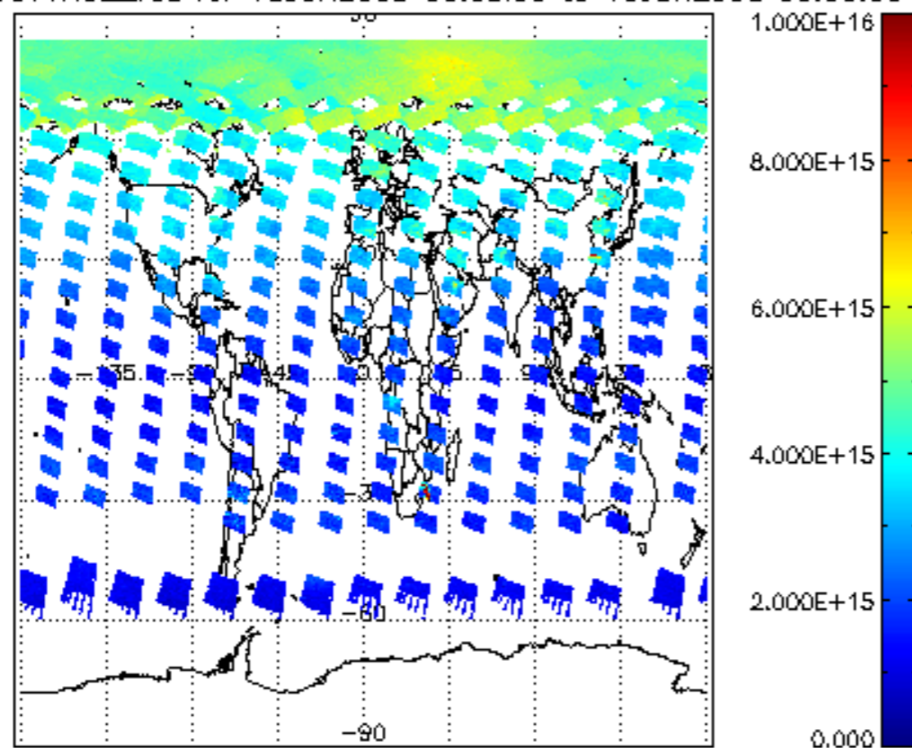
SCIOL2P_NADUV1NO2_vcd for 15JUN2008 00:00:00 to 16JUN2008 00:00:00
