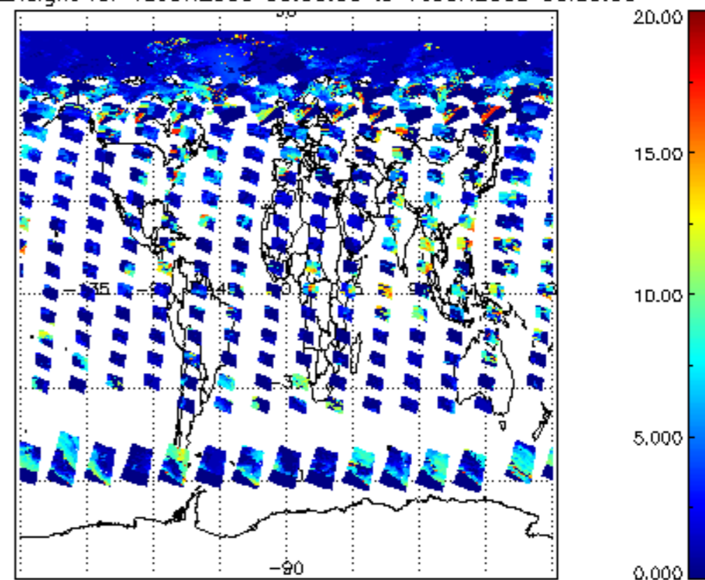
cl_top_height for 15JUN2008 00:00:00 to 16JUN2008 00:00:00
