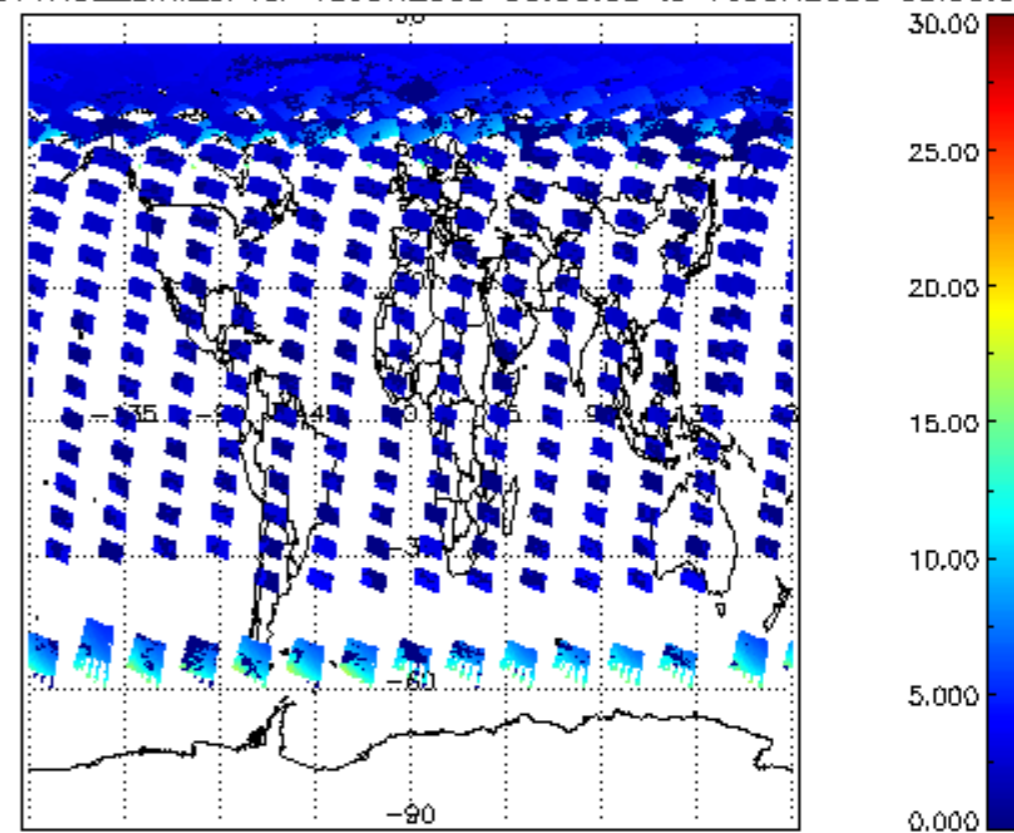
iCIOL2P_NADUV1NO2_amf_cl for 15JUN2008 00:00:00 to 16JUN2008 00:00:00
