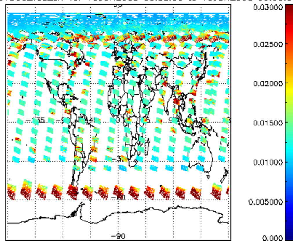
SCIOL2P_NADUV003_vcd_err for 15JUN2008 00:00:00 to 16JUN2008 00:00:00
