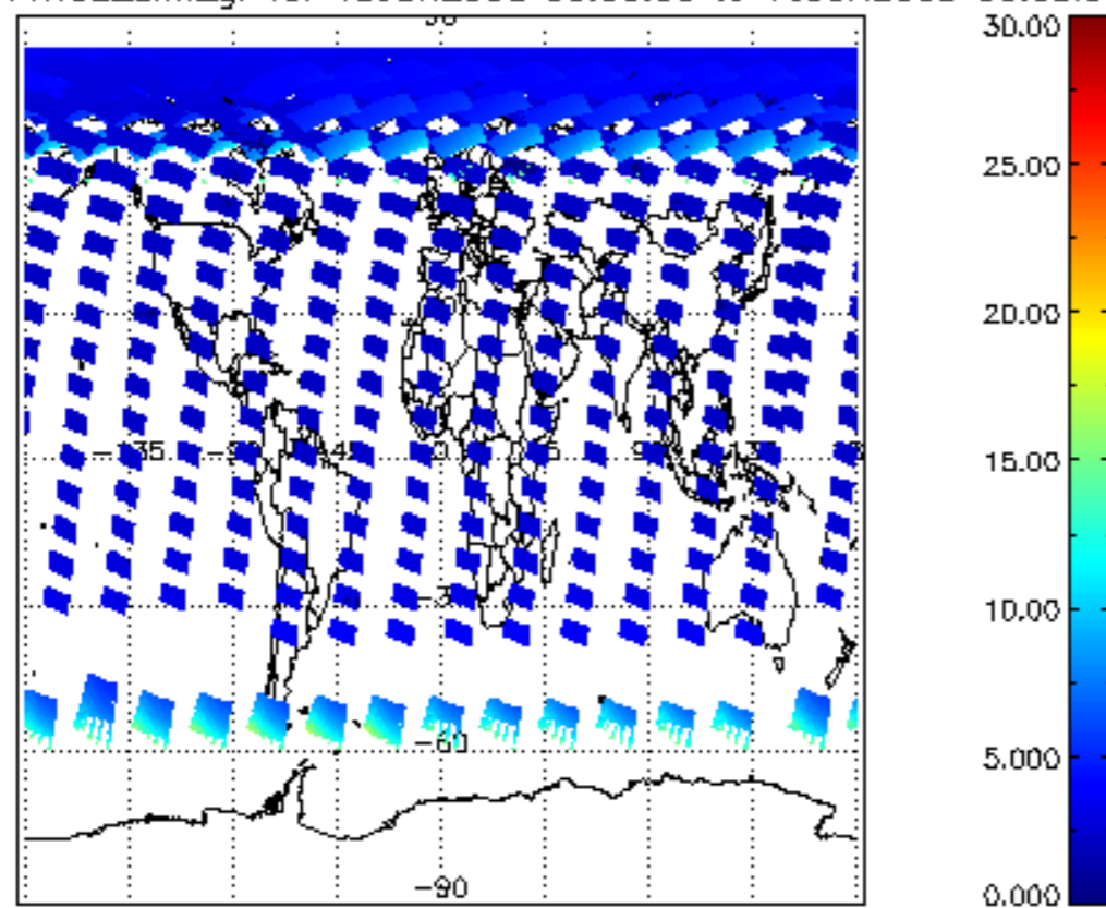
iCIOL2P_NADUV1NO2_amf_gr for 15JUN2008 00:00:00 to 16JUN2008 00:00:00
