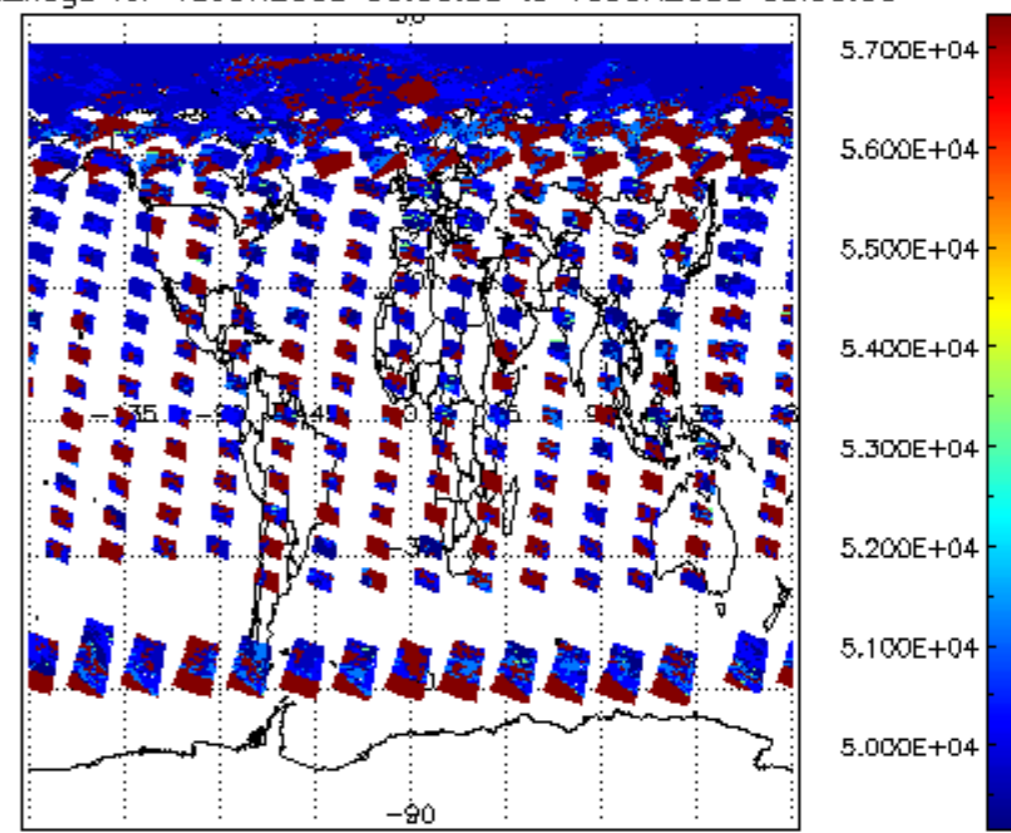
cloud_flags for 15JUN2008 00:00:00 to 16JUN2008 00:00:00
