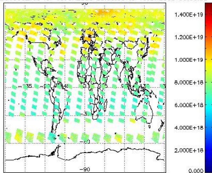
SCIOL2P_NADUV003_vcd for 15JUN2008 00:00:00 to 16JUN2008 00:00:00
