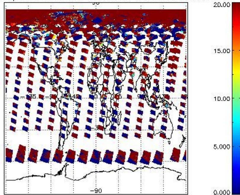
cL_opt_depth for 15JUN2008 00:00:00 to 16JUN2008 00:00:00
