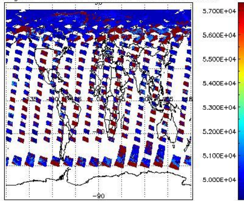
cloud_flags for 14JUN2008 00:00:00 to 15JUN2008 00:00:00
