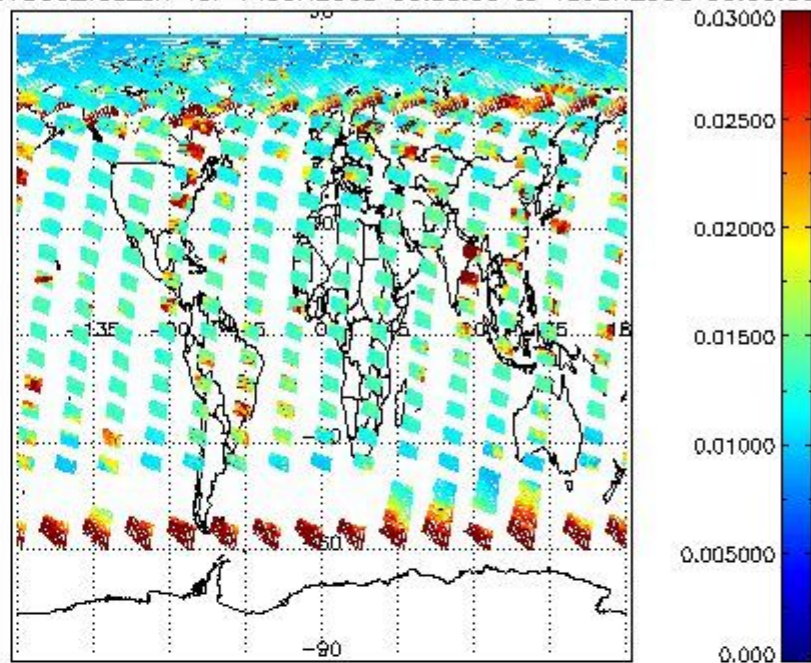
SCIOL2P_NADUV003_vcd_err for 14JUN2008 00:00:00 to 15JUN2008 00:00:00
