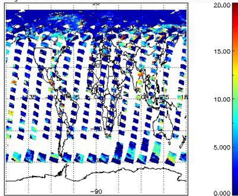
cL_top_height for 14JUN2008 00:00:00 to 15JUN2008 00:00:00
