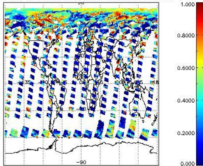
cL_frac for 14JUN2008 00:00:00 to 15JUN2008 00:00:00
