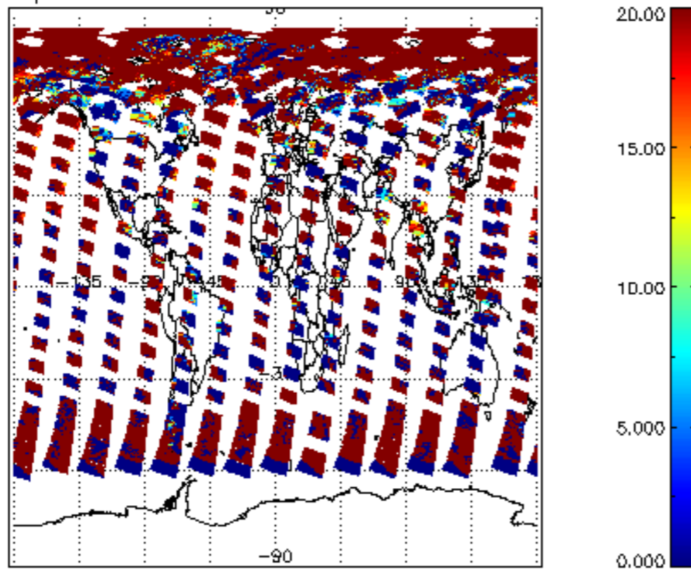
cl_opt_depth for 12JUN2008 00:00:00 to 13JUN2008 00:00:00
