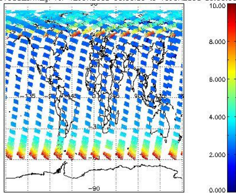
SCIOL2P_NADUV003_amf_gr for 12JUN2008 00:00:00 to 13JUN2008 00:00:00
