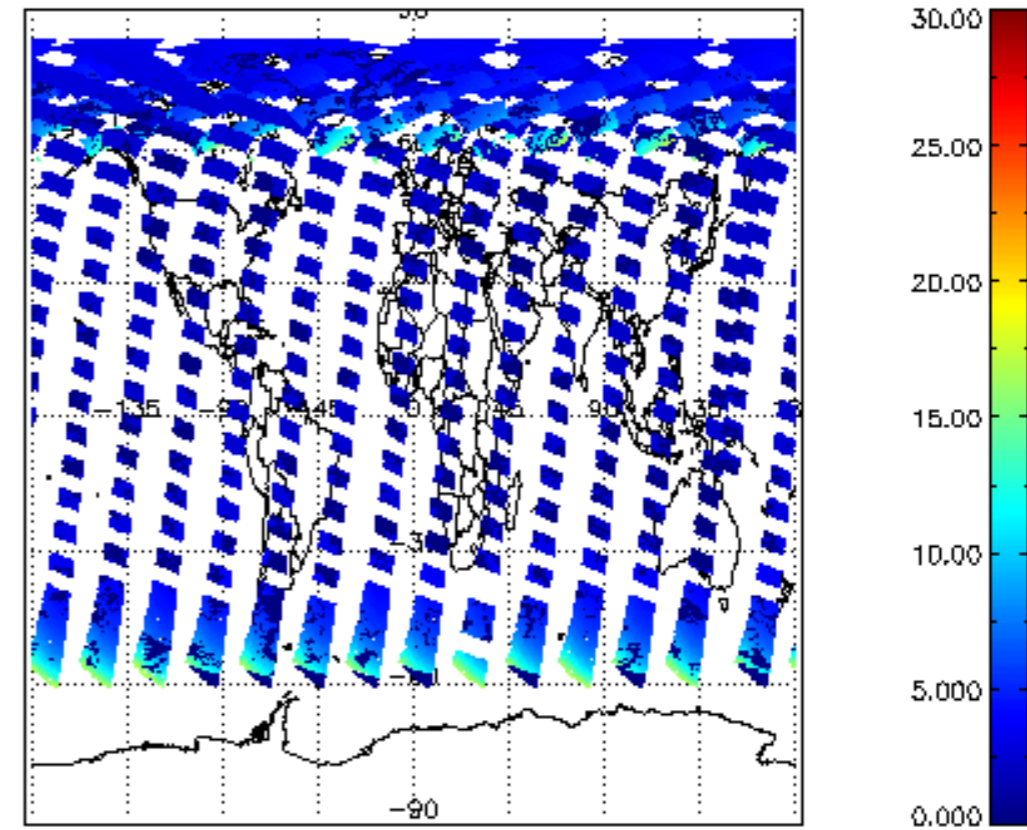
iCIOL2P_NADUV1NO2_amf_cl for 12JUN2008 00:00:00 to 13JUN2008 00:00:00
