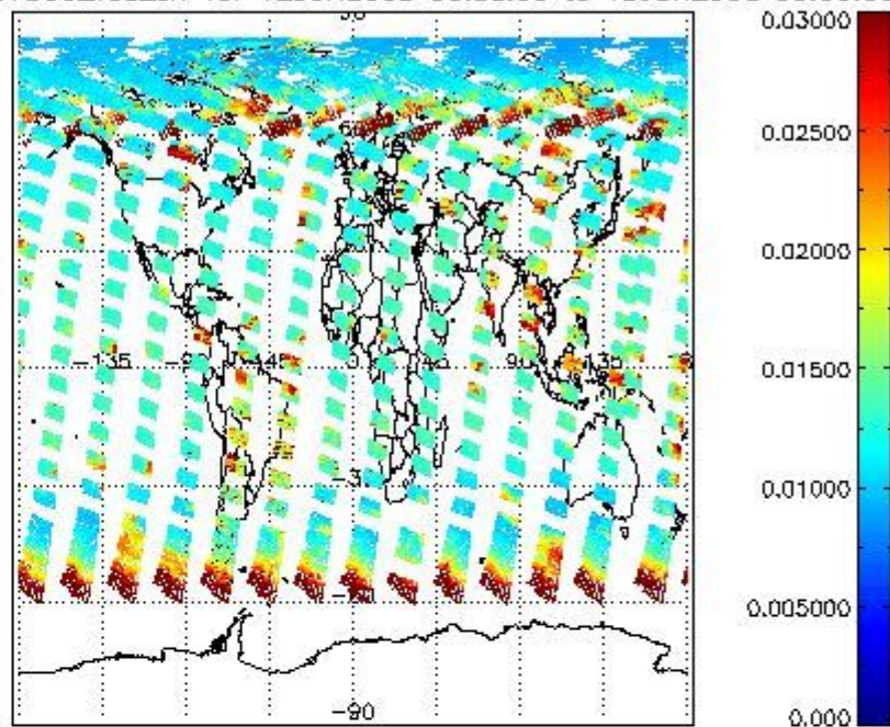
SCIOL2P_NADUV003_vcd_err for 12JUN2008 00:00:00 to 13JUN2008 00:00:00
