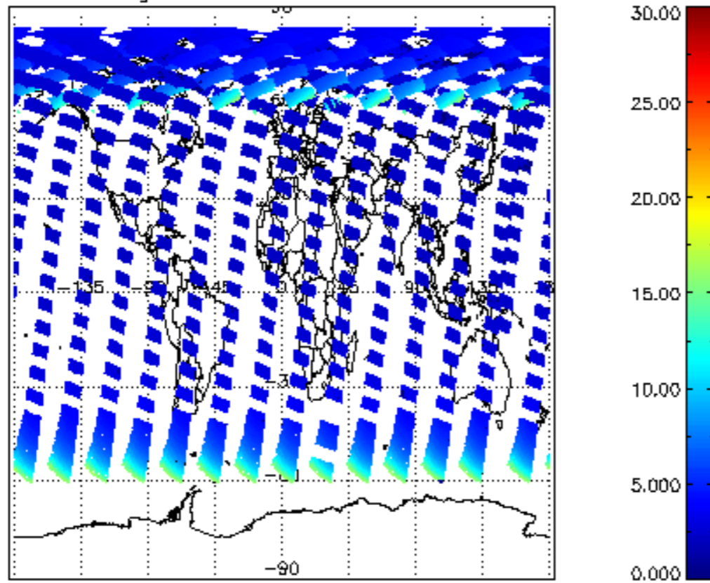
iCIOL2P_NADUV1NO2_amf_gr for 12JUN2008 00:00:00 to 13JUN2008 00:00:00
