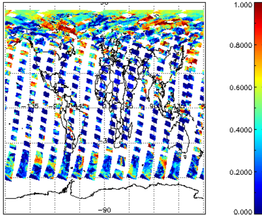
cl_frac for 12JUN2008 00:00:00 to 13JUN2008 00:00:00
