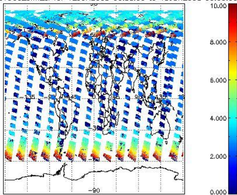
SCIOL2P_NADUV003_amf_cl for 12JUN2008 00:00:00 to 13JUN2008 00:00:00
