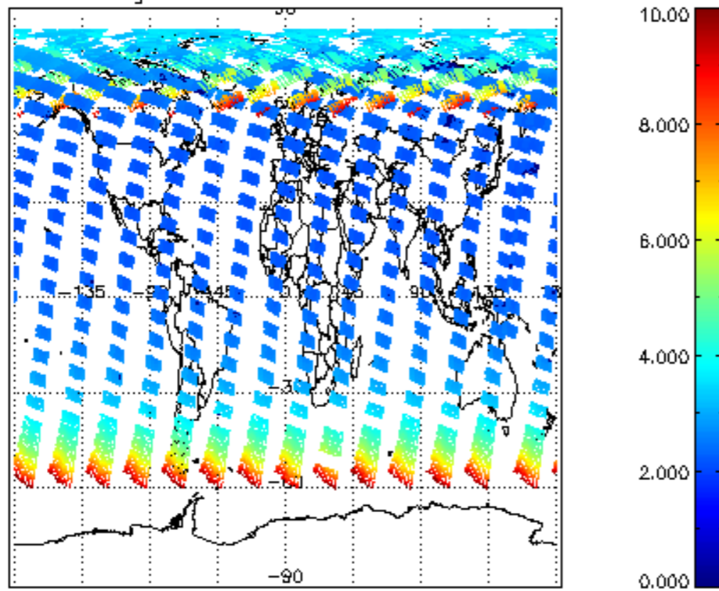
SCIOL2P_NADUV003_amf_gr for 12JUN2008 00:00:00 to 13JUN2008 00:00:00
