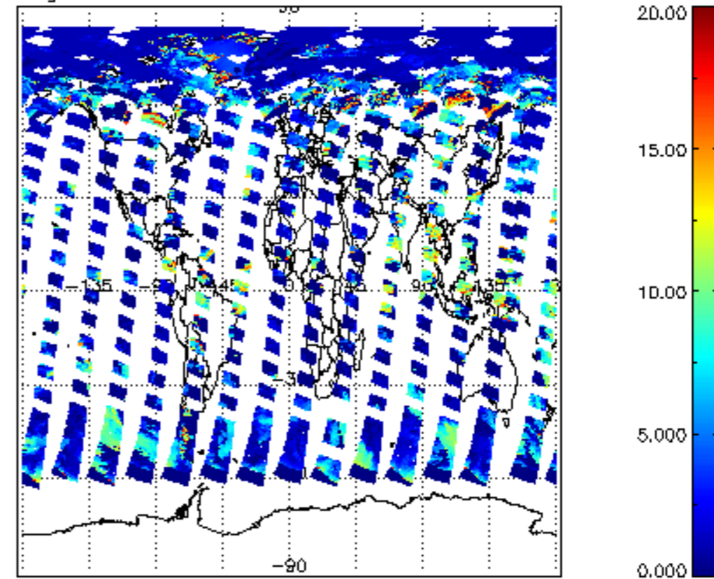
cl_top_height for 12JUN2008 00:00:00 to 13JUN2008 00:00:00
