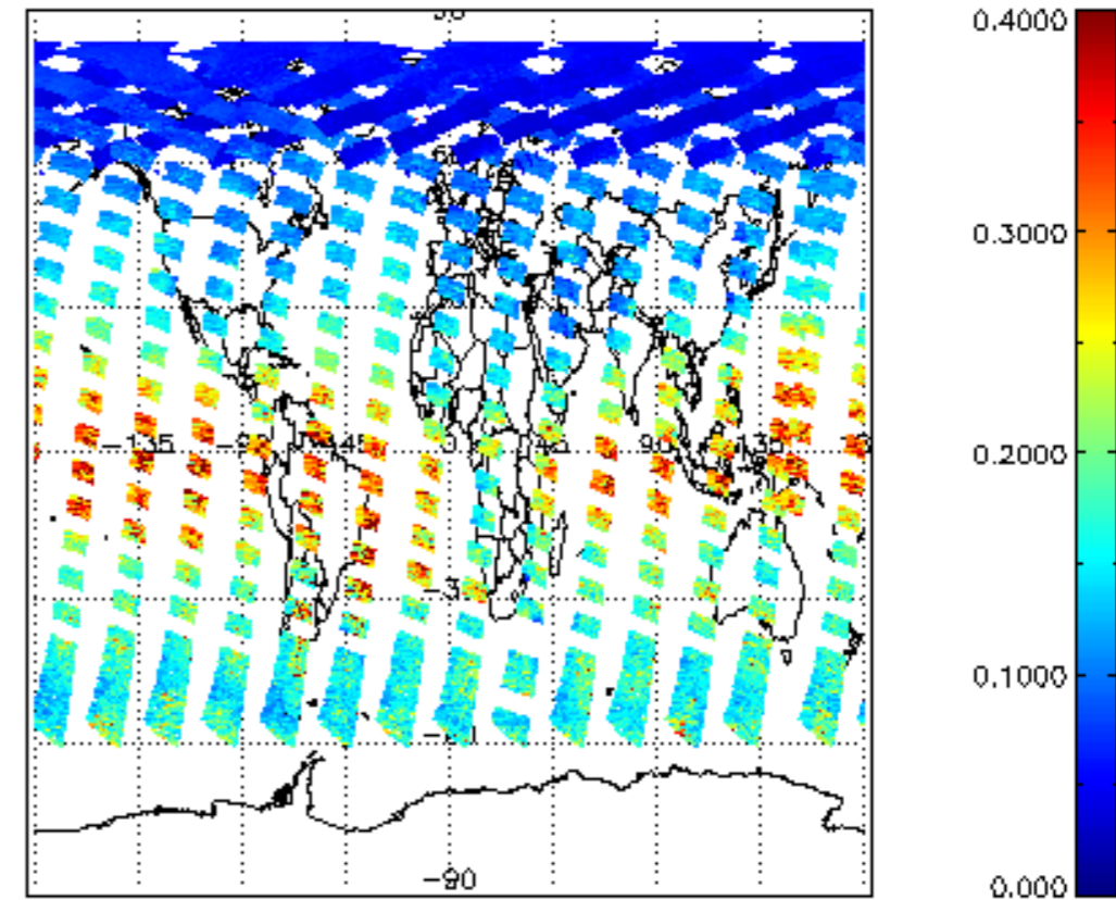
iCIOL2P_NADUV1NO2_vcd_err for 12JUN2008 00:00:00 to 13JUN2008 00:00:00
