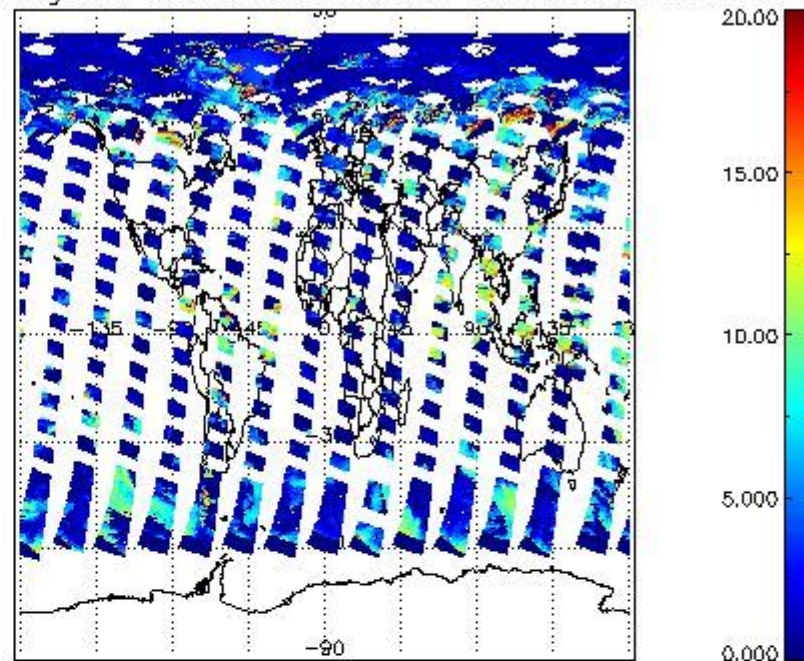
cL_top_height for 12JUN2008 00:00:00 to 13JUN2008 00:00:00
