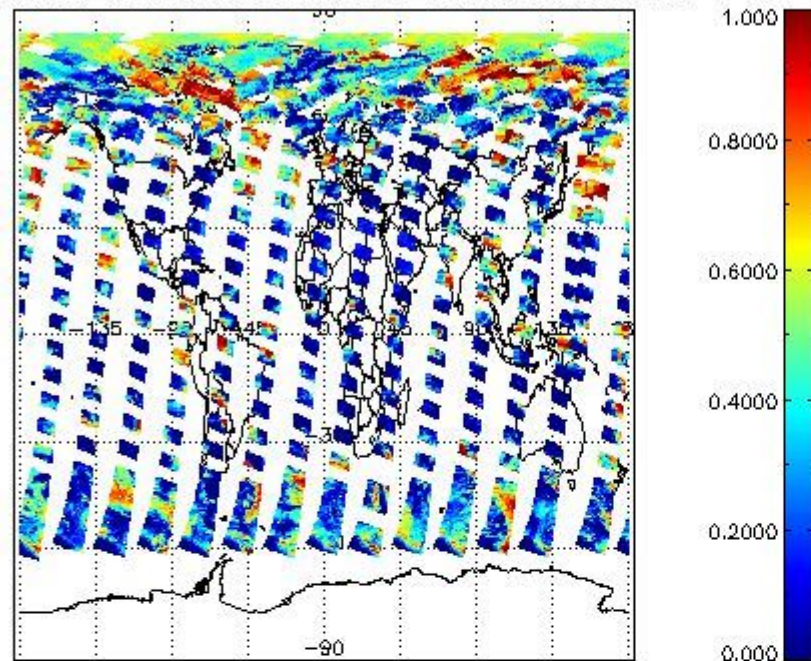
cL_frac for 12JUN2008 00:00:00 to 13JUN2008 00:00:00
