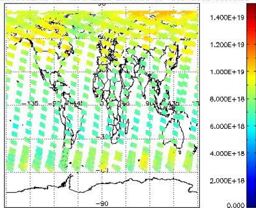
SCIOL2P_NADUV003_vcd for 12JUN2008 00:00:00 to 13JUN2008 00:00:00
