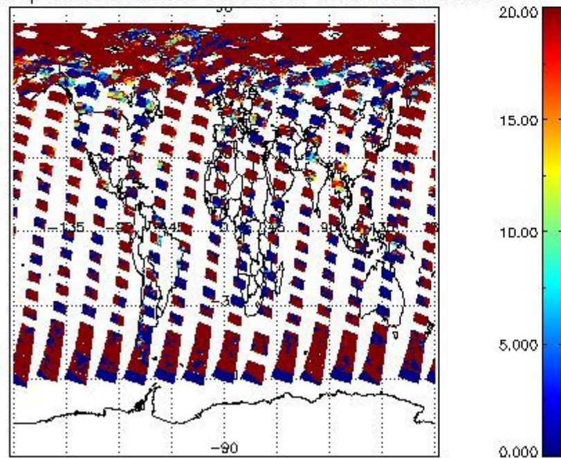
cL_opt_depth for 12JUN2008 00:00:00 to 13JUN2008 00:00:00
