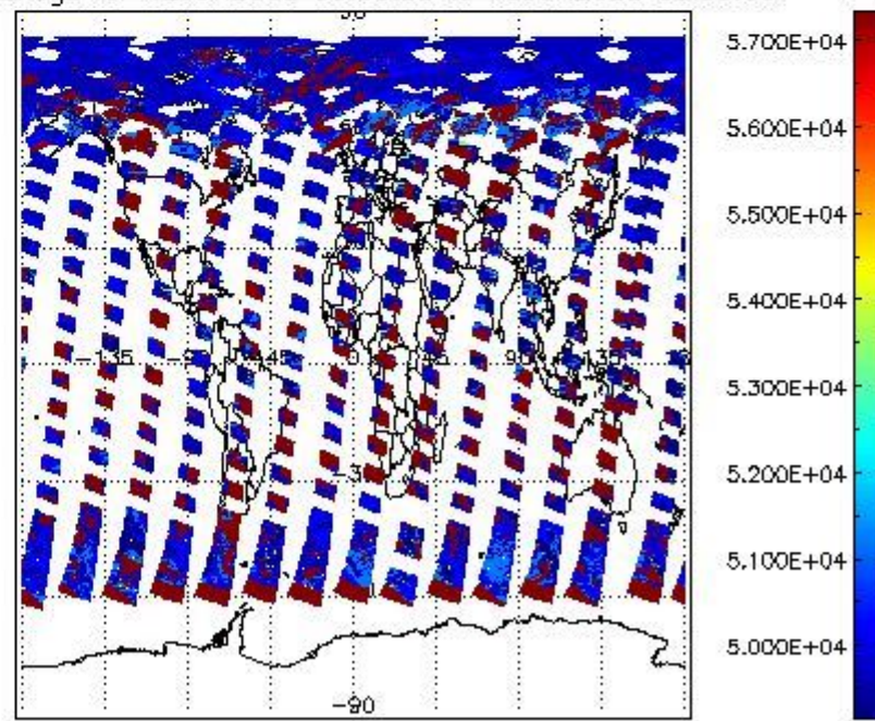
cloud_flags for 12JUN2008 00:00:00 to 13JUN2008 00:00:00
