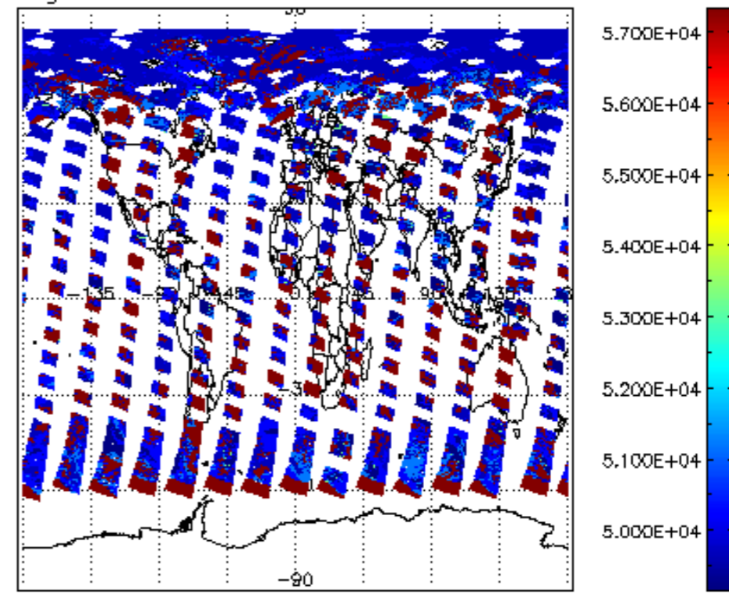
cloud_flags for 12JUN2008 00:00:00 to 13JUN2008 00:00:00
