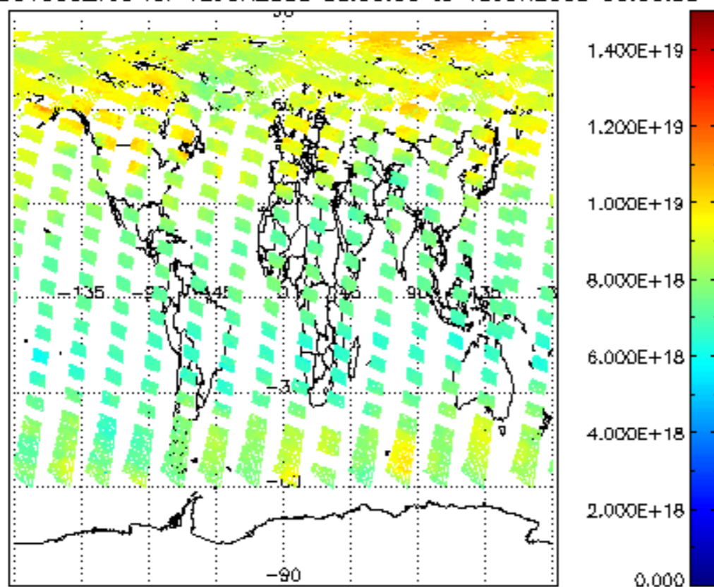
SCIOL2P_NADUV003_vcd for 12JUN2008 00:00:00 to 13JUN2008 00:00:00
