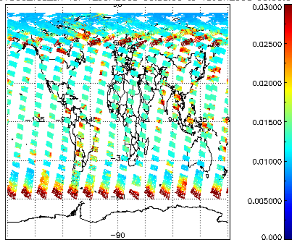
SCIOL2P_NADUV003_vcd_err for 12JUN2008 00:00:00 to 13JUN2008 00:00:00
