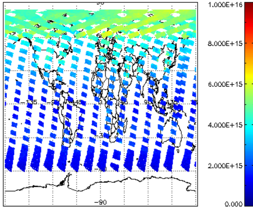
SCIOL2P_NADUV1NO2_vcd for 12JUN2008 00:00:00 to 13JUN2008 00:00:00
