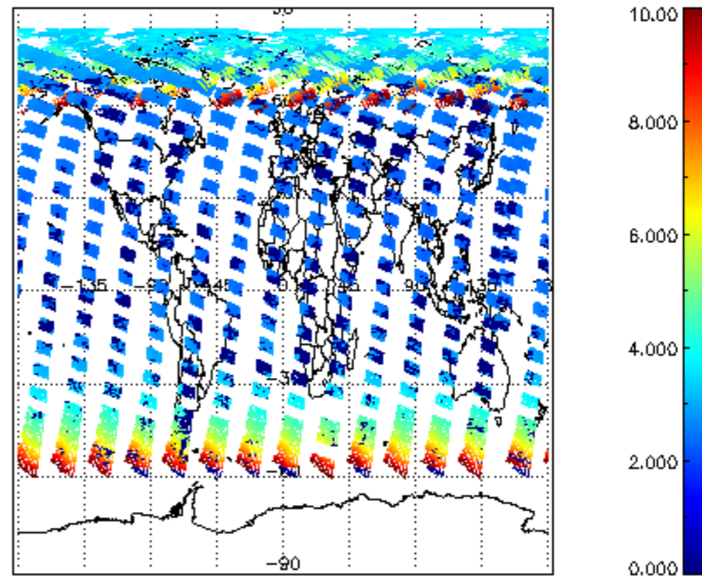
SCIOL2P_NADUV003_amf_cl for 12JUN2008 00:00:00 to 13JUN2008 00:00:00
