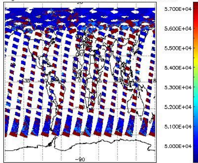
cloud_flags for 11JUN2008 00:00:00 to 12JUN2008 00:00:00
