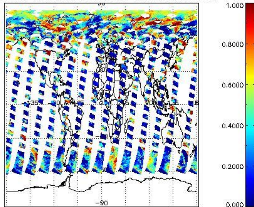
cL_frac for 11JUN2008 00:00:00 to 12JUN2008 00:00:00
