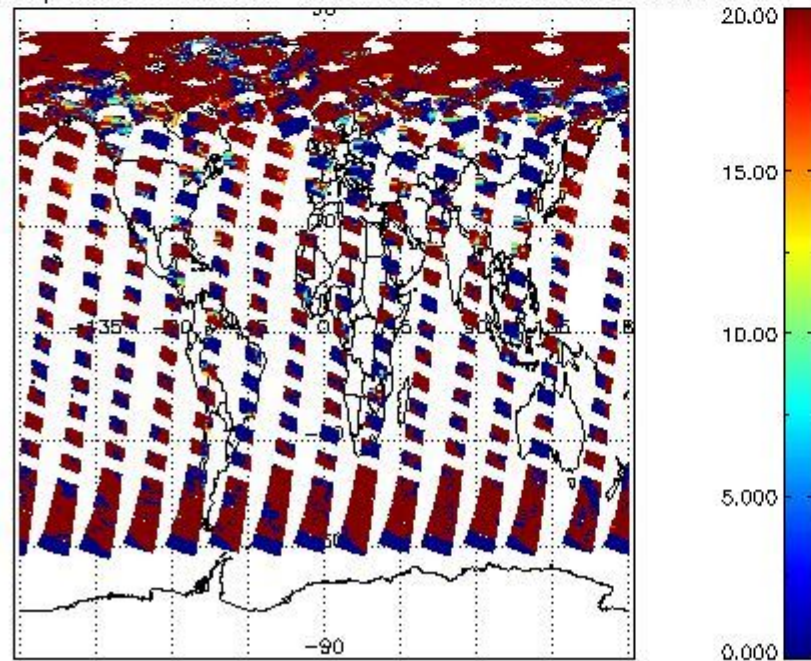
cL_opt_depth for 11JUN2008 00:00:00 to 12JUN2008 00:00:00
