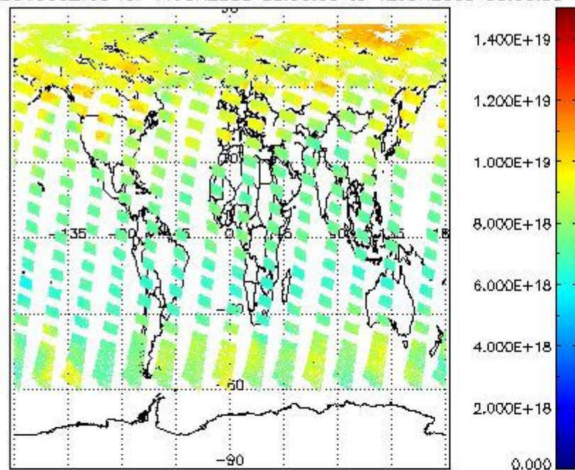
SCIOL2P_NADUV003_vcd for 11JUN2008 00:00:00 to 12JUN2008 00:00:00
