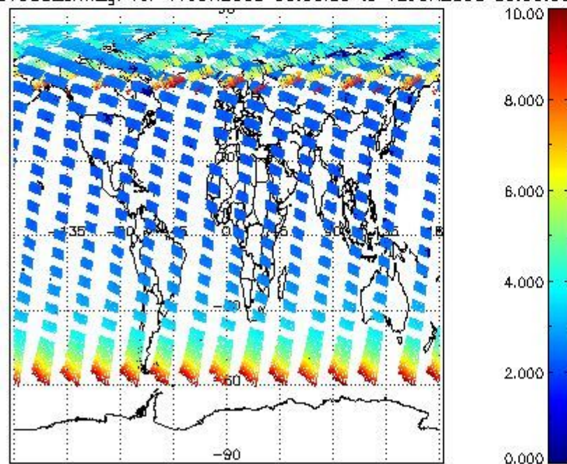
SCIOL2P_NADUV003_amf_gr for 11JUN2008 00:00:00 to 12JUN2008 00:00:00
