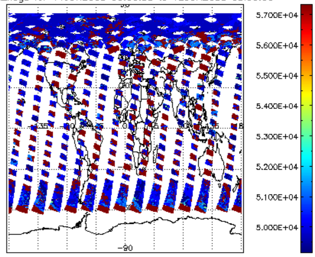
cloud_flags for 11JUN2008 00:00:00 to 12JUN2008 00:00:00
