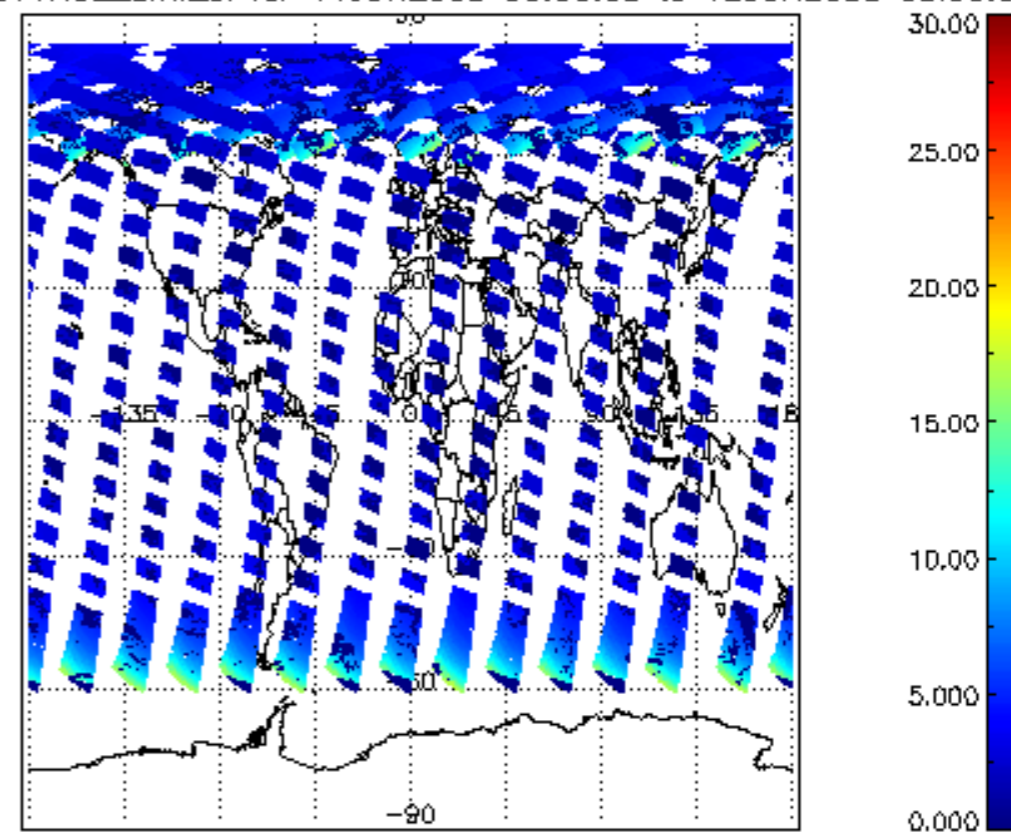
iCIOL2P_NADUV1NO2_amf_cl for 11JUN2008 00:00:00 to 12JUN2008 00:00:00
