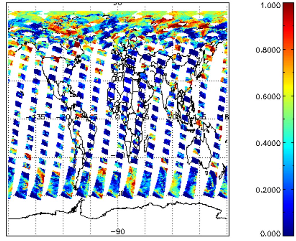
cl_frac for 11JUN2008 00:00:00 to 12JUN2008 00:00:00
