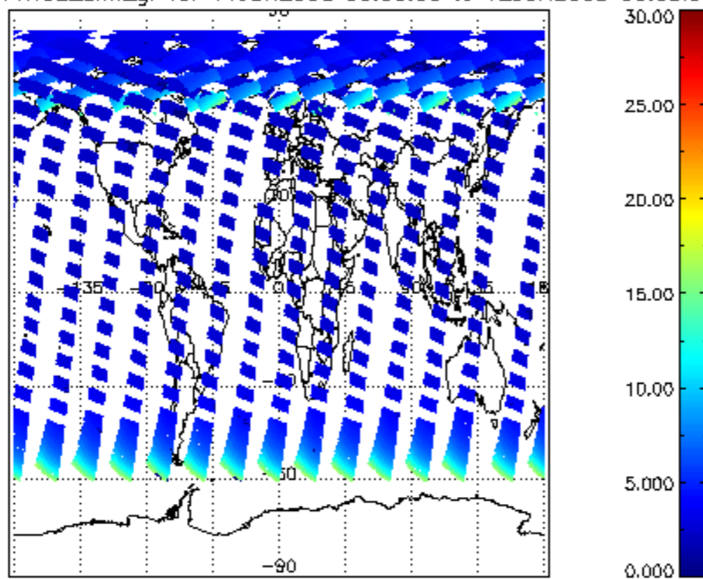
iCIOL2P_NADUV1NO2_amf_gr for 11JUN2008 00:00:00 to 12JUN2008 00:00:00
