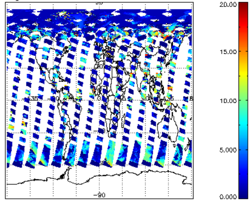
cl_top_height for 11JUN2008 00:00:00 to 12JUN2008 00:00:00
