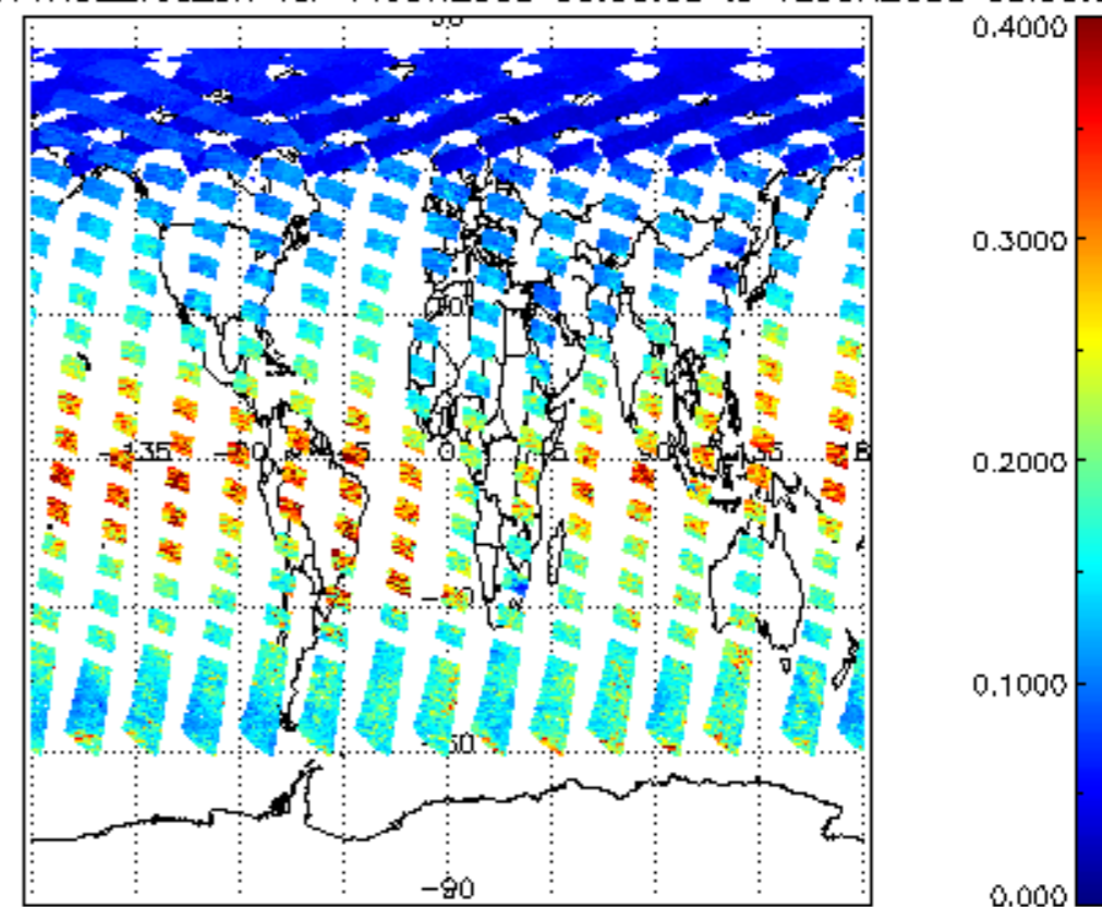
iCIOL2P_NADUV1NO2_vcd_err for 11JUN2008 00:00:00 to 12JUN2008 00:00:00
