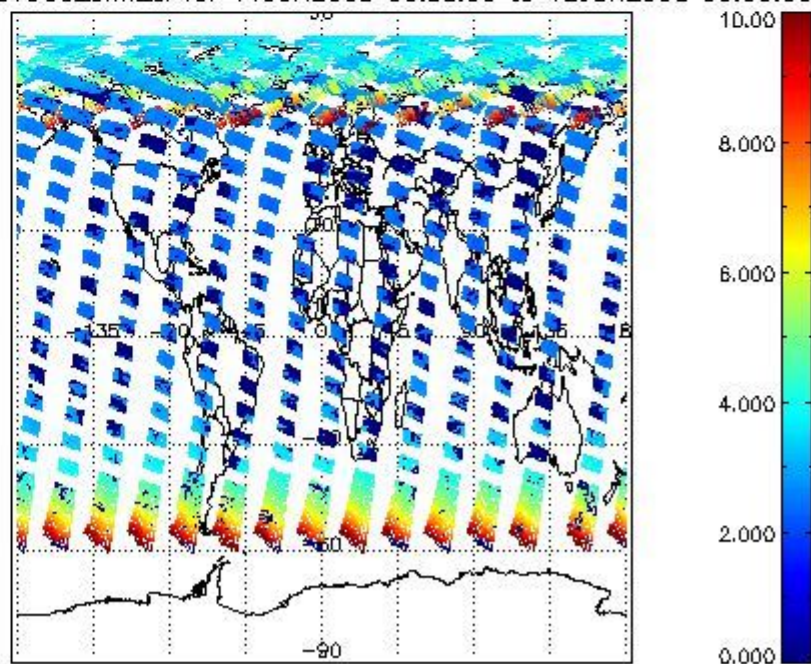
SCIOL2P_NADUV003_amf_cl for 11JUN2008 00:00:00 to 12JUN2008 00:00:00
