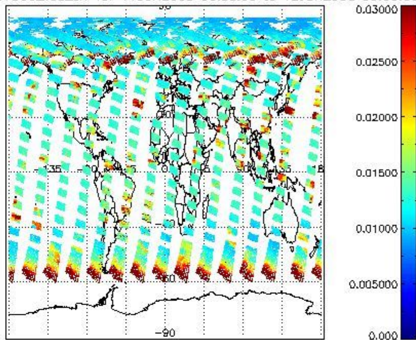
SCIOL2P_NADUV003_vcd_err for 11JUN2008 00:00:00 to 12JUN2008 00:00:00
