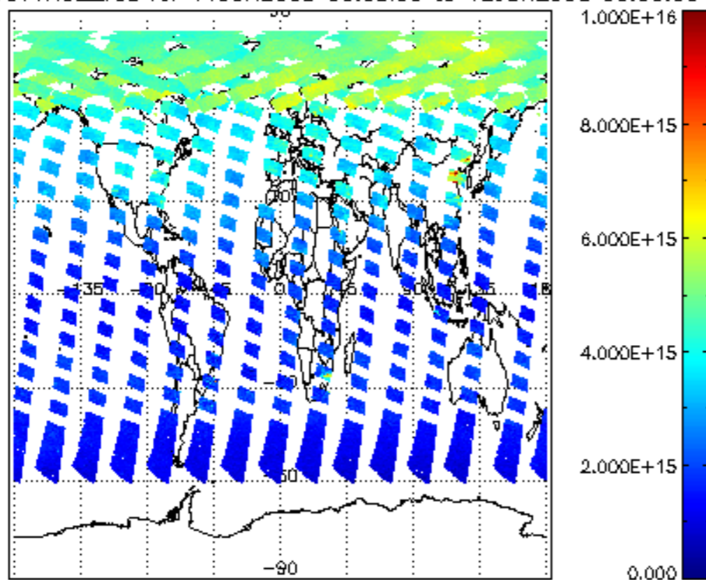
SCIOL2P_NADUV1NO2_vcd for 11JUN2008 00:00:00 to 12JUN2008 00:00:00
