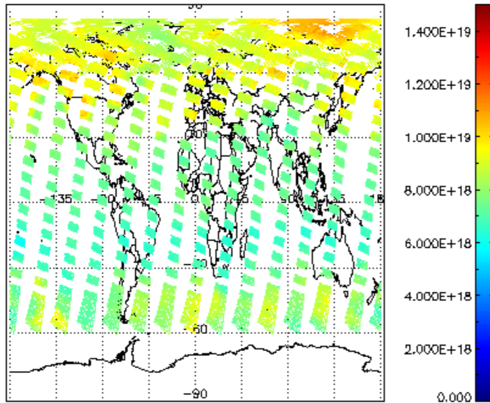
SCIOL2P_NADUV003_vcd for 11JUN2008 00:00:00 to 12JUN2008 00:00:00
