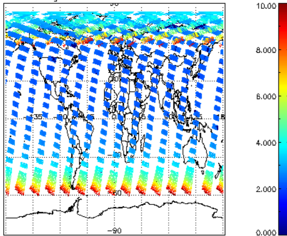
SCIOL2P_NADUV003_amf_gr for 11JUN2008 00:00:00 to 12JUN2008 00:00:00
