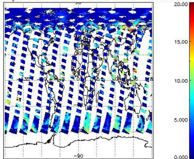
cL_top_height for 11JUN2008 00:00:00 to 12JUN2008 00:00:00
