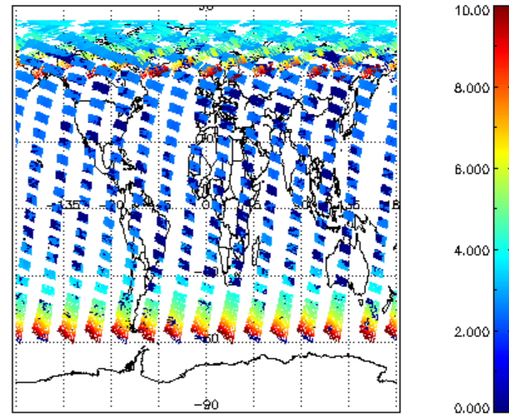
SCIOL2P_NADUV003_amf_cl for 11JUN2008 00:00:00 to 12JUN2008 00:00:00
