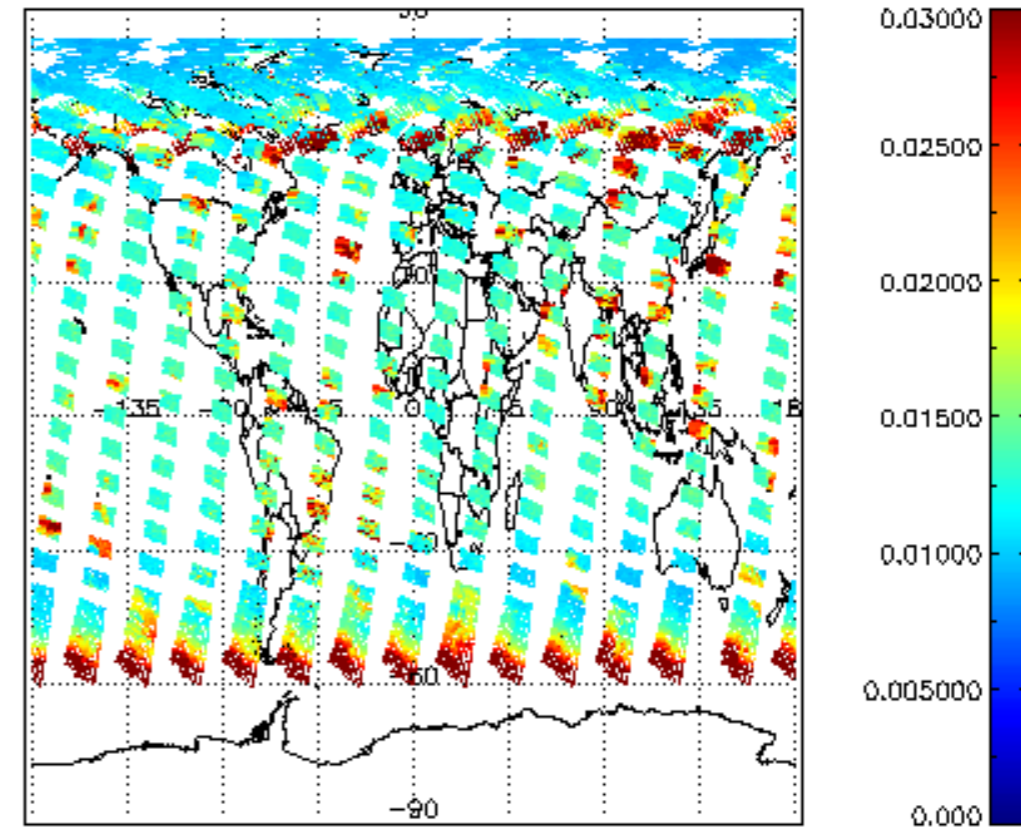
SCIOL2P_NADUV003_vcd_err for 11JUN2008 00:00:00 to 12JUN2008 00:00:00
