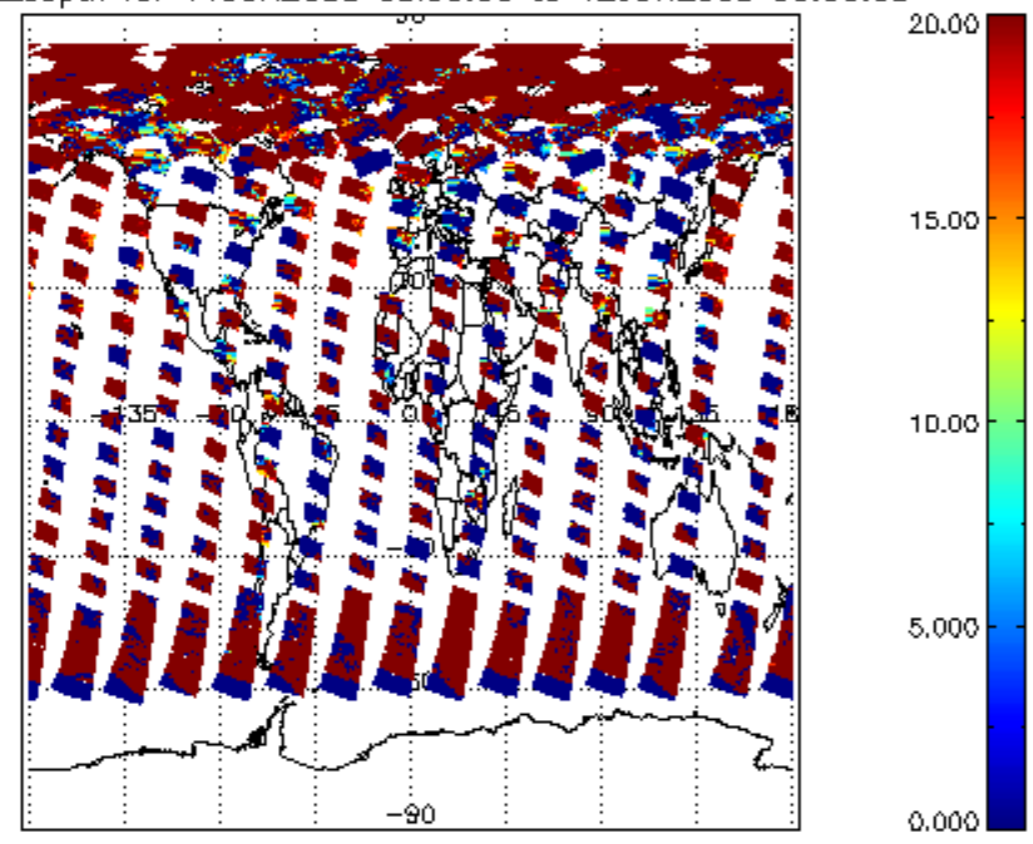
cl_opt_depth for 11JUN2008 00:00:00 to 12JUN2008 00:00:00
