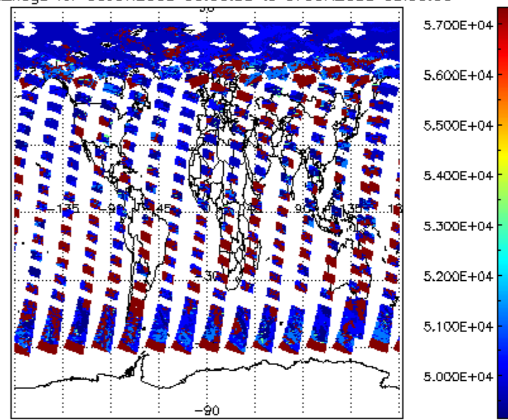
cloud_flags for 06JUN2008 00:00:00 to 07JUN2008 00:00:00
