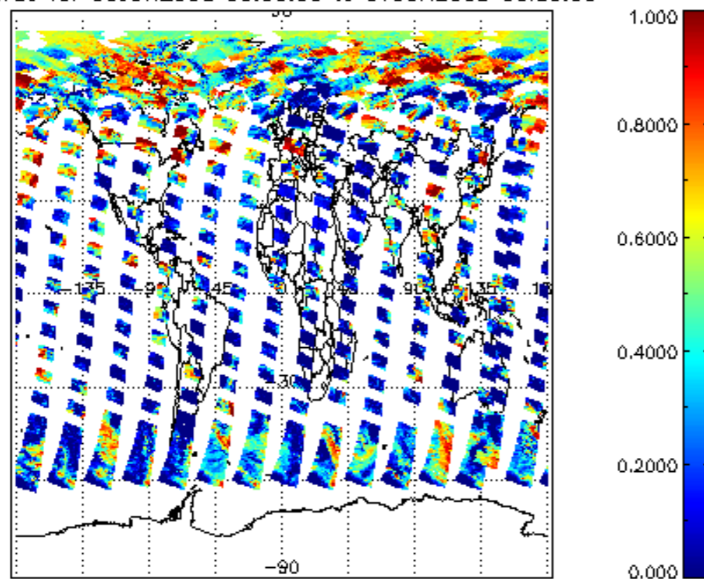
cl_frac for 06JUN2008 00:00:00 to 07JUN2008 00:00:00
