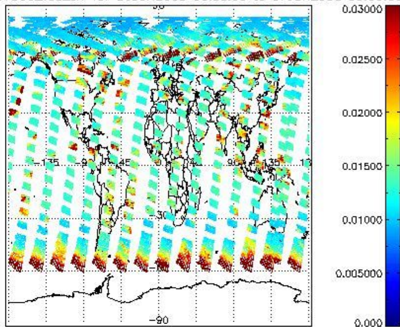
SCIOL2P_NADUV003_vcd_err for 06JUN2008 00:00:00 to 07JUN2008 00:00:00
