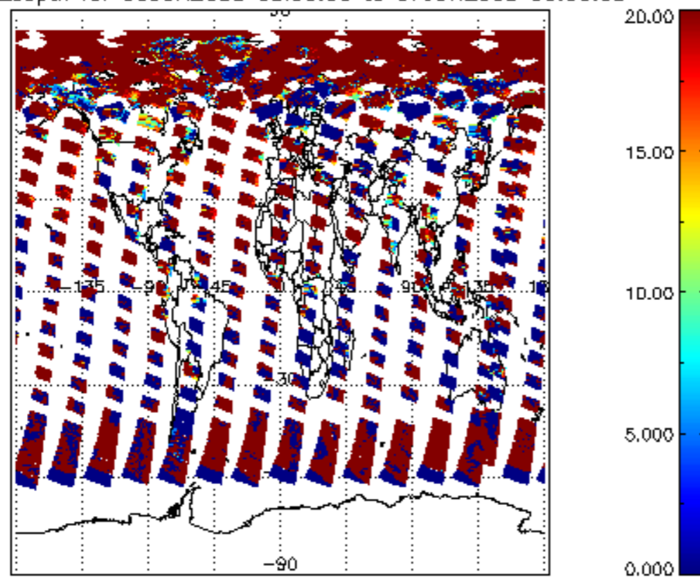
cl_opt_depth for 06JUN2008 00:00:00 to 07JUN2008 00:00:00
