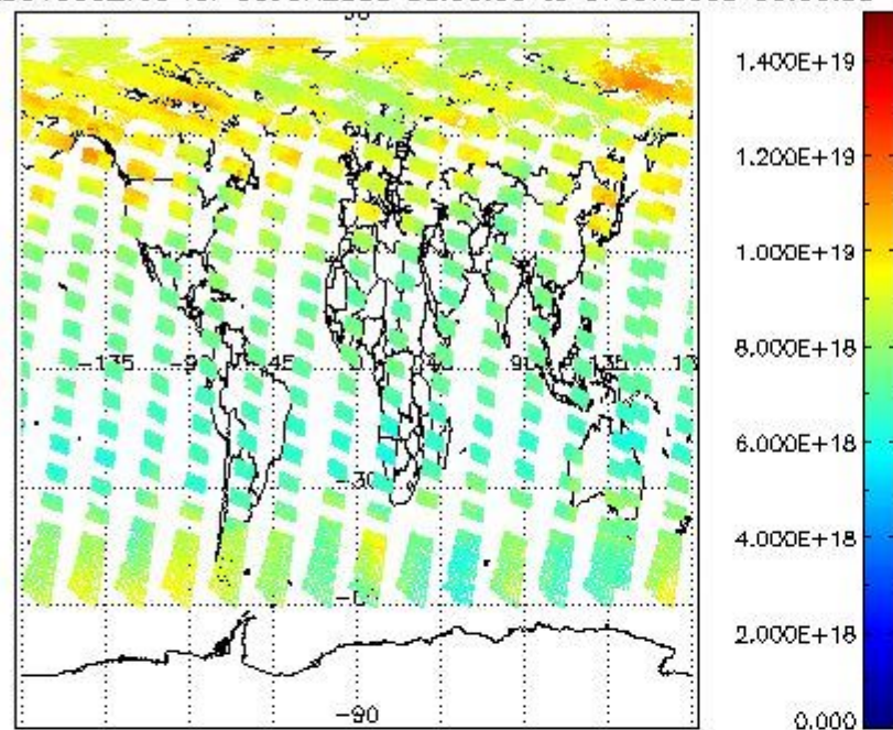
SCIOL2P_NADUV003_vcd for 06JUN2008 00:00:00 to 07JUN2008 00:00:00
