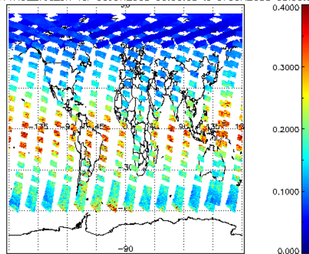
iCIOL2P_NADUV1NO2_vcd_err for 06JUN2008 00:00:00 to 07JUN2008 00:00:00
