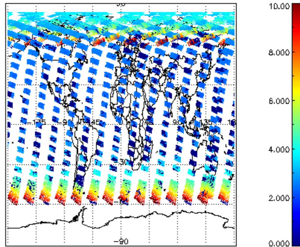
SCIOL2P_NADUV003_amf_cl for 06JUN2008 00:00:00 to 07JUN2008 00:00:00
