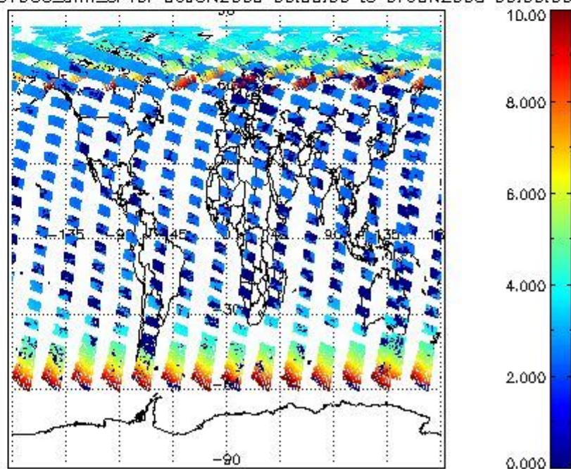
SCIOL2P_NADUV003_amf_cl for 06JUN2008 00:00:00 to 07JUN2008 00:00:00
