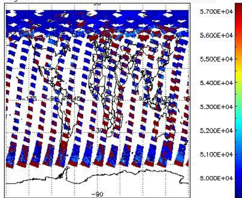
cloud_flags for 06JUN2008 00:00:00 to 07JUN2008 00:00:00
