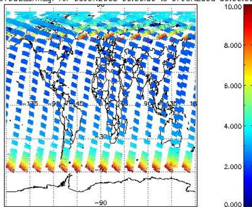
SCIOL2P_NADUV003_amf_gr for 06JUN2008 00:00:00 to 07JUN2008 00:00:00
