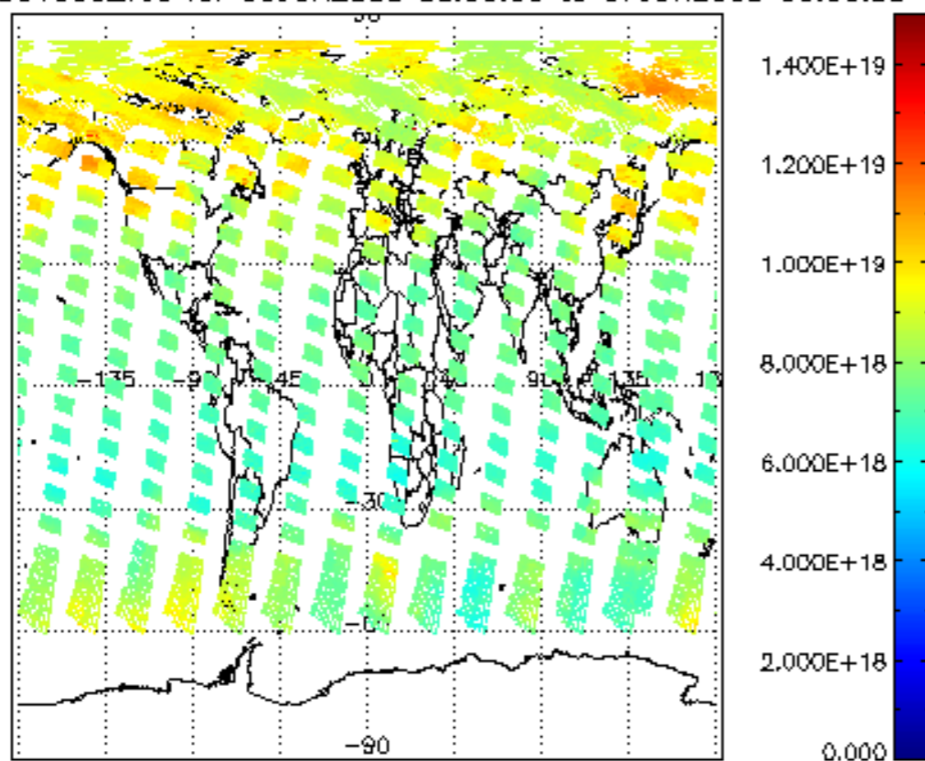
SCIOL2P_NADUV003_vcd for 06JUN2008 00:00:00 to 07JUN2008 00:00:00
