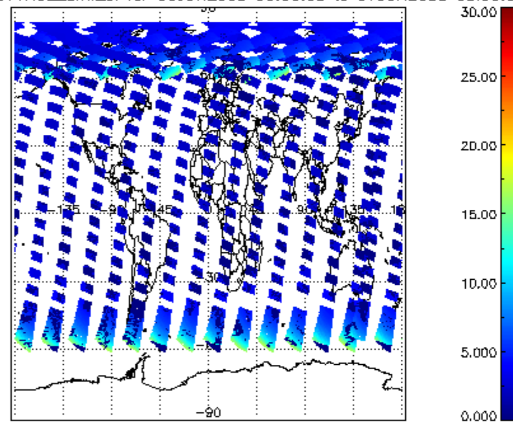
iCIOL2P_NADUV1NO2_amf_cl for 06JUN2008 00:00:00 to 07JUN2008 00:00:00
