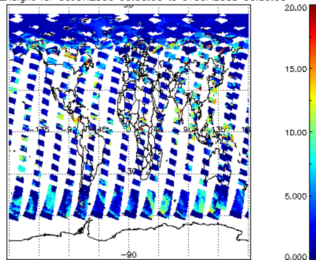
cl_top_height for 06JUN2008 00:00:00 to 07JUN2008 00:00:00
