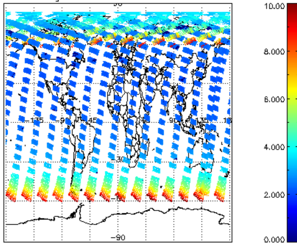
SCIOL2P_NADUV003_amf_gr for 06JUN2008 00:00:00 to 07JUN2008 00:00:00
