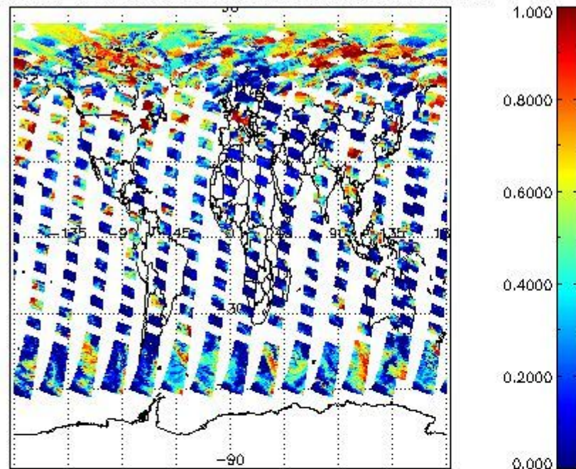
cL_frac for 06JUN2008 00:00:00 to 07JUN2008 00:00:00
