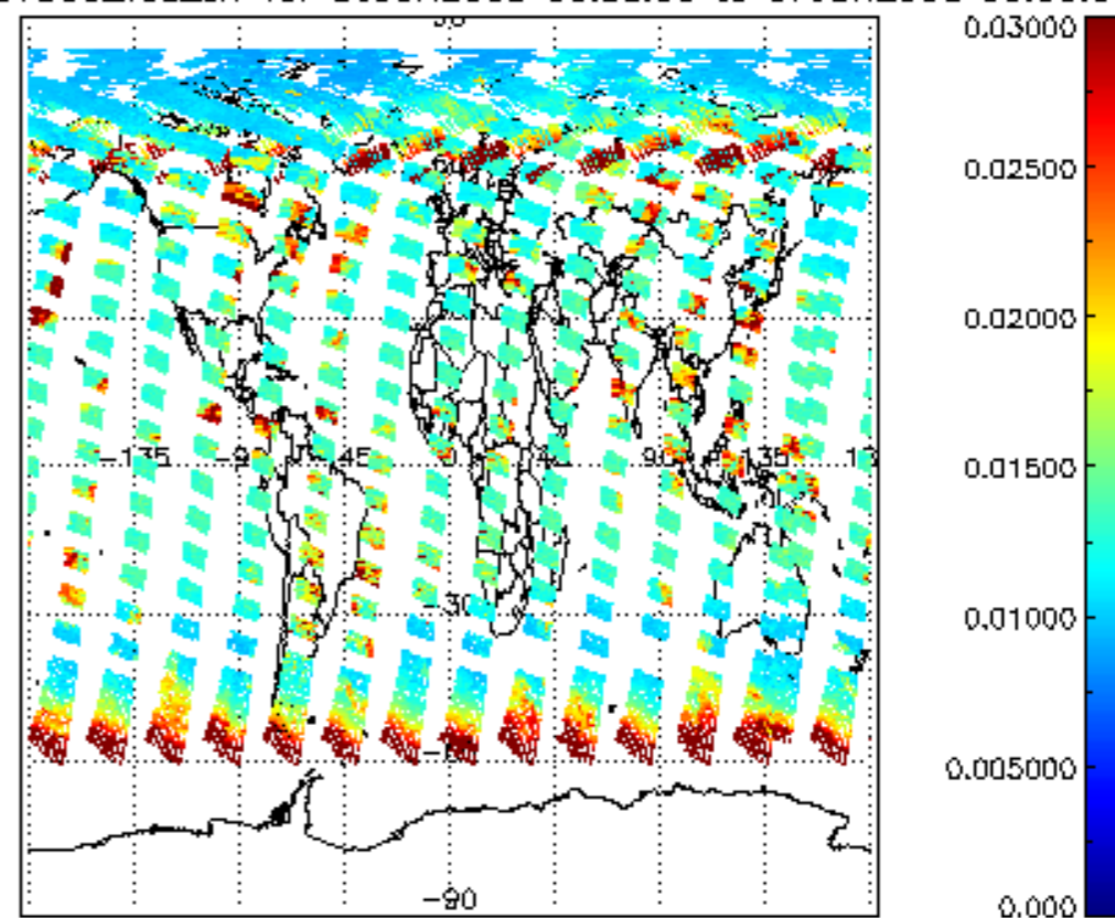
SCIOL2P_NADUV003_vcd_err for 06JUN2008 00:00:00 to 07JUN2008 00:00:00
