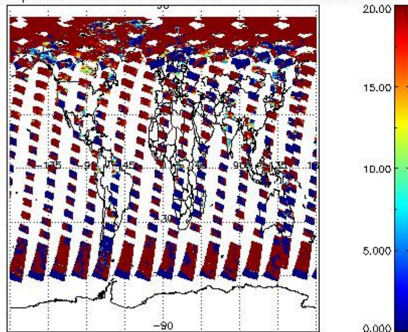
cL_opt_depth for 06JUN2008 00:00:00 to 07JUN2008 00:00:00
