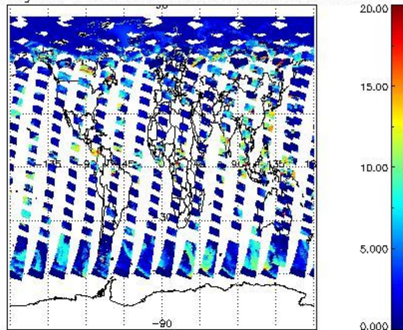
cL_top_height for 06JUN2008 00:00:00 to 07JUN2008 00:00:00
