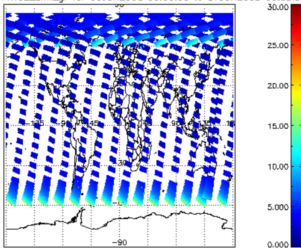
iCIOL2P_NADUV1NO2_amf_gr for 06JUN2008 00:00:00 to 07JUN2008 00:00:00
