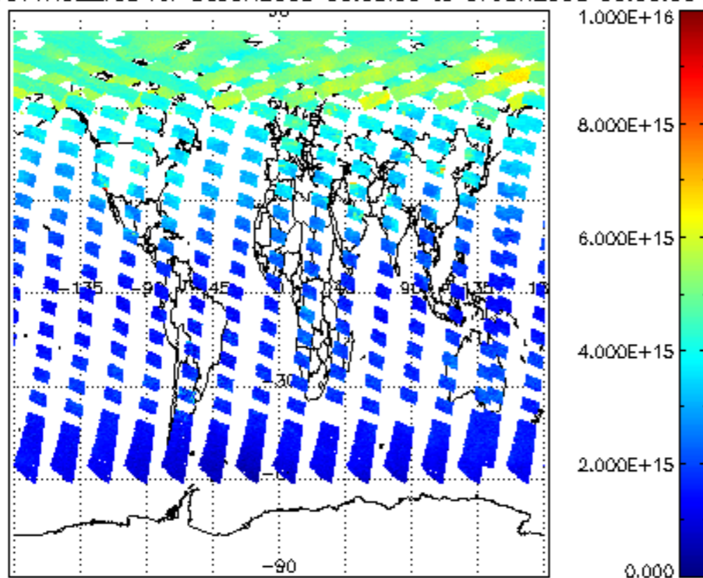
SCIOL2P_NADUV1NO2_vcd for 06JUN2008 00:00:00 to 07JUN2008 00:00:00
