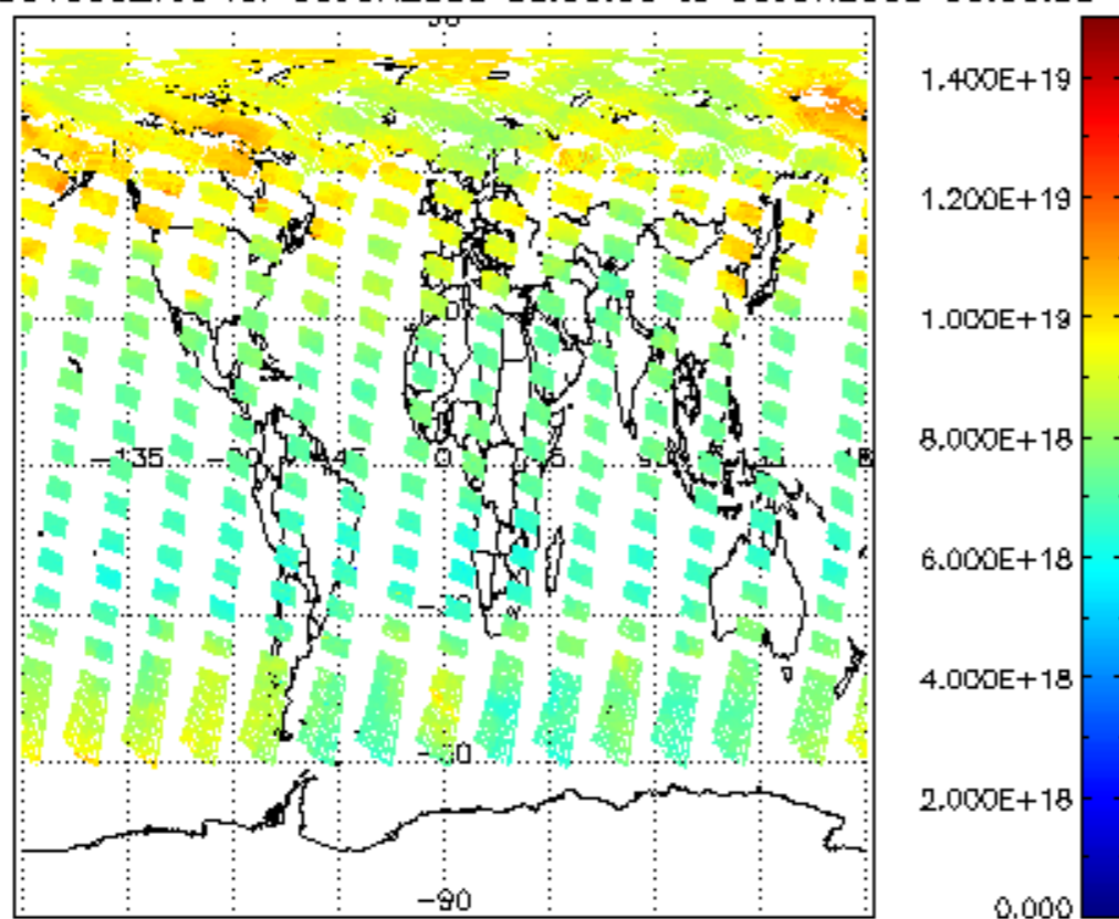
SCIOL2P_NADUV003_vcd for 05JUN2008 00:00:00 to 06JUN2008 00:00:00
