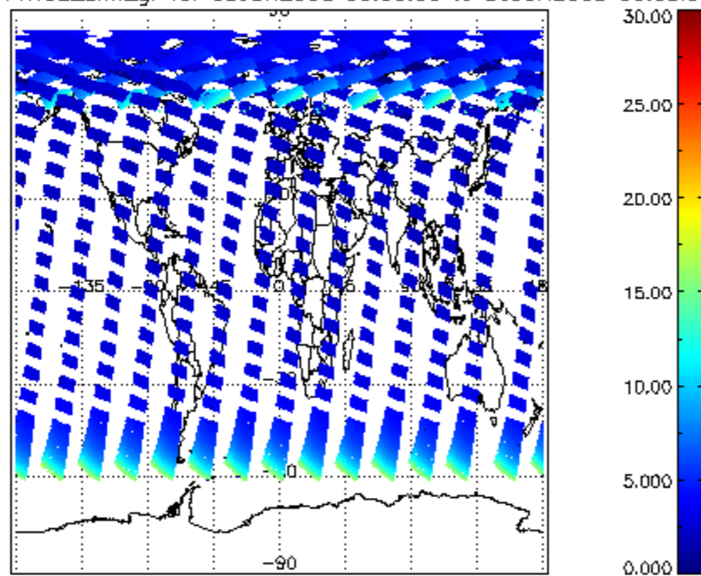
iCIOL2P_NADUV1NO2_amf_gr for 05JUN2008 00:00:00 to 06JUN2008 00:00:00
