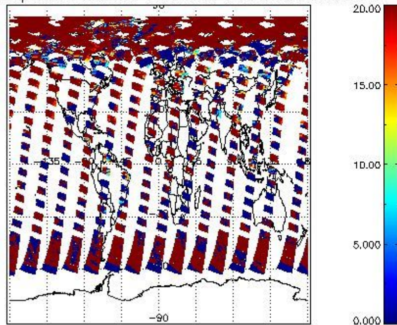
cL_opt_depth for 05JUN2008 00:00:00 to 06JUN2008 00:00:00
