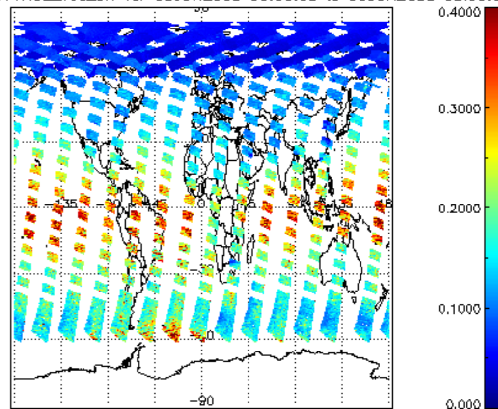
iCIOL2P_NADUV1NO2_vcd_err for 05JUN2008 00:00:00 to 06JUN2008 00:00:00
