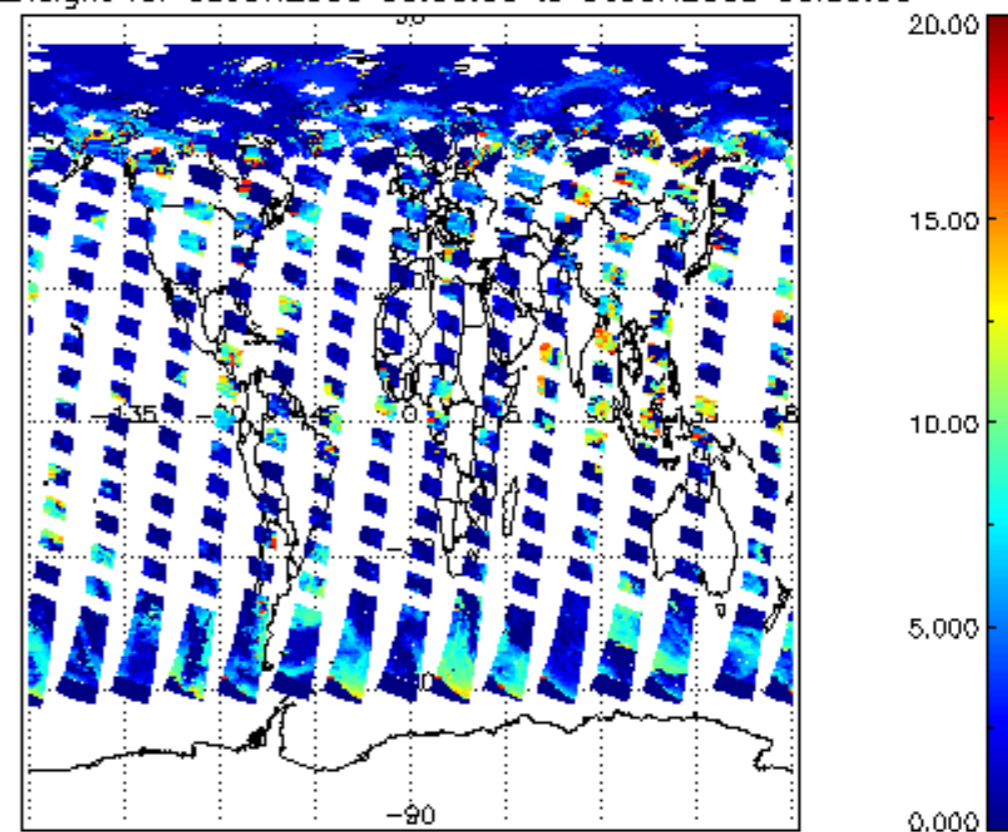
cl_top_height for 05JUN2008 00:00:00 to 06JUN2008 00:00:00
