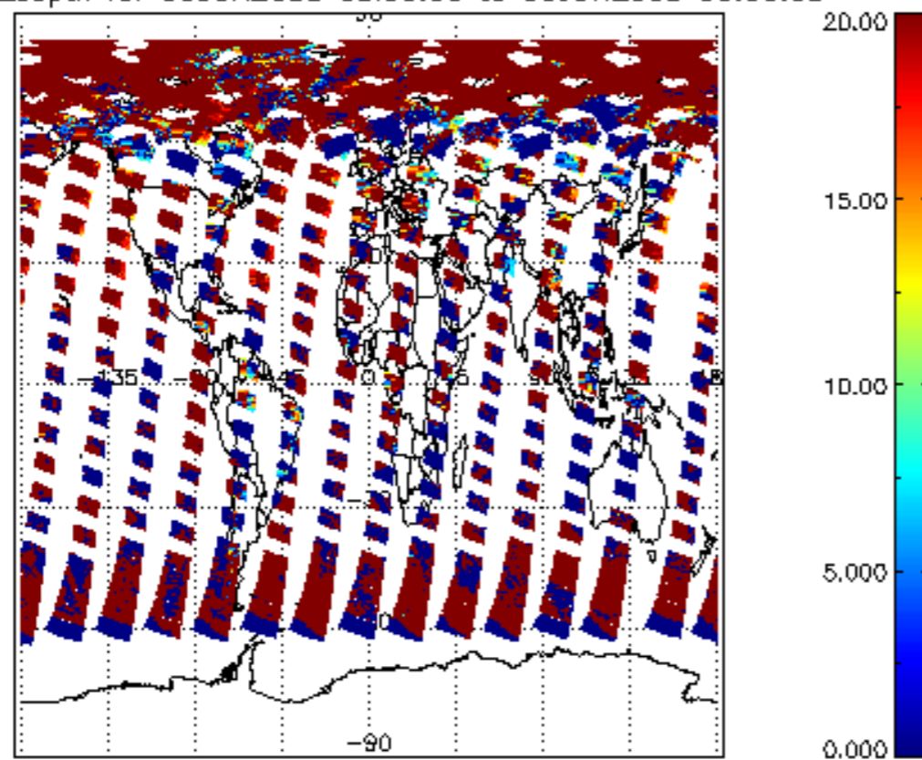
cl_opt_depth for 05JUN2008 00:00:00 to 06JUN2008 00:00:00
