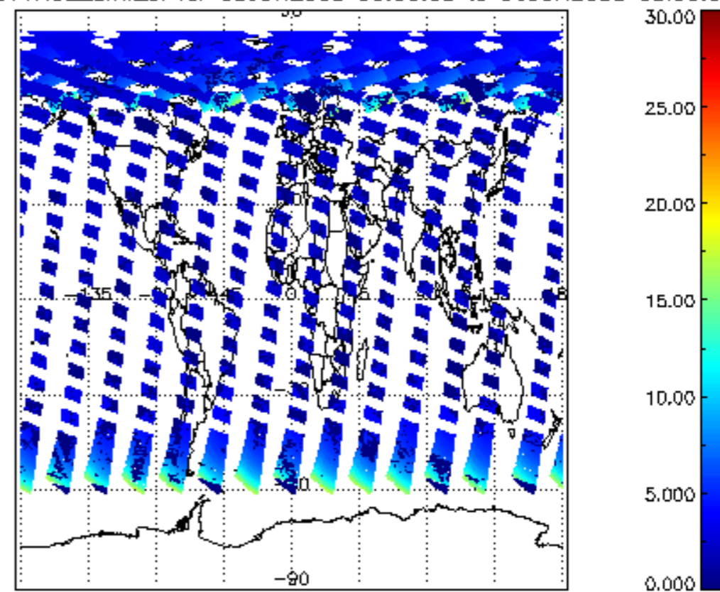
iCIOL2P_NADUV1NO2_amf_cl for 05JUN2008 00:00:00 to 06JUN2008 00:00:00
