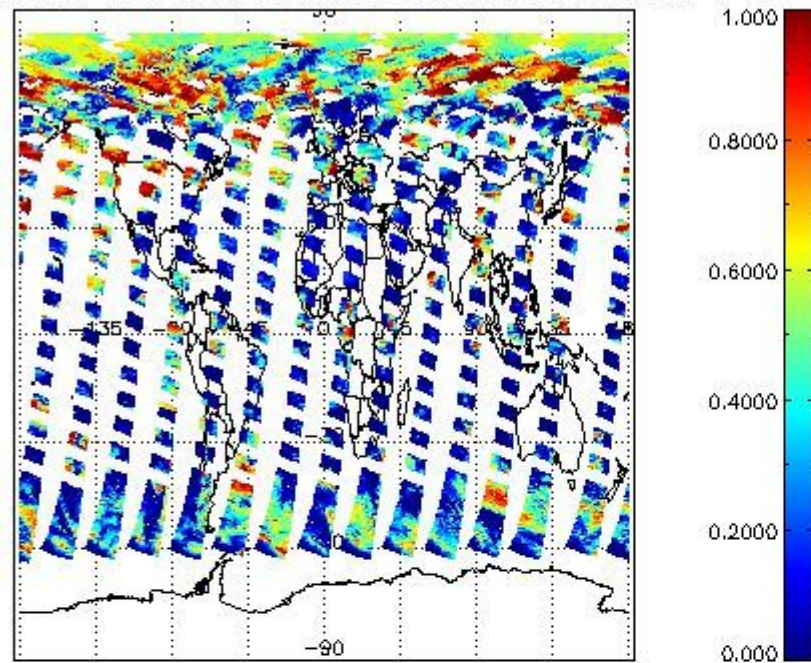
cL_frac for 05JUN2008 00:00:00 to 06JUN2008 00:00:00
