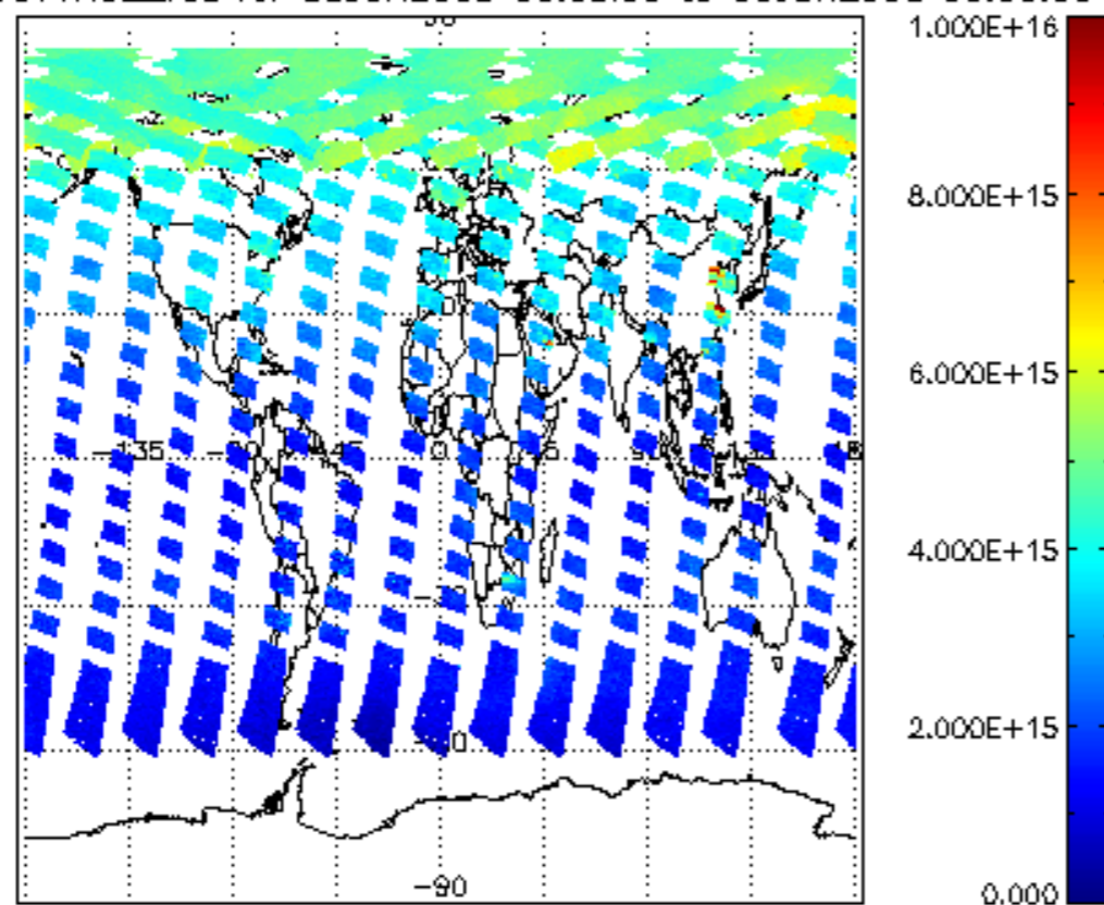
SCIOL2P_NADUV1NO2_vcd for 05JUN2008 00:00:00 to 06JUN2008 00:00:00
