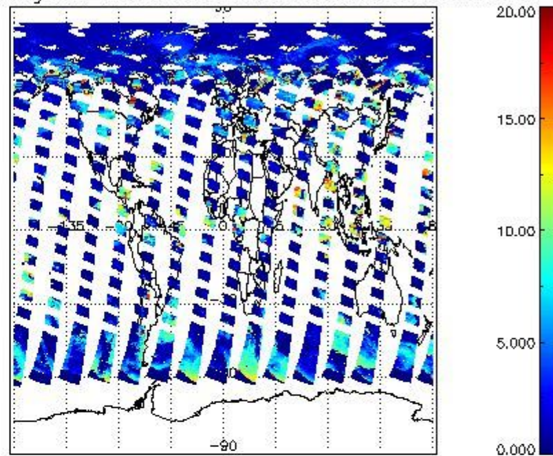
cL_top_height for 05JUN2008 00:00:00 to 06JUN2008 00:00:00
