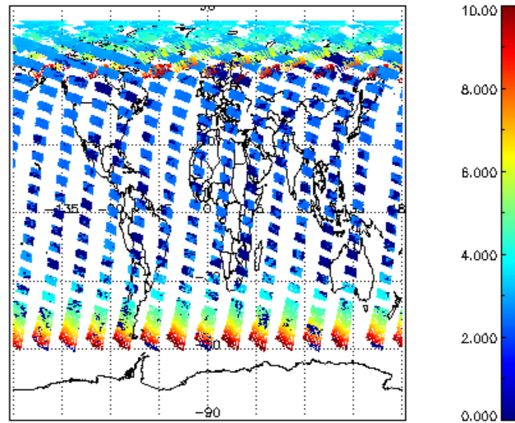
SCIOL2P_NADUV003_amf_cl for 05JUN2008 00:00:00 to 06JUN2008 00:00:00
