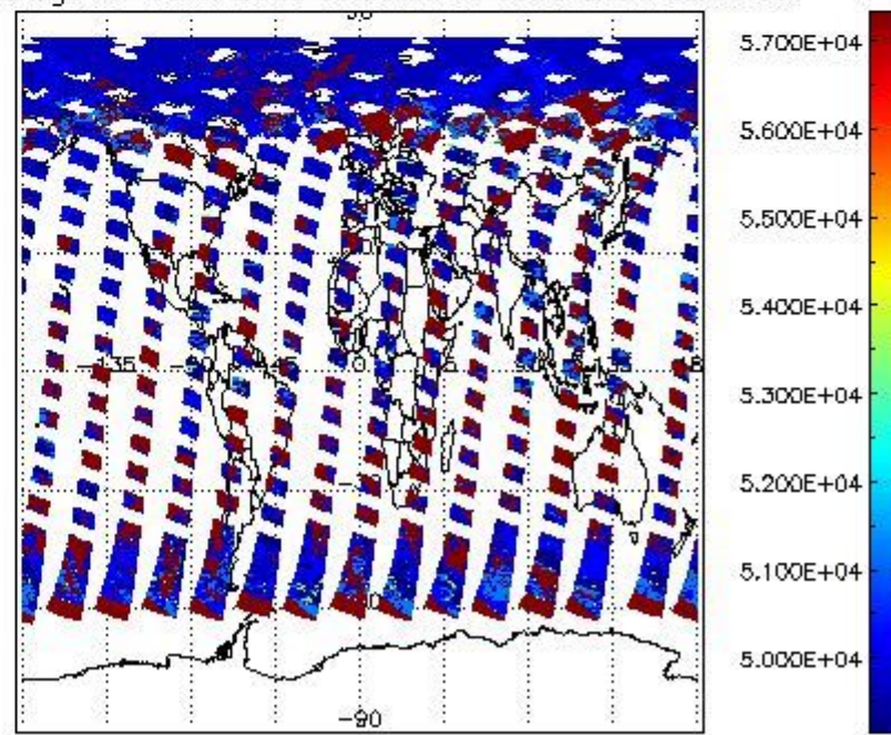
cloud_flags for 05JUN2008 00:00:00 to 06JUN2008 00:00:00
