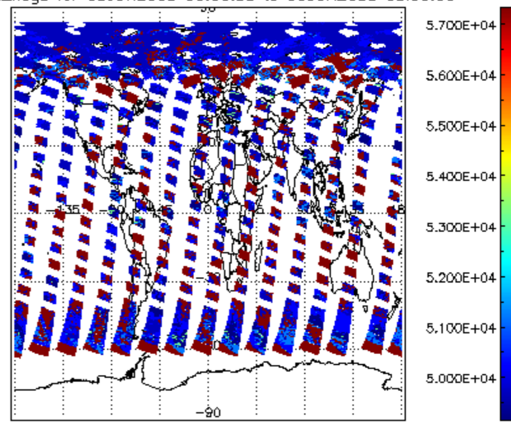
cloud_flags for 05JUN2008 00:00:00 to 06JUN2008 00:00:00
