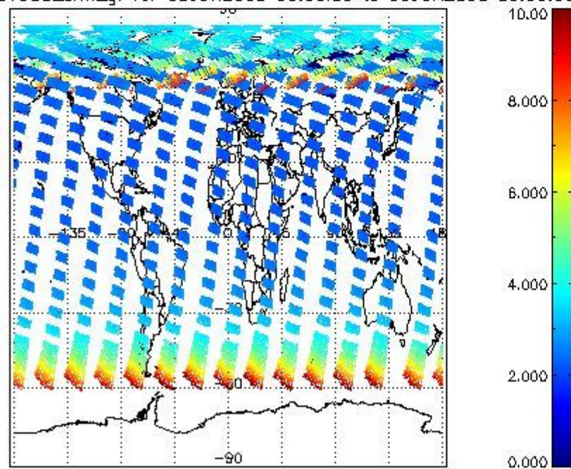
SCIOL2P_NADUV003_amf_gr for 05JUN2008 00:00:00 to 06JUN2008 00:00:00
