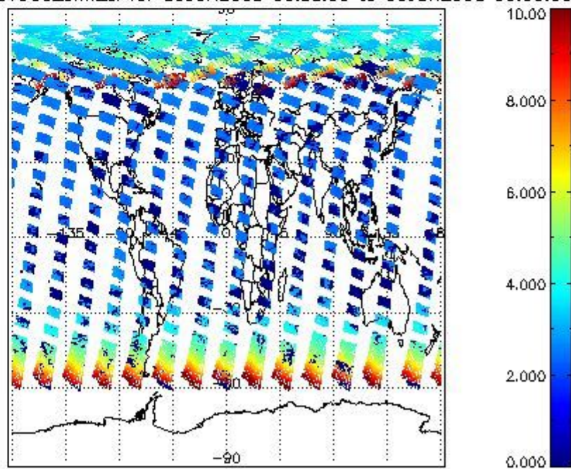
SCIOL2P_NADUV003_amf_cl for 05JUN2008 00:00:00 to 06JUN2008 00:00:00
