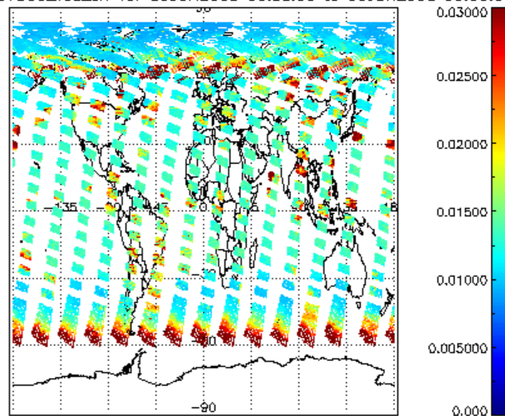
SCIOL2P_NADUV003_vcd_err for 05JUN2008 00:00:00 to 06JUN2008 00:00:00
