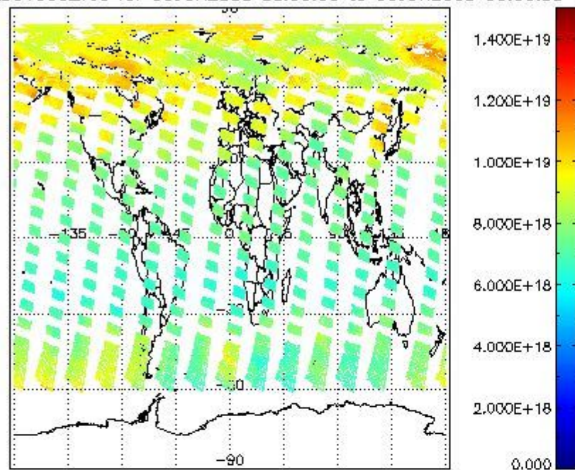
SCIOL2P_NADUV003_vcd for 05JUN2008 00:00:00 to 06JUN2008 00:00:00
