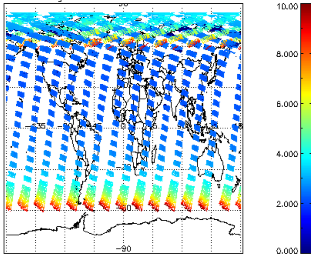
SCIOL2P_NADUV003_amf_gr for 05JUN2008 00:00:00 to 06JUN2008 00:00:00
