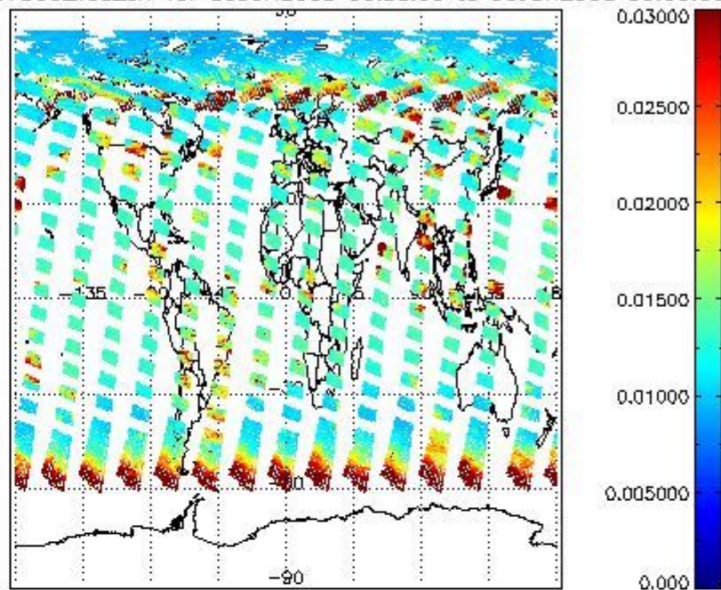
SCIOL2P_NADUV003_vcd_err for 05JUN2008 00:00:00 to 06JUN2008 00:00:00
