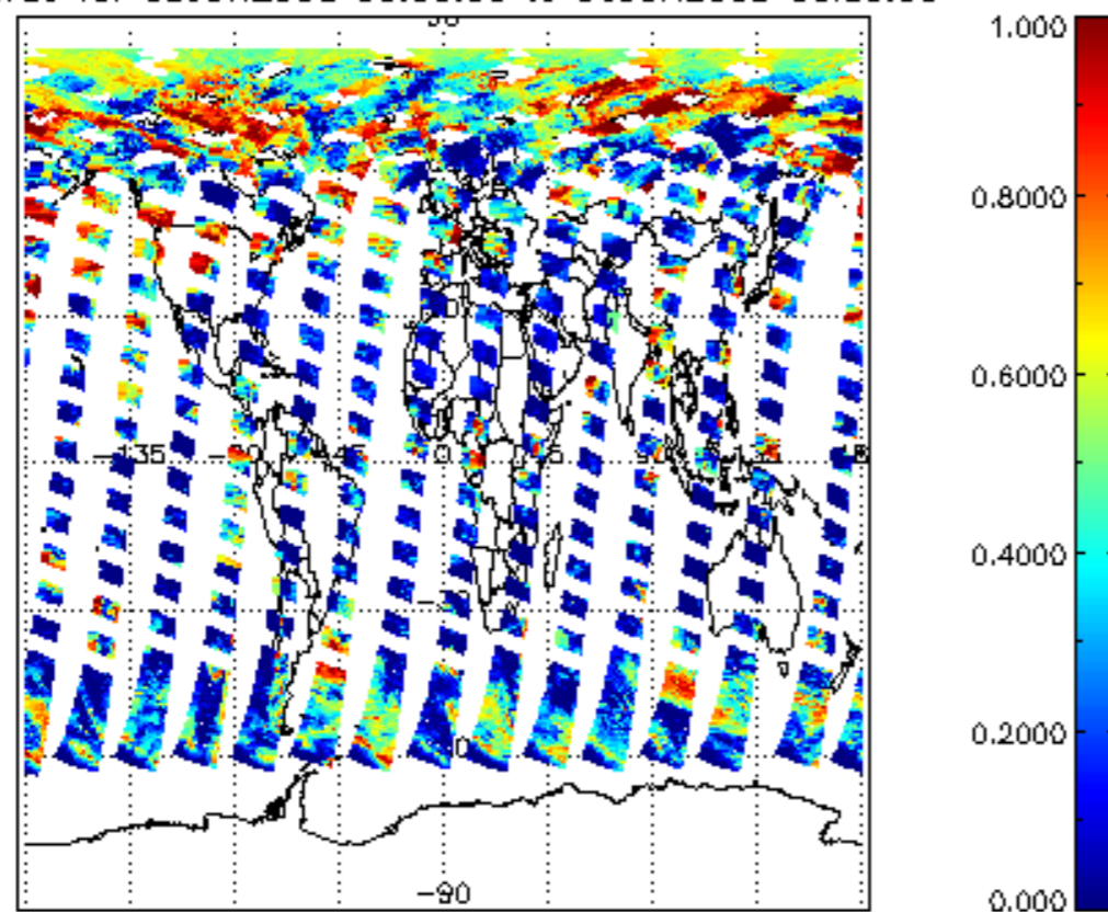
cl_frac for 05JUN2008 00:00:00 to 06JUN2008 00:00:00
