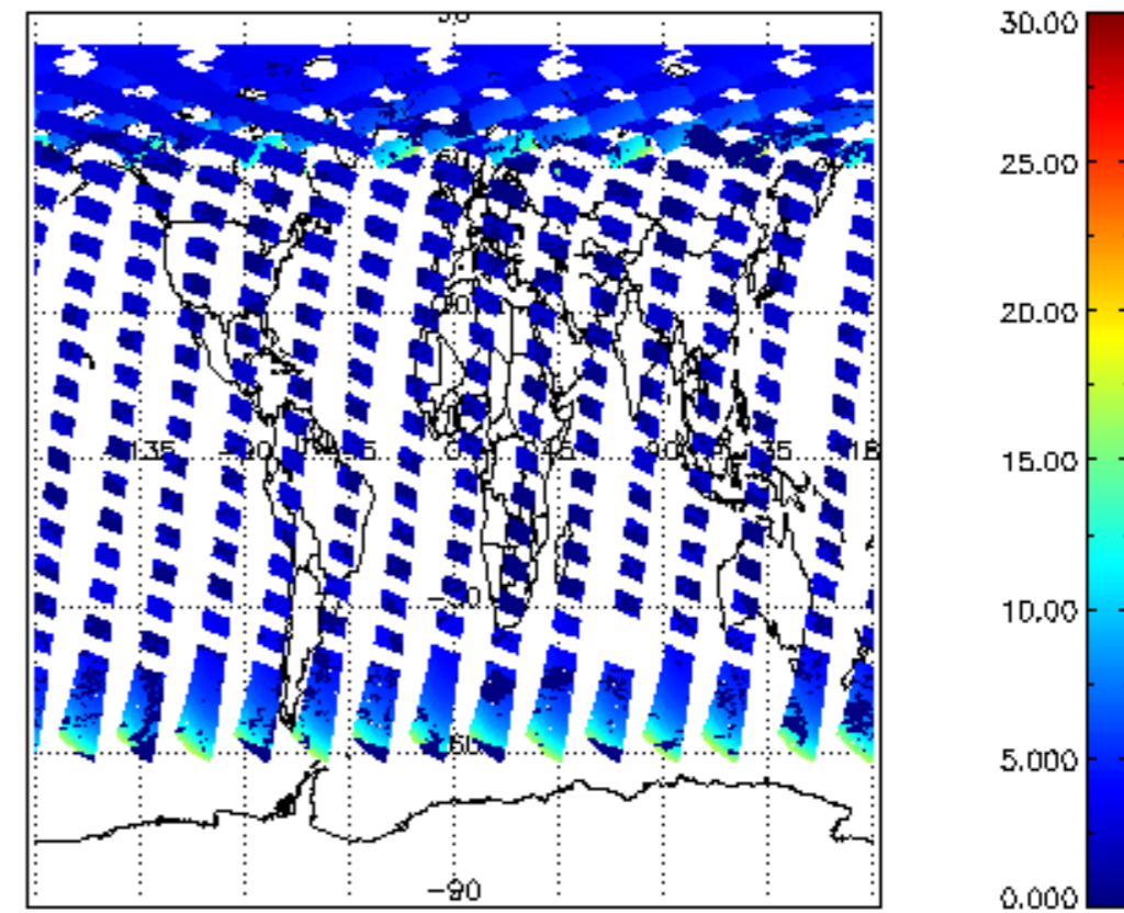
iCIOL2P_NADUV1NO2_amf_cl for 01JUN2008 00:00:00 to 02JUN2008 00:00:00
