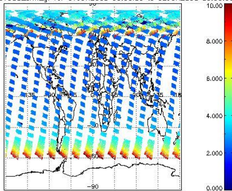
SCIOL2P_NADUV003_amf_gr for 01JUN2008 00:00:00 to 02JUN2008 00:00:00
