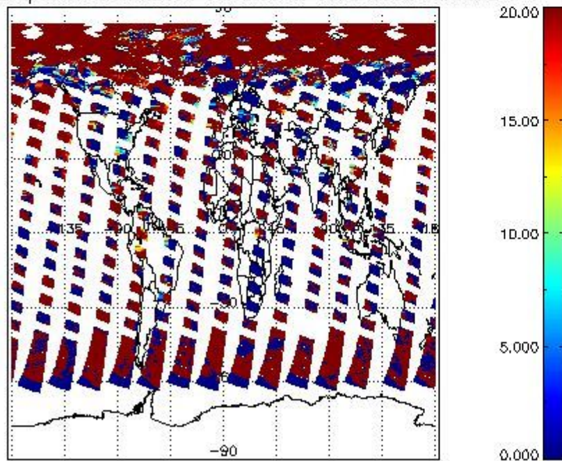
cL_opt_depth for 01JUN2008 00:00:00 to 02JUN2008 00:00:00
