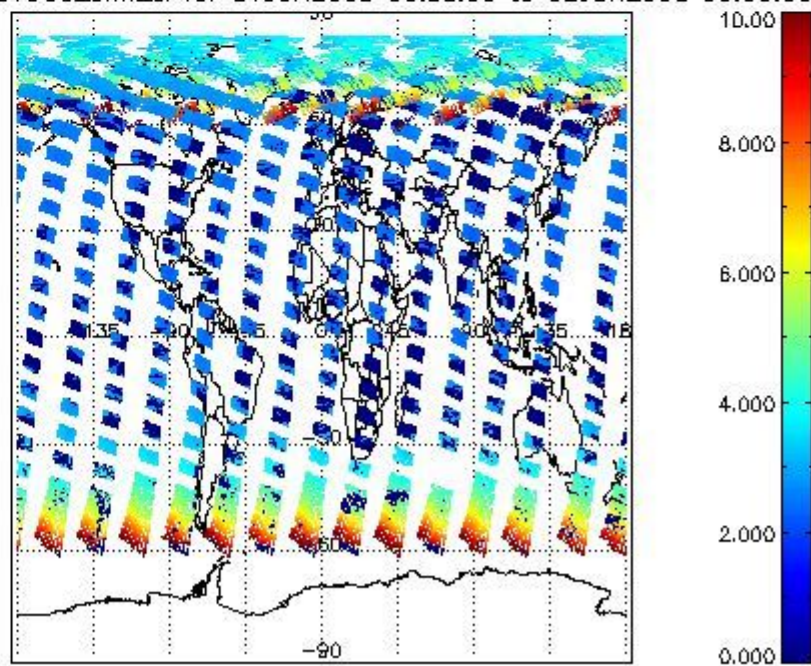
SCIOL2P_NADUV003_amf_cl for 01JUN2008 00:00:00 to 02JUN2008 00:00:00
