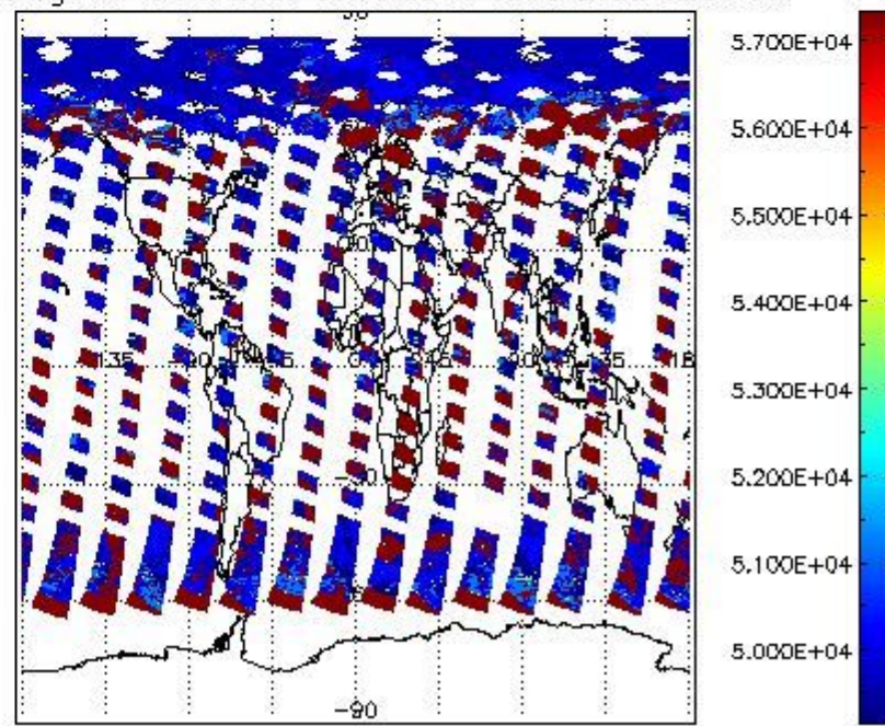
cloud_flags for 01JUN2008 00:00:00 to 02JUN2008 00:00:00
