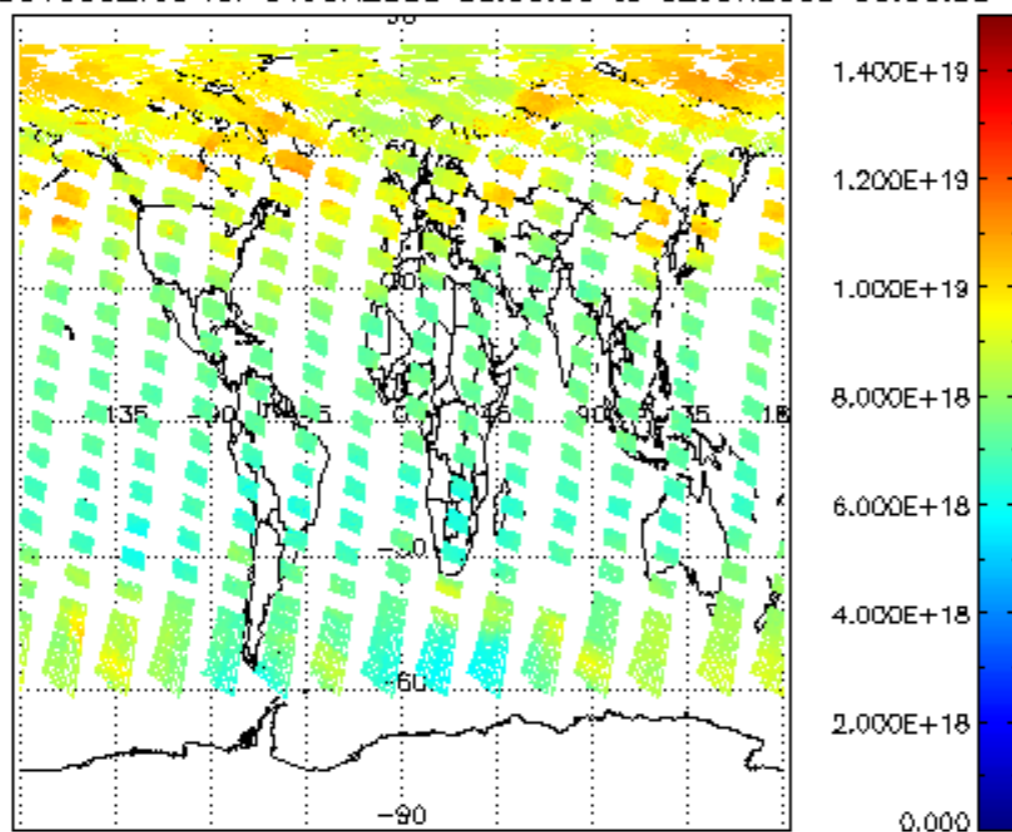
SCIOL2P_NADUV003_vcd for 01JUN2008 00:00:00 to 02JUN2008 00:00:00
