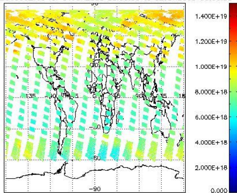
SCIOL2P_NADUV003_vcd for 01JUN2008 00:00:00 to 02JUN2008 00:00:00
