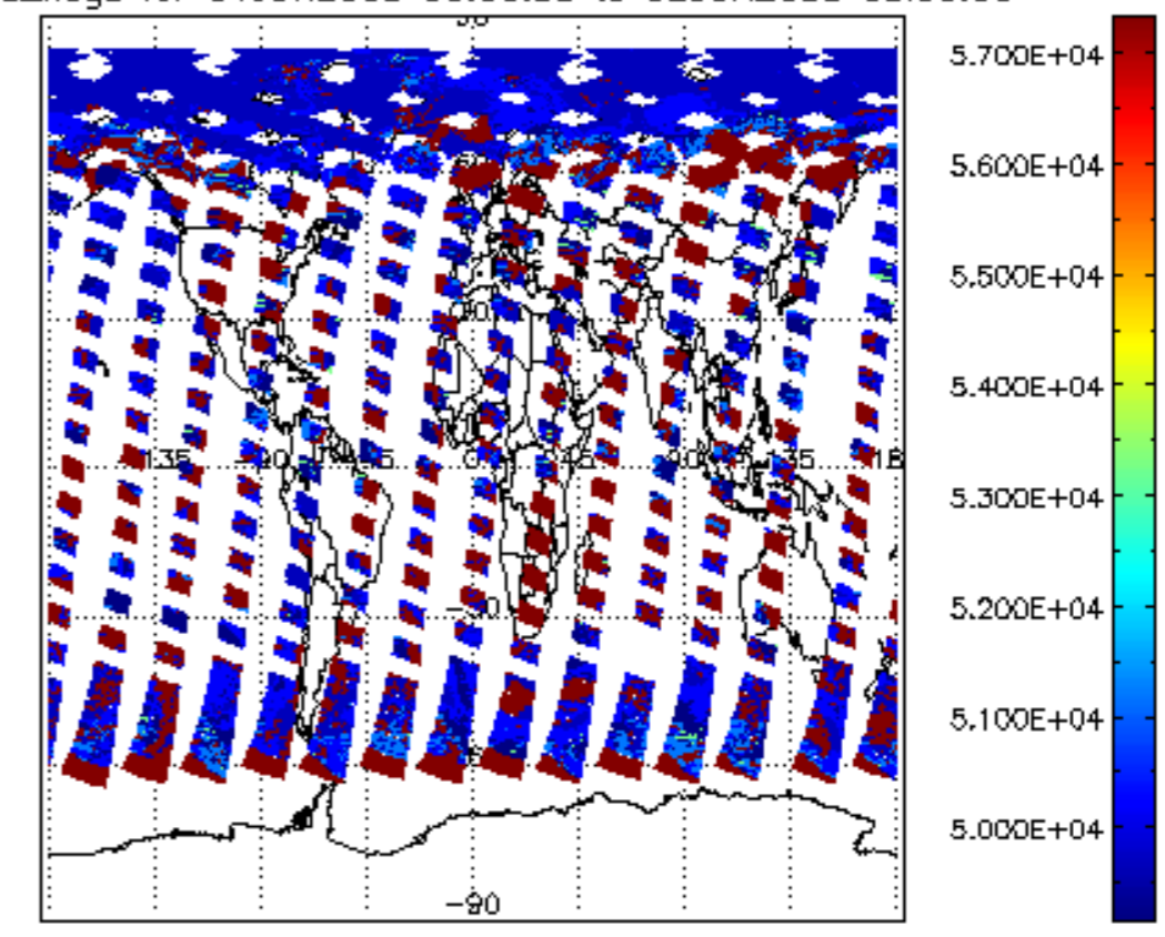
cloud_flags for 01JUN2008 00:00:00 to 02JUN2008 00:00:00
