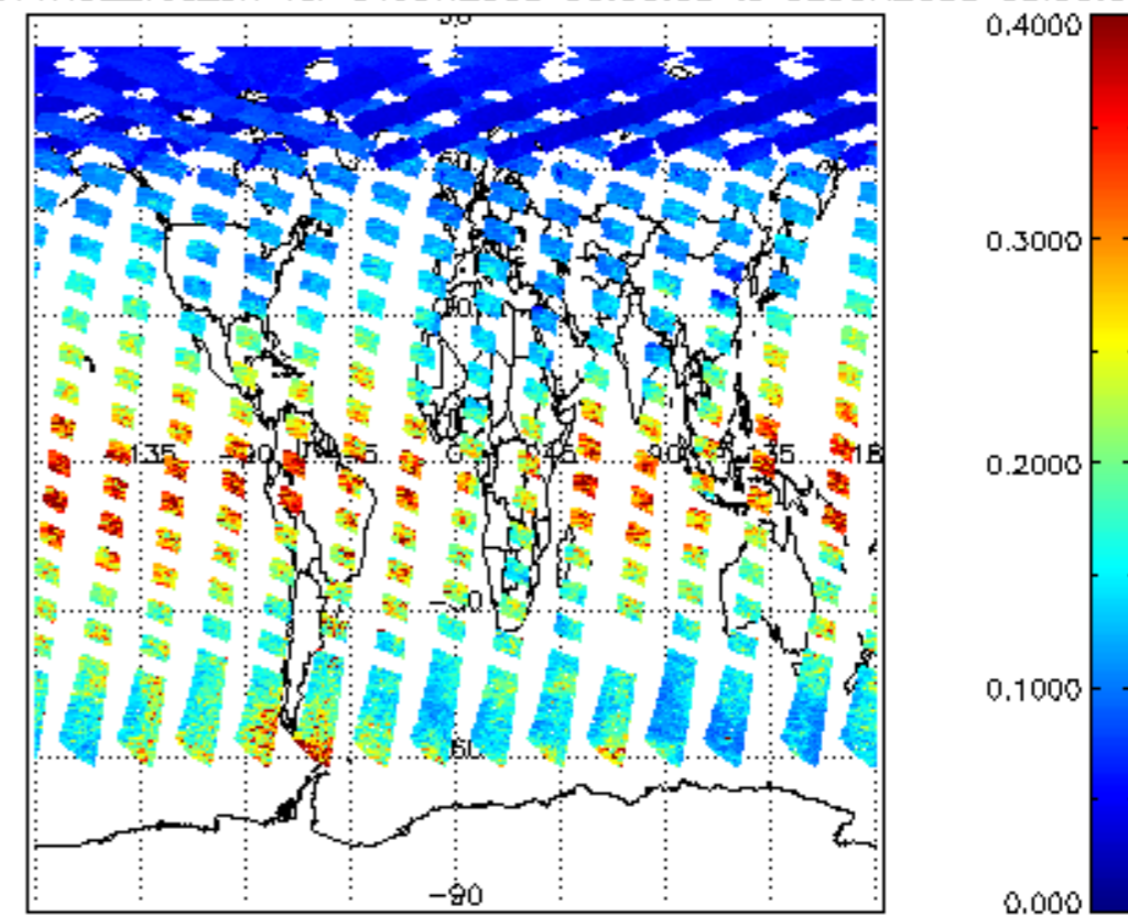
iCIOL2P_NADUV1NO2_vcd_err for 01JUN2008 00:00:00 to 02JUN2008 00:00:00
