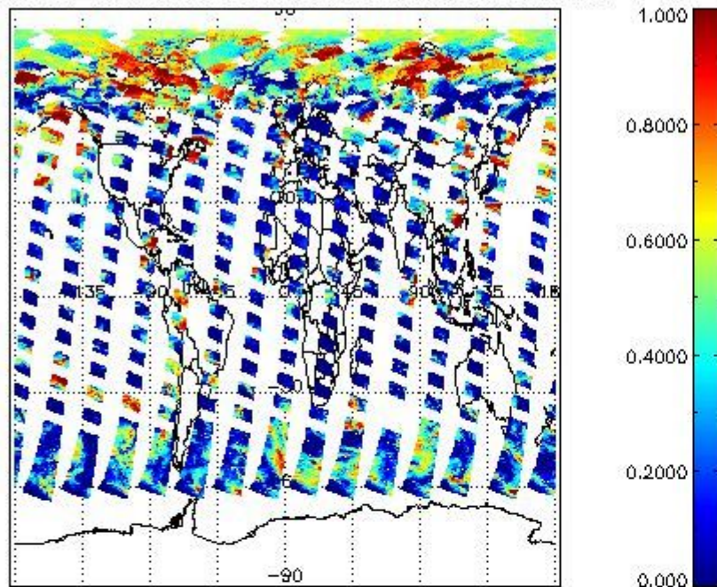
cL_frac for 01JUN2008 00:00:00 to 02JUN2008 00:00:00
