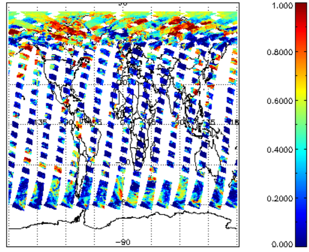
cl_frac for 01JUN2008 00:00:00 to 02JUN2008 00:00:00
