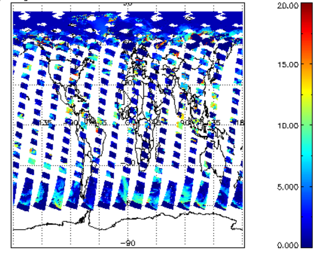
cl_top_height for 01JUN2008 00:00:00 to 02JUN2008 00:00:00
