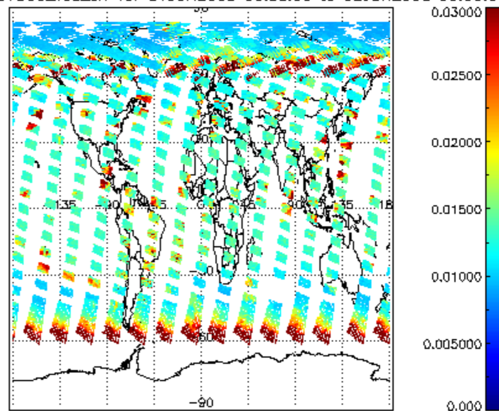
SCIOL2P_NADUV003_vcd_err for 01JUN2008 00:00:00 to 02JUN2008 00:00:00
