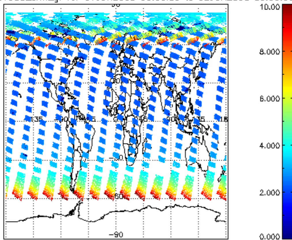
SCIOL2P_NADUV003_amf_gr for 01JUN2008 00:00:00 to 02JUN2008 00:00:00
