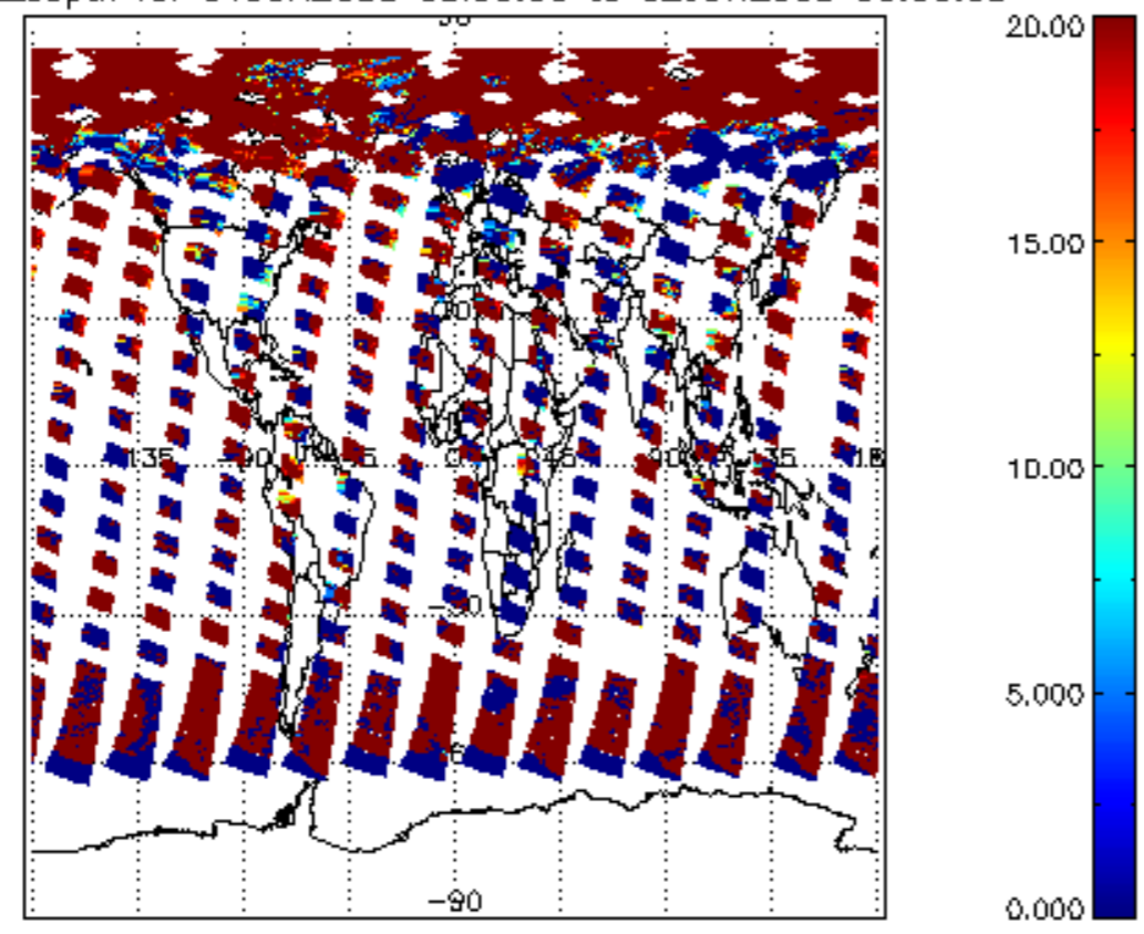
cl_opt_depth for 01JUN2008 00:00:00 to 02JUN2008 00:00:00
