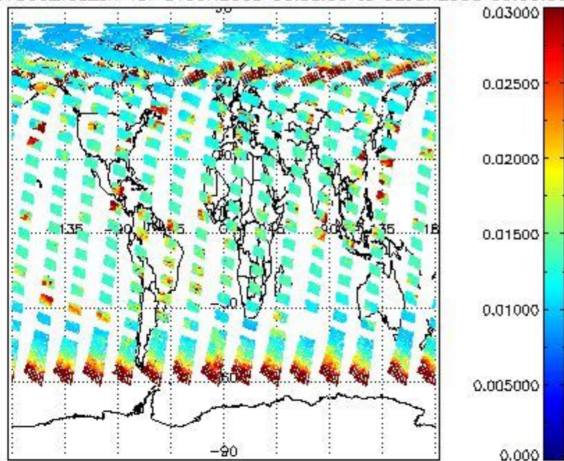
SCIOL2P_NADUV003_vcd_err for 01JUN2008 00:00:00 to 02JUN2008 00:00:00
