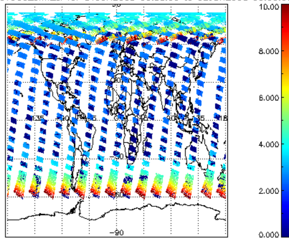
SCIOL2P_NADUV003_amf_cl for 01JUN2008 00:00:00 to 02JUN2008 00:00:00
