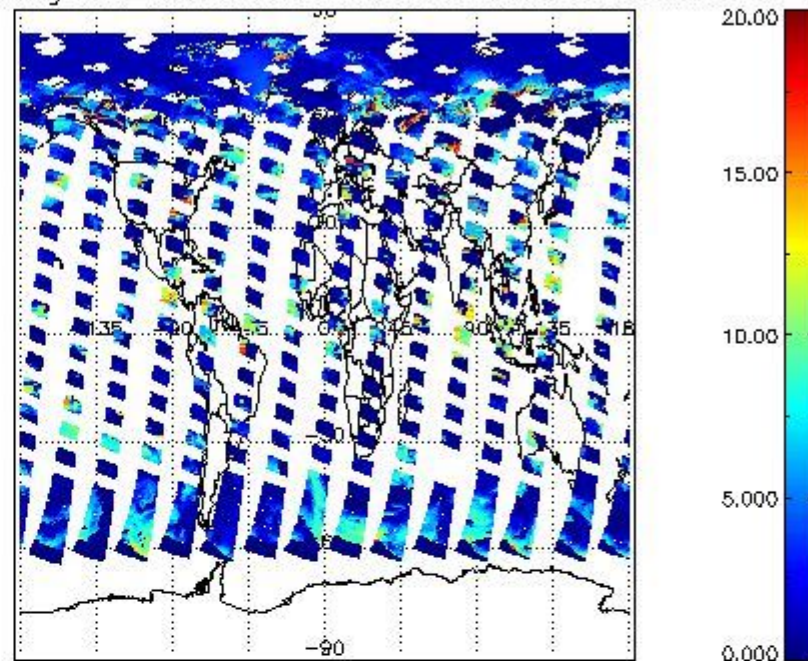
cL_top_height for 01JUN2008 00:00:00 to 02JUN2008 00:00:00
