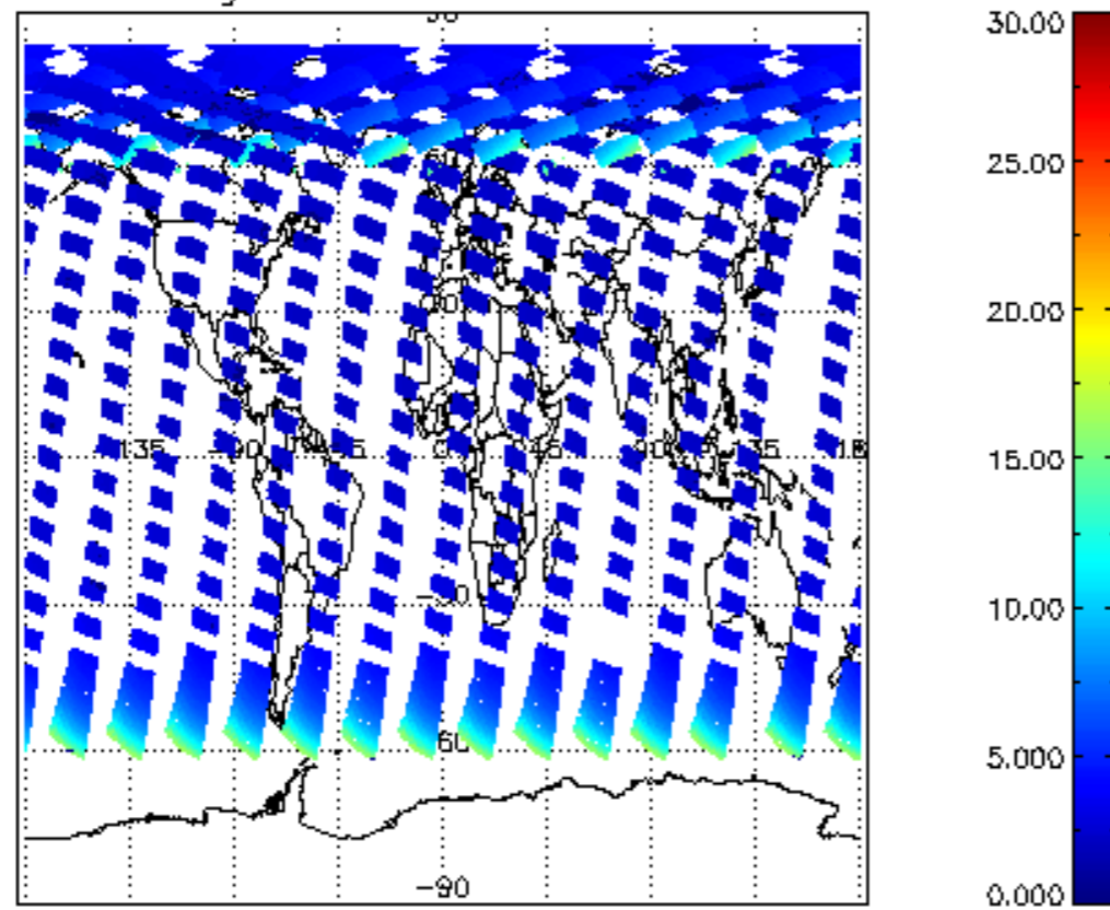
iCIOL2P_NADUV1NO2_amf_gr for 01JUN2008 00:00:00 to 02JUN2008 00:00:00
