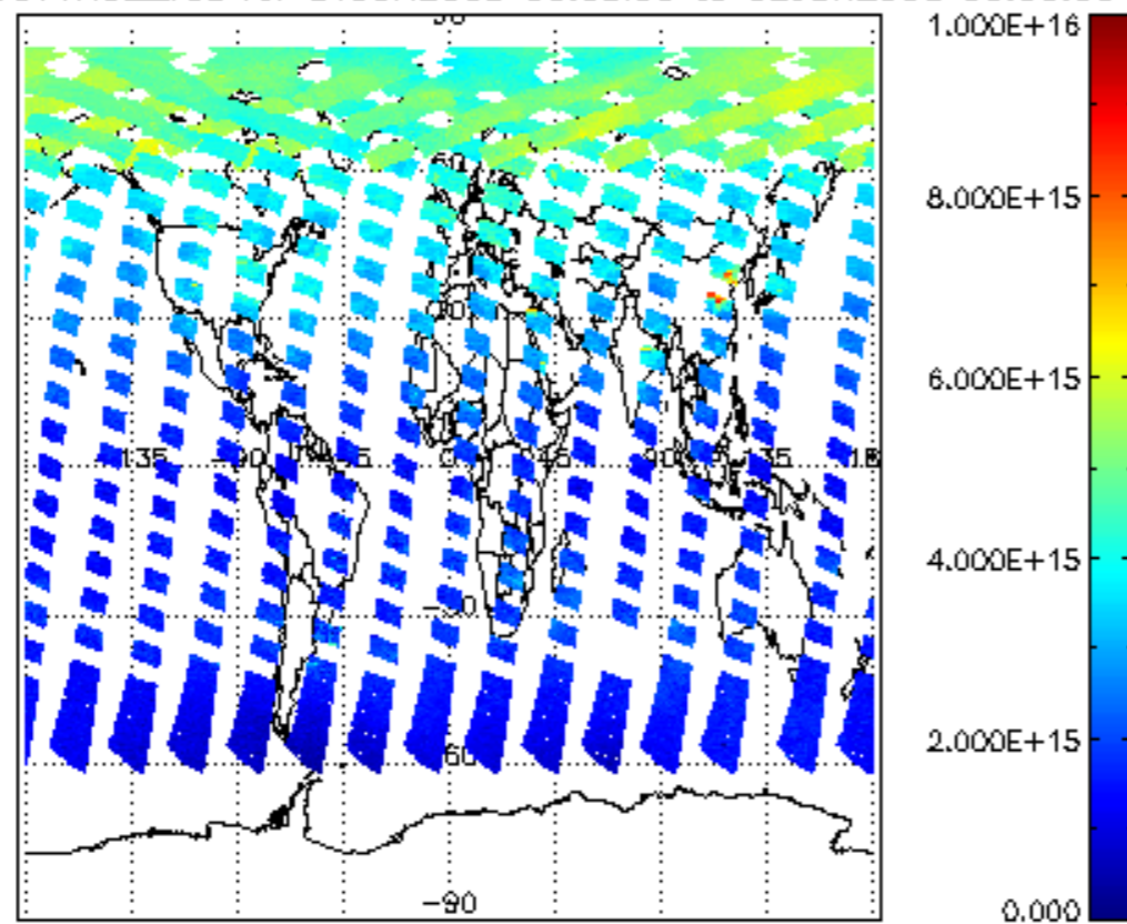
SCIOL2P_NADUV1NO2_vcd for 01JUN2008 00:00:00 to 02JUN2008 00:00:00
