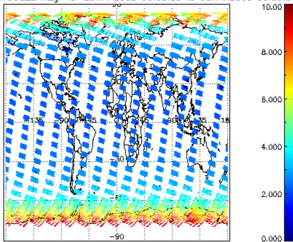
SCIOL2P_NADUV003_amf_gr for 29MAR2008 00:00:00 to 30MAR2008 00:00:00
