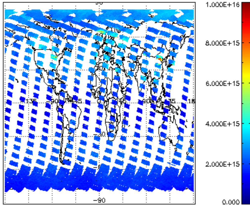
SCIOL2P_NADUV1NO2_vcd for 29MAR2008 00:00:00 to 30MAR2008 00:00:00
