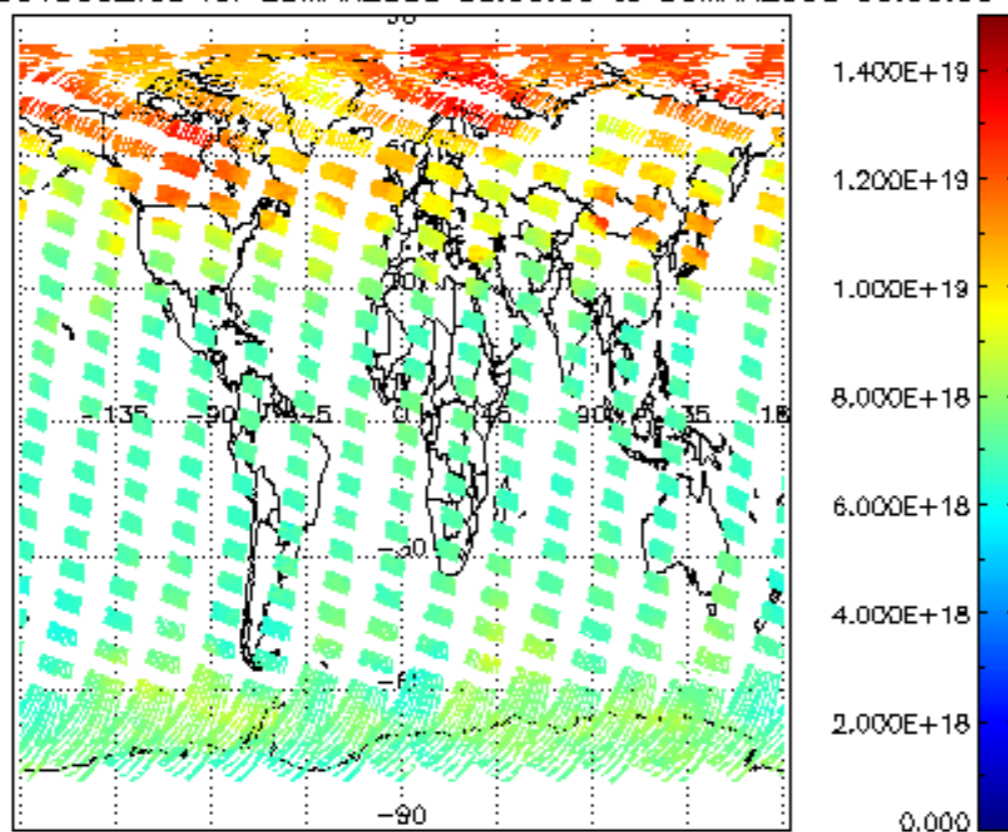
SCIOL2P_NADUV003_vcd for 29MAR2008 00:00:00 to 30MAR2008 00:00:00
