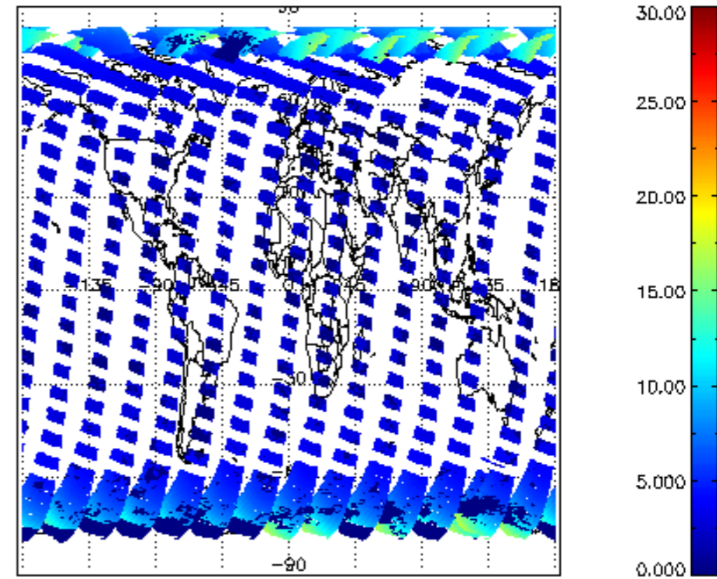
SCIOL2P_NADUV1NO2_amf_cl for 29MAR2008 00:00:00 to 30MAR2008 00:00:00
