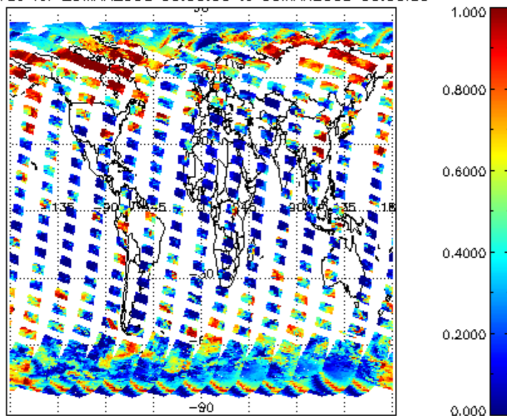
cL_frac for 29MAR2008 00:00:00 to 30MAR2008 00:00:00
