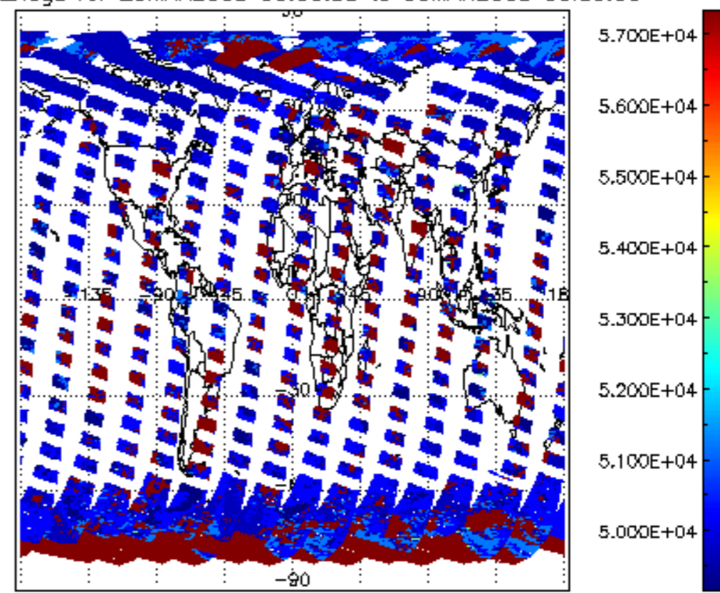
cloud_flags for 29MAR2008 00:00:00 to 30MAR2008 00:00:00
