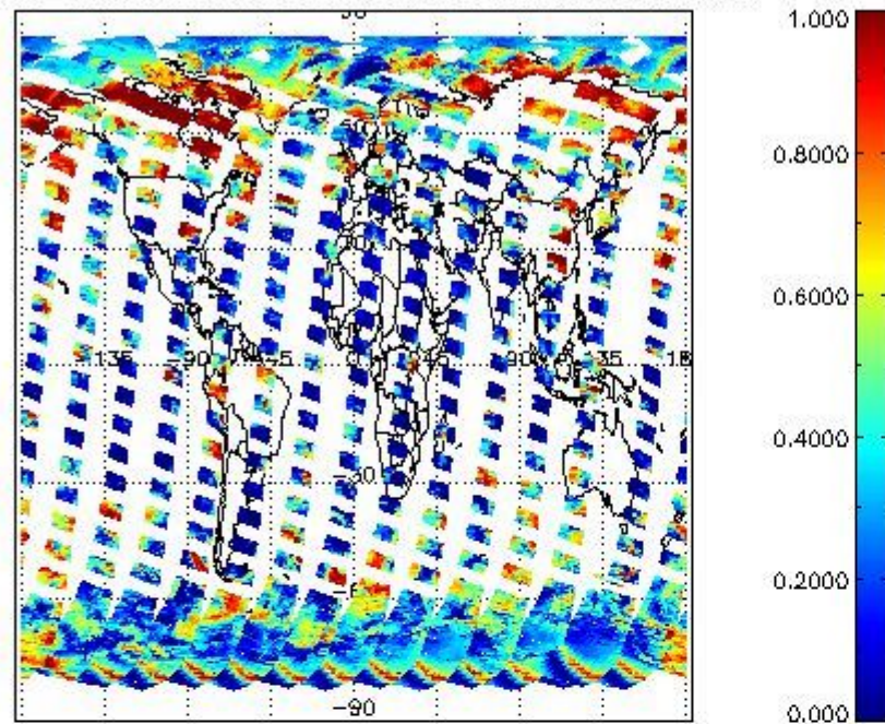
cLfrac for 29MAR2008 00:00:00 to 30MAR2008 00:00:00
