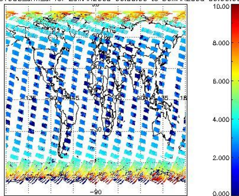
SCIOL2P_NADUV003_amf_gr for 29MAR2008 00:00:00 to 30MAR2008 00:00:00 SCIOL2P_NADUV003_amf_cl for 29MAR2008 00:00:00 to 30MAR2008 00:00:00
