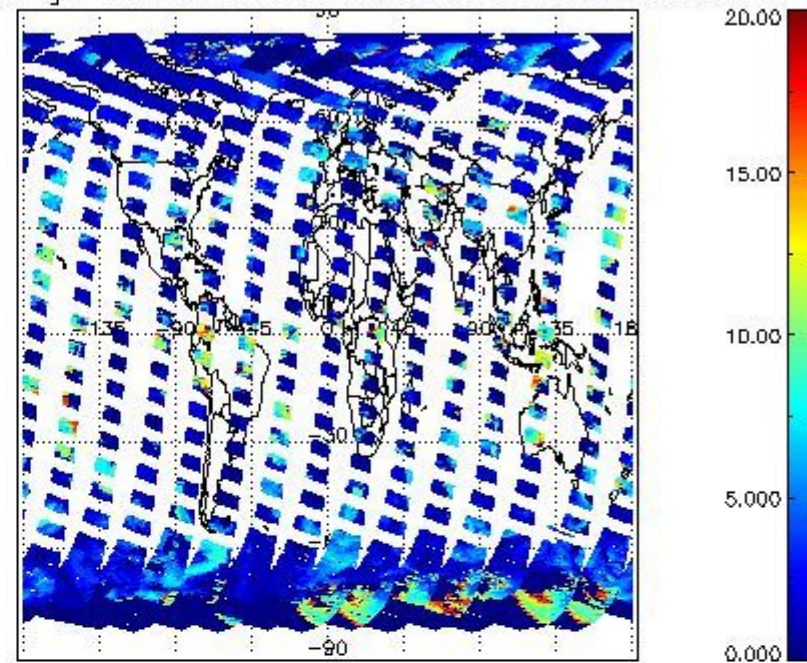
cLtop_height for 29MAR2008 00:00:00 to 30MAR2008 00:00:00
