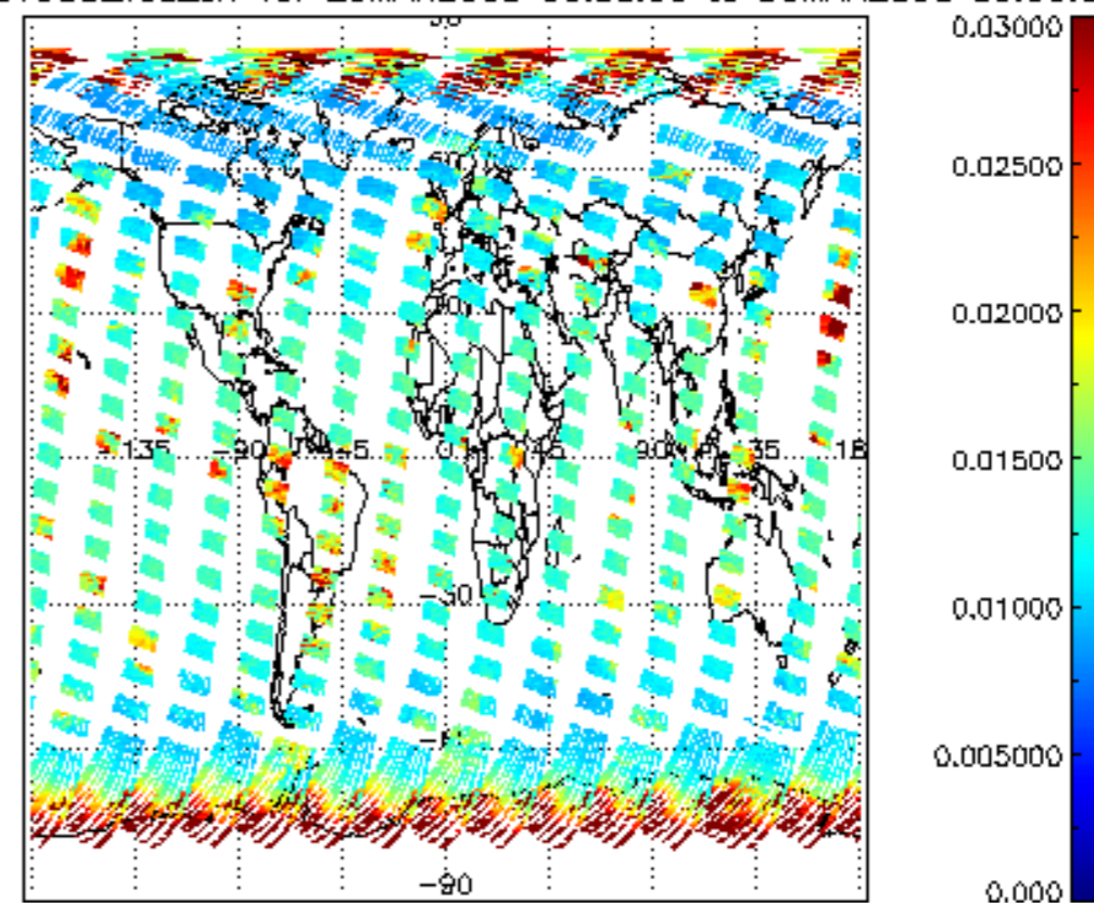
SCIOL2P_NADUV003_vcd_err for 29MAR2008 00:00:00 to 30MAR2008 00:00:00
