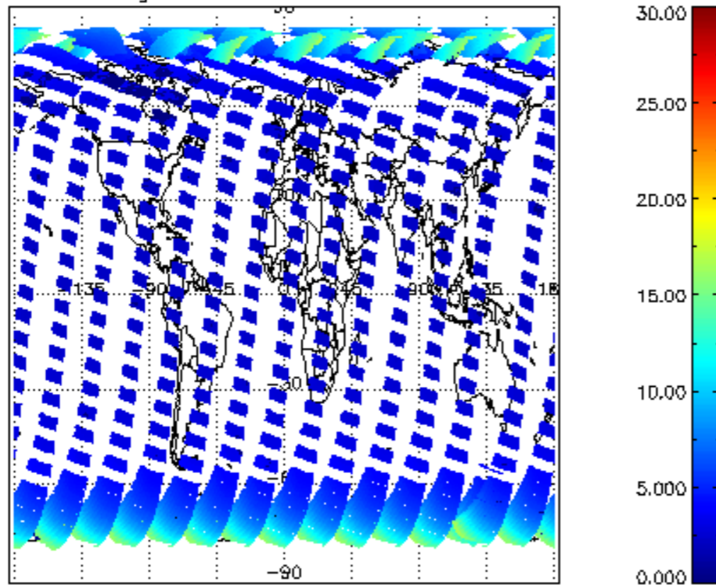
SCIOL2P_NADUV1NO2_amf_gr for 29MAR2008 00:00:00 to 30MAR2008 00:00:00
