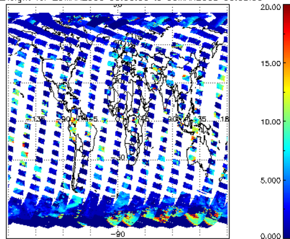
cL_top_height for 29MAR2008 00:00:00 to 30MAR2008 00:00:00
