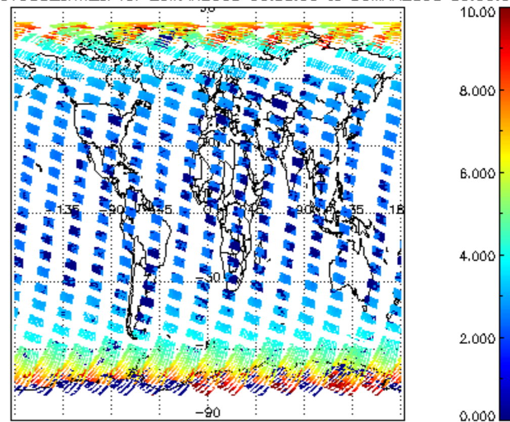
SCIOL2P_NADUV003_amf_cl for 29MAR2008 00:00:00 to 30MAR2008 00:00:00
