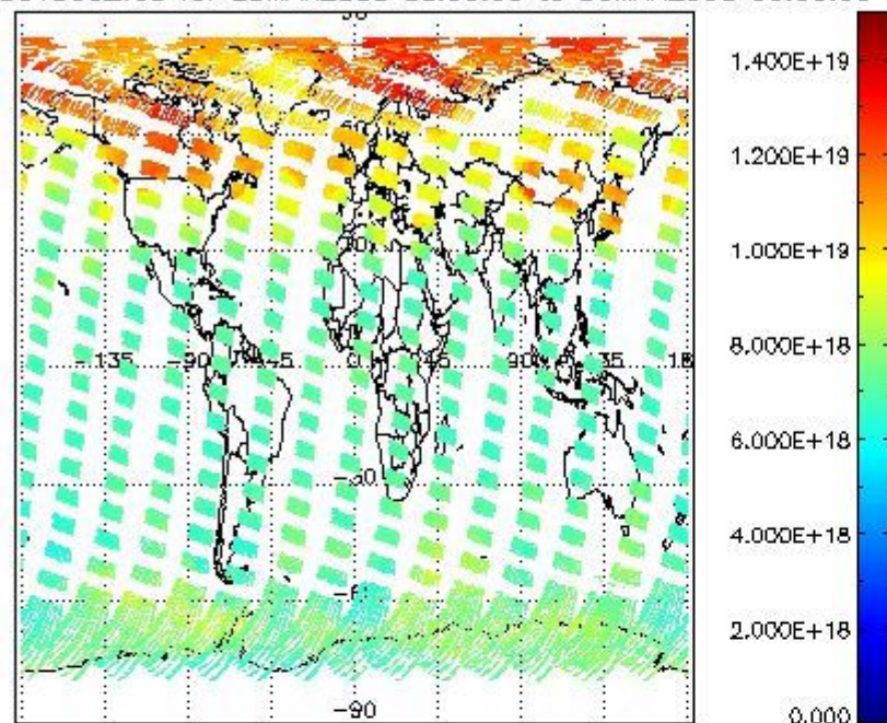
SCIOL2P_NADUV003_vcd for 29MAR2008 00:00:00 to 30MAR2008 00:00:00 SCIOL2P_NADUV003_vcd_err for 29MAR2008 00:00:00 to 30MAR2008 00:00:00
