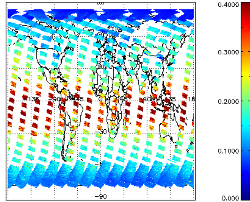
SCIOL2P_NADUV1NO2_vcd_err for 29MAR2008 00:00:00 to 30MAR2008 00:00:00
