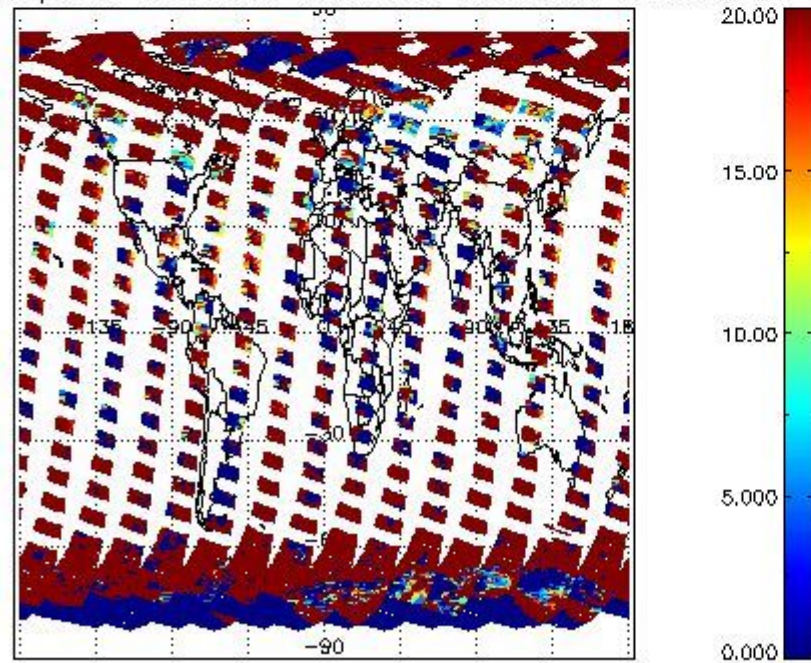
cLopt_depth for 29MAR2008 00:00:00 to 30MAR2008 00:00:00
