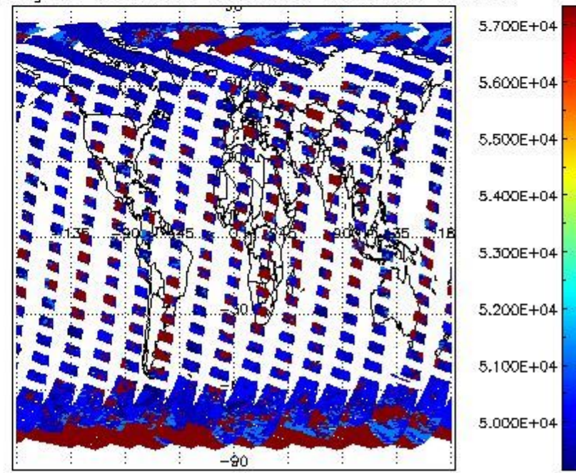
cloud_flags for 29MAR2008 00:00:00 to 30MAR2008 00:00:00
