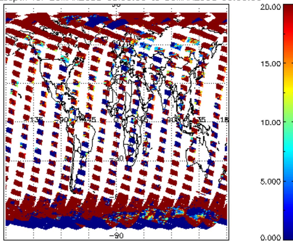
cL_opt_depth for 29MAR2008 00:00:00 to 30MAR2008 00:00:00
