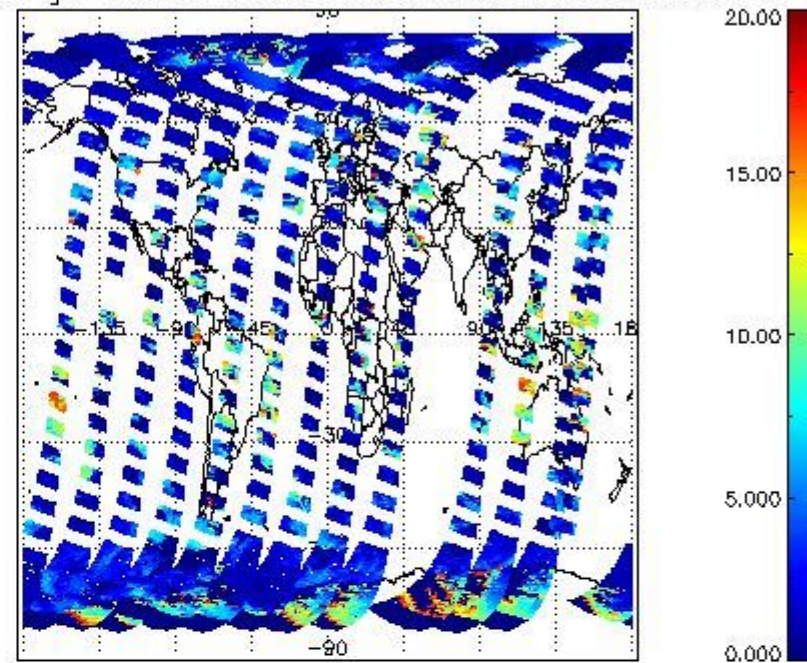
cLtop_height for 28MAR2008 00:00:00 to 29MAR2008 00:00:00
