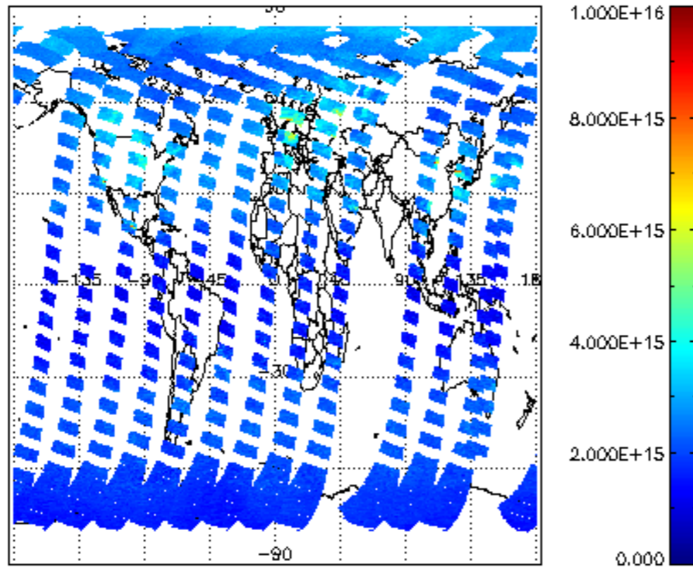
SCIOL2P_NADUV1NO2_vcd for 28MAR2008 00:00:00 to 29MAR2008 00:00:00
