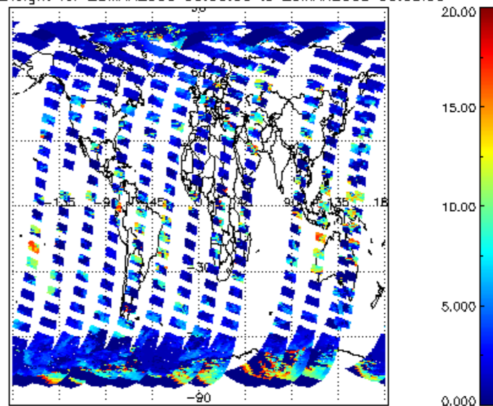
cL_top_height for 28MAR2008 00:00:00 to 29MAR2008 00:00:00
