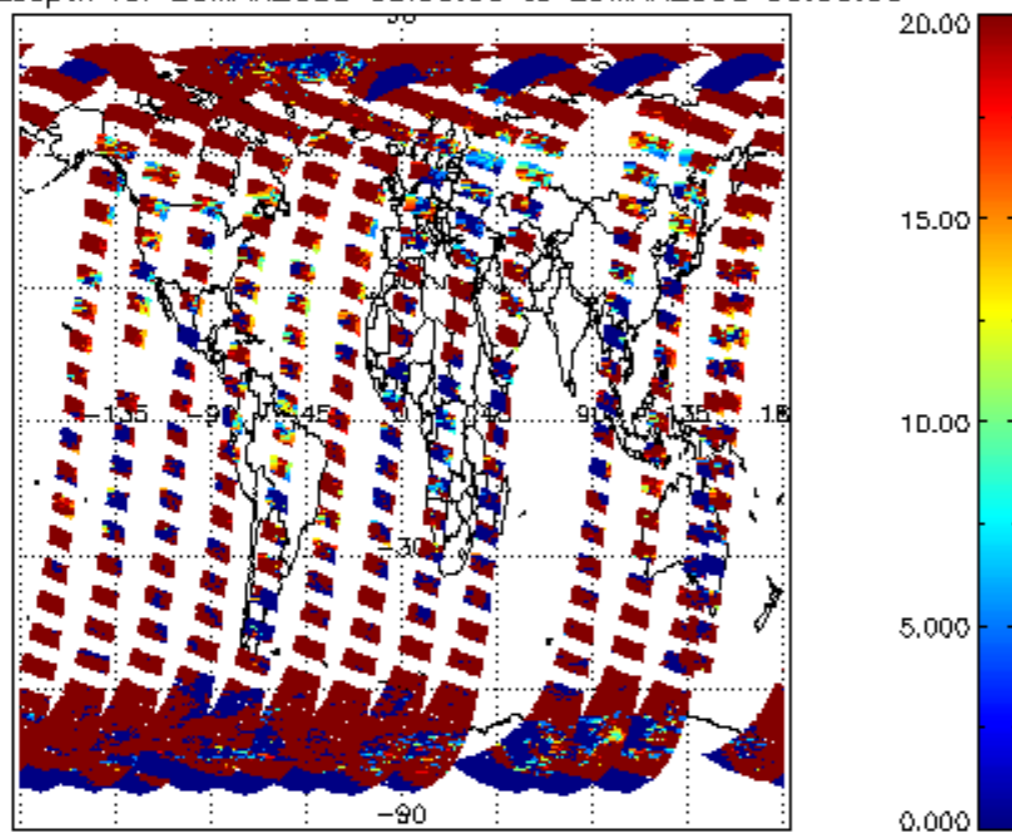
cL_opt_depth for 28MAR2008 00:00:00 to 29MAR2008 00:00:00
