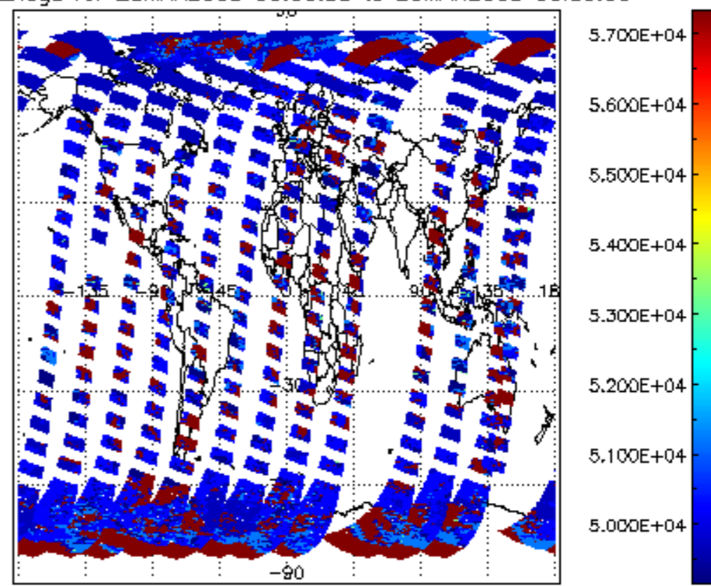
cloud_flags for 28MAR2008 00:00:00 to 29MAR2008 00:00:00
