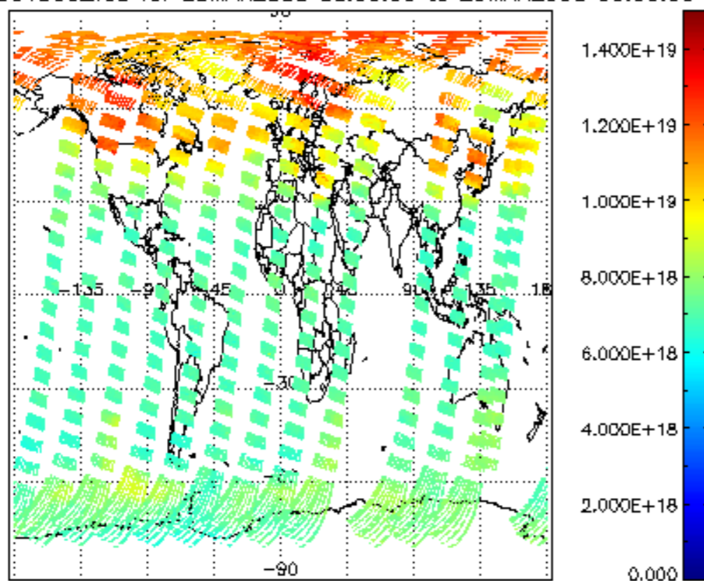
SCIOL2P_NADUV003_vcd for 28MAR2008 00:00:00 to 29MAR2008 00:00:00
