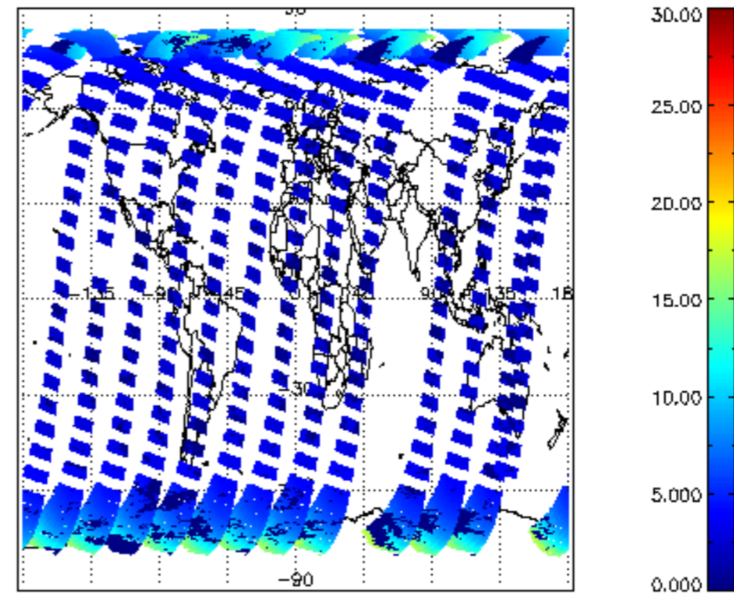
CIOL2P_NADUV1NO2_amf_cl for 28MAR2008 00:00:00 to 29MAR2008 00:00:00
