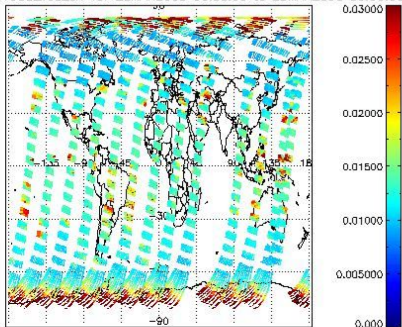
SCIOL2P_NADUV003_vcd for 28MAR2008 00:00:00 to 29MAR2008 00:00:00 SCIOL2P_NADUV003_vcd_err for 28MAR2008 00:00:00 to 29MAR2008 00:00:00
