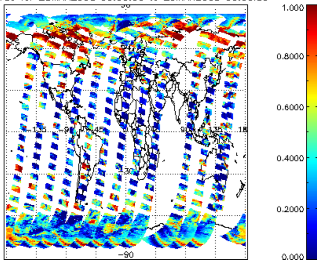
cL_frac for 28MAR2008 00:00:00 to 29MAR2008 00:00:00
