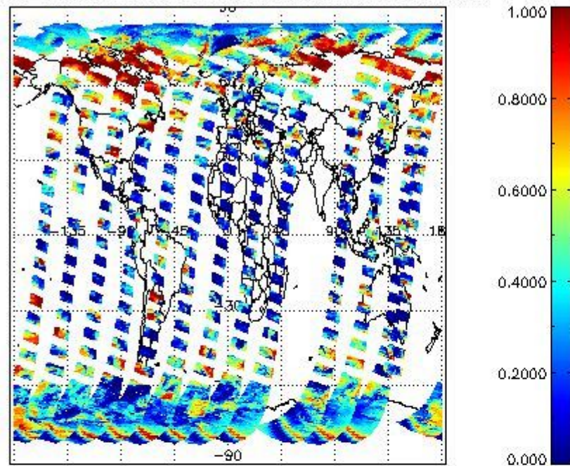
cLfrac for 28MAR2008 00:00:00 to 29MAR2008 00:00:00
