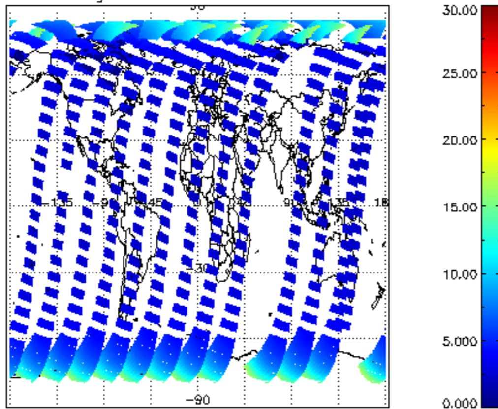
CIOL2P_NADUV1NO2_amf_gr for 28MAR2008 00:00:00 to 29MAR2008 00:00:00
