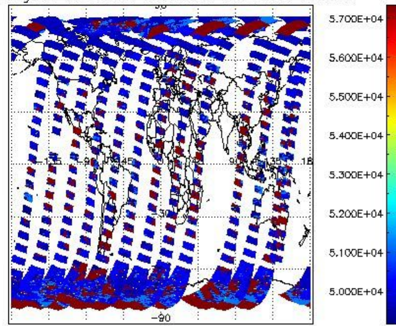
cloud_flags for 28MAR2008 00:00:00 to 29MAR2008 00:00:00
