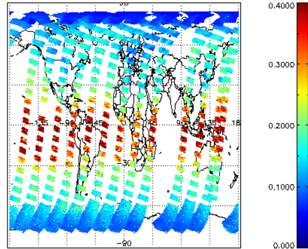
CIOL2P_NADUV1NO2_vcd_err for 28MAR2008 00:00:00 to 29MAR2008 00:00:00
