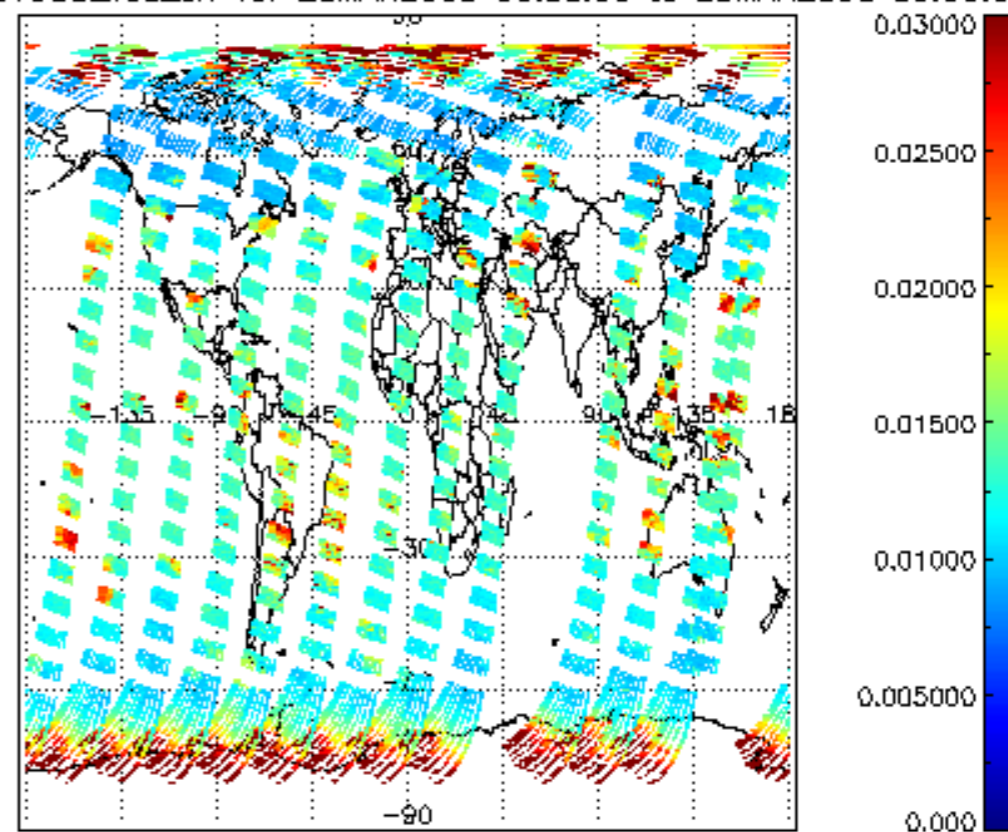
SCIOL2P_NADUV003_vcd_err for 28MAR2008 00:00:00 to 29MAR2008 00:00:00
