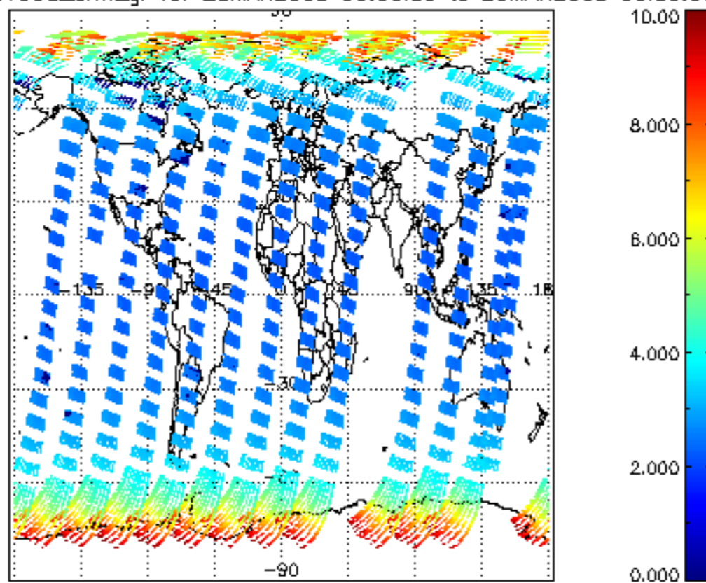
SCIOL2P_NADUV003_amf_gr for 28MAR2008 00:00:00 to 29MAR2008 00:00:00
