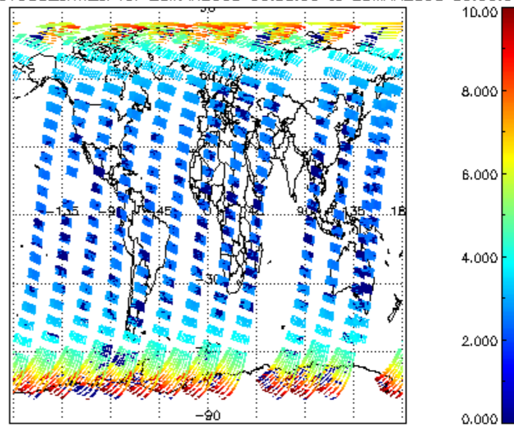
SCIOL2P_NADUV003_amf_cl for 28MAR2008 00:00:00 to 29MAR2008 00:00:00
