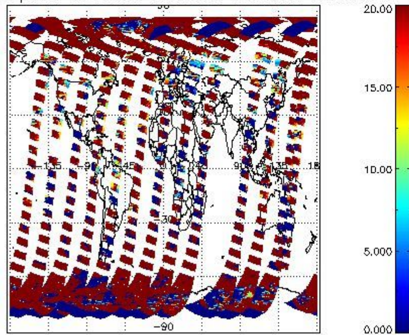
cLopt_depth for 28MAR2008 00:00:00 to 29MAR2008 00:00:00
