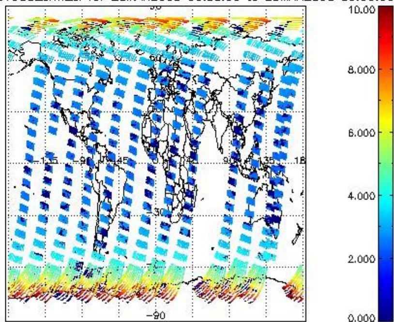
SCIOL2P_NADUV003_amf_gr for 28MAR2008 00:00:00 to 29MAR2008 00:00:00 SCIOL2P_NADUV003_amf_cl for 28MAR2008 00:00:00 to 29MAR2008 00:00:00
