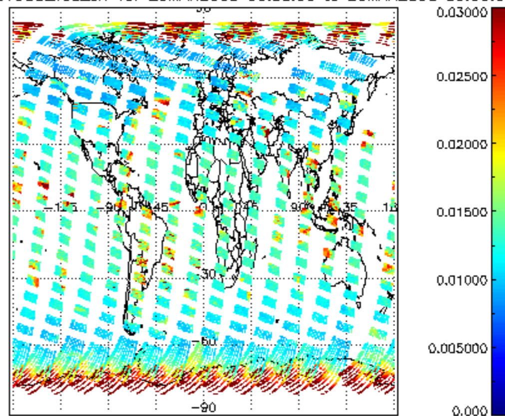
SCIOL2P_NADUV003_vcd_err for 25MAR2008 00:00:00 to 26MAR2008 00:00:00
