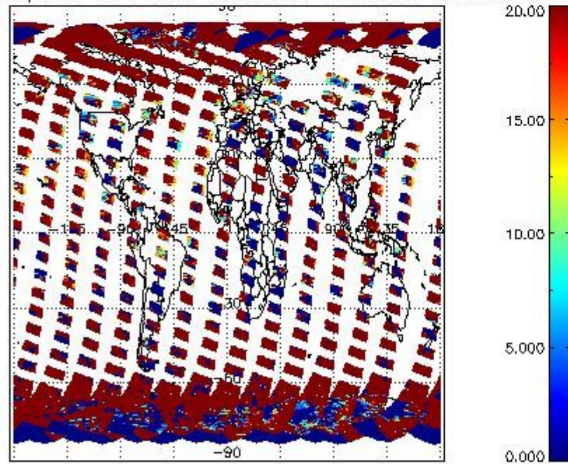
cLopt_depth for 25MAR2008 00:00:00 to 26MAR2008 00:00:00
