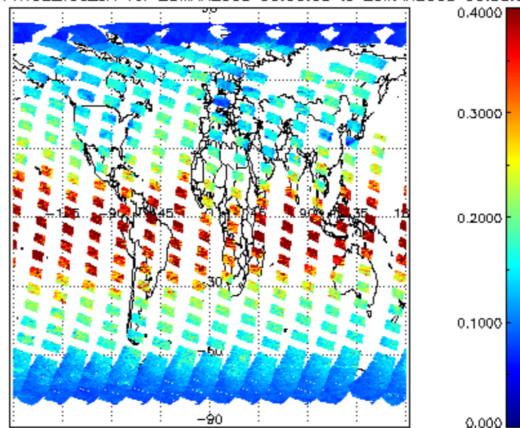
CIOL2P_NADUV1NO2_vcd_err for 25MAR2008 00:00:00 to 26MAR2008 00:00:00
