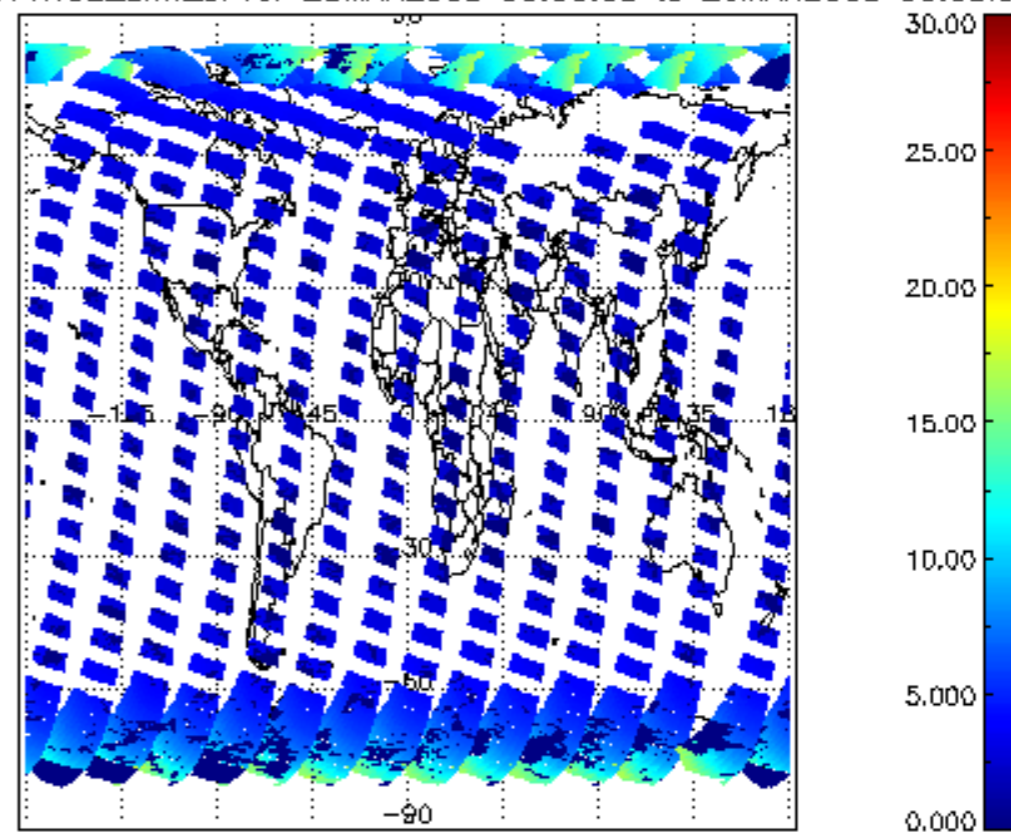
CIOL2P_NADUV1NO2_amf_cl for 25MAR2008 00:00:00 to 26MAR2008 00:00:00
