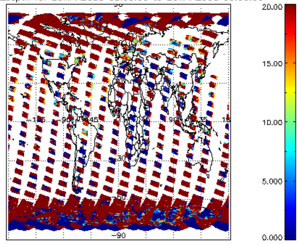
cL_opt_depth for 25MAR2008 00:00:00 to 26MAR2008 00:00:00
