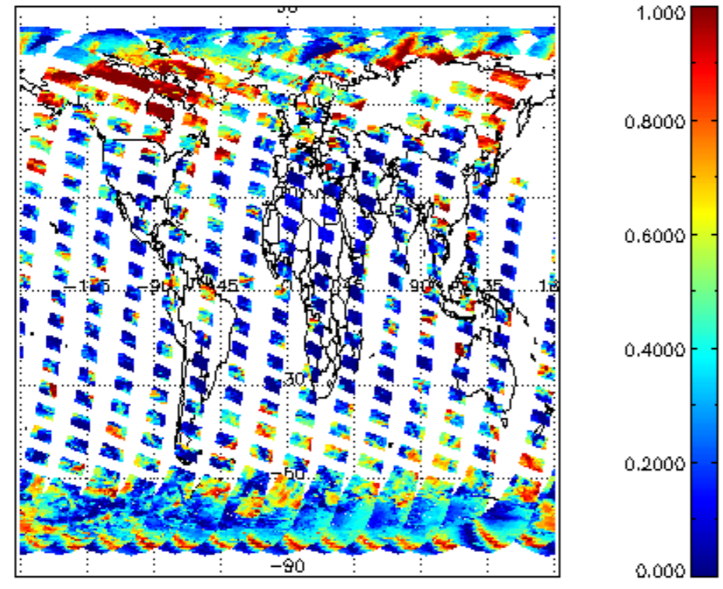
cL_frac for 25MAR2008 00:00:00 to 26MAR2008 00:00:00
