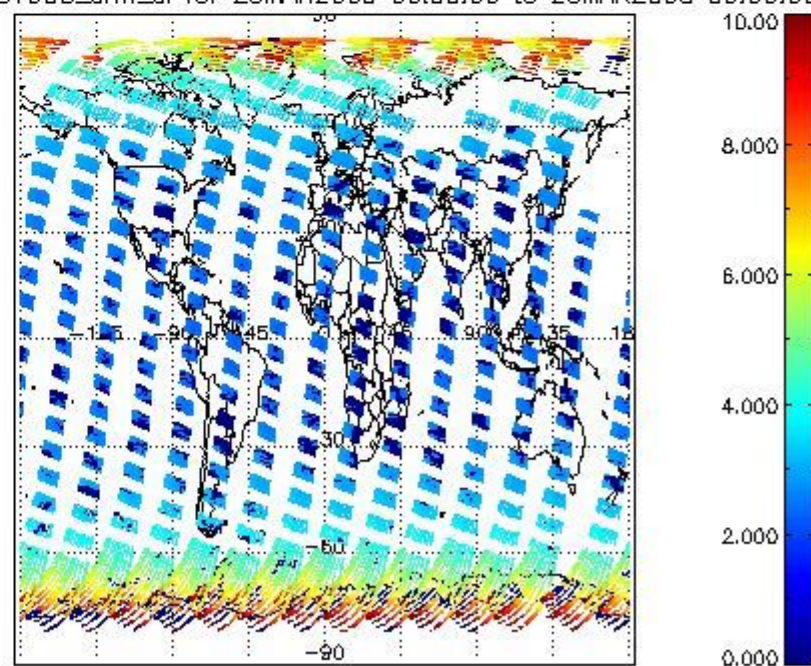
SCIOL2P_NADUV003_amf_gr for 25MAR2008 00:00:00 to 26MAR2008 00:00:00 SCIOL2P_NADUV003_amf_cl for 25MAR2008 00:00:00 to 26MAR2008 00:00:00
