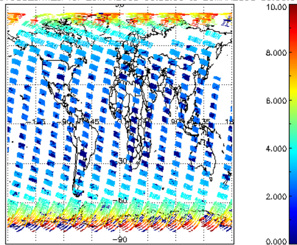
SCIOL2P_NADUV003_amf_cl for 25MAR2008 00:00:00 to 26MAR2008 00:00:00
