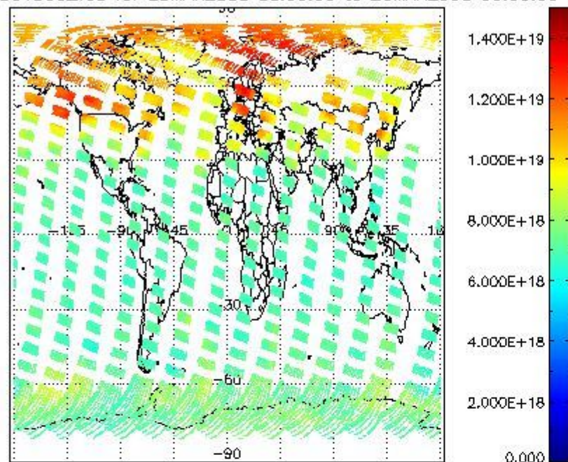
SCIOL2P_NADUV003_vcd for 25MAR2008 00:00:00 to 26MAR2008 00:00:00 SCIOL2P_NADUV003_vcd_err for 25MAR2008 00:00:00 to 26MAR2008 00:00:00
