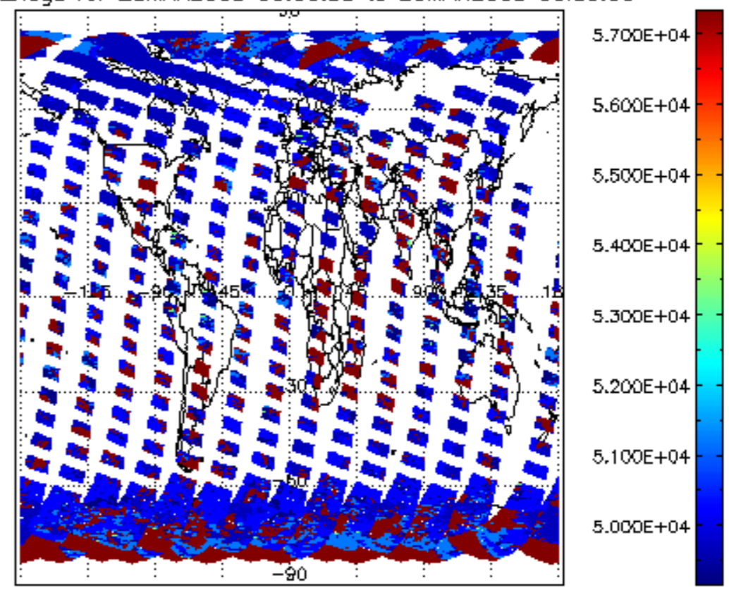
cloud_flags for 25MAR2008 00:00:00 to 26MAR2008 00:00:00
