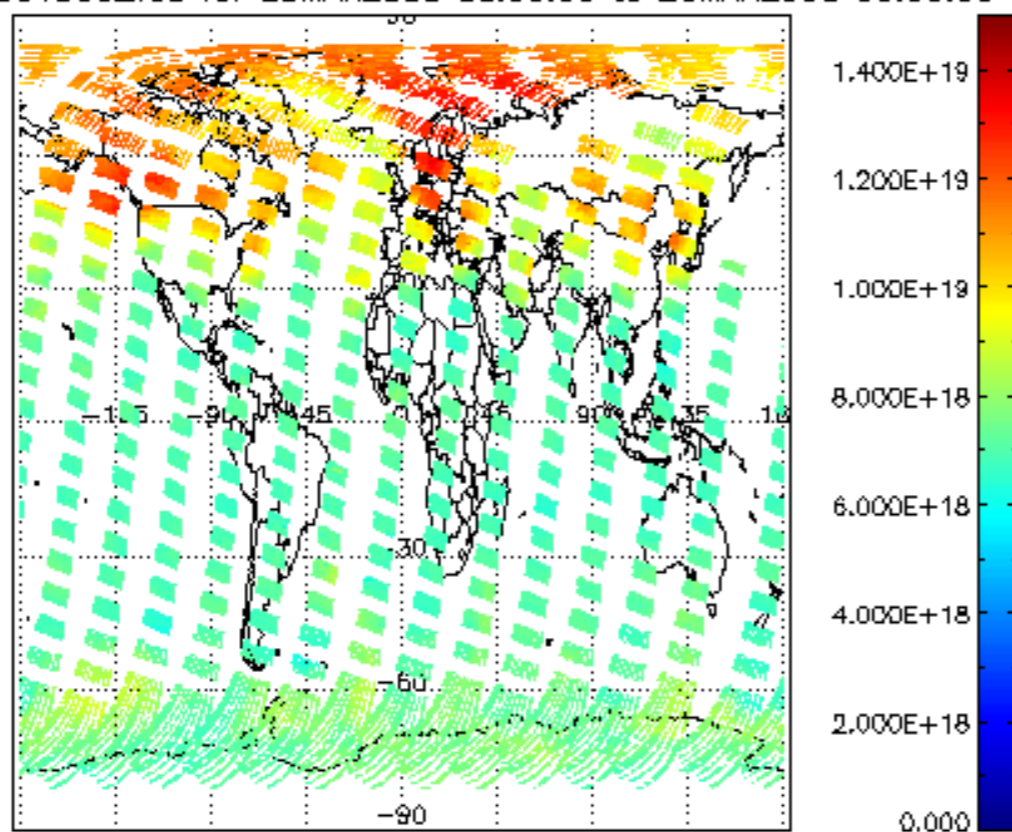
SCIOL2P_NADUV003_vcd for 25MAR2008 00:00:00 to 26MAR2008 00:00:00
