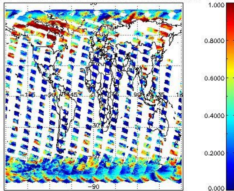
cLfrac for 25MAR2008 00:00:00 to 26MAR2008 00:00:00
