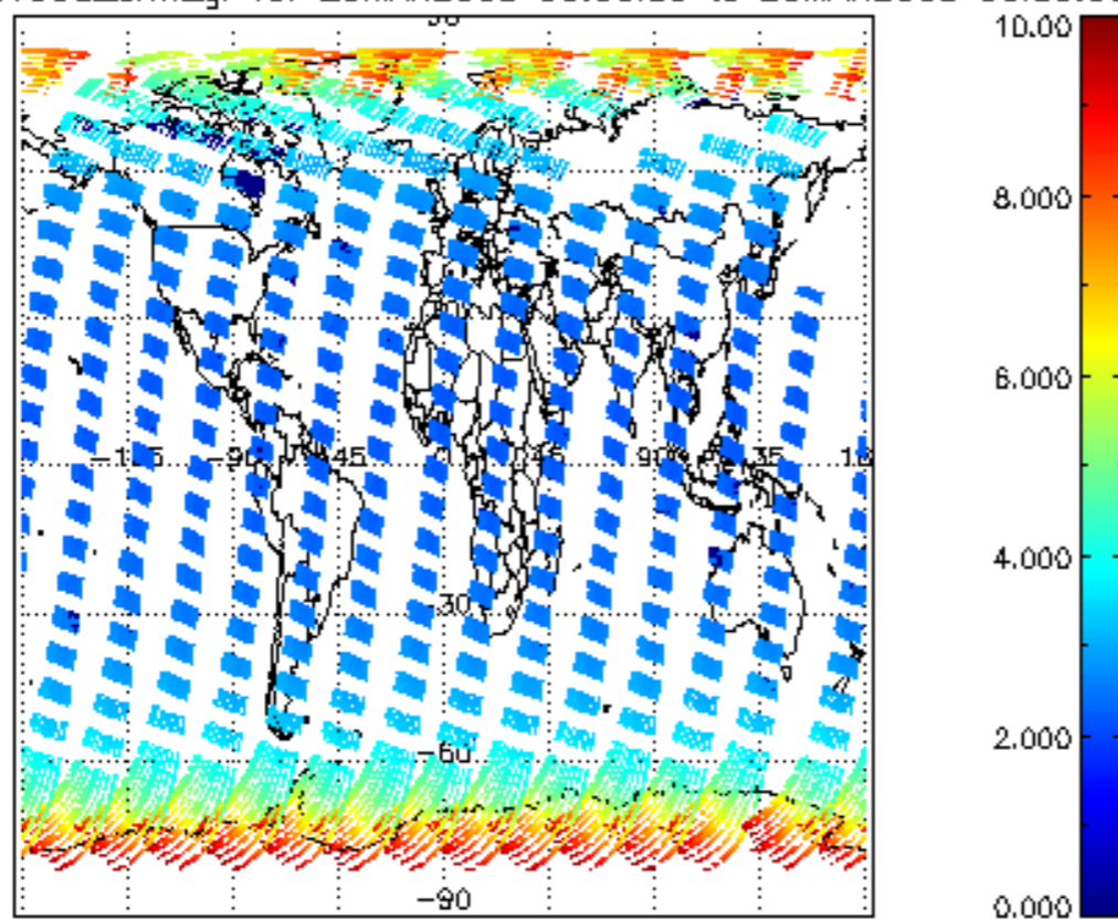
SCIOL2P_NADUV003_amf_gr for 25MAR2008 00:00:00 to 26MAR2008 00:00:00
