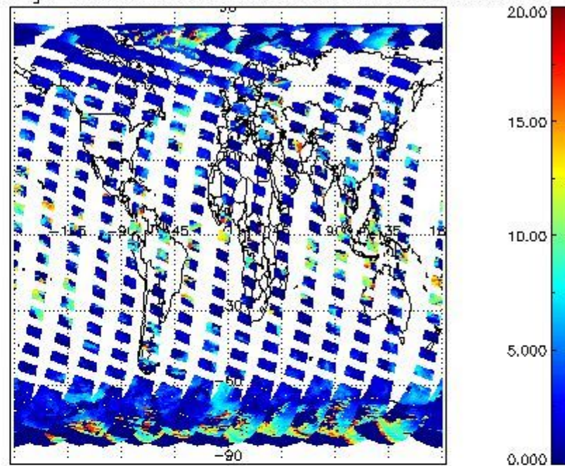
cLtop_height for 25MAR2008 00:00:00 to 26MAR2008 00:00:00
