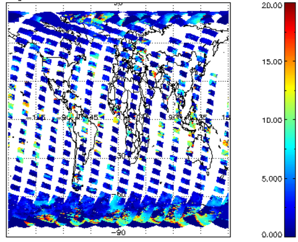
cL_top_height for 25MAR2008 00:00:00 to 26MAR2008 00:00:00
