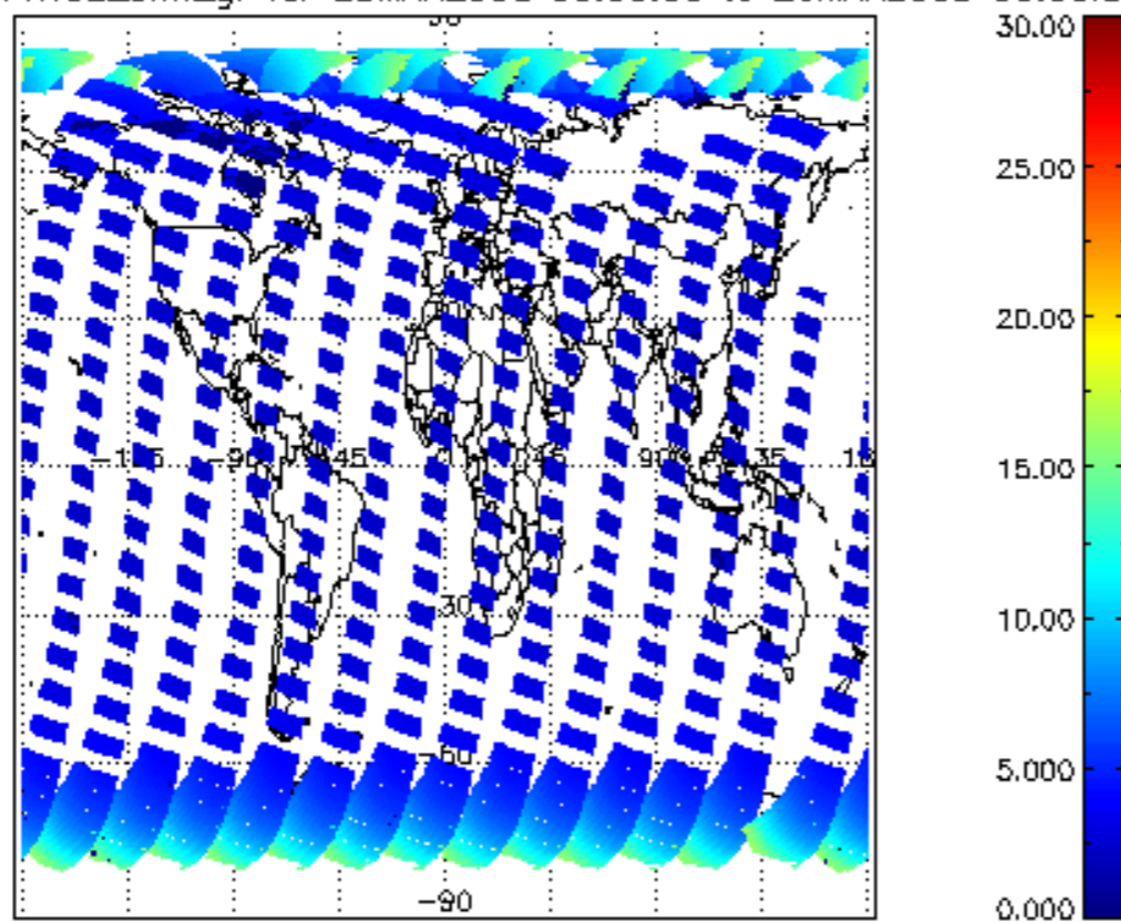
CIOL2P_NADUV1NO2_amf_gr for 25MAR2008 00:00:00 to 26MAR2008 00:00:00
