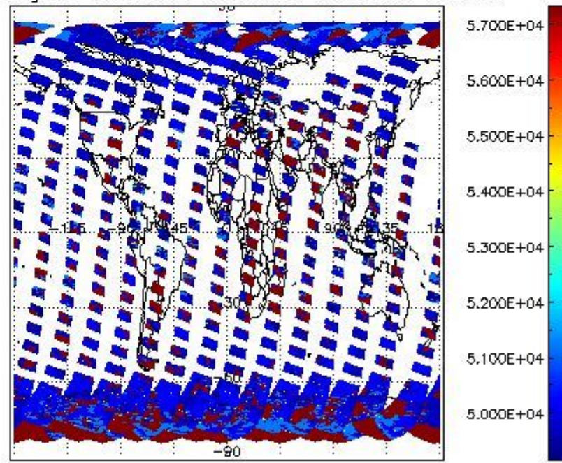
cloud_flags for 25MAR2008 00:00:00 to 26MAR2008 00:00:00
