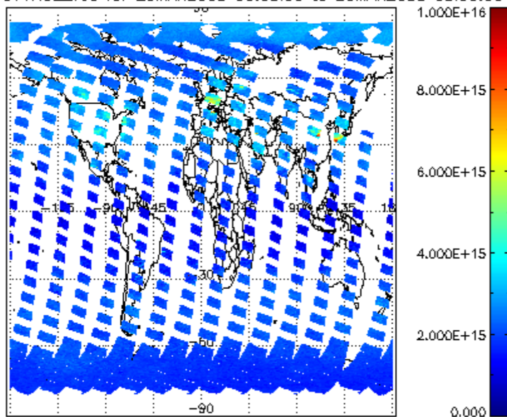
SCIOL2P_NADUV1NO2_vcd for 25MAR2008 00:00:00 to 26MAR2008 00:00:00
