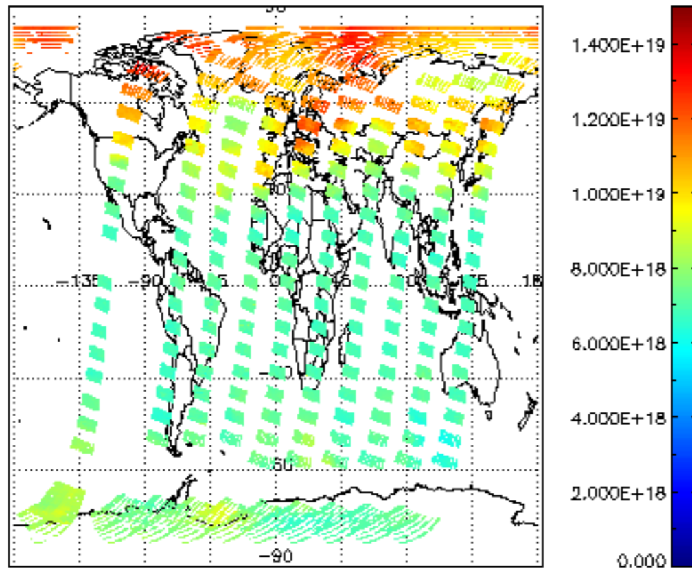
SCIOL2P_NADUV003_vcd for 20MAR2008 00:00:00 to 21MAR2008 00:00:00
