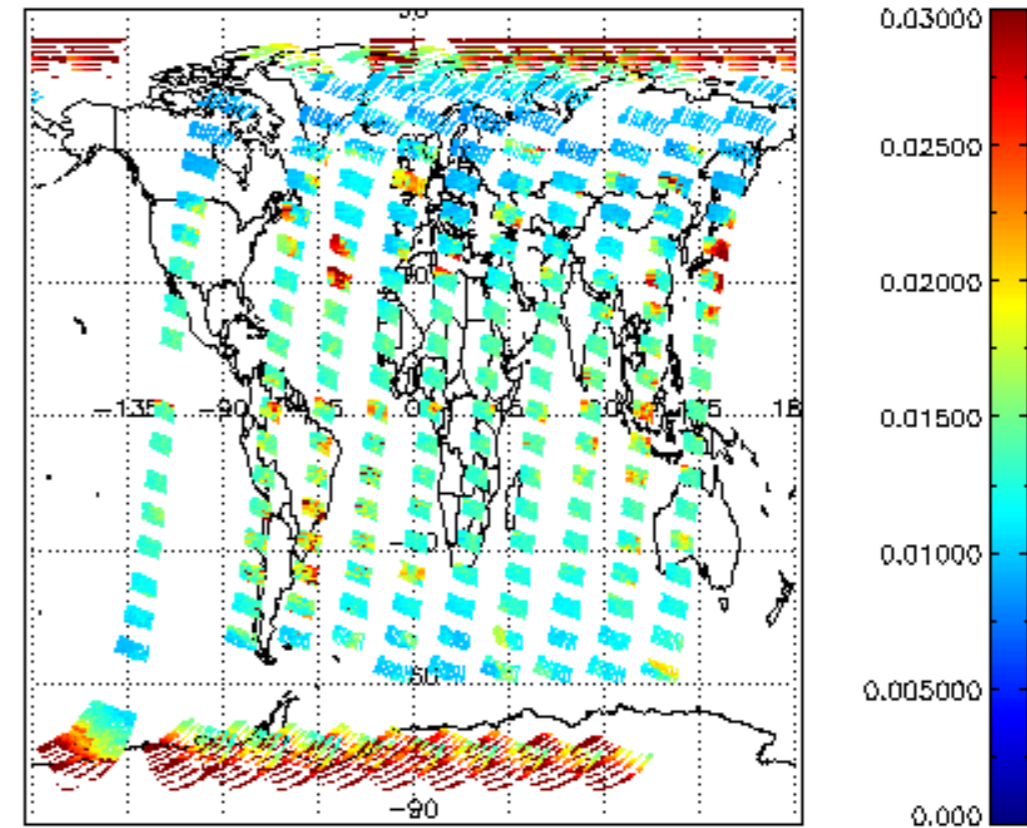
SCIOL2P_NADUV003_vcd_err for 20MAR2008 00:00:00 to 21MAR2008 00:00:00
