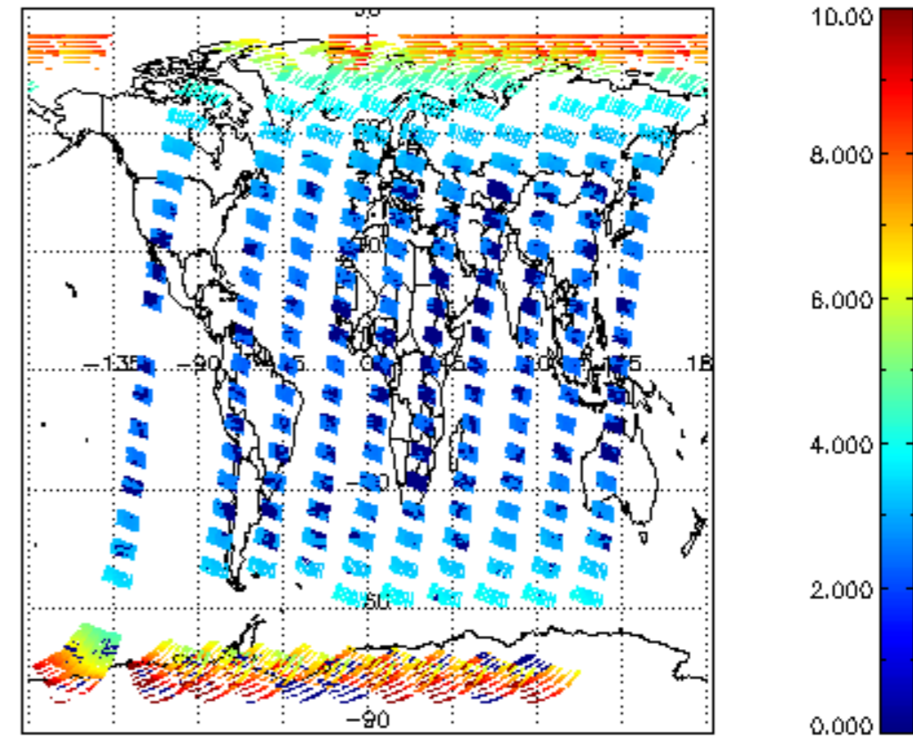
SCIOL2P_NADUV003_amf_cl for 20MAR2008 00:00:00 to 21MAR2008 00:00:00
