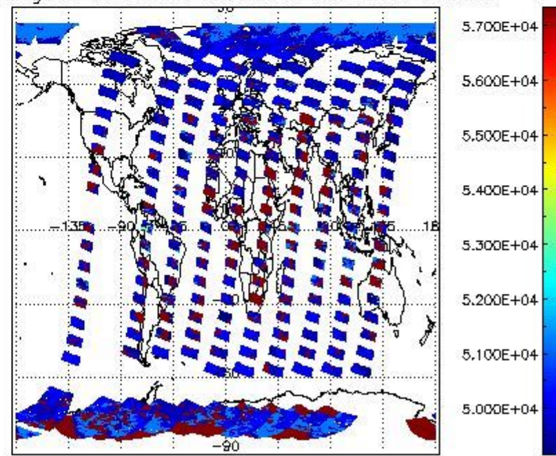
cloud_flags for 20MAR2008 00:00:00 to 21MAR2008 00:00:00
