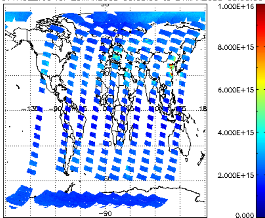
SCIOL2P_NADUV1NO2_vcd for 20MAR2008 00:00:00 to 21MAR2008 00:00:00
