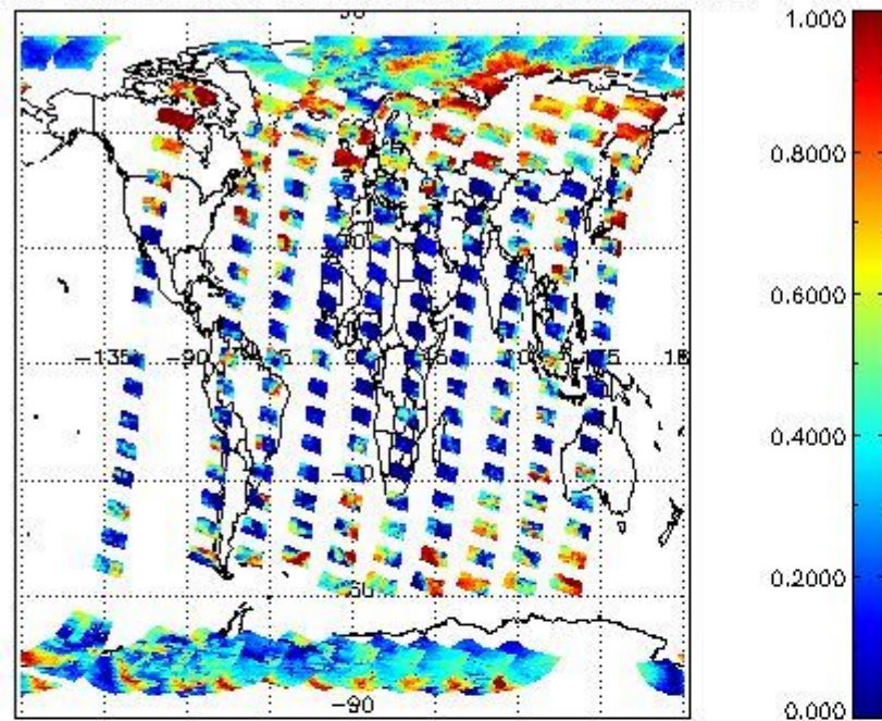
cLfrac for 20MAR2008 00:00:00 to 21MAR2008 00:00:00
