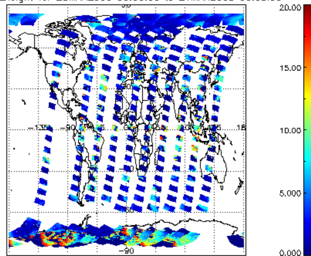
cL_top_height for 20MAR2008 00:00:00 to 21MAR2008 00:00:00
