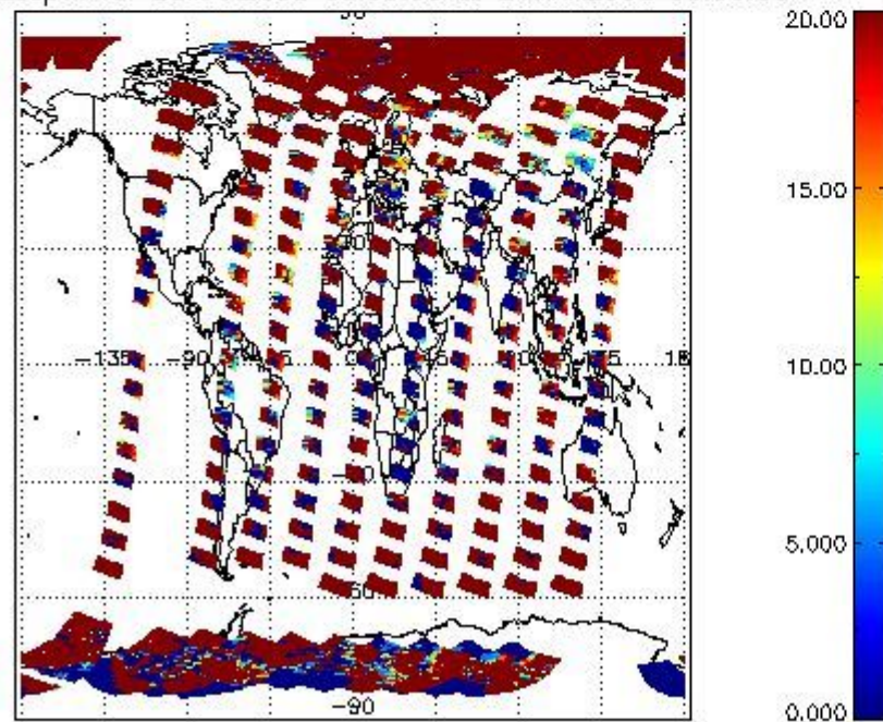
cLopt_depth for 20MAR2008 00:00:00 to 21MAR2008 00:00:00
