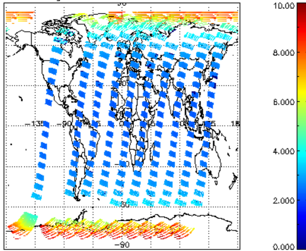
SCIOL2P_NADUV003_amf_gr for 20MAR2008 00:00:00 to 21MAR2008 00:00:00
