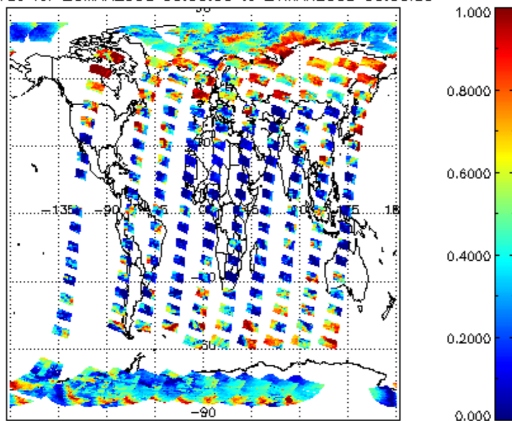
cL_frac for 20MAR2008 00:00:00 to 21MAR2008 00:00:00
