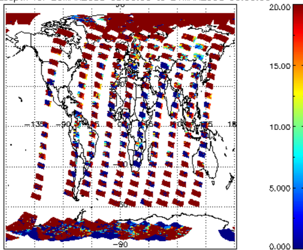
cL_opt_depth for 20MAR2008 00:00:00 to 21MAR2008 00:00:00
