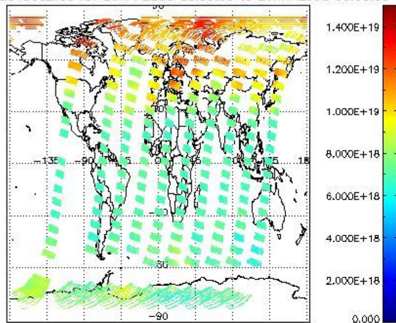
SCIOL2P_NADUV003_vcd for 20MAR2008 00:00:00 to 21MAR2008 00:00:00 SCIOL2P_NADUV003_vcd_err for 20MAR2008 00:00:00 to 21MAR2008 00:00:00
