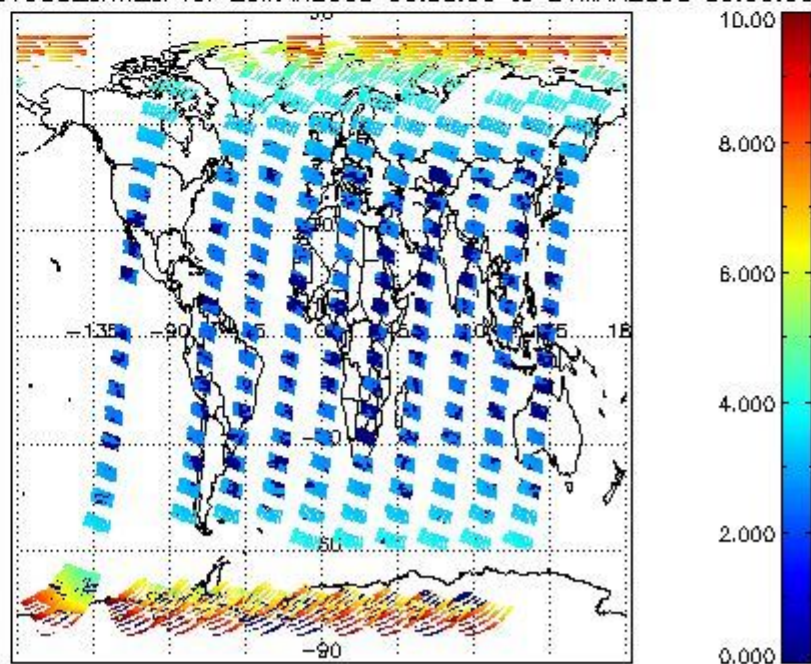
SCIOL2P_NADUV003_amf_gr for 20MAR2008 00:00:00 to 21MAR2008 00:00:00 SCIOL2P_NADUV003_amf_cl for 20MAR2008 00:00:00 to 21MAR2008 00:00:00
