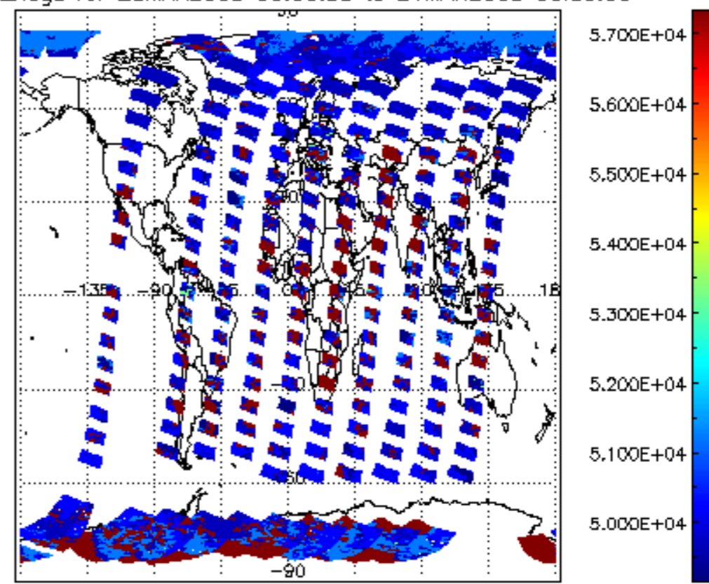
cloud_flags for 20MAR2008 00:00:00 to 21MAR2008 00:00:00
