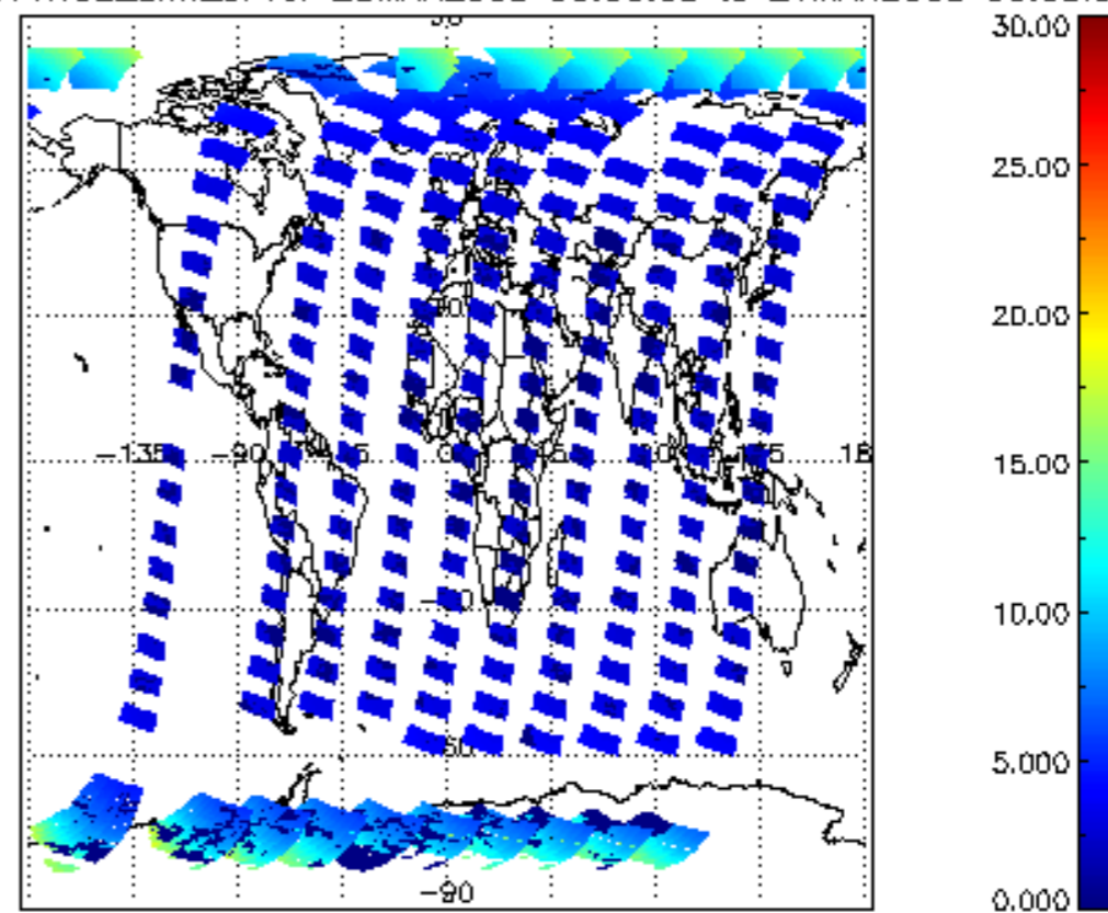
SCIOL2P_NADUV1NO2_amf_cl for 20MAR2008 00:00:00 to 21MAR2008 00:00:00
