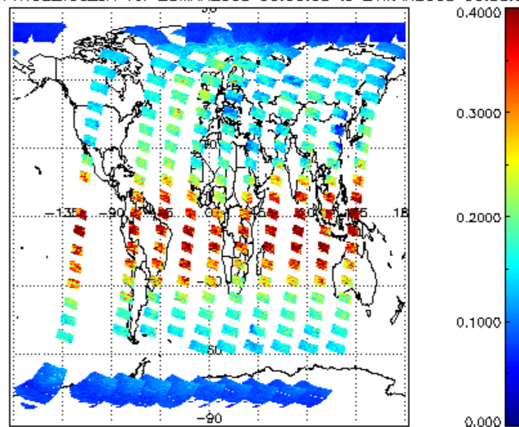
SCIOL2P_NADUV1NO2_vcd_err for 20MAR2008 00:00:00 to 21MAR2008 00:00:00
