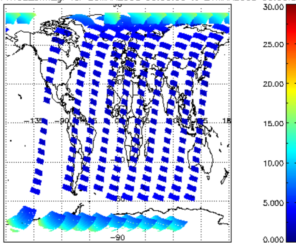
SCIOL2P_NADUV1NO2_amf_gr for 20MAR2008 00:00:00 to 21MAR2008 00:00:00
