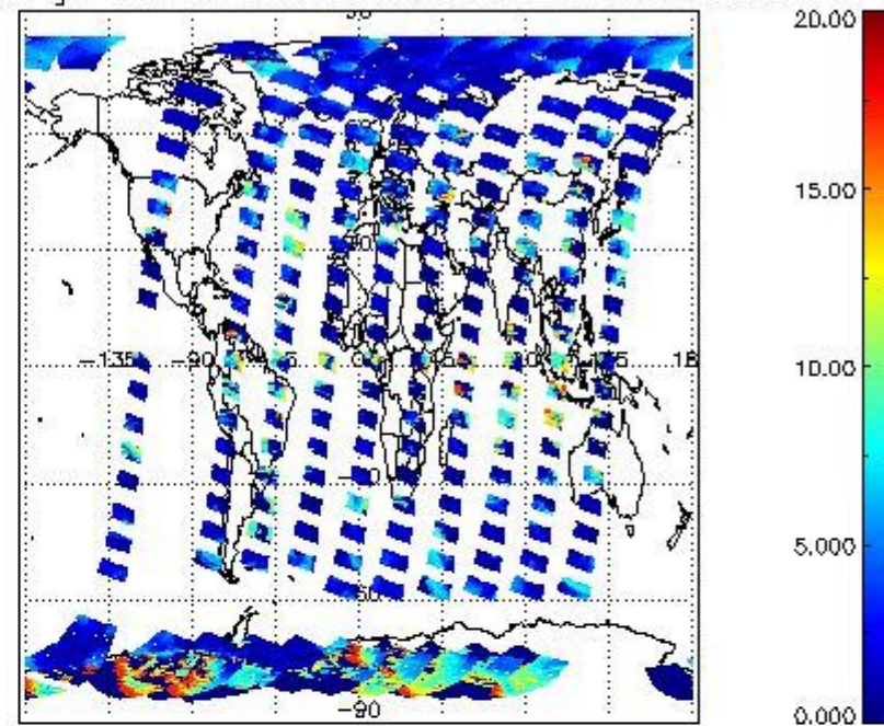
cLtop_height for 20MAR2008 00:00:00 to 21MAR2008 00:00:00
