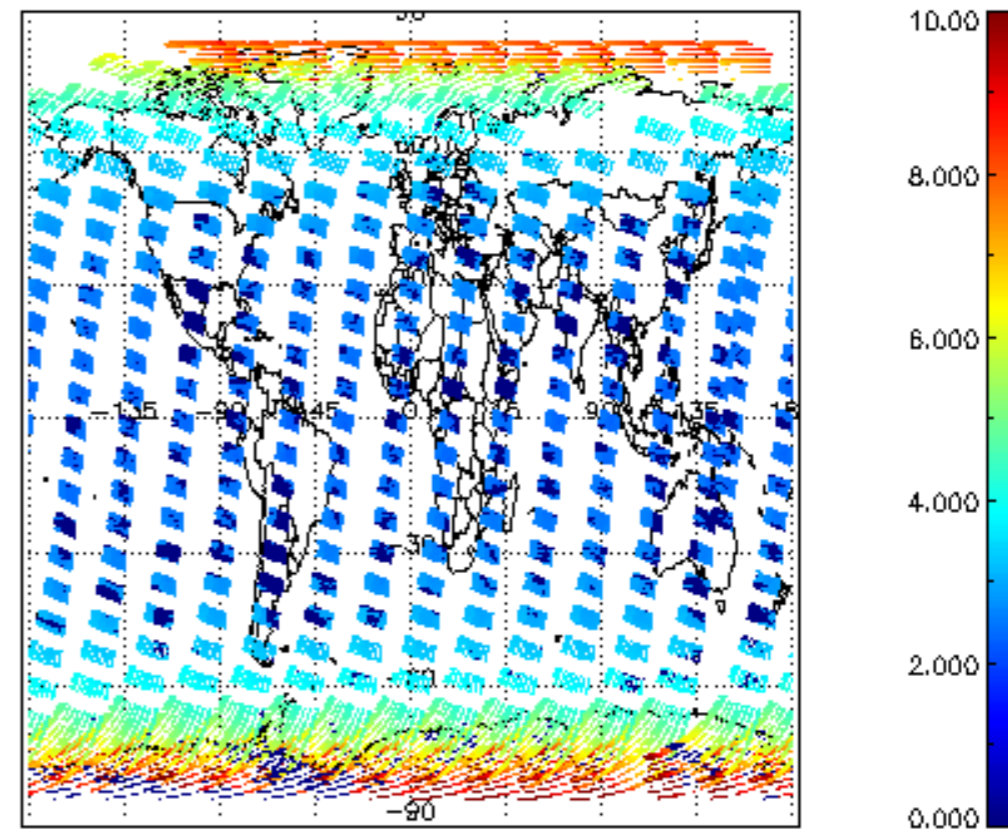
SCIOL2P_NADUV003_amf_cl for 15MAR2008 00:00:00 to 16MAR2008 00:00:00
