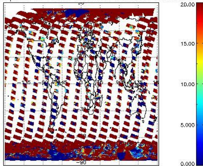
cLopt_depth for 15MAR2008 00:00:00 to 16MAR2008 00:00:00
