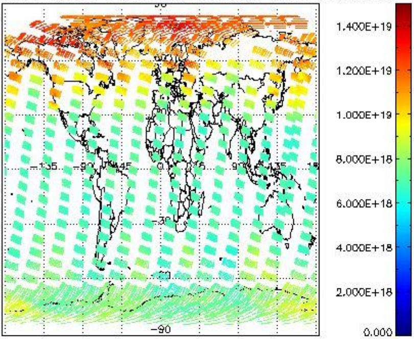
SCIOL2P_NADUV003_vcd for 15MAR2008 00:00:00 to 16MAR2008 00:00:00
