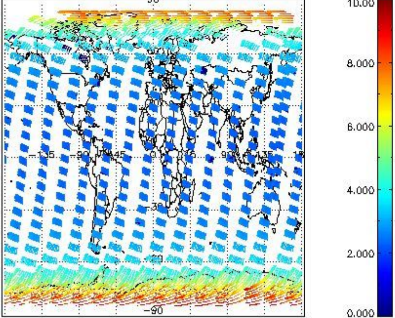
SCIOL2P_NADUV003_amf_gr for 15MAR2008 00:00:00 to 16MAR2008 00:00:00
