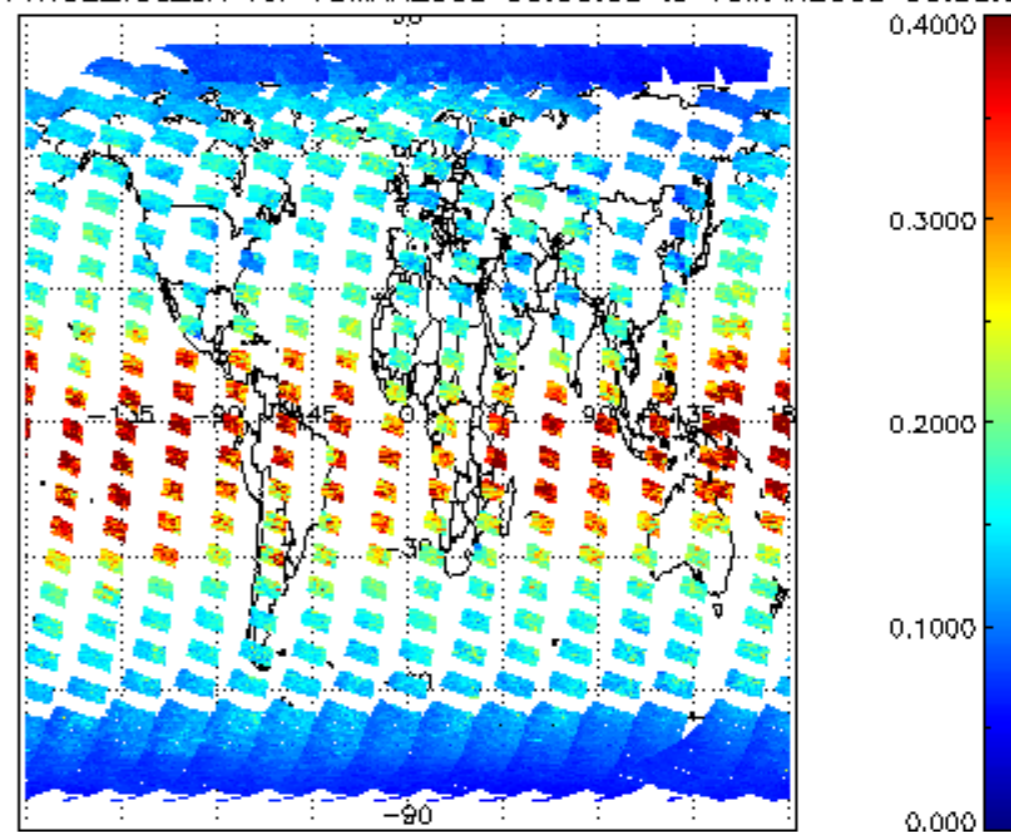
CIOL2P_NADUV1NO2_vcd_err for 15MAR2008 00:00:00 to 16MAR2008 00:00:00
