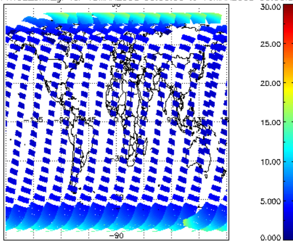
CIOL2P_NADUV1NO2_amf_gr for 15MAR2008 00:00:00 to 16MAR2008 00:00:00
