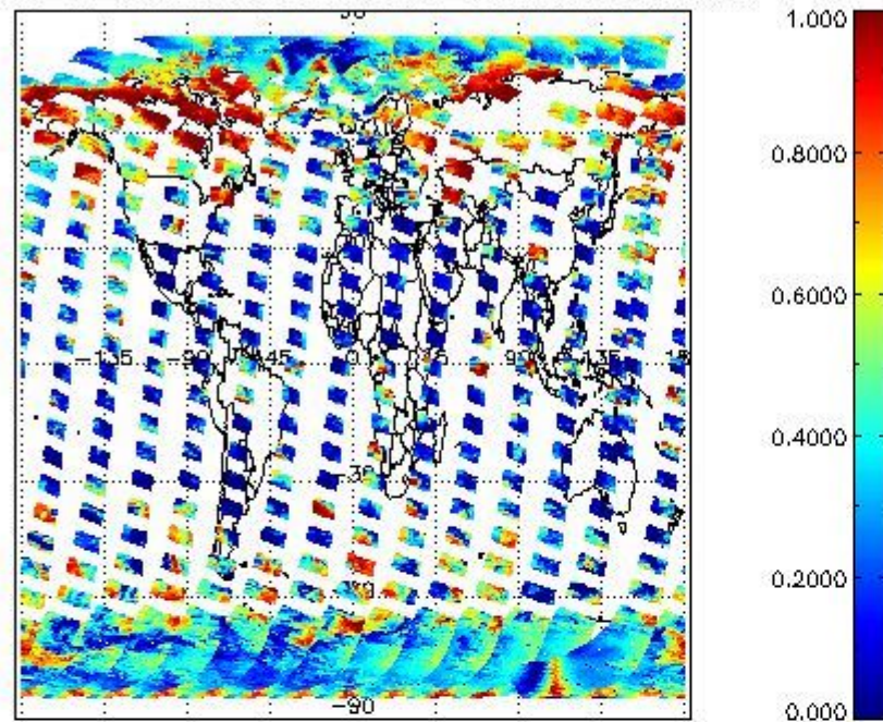
cLfrac for 15MAR2008 00:00:00 to 16MAR2008 00:00:00
