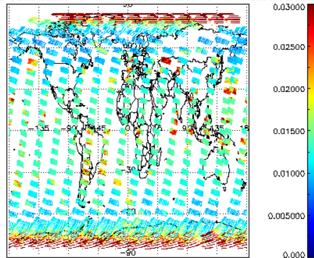
SCIOL2P_NADUV003_vcd_err for 15MAR2008 00:00:00 to 16MAR2008 00:00:00
