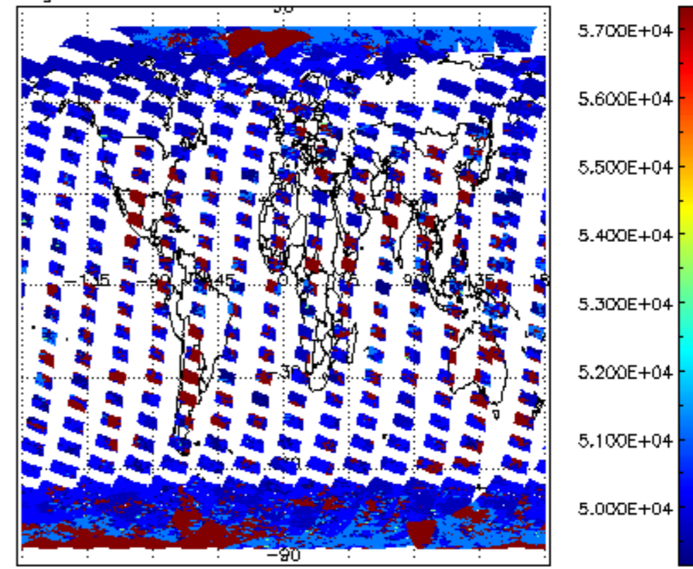
cloud_flags for 15MAR2008 00:00:00 to 16MAR2008 00:00:00
