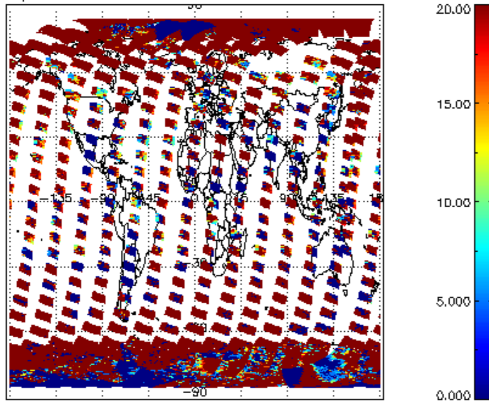
cL_opt_depth for 15MAR2008 00:00:00 to 16MAR2008 00:00:00
