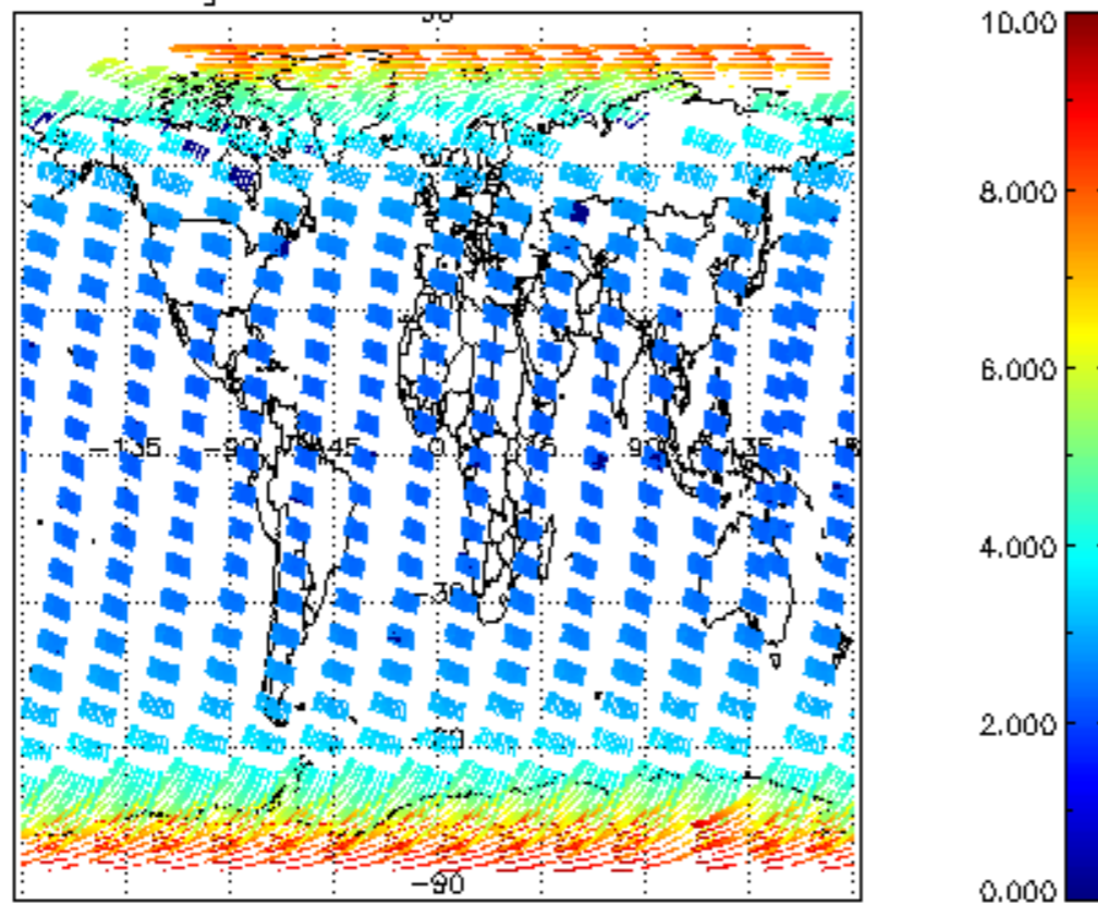
SCIOL2P_NADUV003_amf_gr for 15MAR2008 00:00:00 to 16MAR2008 00:00:00
