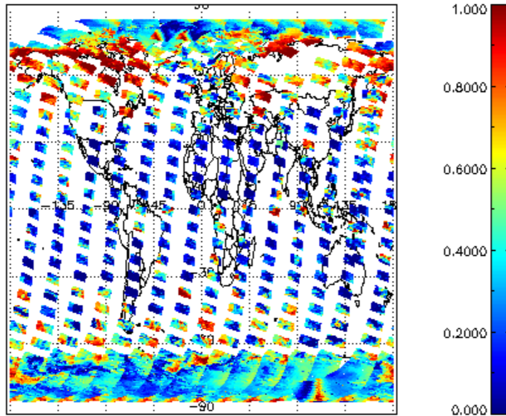
cL_frac for 15MAR2008 00:00:00 to 16MAR2008 00:00:00
