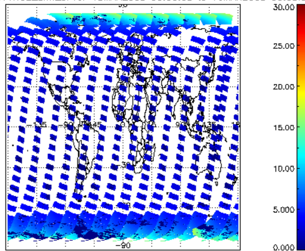
CIOL2P_NADUV1NO2_amf_cl for 15MAR2008 00:00:00 to 16MAR2008 00:00:00
