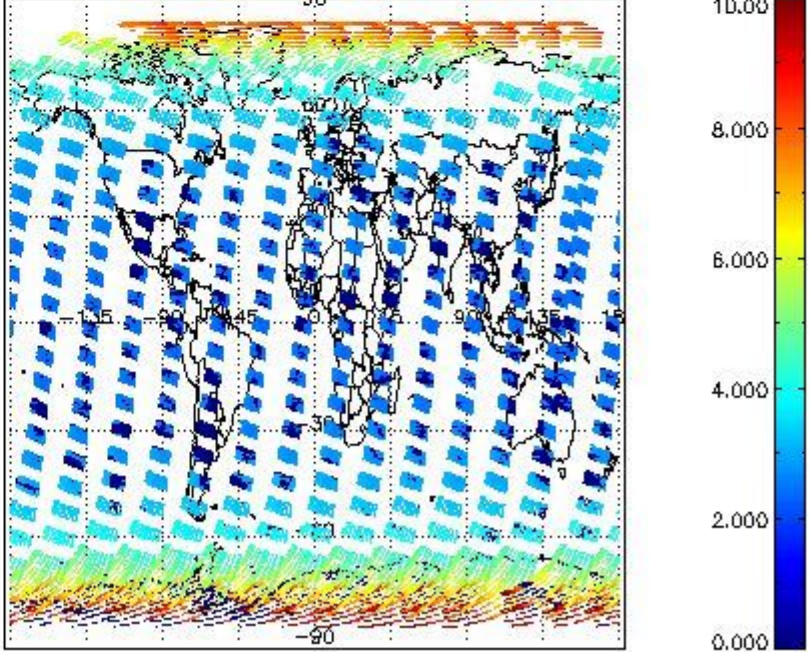
SCIOL2P_NADUV003_amf_cl for 15MAR2008 00:00:00 to 16MAR2008 00:00:00
