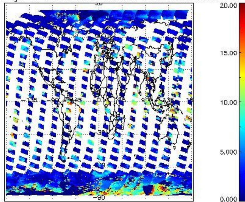
cLtop_height for 15MAR2008 00:00:00 to 16MAR2008 00:00:00
