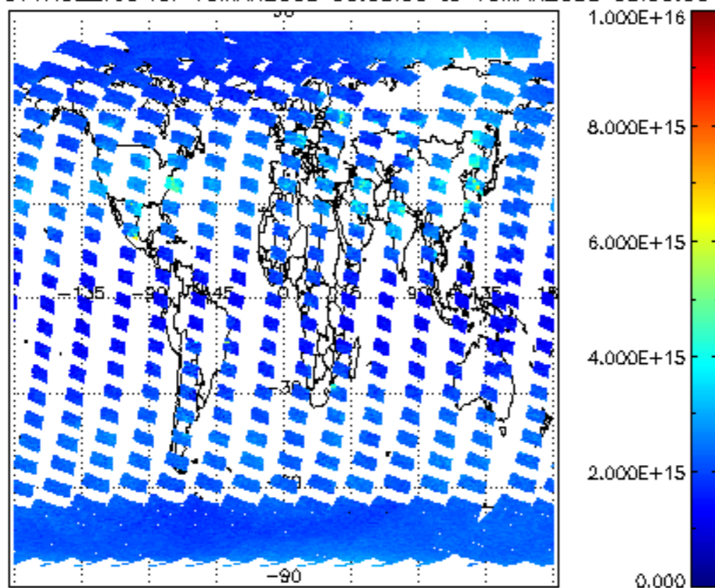
SCIOL2P_NADUV1NO2_vcd for 15MAR2008 00:00:00 to 16MAR2008 00:00:00
