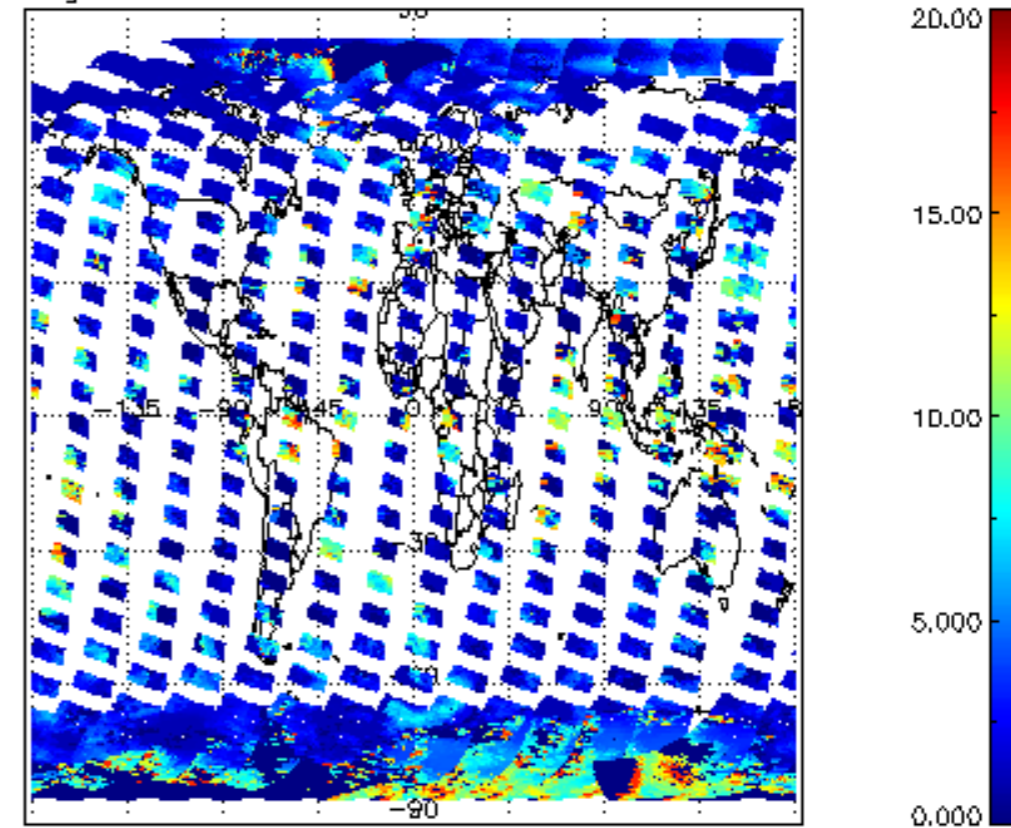
cL_top_height for 15MAR2008 00:00:00 to 16MAR2008 00:00:00
