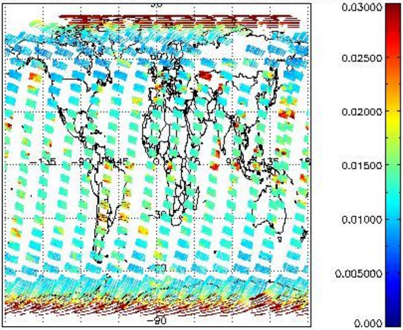
SCIOL2P_NADUV003_vcd_err for 15MAR2008 00:00:00 to 16MAR2008 00:00:00
