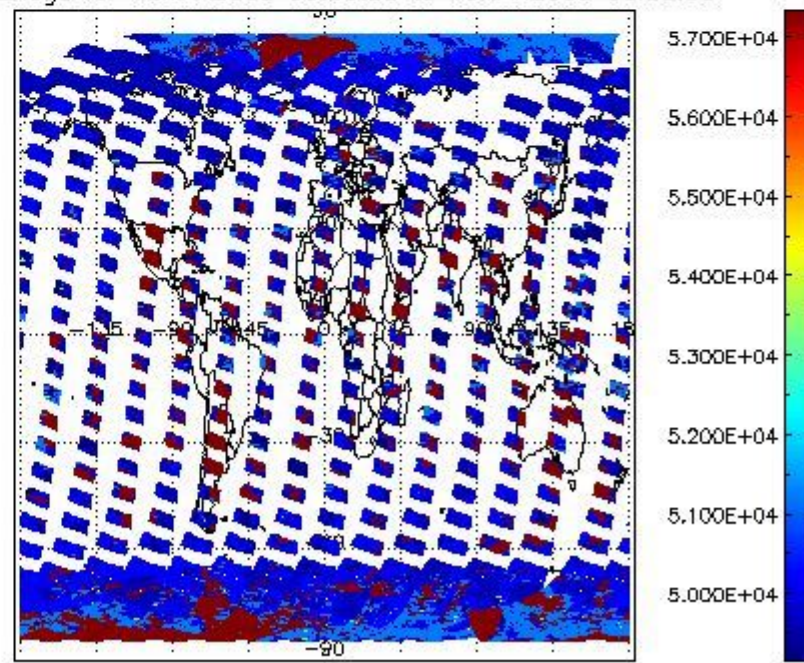
cloud_flags for 15MAR2008 00:00:00 to 16MAR2008 00:00:00
