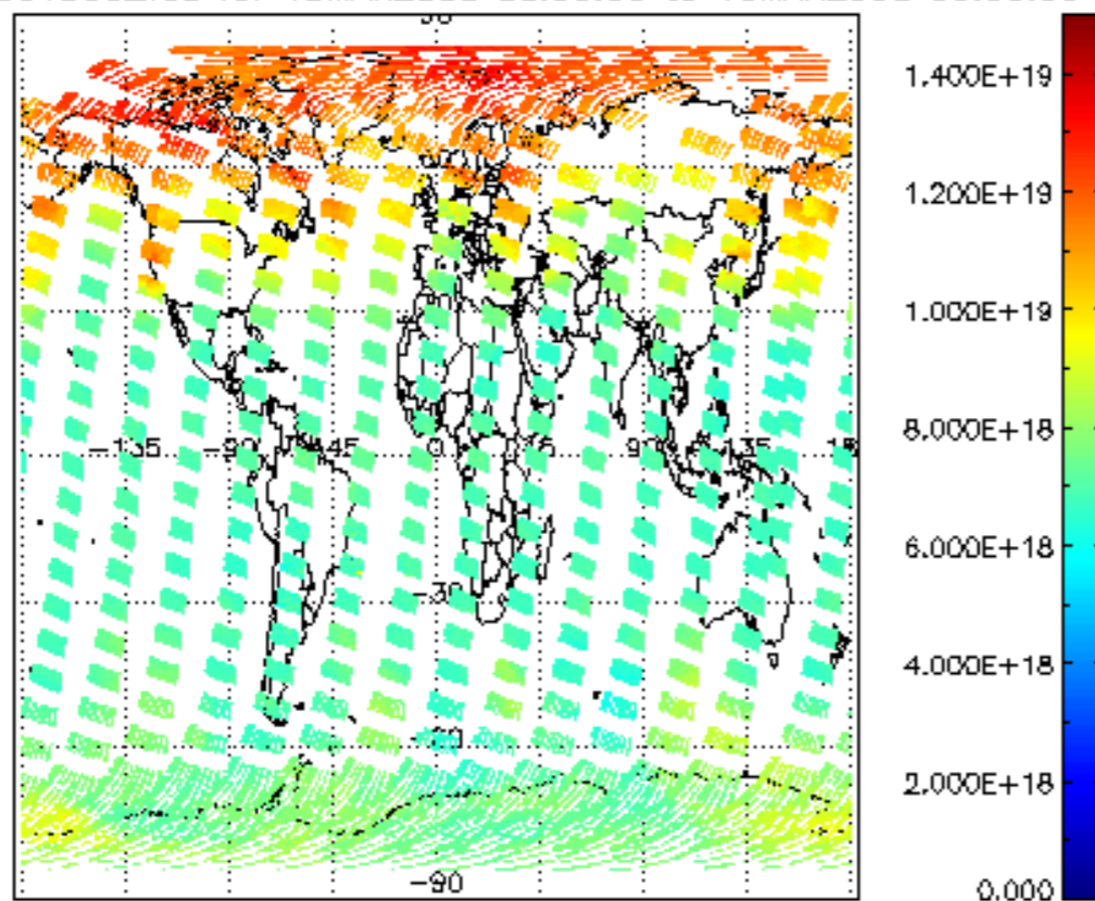
SCIOL2P_NADUV003_vcd for 15MAR2008 00:00:00 to 16MAR2008 00:00:00
