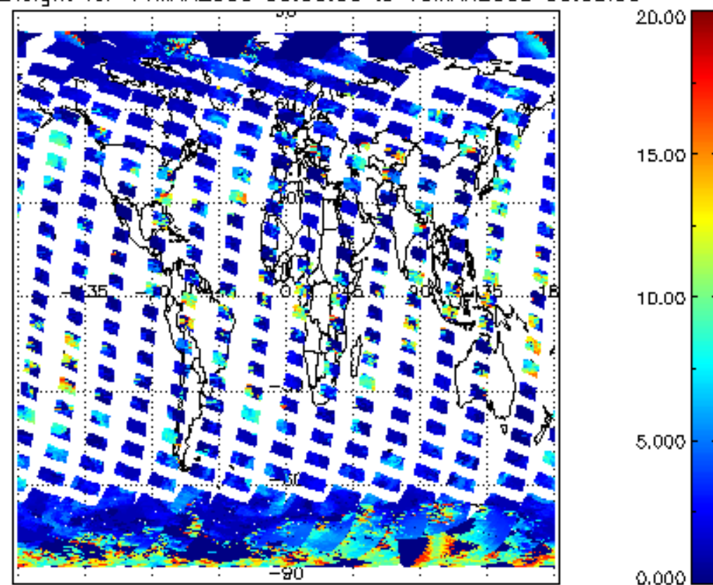
cL_top_height for 14MAR2008 00:00:00 to 15MAR2008 00:00:00
