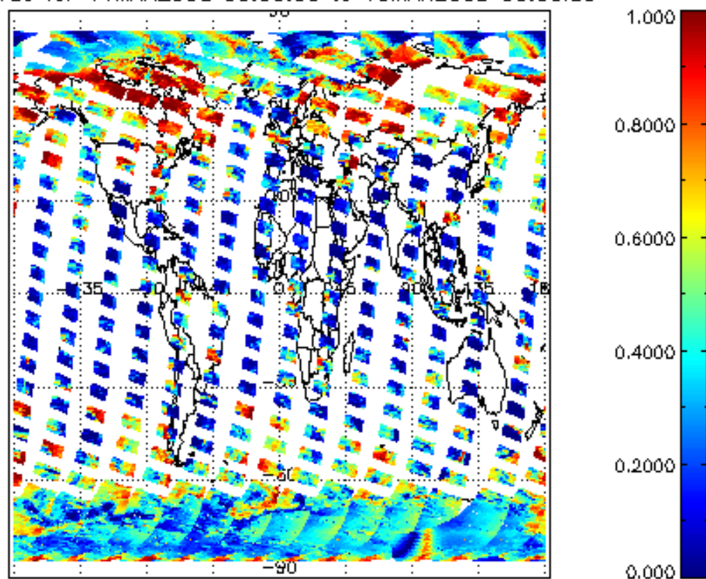
cL_frac for 14MAR2008 00:00:00 to 15MAR2008 00:00:00
