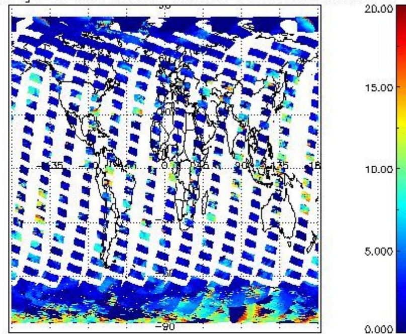
cLtop_height for 14MAR2008 00:00:00 to 15MAR2008 00:00:00
