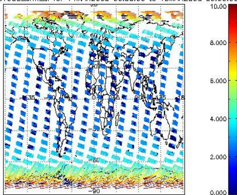
SCIOL2P_NADUV003_amf_gr for 14MAR2008 00:00:00 to 15MAR2008 00:00:00 SCIOL2P_NADUV003_amf_cl for 14MAR2008 00:00:00 to 15MAR2008 00:00:00
