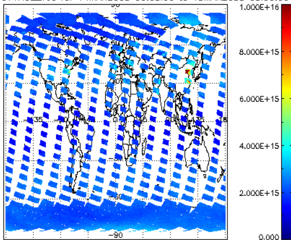
SCIOL2P_NADUV1NO2_vcd for 14MAR2008 00:00:00 to 15MAR2008 00:00:00
