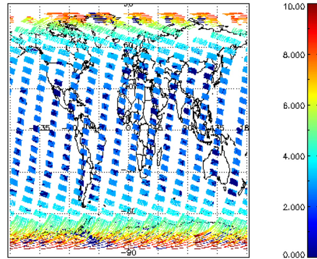
SCIOL2P_NADUV003_amf_cl for 14MAR2008 00:00:00 to 15MAR2008 00:00:00
