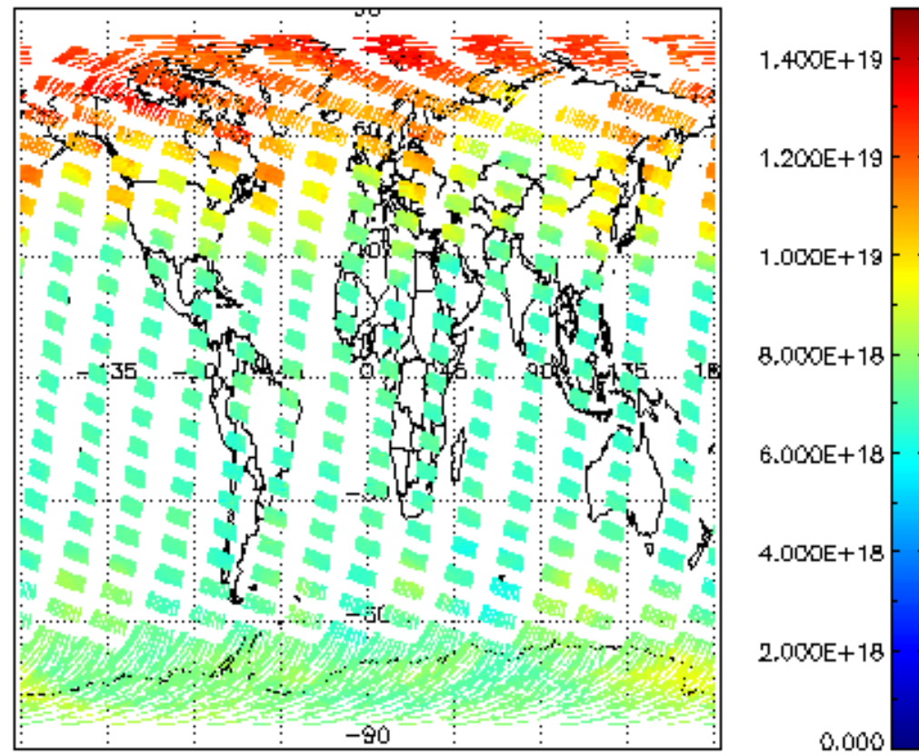
SCIOL2P_NADUV003_vcd for 14MAR2008 00:00:00 to 15MAR2008 00:00:00
