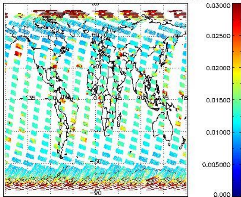
SCIOL2P_NADUV003_vcd for 14MAR2008 00:00:00 to 15MAR2008 00:00:00 SCIOL2P_NADUV003_vcd_err for 14MAR2008 00:00:00 to 15MAR2008 00:00:00
