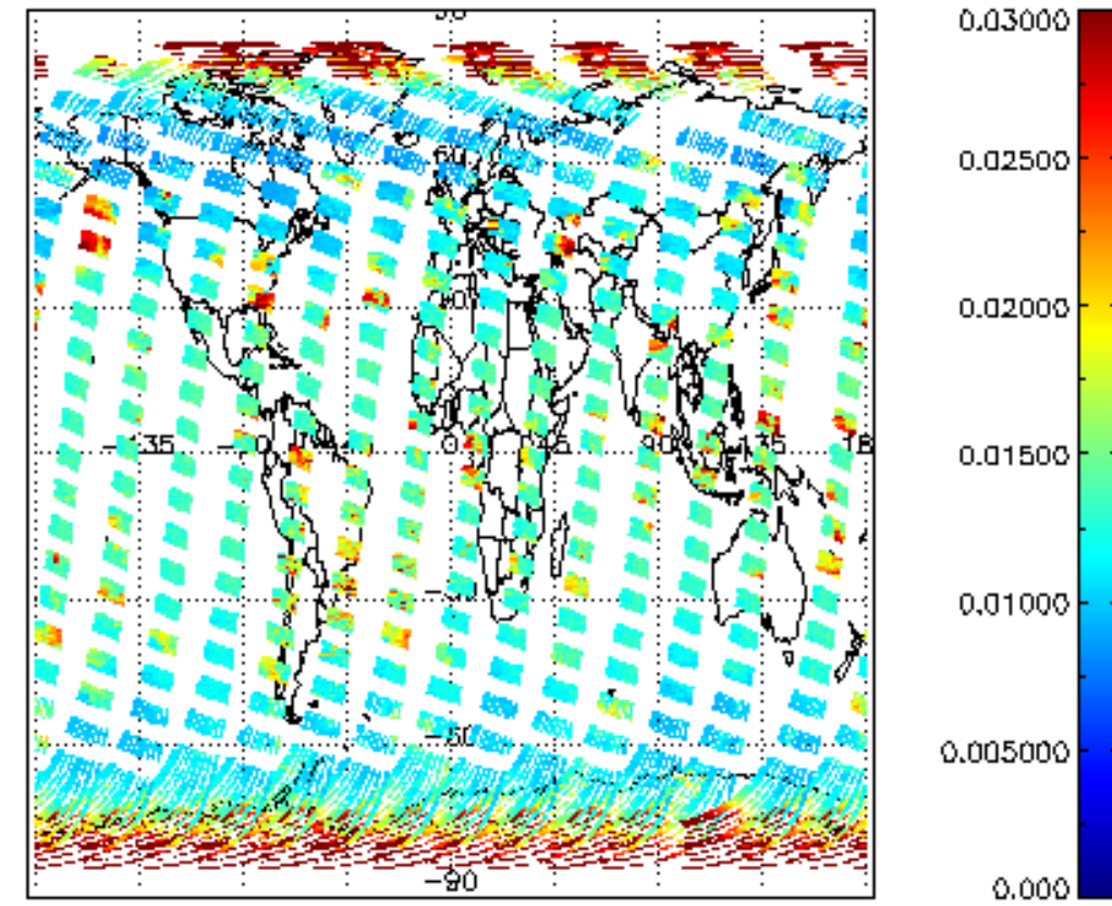
SCIOL2P_NADUV003_vcd_err for 14MAR2008 00:00:00 to 15MAR2008 00:00:00
