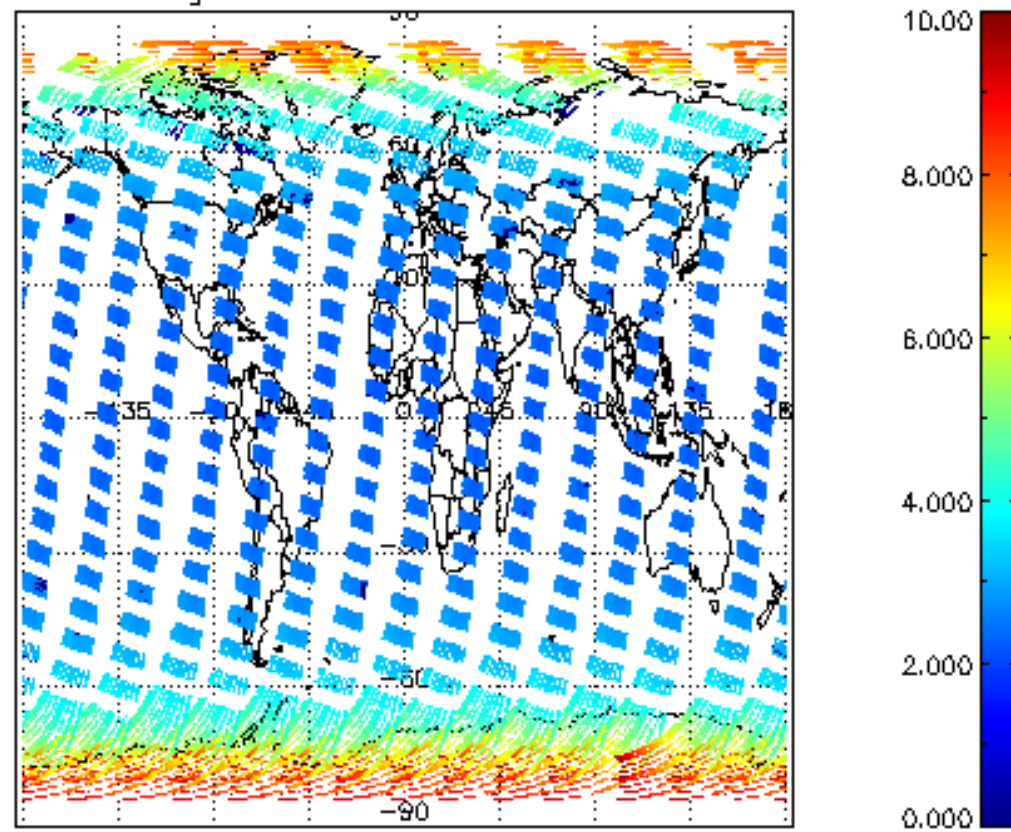
SCIOL2P_NADUV003_amf_gr for 14MAR2008 00:00:00 to 15MAR2008 00:00:00
