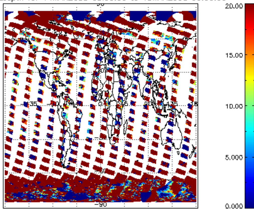
cL_opt_depth for 14MAR2008 00:00:00 to 15MAR2008 00:00:00
