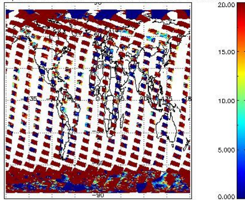
cLopt_depth for 14MAR2008 00:00:00 to 15MAR2008 00:00:00
