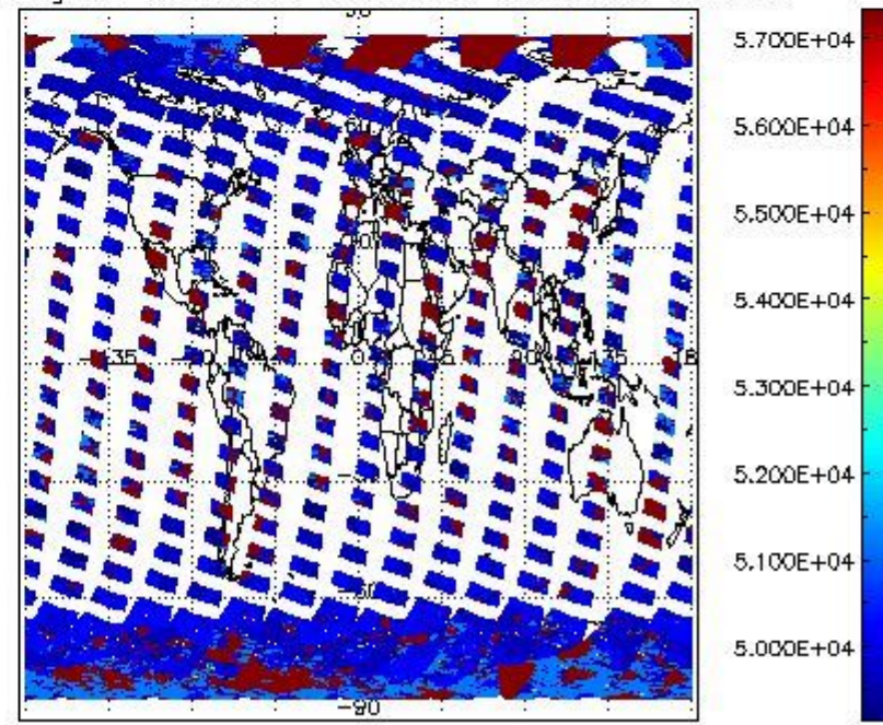
cloud_flags for 14MAR2008 00:00:00 to 15MAR2008 00:00:00
