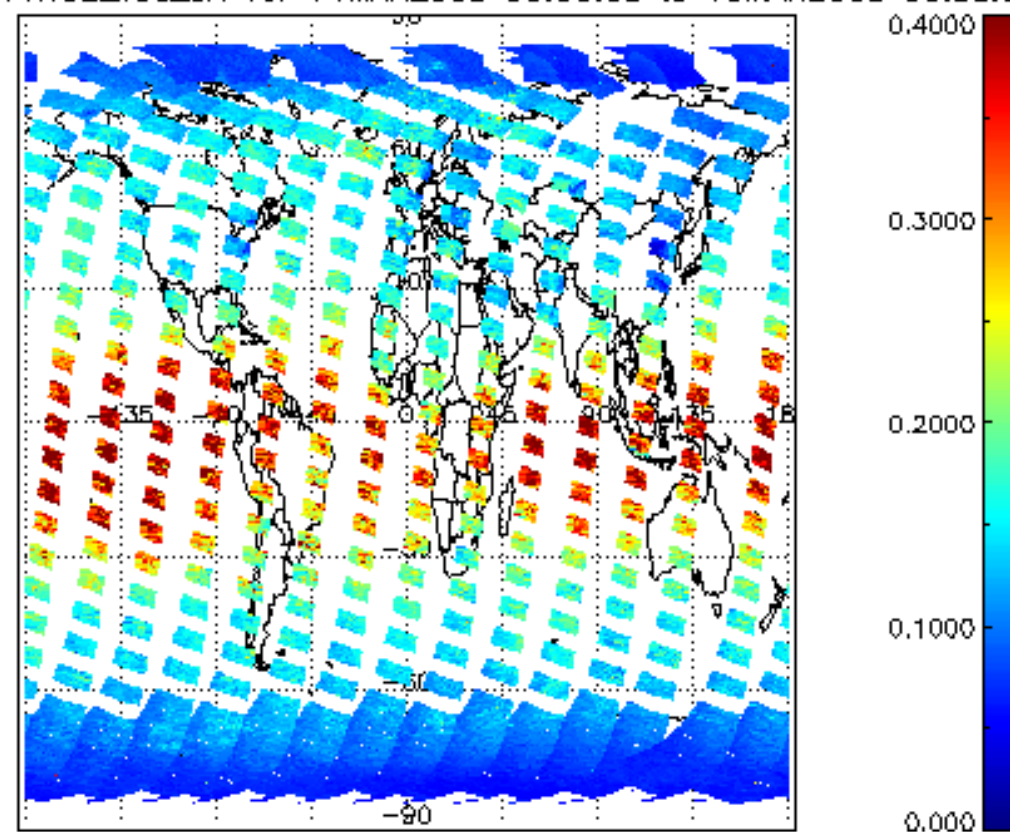
SCIOL2P_NADUV1NO2_vcd_err for 14MAR2008 00:00:00 to 15MAR2008 00:00:00
