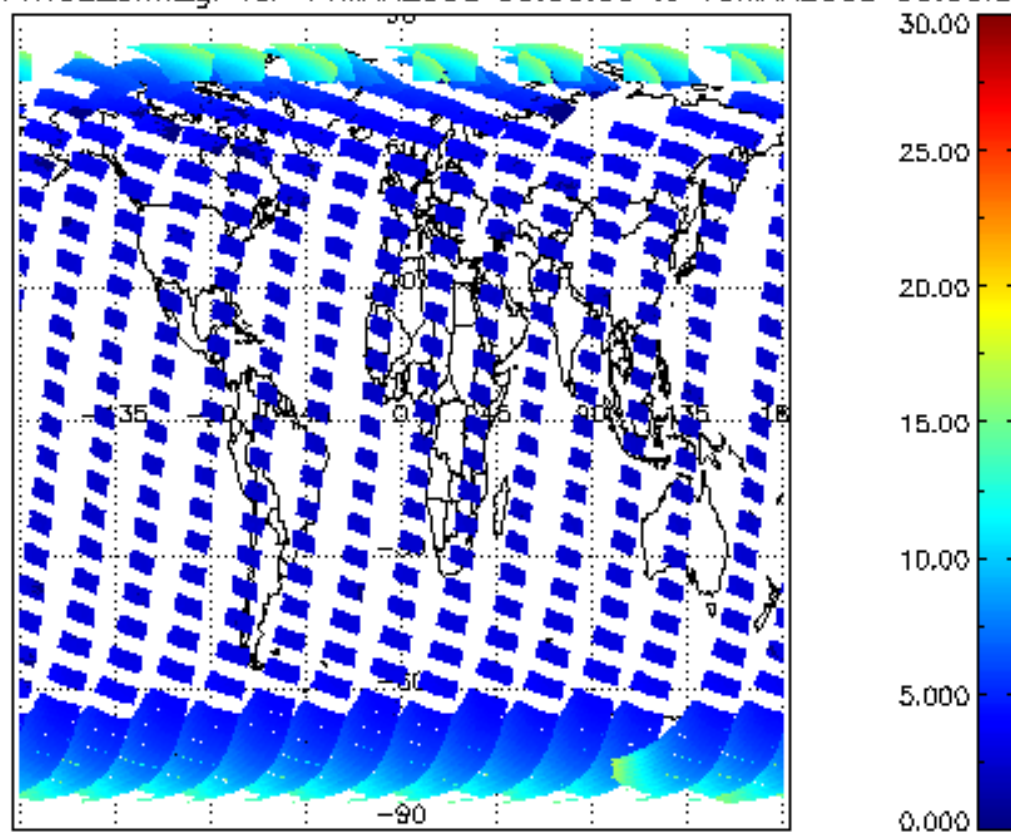
SCIOL2P_NADUV1NO2_amf_gr for 14MAR2008 00:00:00 to 15MAR2008 00:00:00
