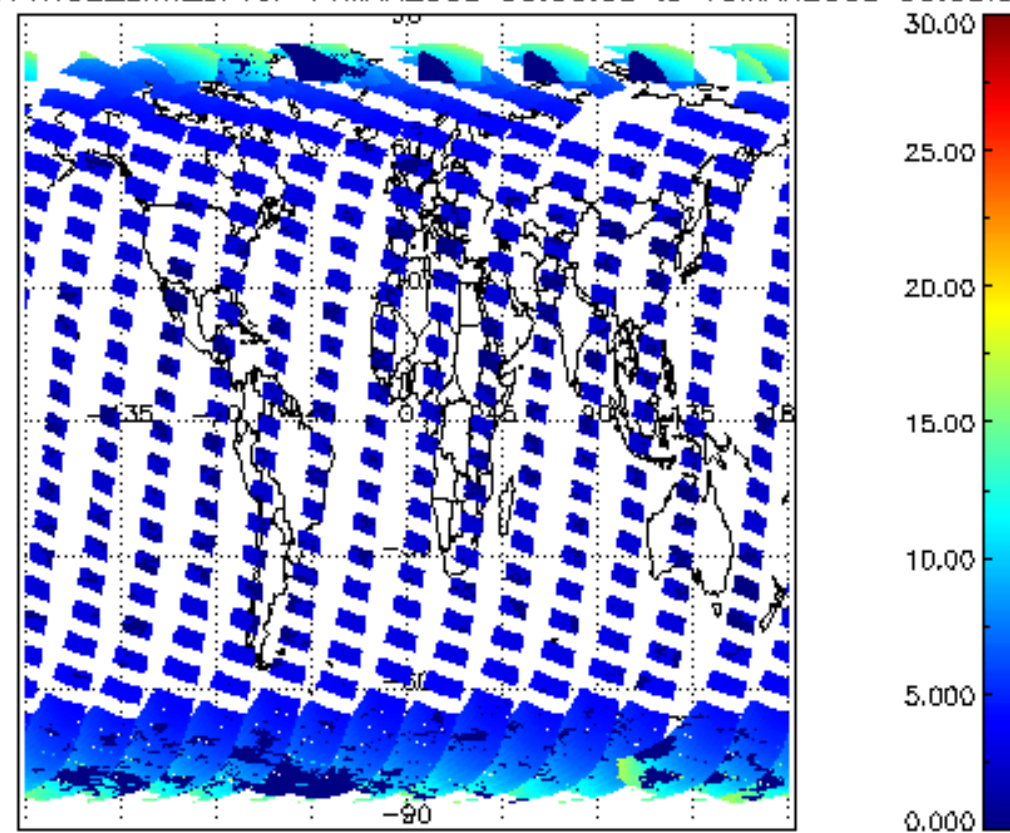
SCIOL2P_NADUV1NO2_amf_cl for 14MAR2008 00:00:00 to 15MAR2008 00:00:00
