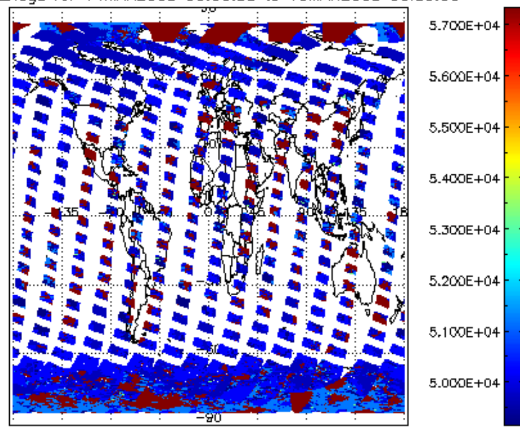
cloud_flags for 14MAR2008 00:00:00 to 15MAR2008 00:00:00
