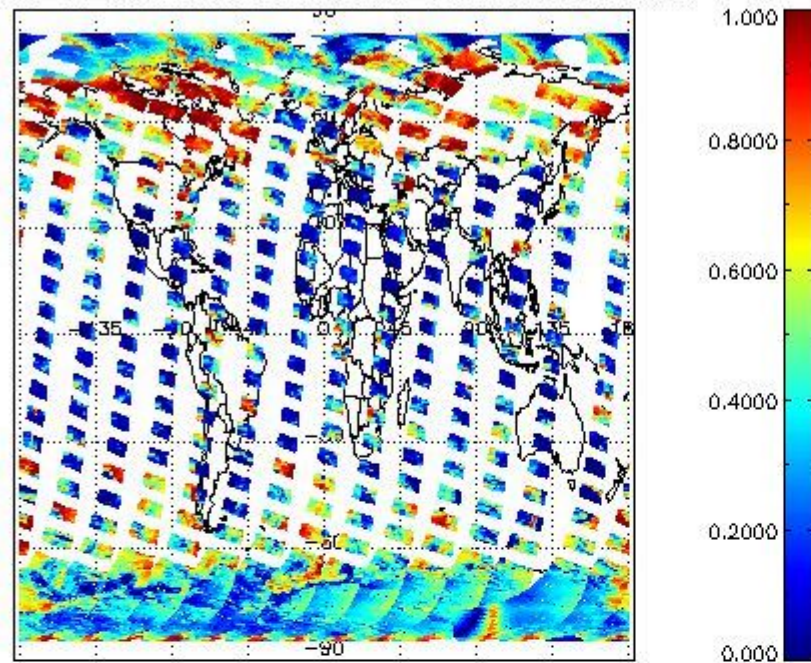
cLfrac for 14MAR2008 00:00:00 to 15MAR2008 00:00:00
