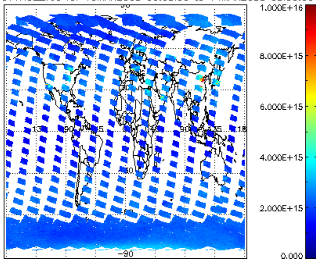
SCIOL2P_NADUV1NO2_vcd for 13MAR2008 00:00:00 to 14MAR2008 00:00:00
