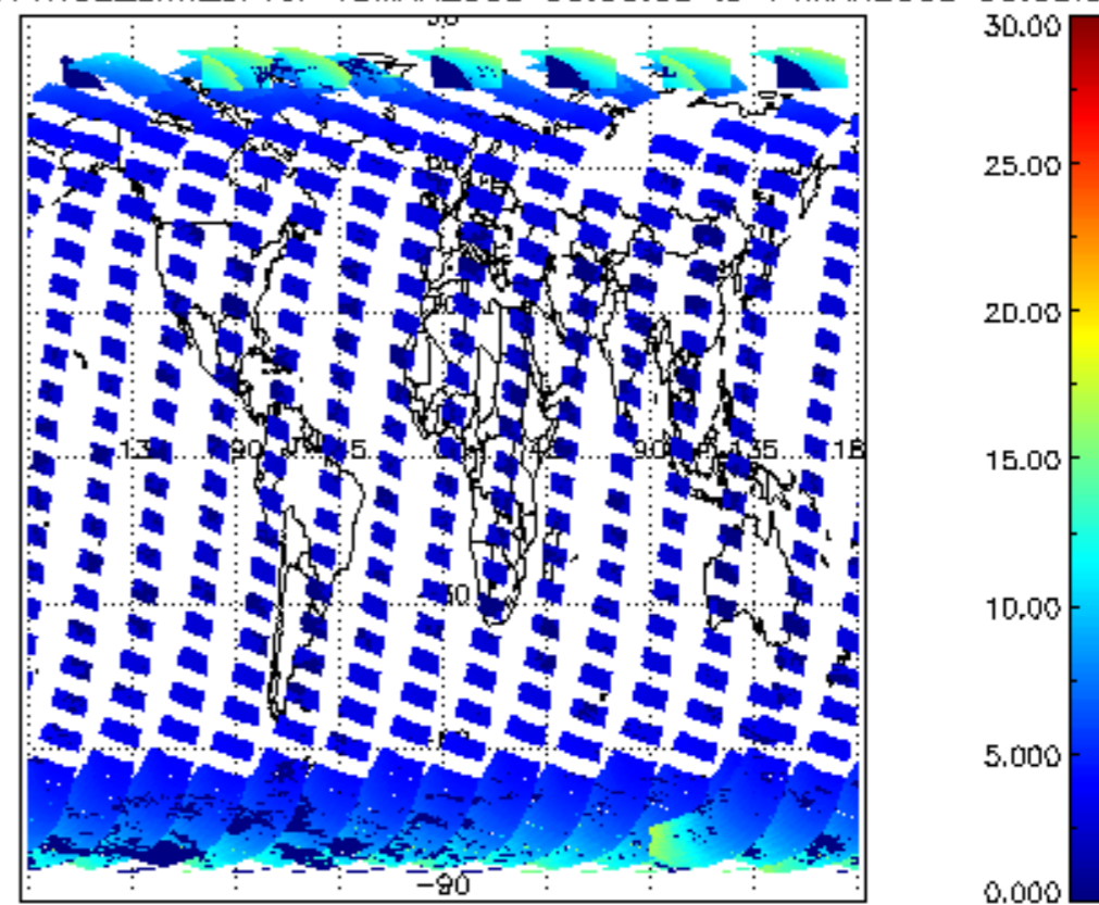
SCIOL2P_NADUV1NO2_amf_cl for 13MAR2008 00:00:00 to 14MAR2008 00:00:00
