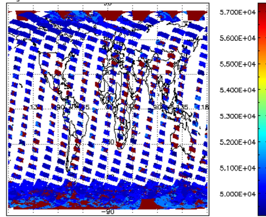
cloud_flags for 13MAR2008 00:00:00 to 14MAR2008 00:00:00
