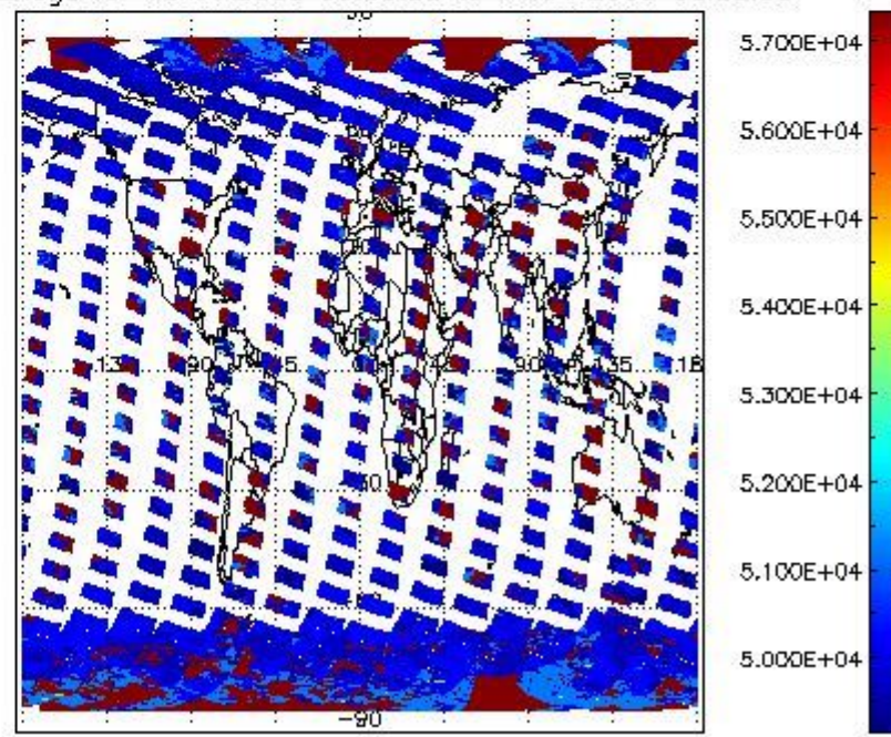
cloud_flags for 13MAR2008 00:00:00 to 14MAR2008 00:00:00
