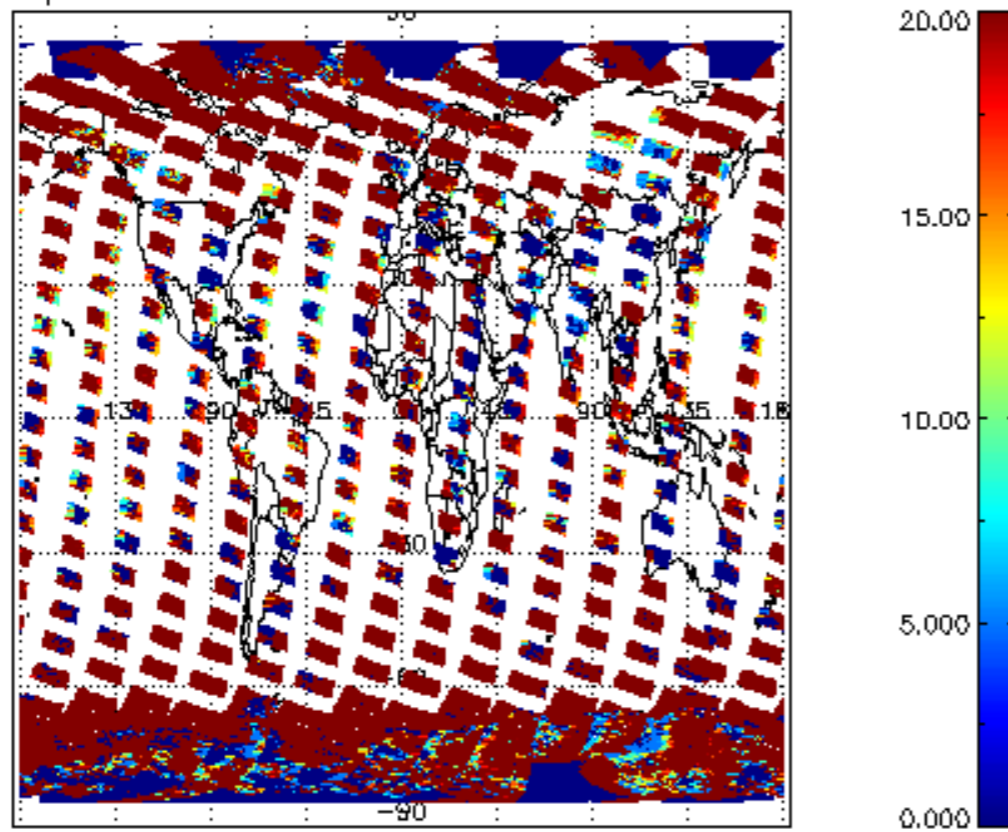
cL_opt_depth for 13MAR2008 00:00:00 to 14MAR2008 00:00:00
