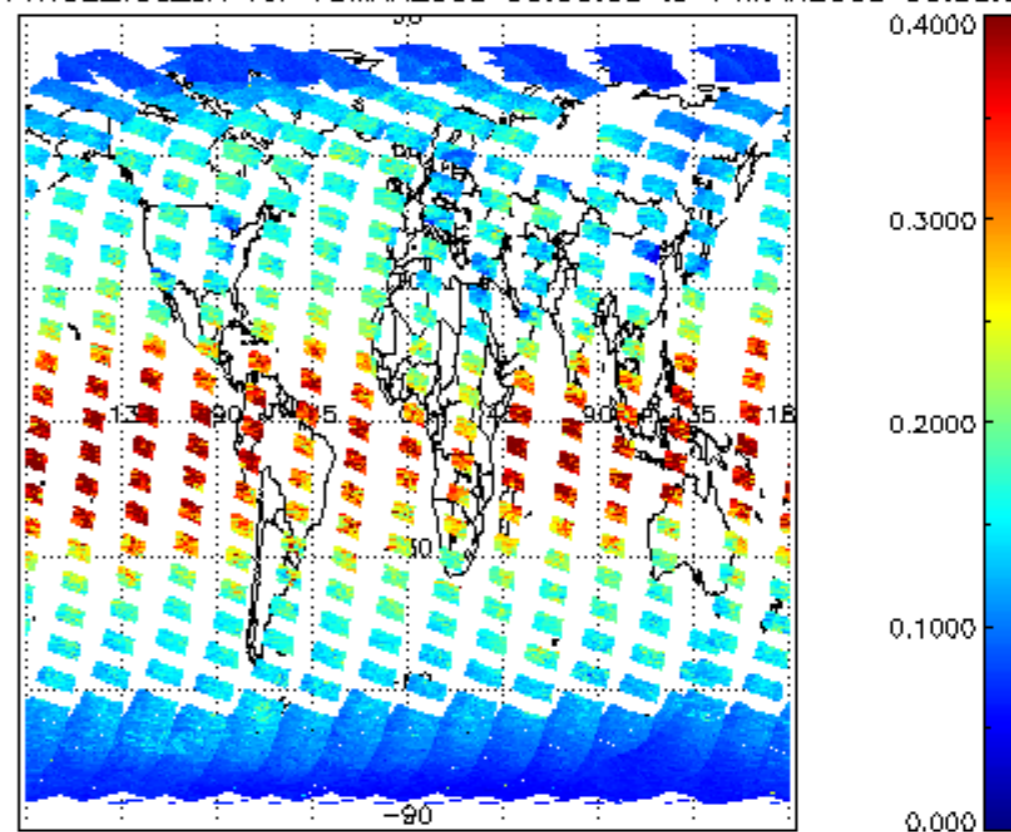
SCIOL2P_NADUV1NO2_vcd_err for 13MAR2008 00:00:00 to 14MAR2008 00:00:00
