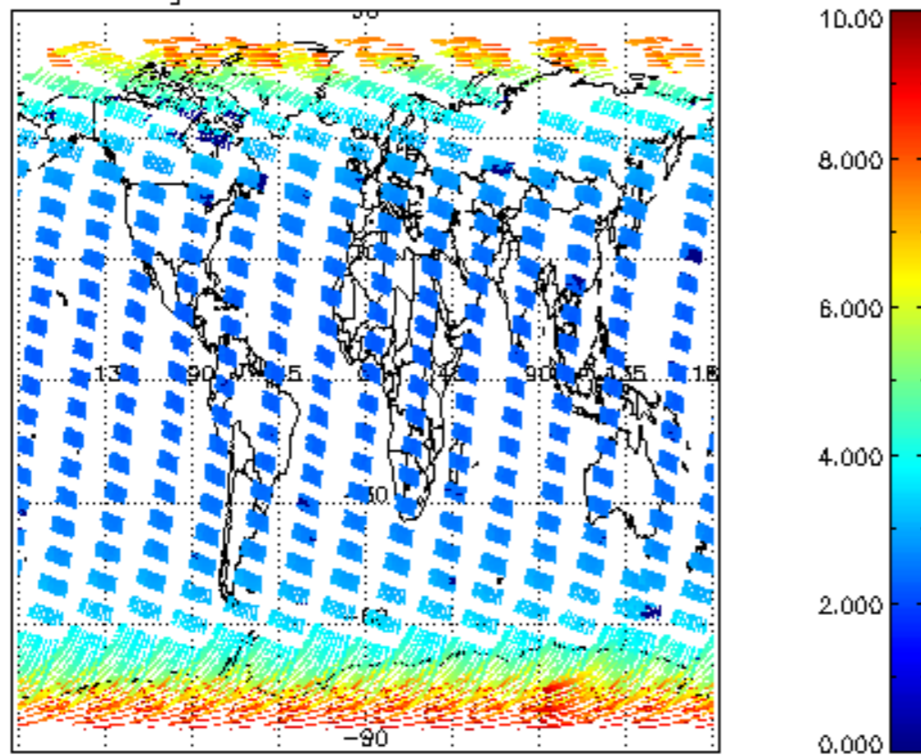
SCIOL2P_NADUV003_amf_gr for 13MAR2008 00:00:00 to 14MAR2008 00:00:00
