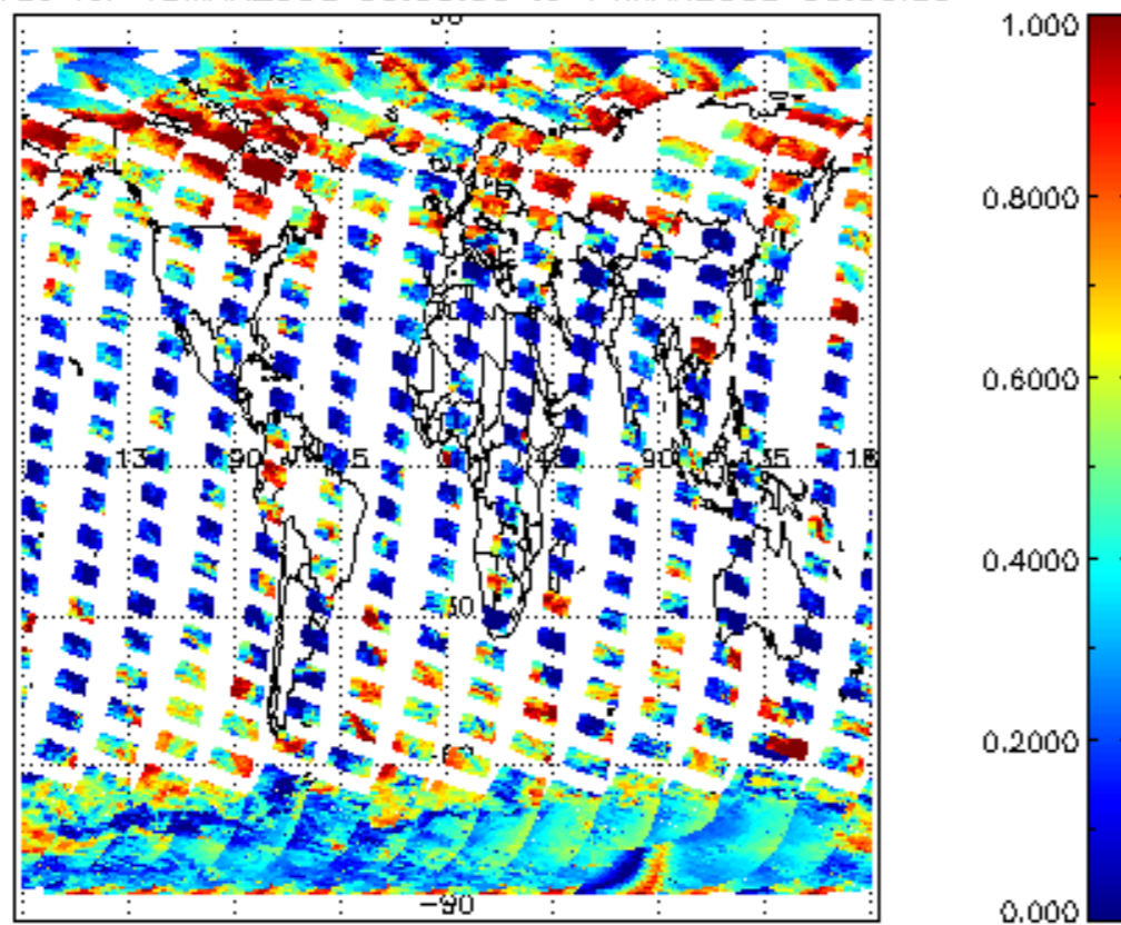
cL_frac for 13MAR2008 00:00:00 to 14MAR2008 00:00:00
