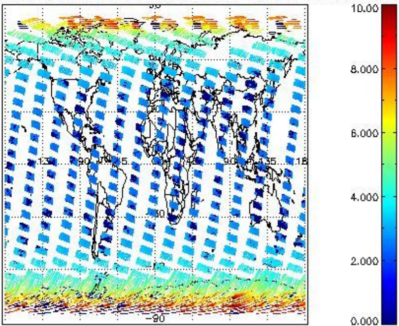
SCIOL2P_NADUV003_amf_cl for 13MAR2008 00:00:00 to 14MAR2008 00:00:00
