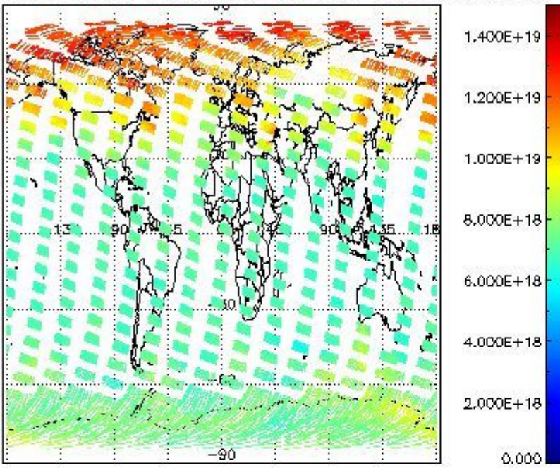
SCIOL2P_NADUV003_vcd for 13MAR2008 00:00:00 to 14MAR2008 00:00:00
