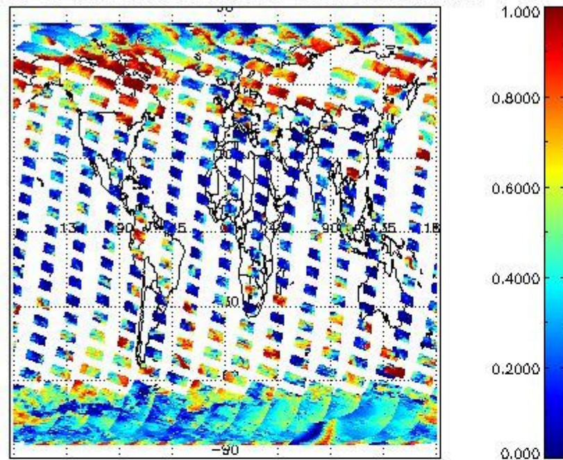
cLfrac for 13MAR2008 00:00:00 to 14MAR2008 00:00:00
