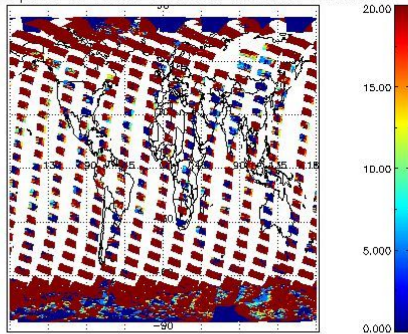
cLopt_depth for 13MAR2008 00:00:00 to 14MAR2008 00:00:00
