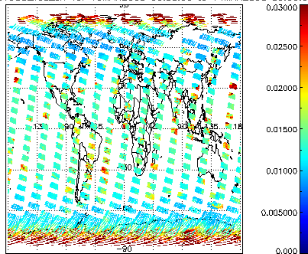
SCIOL2P_NADUV003_vcd_err for 13MAR2008 00:00:00 to 14MAR2008 00:00:00
