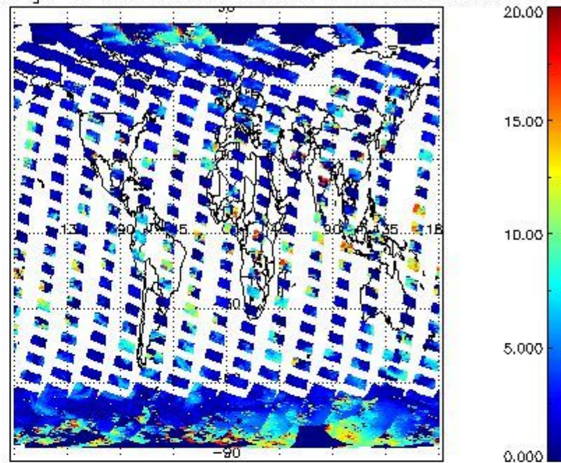
cLtop_height for 13MAR2008 00:00:00 to 14MAR2008 00:00:00
