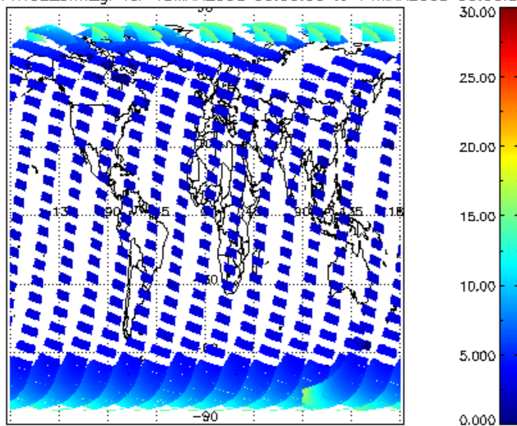
SCIOL2P_NADUV1NO2_amf_gr for 13MAR2008 00:00:00 to 14MAR2008 00:00:00
