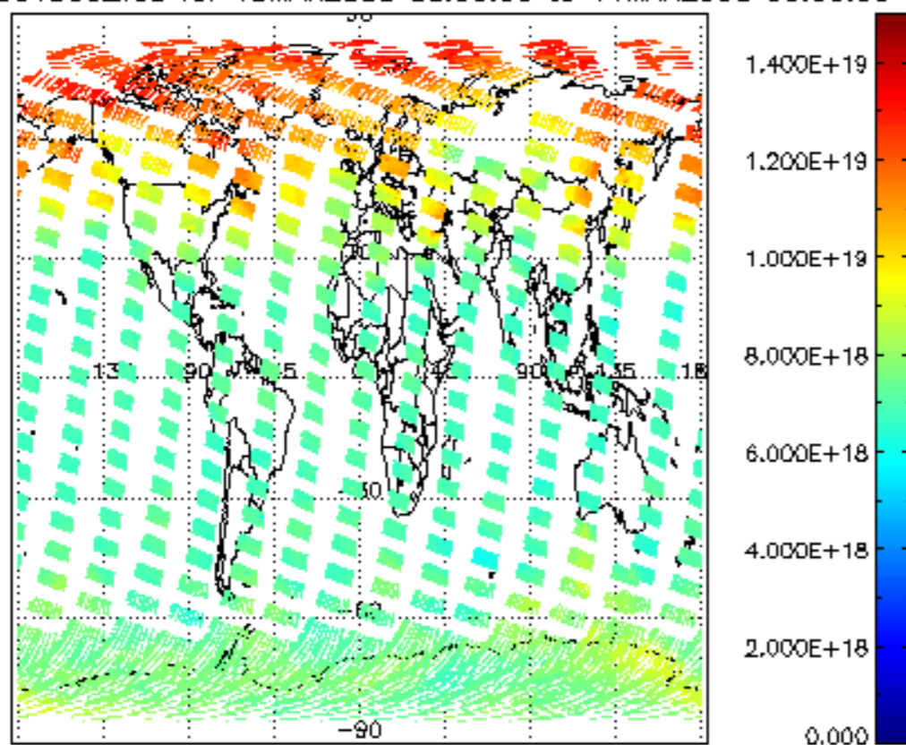
SCIOL2P_NADUV003_vcd for 13MAR2008 00:00:00 to 14MAR2008 00:00:00
