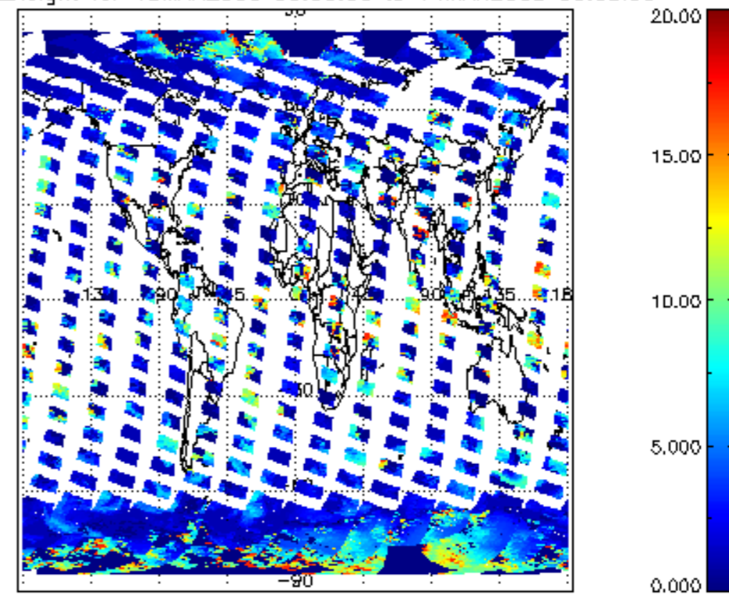
cL_top_height for 13MAR2008 00:00:00 to 14MAR2008 00:00:00
