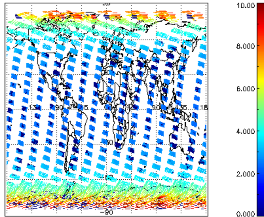
SCIOL2P_NADUV003_amf_cl for 13MAR2008 00:00:00 to 14MAR2008 00:00:00
