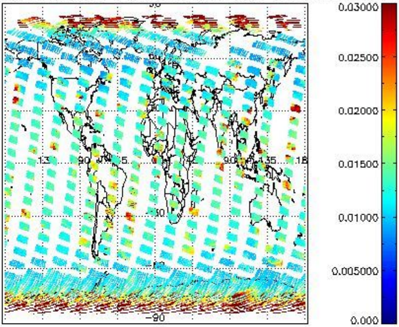
SCIOL2P_NADUV003_vcd_err for 13MAR2008 00:00:00 to 14MAR2008 00:00:00
