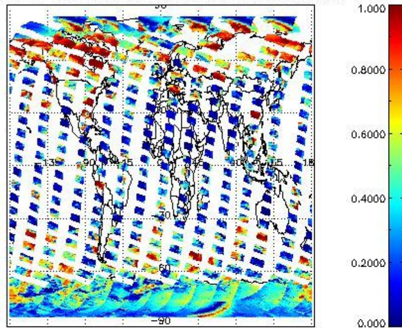
cLfrac for 07MAR2008 00:00:00 to 08MAR2008 00:00:00
