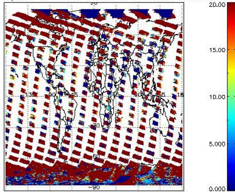
cLopt_depth for 07MAR2008 00:00:00 to 08MAR2008 00:00:00
