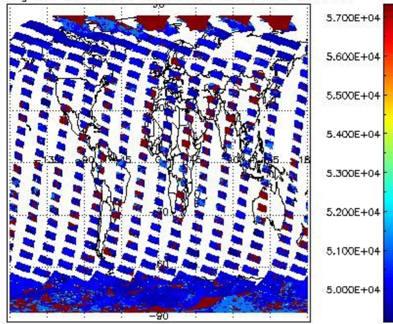
cloud_flags for 07MAR2008 00:00:00 to 08MAR2008 00:00:00
