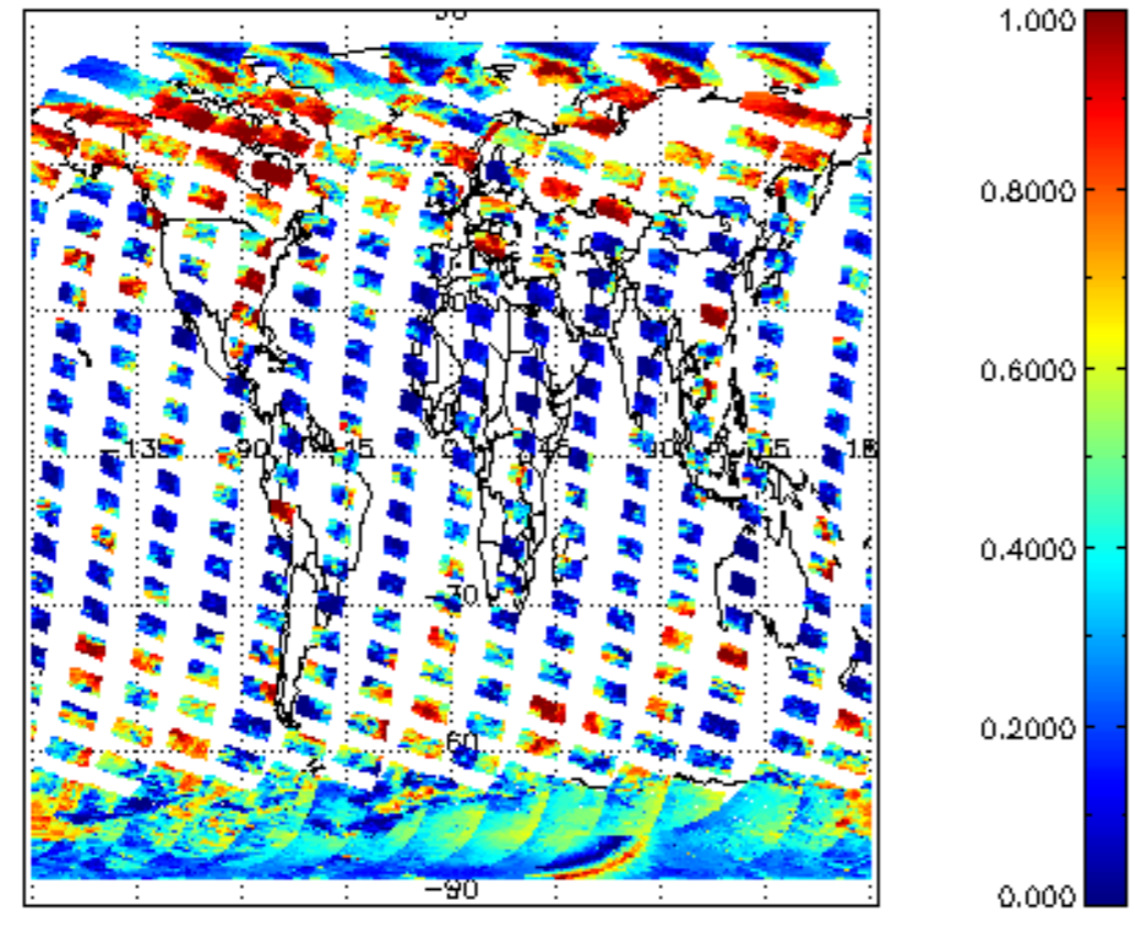
cL_frac for 07MAR2008 00:00:00 to 08MAR2008 00:00:00
