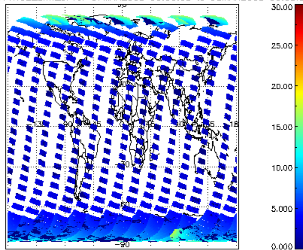
SCIOL2P_NADUV1NO2_amf_cl for 07MAR2008 00:00:00 to 08MAR2008 00:00:00
