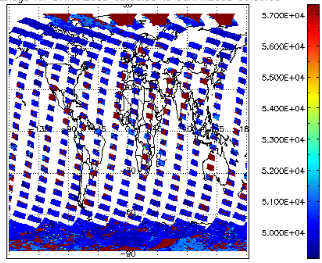
cloud_flags for 07MAR2008 00:00:00 to 08MAR2008 00:00:00
