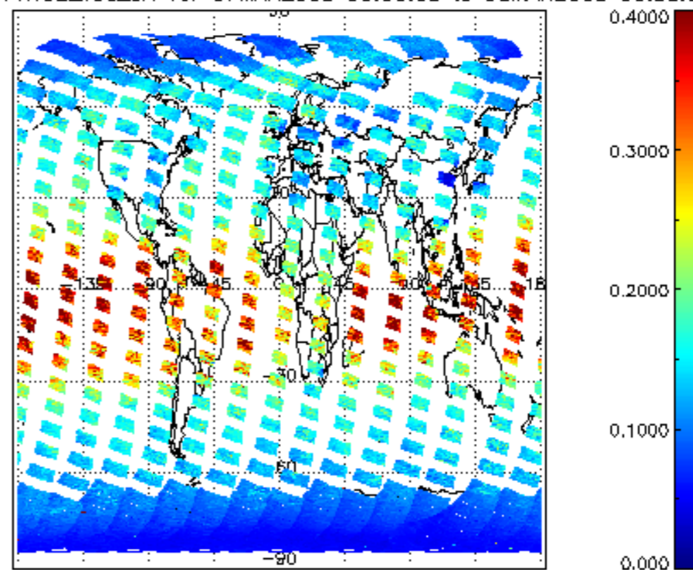
SCIOL2P_NADUV1NO2_vcd_err for 07MAR2008 00:00:00 to 08MAR2008 00:00:00
