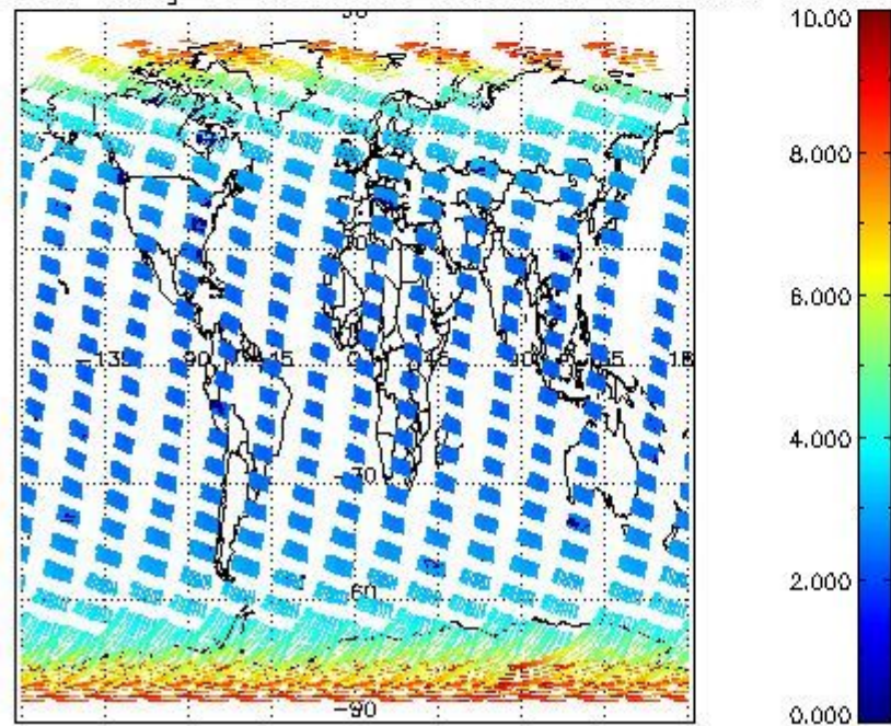
SCIOL2P_NADUV003_amf_gr for 07MAR2008 00:00:00 to 08MAR2008 00:00:00 SCIOL2P_NADUV003_amf_cl for 07MAR2008 00:00:00 to 08MAR2008 00:00:00
