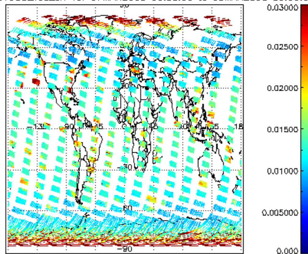
SCIOL2P_NADUV003_vcd_err for 07MAR2008 00:00:00 to 08MAR2008 00:00:00
