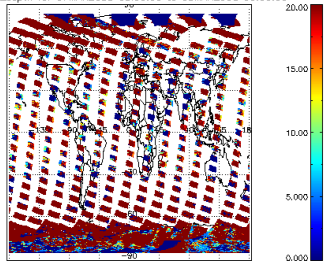
cL_opt_depth for 07MAR2008 00:00:00 to 08MAR2008 00:00:00
