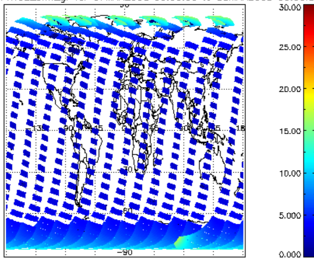
SCIOL2P_NADUV1NO2_amf_gr for 07MAR2008 00:00:00 to 08MAR2008 00:00:00
