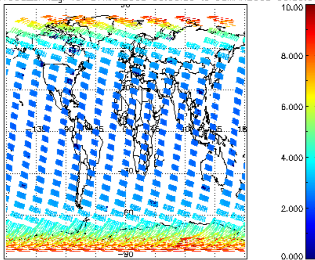
SCIOL2P_NADUV003_amf_gr for 07MAR2008 00:00:00 to 08MAR2008 00:00:00
