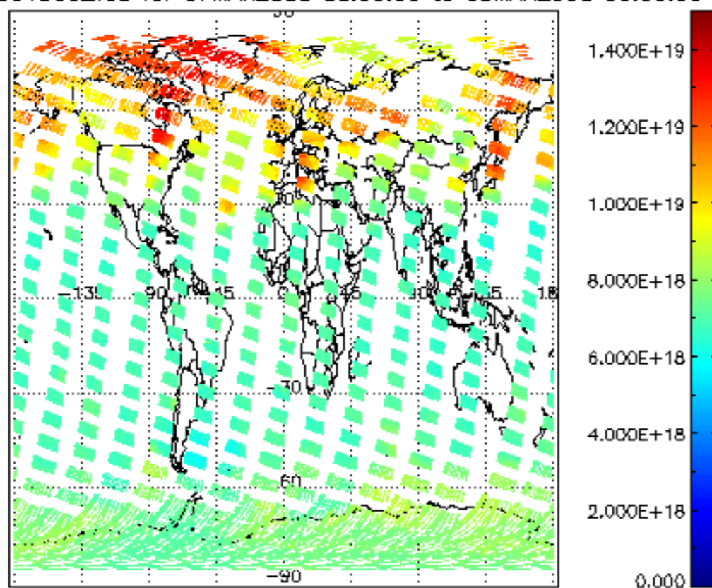
SCIOL2P_NADUV003_vcd for 07MAR2008 00:00:00 to 08MAR2008 00:00:00
