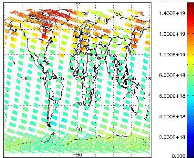
SCIOL2P_NADUV003_vcd for 07MAR2008 00:00:00 to 08MAR2008 00:00:00 SCIOL2P_NADUV003_vcd_err for 07MAR2008 00:00:00 to 08MAR2008 00:00:00
