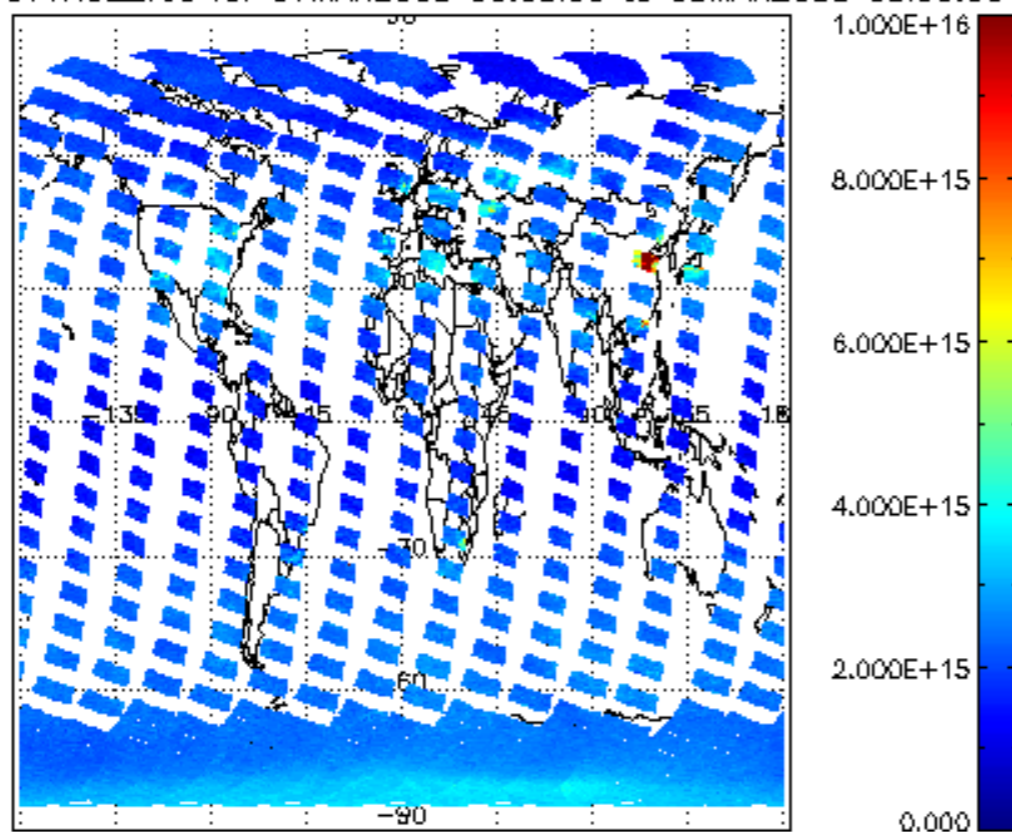
SCIOL2P_NADUV1NO2_vcd for 07MAR2008 00:00:00 to 08MAR2008 00:00:00
