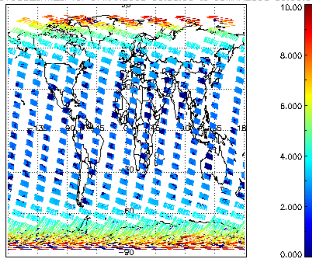
SCIOL2P_NADUV003_amf_cl for 07MAR2008 00:00:00 to 08MAR2008 00:00:00
