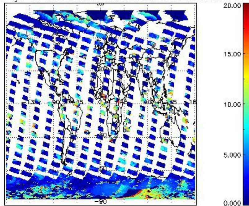
cLtop_height for 07MAR2008 00:00:00 to 08MAR2008 00:00:00
