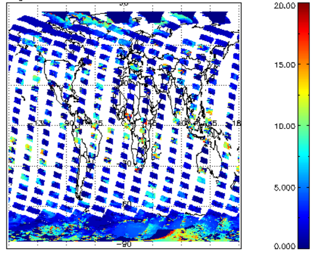
cL_top_height for 07MAR2008 00:00:00 to 08MAR2008 00:00:00
