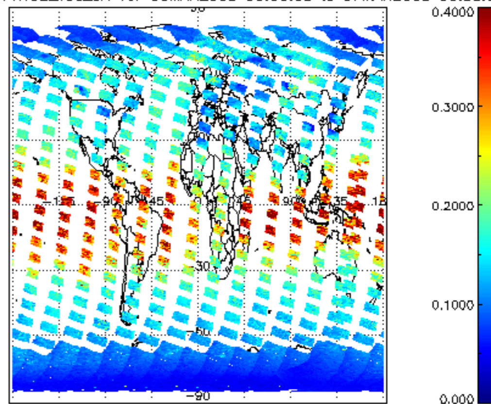
SCIOL2P_NADUV1NO2_vcd_err for 06MAR2008 00:00:00 to 07MAR2008 00:00:00
