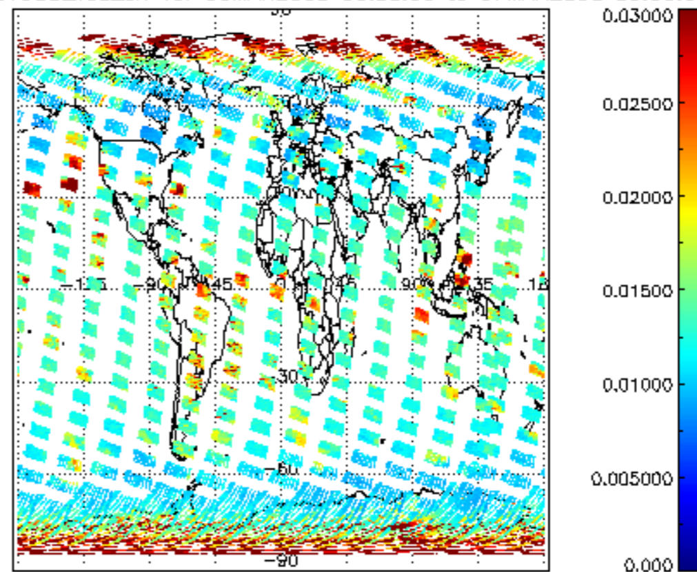
SCIOL2P_NADUV003_vcd_err for 06MAR2008 00:00:00 to 07MAR2008 00:00:00
