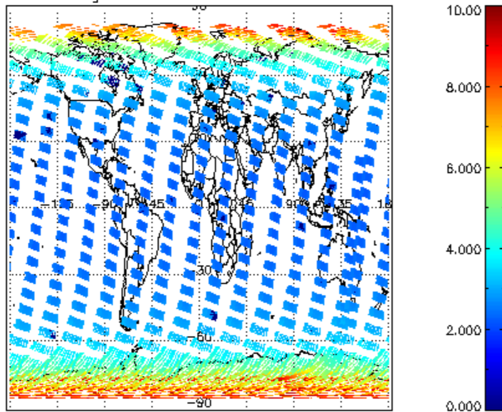
SCIOL2P_NADUV003_amf_gr for 06MAR2008 00:00:00 to 07MAR2008 00:00:00
