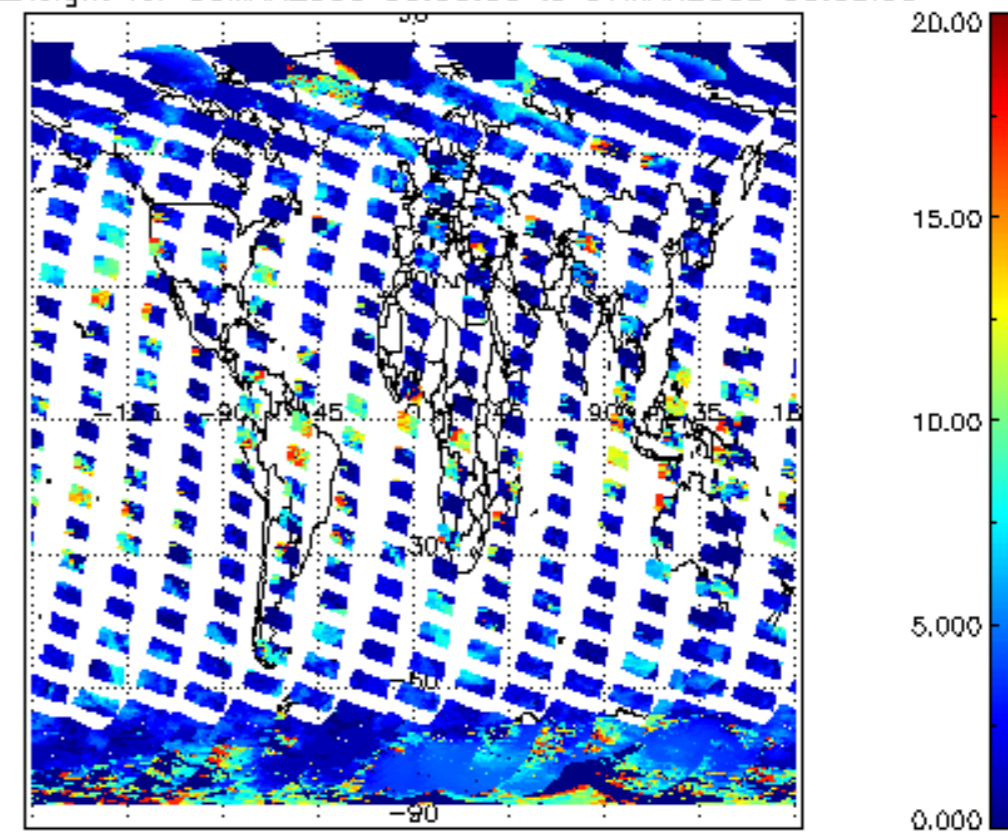
cL_top_height for 06MAR2008 00:00:00 to 07MAR2008 00:00:00
