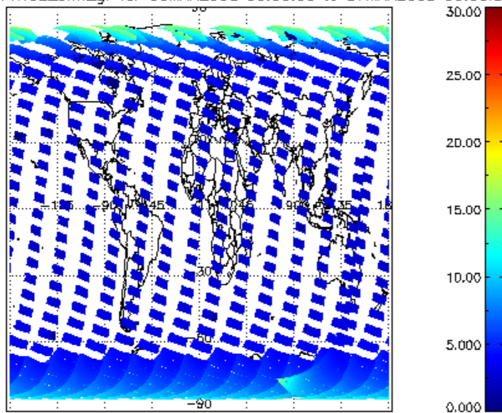
SCIOL2P_NADUV1NO2_amf_gr for 06MAR2008 00:00:00 to 07MAR2008 00:00:00
