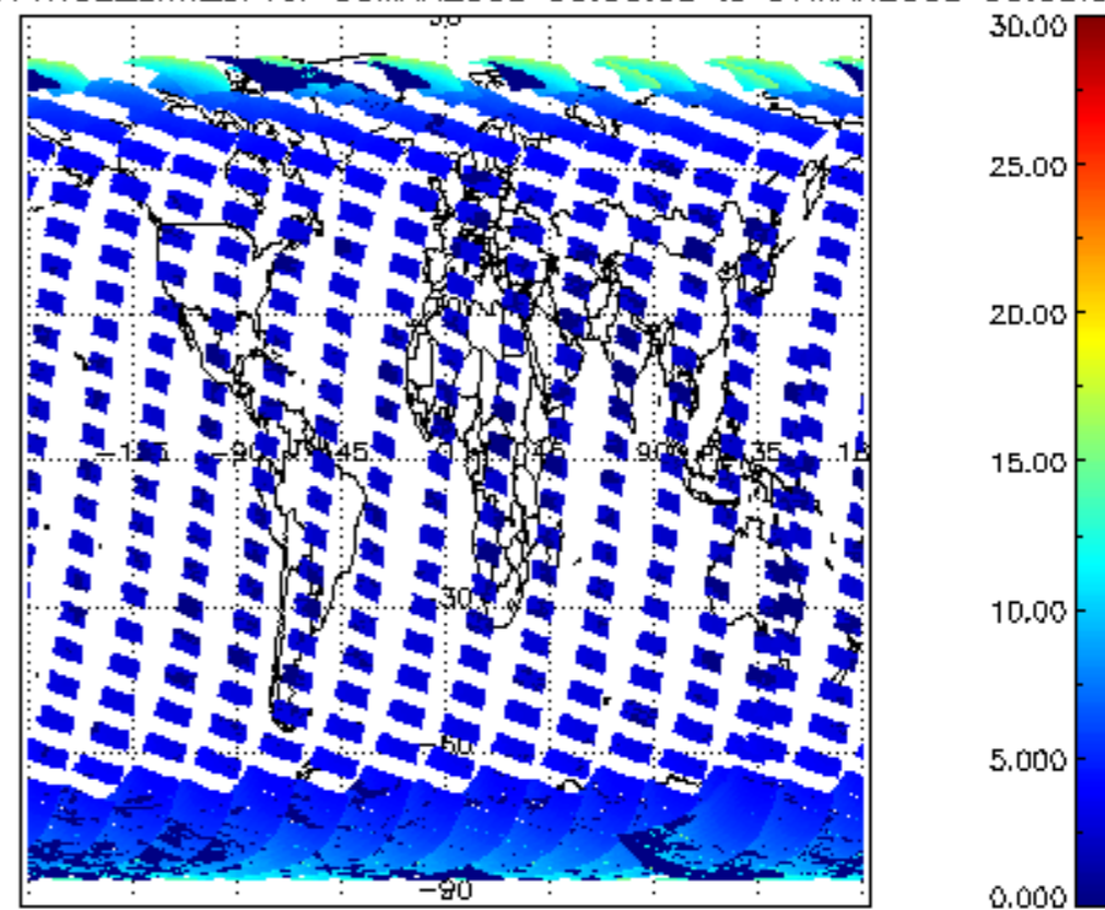
SCIOL2P_NADUV1NO2_amf_cl for 06MAR2008 00:00:00 to 07MAR2008 00:00:00
