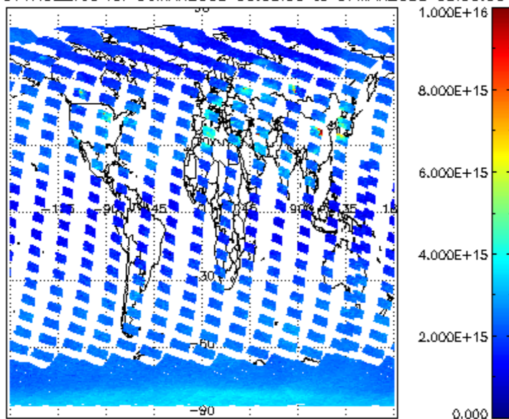
SCIOL2P_NADUV1NO2_vcd for 06MAR2008 00:00:00 to 07MAR2008 00:00:00
