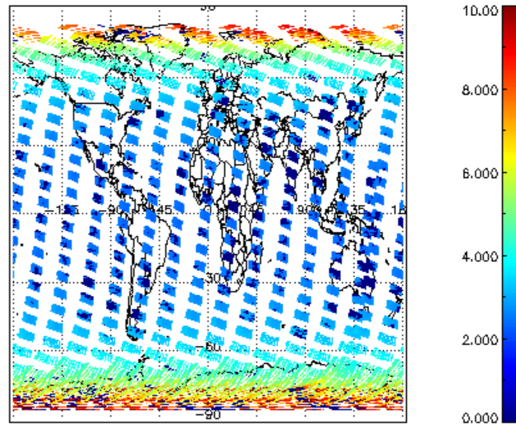
SCIOL2P_NADUV003_amf_cl for 06MAR2008 00:00:00 to 07MAR2008 00:00:00
