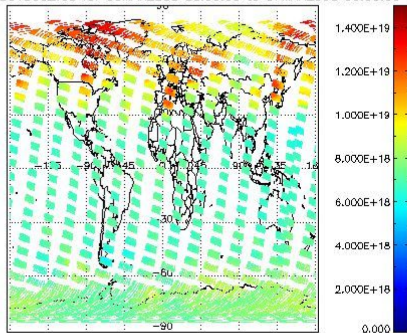
SCIOL2P_NADUV003_vcd for 06MAR2008 00:00:00 to 07MAR2008 00:00:00 SCIOL2P_NADUV003_vcd_err for 06MAR2008 00:00:00 to 07MAR2008 00:00:00
