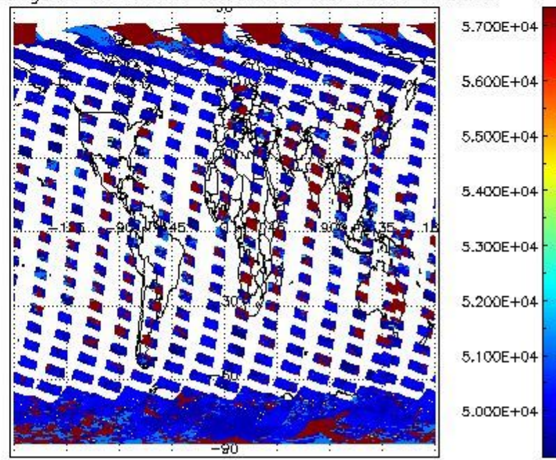
cloud_flags for 06MAR2008 00:00:00 to 07MAR2008 00:00:00
