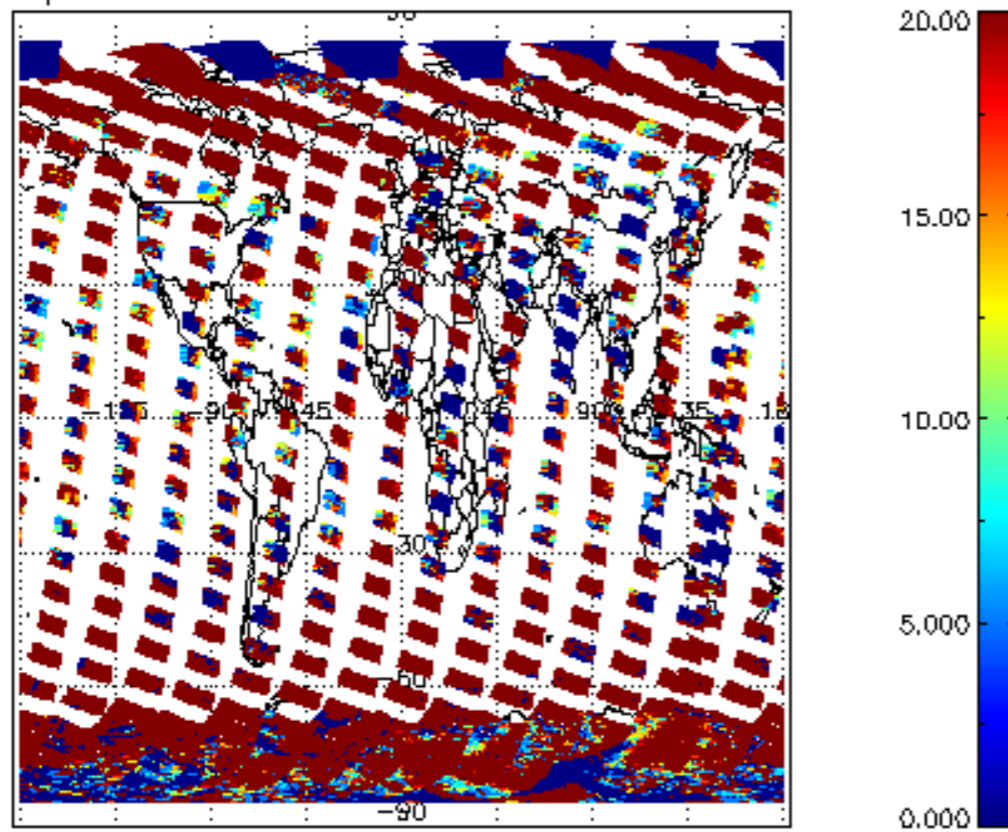
cL_opt_depth for 06MAR2008 00:00:00 to 07MAR2008 00:00:00
