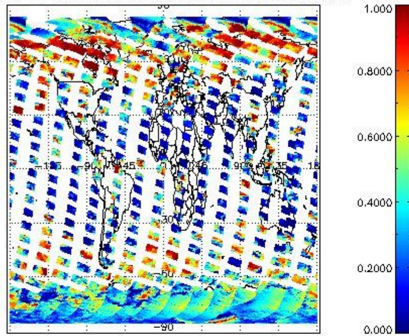
cLfrac for 06MAR2008 00:00:00 to 07MAR2008 00:00:00
