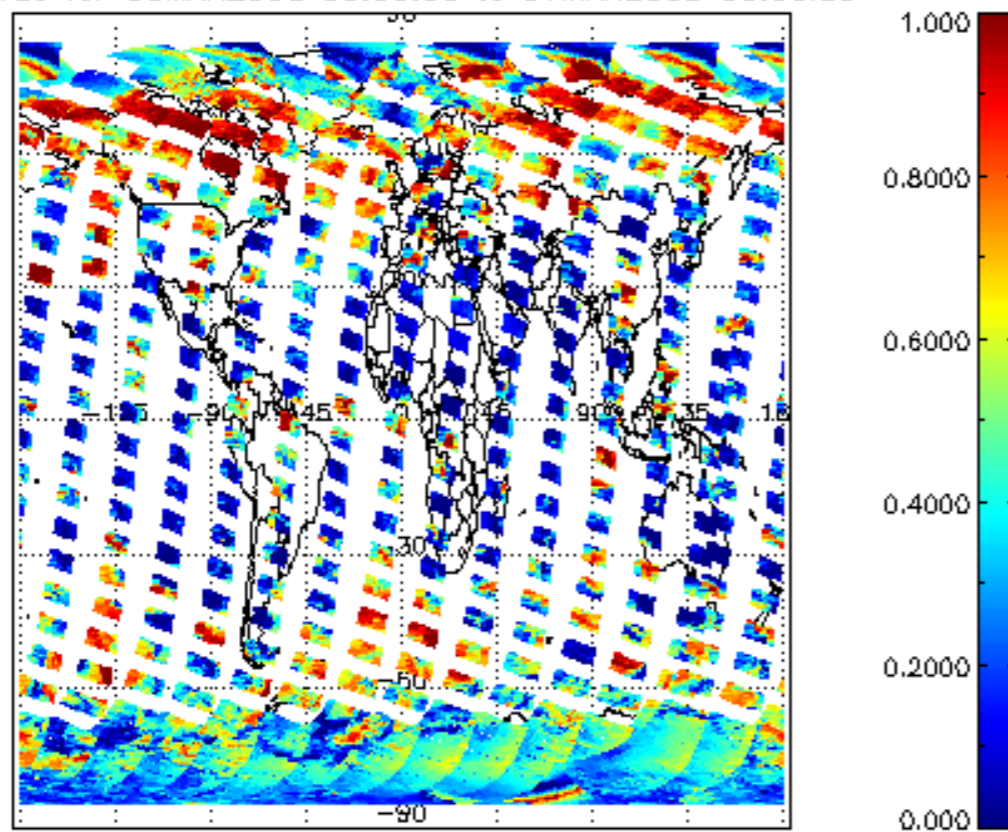
cL_frac for 06MAR2008 00:00:00 to 07MAR2008 00:00:00
