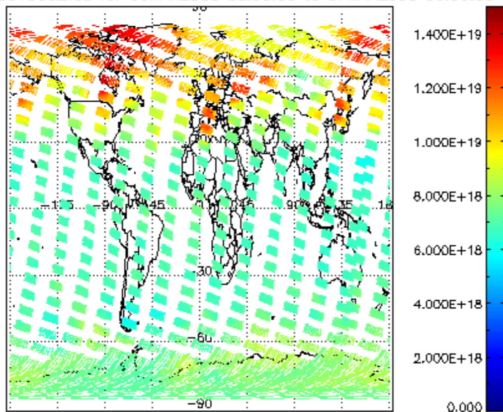
SCIOL2P_NADUV003_vcd for 06MAR2008 00:00:00 to 07MAR2008 00:00:00
