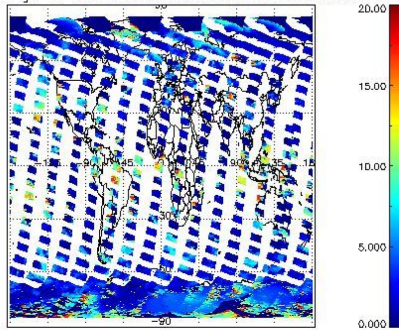
cLtop_height for 06MAR2008 00:00:00 to 07MAR2008 00:00:00
