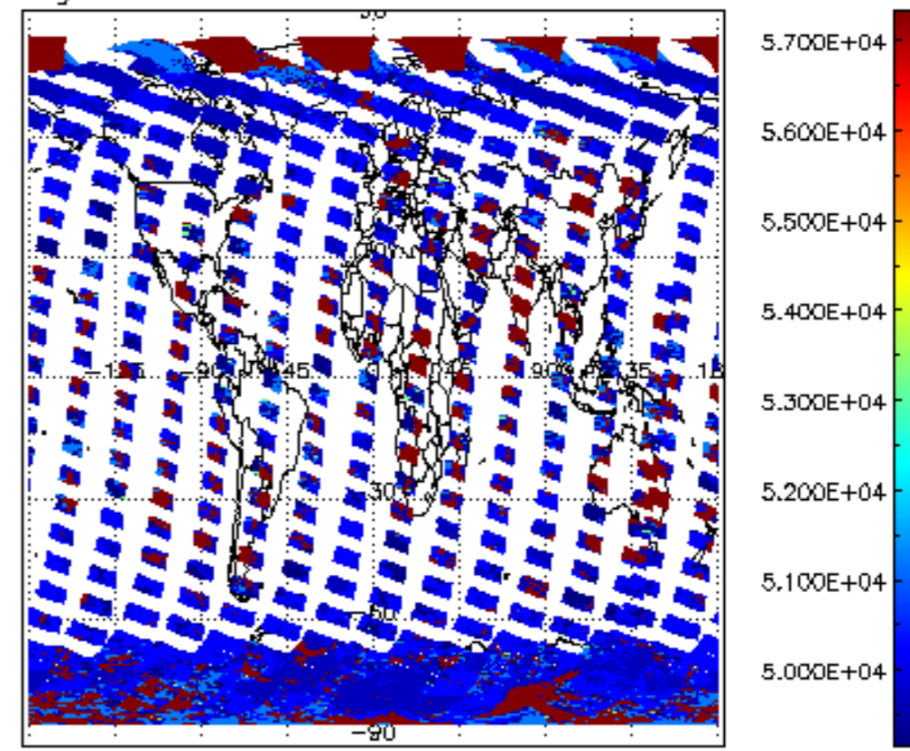
cloud_flags for 06MAR2008 00:00:00 to 07MAR2008 00:00:00
