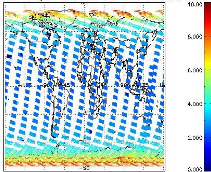
SCIOL2P_NADUV003_amf_gr for 06MAR2008 00:00:00 to 07MAR2008 00:00:00 SCIOL2P_NADUV003_amf_cl for 06MAR2008 00:00:00 to 07MAR2008 00:00:00
