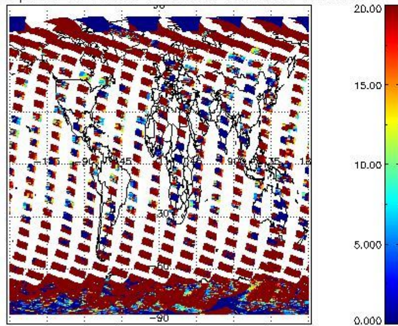
cLopt_depth for 06MAR2008 00:00:00 to 07MAR2008 00:00:00
