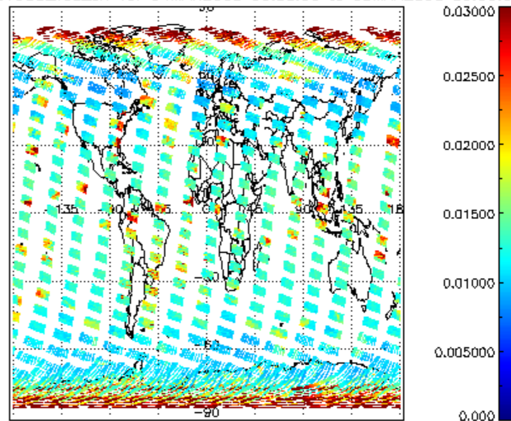
SCIOL2P_NADUV003_vcd_err for 04MAR2008 00:00:00 to 05MAR2008 00:00:00
