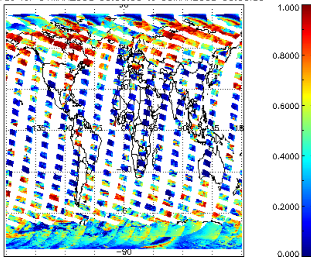
cL_frac for 04MAR2008 00:00:00 to 05MAR2008 00:00:00
