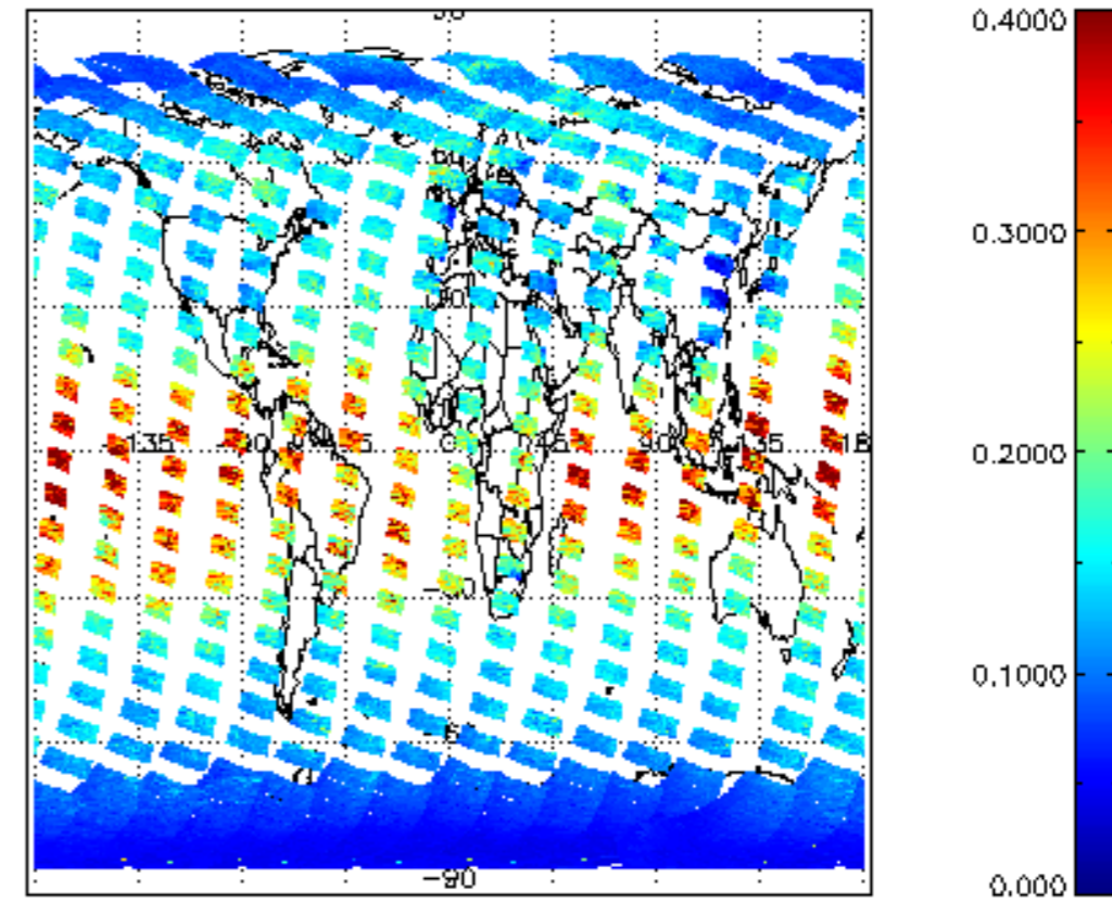
SCIOL2P_NADUV1NO2_vcd_err for 04MAR2008 00:00:00 to 05MAR2008 00:00:00
