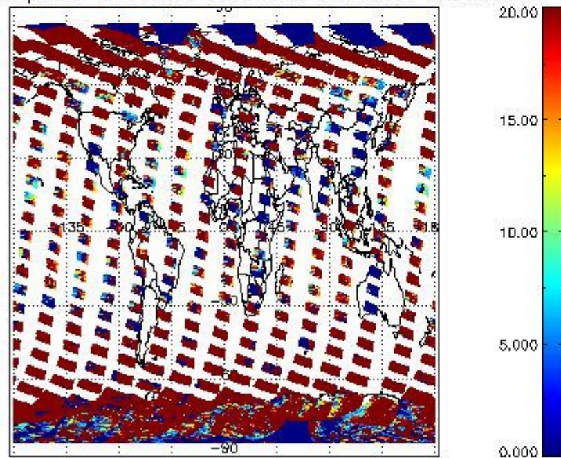
cLopt_depth for 04MAR2008 00:00:00 to 05MAR2008 00:00:00
