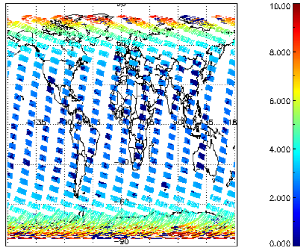
SCIOL2P_NADUV003_amf_cl for 04MAR2008 00:00:00 to 05MAR2008 00:00:00
