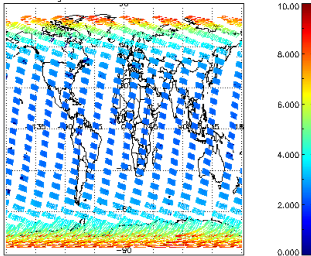
SCIOL2P_NADUV003_amf_gr for 04MAR2008 00:00:00 to 05MAR2008 00:00:00
