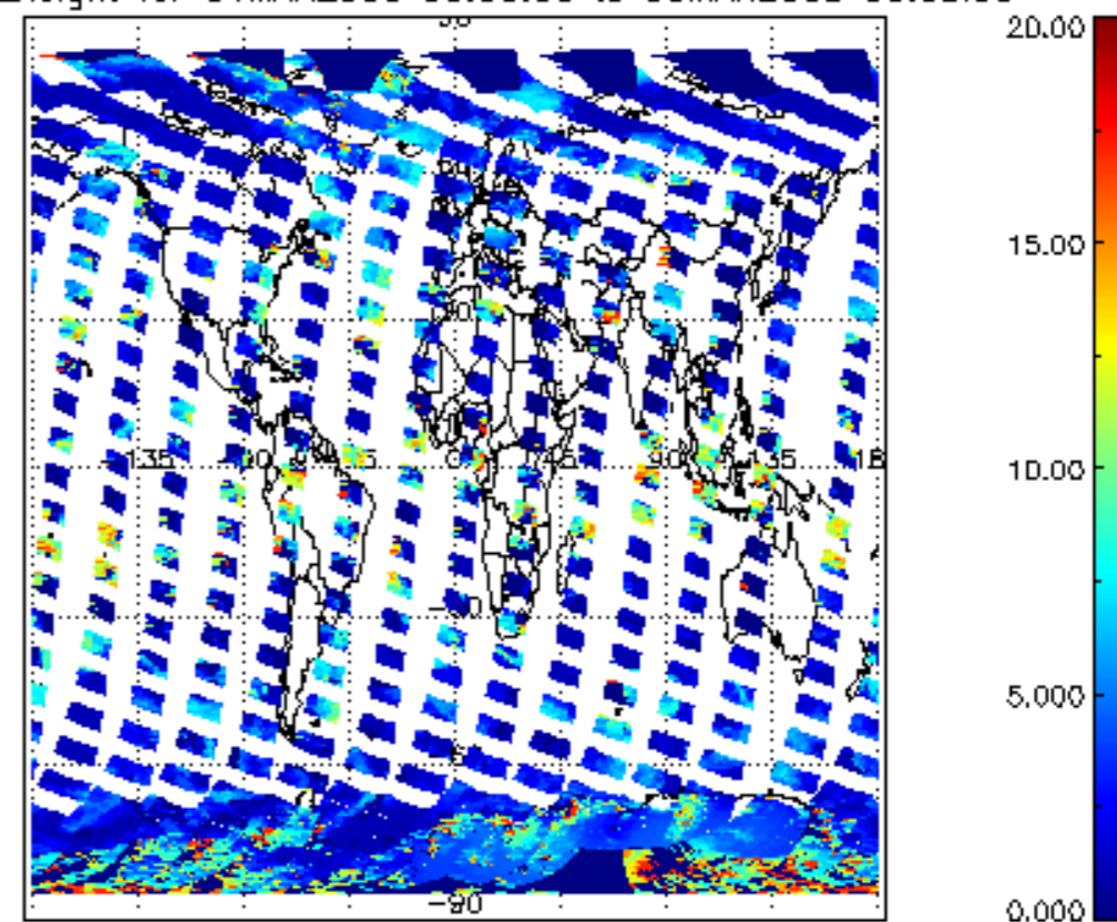
cL_top_height for 04MAR2008 00:00:00 to 05MAR2008 00:00:00
