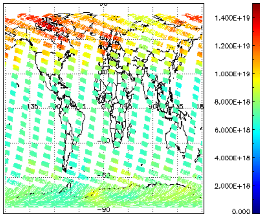
SCIOL2P_NADUV003_vcd for 04MAR2008 00:00:00 to 05MAR2008 00:00:00
