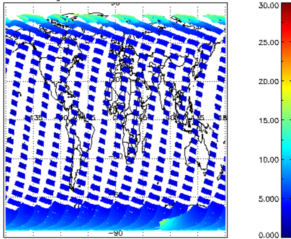
SCIOL2P_NADUV1NO2_amf_gr for 04MAR2008 00:00:00 to 05MAR2008 00:00:00
