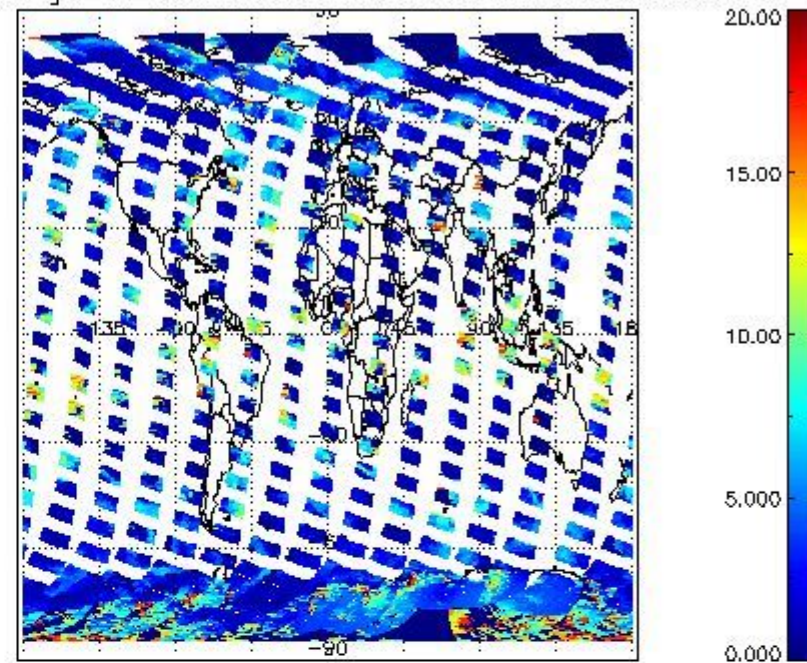
cLtop_height for 04MAR2008 00:00:00 to 05MAR2008 00:00:00
