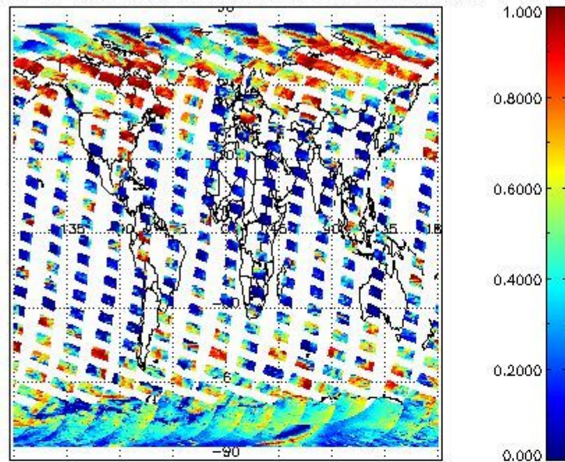
cLfrac for 04MAR2008 00:00:00 to 05MAR2008 00:00:00
