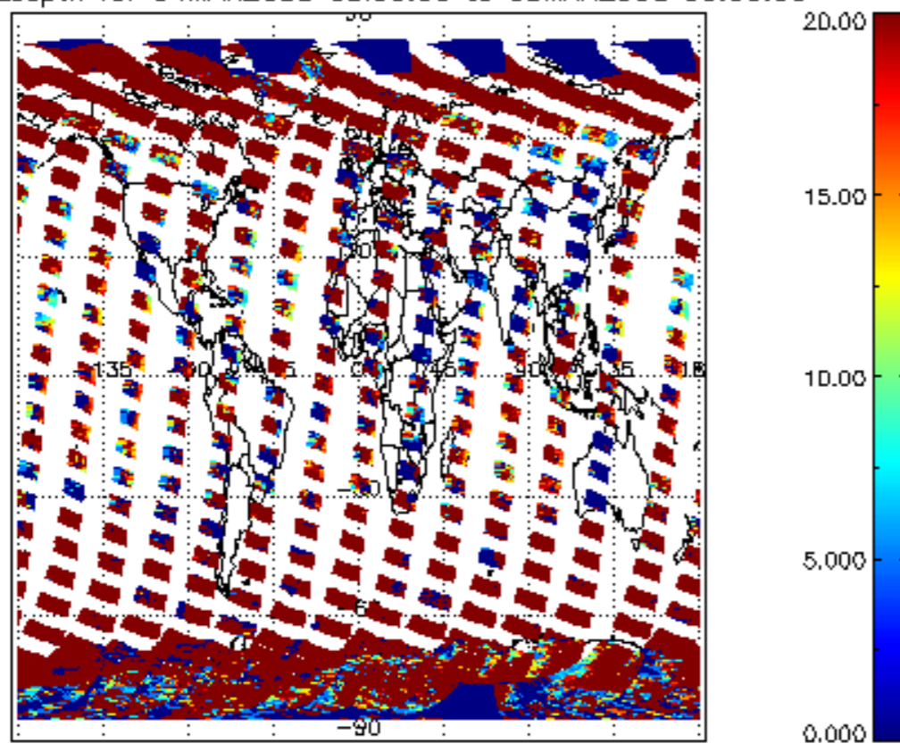
cL_opt_depth for 04MAR2008 00:00:00 to 05MAR2008 00:00:00
