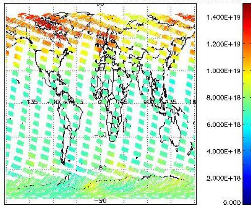
SCIOL2P_NADUV003_vcd for 04MAR2008 00:00:00 to 05MAR2008 00:00:00
