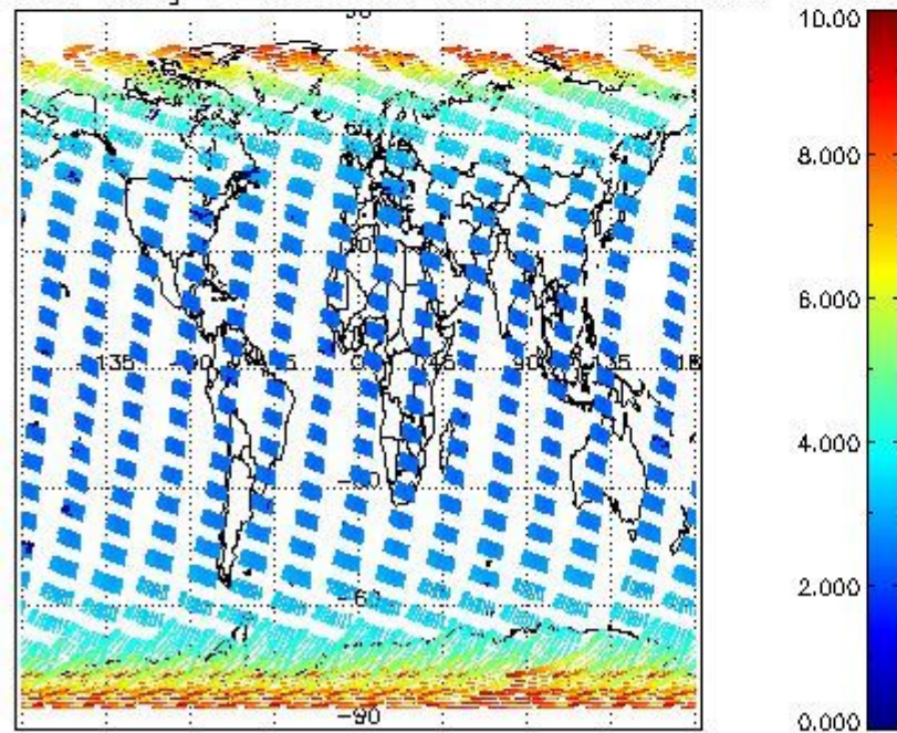
SCIOL2P_NADUV003_amf_gr for 04MAR2008 00:00:00 to 05MAR2008 00:00:00
