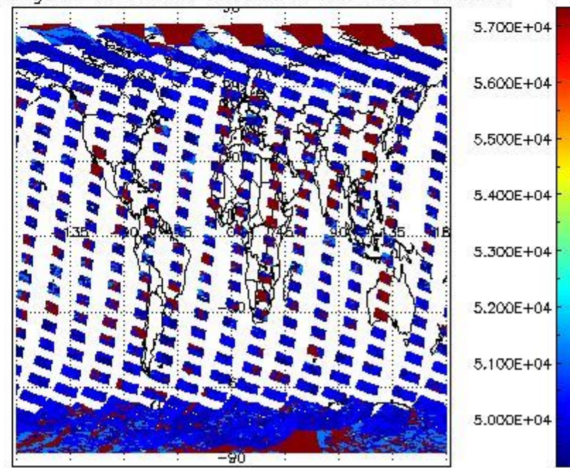
cloud_flags for 04MAR2008 00:00:00 to 05MAR2008 00:00:00
