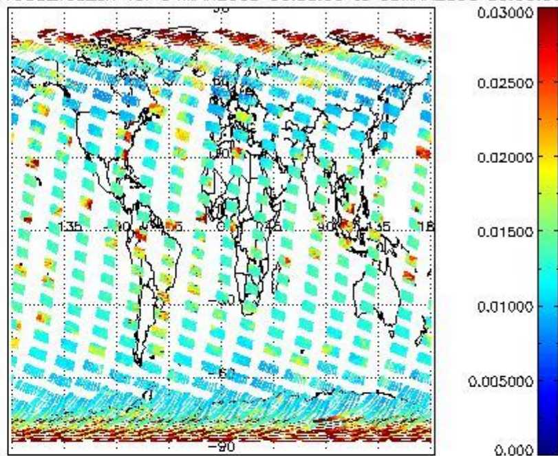
SCIOL2P_NADUV003_vcd_err for 04MAR2008 00:00:00 to 05MAR2008 00:00:00
