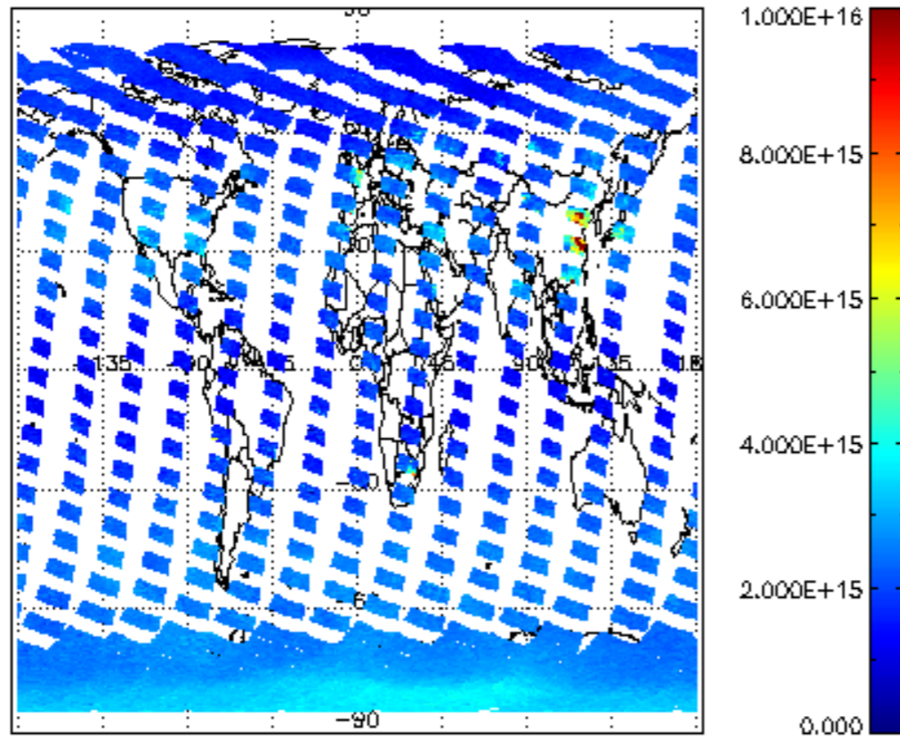
SCIOL2P_NADUV1NO2_vcd for 04MAR2008 00:00:00 to 05MAR2008 00:00:00
