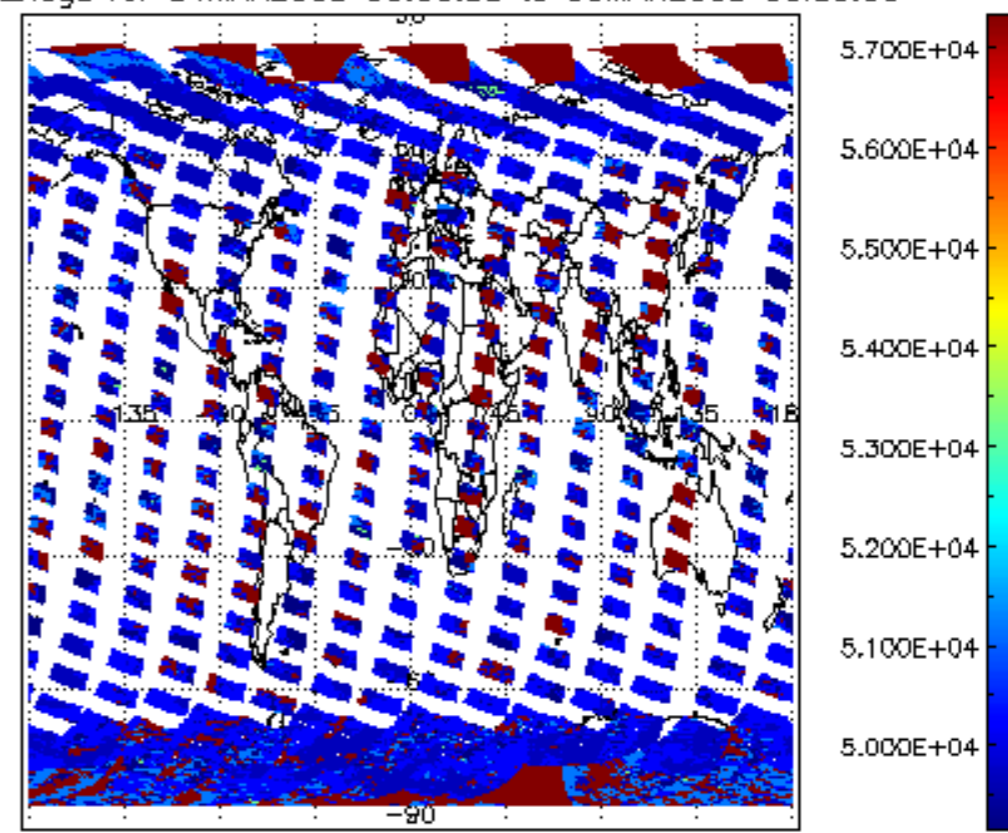
cloud_flags for 04MAR2008 00:00:00 to 05MAR2008 00:00:00
