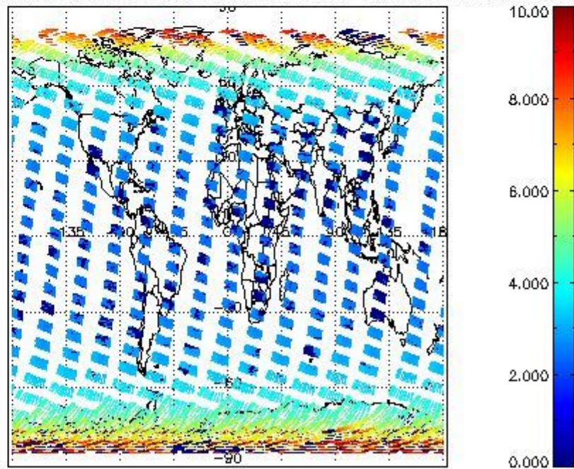
SCIOL2P_NADUV003_amf_cl for 04MAR2008 00:00:00 to 05MAR2008 00:00:00
