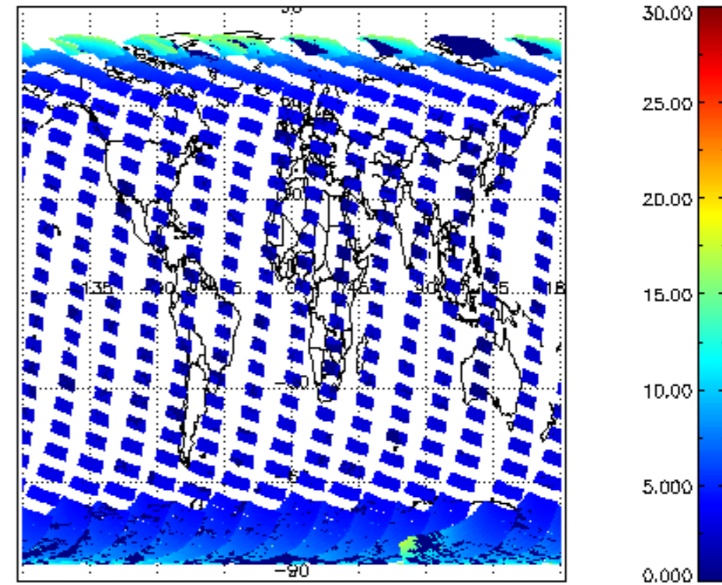
SCIOL2P_NADUV1NO2_amf_cl for 04MAR2008 00:00:00 to 05MAR2008 00:00:00
