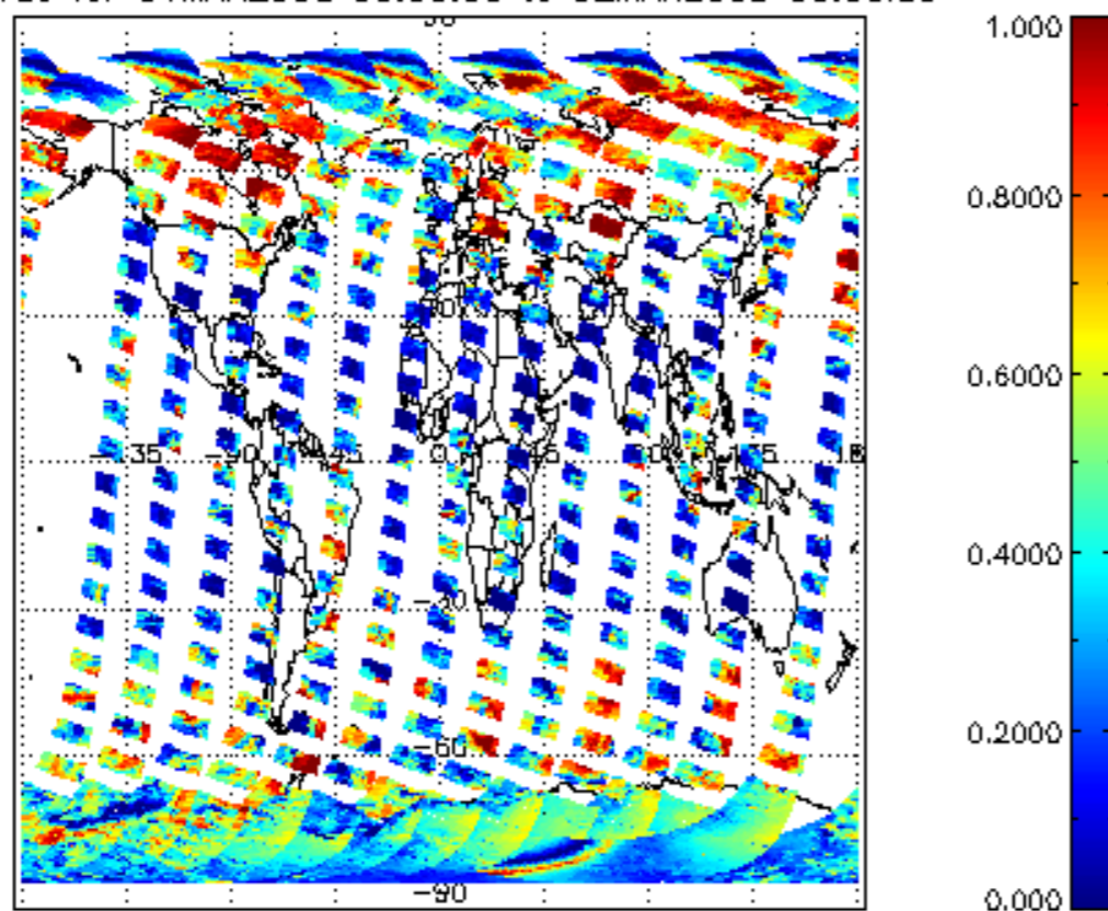
cL_frac for 01MAR2008 00:00:00 to 02MAR2008 00:00:00
