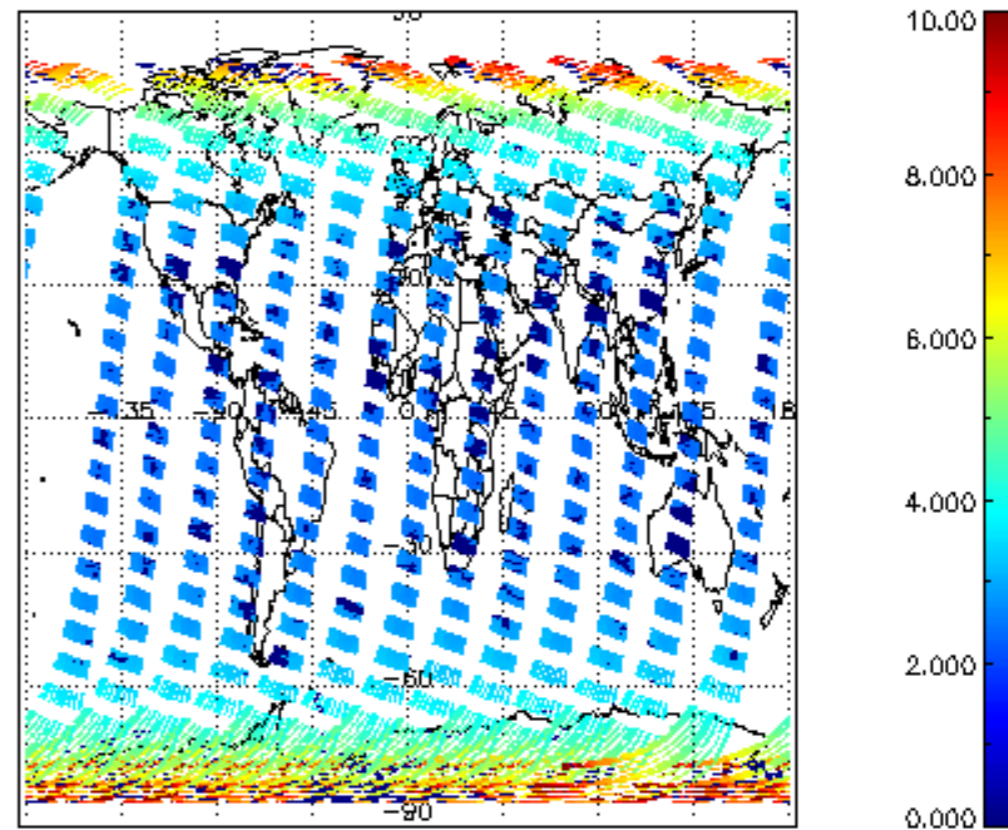
SCIOL2P_NADUV003_amf_cl for 01MAR2008 00:00:00 to 02MAR2008 00:00:00
