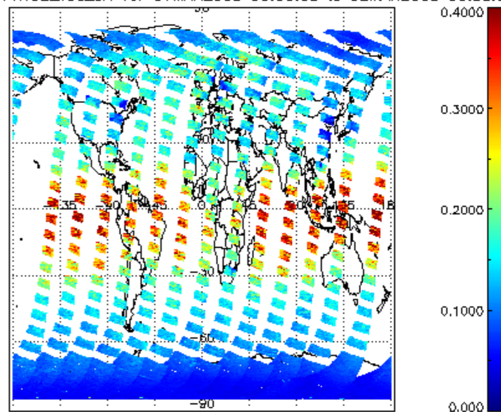
SCIOL2P_NADUV1NO2_vcd_err for 01MAR2008 00:00:00 to 02MAR2008 00:00:00
