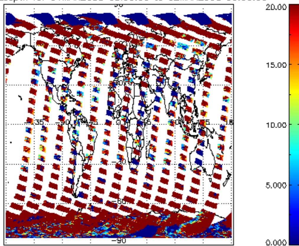
cL_opt_depth for 01MAR2008 00:00:00 to 02MAR2008 00:00:00
