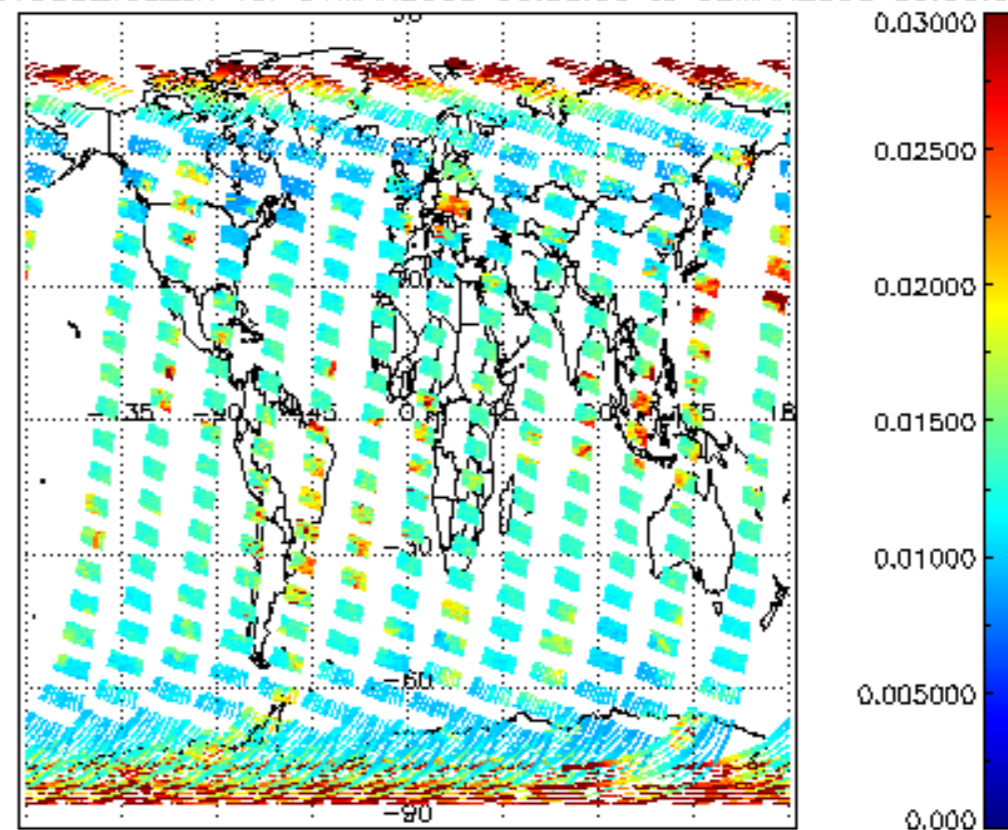
SCIOL2P_NADUV003_vcd_err for 01MAR2008 00:00:00 to 02MAR2008 00:00:00
