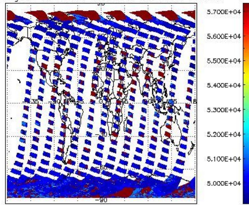
cloud_flags for 01MAR2008 00:00:00 to 02MAR2008 00:00:00
