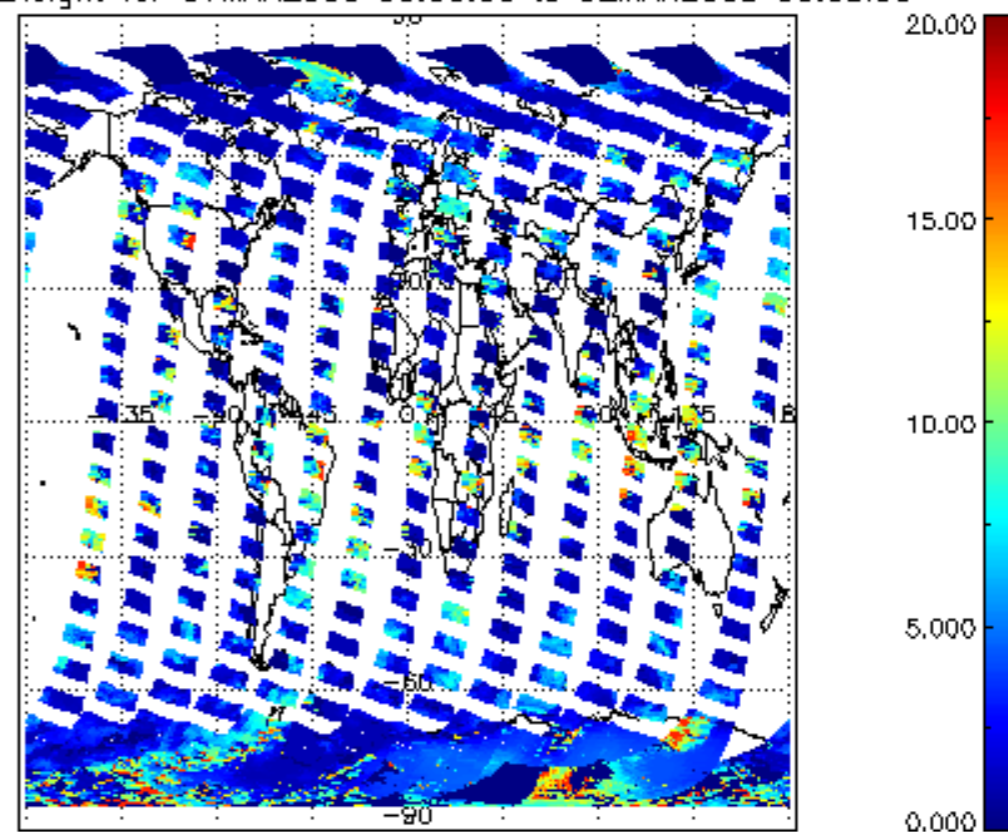
cL_top_height for 01MAR2008 00:00:00 to 02MAR2008 00:00:00
