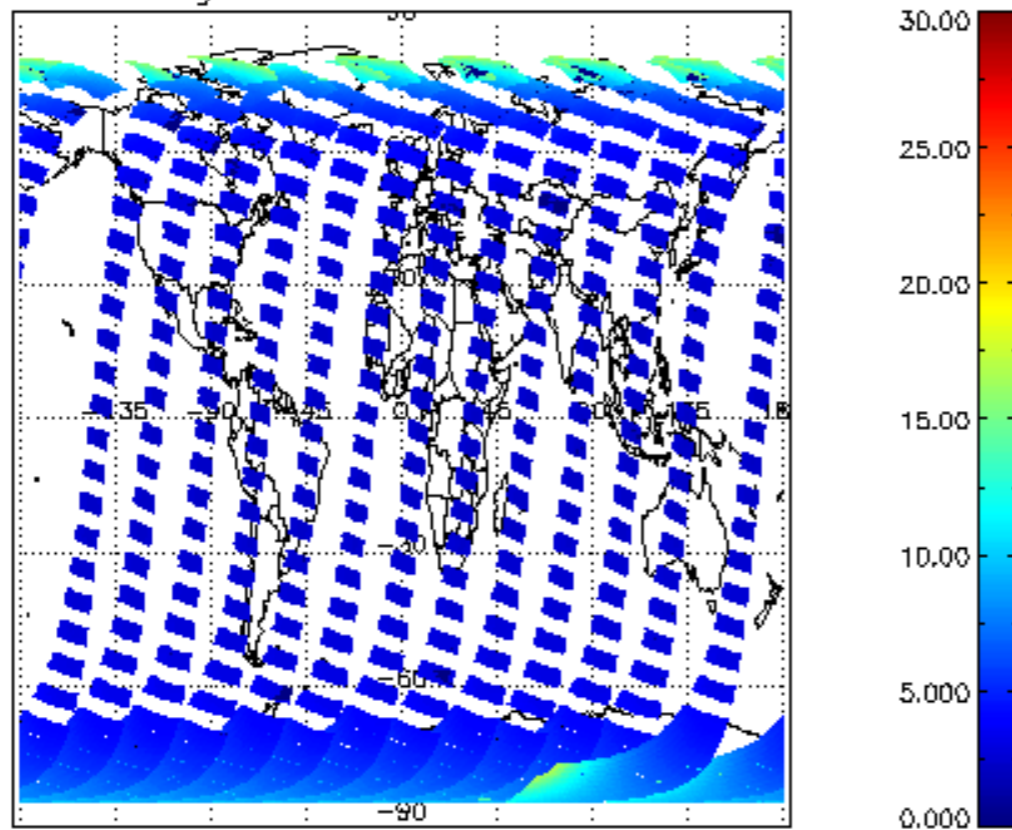
SCIOL2P_NADUV1NO2_amf_gr for 01MAR2008 00:00:00 to 02MAR2008 00:00:00
