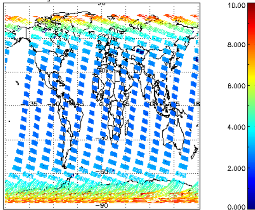
SCIOL2P_NADUV003_amf_gr for 01MAR2008 00:00:00 to 02MAR2008 00:00:00
