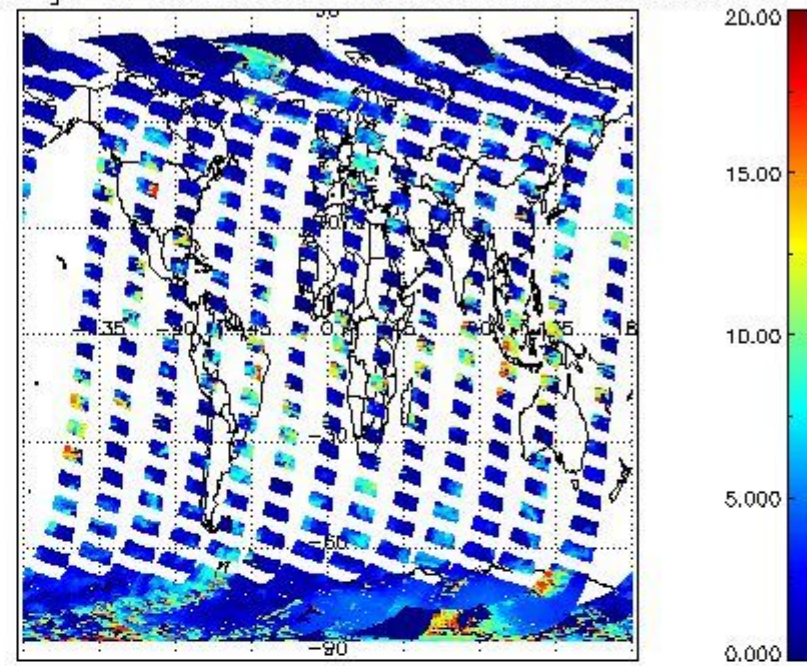
cLtop_height for 01MAR2008 00:00:00 to 02MAR2008 00:00:00
