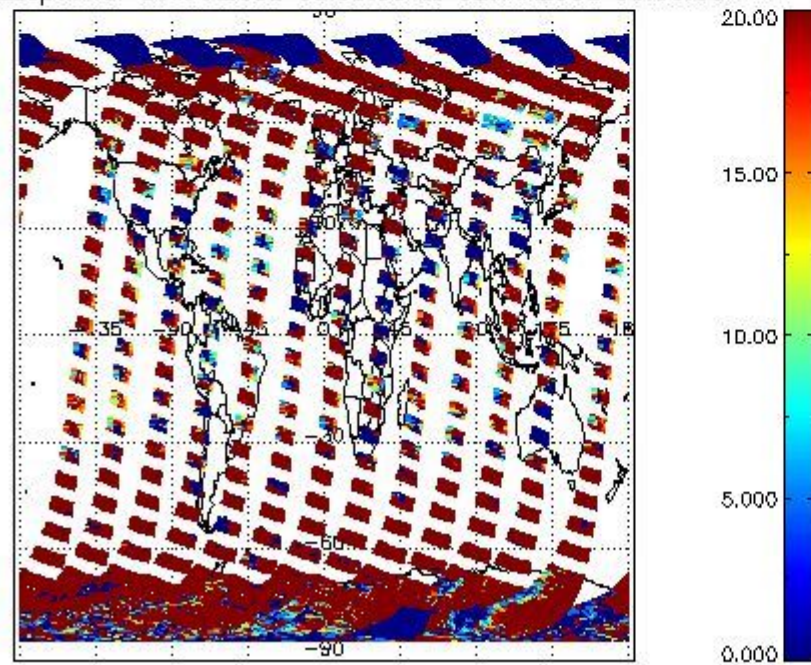
cLopt_depth for 01MAR2008 00:00:00 to 02MAR2008 00:00:00
