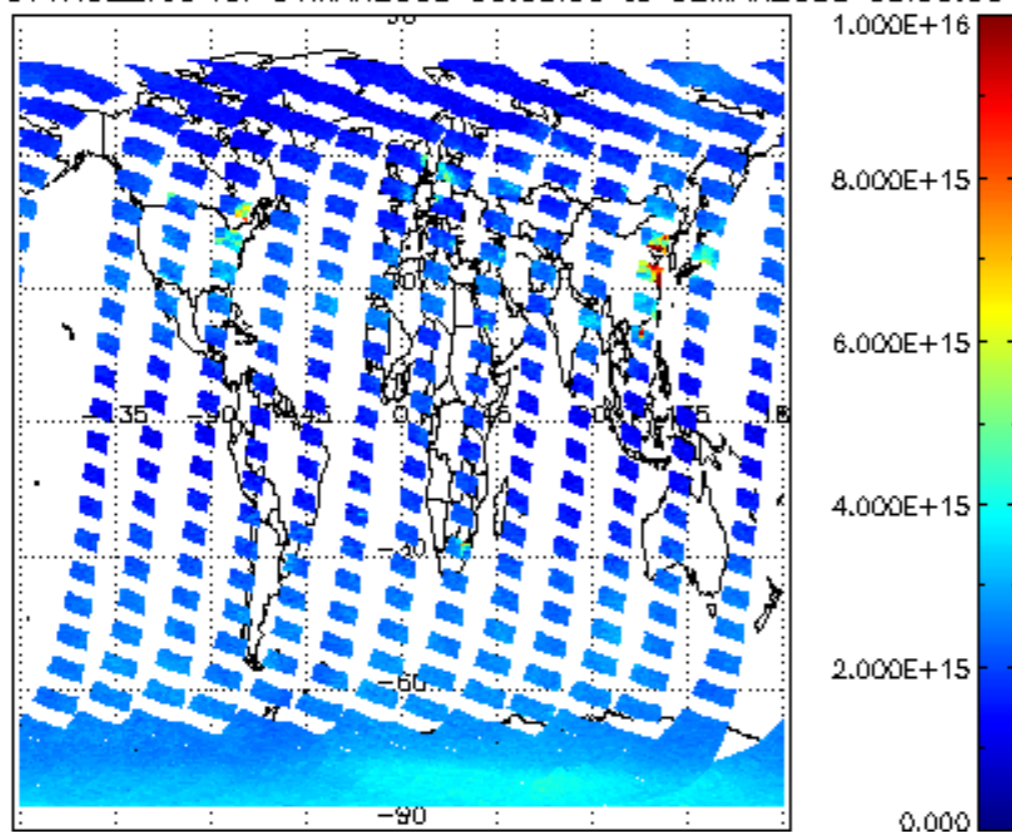
SCIOL2P_NADUV1NO2_vcd for 01MAR2008 00:00:00 to 02MAR2008 00:00:00
