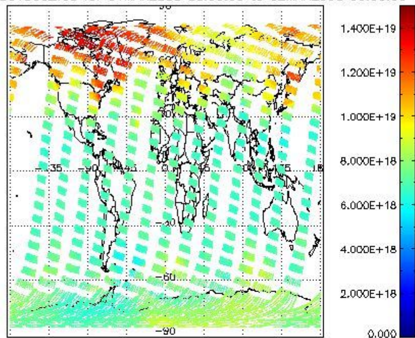
SCIOL2P_NADUV003_vcd for 01MAR2008 00:00:00 to 02MAR2008 00:00:00 SCIOL2P_NADUV003_vcd_err for 01MAR2008 00:00:00 to 02MAR2008 00:00:00
