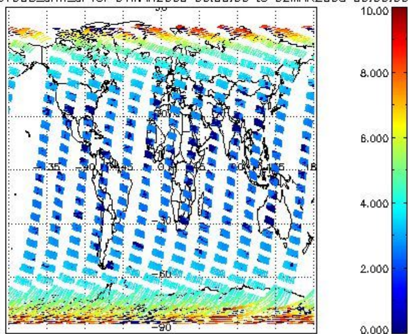
SCIOL2P_NADUV003_amf_gr for 01MAR2008 00:00:00 to 02MAR2008 00:00:00 SCIOL2P_NADUV003_amf_cl for 01MAR2008 00:00:00 to 02MAR2008 00:00:00
