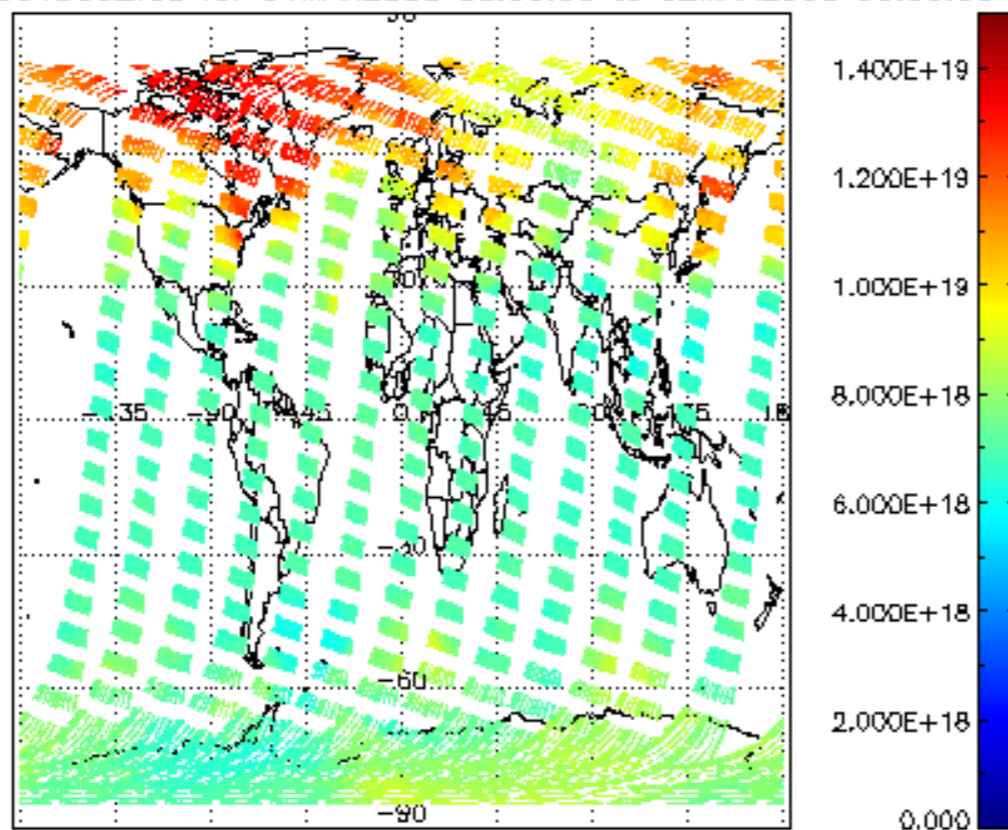
SCIOL2P_NADUV003_vcd for 01MAR2008 00:00:00 to 02MAR2008 00:00:00
