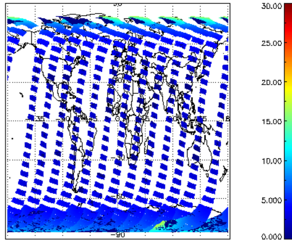
SCIOL2P_NADUV1NO2_amf_cl for 01MAR2008 00:00:00 to 02MAR2008 00:00:00
