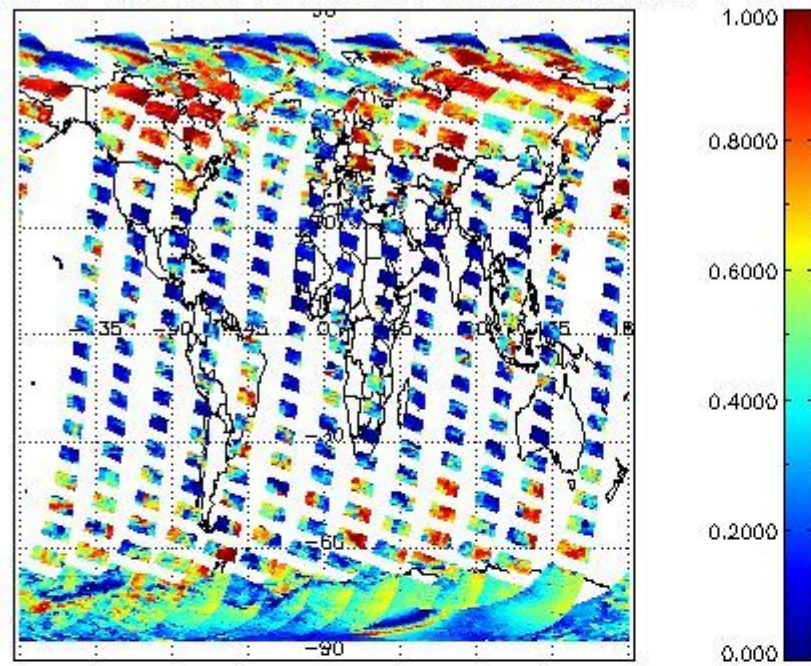
cLfrac for 01MAR2008 00:00:00 to 02MAR2008 00:00:00
