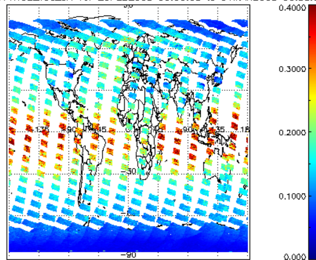
SCIOL2P_NADUV1NO2_vcd_err for 29FEB2008 00:00:00 to 01MAR2008 00:00:00
