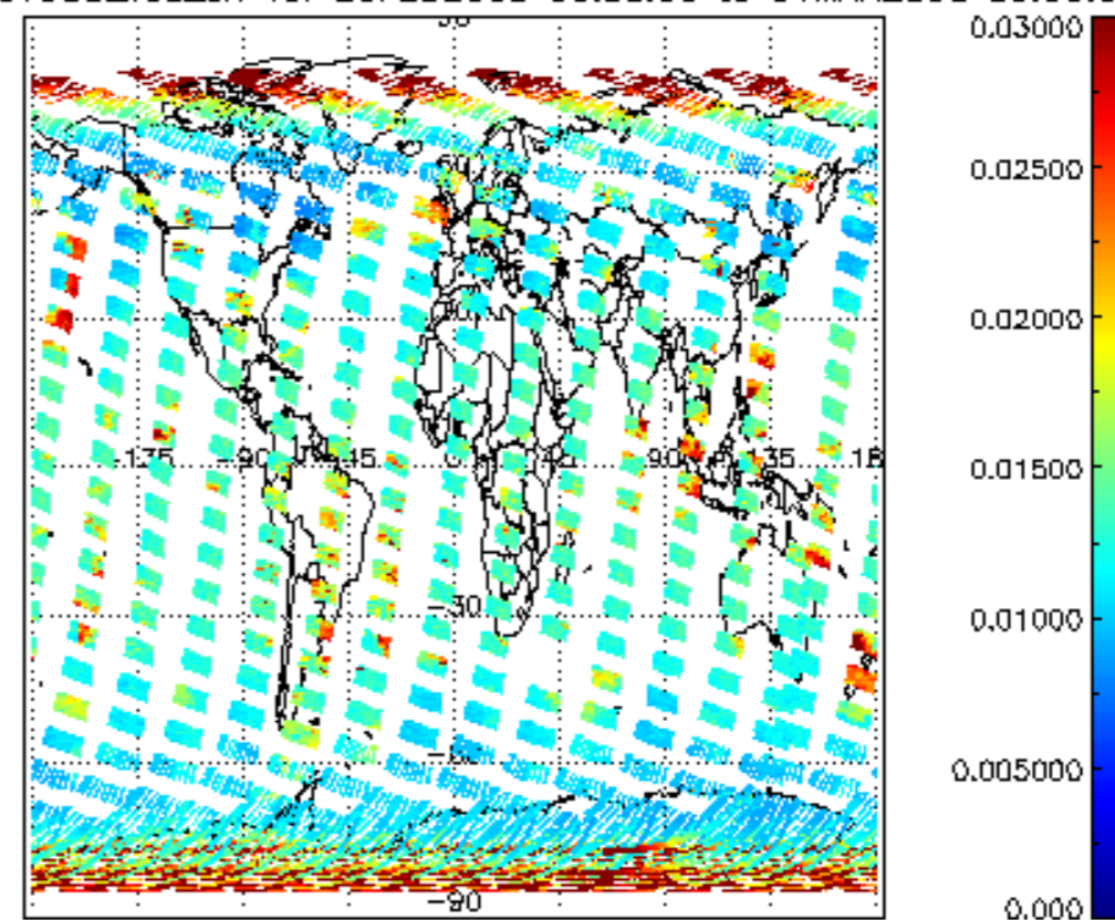
SCIOL2P_NADUV003_vcd_err for 29FEB2008 00:00:00 to 01MAR2008 00:00:00
