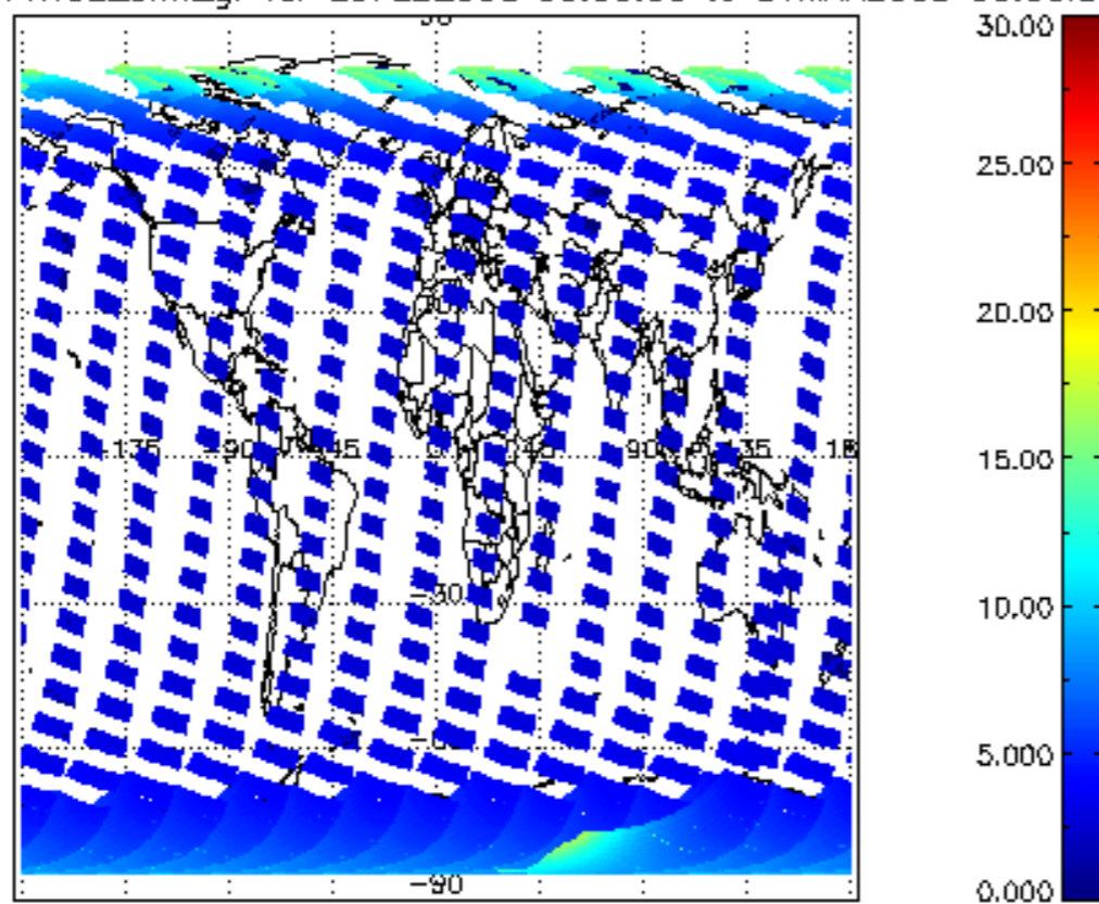
SCIOL2P_NADUV1NO2_amf_gr for 29FEB2008 00:00:00 to 01MAR2008 00:00:00
