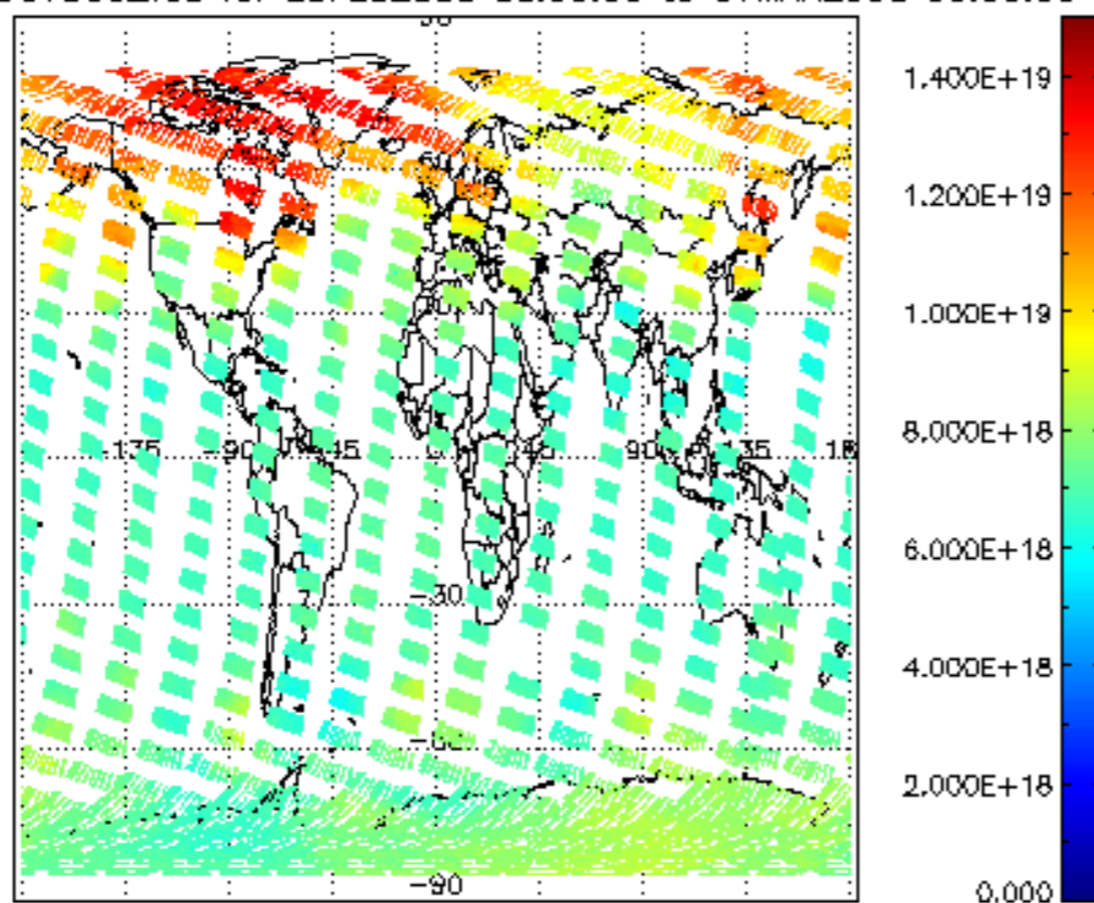
SCIOL2P_NADUV003_vcd for 29FEB2008 00:00:00 to 01MAR2008 00:00:00
