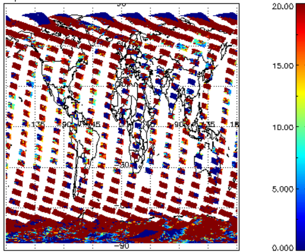
cL_opt_depth for 29FEB2008 00:00:00 to 01MAR2008 00:00:00
