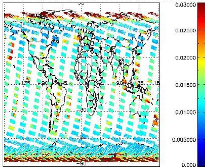
SCIOL2P_NADUV003_vcd_err for 29FEB2008 00:00:00 to 01MAR2008 00:00:00
