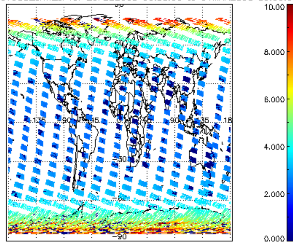
SCIOL2P_NADUV003_amf_cl for 29FEB2008 00:00:00 to 01MAR2008 00:00:00
