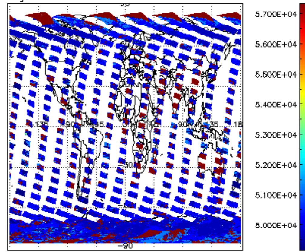
cloud_flags for 29FEB2008 00:00:00 to 01MAR2008 00:00:00
