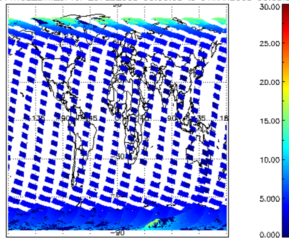
SCIOL2P_NADUV1NO2_amf_cl for 29FEB2008 00:00:00 to 01MAR2008 00:00:00
