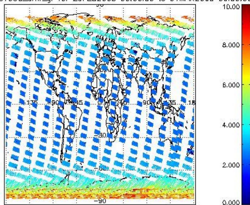
SCIOL2P_NADUV003_amf_gr for 29FEB2008 00:00:00 to 01MAR2008 00:00:00
