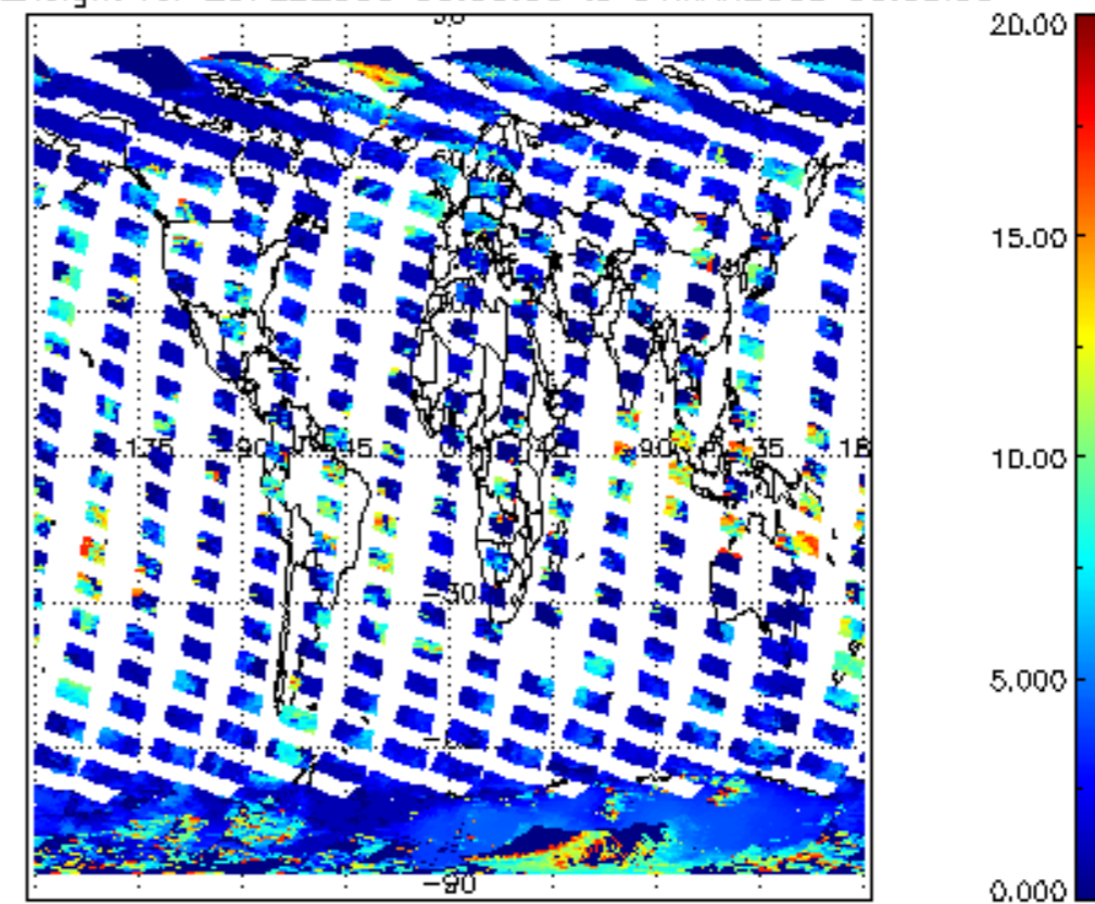
cL_top_height for 29FEB2008 00:00:00 to 01MAR2008 00:00:00
