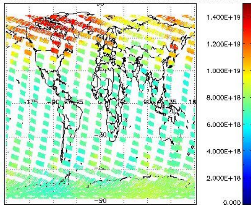
SCIOL2P_NADUV003_vcd for 29FEB2008 00:00:00 to 01MAR2008 00:00:00
