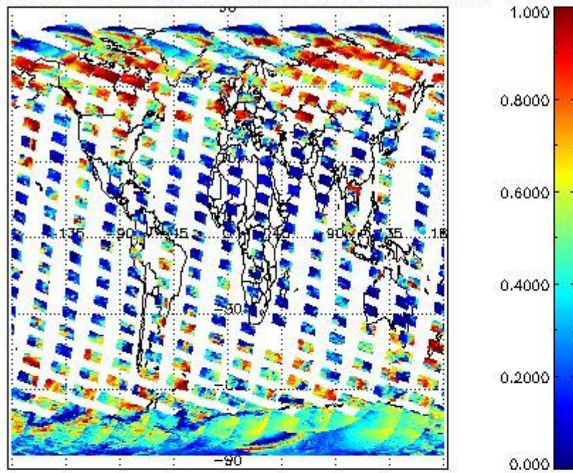
cLfrac for 29FEB2008 00:00:00 to 01MAR2008 00:00:00
