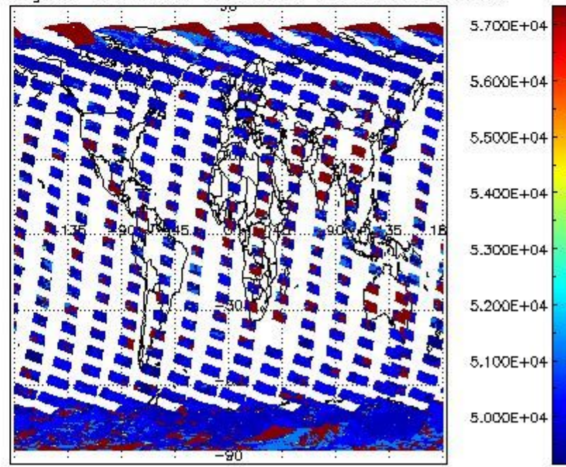
cloud_flags for 29FEB2008 00:00:00 to 01MAR2008 00:00:00
