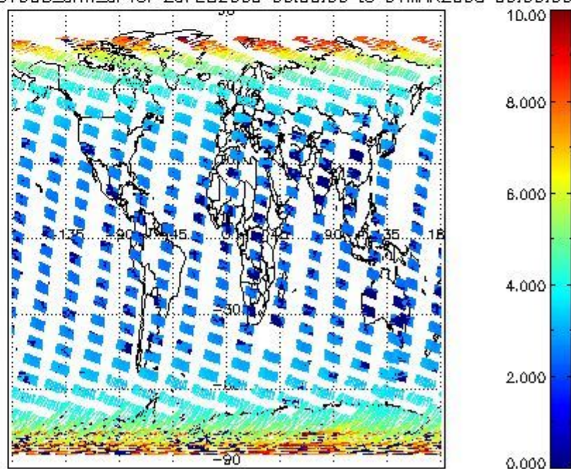
SCIOL2P_NADUV003_amf_sl for 29FEB2008 00:00:00 to 01MAR2008 00:00:00
