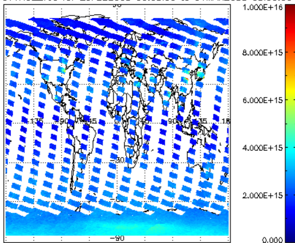
SCIOL2P_NADUV1NO2_vcd for 29FEB2008 00:00:00 to 01MAR2008 00:00:00
