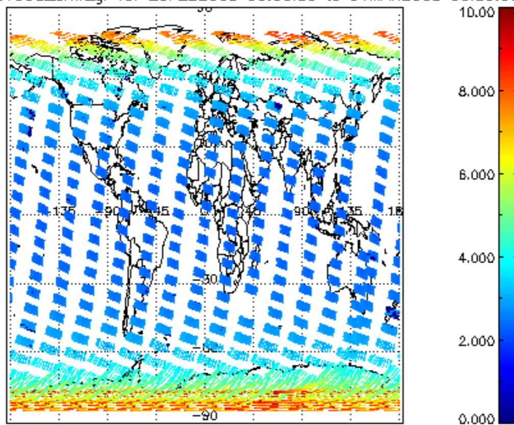
SCIOL2P_NADUV003_amf_gr for 29FEB2008 00:00:00 to 01MAR2008 00:00:00
