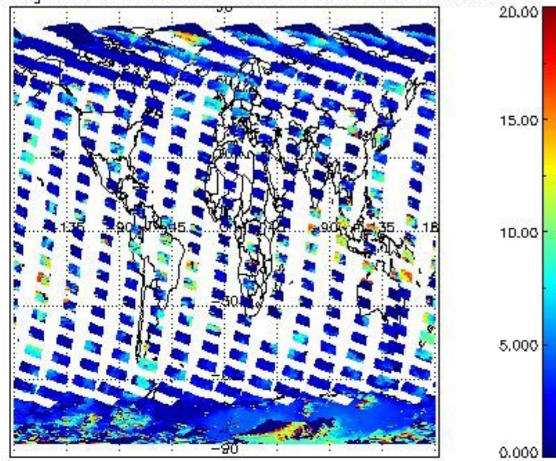
cLtop_height for 29FEB2008 00:00:00 to 01MAR2008 00:00:00
