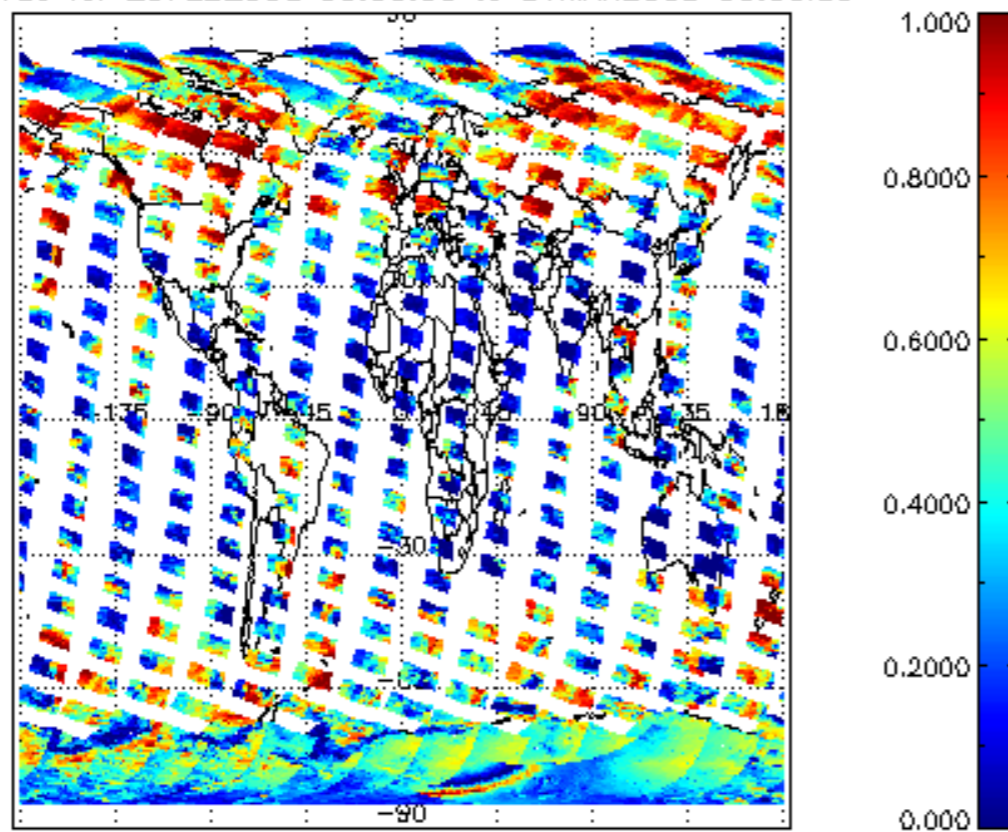
cL_frac for 29FEB2008 00:00:00 to 01MAR2008 00:00:00
