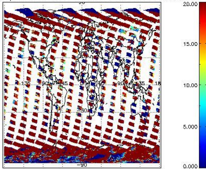
cLopt_depth for 29FEB2008 00:00:00 to 01MAR2008 00:00:00
