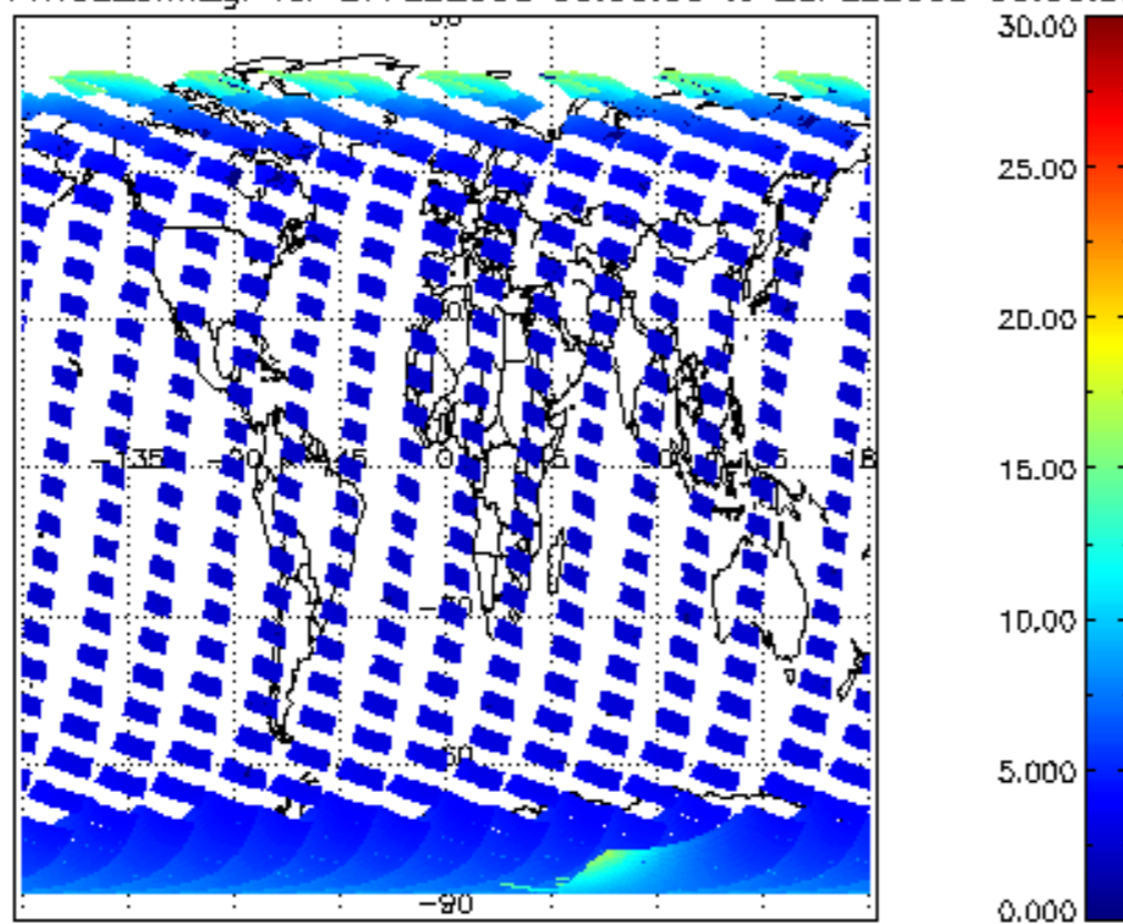
SCIOL2P_NADUV1NO2_amf_gr for 27FEB2008 00:00:00 to 28FEB2008 00:00:00
