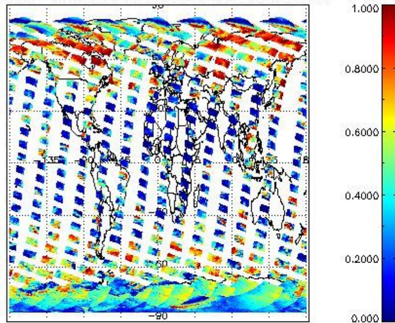
cL_frac for 27FEB2008 00:00:00 to 28FEB2008 00:00:00
