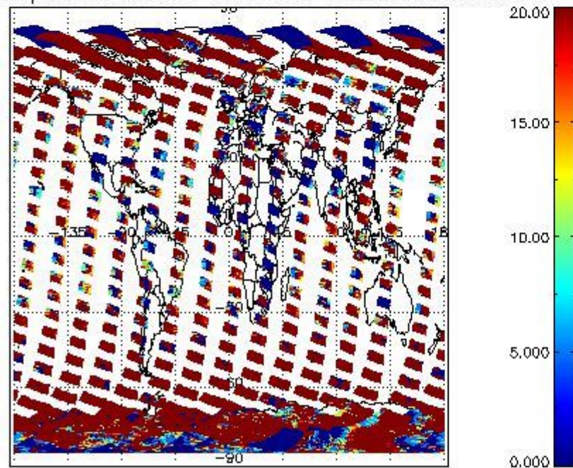
cL_opt_depth for 27FEB2008 00:00:00 to 28FEB2008 00:00:00
