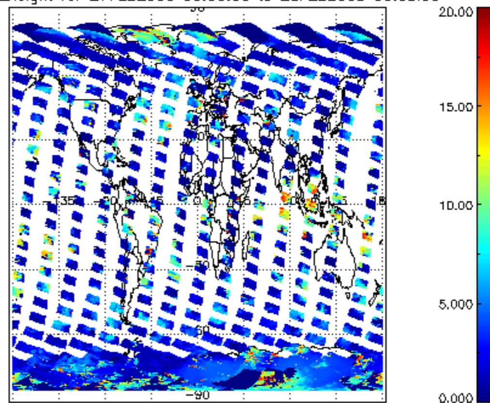
cI_top_height for 27FEB2008 00:00:00 to 28FEB2008 00:00:00
