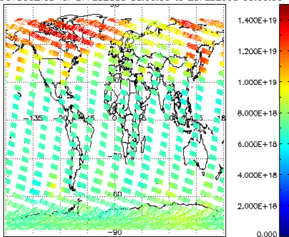
SCIOL2P_NADUV003_vcd for 27FEB2008 00:00:00 to 28FEB2008 00:00:00
