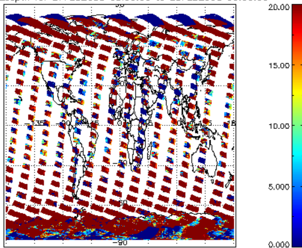
cI_opt_depth for 27FEB2008 00:00:00 to 28FEB2008 00:00:00
