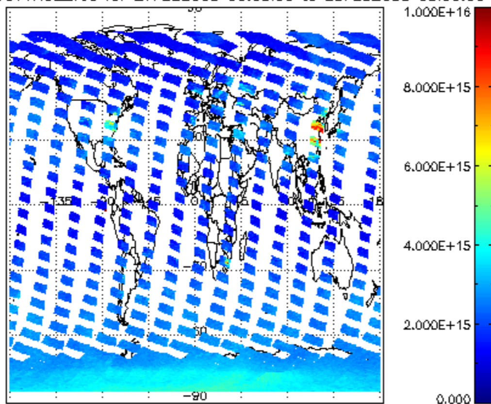
SCIOL2P_NADUV1NO2_vcd for 27FEB2008 00:00:00 to 28FEB2008 00:00:00
