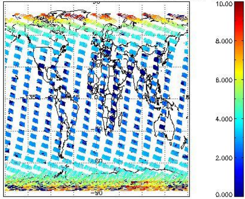
SCIOL2P_NADUV003_amf_cl for 27FEB2008 00:00:00 to 28FEB2008 00:00:00
