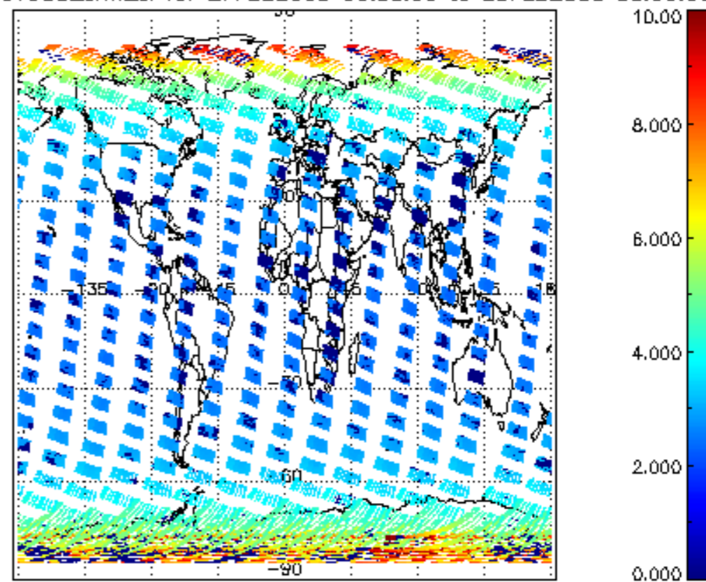
SCIOL2P_NADUV003_amf_cl for 27FEB2008 00:00:00 to 28FEB2008 00:00:00
