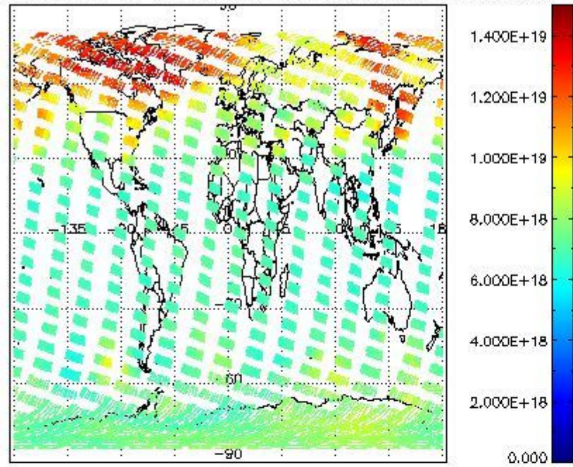
SCIOL2P_NADUV003_vcd for 27FEB2008 00:00:00 to 28FEB2008 00:00:00
