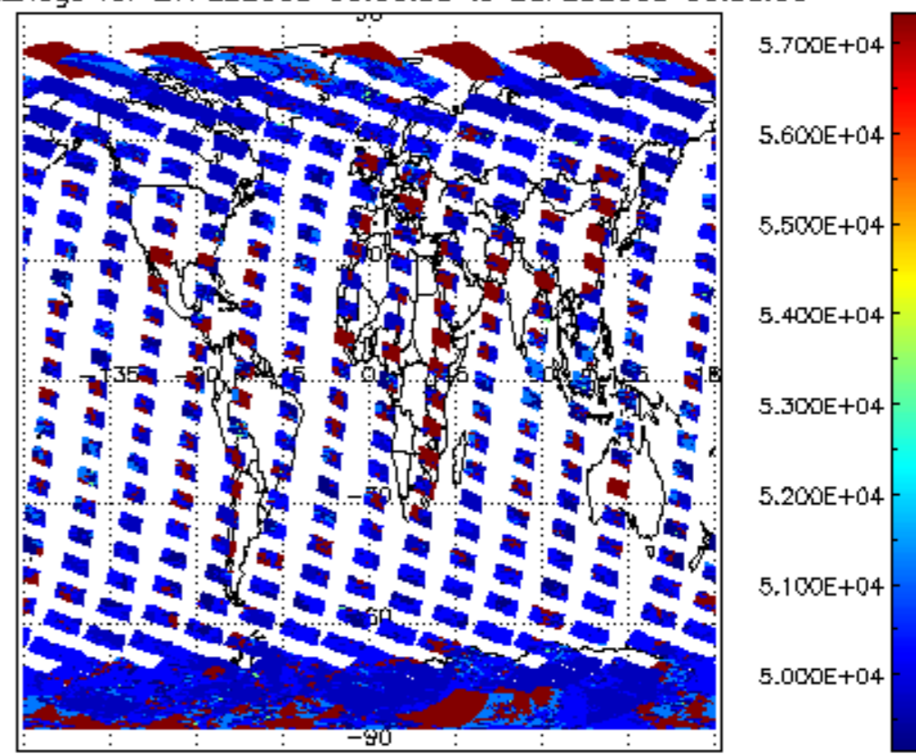
cloud_flags for 27FEB2008 00:00:00 to 28FEB2008 00:00:00
