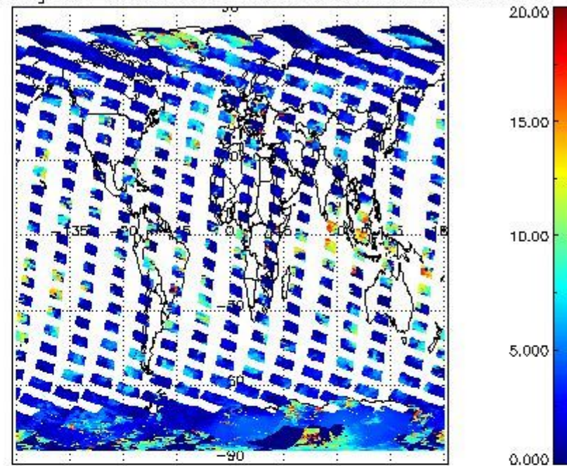
cL_top_height for 27FEB2008 00:00:00 to 28FEB2008 00:00:00
