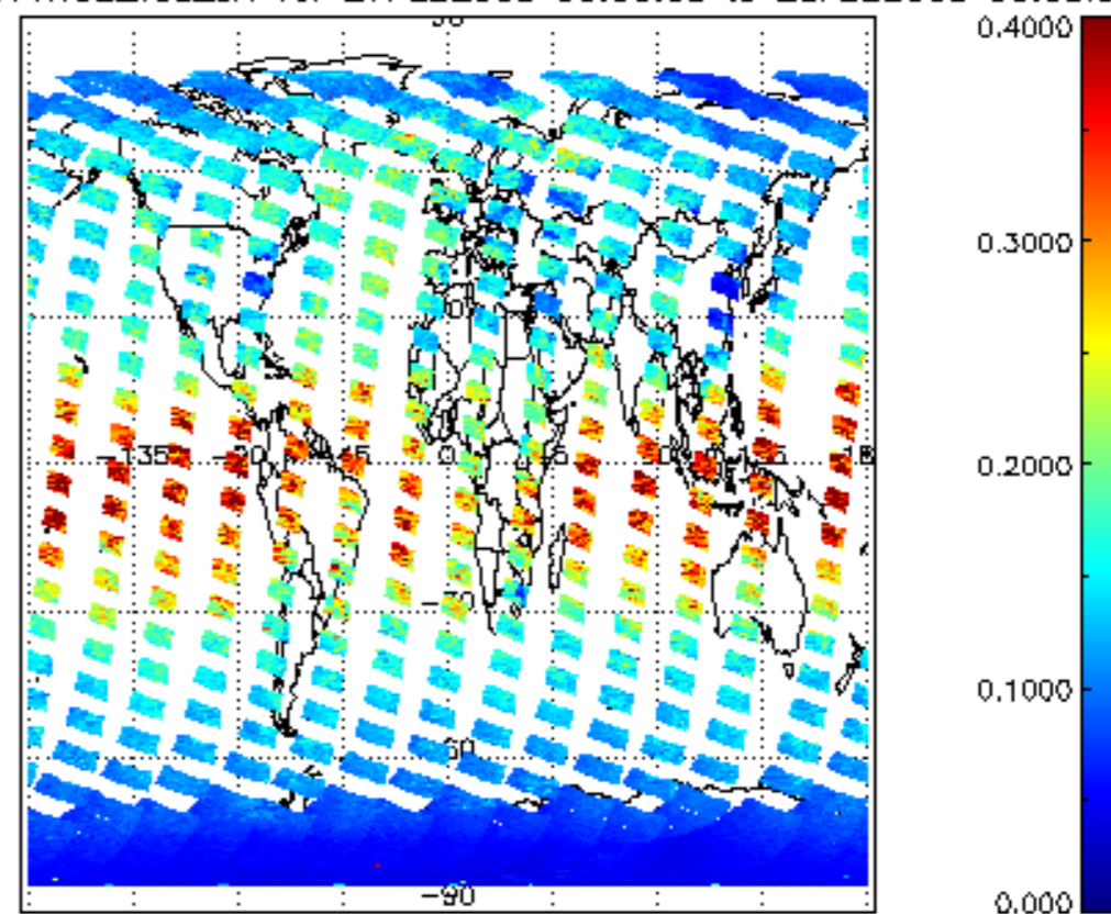
SCIOL2P_NADUV1NO2_vcd_err for 27FEB2008 00:00:00 to 28FEB2008 00:00:00
