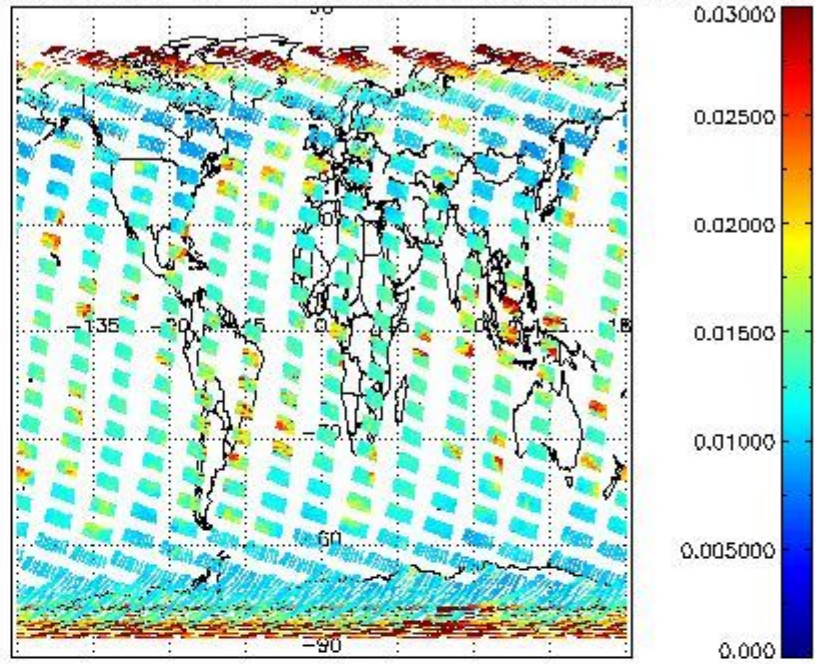
SCIOL2P_NADUV003_vcd_err for 27FEB2008 00:00:00 to 28FEB2008 00:00:00
