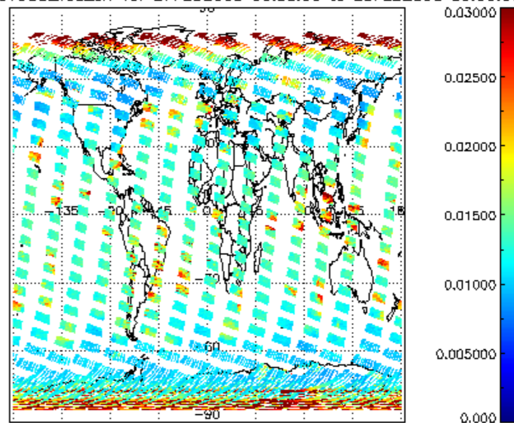
SCIOL2P_NADUV003_vcd_err for 27FEB2008 00:00:00 to 28FEB2008 00:00:00
