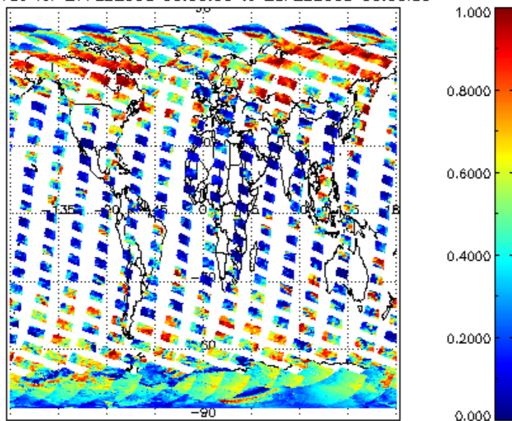
cI_frac for 27FEB2008 00:00:00 to 28FEB2008 00:00:00
