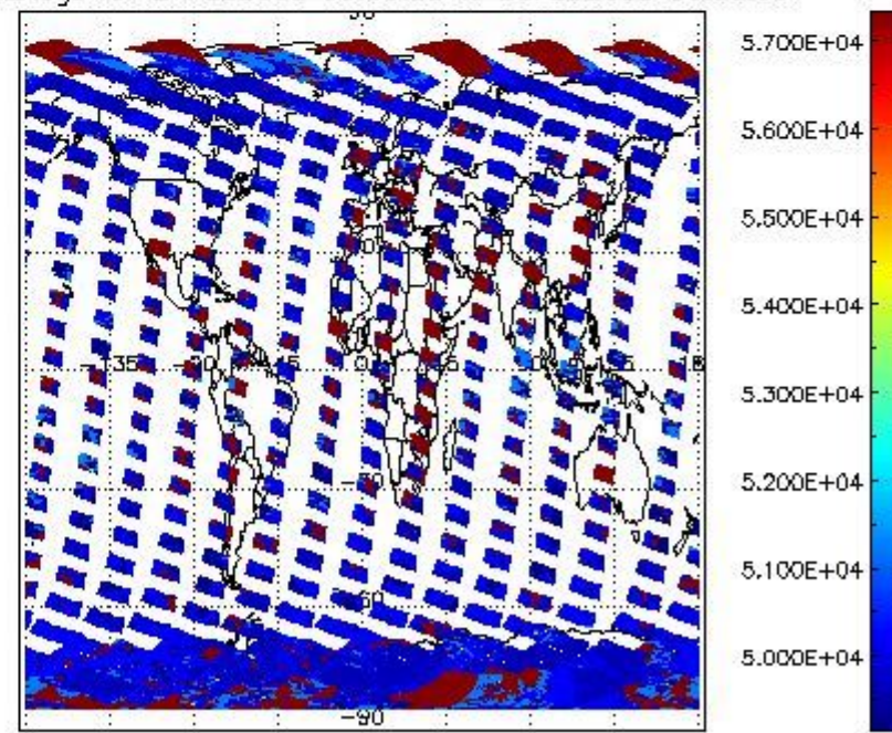
cloud_flags for 27FEB2008 00:00:00 to 28FEB2008 00:00:00
