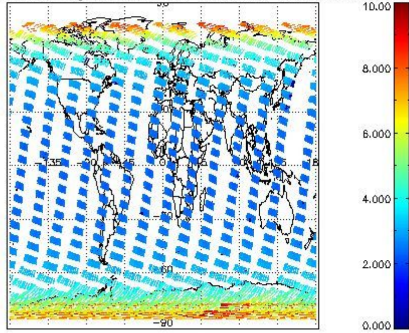
SCIOL2P_NADUV003_amf_gr for 27FEB2008 00:00:00 to 28FEB2008 00:00:00
