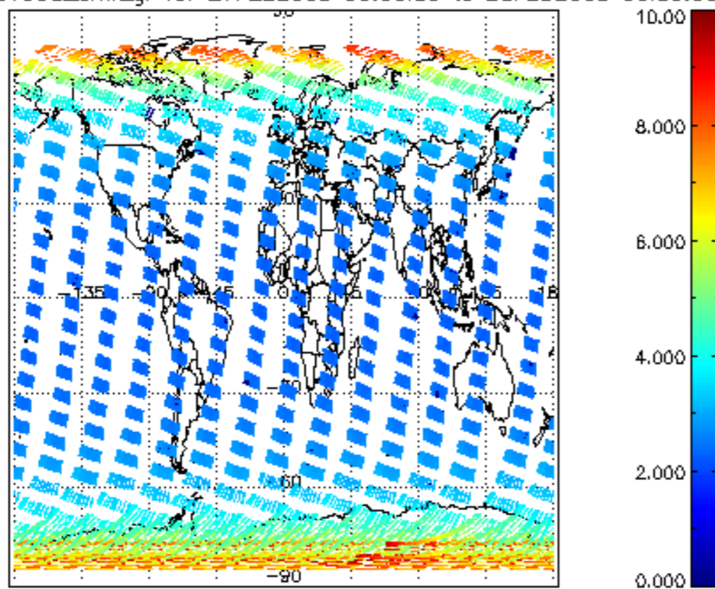
SCIOL2P_NADUV003_amf_gr for 27FEB2008 00:00:00 to 28FEB2008 00:00:00
