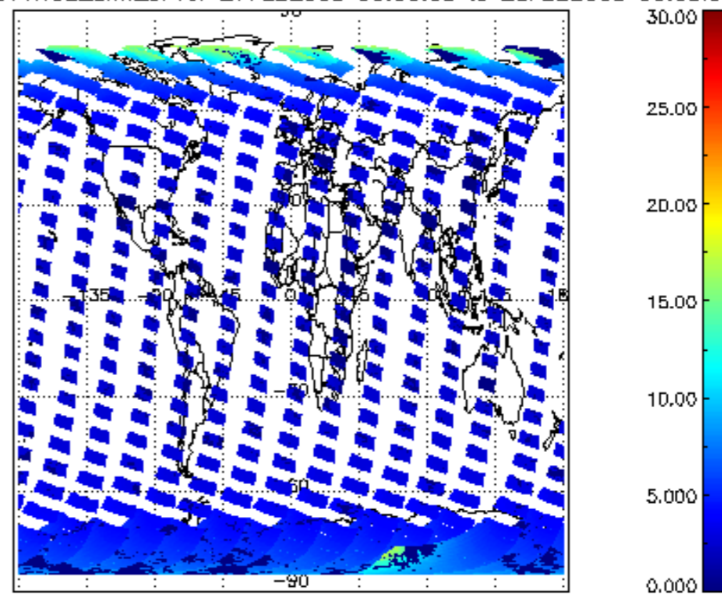
SCIOL2P_NADUV1NO2_amf_cl for 27FEB2008 00:00:00 to 28FEB2008 00:00:00
