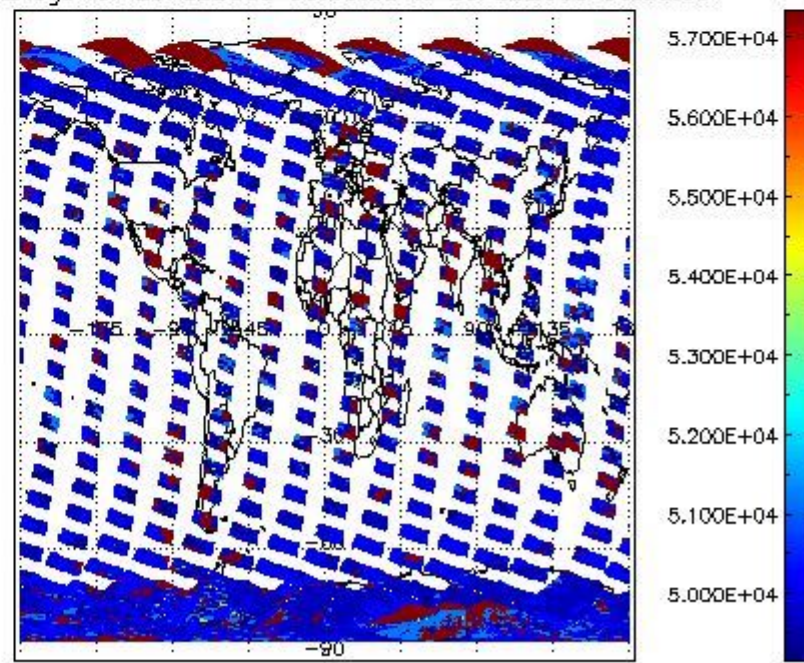
cloud_flags for 25FEB2008 00:00:00 to 26FEB2008 00:00:00
