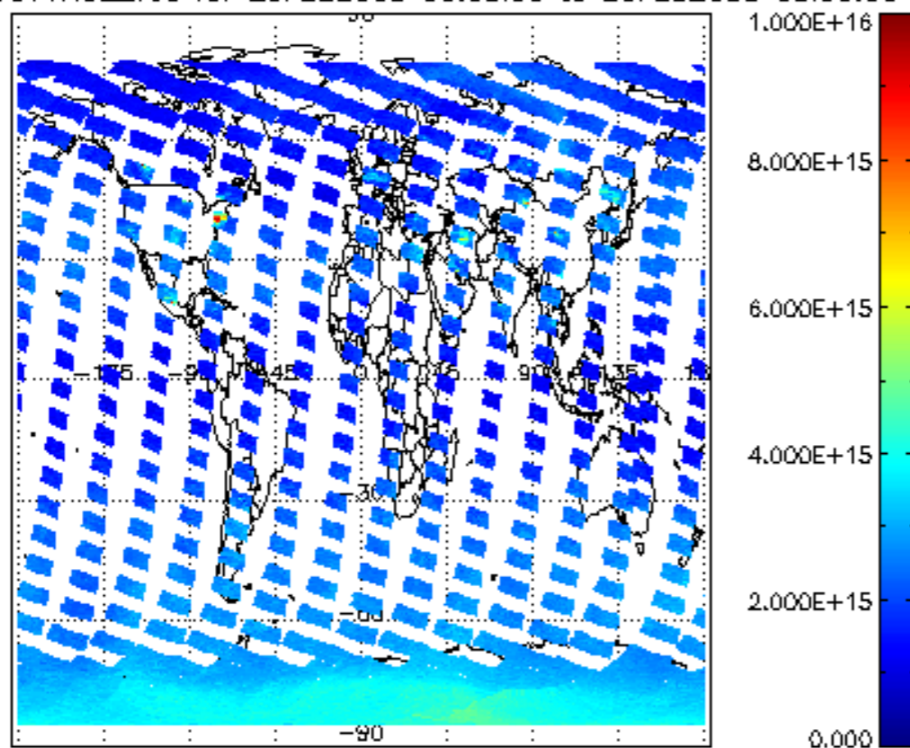
SCIOL2P_NADUV1NO2_vcd for 25FEB2008 00:00:00 to 26FEB2008 00:00:00
