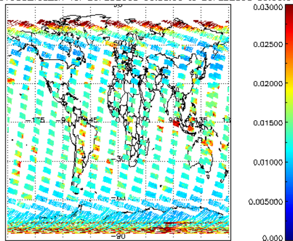
SCIOL2P_NADUV003_vcd_err for 25FEB2008 00:00:00 to 26FEB2008 00:00:00
