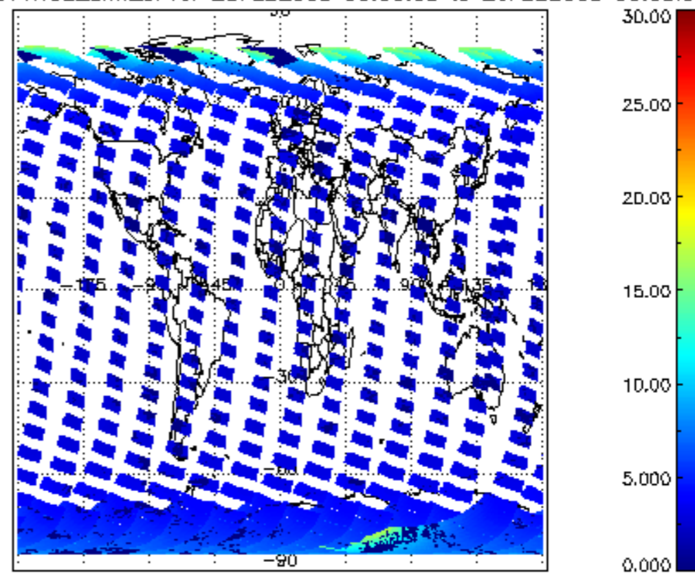
SCIOL2P_NADUV1NO2_amf_cl for 25FEB2008 00:00:00 to 26FEB2008 00:00:00
