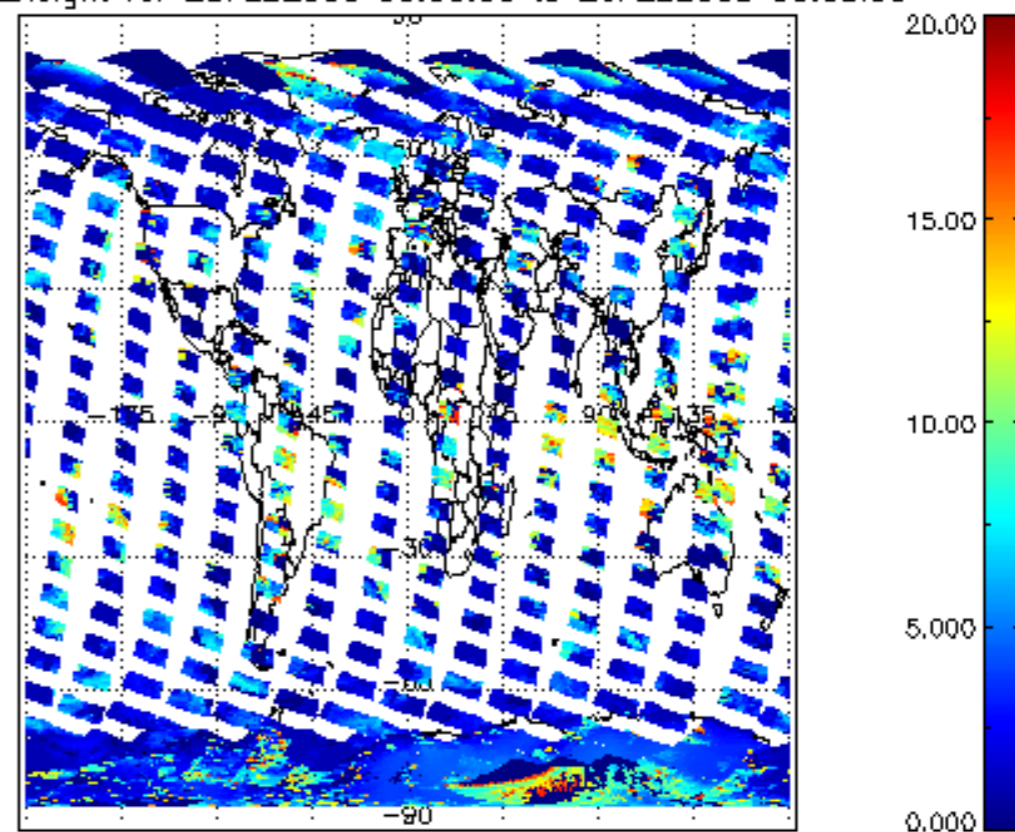
cl_top_height for 25FEB2008 00:00:00 to 26FEB2008 00:00:00
