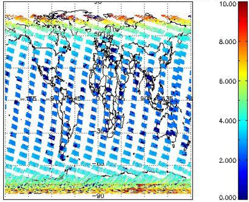
SCIOL2P_NADUV003_amf_cl for 25FEB2008 00:00:00 to 26FEB2008 00:00:00
