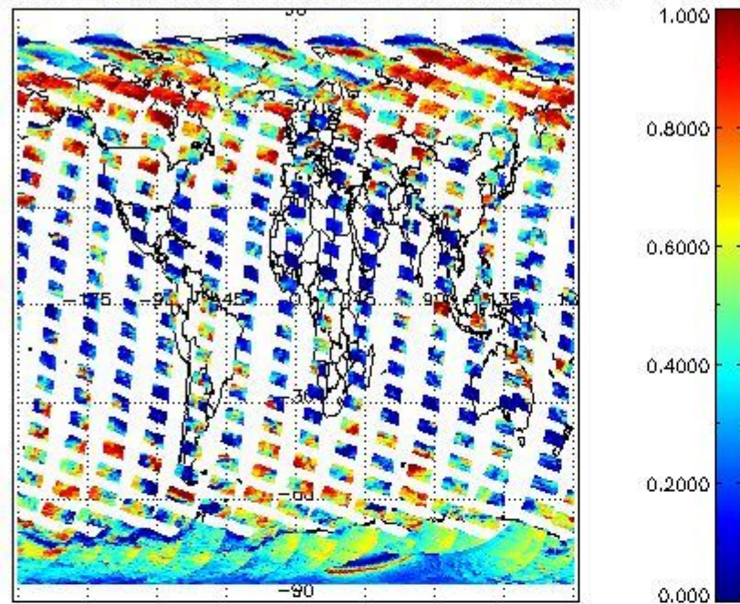
cL_frac for 25FEB2008 00:00:00 to 26FEB2008 00:00:00
