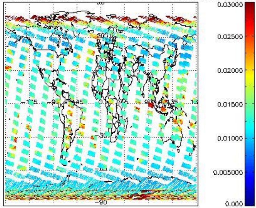
SCIOL2P_NADUV003_vcd_err for 25FEB2008 00:00:00 to 26FEB2008 00:00:00
