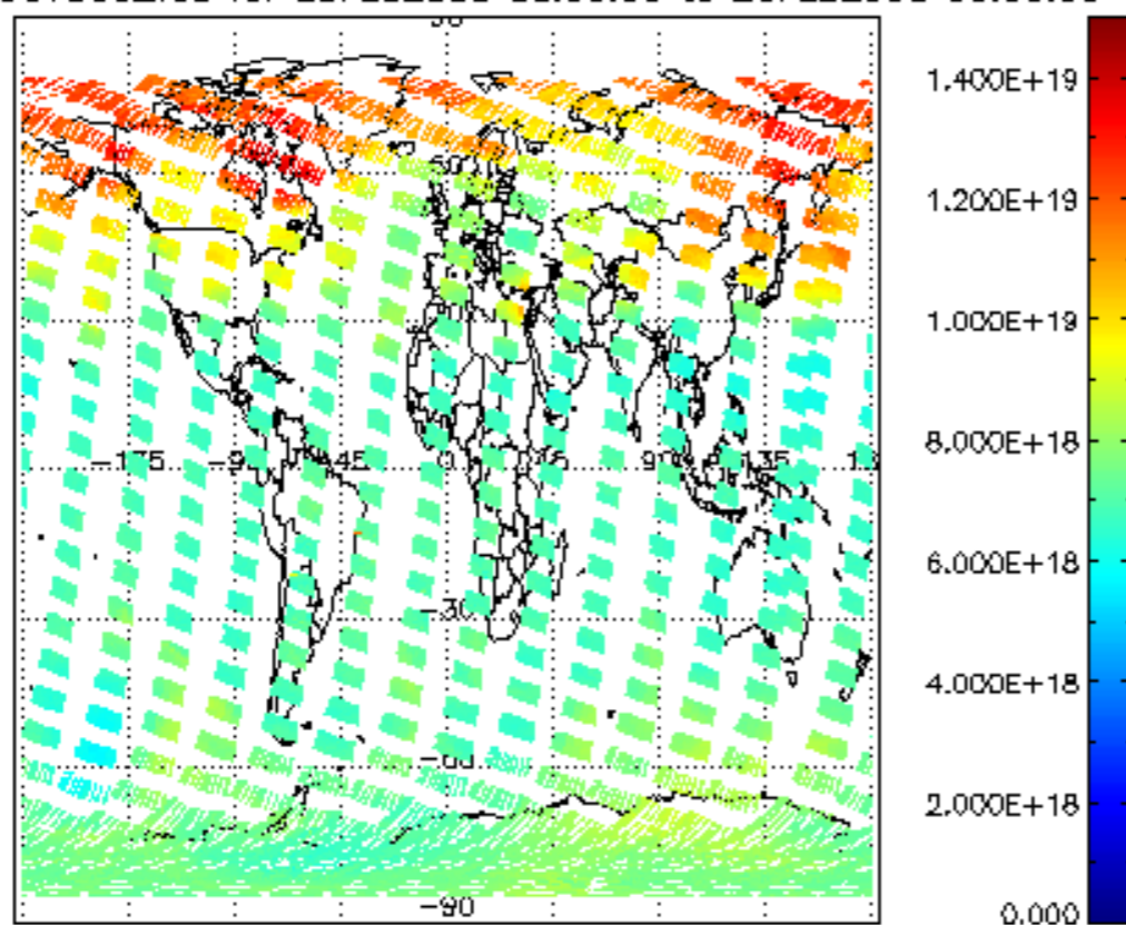
SCIOL2P_NADUV003_vcd for 25FEB2008 00:00:00 to 26FEB2008 00:00:00
