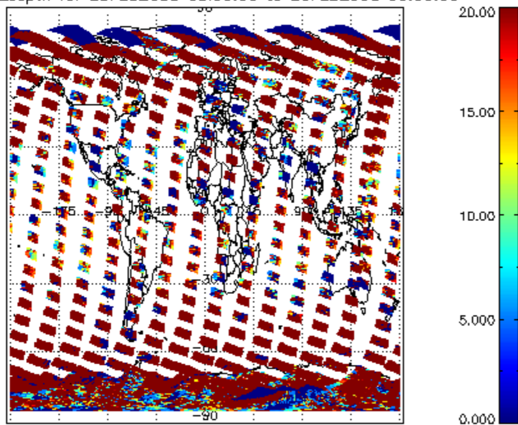
cl_opt_depth for 25FEB2008 00:00:00 to 26FEB2008 00:00:00
