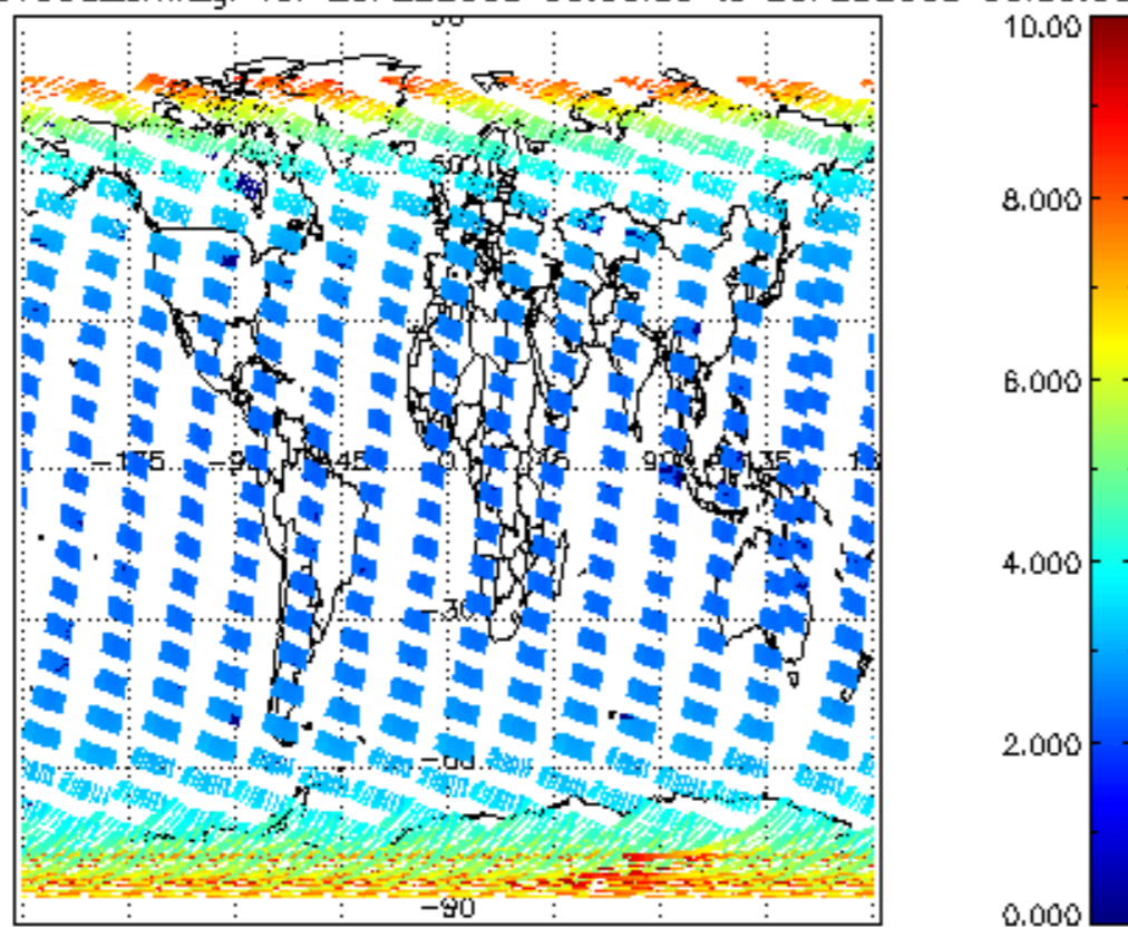
SCIOL2P_NADUV003_amf_gr for 25FEB2008 00:00:00 to 26FEB2008 00:00:00
