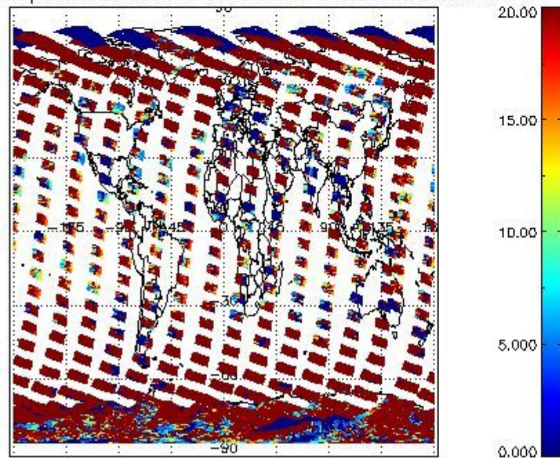
cL_opt_depth for 25FEB2008 00:00:00 to 26FEB2008 00:00:00
