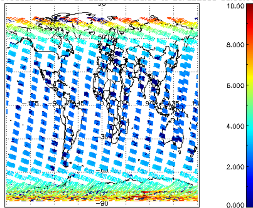
SCIOL2P_NADUV003_amf_cl for 25FEB2008 00:00:00 to 26FEB2008 00:00:00
