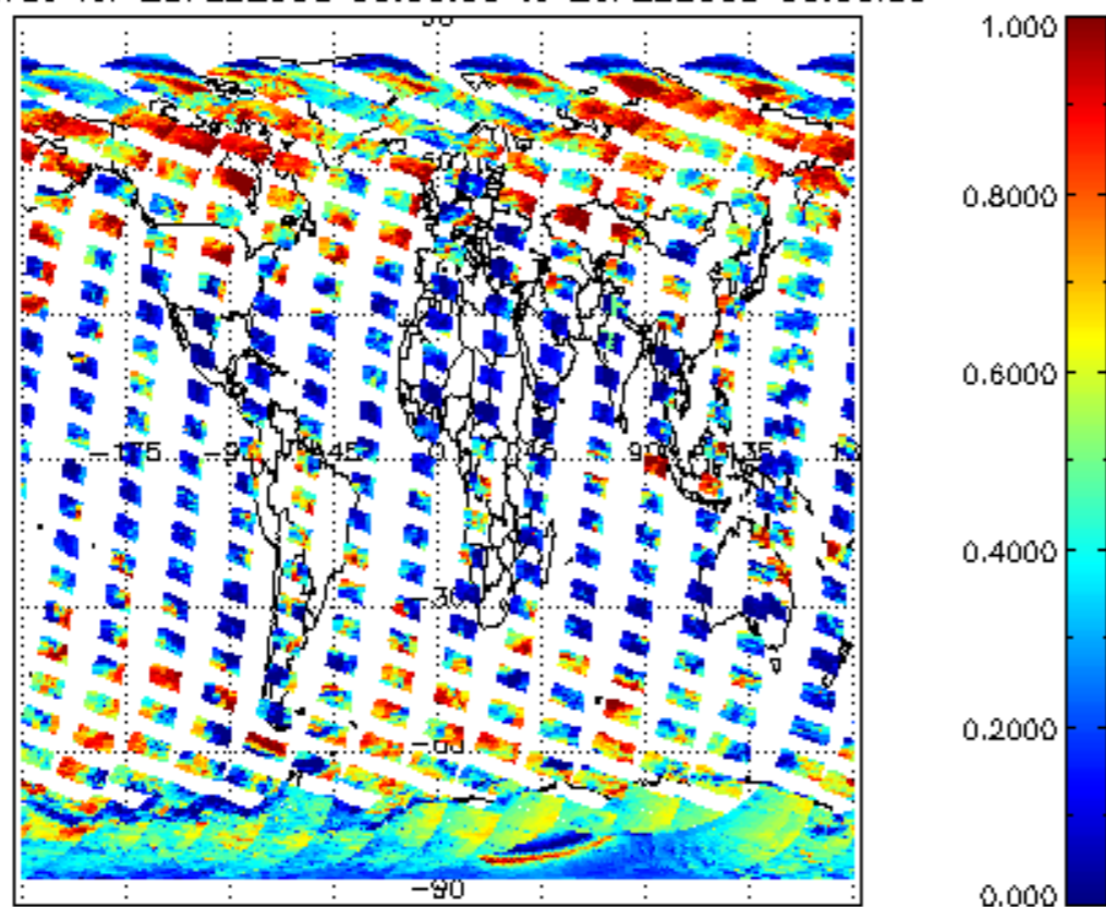
cl_frac for 25FEB2008 00:00:00 to 26FEB2008 00:00:00
