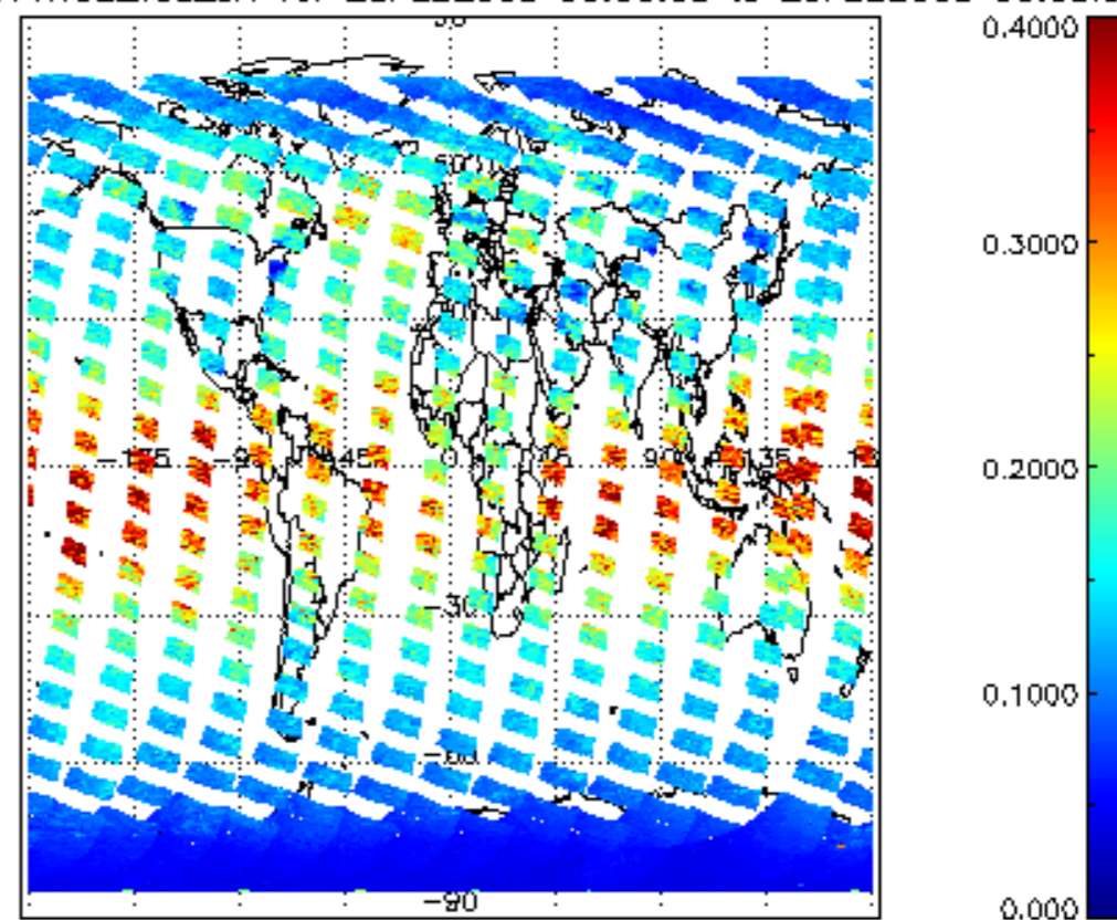
SCIOL2P_NADUV1NO2_vcd_err for 25FEB2008 00:00:00 to 26FEB2008 00:00:00
