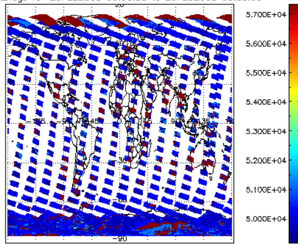
cloud_flags for 25FEB2008 00:00:00 to 26FEB2008 00:00:00
