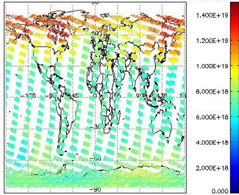
SCIOL2P_NADUV003_vcd for 25FEB2008 00:00:00 to 26FEB2008 00:00:00
