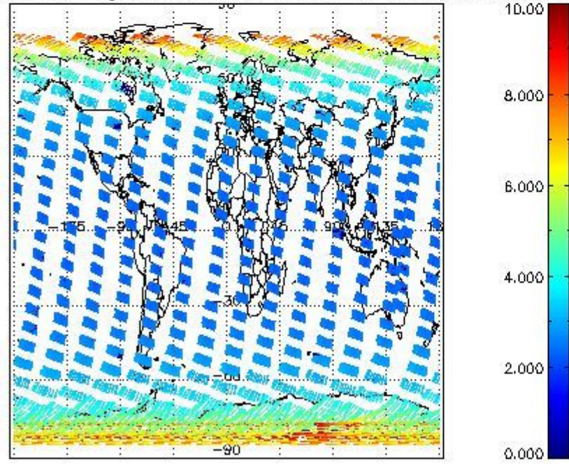
SCIOL2P_NADUV003_amf_gr for 25FEB2008 00:00:00 to 26FEB2008 00:00:00
