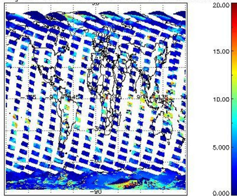
cL_top_height for 25FEB2008 00:00:00 to 26FEB2008 00:00:00
