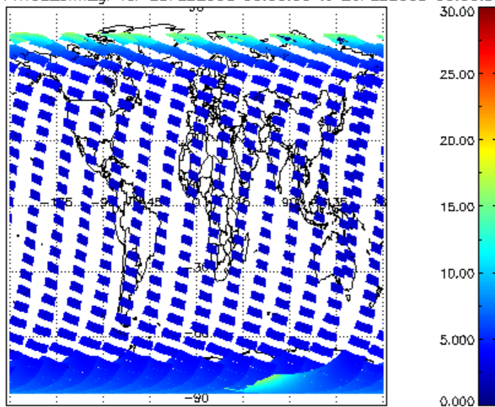
SCIOL2P_NADUV1NO2_amf_gr for 25FEB2008 00:00:00 to 26FEB2008 00:00:00
