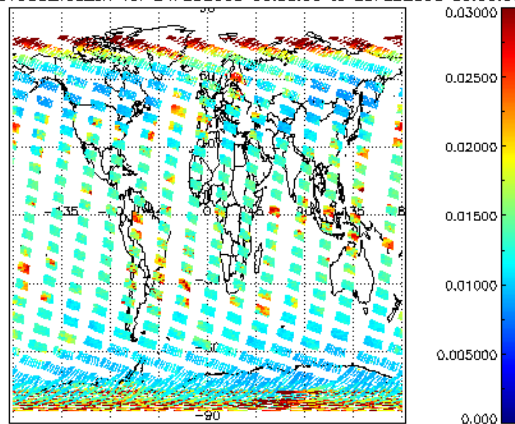
SCIOL2P_NADUV003_vcd_err for 24FEB2008 00:00:00 to 25FEB2008 00:00:00
