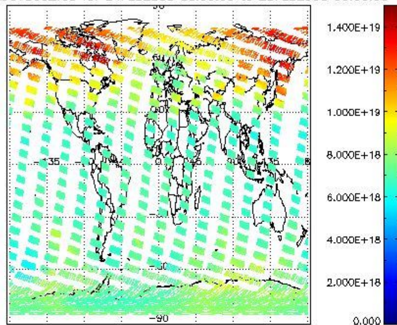
SCIOL2P_NADUV003_vcd for 24FEB2008 00:00:00 to 25FEB2008 00:00:00
