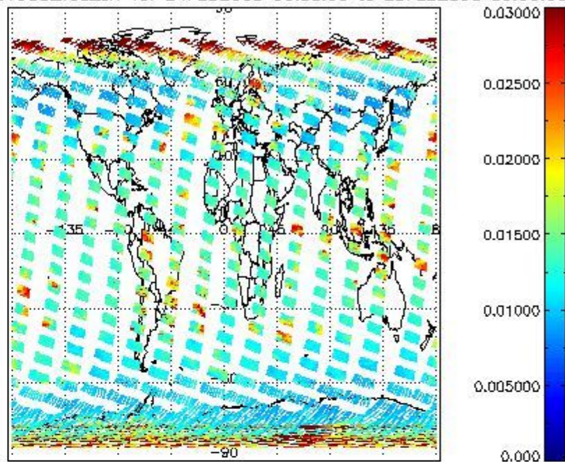
SCIOL2P_NADUV003_vcd_err for 24FEB2008 00:00:00 to 25FEB2008 00:00:00
