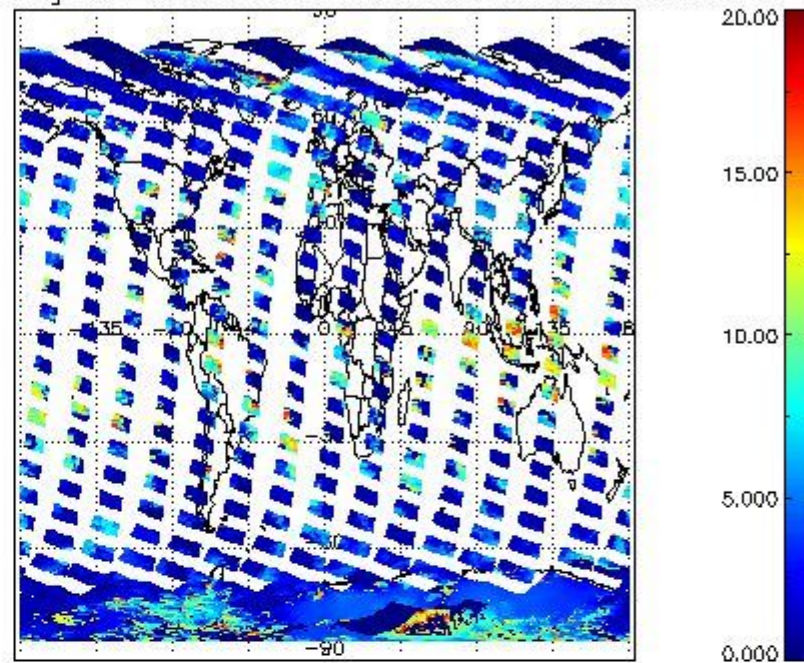
cL_top_height for 24FEB2008 00:00:00 to 25FEB2008 00:00:00
