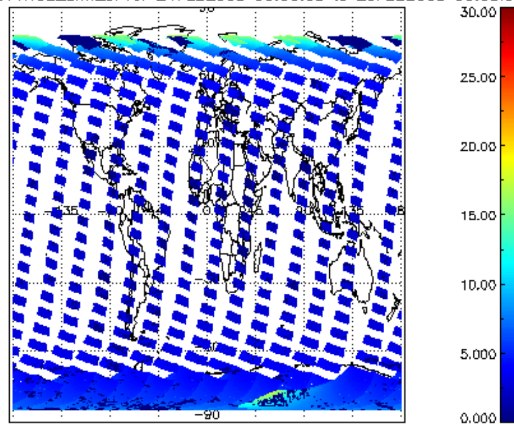
SCIOL2P_NADUV1NO2_amf_cl for 24FEB2008 00:00:00 to 25FEB2008 00:00:00
