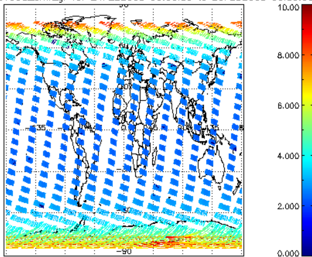
SCIOL2P_NADUV003_amf_gr for 24FEB2008 00:00:00 to 25FEB2008 00:00:00
