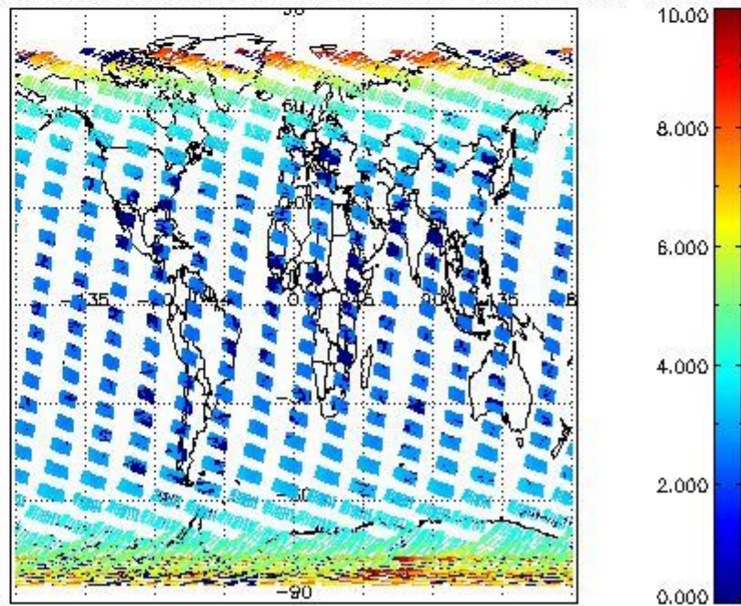
SCIOL2P_NADUV003_amf_cl for 24FEB2008 00:00:00 to 25FEB2008 00:00:00
