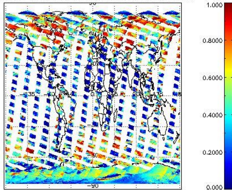
cLfrac for 24FEB2008 00:00:00 to 25FEB2008 00:00:00
