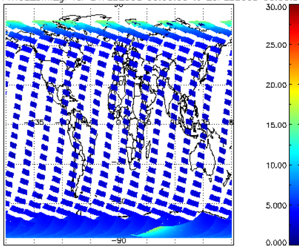
SCIOL2P_NADUV1NO2_amf_gr for 24FEB2008 00:00:00 to 25FEB2008 00:00:00
