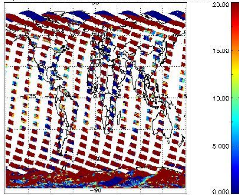
cLopt_depth for 24FEB2008 00:00:00 to 25FEB2008 00:00:00
