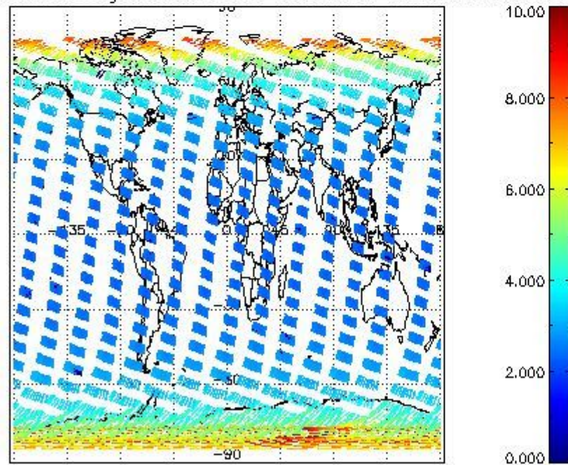
SCIOL2P_NADUV003_amf_gr for 24FEB2008 00:00:00 to 25FEB2008 00:00:00
