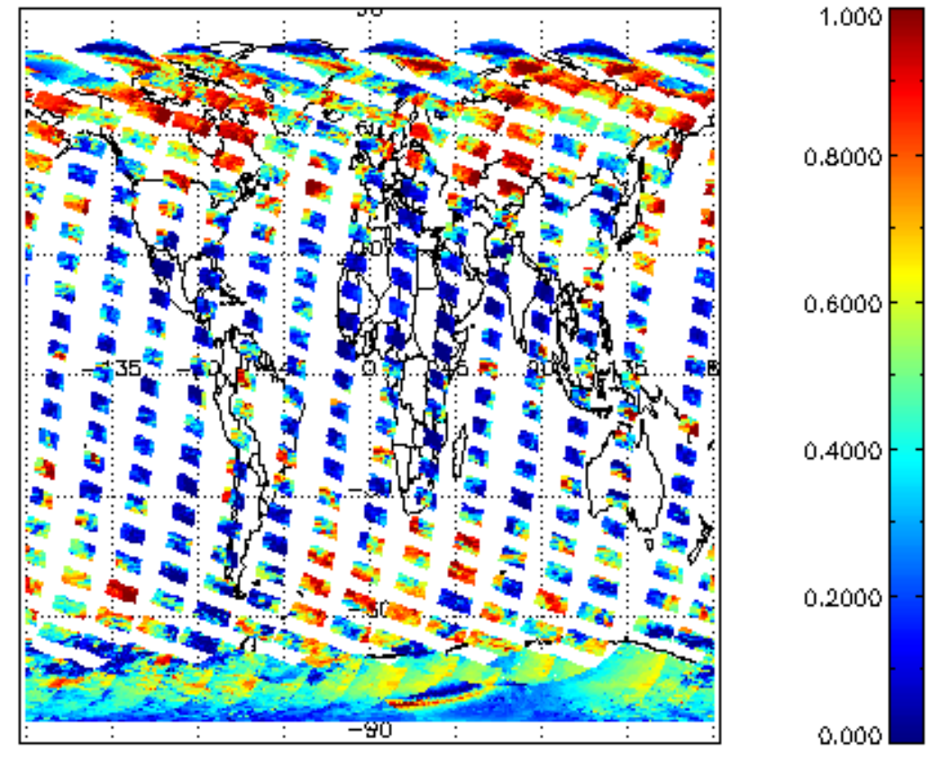
cl_frac for 24FEB2008 00:00:00 to 25FEB2008 00:00:00
