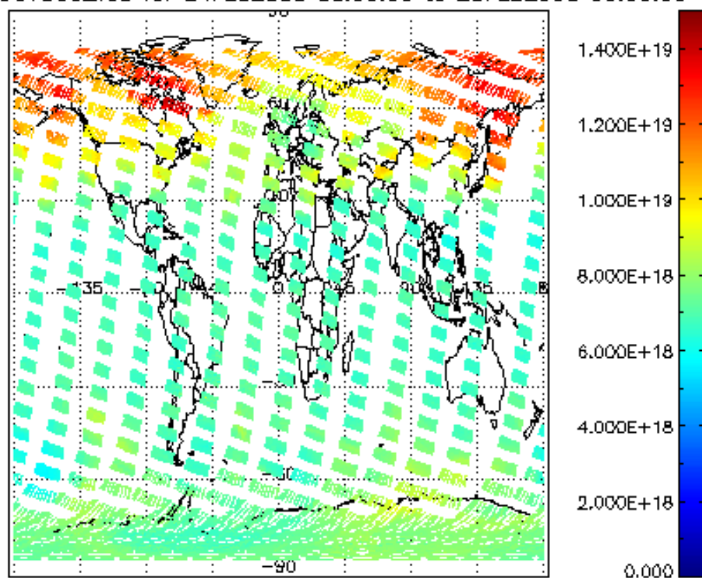
SCIOL2P_NADUV003_vcd for 24FEB2008 00:00:00 to 25FEB2008 00:00:00
