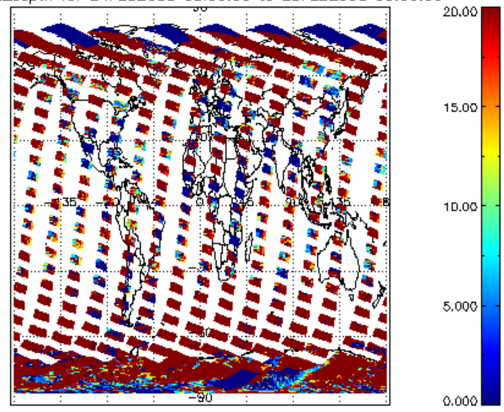
cl_opt_depth for 24FEB2008 00:00:00 to 25FEB2008 00:00:00
