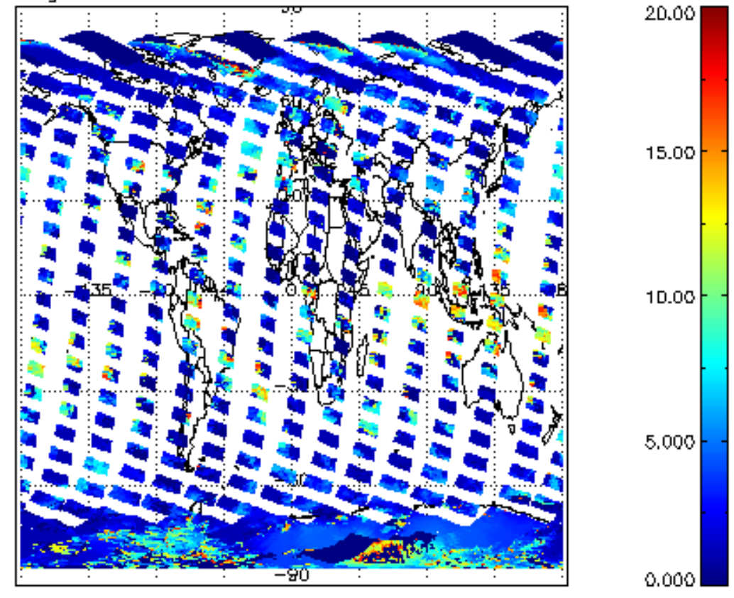
cl_top_height for 24FEB2008 00:00:00 to 25FEB2008 00:00:00
