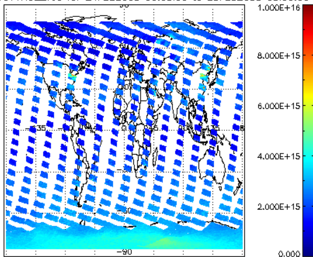
SCIOL2P_NADUV1NO2_vcd for 24FEB2008 00:00:00 to 25FEB2008 00:00:00
