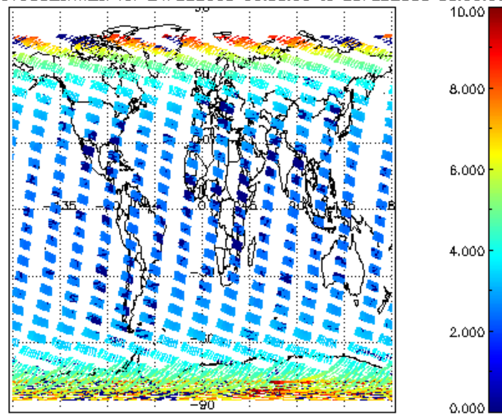
SCIOL2P_NADUV003_amf_cl for 24FEB2008 00:00:00 to 25FEB2008 00:00:00
