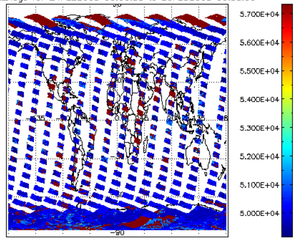
cloud_flags for 24FEB2008 00:00:00 to 25FEB2008 00:00:00
