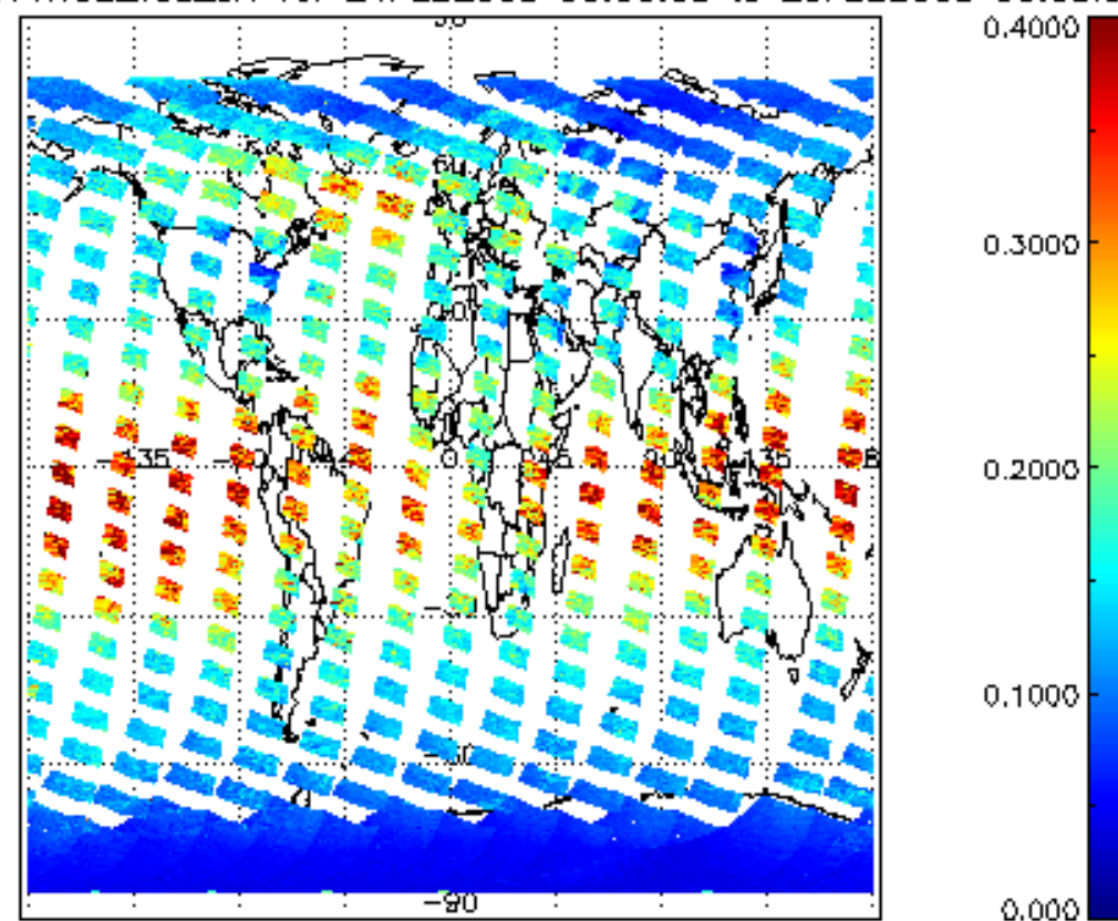
SCIOL2P_NADUV1NO2_vcd_err for 24FEB2008 00:00:00 to 25FEB2008 00:00:00
