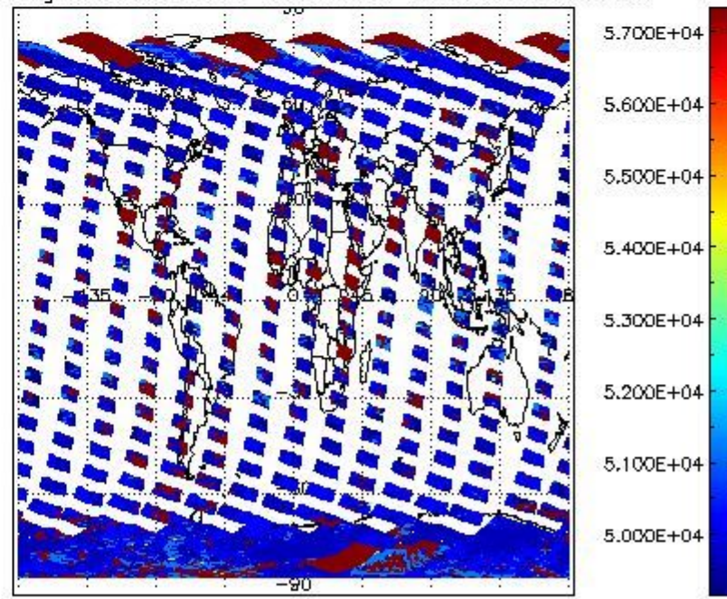
cloud_flags for 24FEB2008 00:00:00 to 25FEB2008 00:00:00
