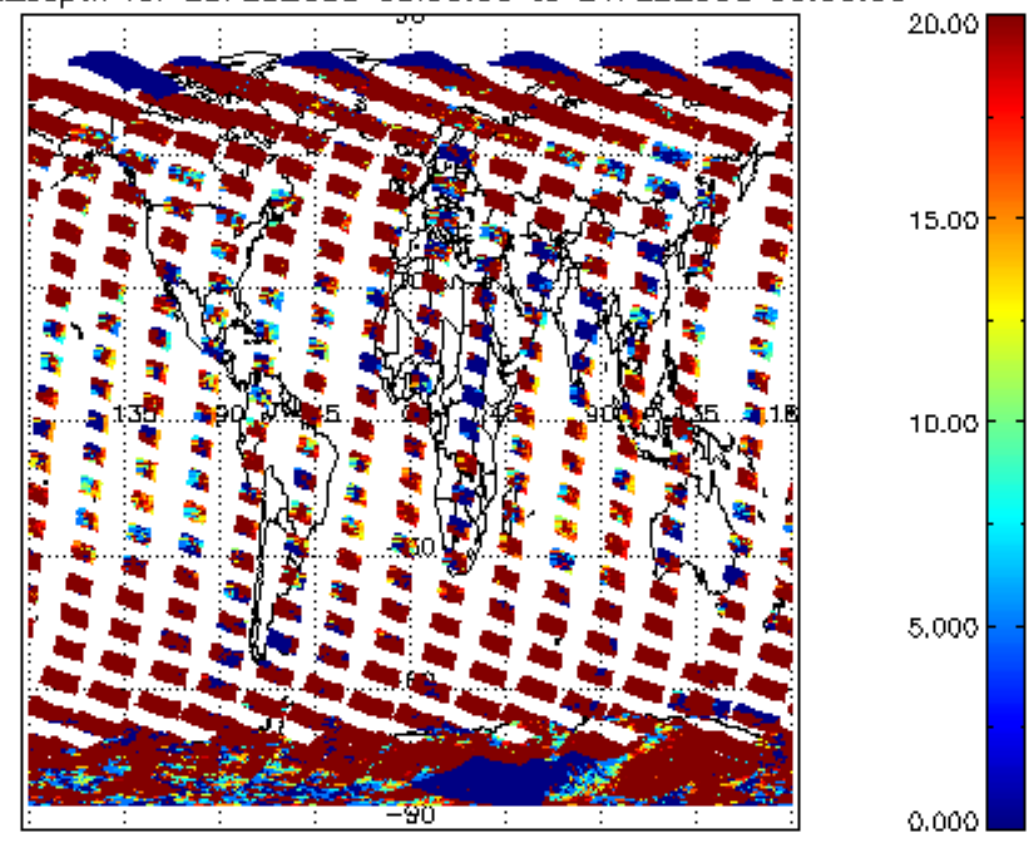
cl_opt_depth for 23FEB2008 00:00:00 to 24FEB2008 00:00:00
