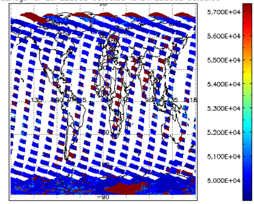
cloud_flags for 23FEB2008 00:00:00 to 24FEB2008 00:00:00
