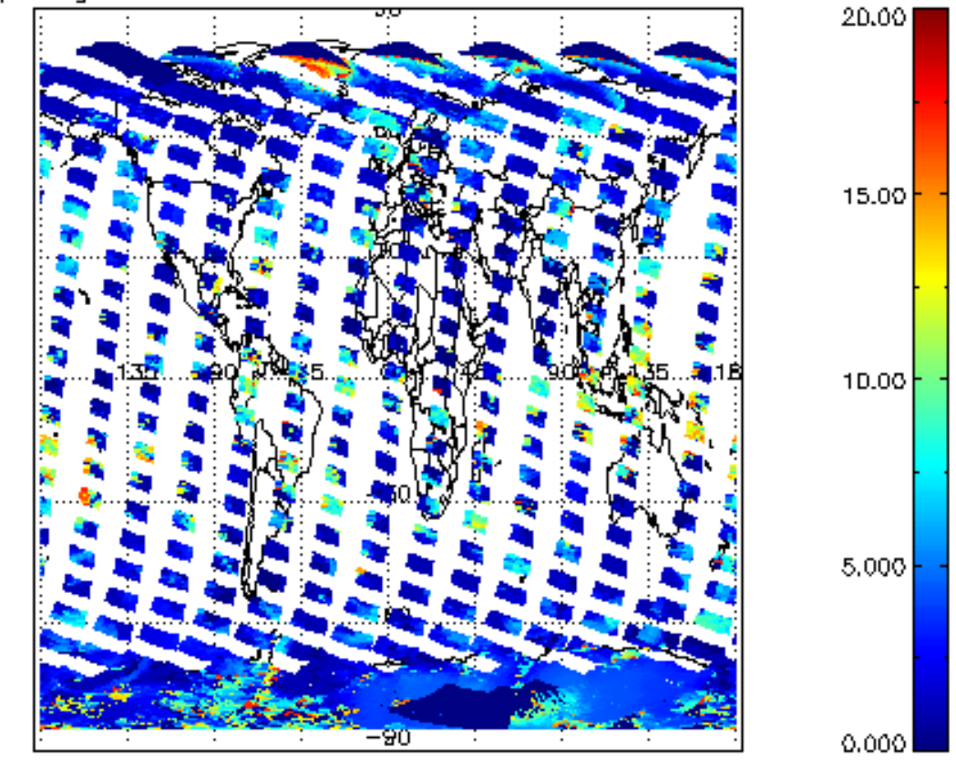
cl_top_height for 23FEB2008 00:00:00 to 24FEB2008 00:00:00
