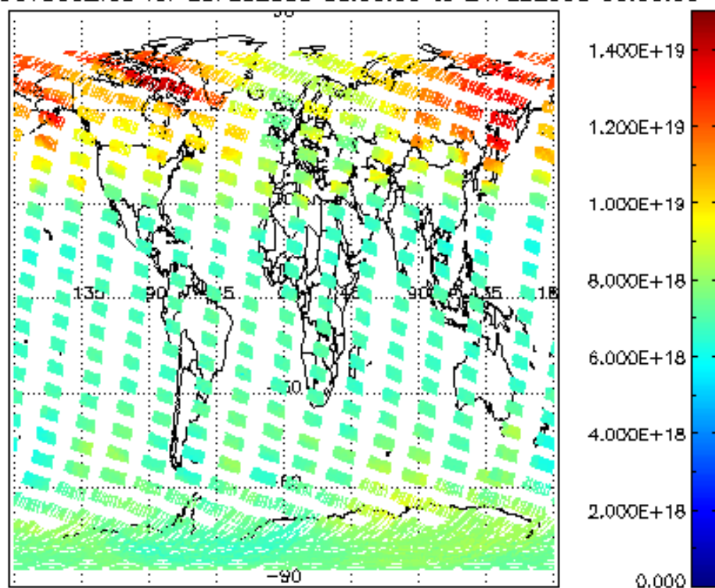
SCIOL2P_NADUV003_vcd for 23FEB2008 00:00:00 to 24FEB2008 00:00:00
