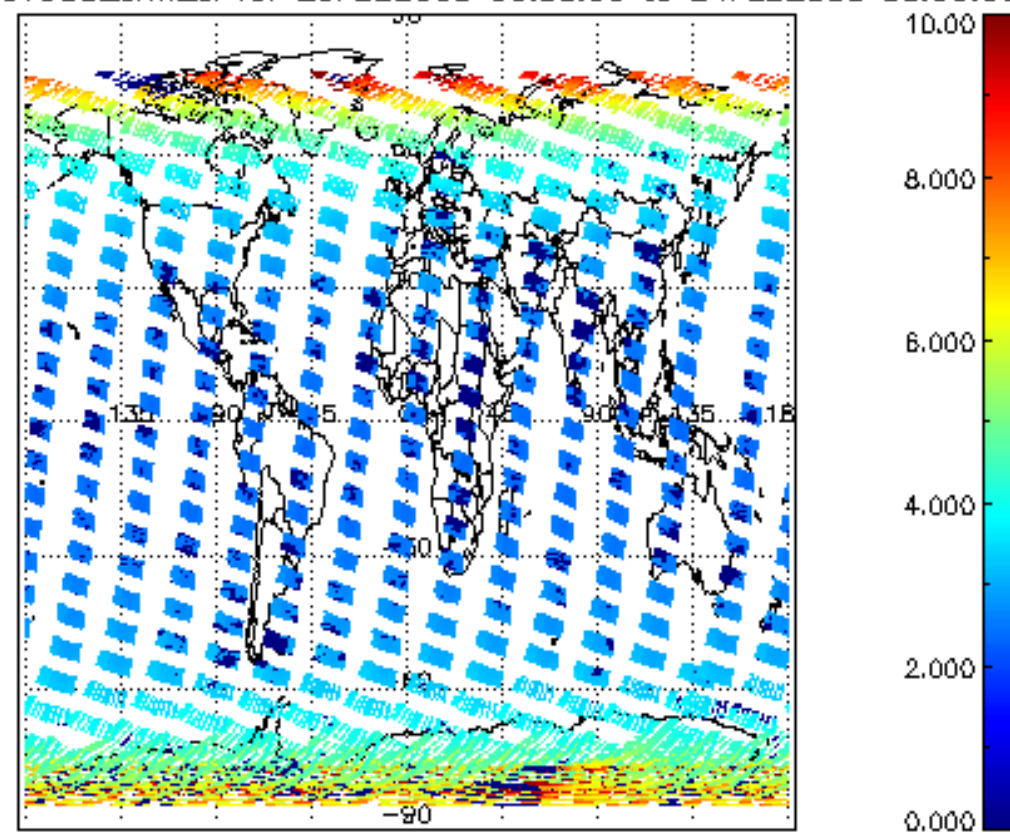
SCIOL2P_NADUV003_amf_cl for 23FEB2008 00:00:00 to 24FEB2008 00:00:00
