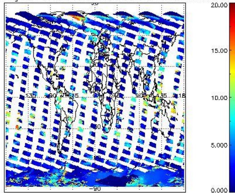
cL_top_height for 23FEB2008 00:00:00 to 24FEB2008 00:00:00
