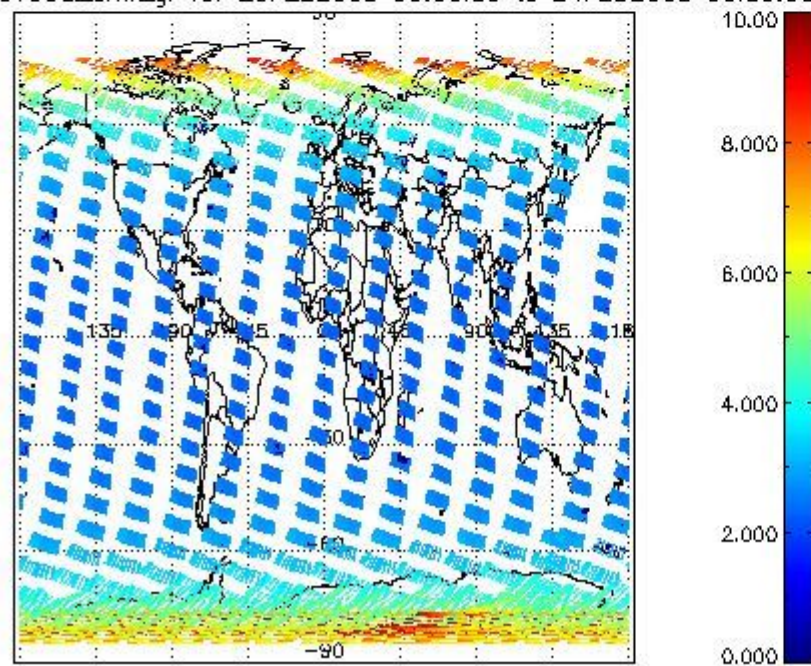
SCIOL2P_NADUV003_amf_gr for 23FEB2008 00:00:00 to 24FEB2008 00:00:00
