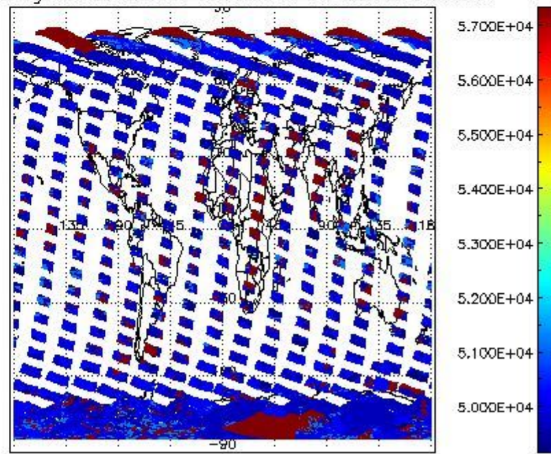
cloud_flags for 23FEB2008 00:00:00 to 24FEB2008 00:00:00
