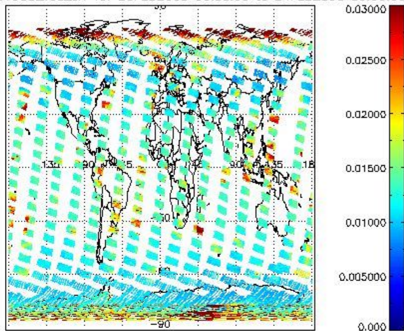
SCIOL2P_NADUV003_vcd_err for 23FEB2008 00:00:00 to 24FEB2008 00:00:00
