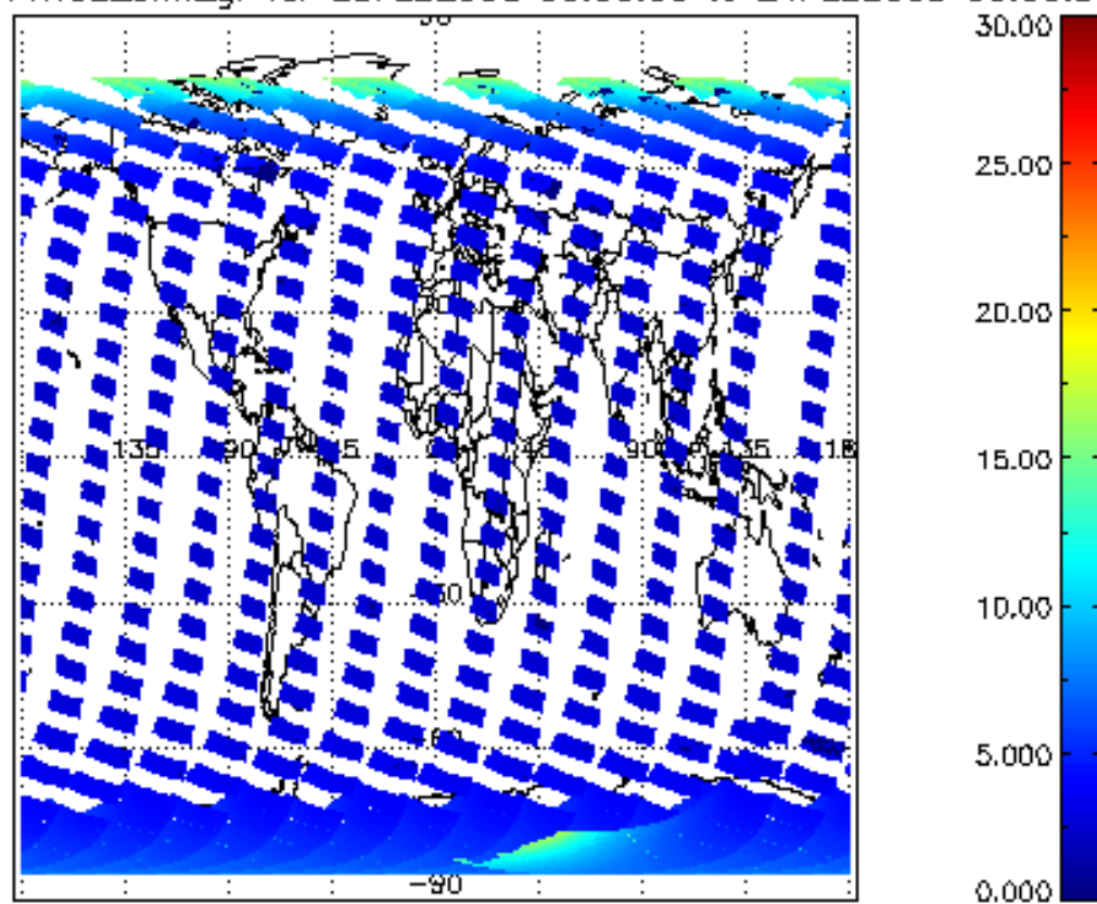
SCIOL2P_NADUV1NO2_amf_gr for 23FEB2008 00:00:00 to 24FEB2008 00:00:00
