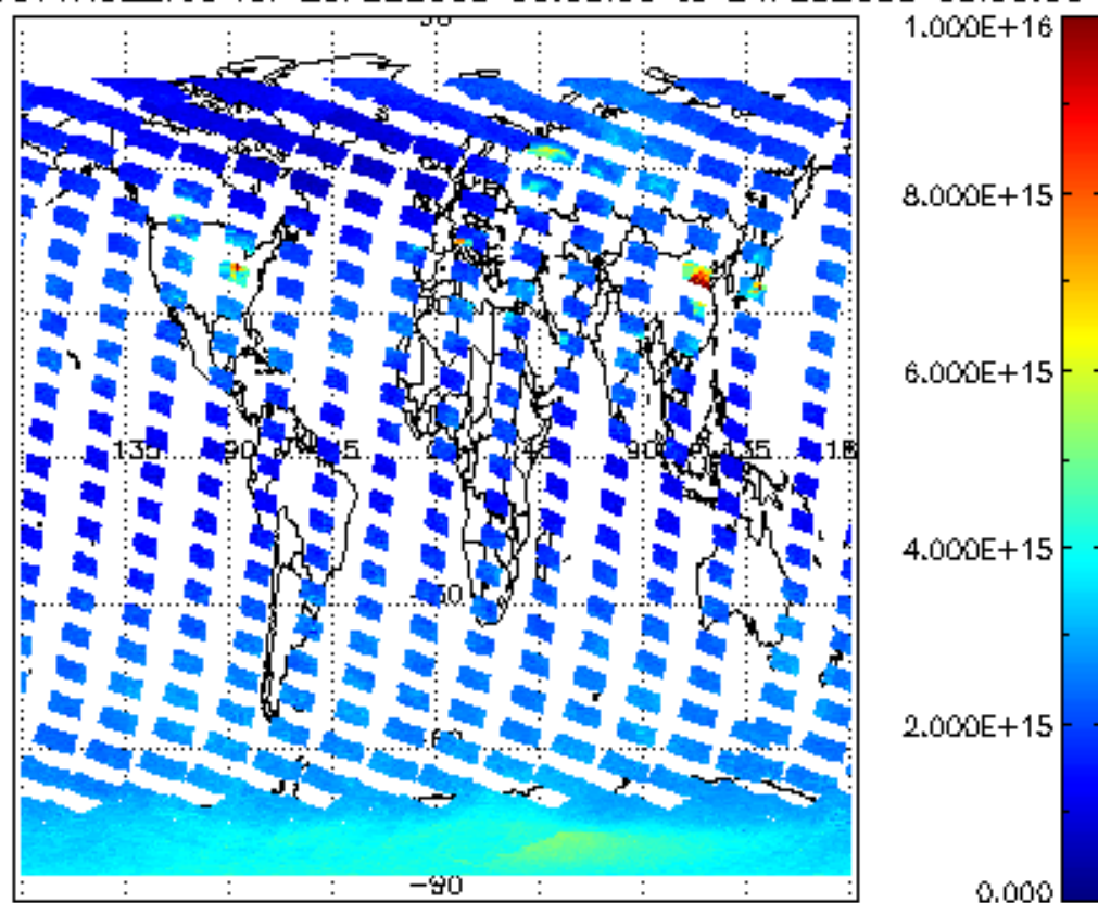
SCIOL2P_NADUV1NO2_vcd for 23FEB2008 00:00:00 to 24FEB2008 00:00:00
