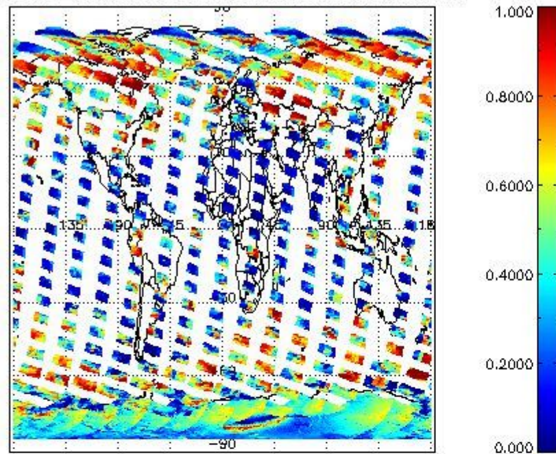
cL_frac for 23FEB2008 00:00:00 to 24FEB2008 00:00:00
