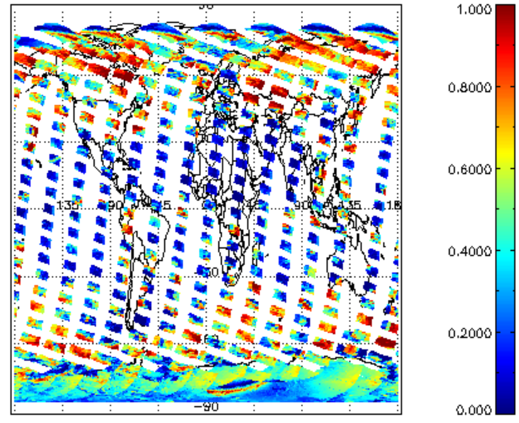
cl_frac for 23FEB2008 00:00:00 to 24FEB2008 00:00:00
