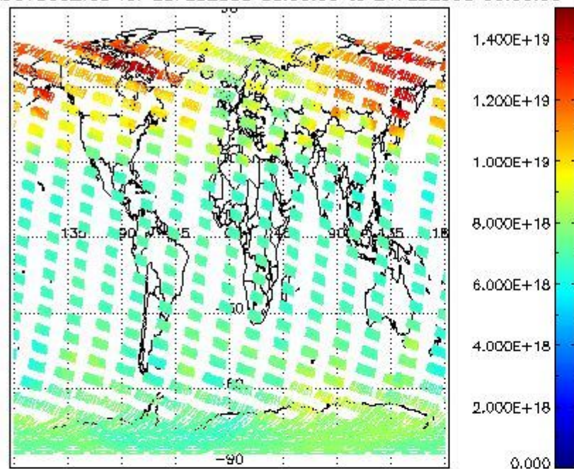
SCIOL2P_NADUV003_vcd for 23FEB2008 00:00:00 to 24FEB2008 00:00:00
