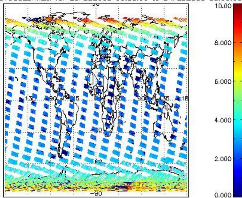
SCIOL2P_NADUV003_amf_cl for 23FEB2008 00:00:00 to 24FEB2008 00:00:00
