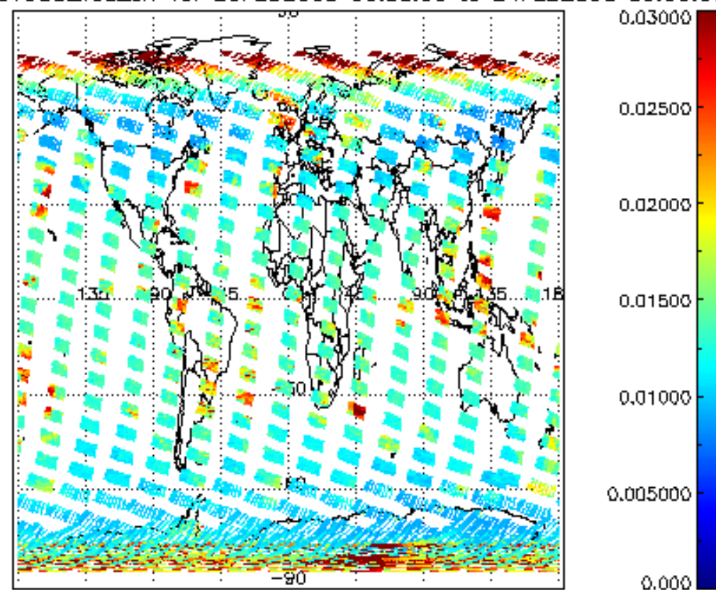
SCIOL2P_NADUV003_vcd_err for 23FEB2008 00:00:00 to 24FEB2008 00:00:00
