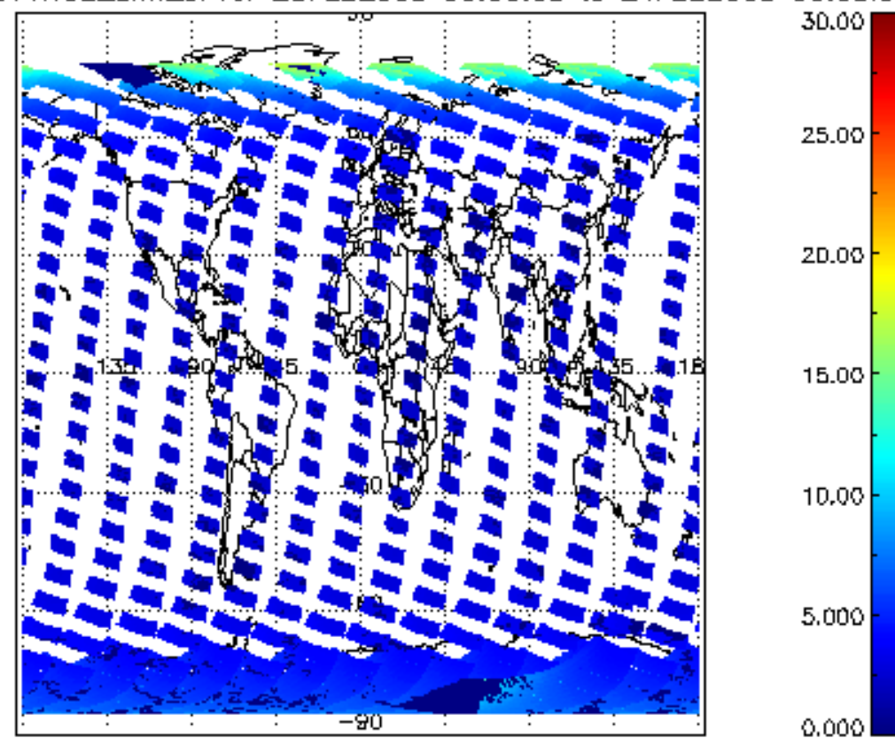
SCIOL2P_NADUV1NO2_amf_cl for 23FEB2008 00:00:00 to 24FEB2008 00:00:00
