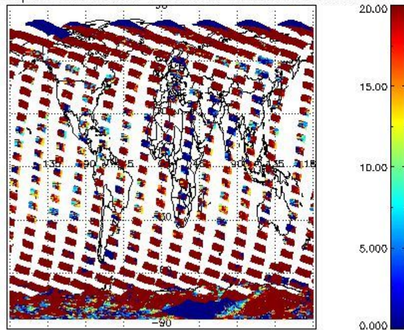
cL_opt_depth for 23FEB2008 00:00:00 to 24FEB2008 00:00:00
