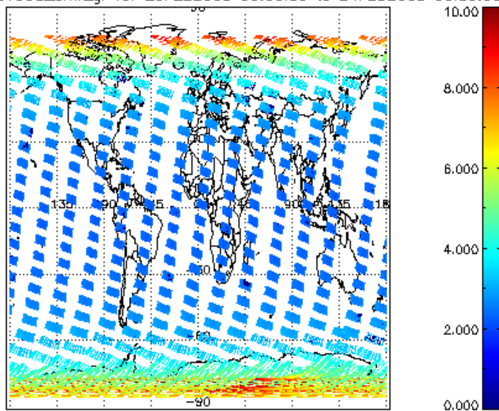
SCIOL2P_NADUV003_amf_gr for 23FEB2008 00:00:00 to 24FEB2008 00:00:00
