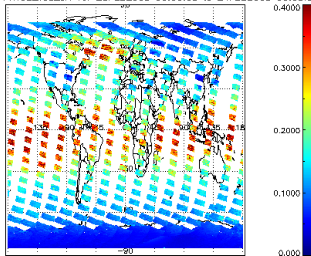
SCIOL2P_NADUV1NO2_vcd_err for 23FEB2008 00:00:00 to 24FEB2008 00:00:00
