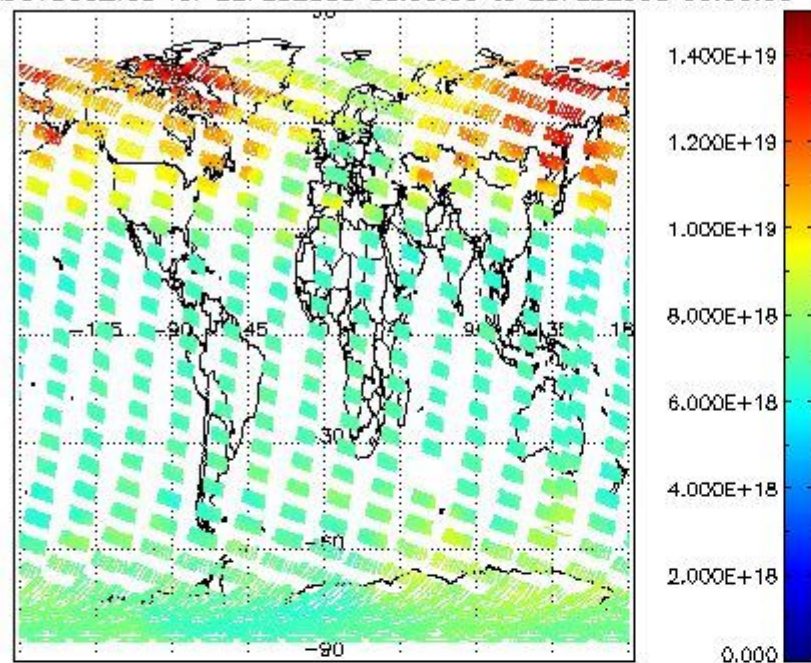
SCIOL2P_NADUV003_vcd for 22FEB2008 00:00:00 to 23FEB2008 00:00:00
