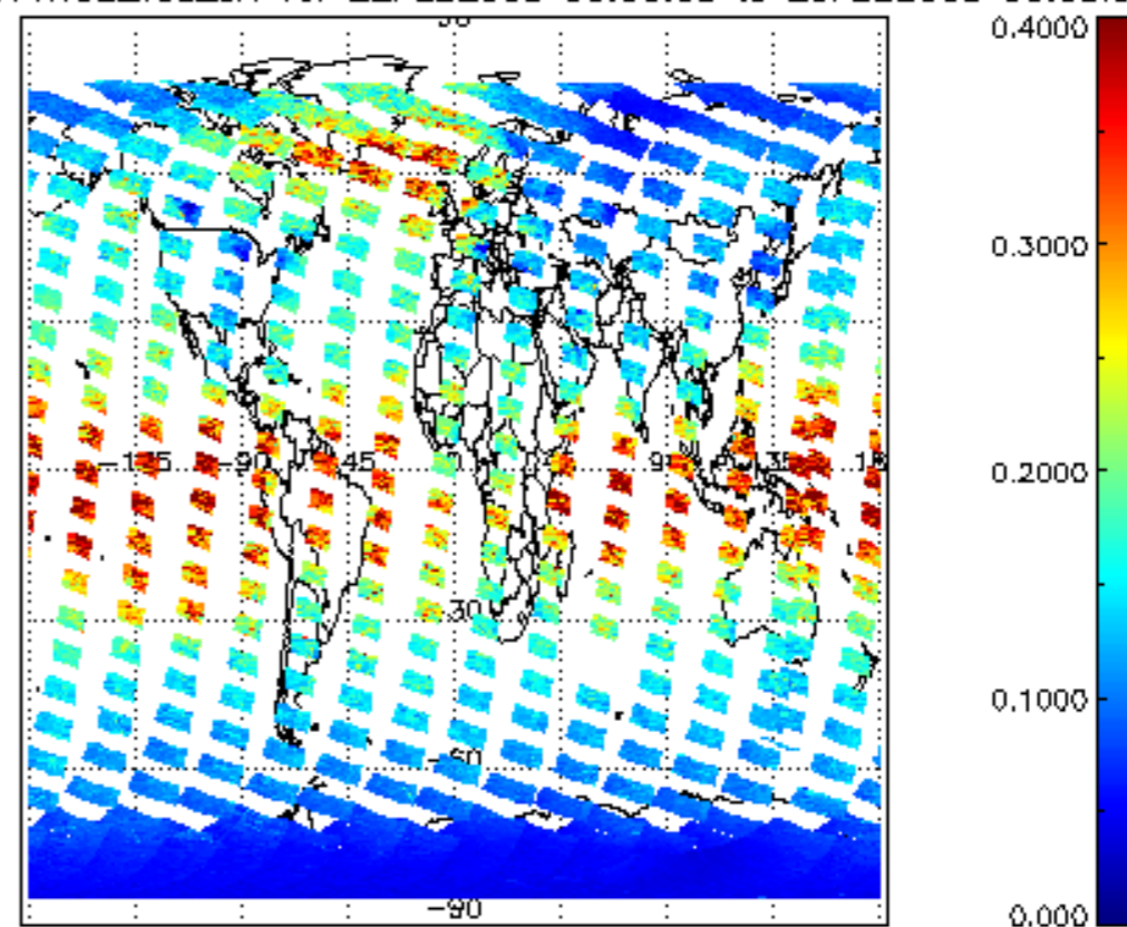
SCIOL2P_NADUV1NO2_vcd_err for 22FEB2008 00:00:00 to 23FEB2008 00:00:00
