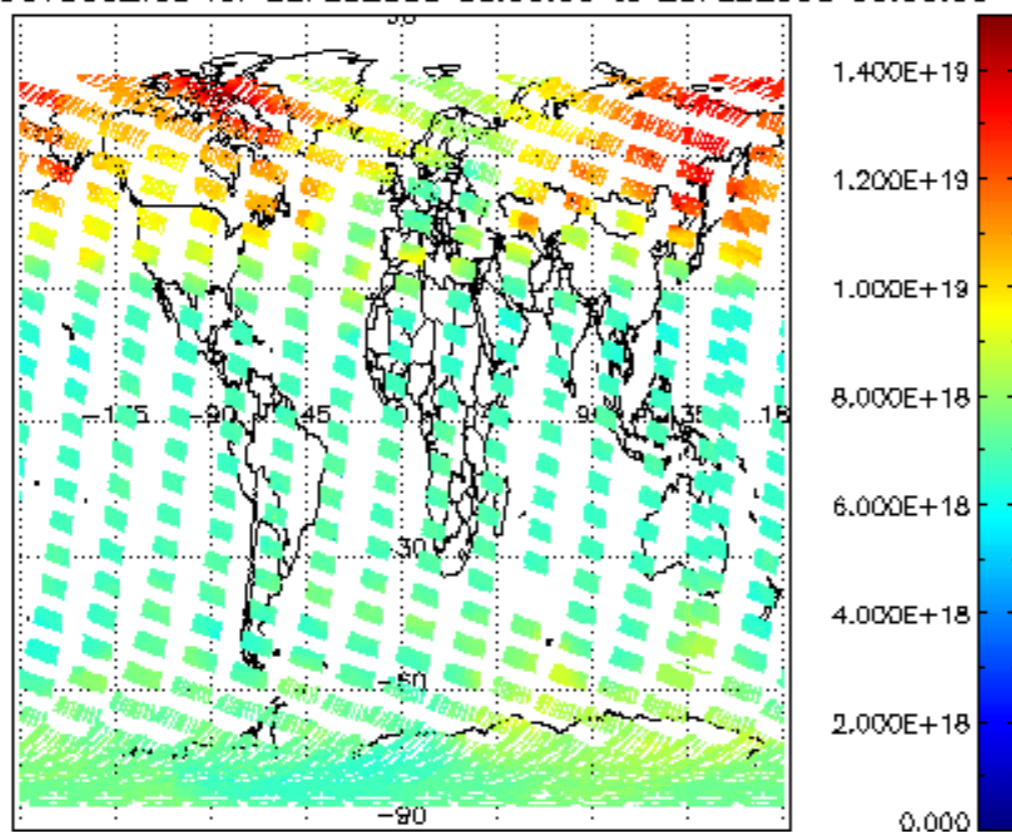
SCIOL2P_NADUV003_vcd for 22FEB2008 00:00:00 to 23FEB2008 00:00:00
