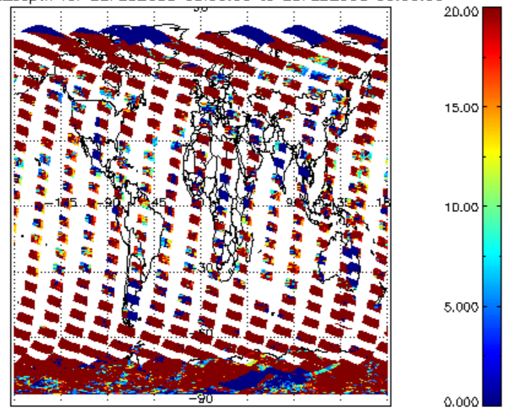
cl_opt_depth for 22FEB2008 00:00:00 to 23FEB2008 00:00:00
