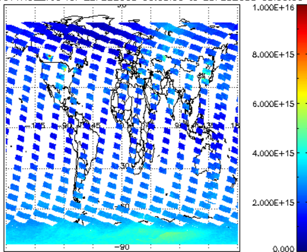
SCIOL2P_NADUV1NO2_vcd for 22FEB2008 00:00:00 to 23FEB2008 00:00:00
