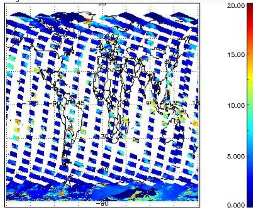
cL_top_height for 22FEB2008 00:00:00 to 23FEB2008 00:00:00
