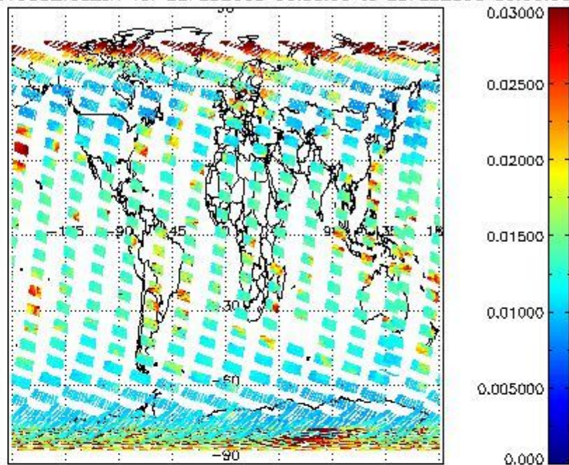
SCIOL2P_NADUV003_vcd_err for 22FEB2008 00:00:00 to 23FEB2008 00:00:00
