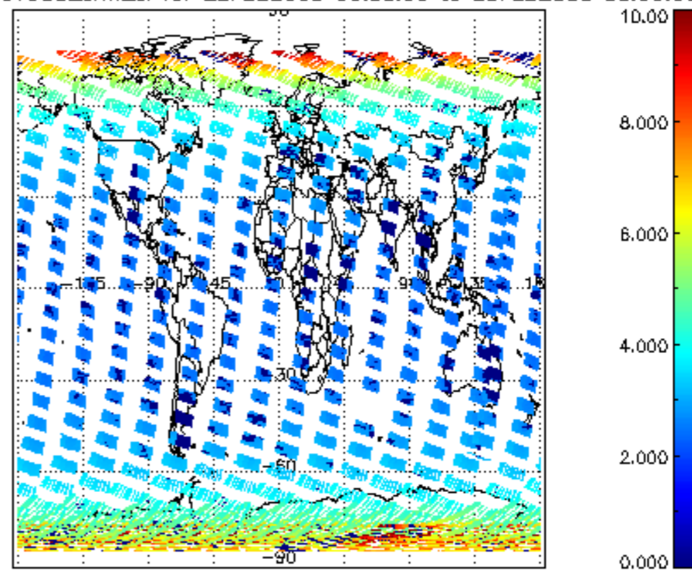
SCIOL2P_NADUV003_amf_cl for 22FEB2008 00:00:00 to 23FEB2008 00:00:00
