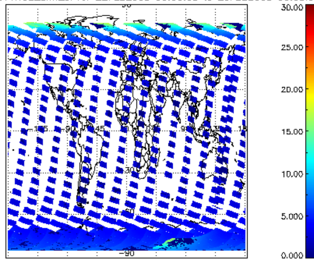
SCIOL2P_NADUV1NO2_amf_cl for 22FEB2008 00:00:00 to 23FEB2008 00:00:00
