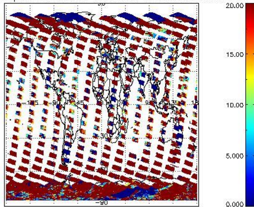
cL_opt_depth for 22FEB2008 00:00:00 to 23FEB2008 00:00:00
