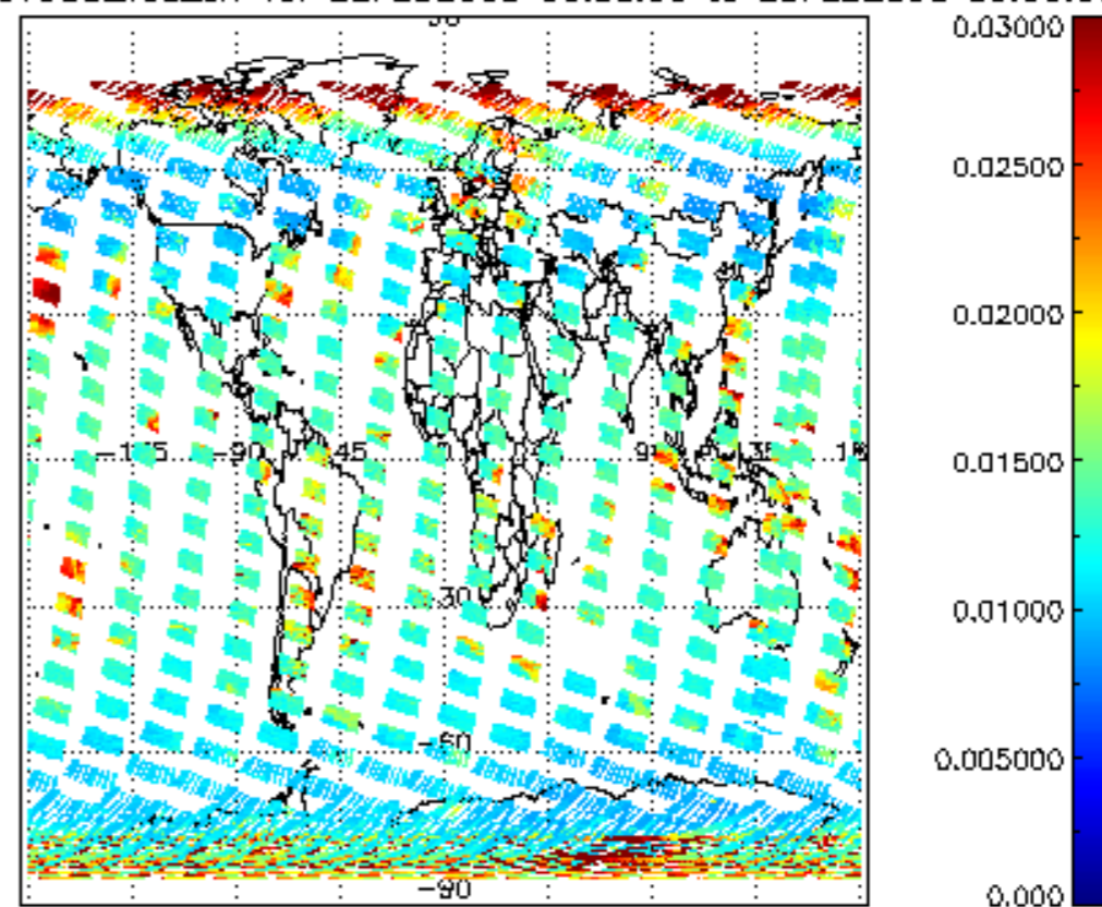
SCIOL2P_NADUV003_vcd_err for 22FEB2008 00:00:00 to 23FEB2008 00:00:00
