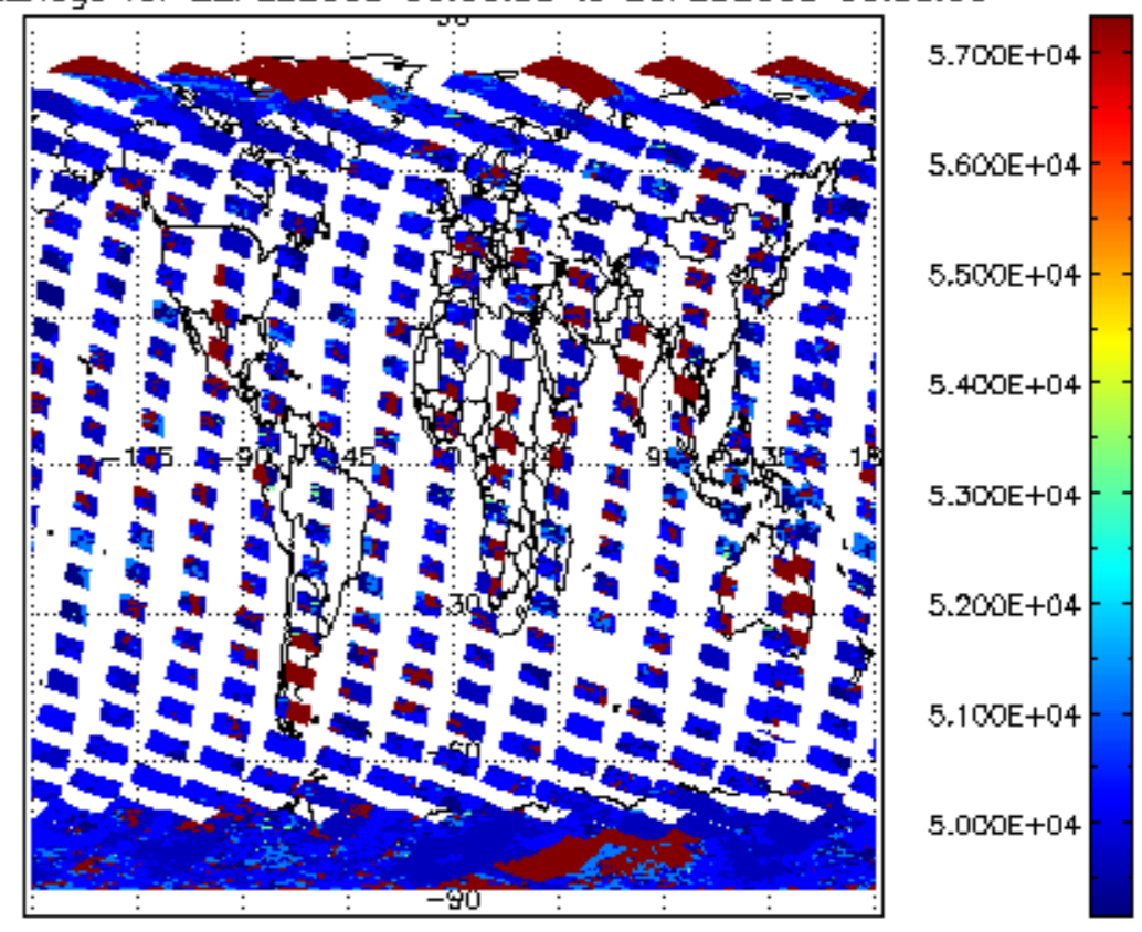
cloud_flags for 22FEB2008 00:00:00 to 23FEB2008 00:00:00
