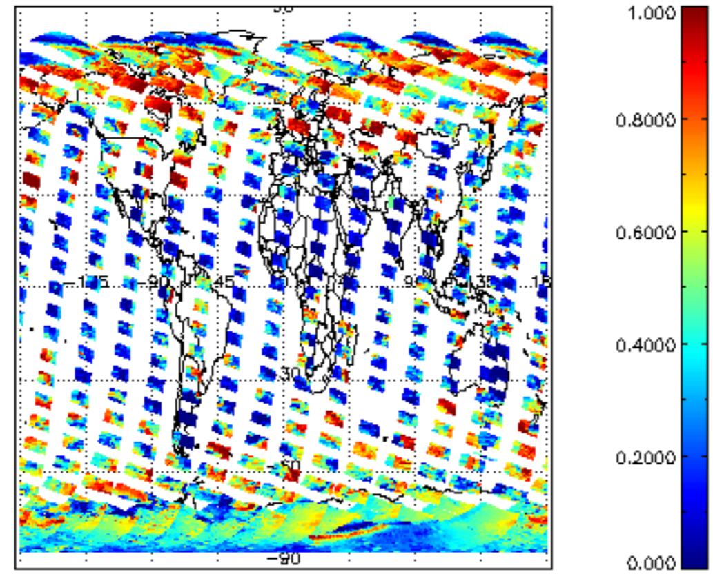
cl_frac for 22FEB2008 00:00:00 to 23FEB2008 00:00:00
