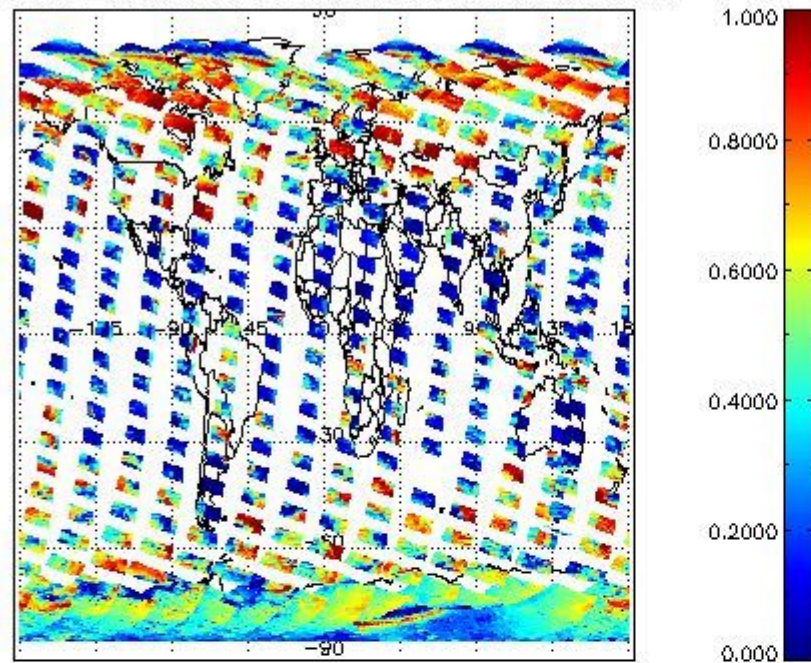
cL_frac for 22FEB2008 00:00:00 to 23FEB2008 00:00:00
