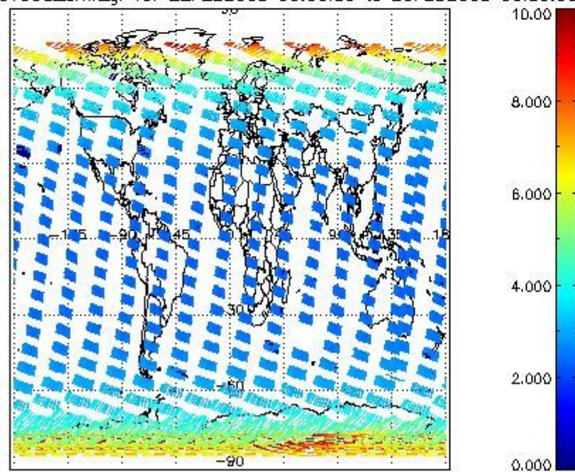
SCIOL2P_NADUV003_amf_gr for 22FEB2008 00:00:00 to 23FEB2008 00:00:00
