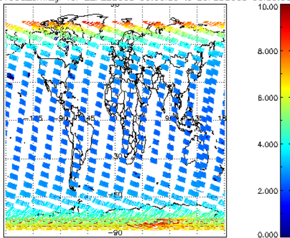
SCIOL2P_NADUV003_amf_gr for 22FEB2008 00:00:00 to 23FEB2008 00:00:00
