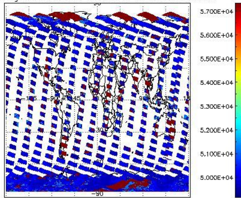
cloud_flags for 22FEB2008 00:00:00 to 23FEB2008 00:00:00
