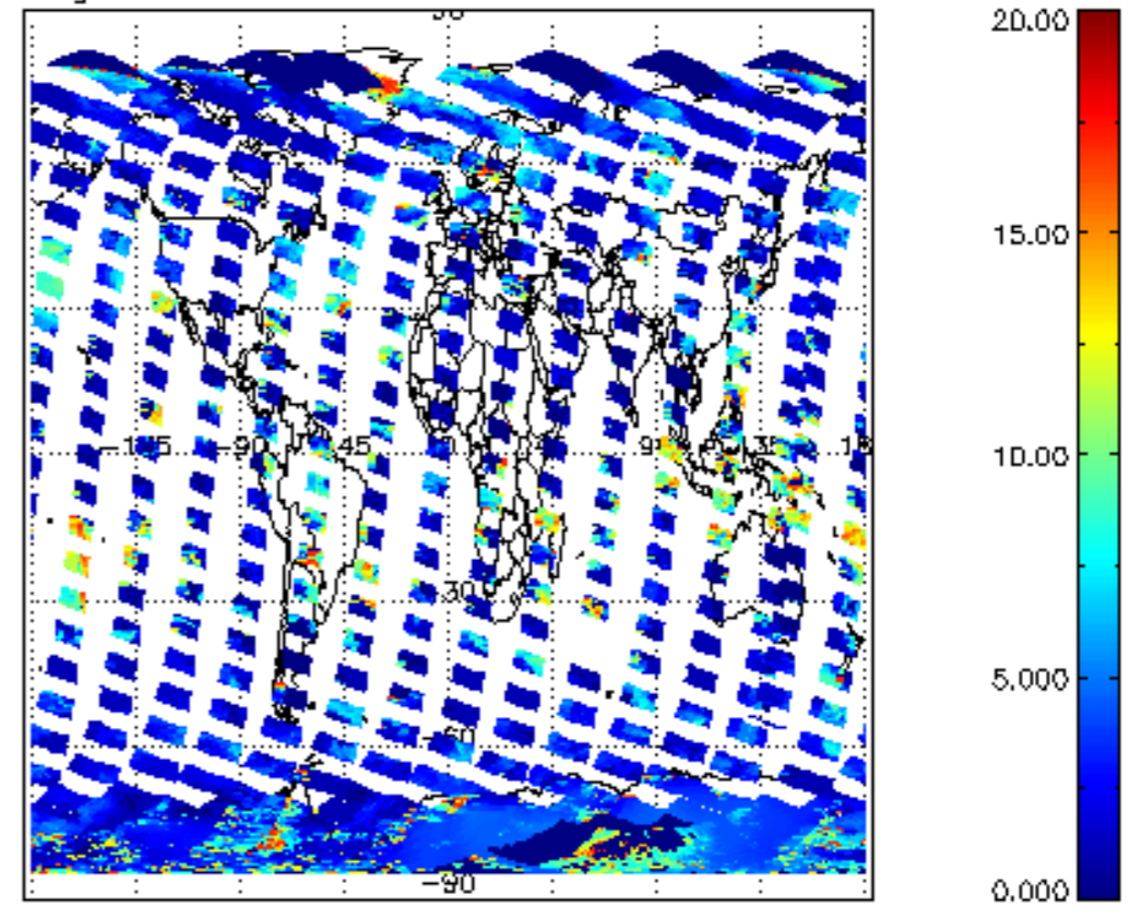
cl_top_height for 22FEB2008 00:00:00 to 23FEB2008 00:00:00
