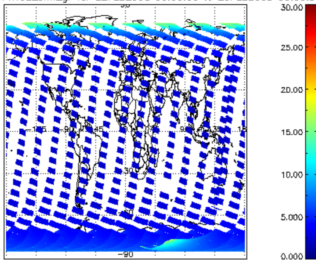
SCIOL2P_NADUV1NO2_amf_gr for 22FEB2008 00:00:00 to 23FEB2008 00:00:00
