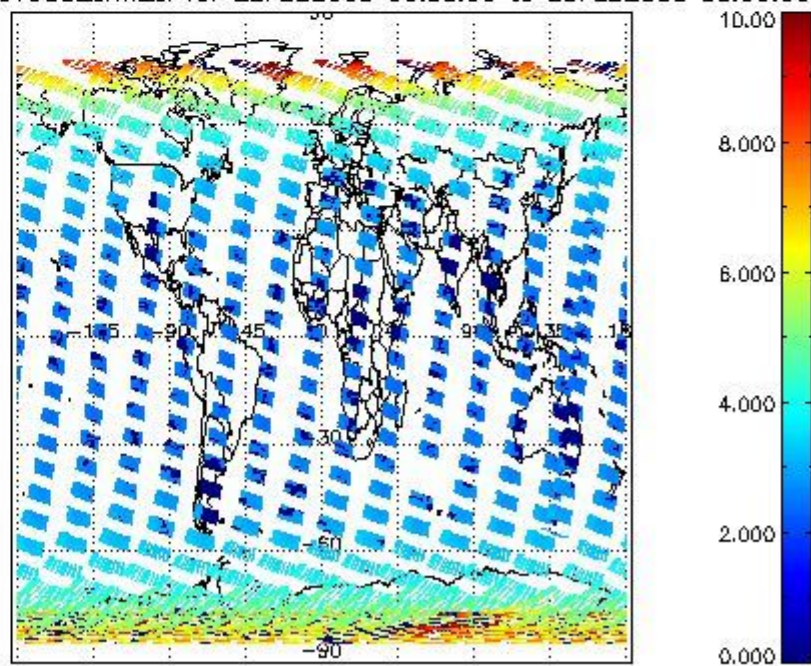
SCIOL2P_NADUV003_amf_cl for 22FEB2008 00:00:00 to 23FEB2008 00:00:00
