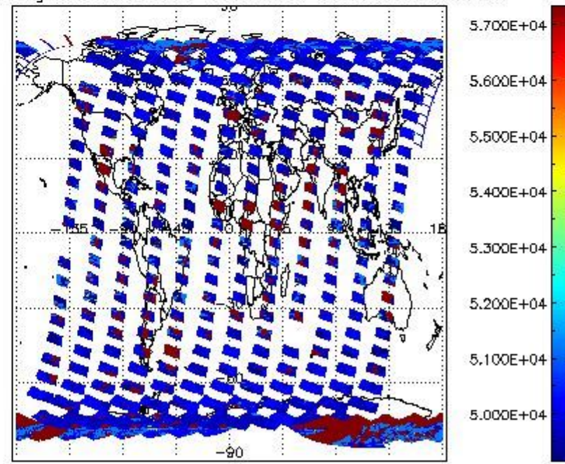
cloud_flags for 18FEB2008 00:00:00 to 19FEB2008 00:00:00
