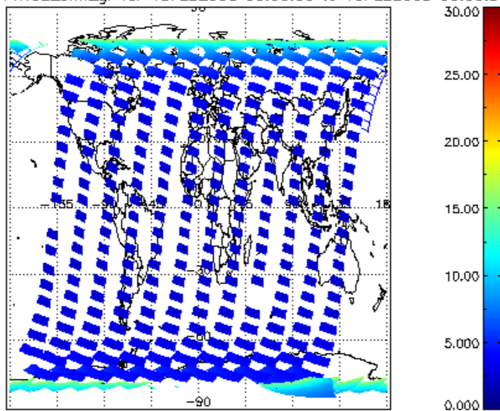
SCIOL2P_NADUV1NO2_amf_gr for 18FEB2008 00:00:00 to 19FEB2008 00:00:00
