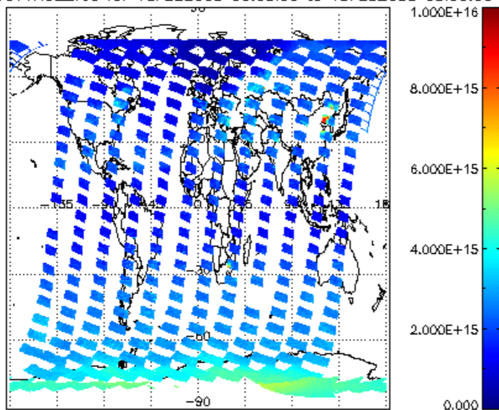
SCIOL2P_NADUV1NO2_vcd for 18FEB2008 00:00:00 to 19FEB2008 00:00:00
