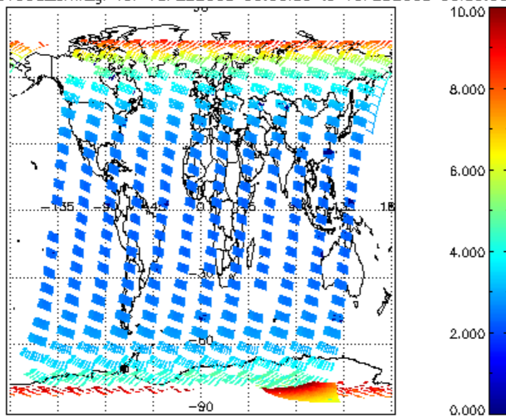
SCIOL2P_NADUV003_amf_gr for 18FEB2008 00:00:00 to 19FEB2008 00:00:00
