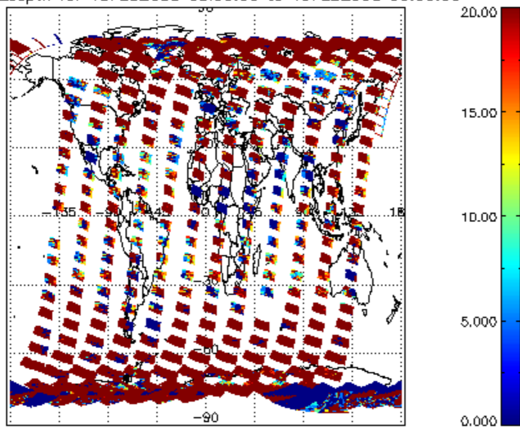
cl_opt_depth for 18FEB2008 00:00:00 to 19FEB2008 00:00:00
