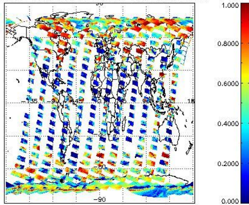
cLfrac for 18FEB2008 00:00:00 to 19FEB2008 00:00:00
