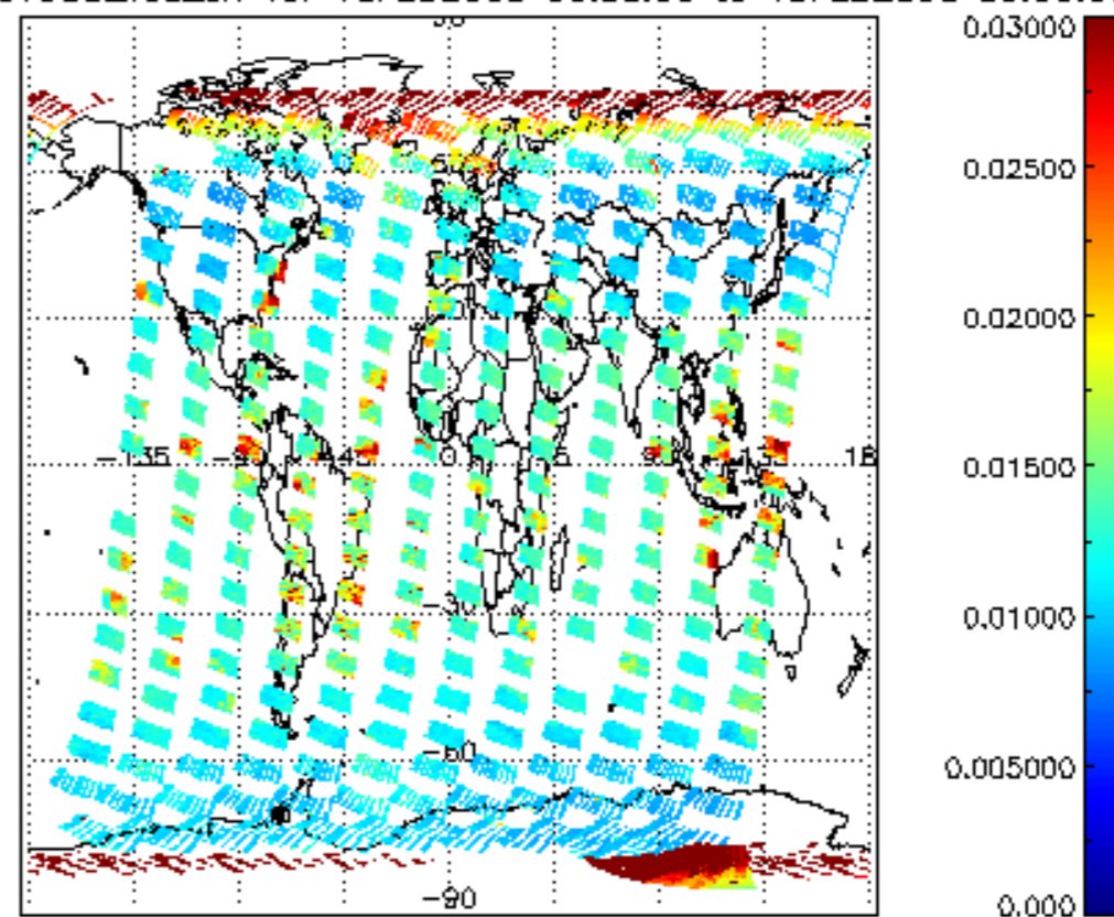
SCIOL2P_NADUV003_vcd_err for 18FEB2008 00:00:00 to 19FEB2008 00:00:00
