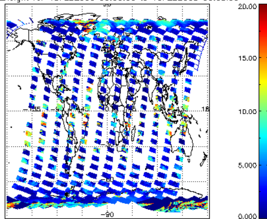
cl_top_height for 18FEB2008 00:00:00 to 19FEB2008 00:00:00
