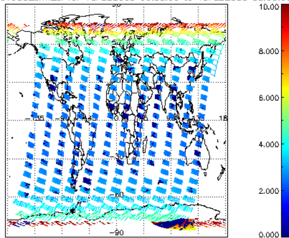
SCIOL2P_NADUV003_amf_cl for 18FEB2008 00:00:00 to 19FEB2008 00:00:00
