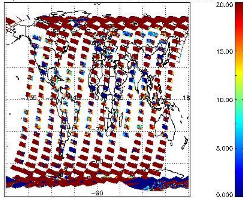
cLopt_depth for 18FEB2008 00:00:00 to 19FEB2008 00:00:00
