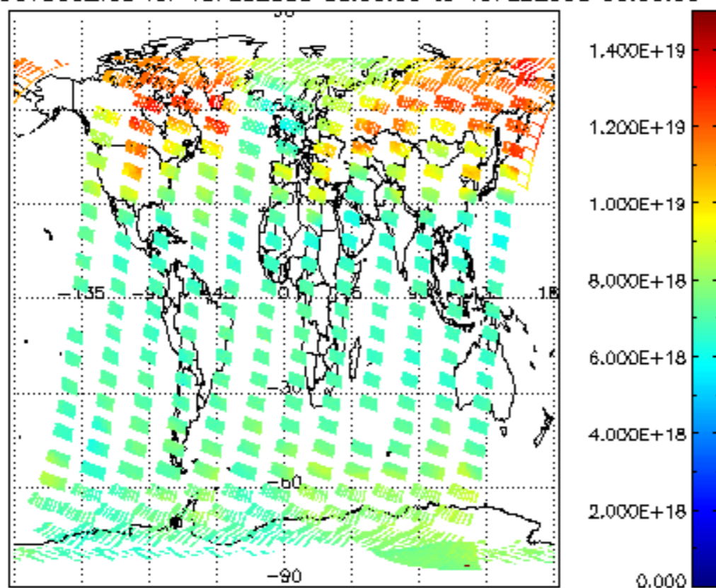
SCIOL2P_NADUV003_vcd for 18FEB2008 00:00:00 to 19FEB2008 00:00:00
