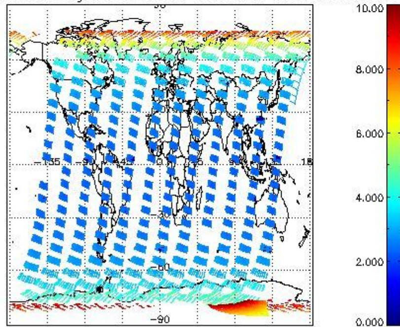
SCIOL2P_NADUV003_amf_gr for 18FEB2008 00:00:00 to 19FEB2008 00:00:00
