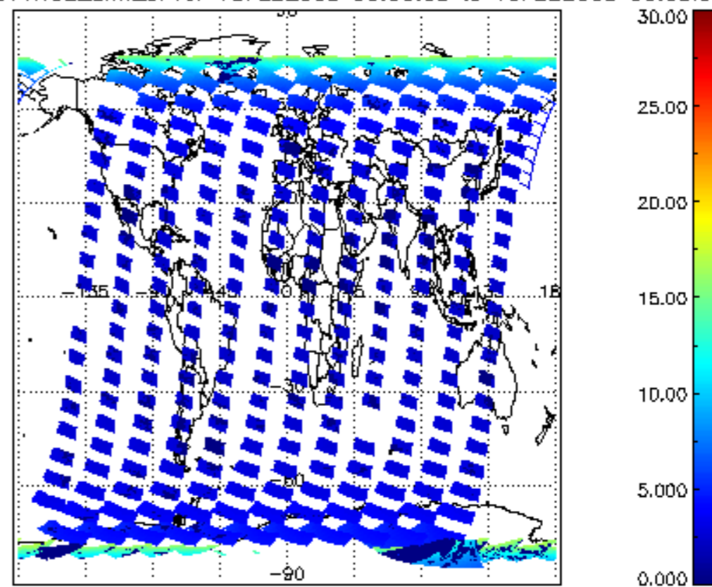
SCIOL2P_NADUV1NO2_amf_cl for 18FEB2008 00:00:00 to 19FEB2008 00:00:00
