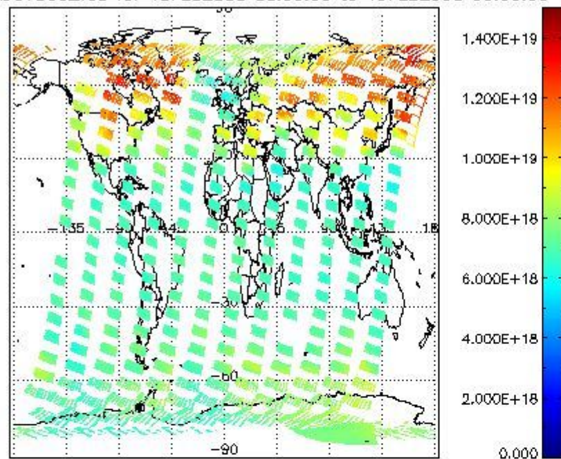
SCIOL2P_NADUV003_vcd for 18FEB2008 00:00:00 to 19FEB2008 00:00:00
