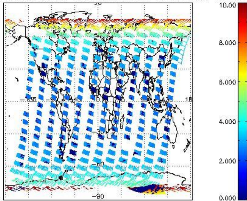
SCIOL2P_NADUV003_amf_cl for 18FEB2008 00:00:00 to 19FEB2008 00:00:00
