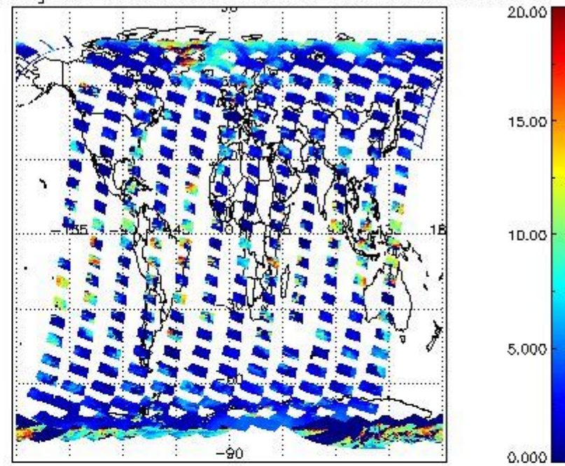
cL_top_height for 18FEB2008 00:00:00 to 19FEB2008 00:00:00
