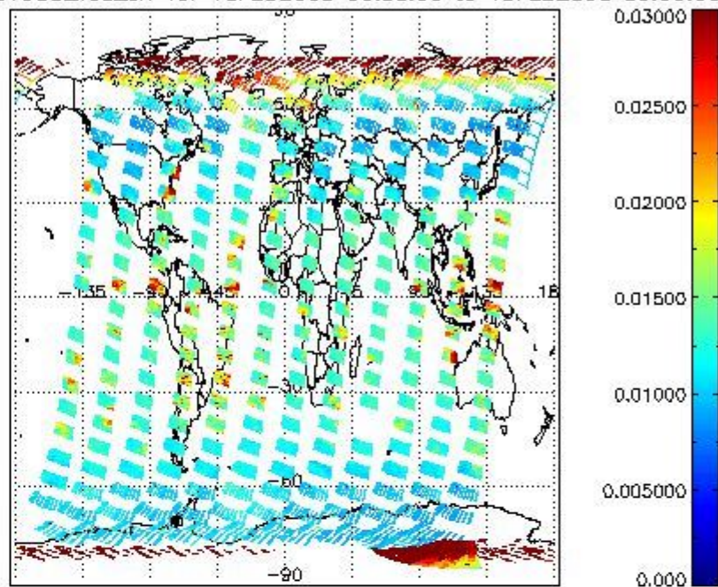
SCIOL2P_NADUV003_vcd_err for 18FEB2008 00:00:00 to 19FEB2008 00:00:00
