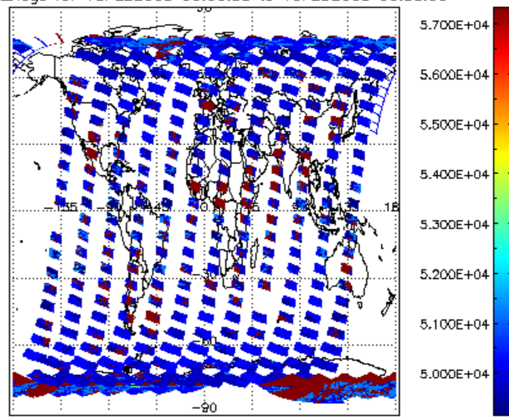
cloud_flags for 18FEB2008 00:00:00 to 19FEB2008 00:00:00
