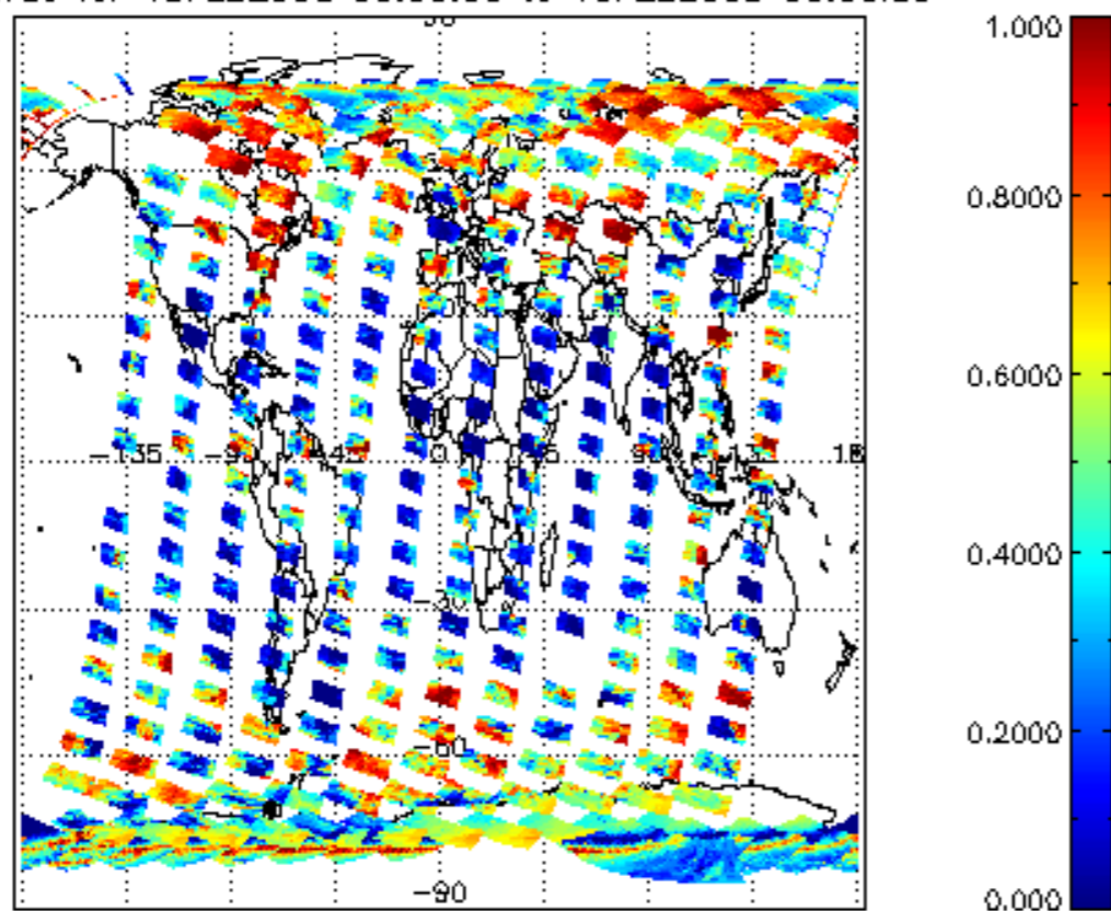
cl_frac for 18FEB2008 00:00:00 to 19FEB2008 00:00:00
