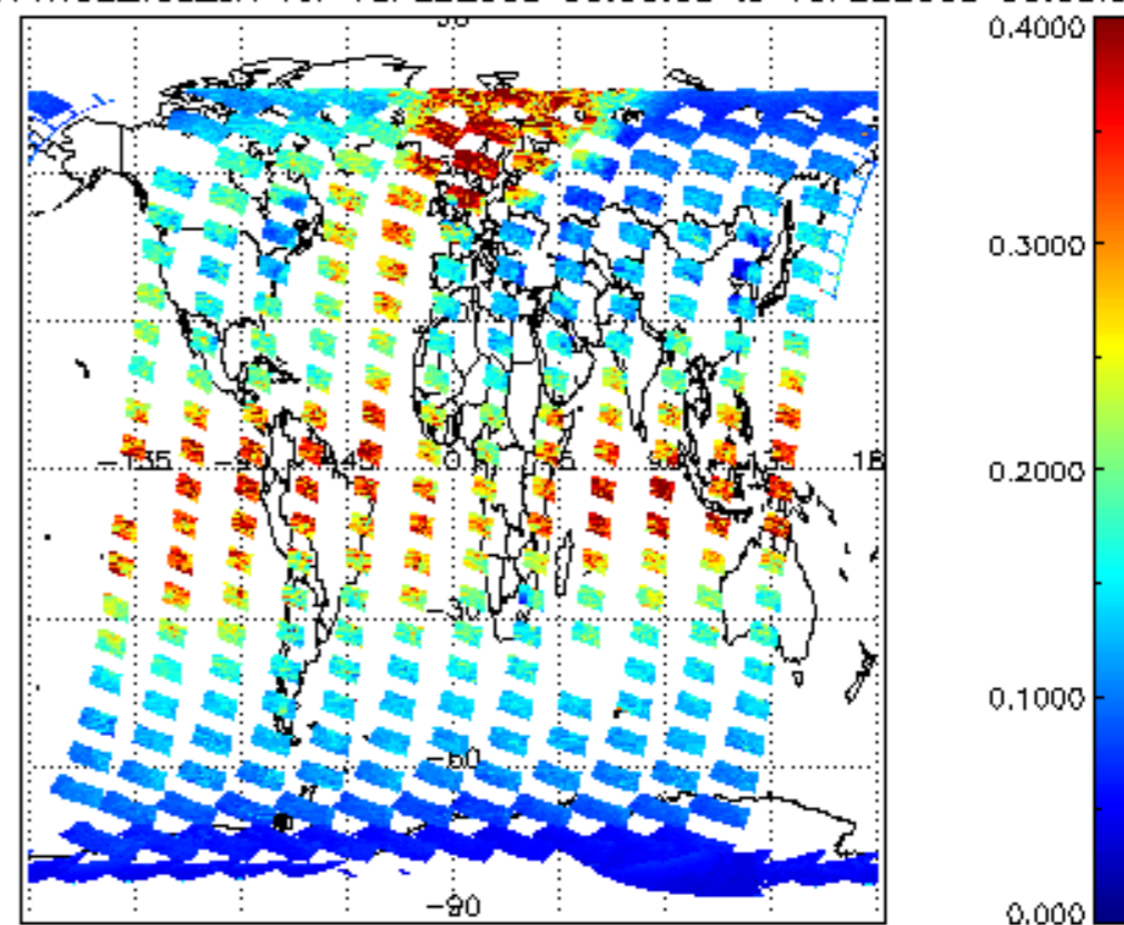
SCIOL2P_NADUV1NO2_vcd_err for 18FEB2008 00:00:00 to 19FEB2008 00:00:00
