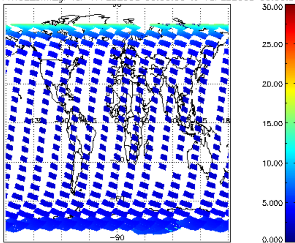
SCIOL2P_NADUV1NO2_amf_gr for 17FEB2008 00:00:00 to 18FEB2008 00:00:00
