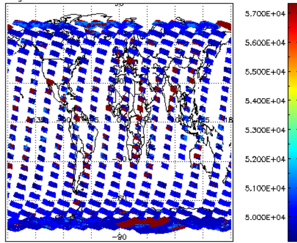
cloud_flags for 17FEB2008 00:00:00 to 18FEB2008 00:00:00
