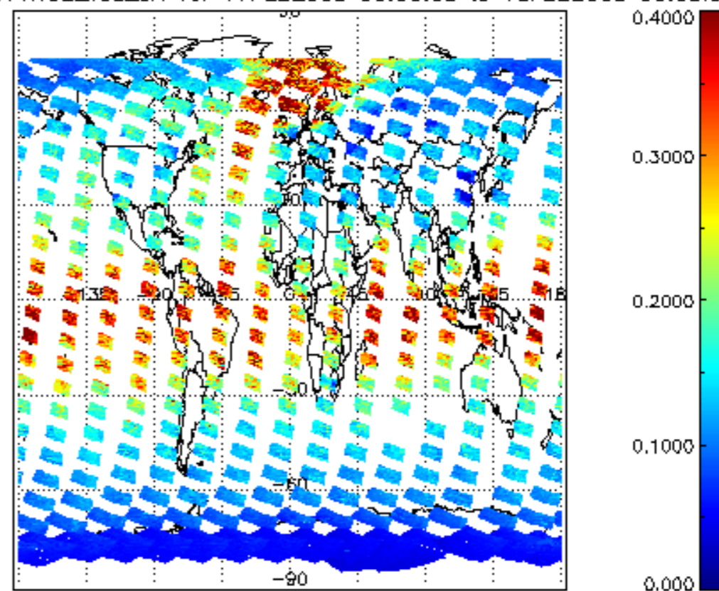
SCIOL2P_NADUV1NO2_vcd_err for 17FEB2008 00:00:00 to 18FEB2008 00:00:00
