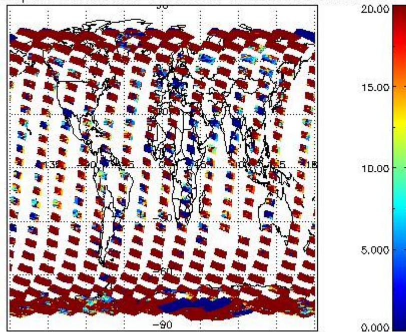
cLopt_depth for 17FEB2008 00:00:00 to 18FEB2008 00:00:00
