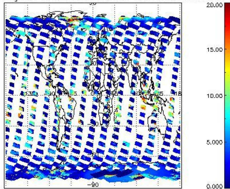
cL_top_height for 17FEB2008 00:00:00 to 18FEB2008 00:00:00
