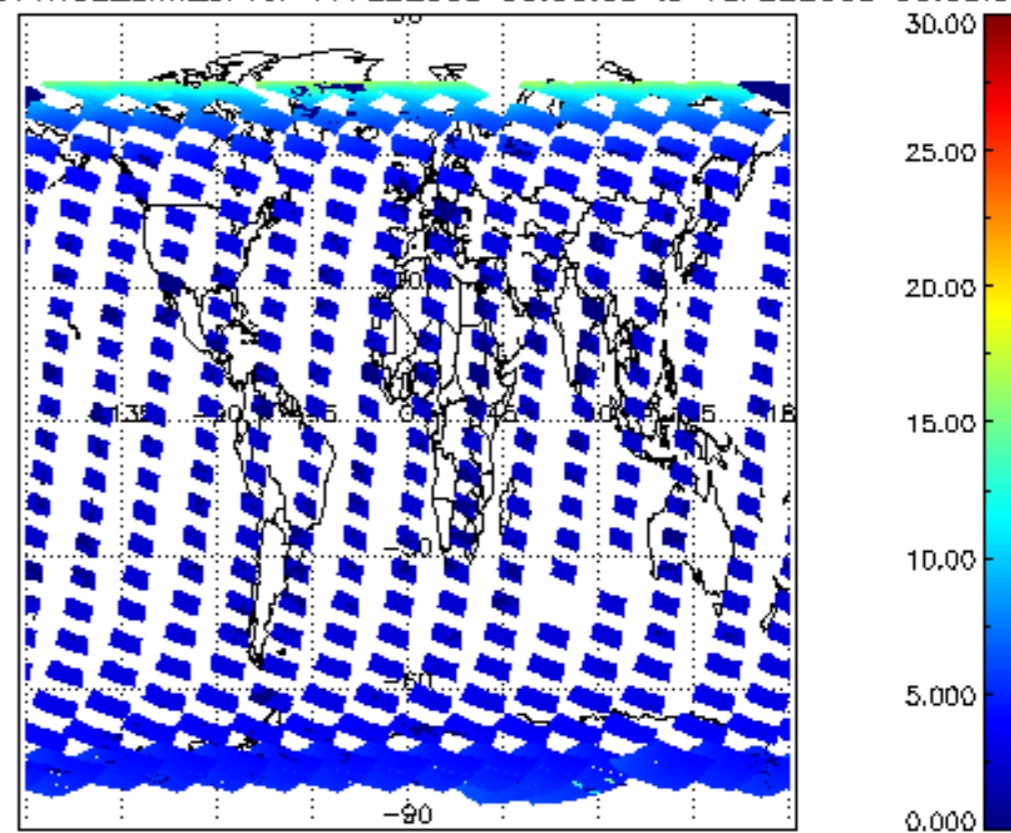
SCIOL2P_NADUV1NO2_amf_cl for 17FEB2008 00:00:00 to 18FEB2008 00:00:00
