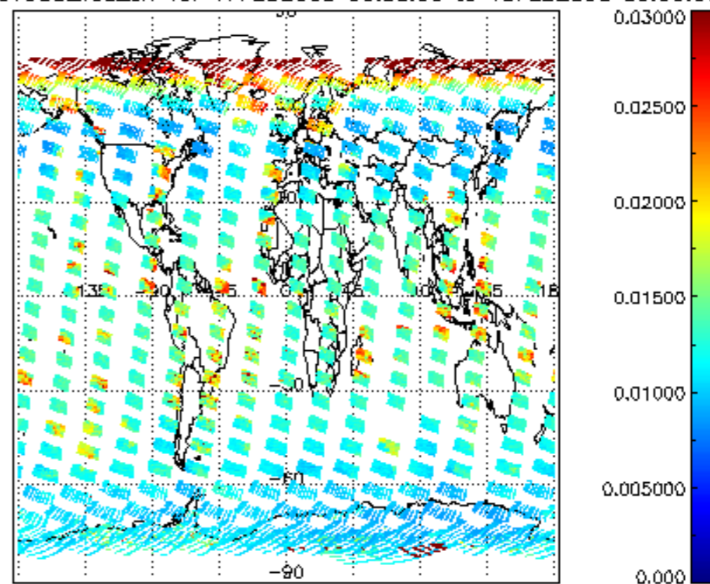
SCIOL2P_NADUV003_vcd_err for 17FEB2008 00:00:00 to 18FEB2008 00:00:00
