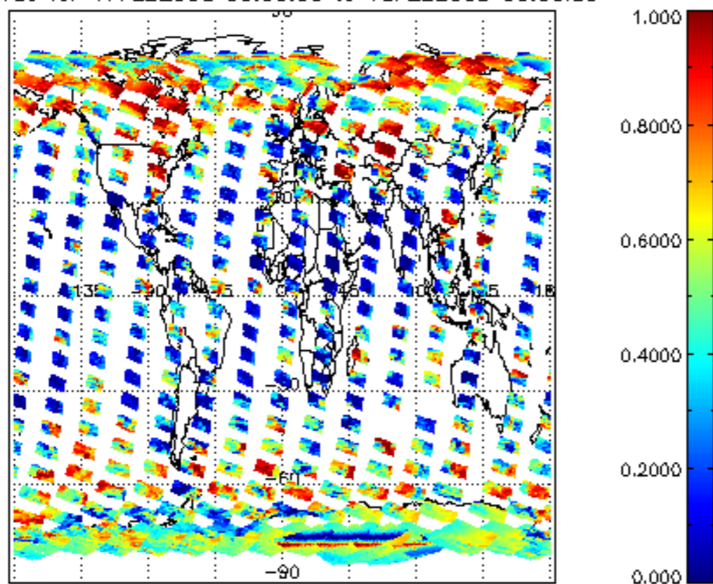
cl_frac for 17FEB2008 00:00:00 to 18FEB2008 00:00:00
