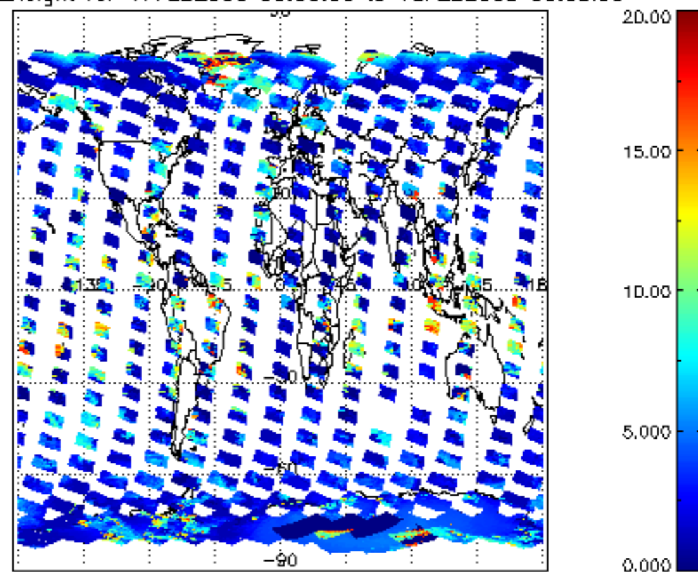
cl_top_height for 17FEB2008 00:00:00 to 18FEB2008 00:00:00
