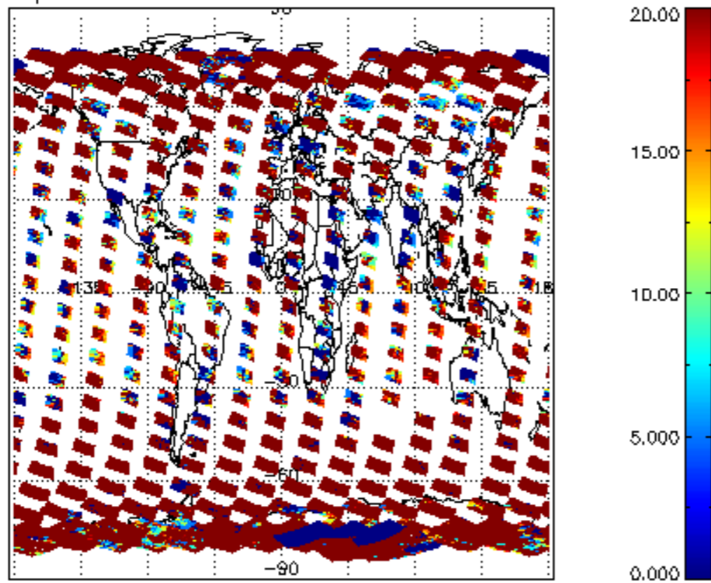
cl_lopt_depth for 17FEB2008 00:00:00 to 18FEB2008 00:00:00
