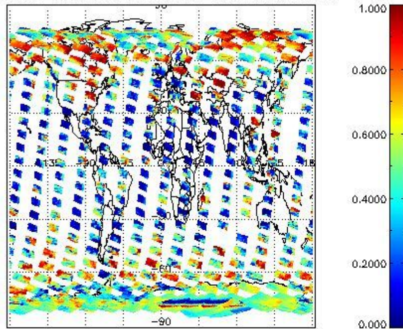
cLfrac for 17FEB2008 00:00:00 to 18FEB2008 00:00:00
