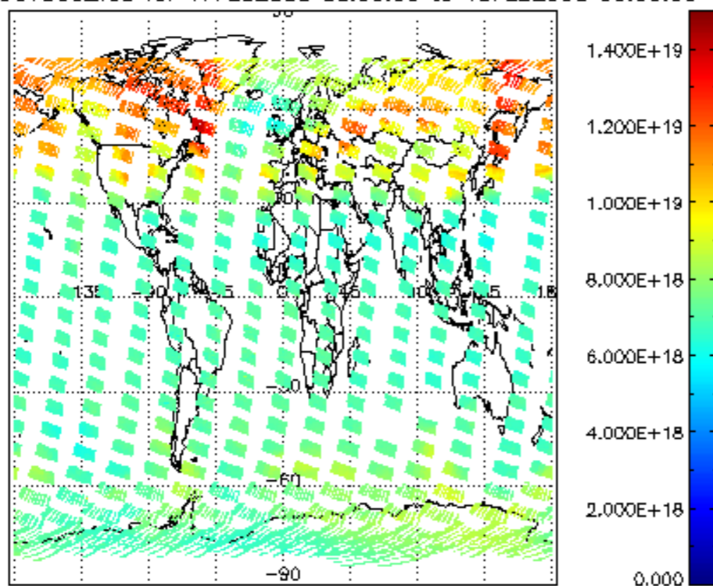
SCIOL2P_NADUV003_vcd for 17FEB2008 00:00:00 to 18FEB2008 00:00:00
