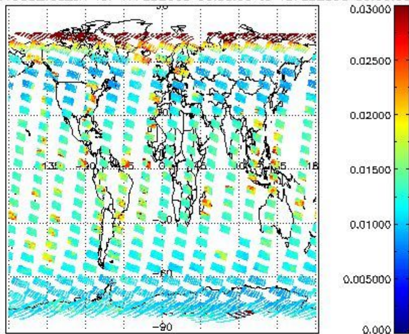
SCIOL2P_NADUV003_vcd_err for 17FEB2008 00:00:00 to 18FEB2008 00:00:00
