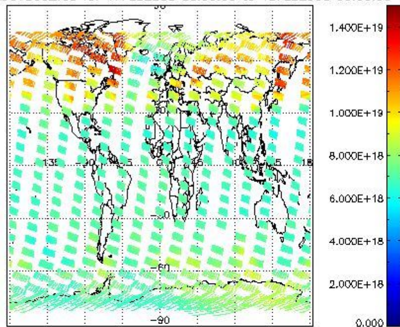
SCIOL2P_NADUV003_vcd for 17FEB2008 00:00:00 to 18FEB2008 00:00:00
