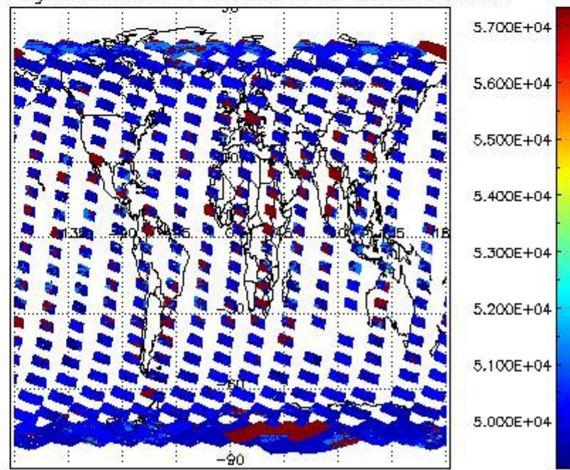
cloud_flags for 17FEB2008 00:00:00 to 18FEB2008 00:00:00
