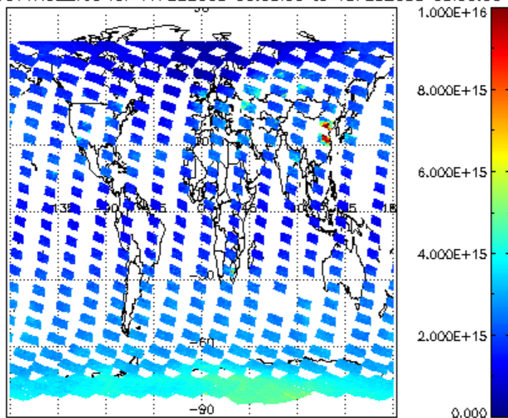
SCIOL2P_NADUV1NO2_vcd for 17FEB2008 00:00:00 to 18FEB2008 00:00:00
