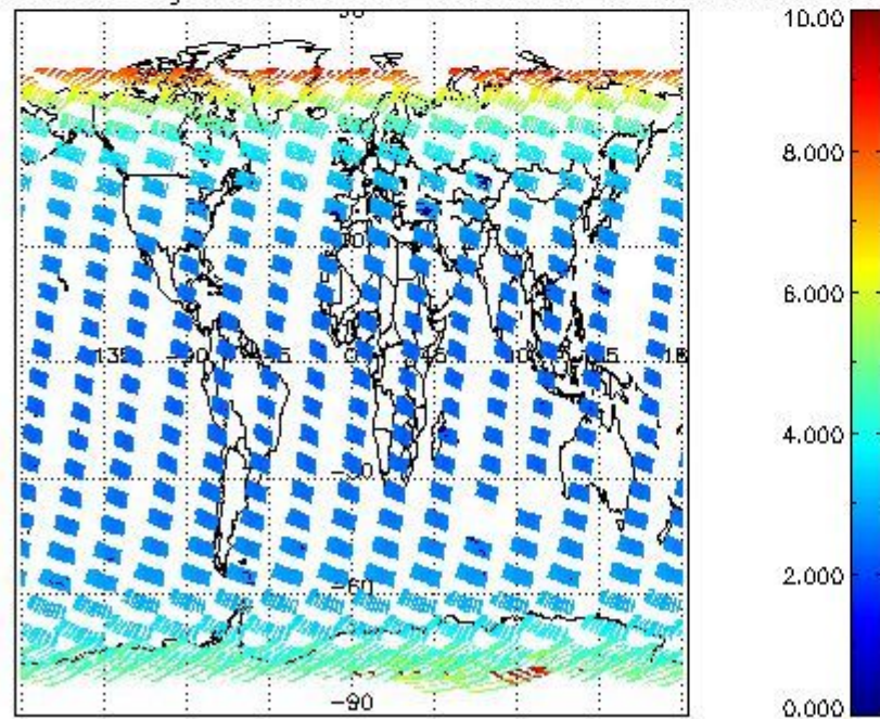
SCIOL2P_NADUV003_amf_gr for 17FEB2008 00:00:00 to 18FEB2008 00:00:00
