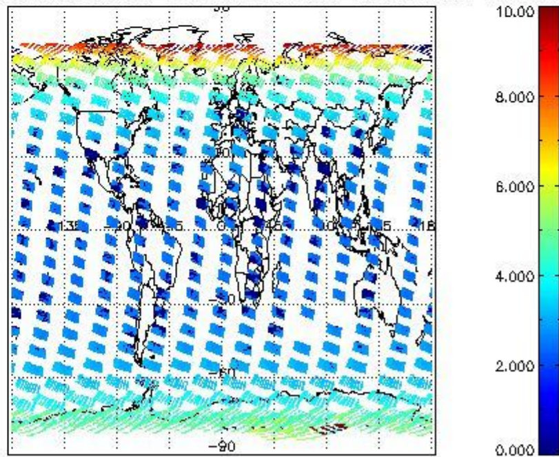
SCIOL2P_NADUV003_amf_cl for 17FEB2008 00:00:00 to 18FEB2008 00:00:00
