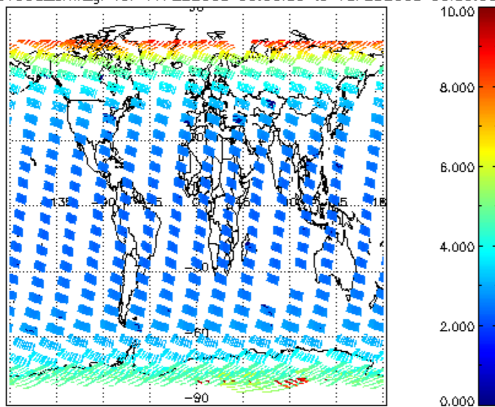
SCIOL2P_NADUV003_amf_gr for 17FEB2008 00:00:00 to 18FEB2008 00:00:00
