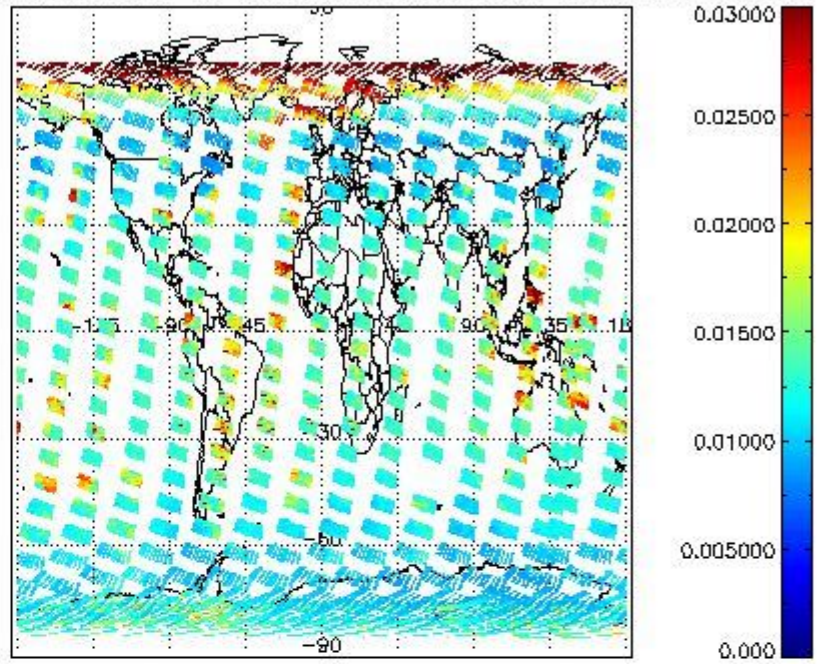
SCIOL2P_NADUV003_vcd_err for 16FEB2008 00:00:00 to 17FEB2008 00:00:00
