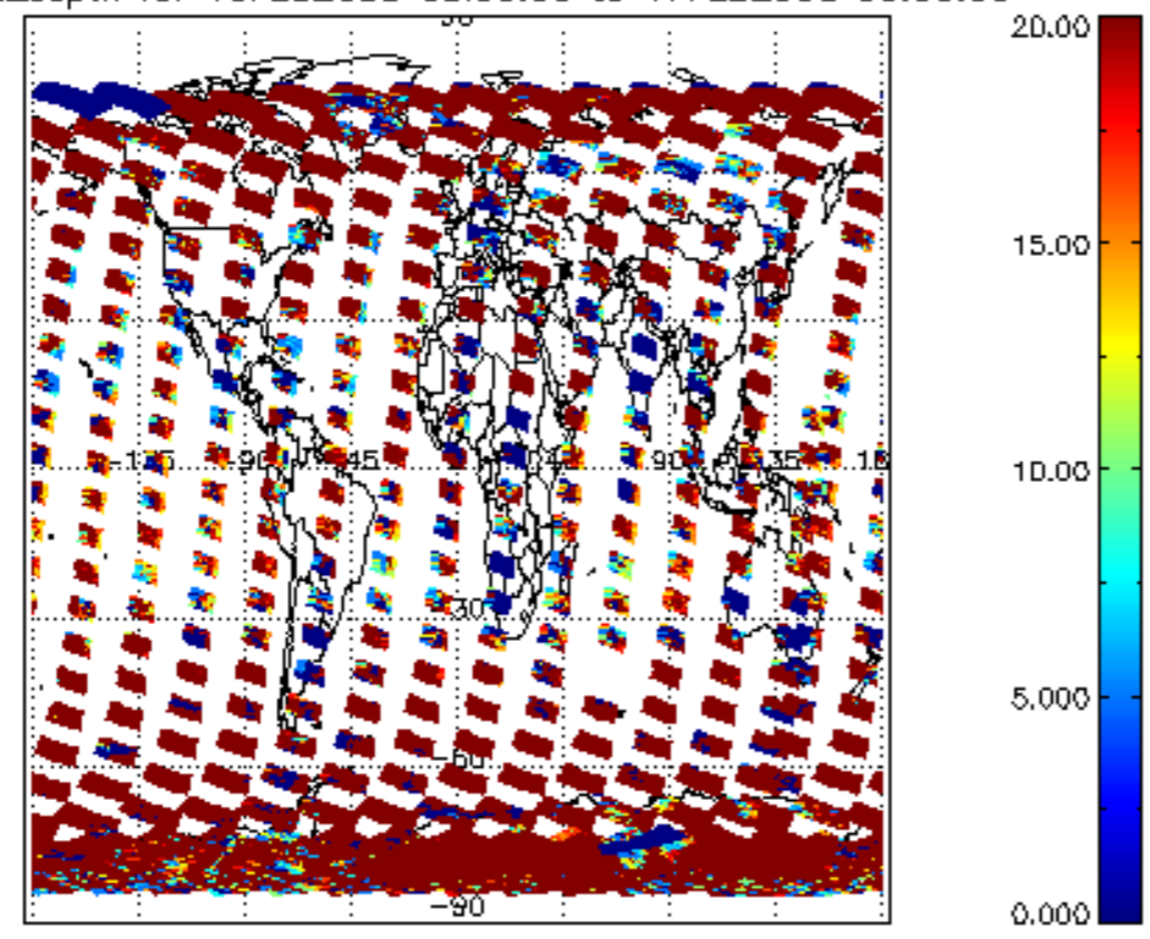
cl_lopt_depth for 16FEB2008 00:00:00 to 17FEB2008 00:00:00
