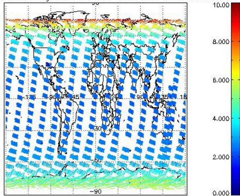
SCIOL2P_NADUV003_amf_gr for 16FEB2008 00:00:00 to 17FEB2008 00:00:00
