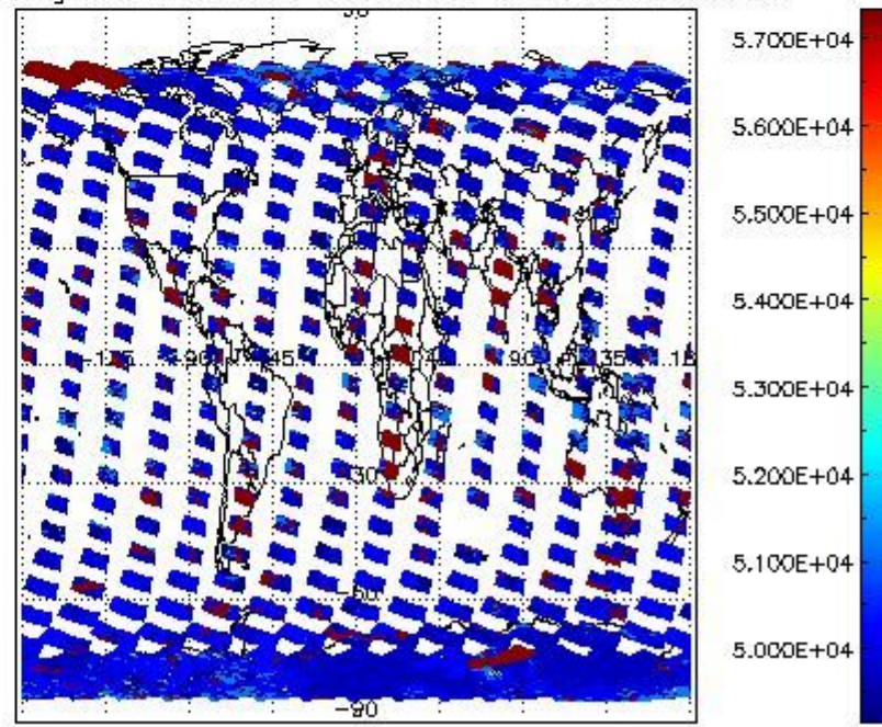
cloud_flags for 16FEB2008 00:00:00 to 17FEB2008 00:00:00
