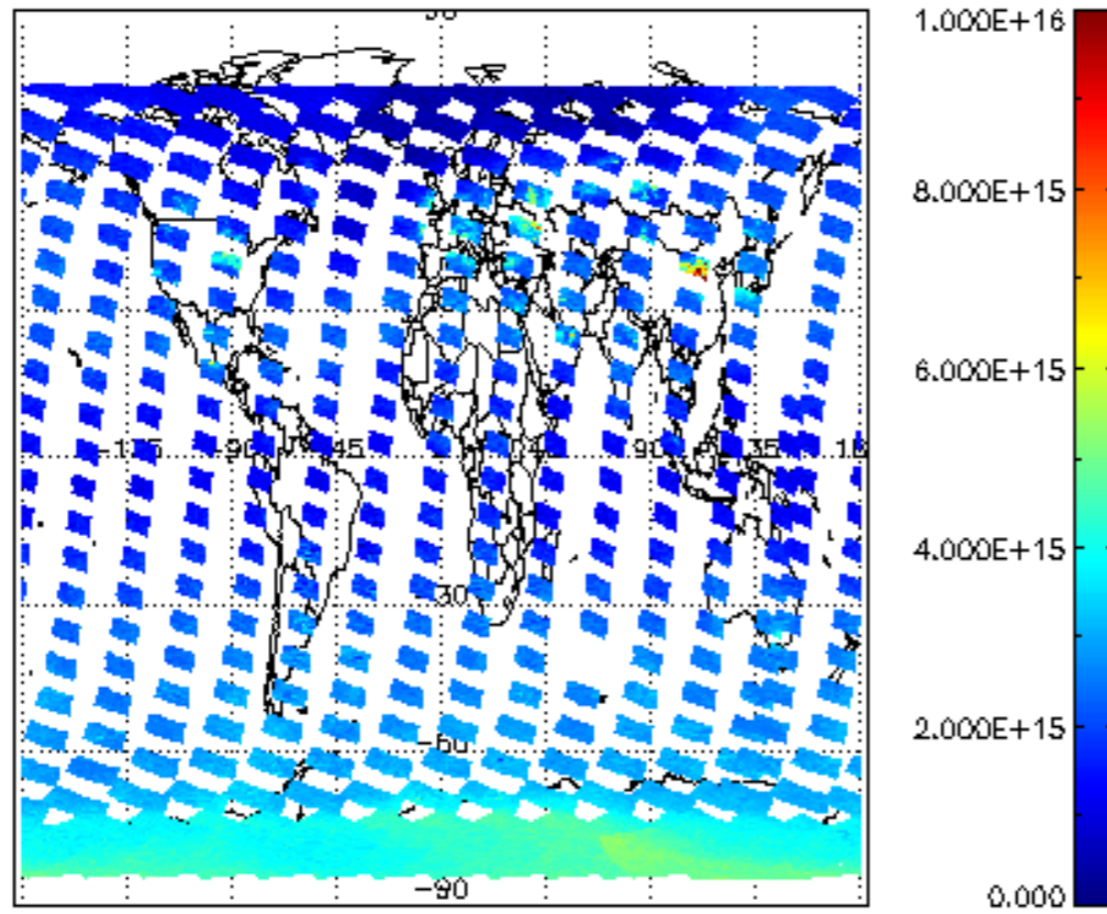
SCIOL2P_NADUV1NO2_vcd for 16FEB2008 00:00:00 to 17FEB2008 00:00:00
