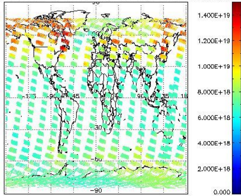
SCIOL2P_NADUV003_vcd for 16FEB2008 00:00:00 to 17FEB2008 00:00:00
