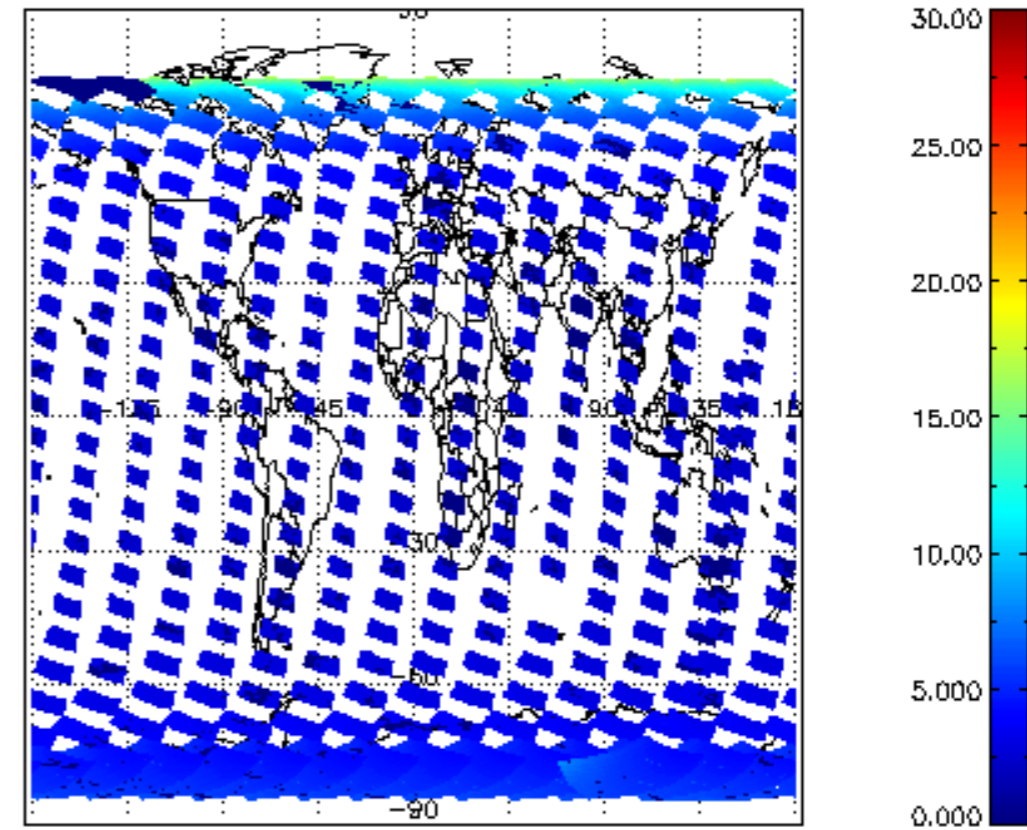
SCIOL2P_NADUV1NO2_amf_cl for 16FEB2008 00:00:00 to 17FEB2008 00:00:00
