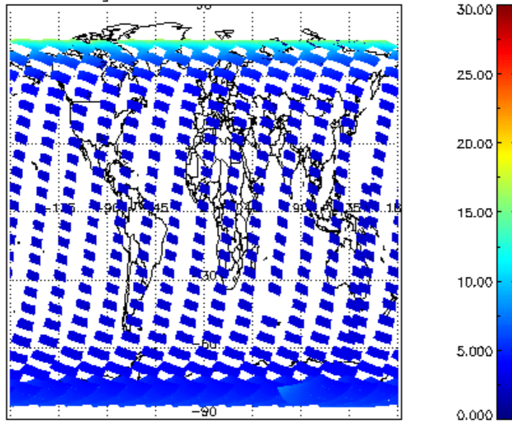
SCIOL2P_NADUV1NO2_amf_gr for 16FEB2008 00:00:00 to 17FEB2008 00:00:00
