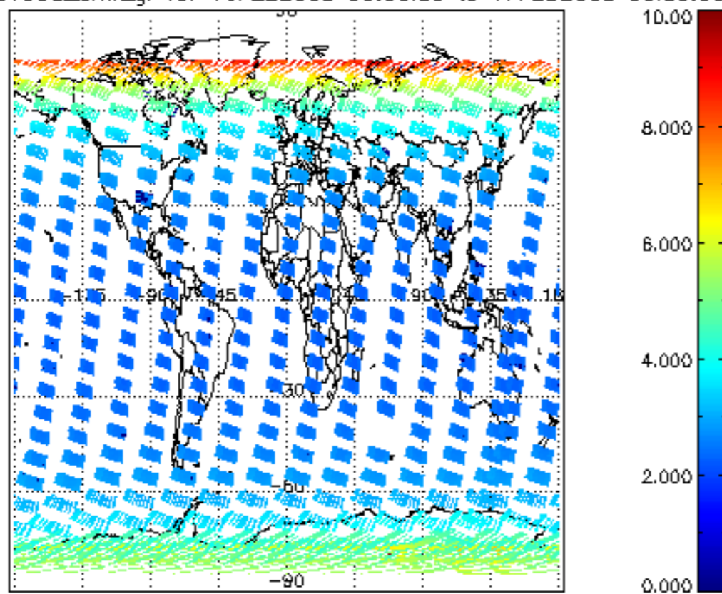
SCIOL2P_NADUV003_amf_gr for 16FEB2008 00:00:00 to 17FEB2008 00:00:00
