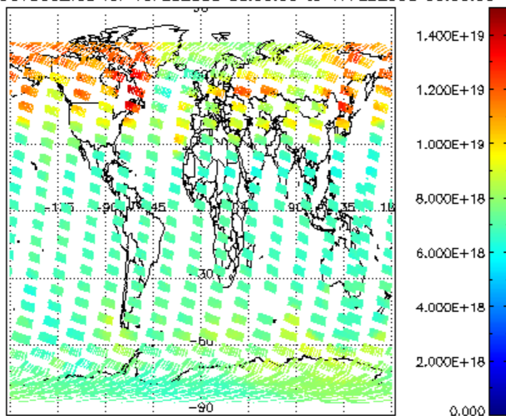
SCIOL2P_NADUV003_vcd for 16FEB2008 00:00:00 to 17FEB2008 00:00:00
