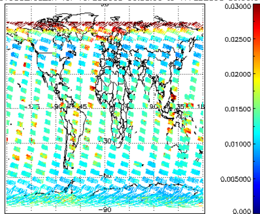
SCIOL2P_NADUV003_vcd_err for 16FEB2008 00:00:00 to 17FEB2008 00:00:00
