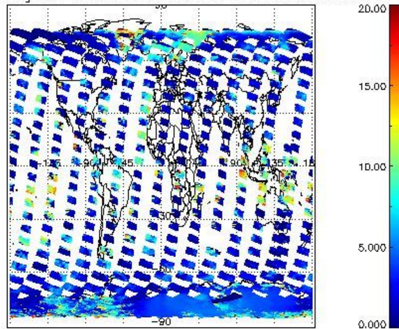
cL_top_height for 16FEB2008 00:00:00 to 17FEB2008 00:00:00
