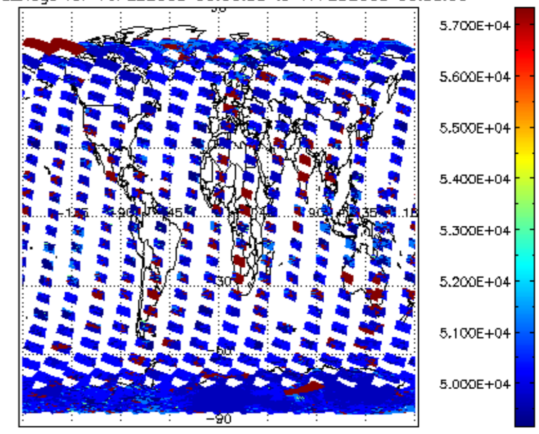
cloud_flags for 16FEB2008 00:00:00 to 17FEB2008 00:00:00
