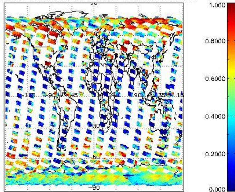
cL_frac for 16FEB2008 00:00:00 to 17FEB2008 00:00:00
