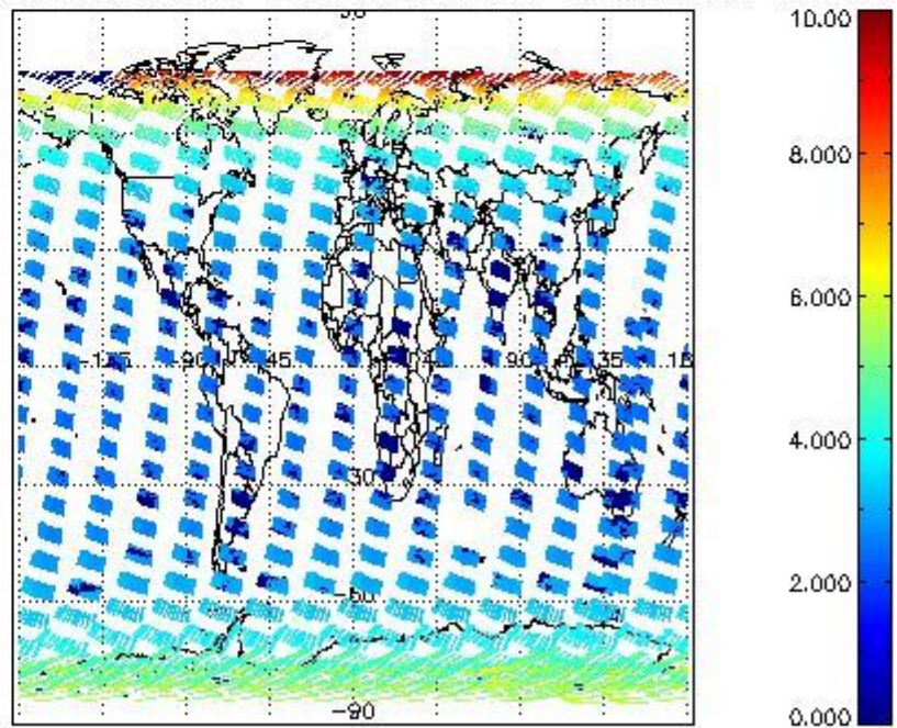
SCIOL2P_NADUV003_amf_cl for 16FEB2008 00:00:00 to 17FEB2008 00:00:00
