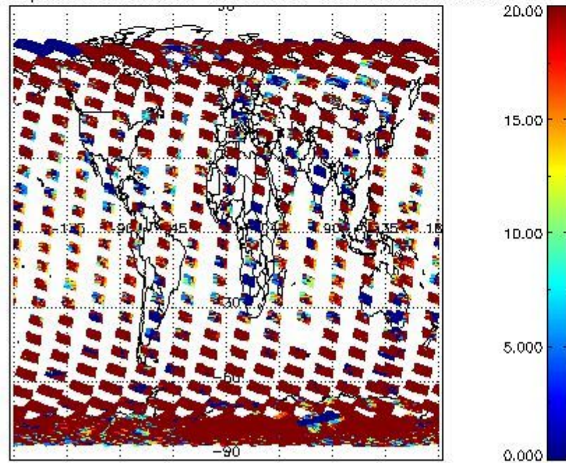
cL_opt_depth for 16FEB2008 00:00:00 to 17FEB2008 00:00:00
