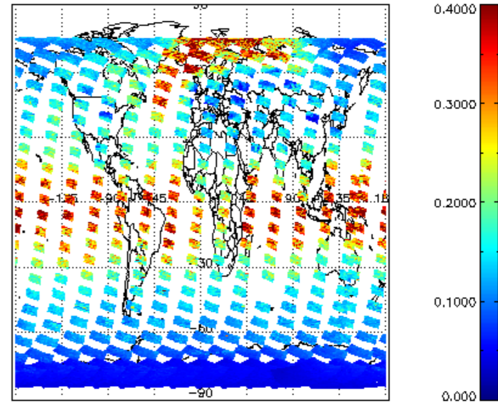
SCIOL2P_NADUV1NO2_vcd_err for 16FEB2008 00:00:00 to 17FEB2008 00:00:00
