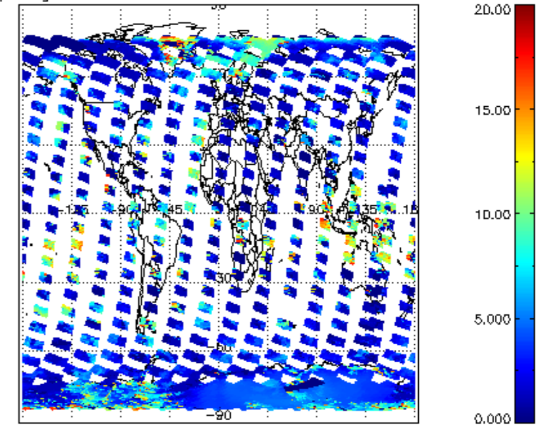
cl_top_height for 16FEB2008 00:00:00 to 17FEB2008 00:00:00
