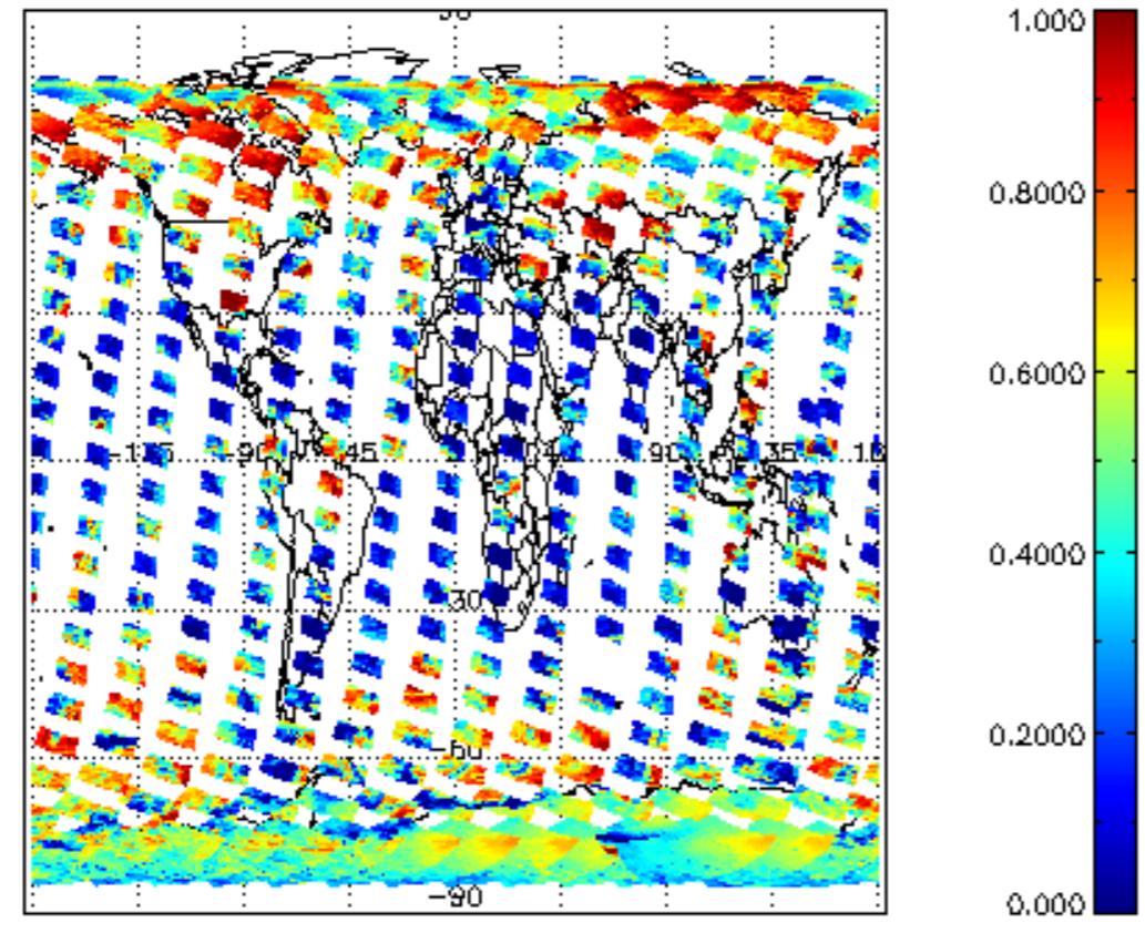
cl_frac for 16FEB2008 00:00:00 to 17FEB2008 00:00:00
