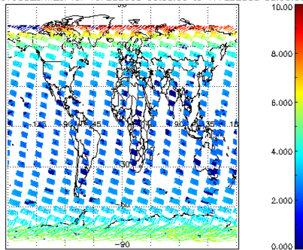
SCIOL2P_NADUV003_amf_cl for 16FEB2008 00:00:00 to 17FEB2008 00:00:00
