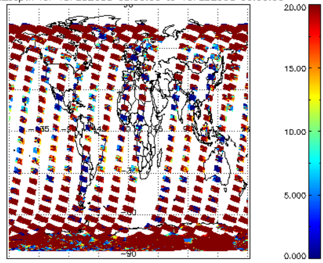
cL_opt_depth for 15FEB2008 00:00:00 to 16FEB2008 00:00:00
