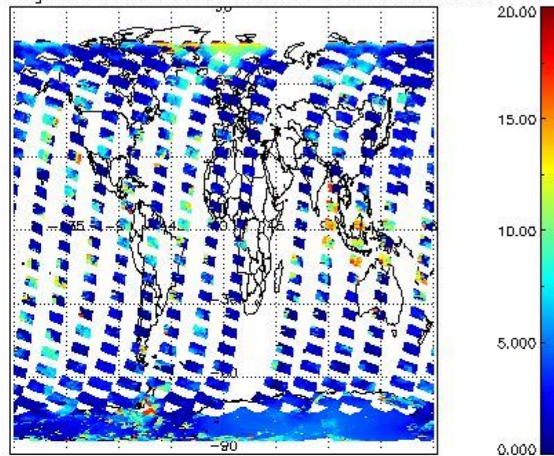
cL_top_height for 15FEB2008 00:00:00 to 16FEB2008 00:00:00
