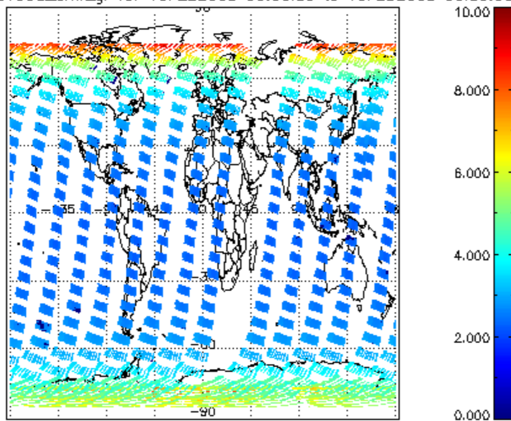
SCIOL2P_NADUV003_amf_gr for 15FEB2008 00:00:00 to 16FEB2008 00:00:00
