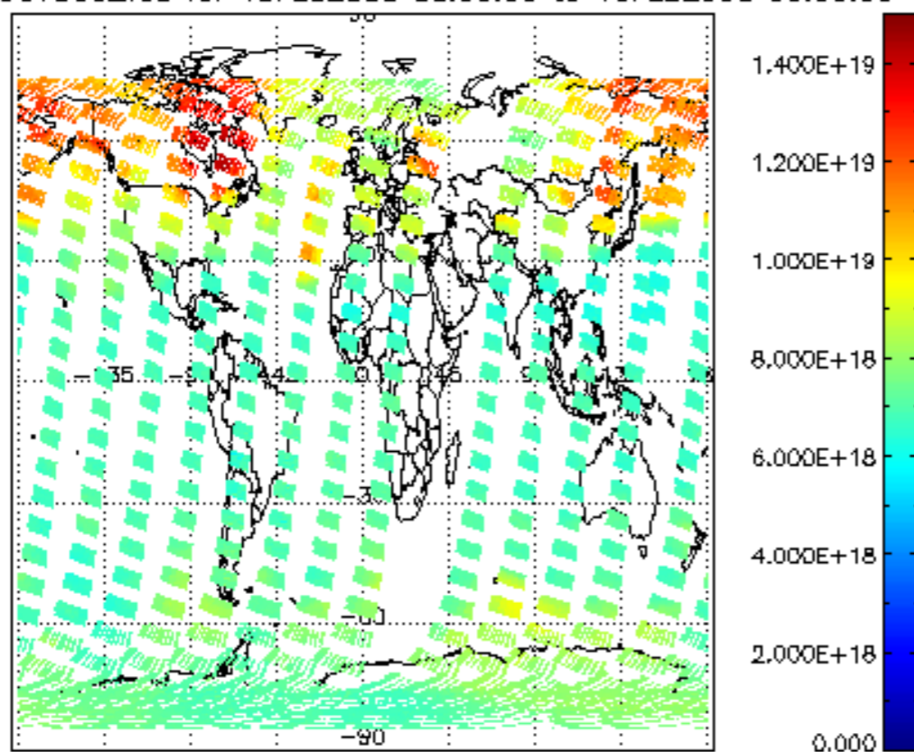
SCIOL2P_NADUV003_vcd for 15FEB2008 00:00:00 to 16FEB2008 00:00:00
