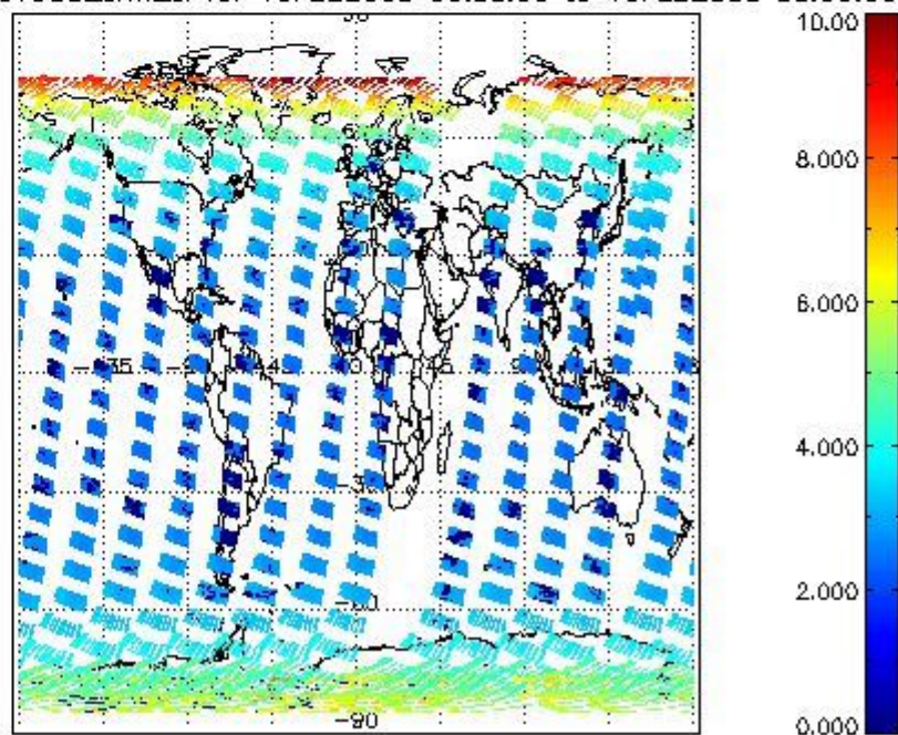
SCIOL2P_NADUV003_amf_cl for 15FEB2008 00:00:00 to 16FEB2008 00:00:00
