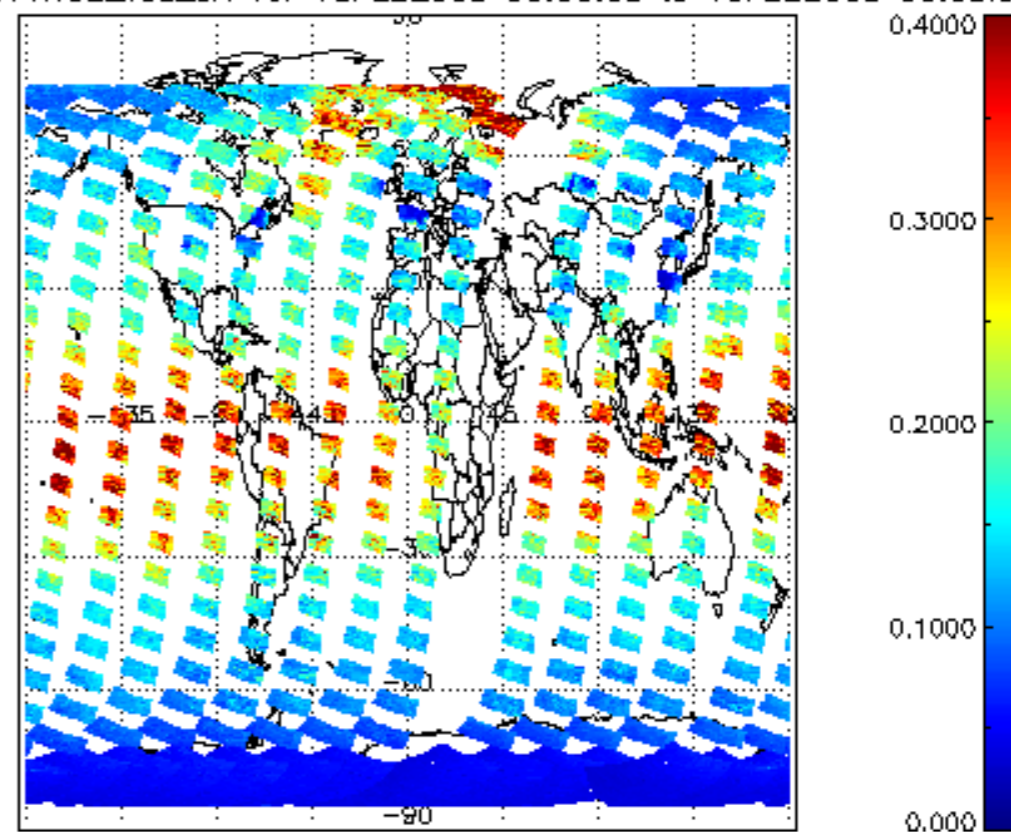
SCIOL2P_NADUV1NO2_vcd_err for 15FEB2008 00:00:00 to 16FEB2008 00:00:00
