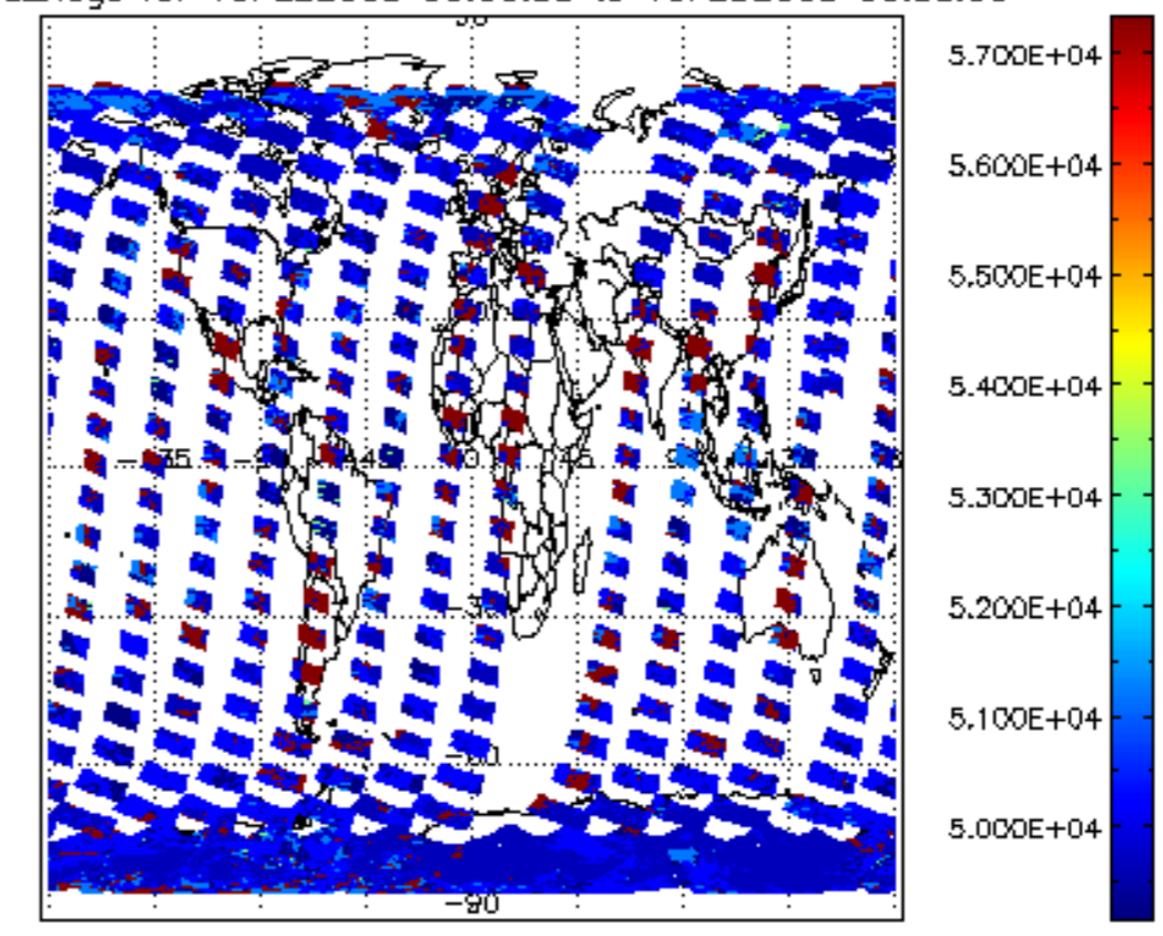
cloud_flags for 15FEB2008 00:00:00 to 16FEB2008 00:00:00
