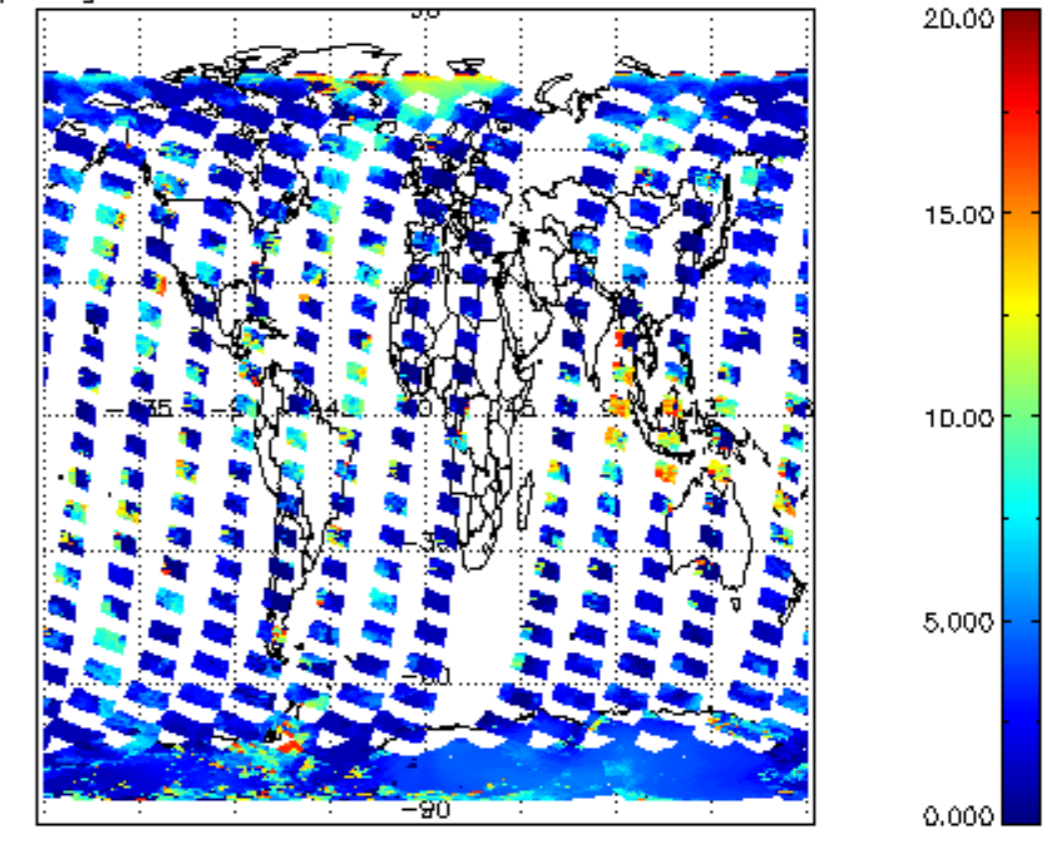
cL_top_height for 15FEB2008 00:00:00 to 16FEB2008 00:00:00
