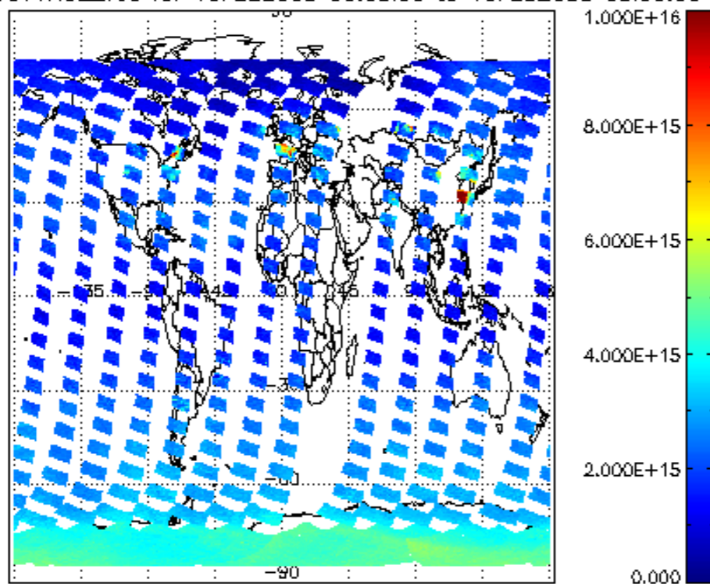
SCIOL2P_NADUV1NO2_vcd for 15FEB2008 00:00:00 to 16FEB2008 00:00:00
