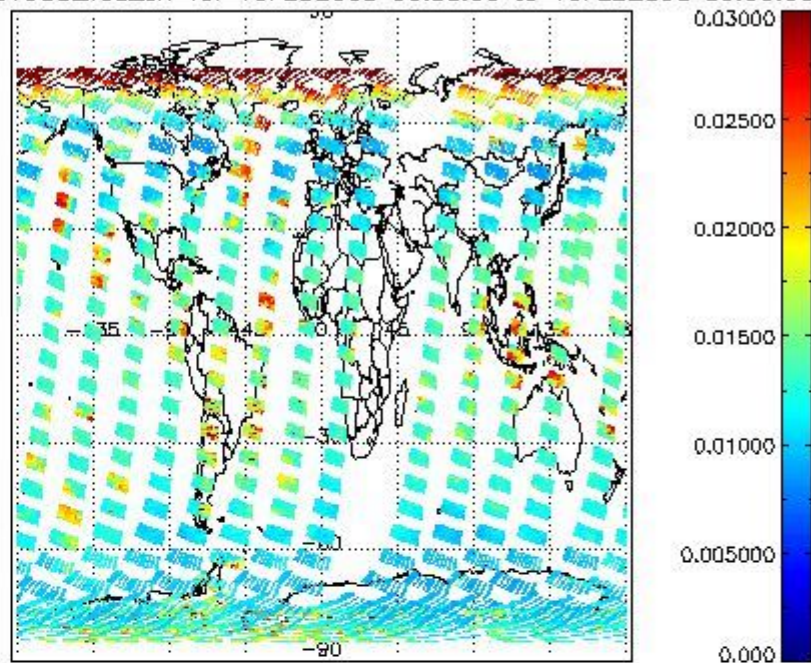
SCIOL2P_NADUV003_vcd_err for 15FEB2008 00:00:00 to 16FEB2008 00:00:00
