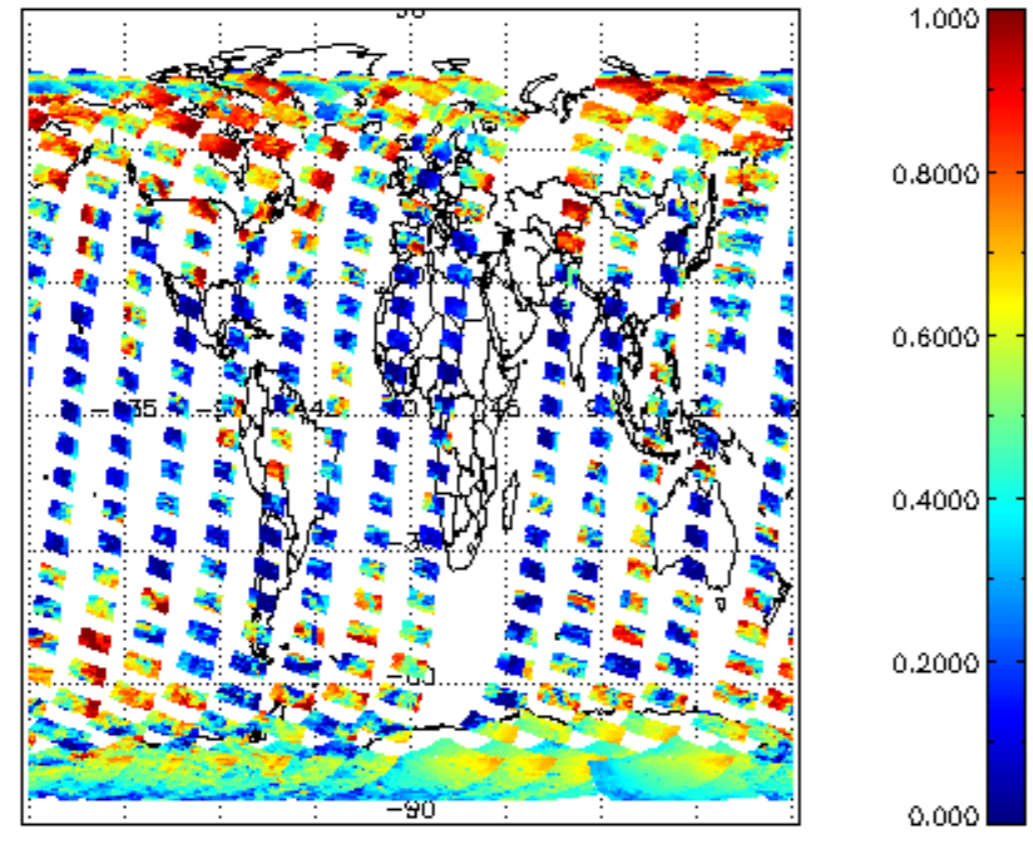
cL_frac for 15FEB2008 00:00:00 to 16FEB2008 00:00:00
