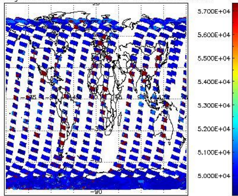
cloud_flags for 15FEB2008 00:00:00 to 16FEB2008 00:00:00
