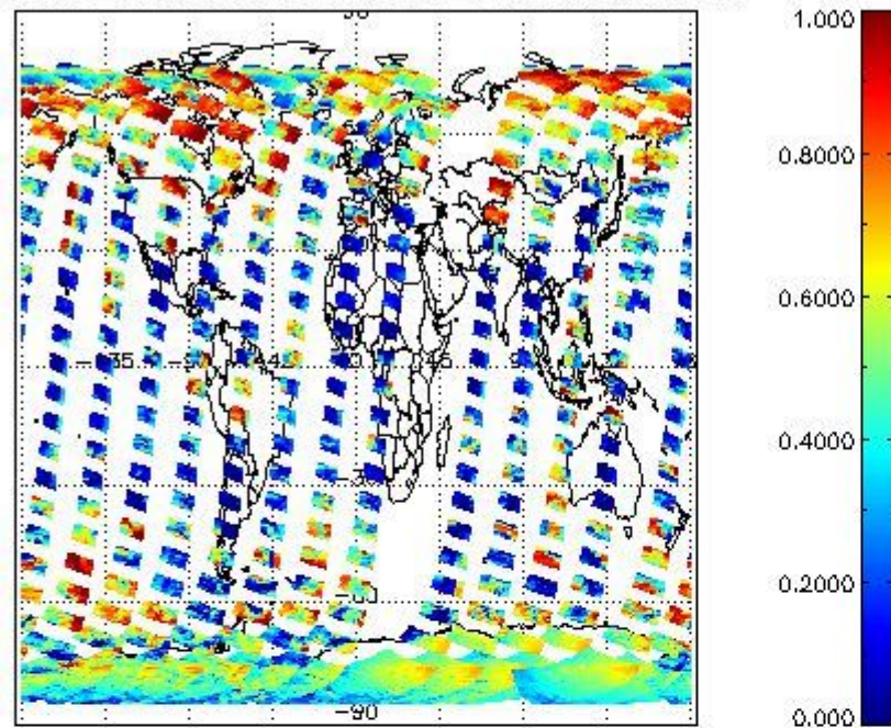
cLfrac for 15FEB2008 00:00:00 to 16FEB2008 00:00:00
