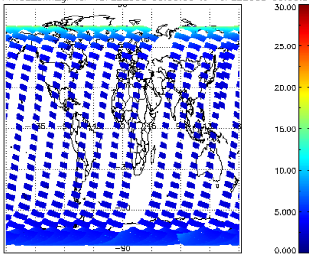
SCIOL2P_NADUV1NO2_amf_gr for 15FEB2008 00:00:00 to 16FEB2008 00:00:00
