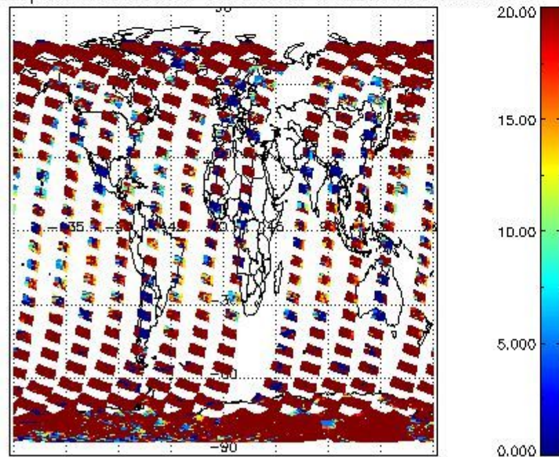
cLopt_depth for 15FEB2008 00:00:00 to 16FEB2008 00:00:00
