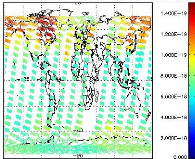
SCIOL2P_NADUV003_vcd for 15FEB2008 00:00:00 to 16FEB2008 00:00:00
