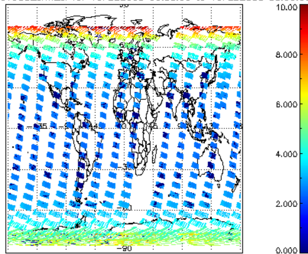
SCIOL2P_NADUV003_amf_cl for 15FEB2008 00:00:00 to 16FEB2008 00:00:00
