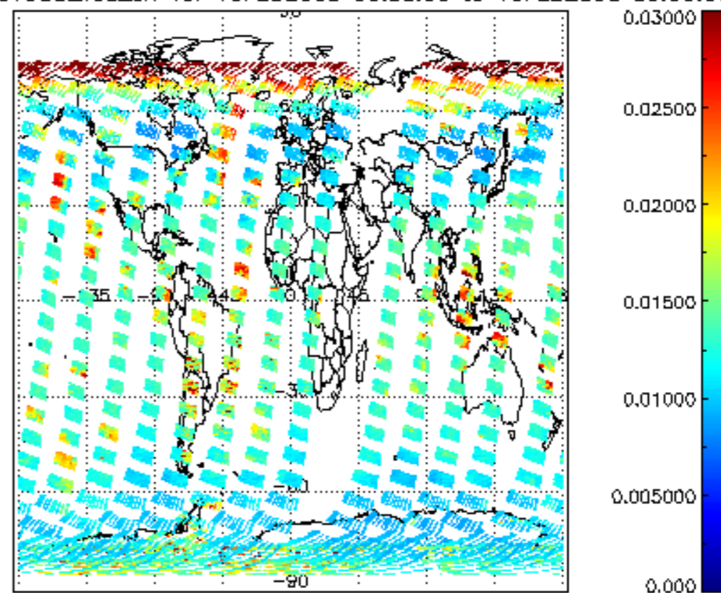
SCIOL2P_NADUV003_vcd_err for 15FEB2008 00:00:00 to 16FEB2008 00:00:00
