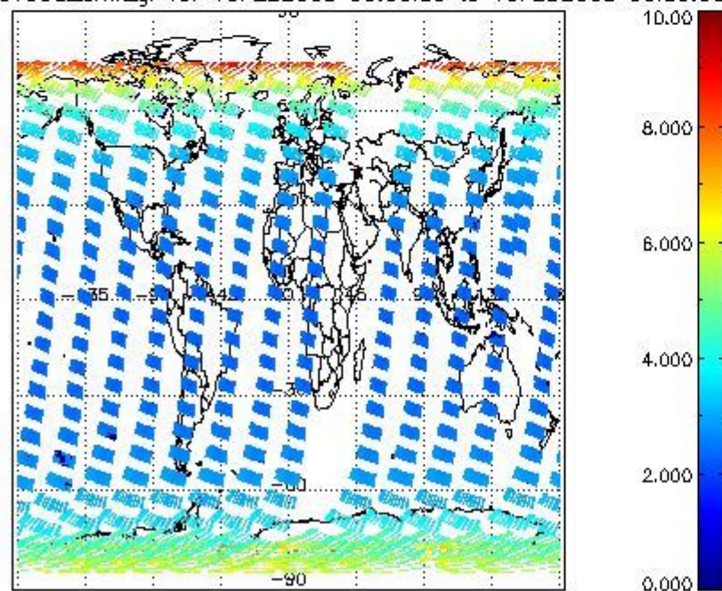
SCIOL2P_NADUV003_amf_gr for 15FEB2008 00:00:00 to 16FEB2008 00:00:00
