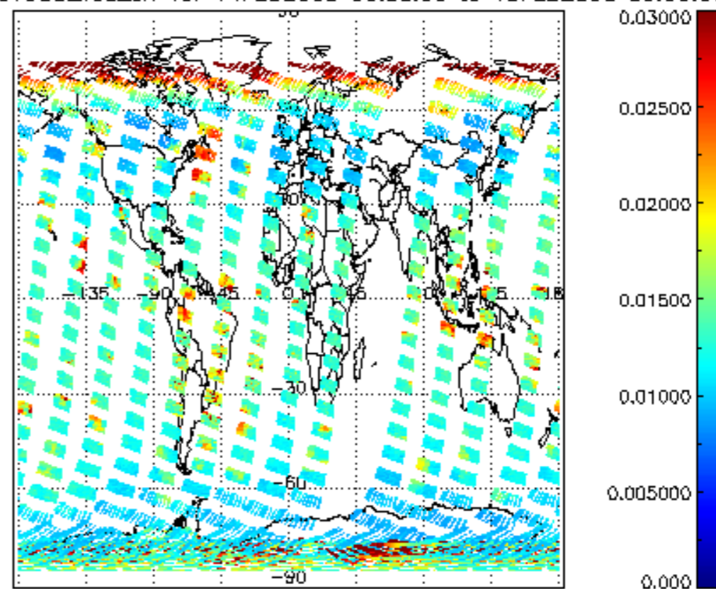
SCIOL2P_NADUV003_vcd_err for 14FEB2008 00:00:00 to 15FEB2008 00:00:00
