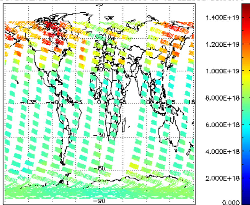
SCIOL2P_NADUV003_vcd for 14FEB2008 00:00:00 to 15FEB2008 00:00:00
