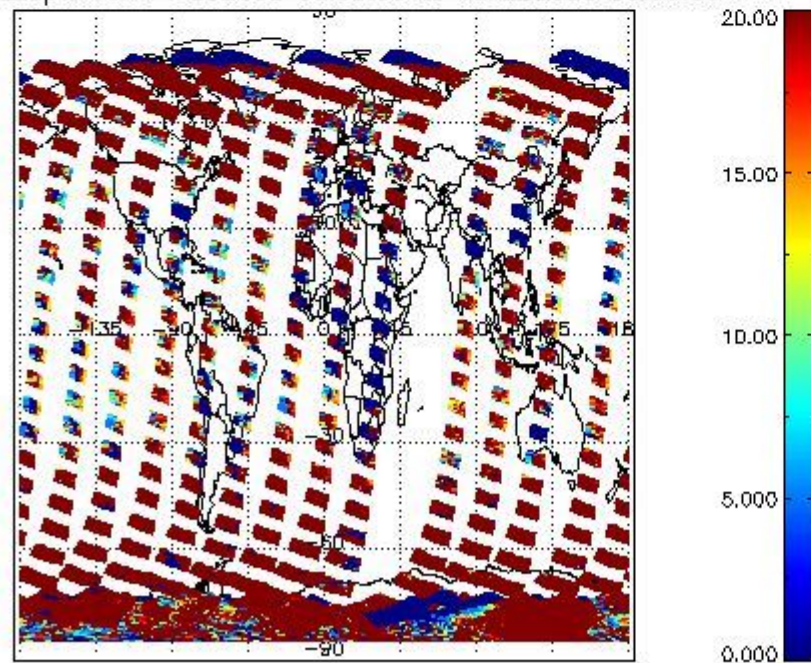
cLopt_depth for 14FEB2008 00:00:00 to 15FEB2008 00:00:00
