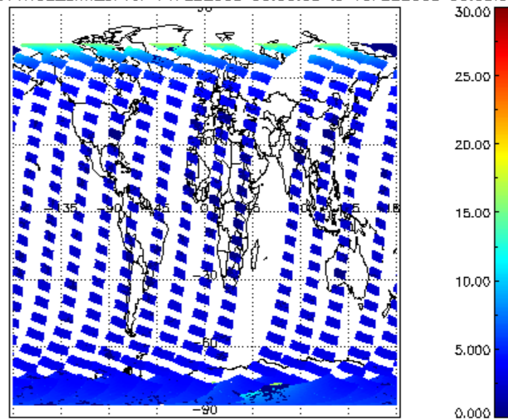
SCIOL2P_NADUV1NO2_amf_cl for 14FEB2008 00:00:00 to 15FEB2008 00:00:00
