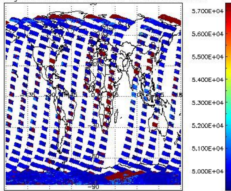
cloud_flags for 14FEB2008 00:00:00 to 15FEB2008 00:00:00
