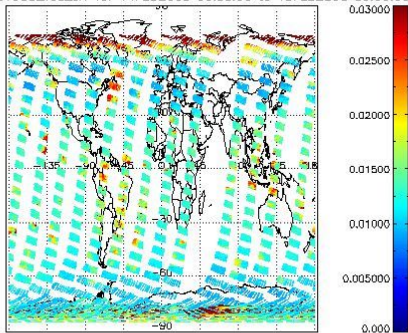
SCIOL2P_NADUV003_vcd_err for 14FEB2008 00:00:00 to 15FEB2008 00:00:00
