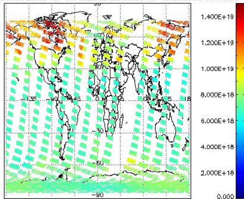
SCIOL2P_NADUV003_vcd for 14FEB2008 00:00:00 to 15FEB2008 00:00:00
