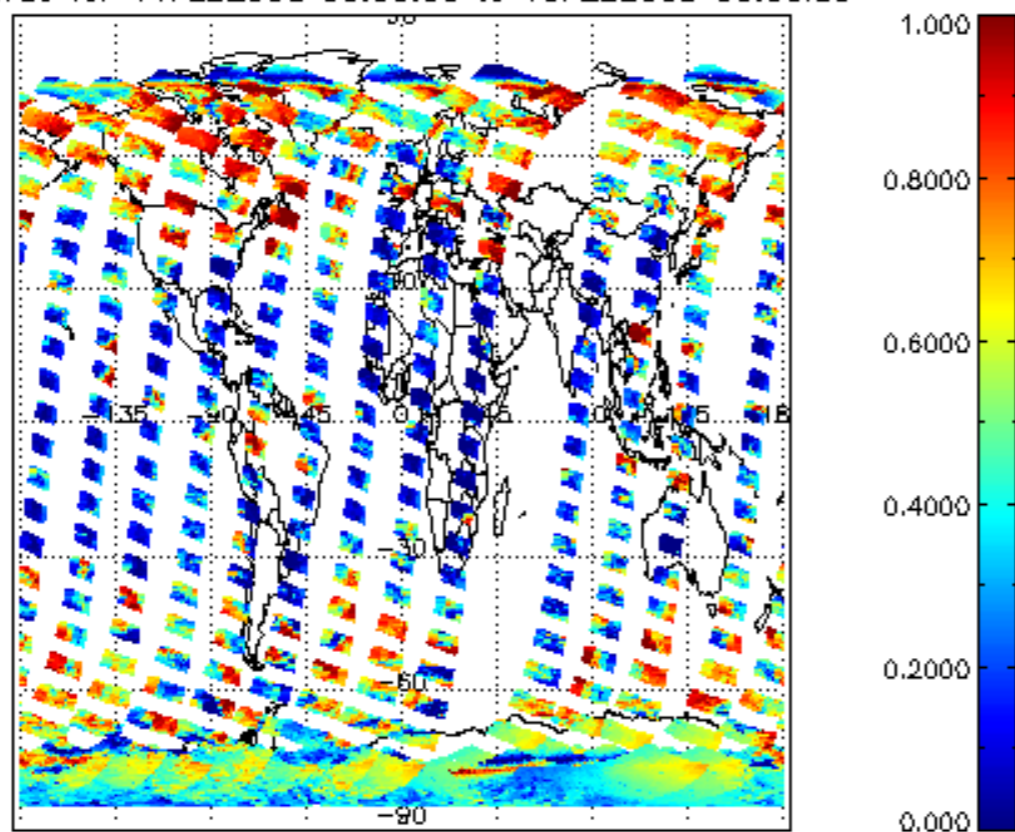
cl_frac for 14FEB2008 00:00:00 to 15FEB2008 00:00:00
