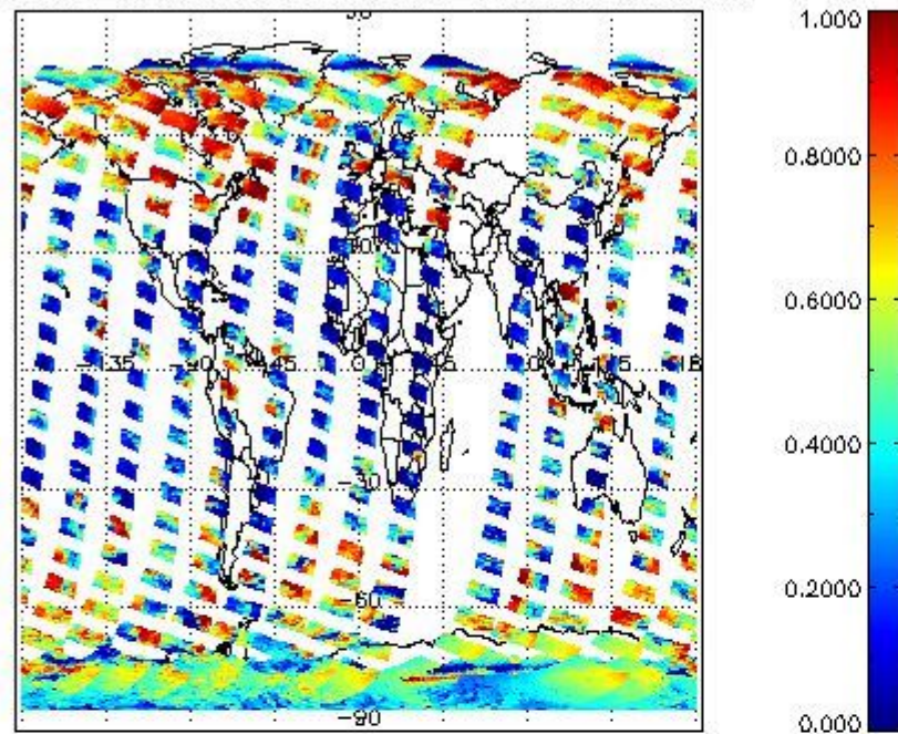
cLfrac for 14FEB2008 00:00:00 to 15FEB2008 00:00:00
