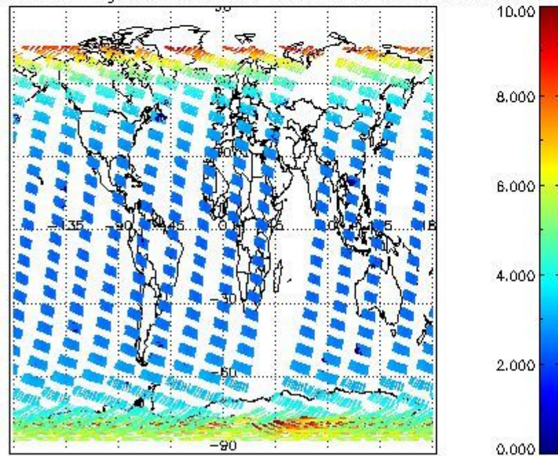
SCIOL2P_NADUV003_amf_gr for 14FEB2008 00:00:00 to 15FEB2008 00:00:00
