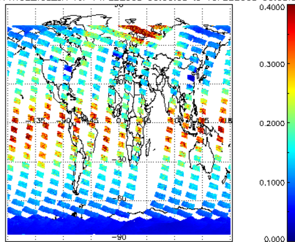
SCIOL2P_NADUV1NO2_vcd_err for 14FEB2008 00:00:00 to 15FEB2008 00:00:00
