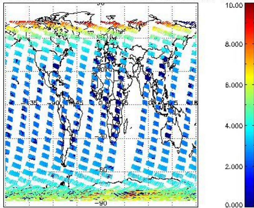
SCIOL2P_NADUV003_amf_cl for 14FEB2008 00:00:00 to 15FEB2008 00:00:00
