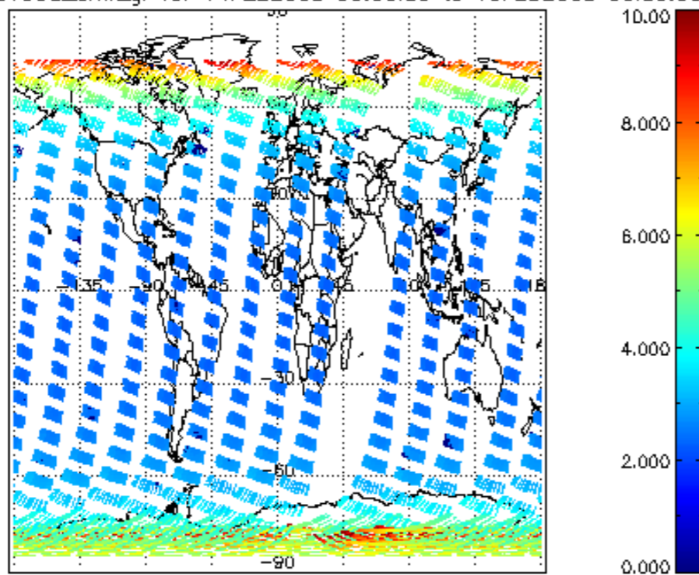
SCIOL2P_NADUV003_amf_gr for 14FEB2008 00:00:00 to 15FEB2008 00:00:00
