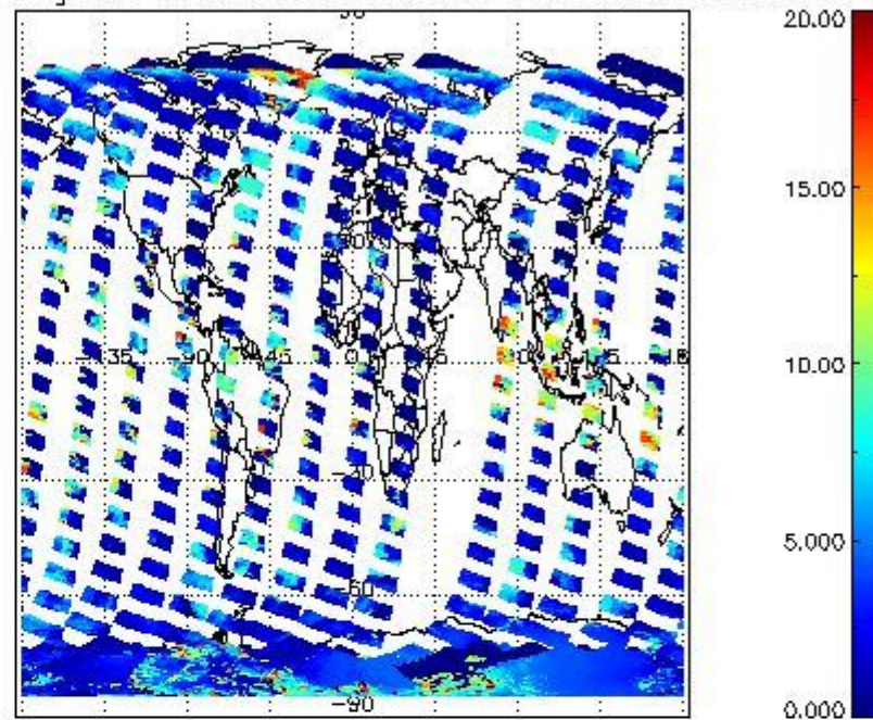
cL_top_height for 14FEB2008 00:00:00 to 15FEB2008 00:00:00
