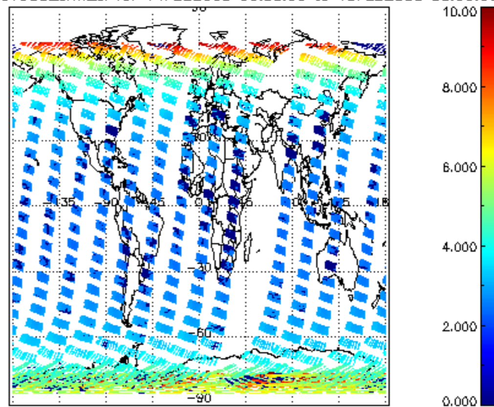
SCIOL2P_NADUV003_amf_cl for 14FEB2008 00:00:00 to 15FEB2008 00:00:00
