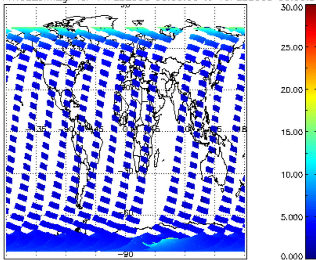
SCIOL2P_NADUV1NO2_amf_gr for 14FEB2008 00:00:00 to 15FEB2008 00:00:00
