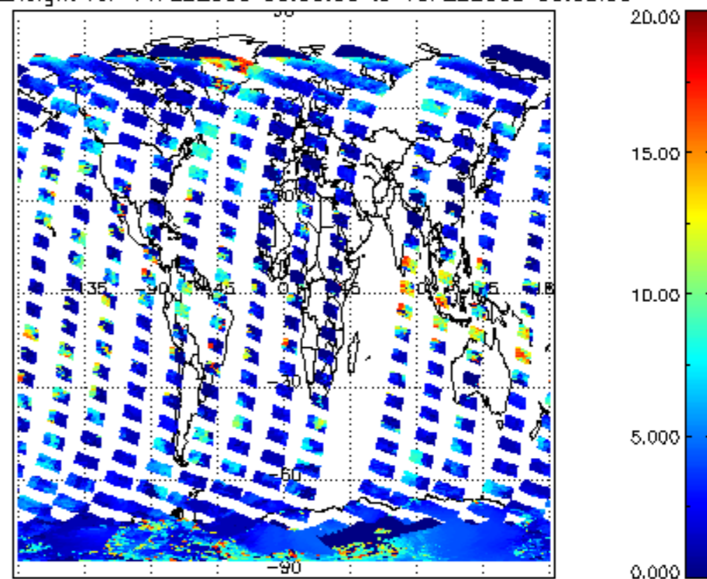
cl_top_height for 14FEB2008 00:00:00 to 15FEB2008 00:00:00
