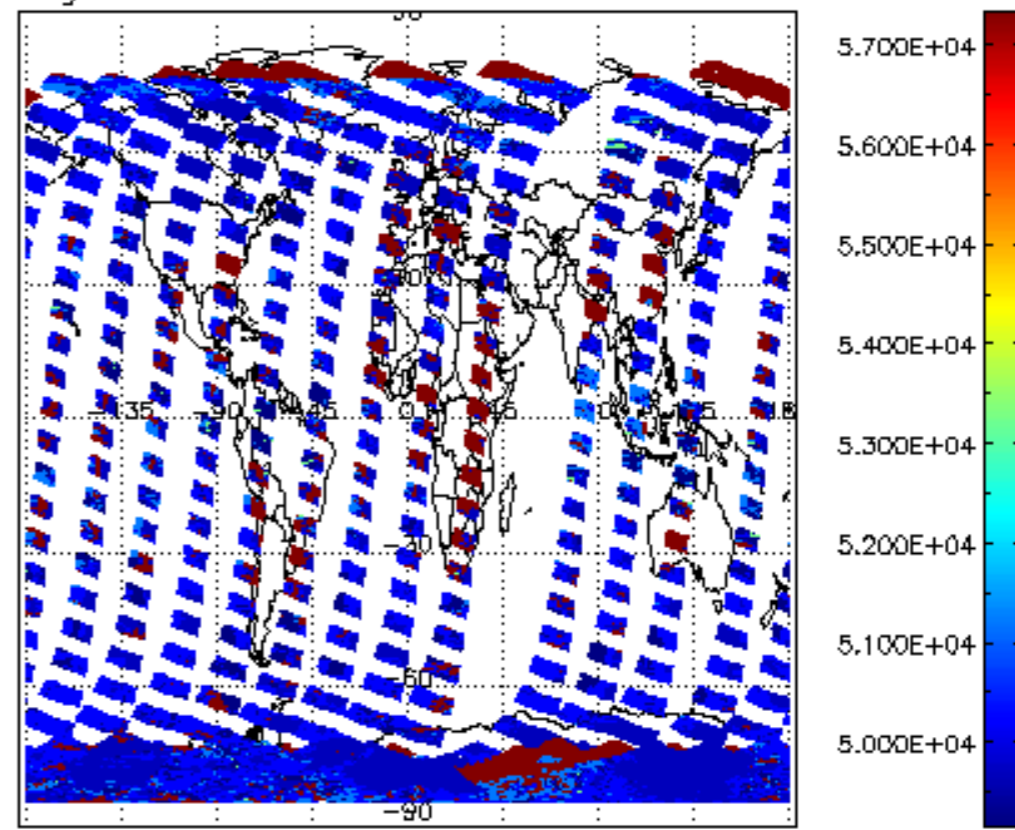
cloud_flags for 14FEB2008 00:00:00 to 15FEB2008 00:00:00
