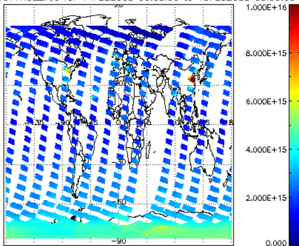
SCIOL2P_NADUV1NO2_vcd for 14FEB2008 00:00:00 to 15FEB2008 00:00:00
