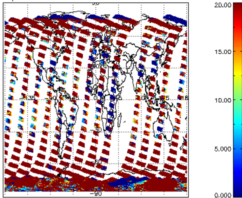
cl_opt_depth for 14FEB2008 00:00:00 to 15FEB2008 00:00:00
