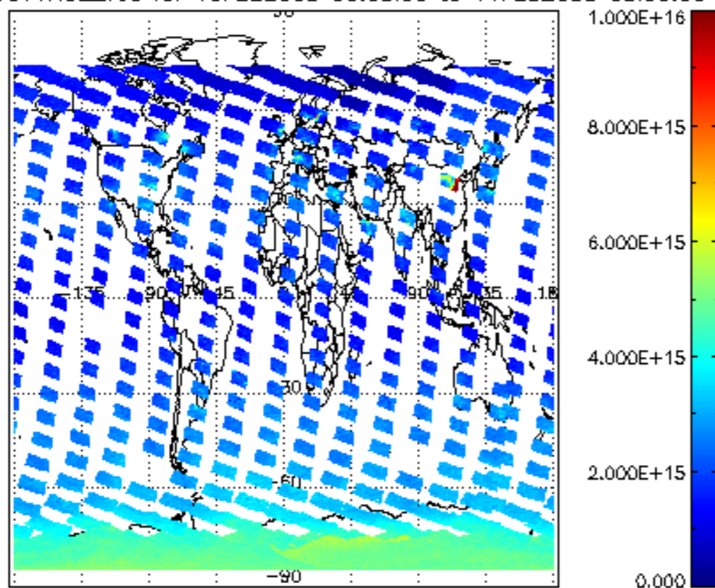
SCIOL2P_NADUV1NO2_vcd for 10FEB2008 00:00:00 to 11FEB2008 00:00:00
