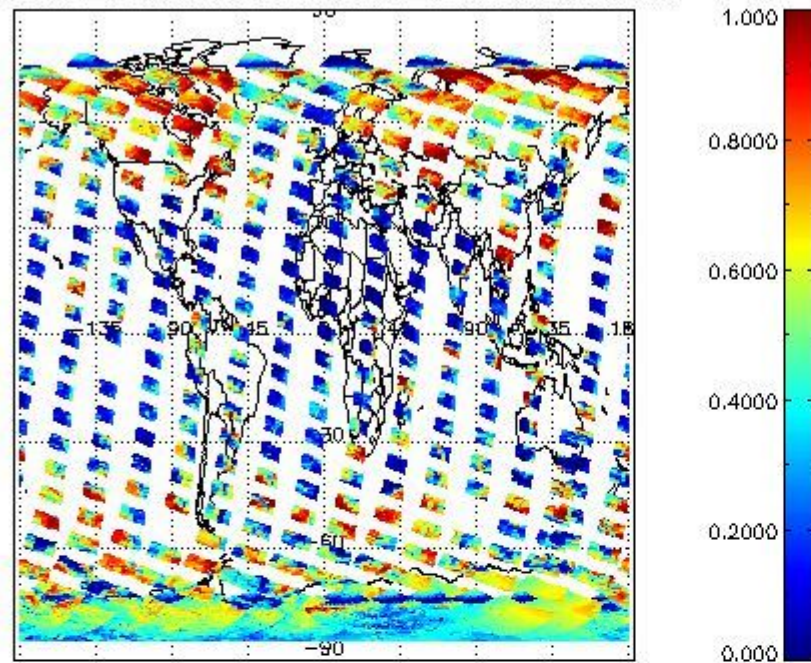
cLfrac for 10FEB2008 00:00:00 to 11FEB2008 00:00:00
