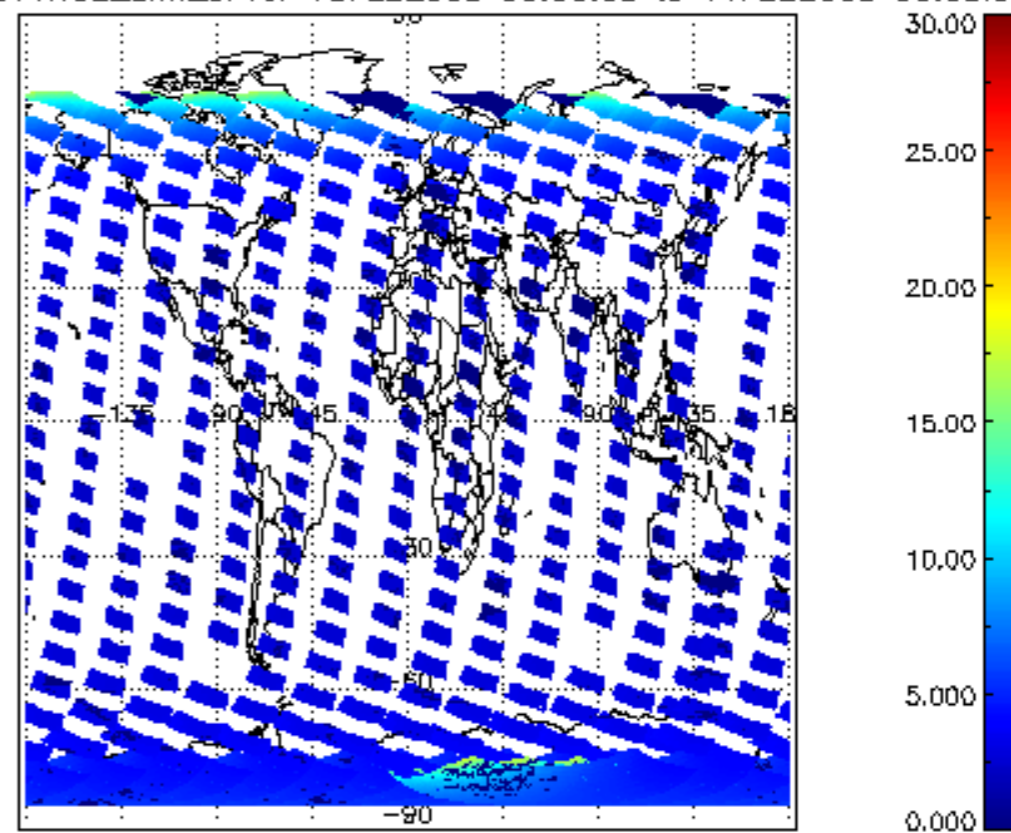
SCIOL2P_NADUV1NO2_amf_cl for 10FEB2008 00:00:00 to 11FEB2008 00:00:00
