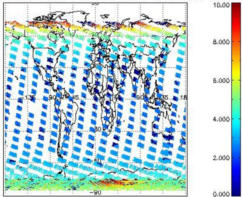
SCIOL2P_NADUV003_amf_cl for 10FEB2008 00:00:00 to 11FEB2008 00:00:00
