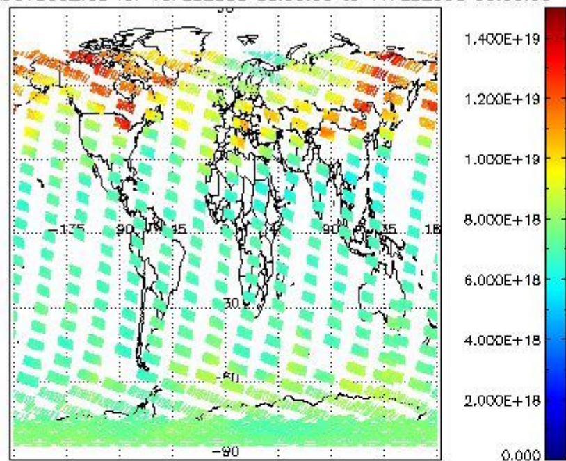
SCIOL2P_NADUV003_vcd for 10FEB2008 00:00:00 to 11FEB2008 00:00:00
