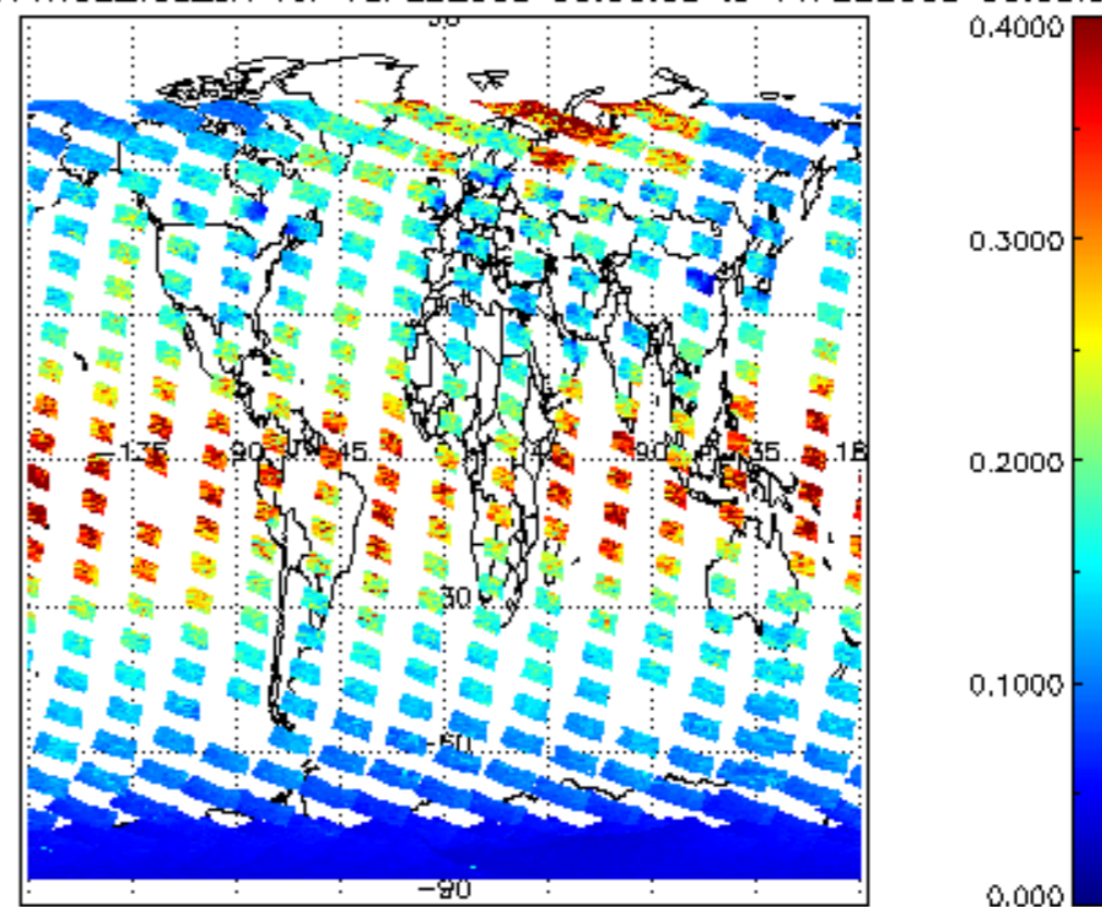
SCIOL2P_NADUV1NO2_vcd_err for 10FEB2008 00:00:00 to 11FEB2008 00:00:00
