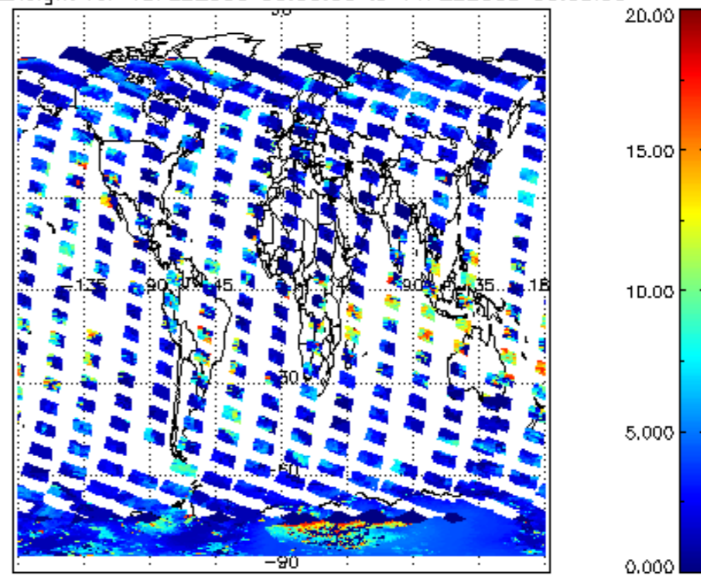
cl_top_height for 10FEB2008 00:00:00 to 11FEB2008 00:00:00
