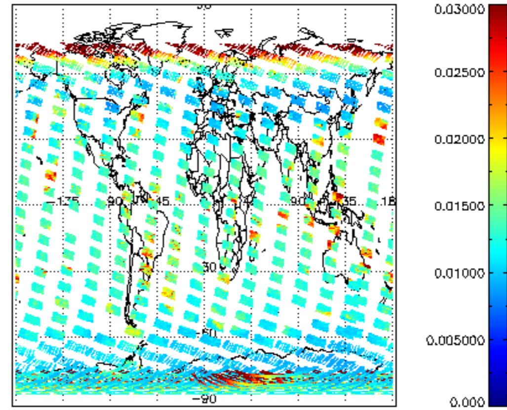
SCIOL2P_NADUV003_vcd_err for 10FEB2008 00:00:00 to 11FEB2008 00:00:00
