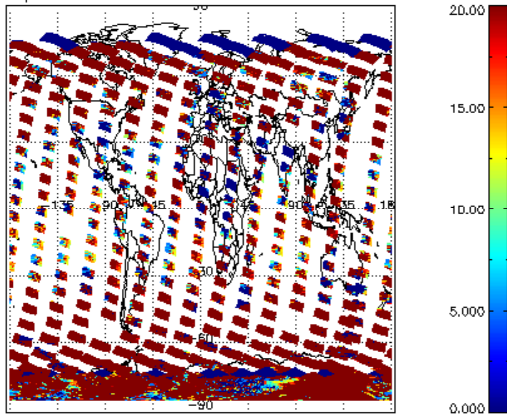
cl_opt_depth for 10FEB2008 00:00:00 to 11FEB2008 00:00:00
