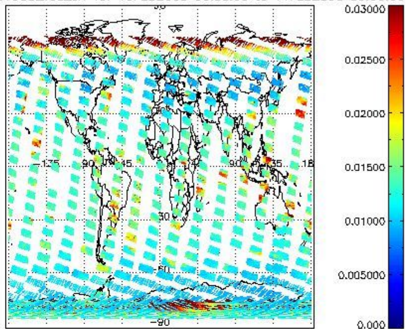
SCIOL2P_NADUV003_vcd_err for 10FEB2008 00:00:00 to 11FEB2008 00:00:00
