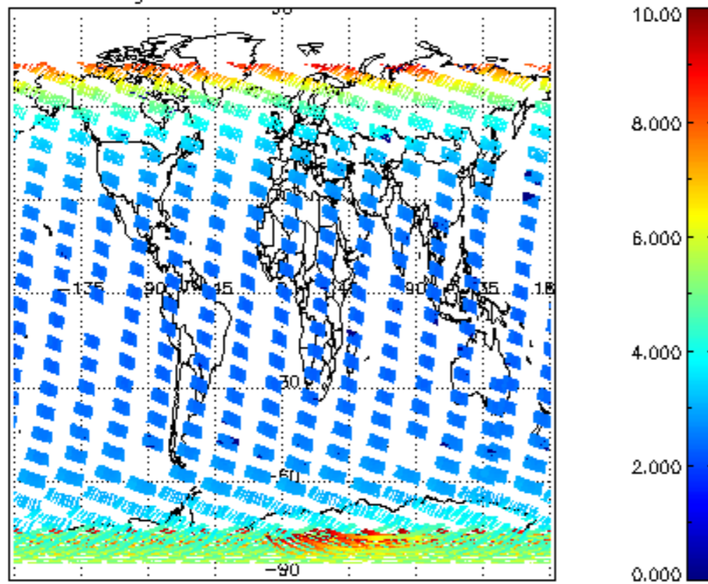
SCIOL2P_NADUV003_amf_gr for 10FEB2008 00:00:00 to 11FEB2008 00:00:00
