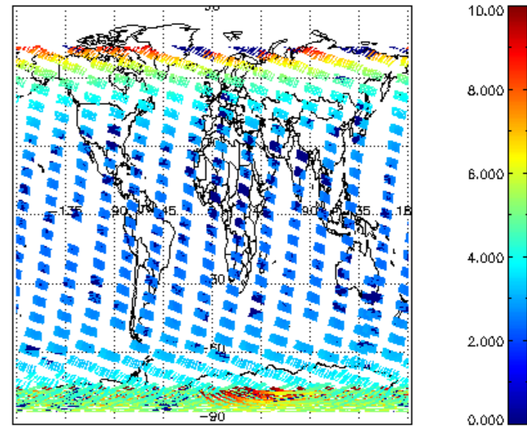
SCIOL2P_NADUV003_amf_cl for 10FEB2008 00:00:00 to 11FEB2008 00:00:00
