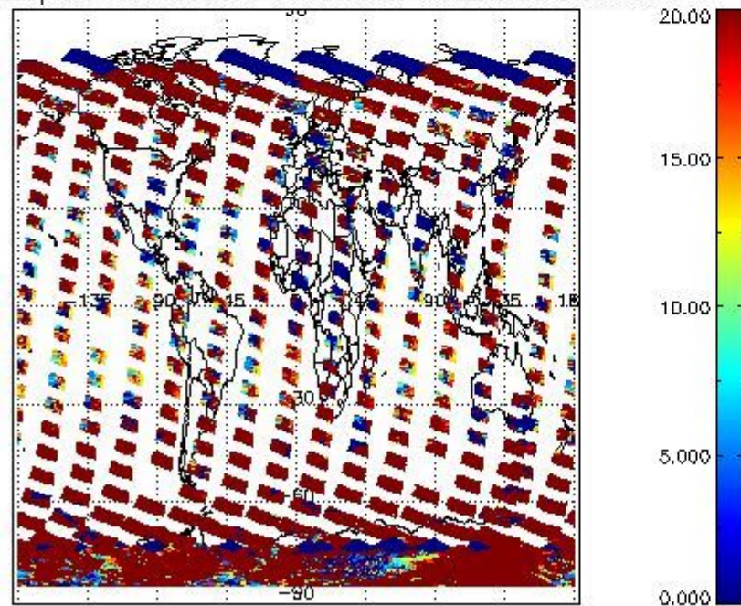
cLopt_depth for 10FEB2008 00:00:00 to 11FEB2008 00:00:00
