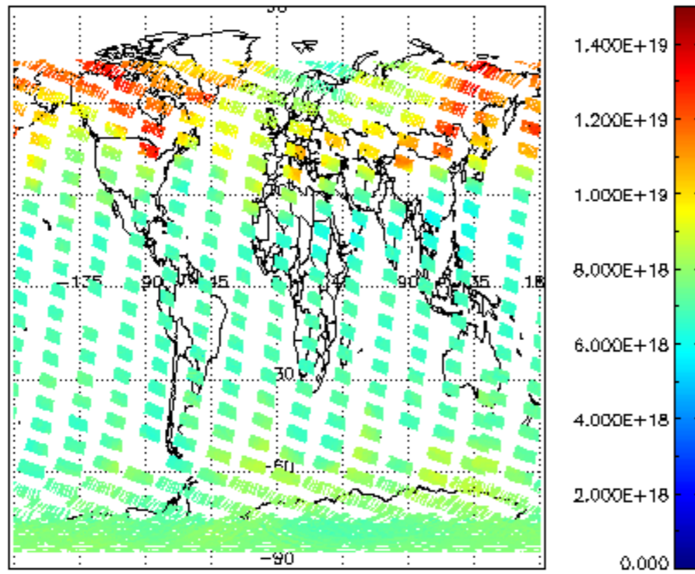
SCIOL2P_NADUV003_vcd for 10FEB2008 00:00:00 to 11FEB2008 00:00:00
