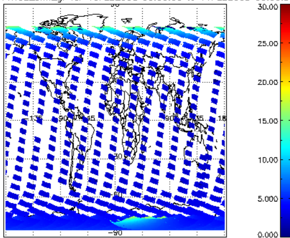
SCIOL2P_NADUV1NO2_amf_gr for 10FEB2008 00:00:00 to 11FEB2008 00:00:00
