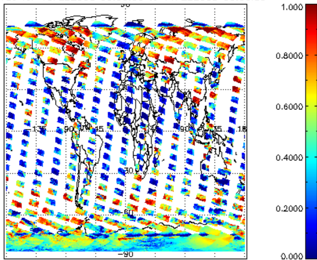
cl_frac for 10FEB2008 00:00:00 to 11FEB2008 00:00:00
