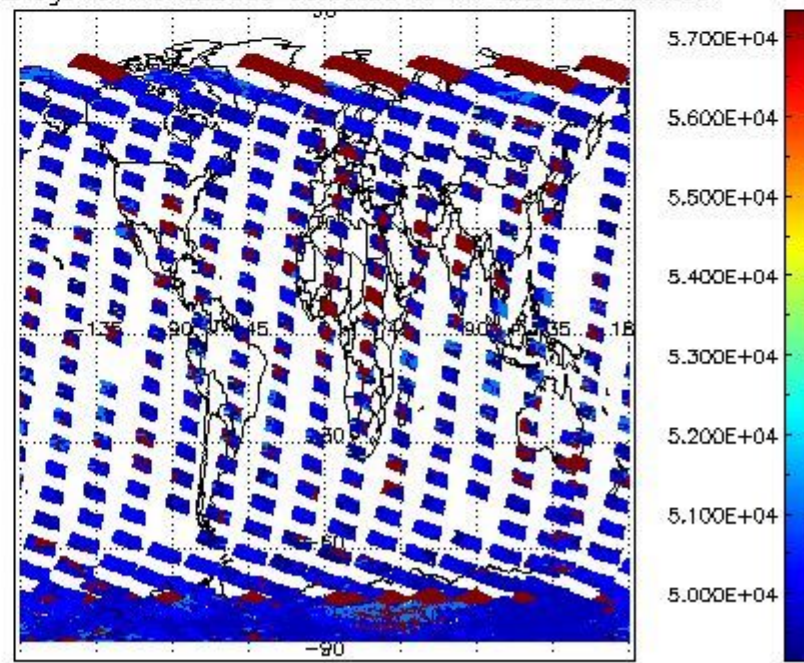
cloud_flags for 10FEB2008 00:00:00 to 11FEB2008 00:00:00
