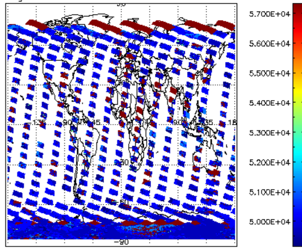
cloud_flags for 10FEB2008 00:00:00 to 11FEB2008 00:00:00
