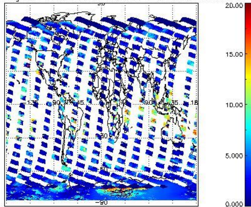
cL_top_height for 10FEB2008 00:00:00 to 11FEB2008 00:00:00
