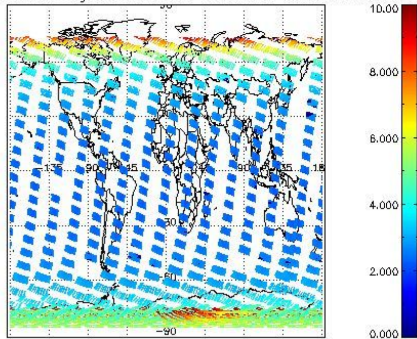
SCIOL2P_NADUV003_amf_gr for 10FEB2008 00:00:00 to 11FEB2008 00:00:00
