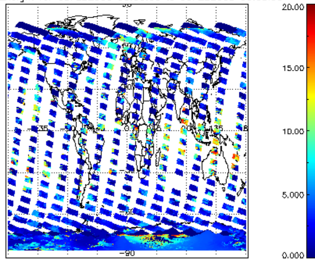
cl_top_height for 08FEB2008 00:00:00 to 09FEB2008 00:00:00
