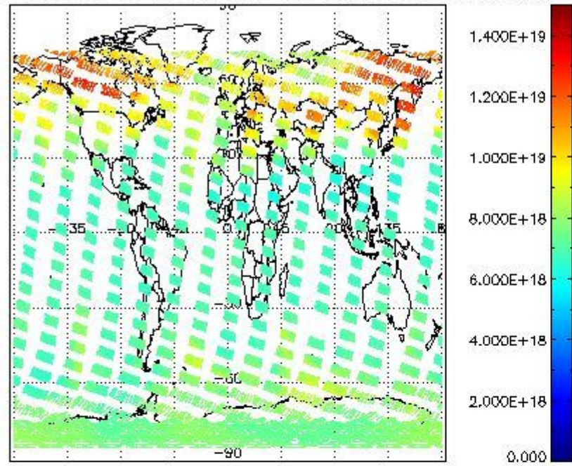
SCIOL2P_NADUV003_vcd for 08FEB2008 00:00:00 to 09FEB2008 00:00:00
