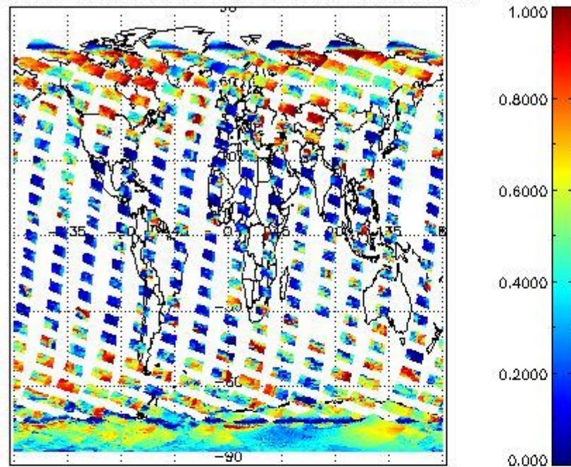
cLfrac for 08FEB2008 00:00:00 to 09FEB2008 00:00:00
