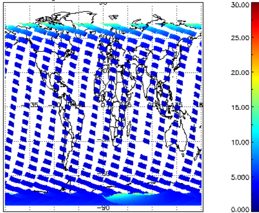
SCIOL2P_NADUV1NO2_amf_gr for 08FEB2008 00:00:00 to 09FEB2008 00:00:00
