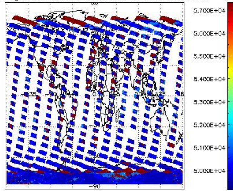
cloud_flags for 08FEB2008 00:00:00 to 09FEB2008 00:00:00
