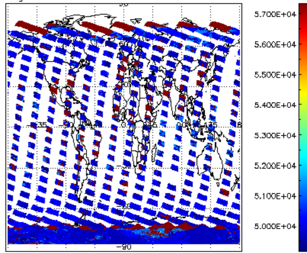
cloud_flags for 08FEB2008 00:00:00 to 09FEB2008 00:00:00
