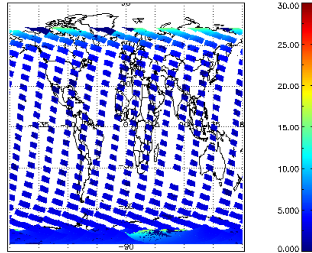
SCIOL2P_NADUV1NO2_amf_cl for 08FEB2008 00:00:00 to 09FEB2008 00:00:00
