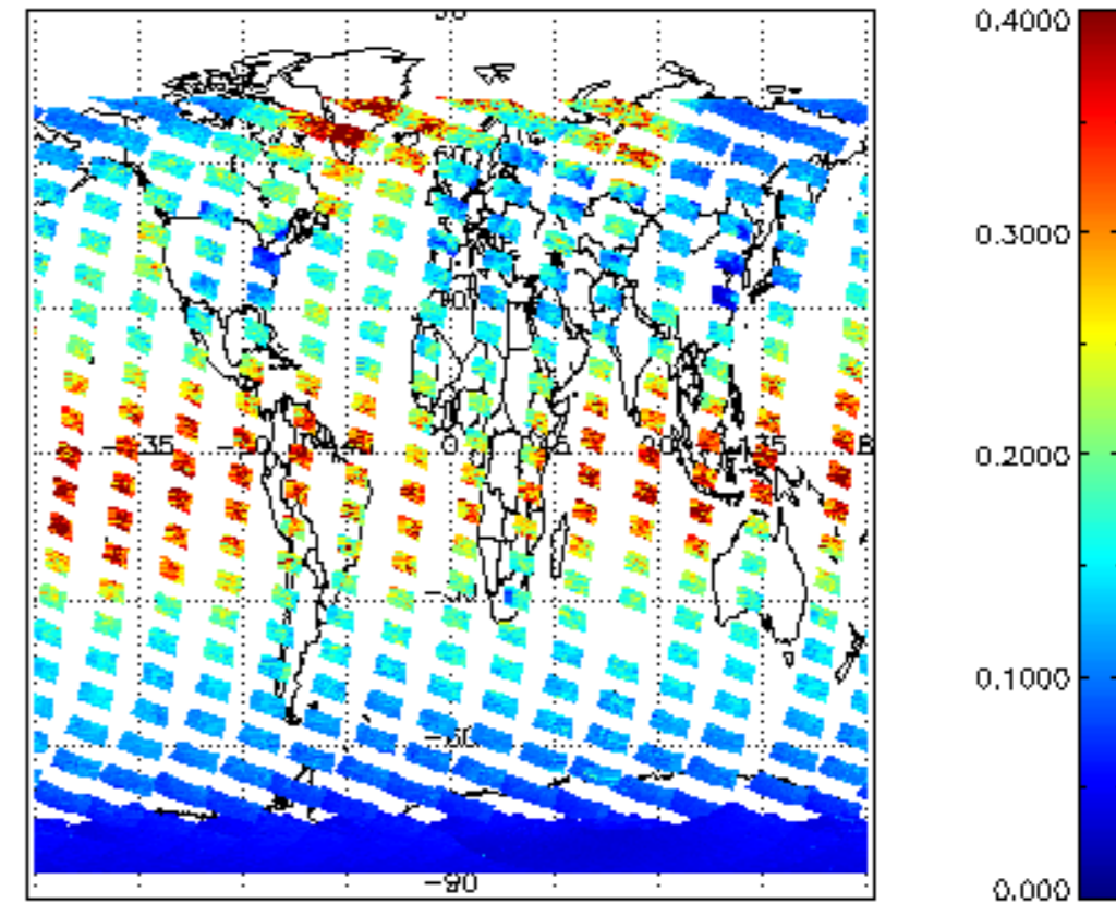
SCIOL2P_NADUV1NO2_vcd_err for 08FEB2008 00:00:00 to 09FEB2008 00:00:00
