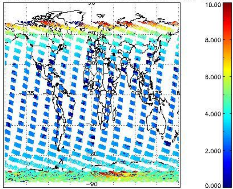
SCIOL2P_NADUV003_amf_cl for 08FEB2008 00:00:00 to 09FEB2008 00:00:00
