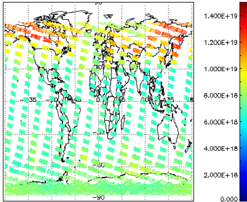
SCIOL2P_NADUV003_vcd for 08FEB2008 00:00:00 to 09FEB2008 00:00:00
