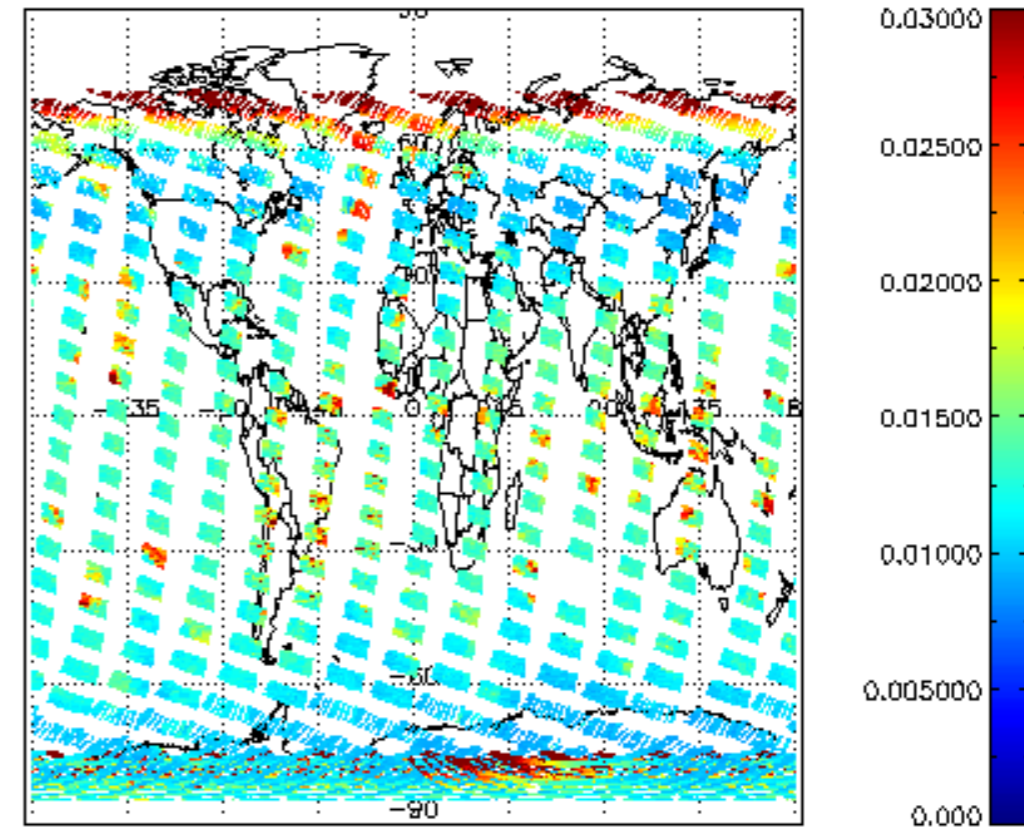
SCIOL2P_NADUV003_vcd_err for 08FEB2008 00:00:00 to 09FEB2008 00:00:00
