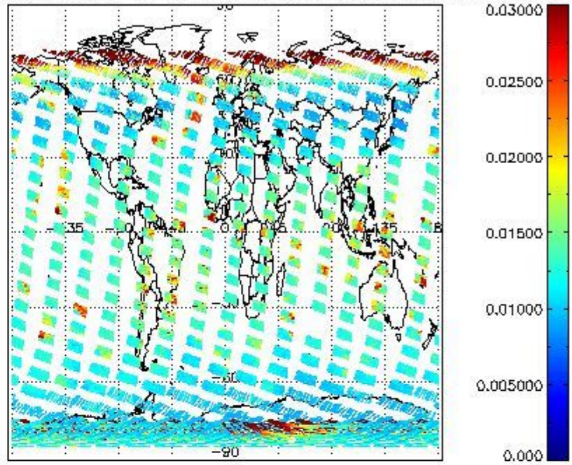
SCIOL2P_NADUV003_vcd_err for 08FEB2008 00:00:00 to 09FEB2008 00:00:00
