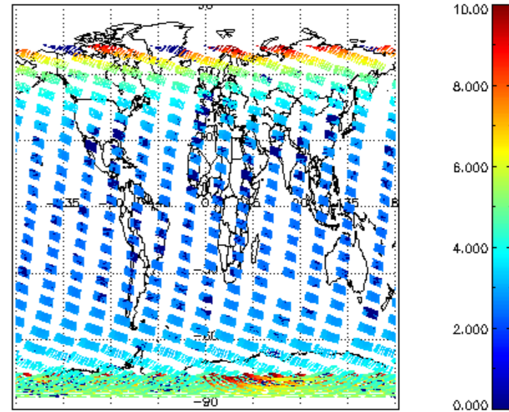
SCIOL2P_NADUV003_amf_cl for 08FEB2008 00:00:00 to 09FEB2008 00:00:00
