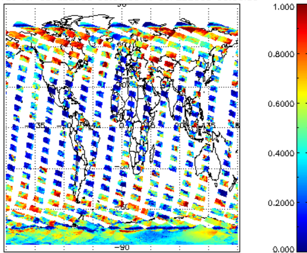
cl_frac for 08FEB2008 00:00:00 to 09FEB2008 00:00:00
