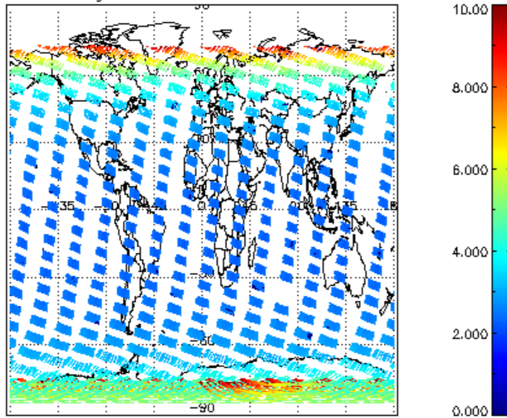
SCIOL2P_NADUV003_amf_gr for 08FEB2008 00:00:00 to 09FEB2008 00:00:00
