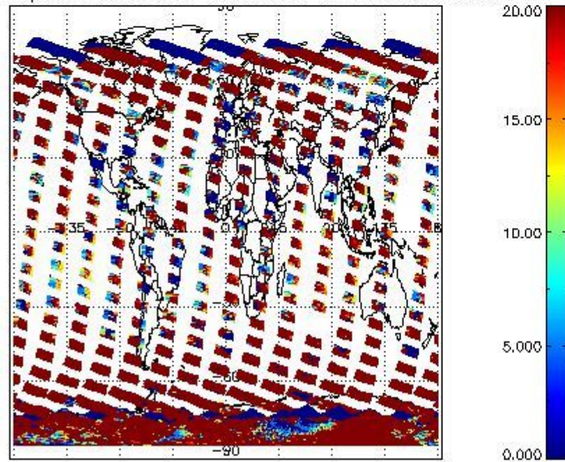
cLopt_depth for 08FEB2008 00:00:00 to 09FEB2008 00:00:00
