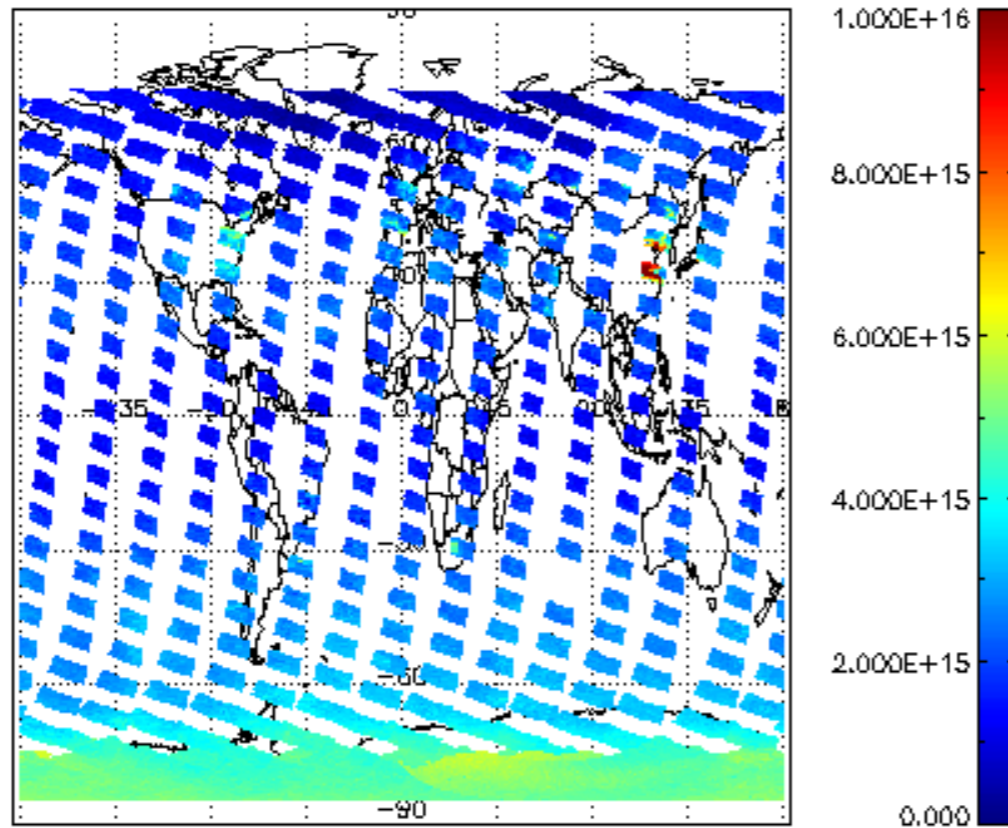
SCIOL2P_NADUV1NO2_vcd for 08FEB2008 00:00:00 to 09FEB2008 00:00:00
