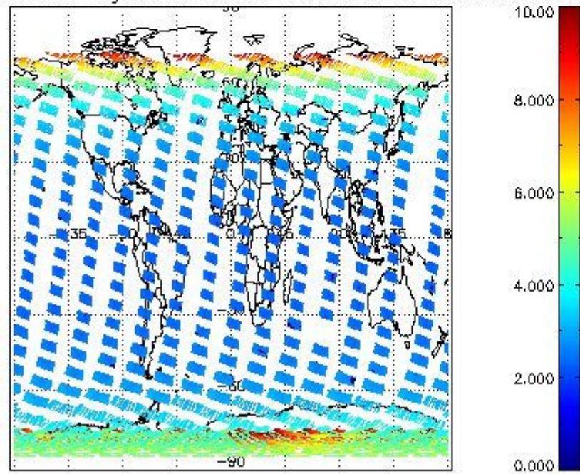
SCIOL2P_NADUV003_amf_gr for 08FEB2008 00:00:00 to 09FEB2008 00:00:00
