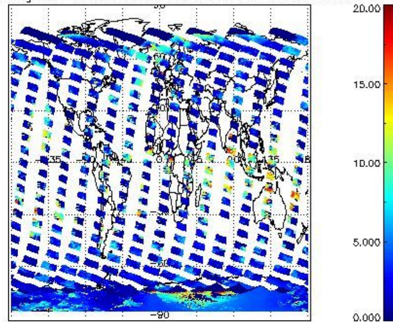
cL_top_height for 08FEB2008 00:00:00 to 09FEB2008 00:00:00
