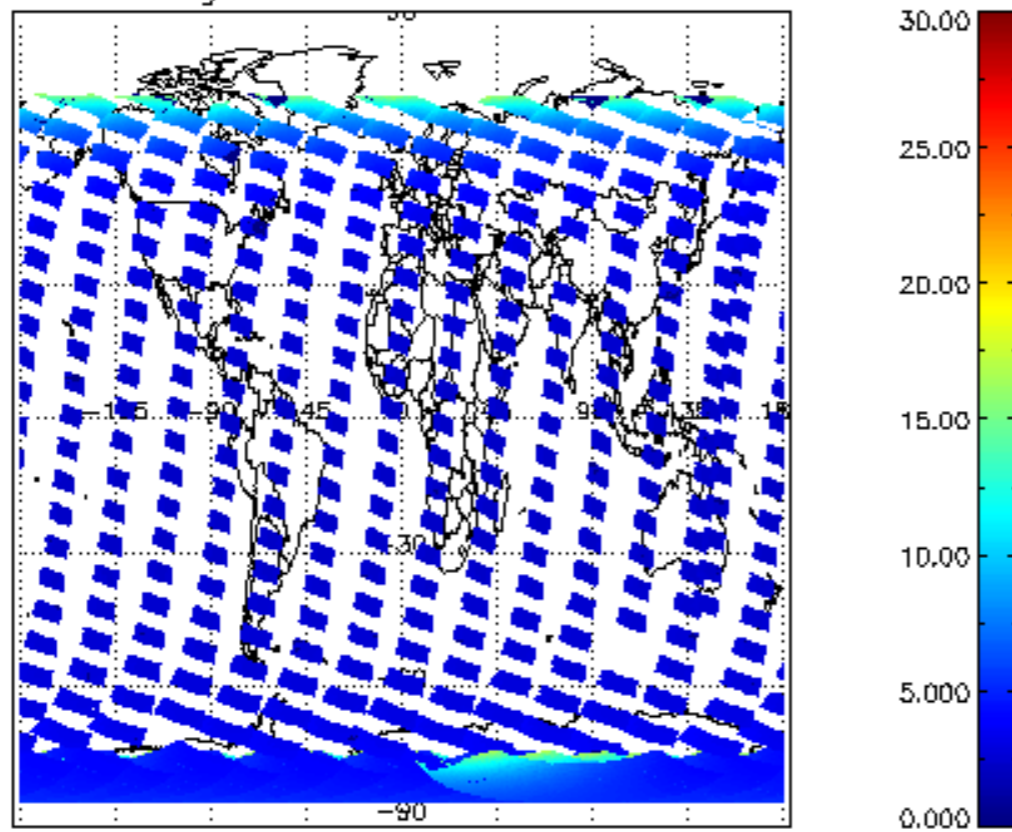
SCIOL2P_NADUV1NO2_amf_gr for 06FEB2008 00:00:00 to 07FEB2008 00:00:00
