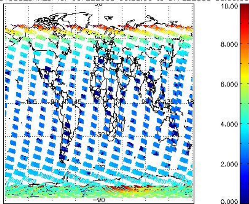
SCIOL2P_NADUV003_amf_cl for 06FEB2008 00:00:00 to 07FEB2008 00:00:00
