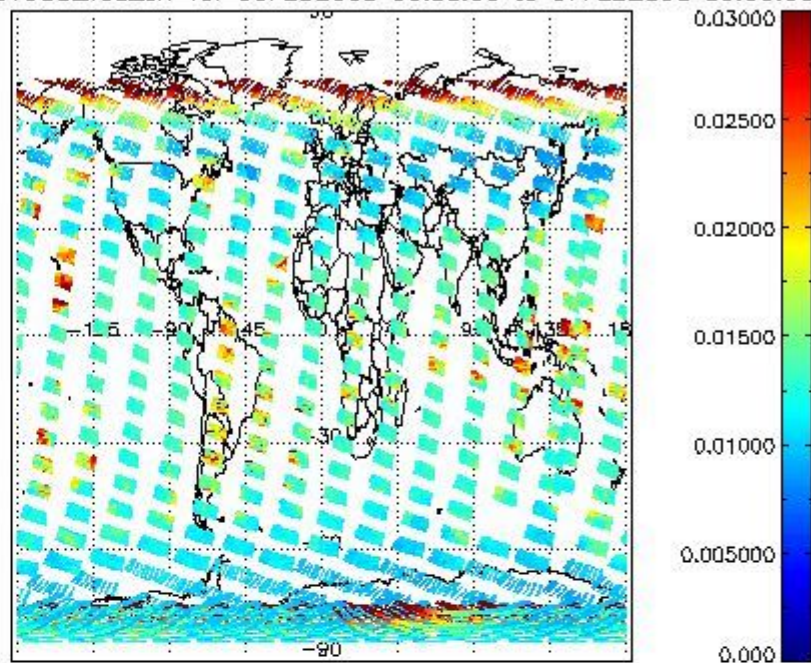
SCIOL2P_NADUV003_vcd_err for 06FEB2008 00:00:00 to 07FEB2008 00:00:00
