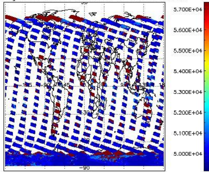
cloud_flags for 06FEB2008 00:00:00 to 07FEB2008 00:00:00
