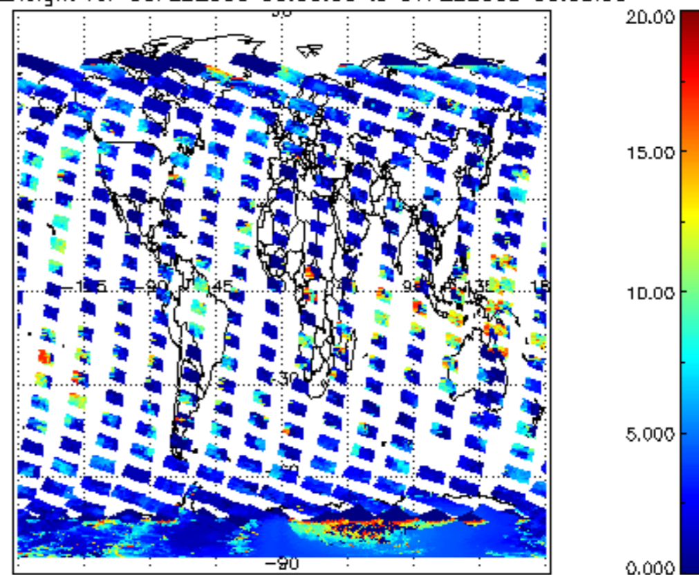
cl_top_height for 06FEB2008 00:00:00 to 07FEB2008 00:00:00
