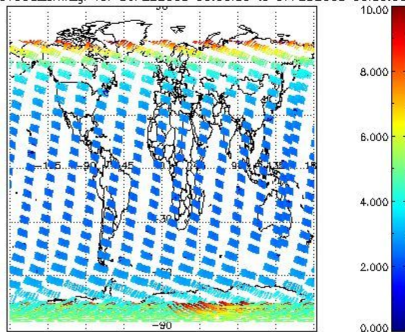
SCIOL2P_NADUV003_amf_gr for 06FEB2008 00:00:00 to 07FEB2008 00:00:00
