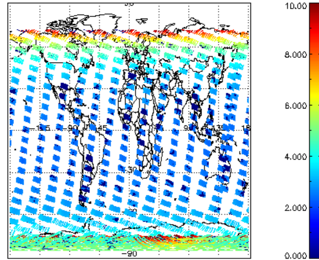
SCIOL2P_NADUV003_amf_cl for 06FEB2008 00:00:00 to 07FEB2008 00:00:00
