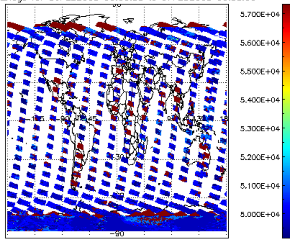
cloud_flags for 06FEB2008 00:00:00 to 07FEB2008 00:00:00
