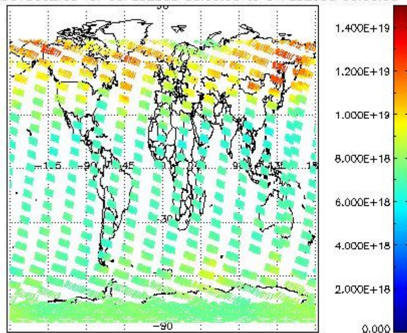
SCIOL2P_NADUV003_vcd for 06FEB2008 00:00:00 to 07FEB2008 00:00:00
