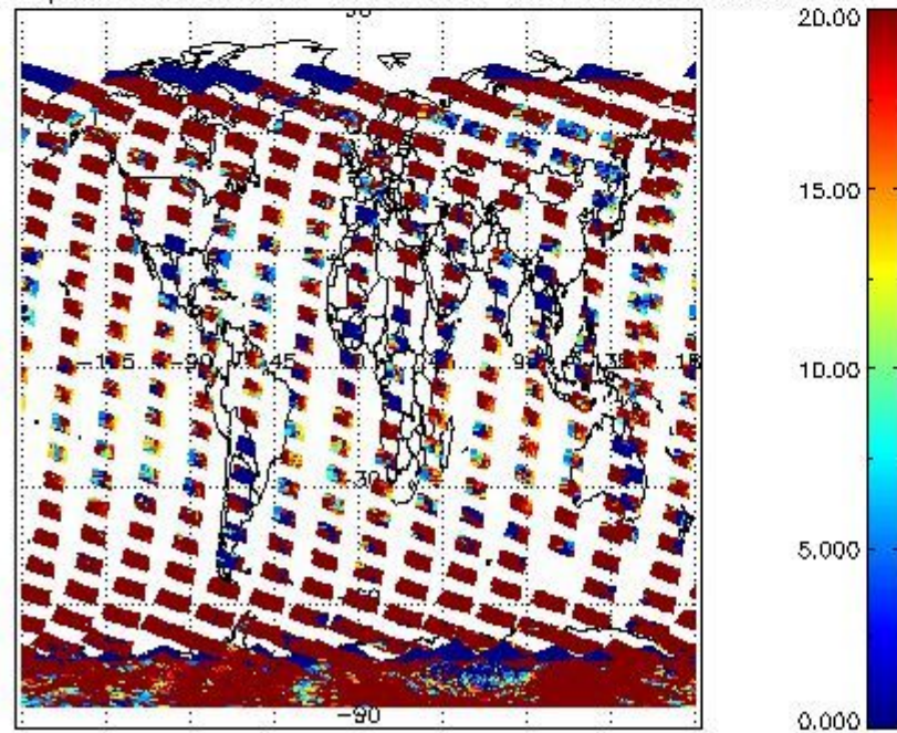
cL_opt_depth for 06FEB2008 00:00:00 to 07FEB2008 00:00:00
