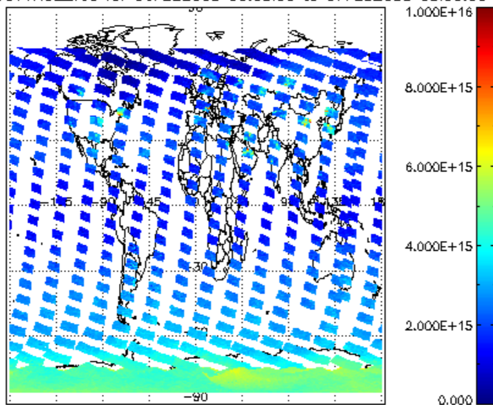
SCIOL2P_NADUV1NO2_vcd for 06FEB2008 00:00:00 to 07FEB2008 00:00:00
