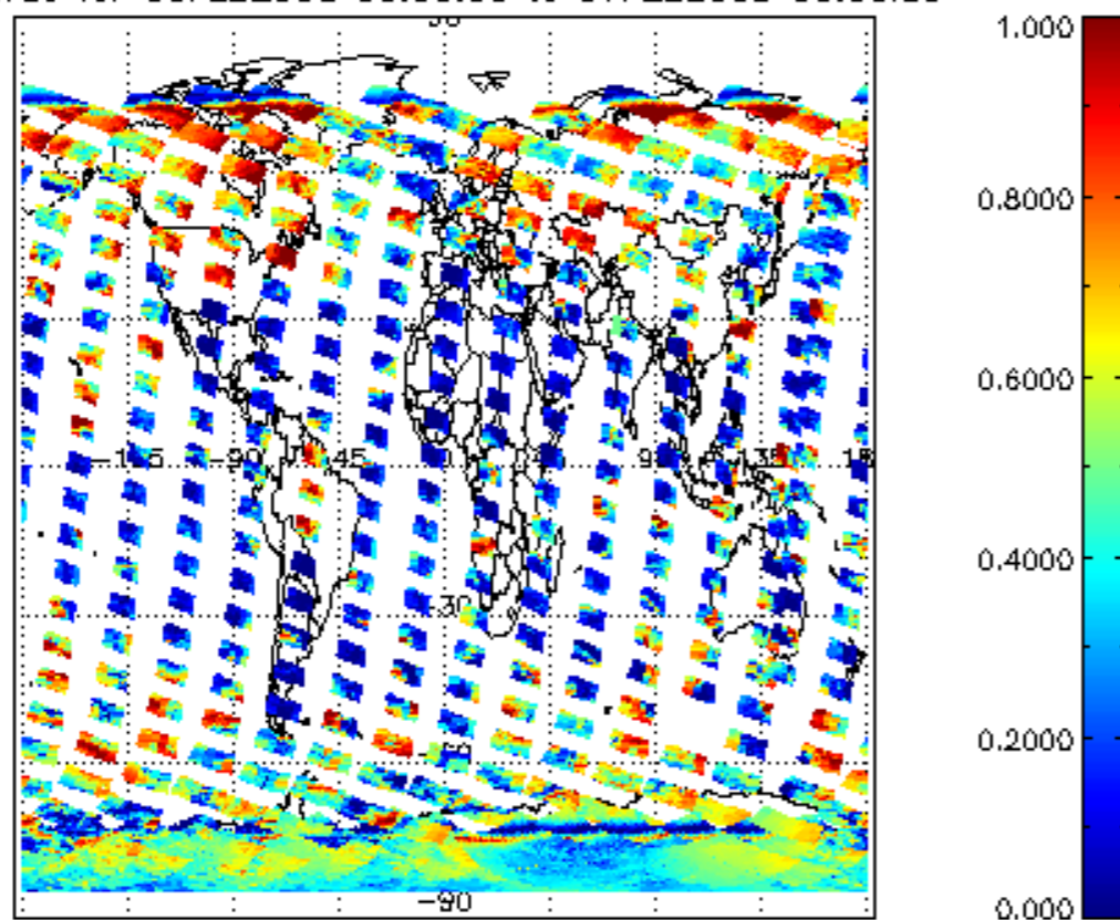
cl_frac for 06FEB2008 00:00:00 to 07FEB2008 00:00:00
