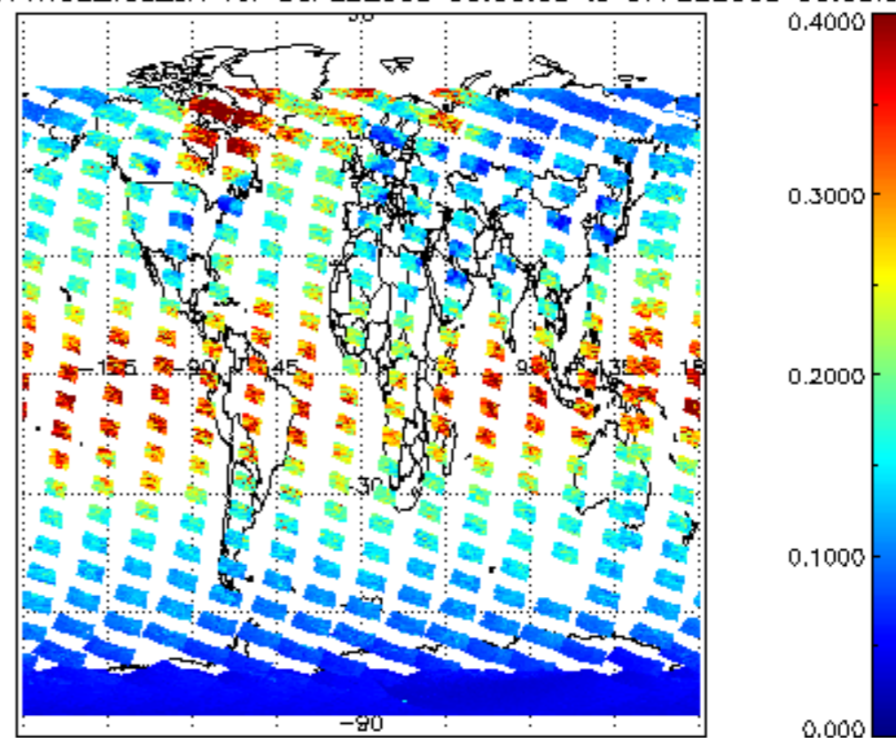
SCIOL2P_NADUV1NO2_vcd_err for 06FEB2008 00:00:00 to 07FEB2008 00:00:00
