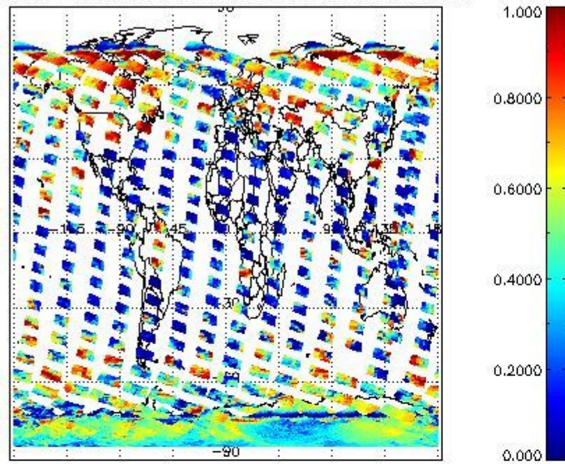
cL_frac for 06FEB2008 00:00:00 to 07FEB2008 00:00:00
