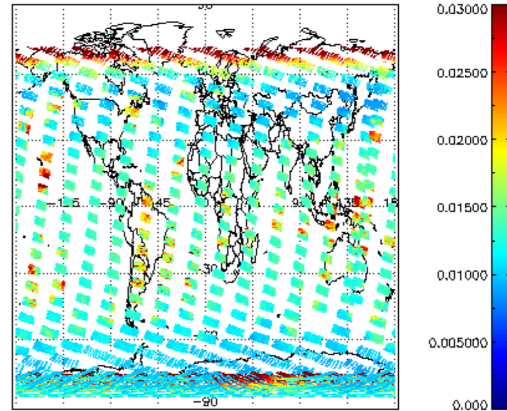
SCIOL2P_NADUV003_vcd_err for 06FEB2008 00:00:00 to 07FEB2008 00:00:00
