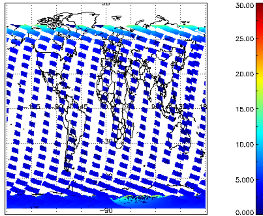
SCIOL2P_NADUV1NO2_amf_cl for 06FEB2008 00:00:00 to 07FEB2008 00:00:00
