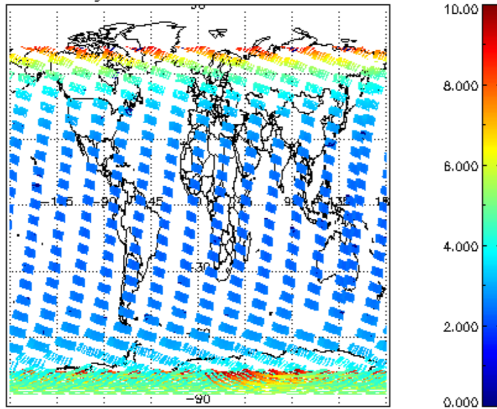
SCIOL2P_NADUV003_amf_gr for 06FEB2008 00:00:00 to 07FEB2008 00:00:00
