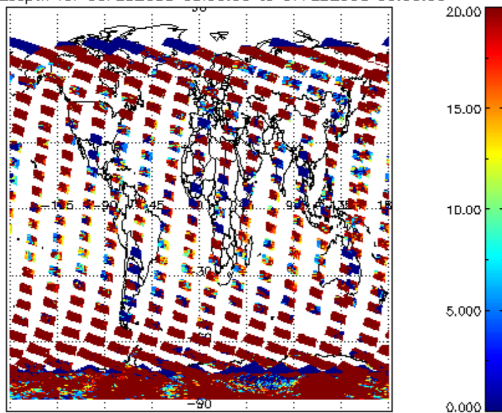
cl_opt_depth for 06FEB2008 00:00:00 to 07FEB2008 00:00:00
