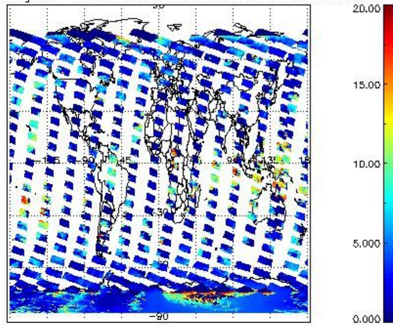
cL_top_height for 06FEB2008 00:00:00 to 07FEB2008 00:00:00
