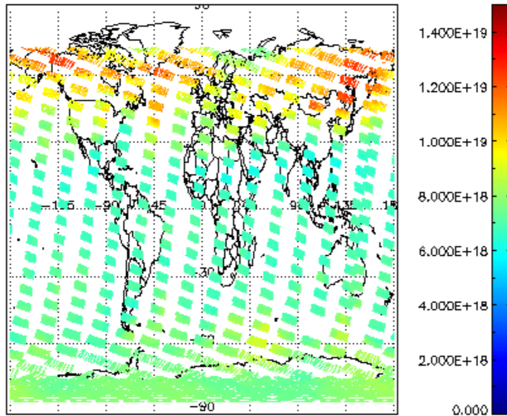
SCIOL2P_NADUV003_vcd for 06FEB2008 00:00:00 to 07FEB2008 00:00:00
