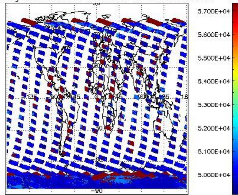
cloud_flags for 04FEB2008 00:00:00 to 05FEB2008 00:00:00
