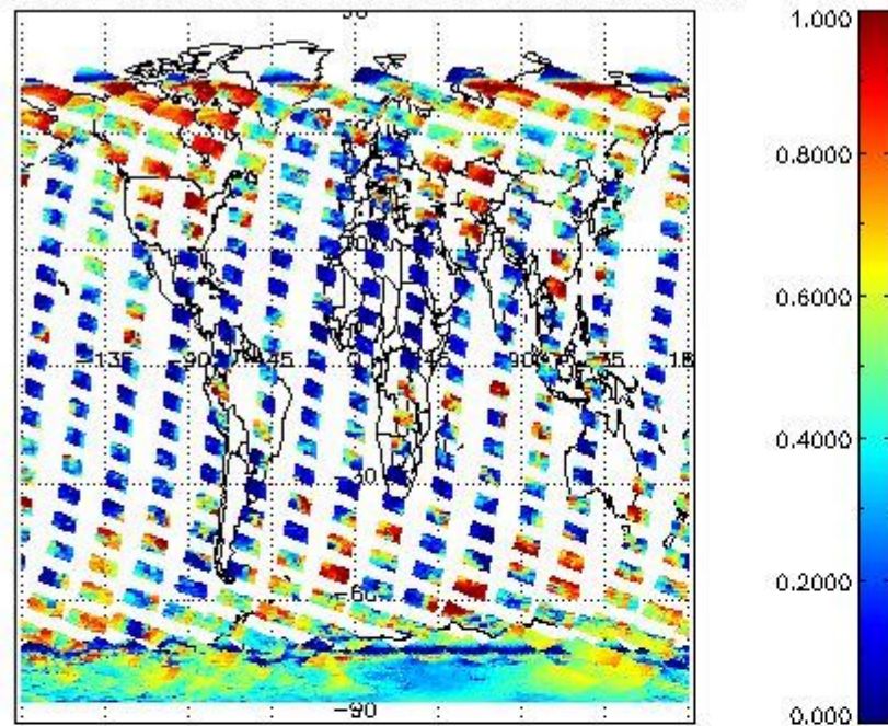
cLfrac for 04FEB2008 00:00:00 to 05FEB2008 00:00:00
