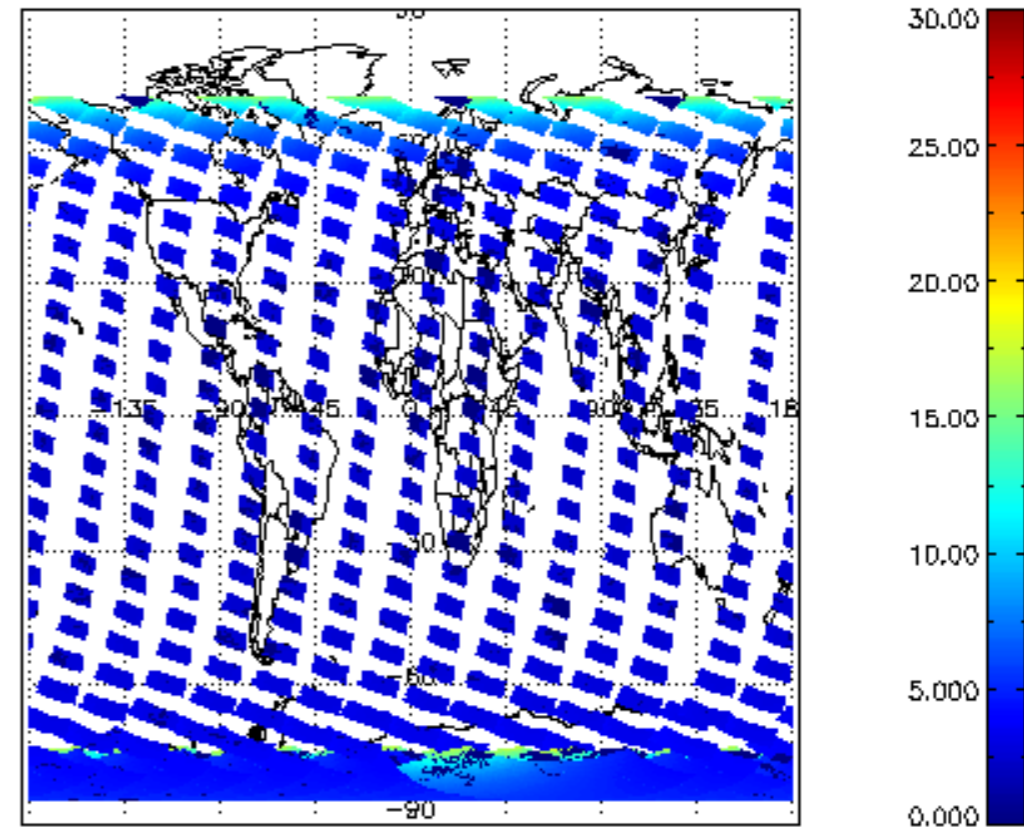
SCIOL2P_NADUV1NO2_amf_cl for 04FEB2008 00:00:00 to 05FEB2008 00:00:00
