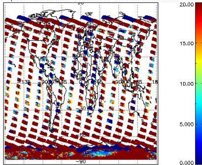
cLopt_depth for 04FEB2008 00:00:00 to 05FEB2008 00:00:00
