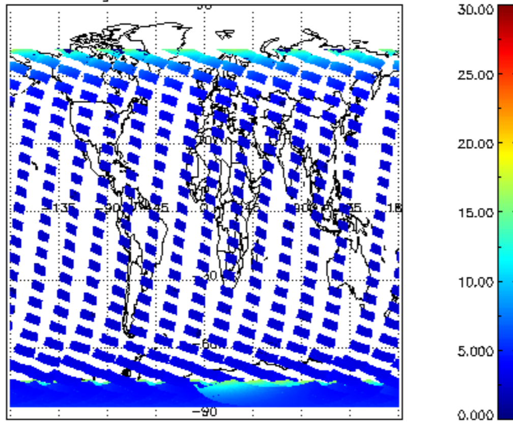
SCIOL2P_NADUV1NO2_amf_gr for 04FEB2008 00:00:00 to 05FEB2008 00:00:00
