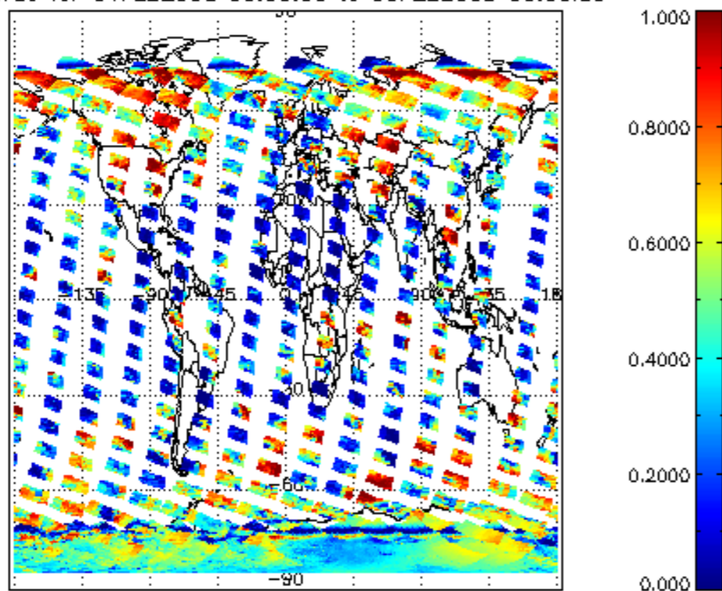
cl_frac for 04FEB2008 00:00:00 to 05FEB2008 00:00:00
