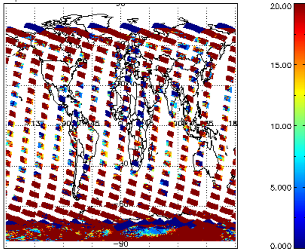
cl_opt_depth for 04FEB2008 00:00:00 to 05FEB2008 00:00:00
