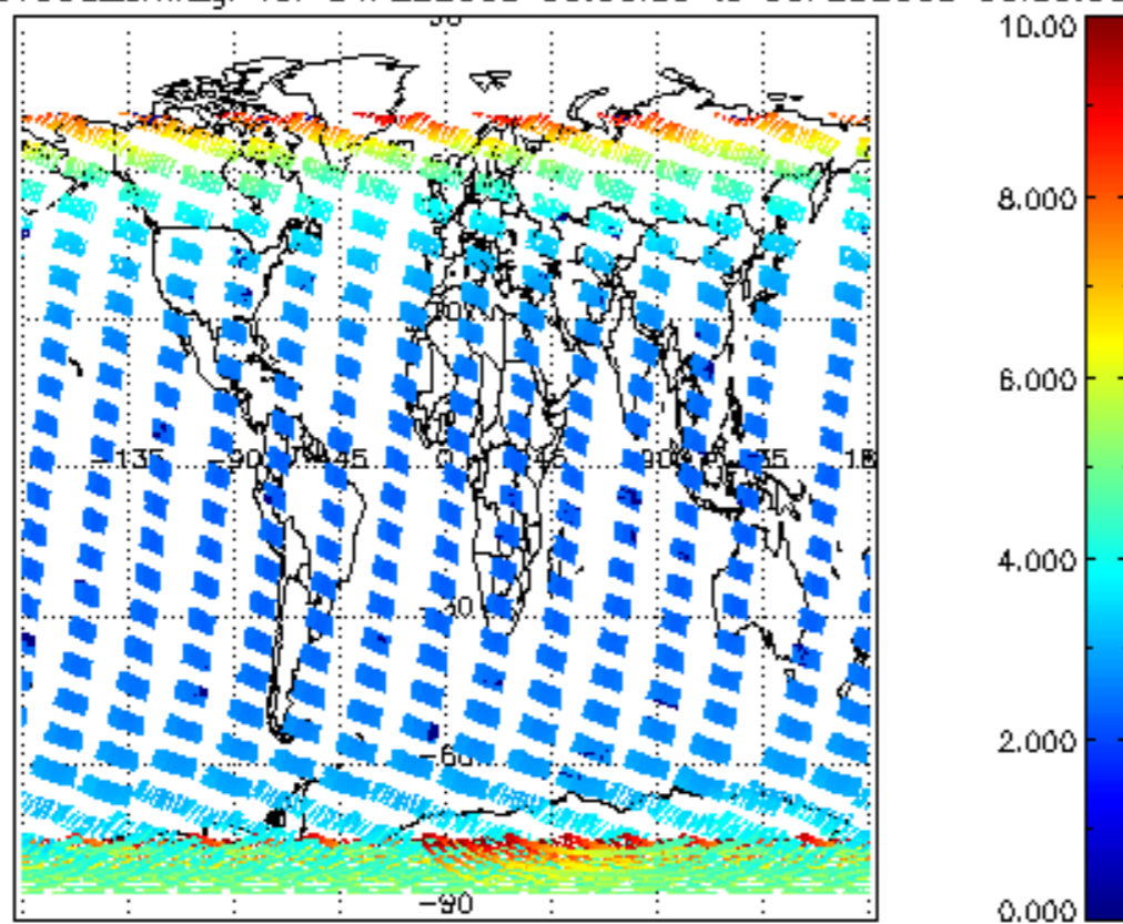
SCIOL2P_NADUV003_amf_gr for 04FEB2008 00:00:00 to 05FEB2008 00:00:00
