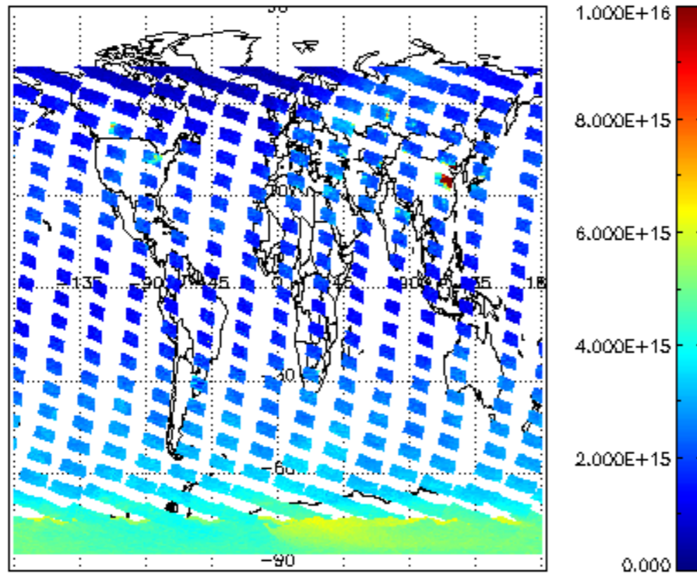
SCIOL2P_NADUV1NO2_vcd for 04FEB2008 00:00:00 to 05FEB2008 00:00:00
