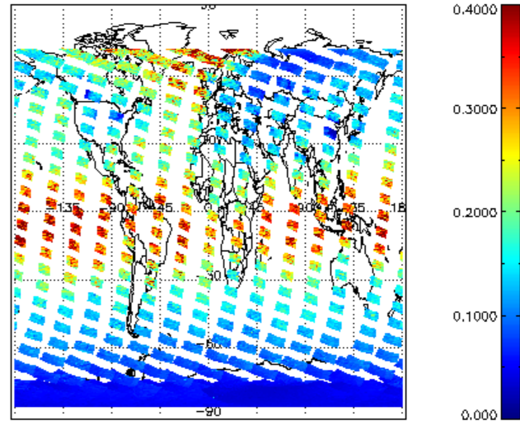
SCIOL2P_NADUV1NO2_vcd_err for 04FEB2008 00:00:00 to 05FEB2008 00:00:00
