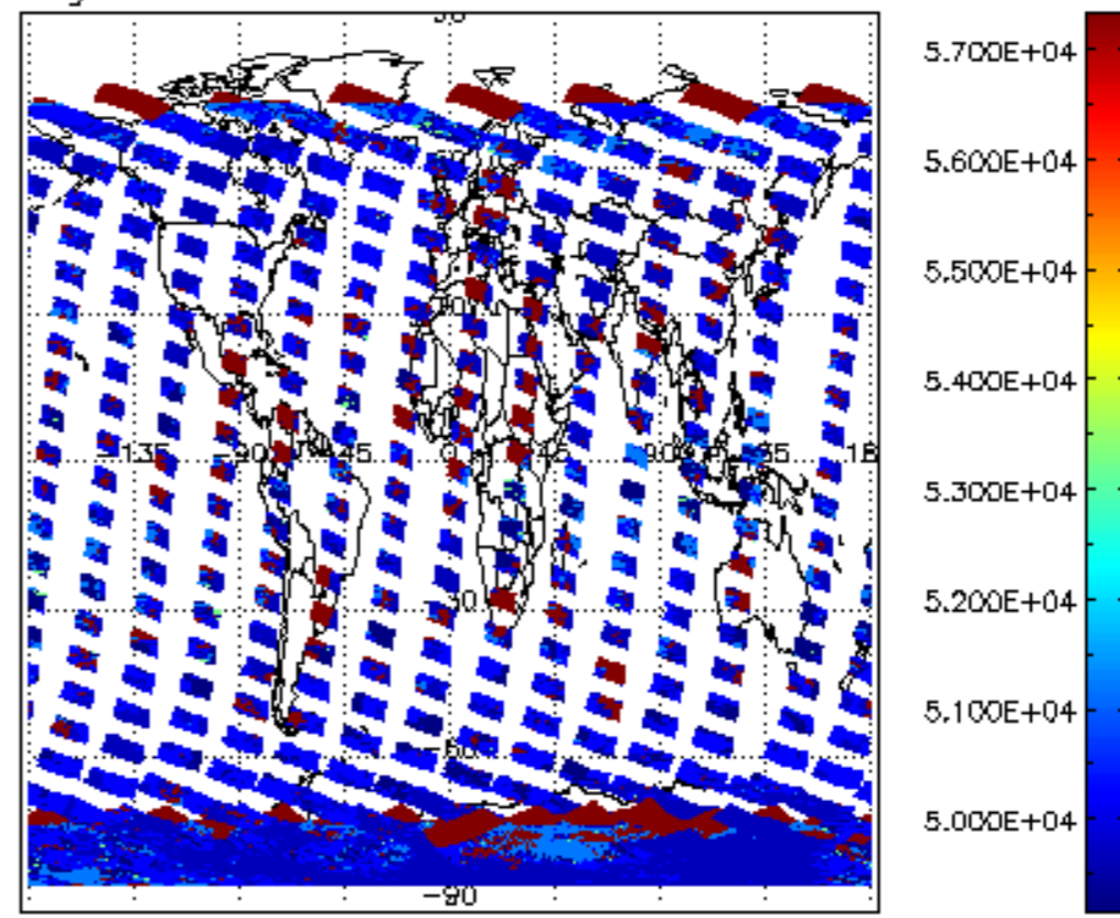
cloud_flags for 04FEB2008 00:00:00 to 05FEB2008 00:00:00
