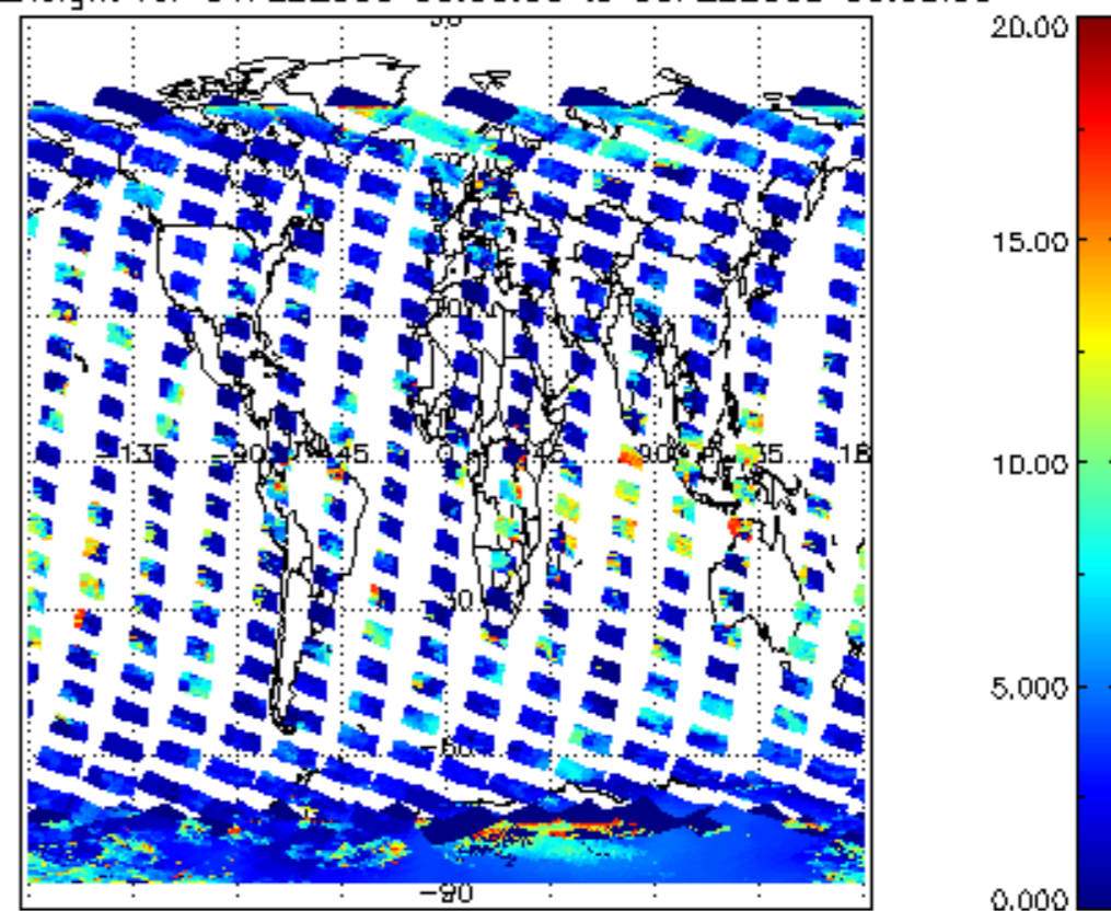
cl_top_height for 04FEB2008 00:00:00 to 05FEB2008 00:00:00
