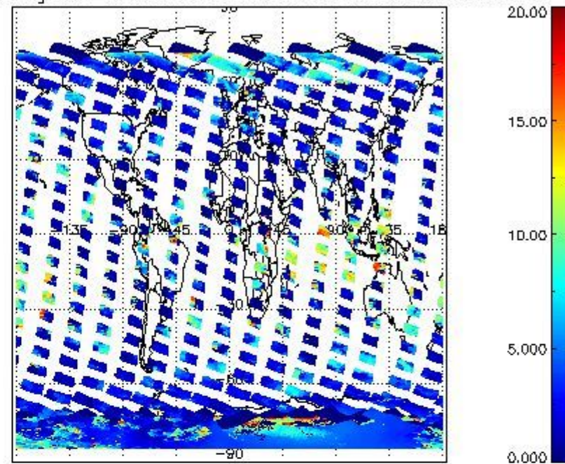
cL_top_height for 04FEB2008 00:00:00 to 05FEB2008 00:00:00
