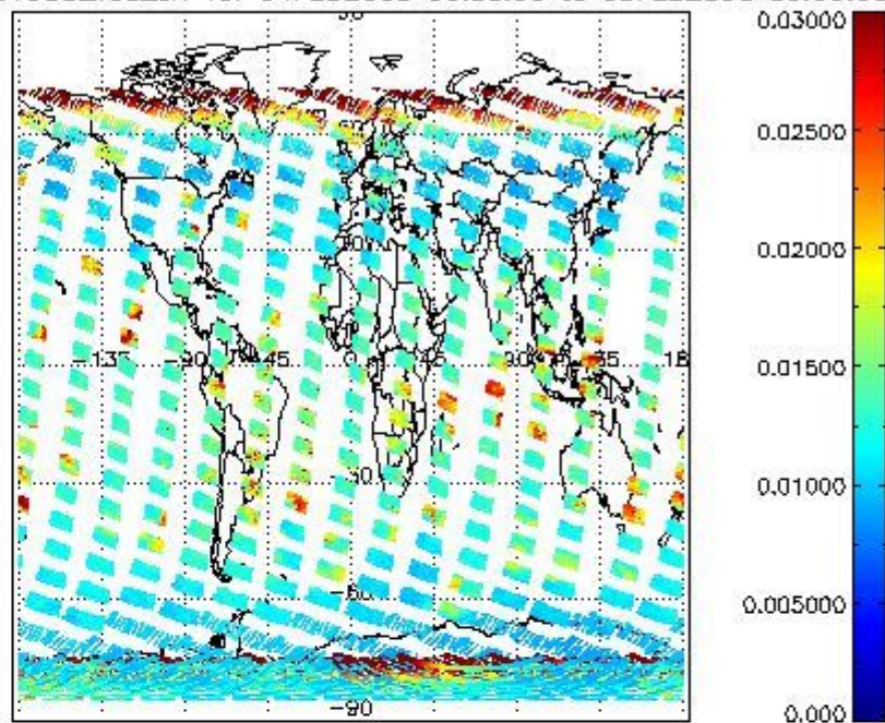
SCIOL2P_NADUV003_vcd_err for 04FEB2008 00:00:00 to 05FEB2008 00:00:00
