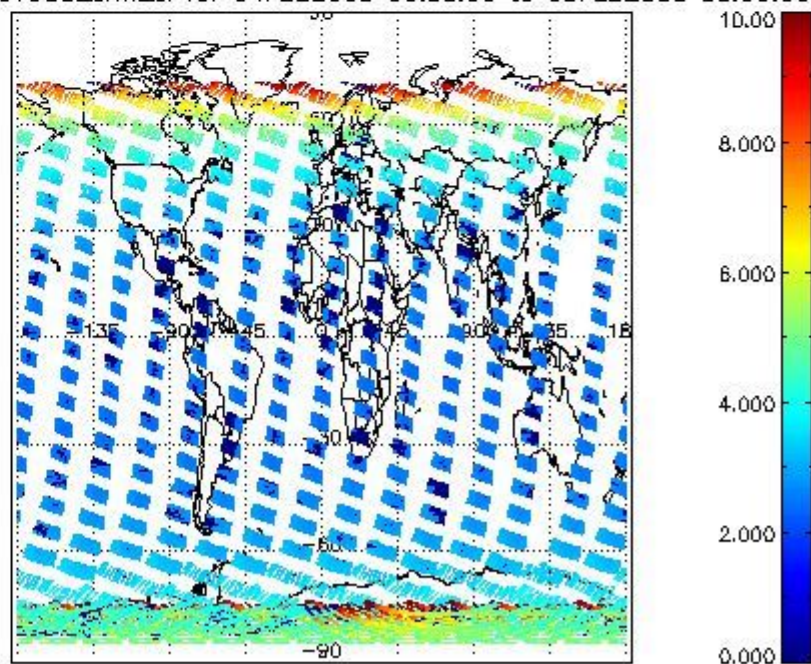
SCIOL2P_NADUV003_amf_sl for 04FEB2008 00:00:00 to 05FEB2008 00:00:00
