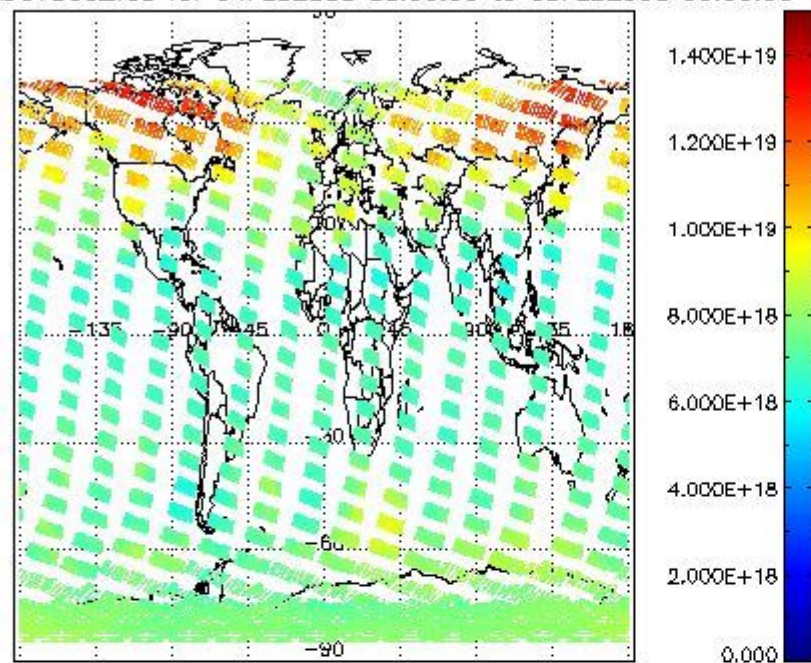
SCIOL2P_NADUV003_vcd for 04FEB2008 00:00:00 to 05FEB2008 00:00:00
