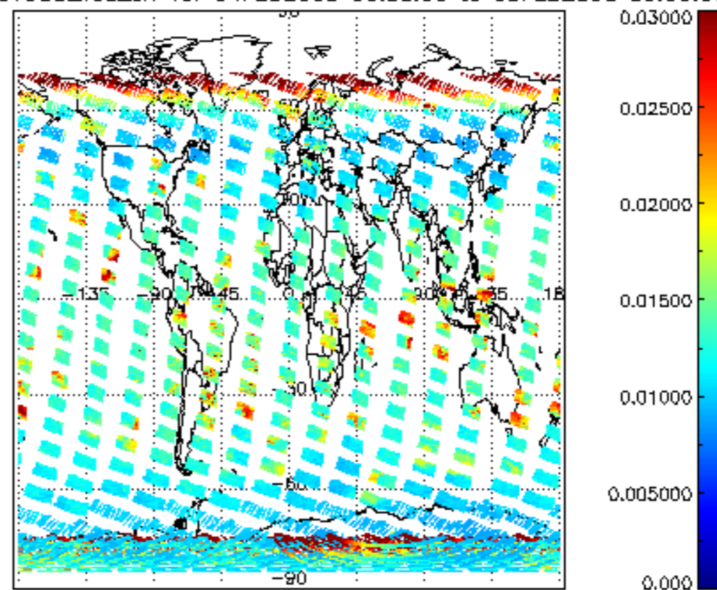
SCIOL2P_NADUV003_vcd_err for 04FEB2008 00:00:00 to 05FEB2008 00:00:00
