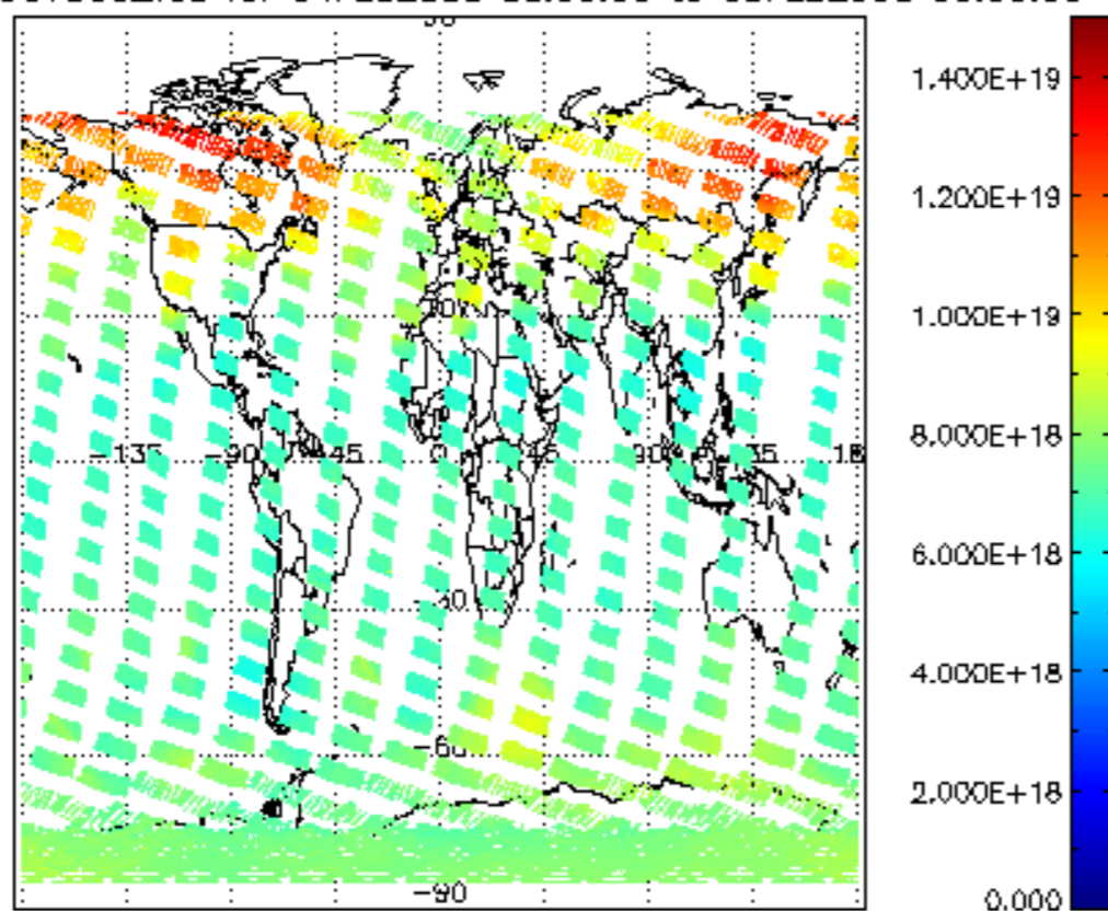
SCIOL2P_NADUV003_vcd for 04FEB2008 00:00:00 to 05FEB2008 00:00:00
