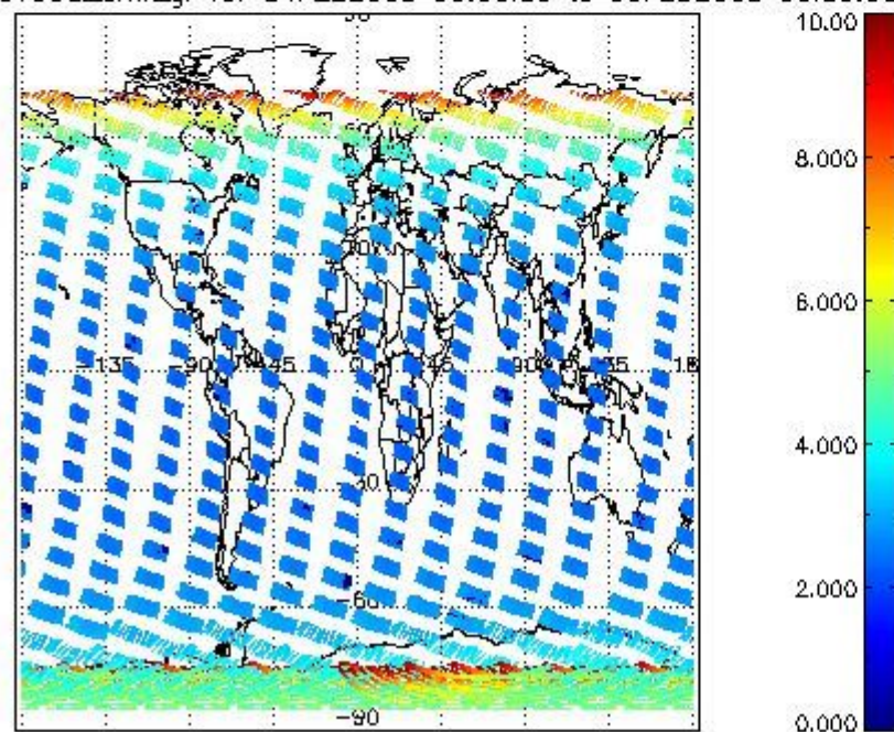
SCIOL2P_NADUV003_amf_gr for 04FEB2008 00:00:00 to 05FEB2008 00:00:00
