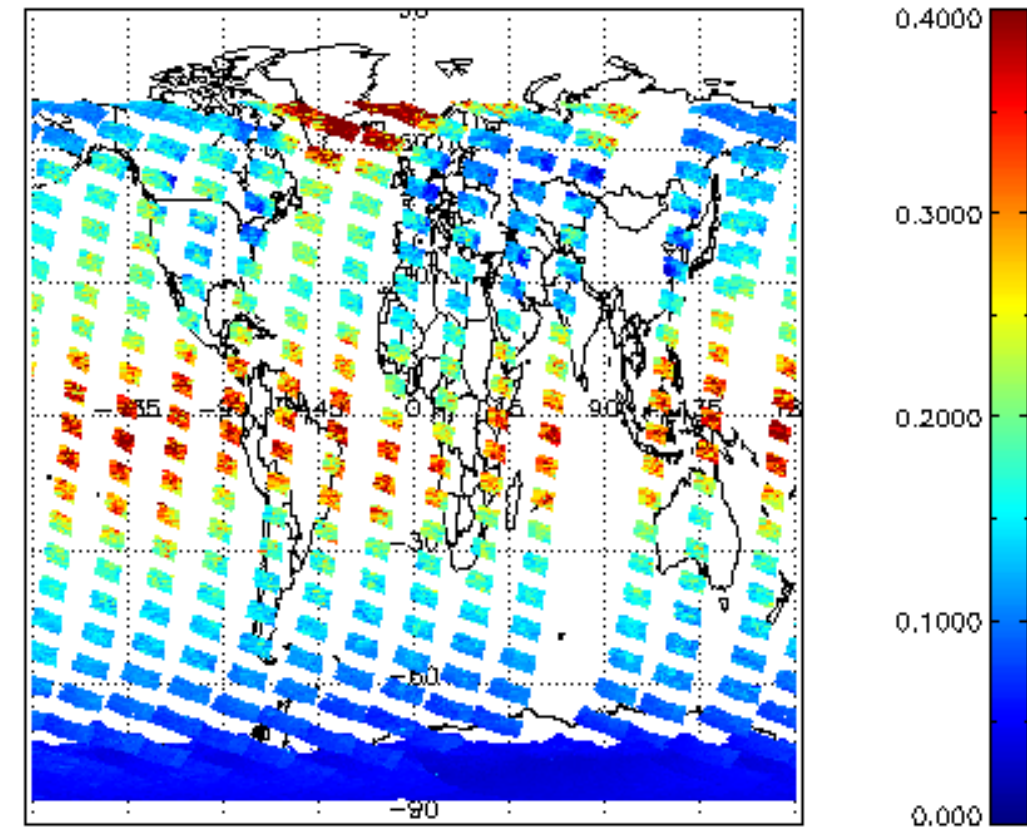
SCIOL2P_NADUV1NO2_vcd_err for 30JAN2008 00:00:00 to 31JAN2008 00:00:00
