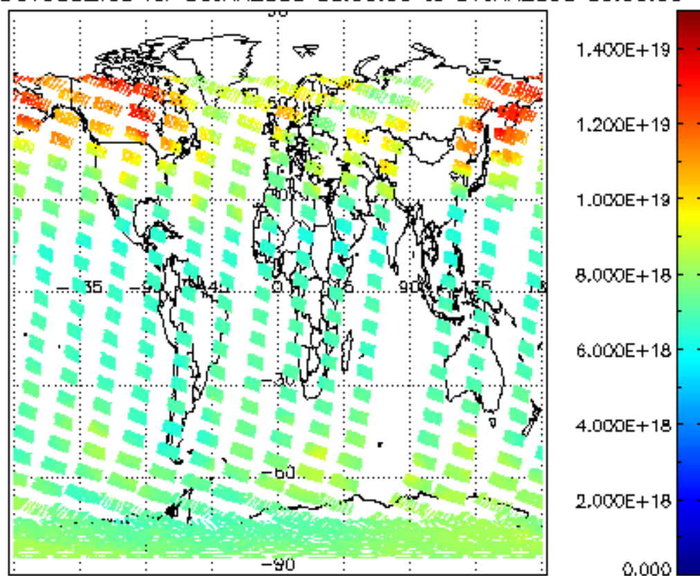
SCIOL2P_NADUV003_vcd for 30JAN2008 00:00:00 to 31JAN2008 00:00:00
