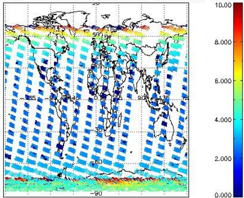
SCIOL2P_NADUV003_amf_cl for 30JAN2008 00:00:00 to 31JAN2008 00:00:00
