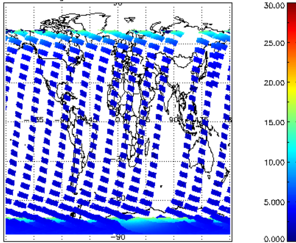
SCIOL2P_NADUV1NO2_amf_gr for 30JAN2008 00:00:00 to 31JAN2008 00:00:00
