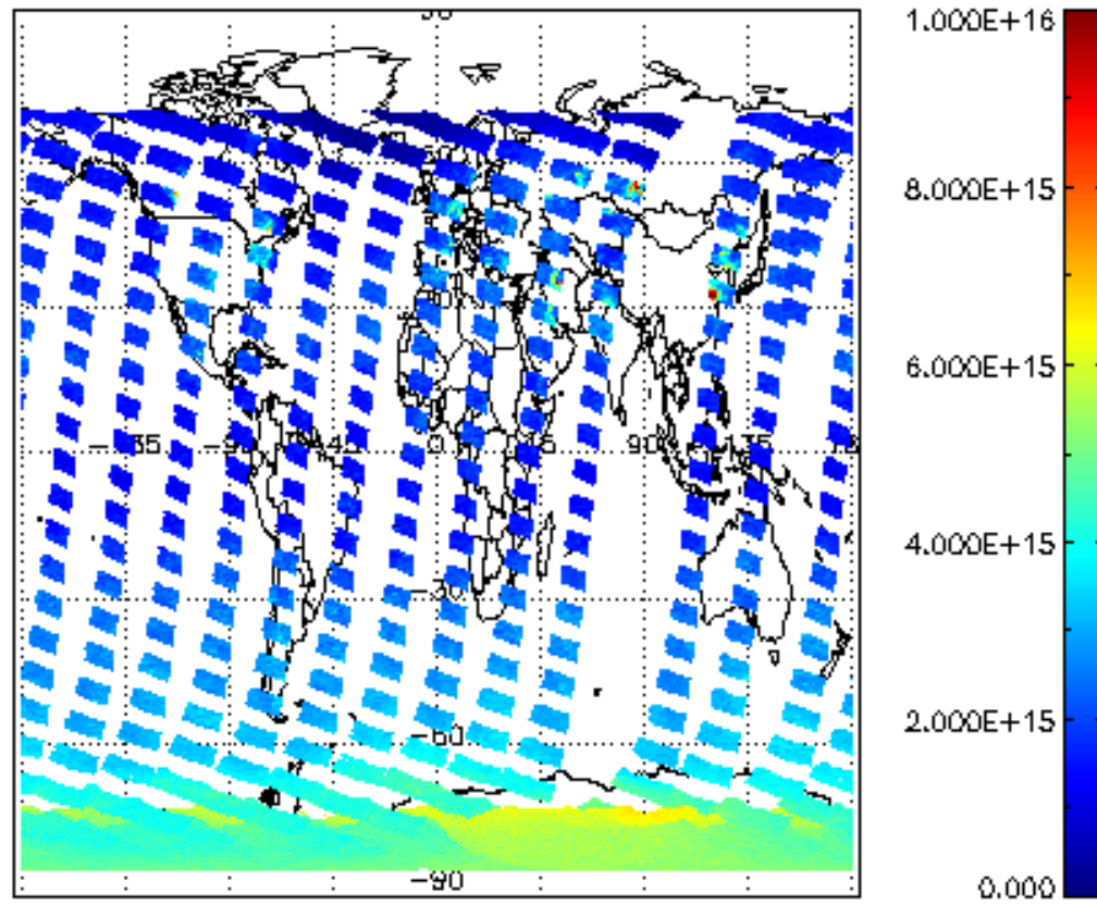
SCIOL2P_NADUV1NO2_vcd for 30JAN2008 00:00:00 to 31JAN2008 00:00:00
