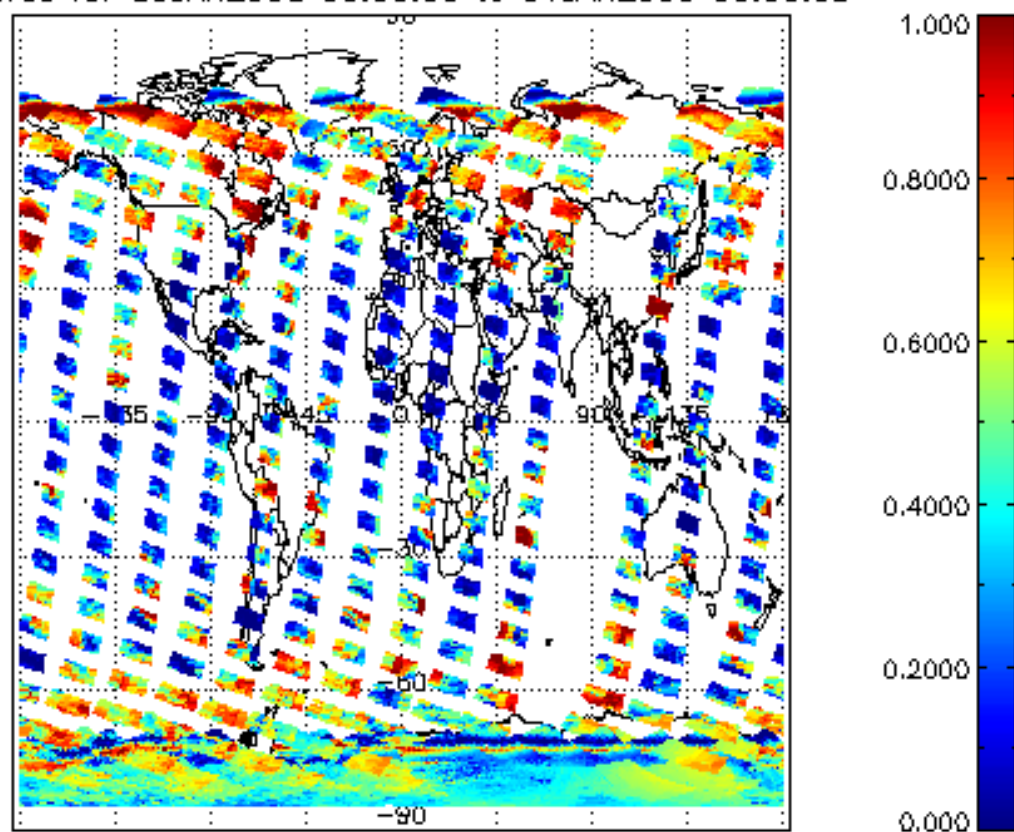
cL_frac for 30JAN2008 00:00:00 to 31JAN2008 00:00:00
