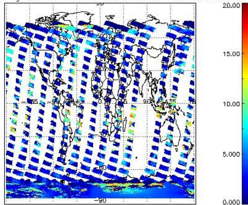
cL_top_height for 30JAN2008 00:00:00 to 31JAN2008 00:00:00
