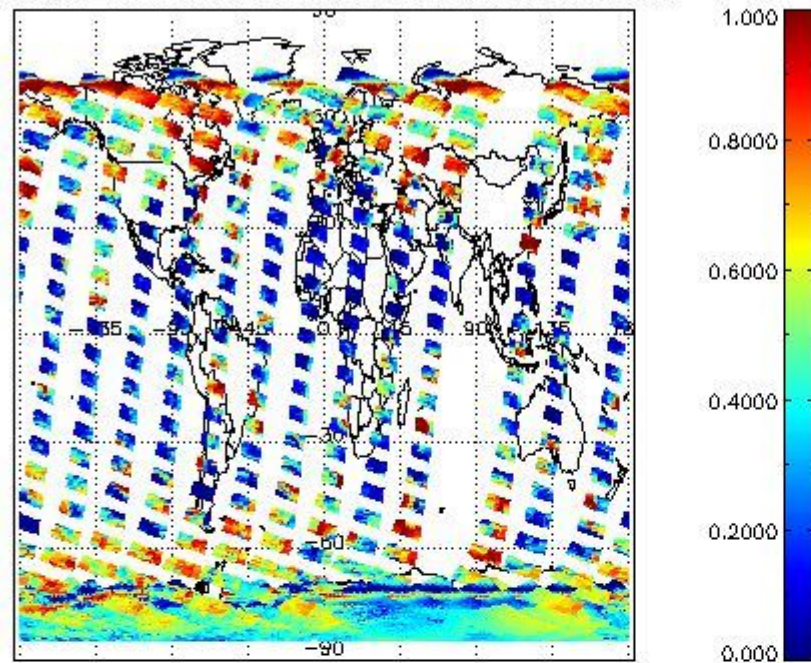
cL_frac for 30JAN2008 00:00:00 to 31JAN2008 00:00:00
