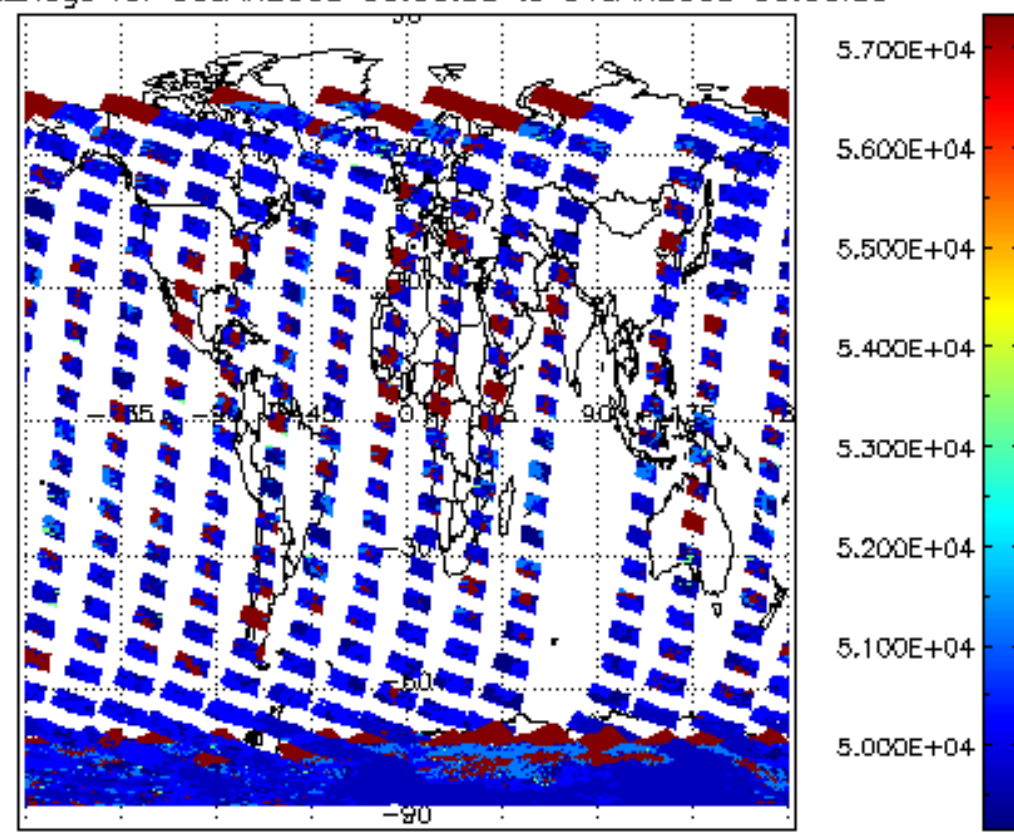
cloud_flags for 30JAN2008 00:00:00 to 31JAN2008 00:00:00
