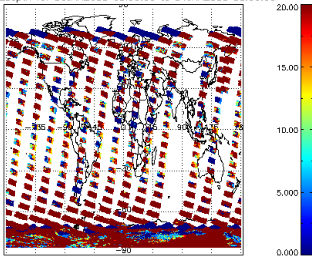
cLopt_depth for 30JAN2008 00:00:00 to 31JAN2008 00:00:00
