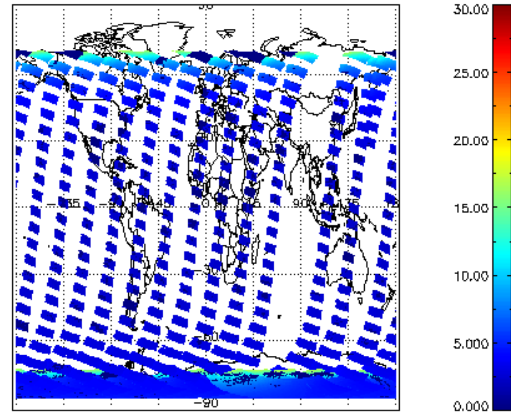
SCIOL2P_NADUV1NO2_amf_cl for 30JAN2008 00:00:00 to 31JAN2008 00:00:00
