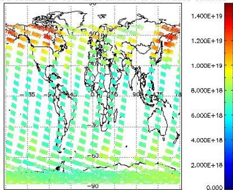
SCIOL2P_NADUV003_vcd for 30JAN2008 00:00:00 to 31JAN2008 00:00:00
