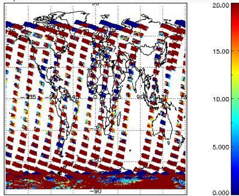
cLopt_depth for 30JAN2008 00:00:00 to 31JAN2008 00:00:00
