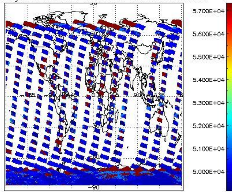
cloud_flags for 30JAN2008 00:00:00 to 31JAN2008 00:00:00
