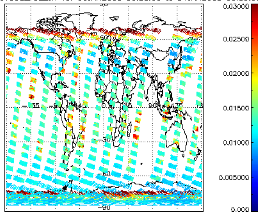
SCIOL2P_NADUV003_vcd_err for 30JAN2008 00:00:00 to 31JAN2008 00:00:00
