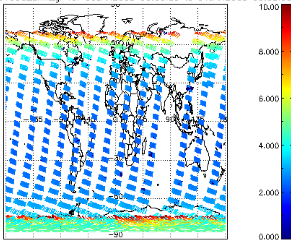
SCIOL2P_NADUV003_amf_gr for 30JAN2008 00:00:00 to 31JAN2008 00:00:00
