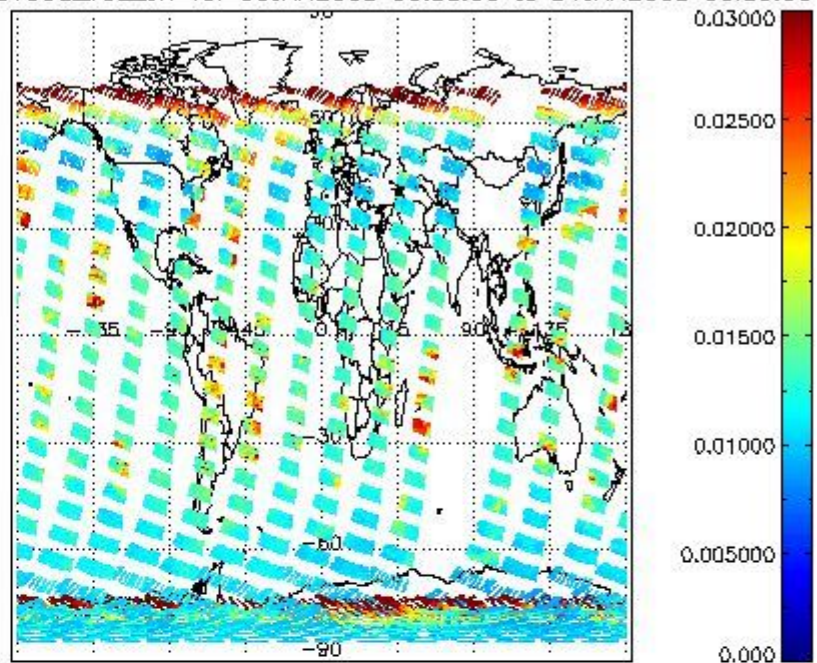
SCIOL2P_NADUV003_vcd_err for 30JAN2008 00:00:00 to 31JAN2008 00:00:00
