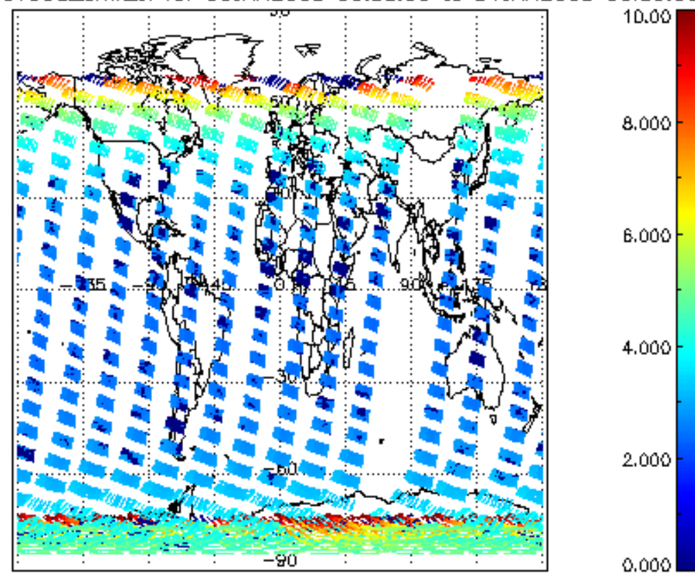
SCIOL2P_NADUV003_amf_cl for 30JAN2008 00:00:00 to 31JAN2008 00:00:00
