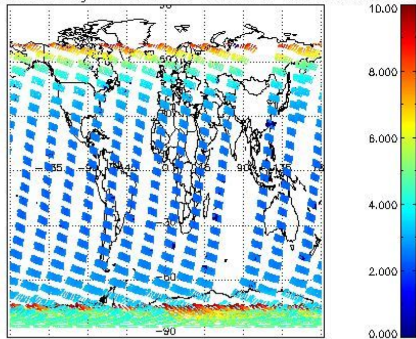
SCIOL2P_NADUV003_amf_gr for 30JAN2008 00:00:00 to 31JAN2008 00:00:00
