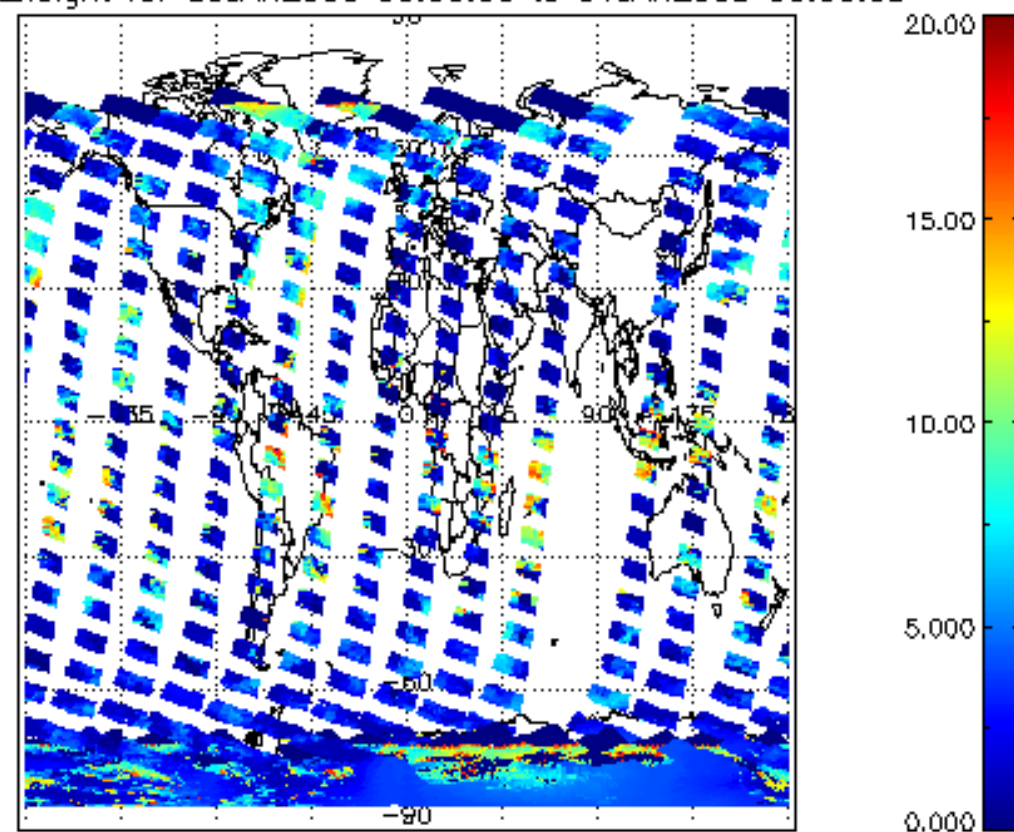
cL_top_height for 30JAN2008 00:00:00 to 31JAN2008 00:00:00
