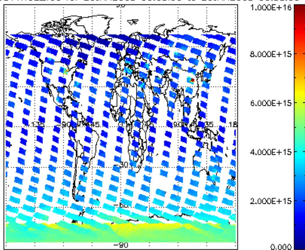
SCIOL2P_NADUV1NO2_vcd for 25JAN2008 00:00:00 to 26JAN2008 00:00:00
