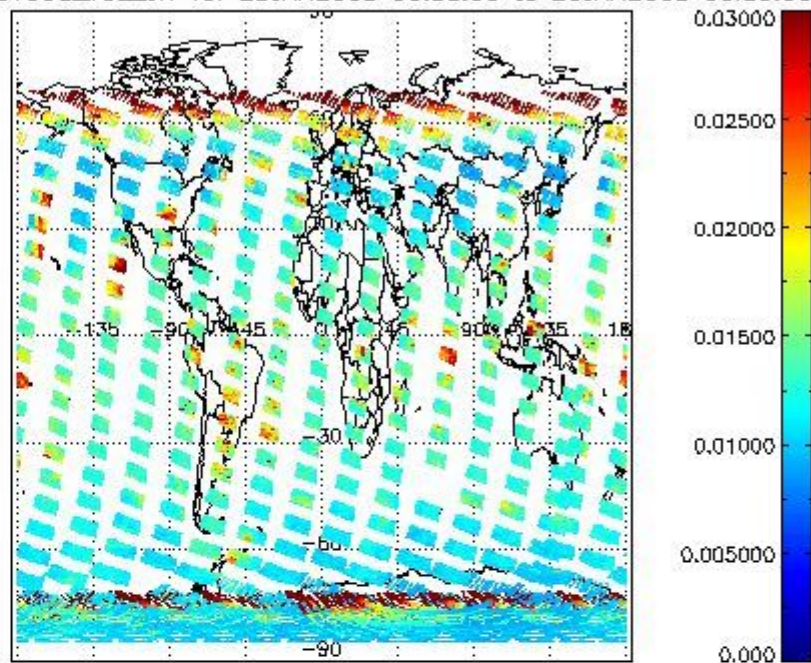
SCIOL2P_NADUV003_vcd_err for 25JAN2008 00:00:00 to 26JAN2008 00:00:00
