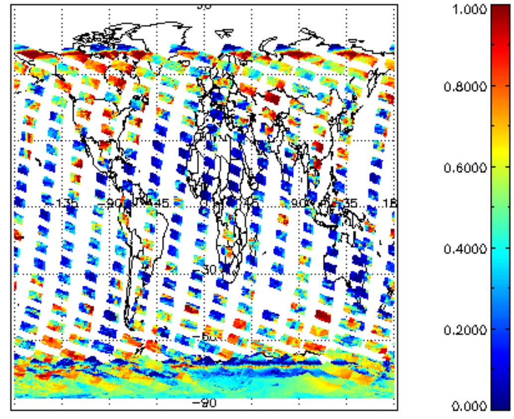
cL_frac for 25JAN2008 00:00:00 to 26JAN2008 00:00:00
