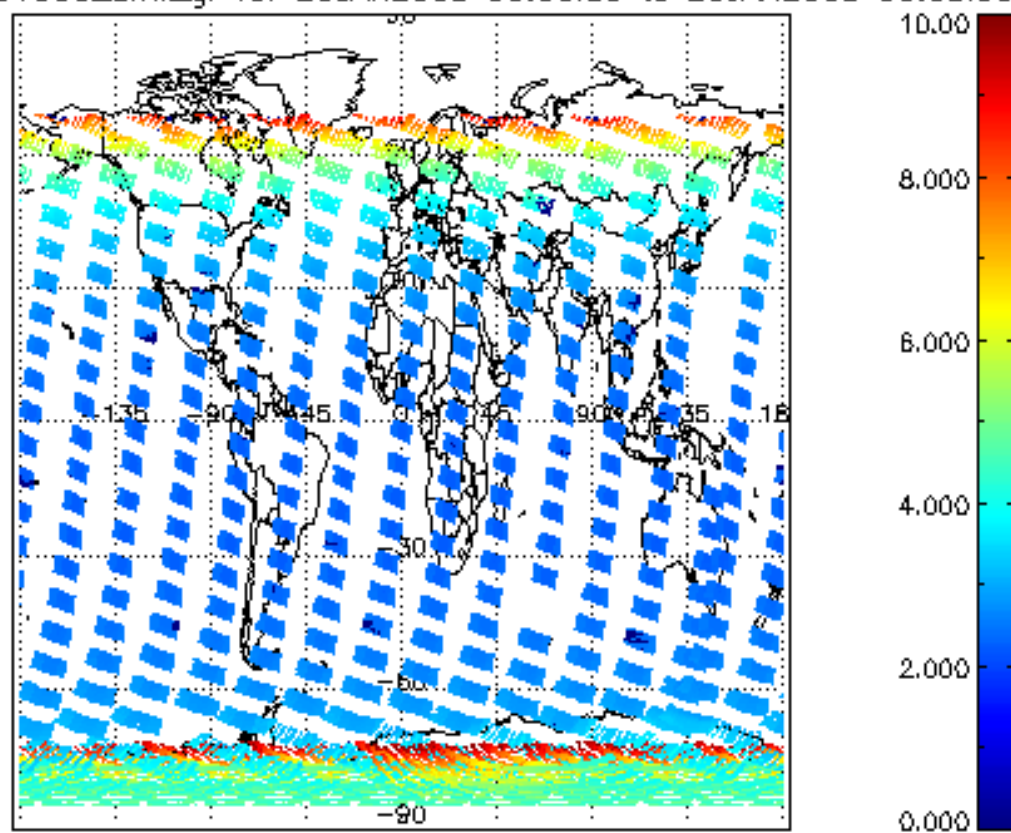
SCIOL2P_NADUV003_amf_gr for 25JAN2008 00:00:00 to 26JAN2008 00:00:00
