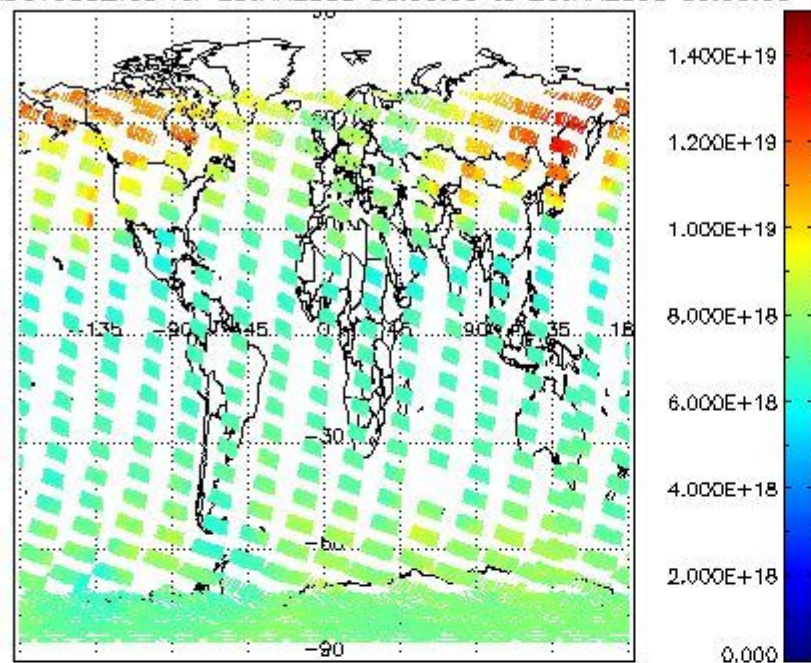
SCIOL2P_NADUV003_vcd for 25JAN2008 00:00:00 to 26JAN2008 00:00:00
