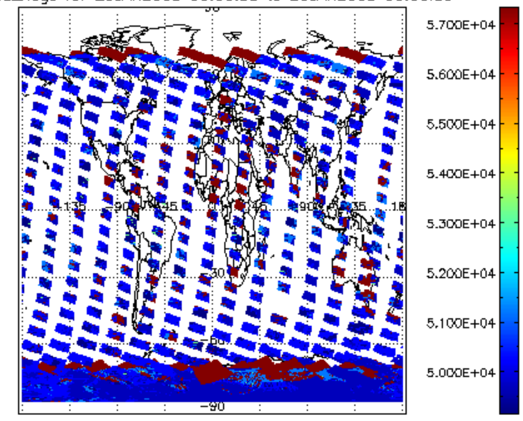
cloud_flags for 25JAN2008 00:00:00 to 26JAN2008 00:00:00
