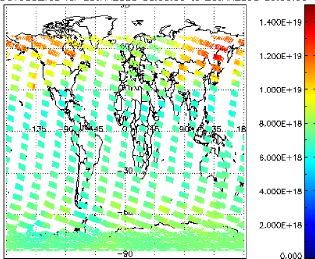
SCIOL2P_NADUV003_vcd for 25JAN2008 00:00:00 to 26JAN2008 00:00:00
