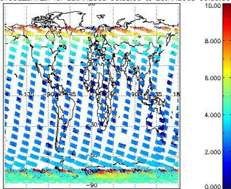
SCIOL2P_NADUV003_amf_cl for 25JAN2008 00:00:00 to 26JAN2008 00:00:00
