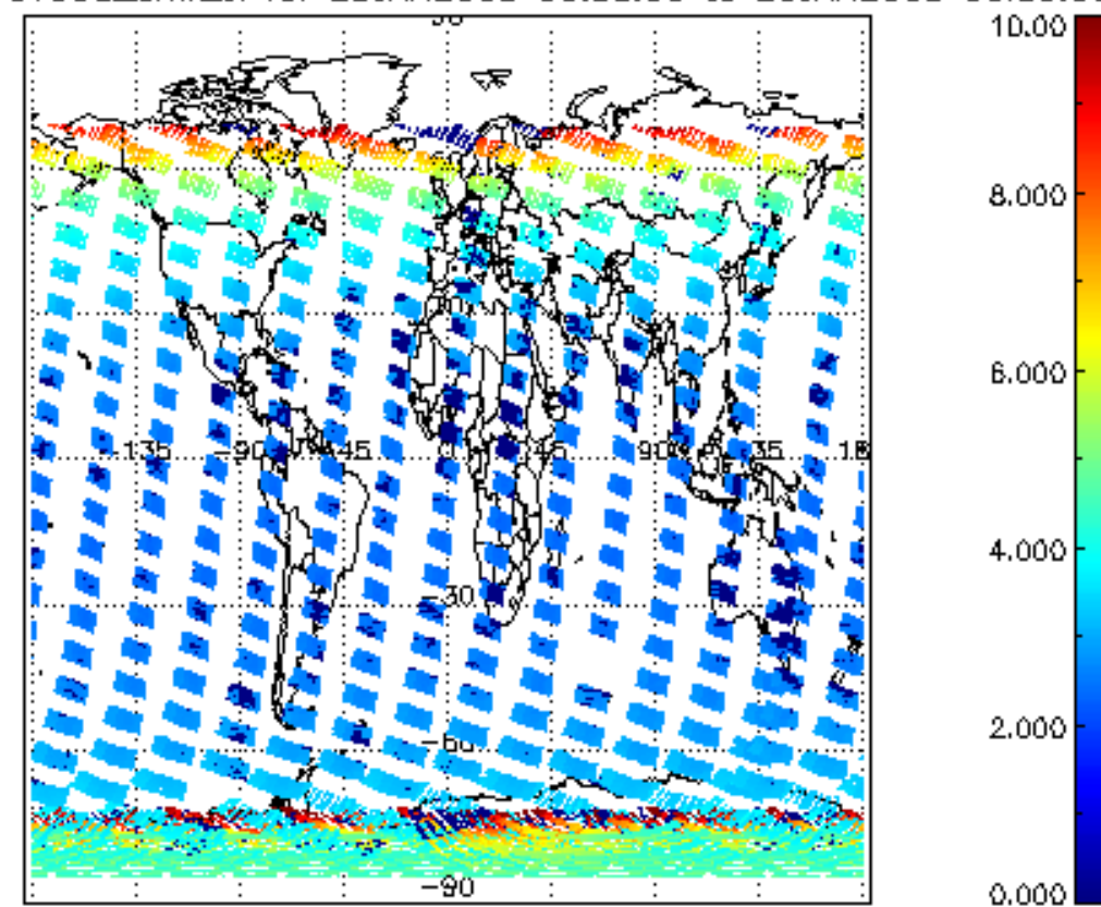
SCIOL2P_NADUV003_amf_cl for 25JAN2008 00:00:00 to 26JAN2008 00:00:00
