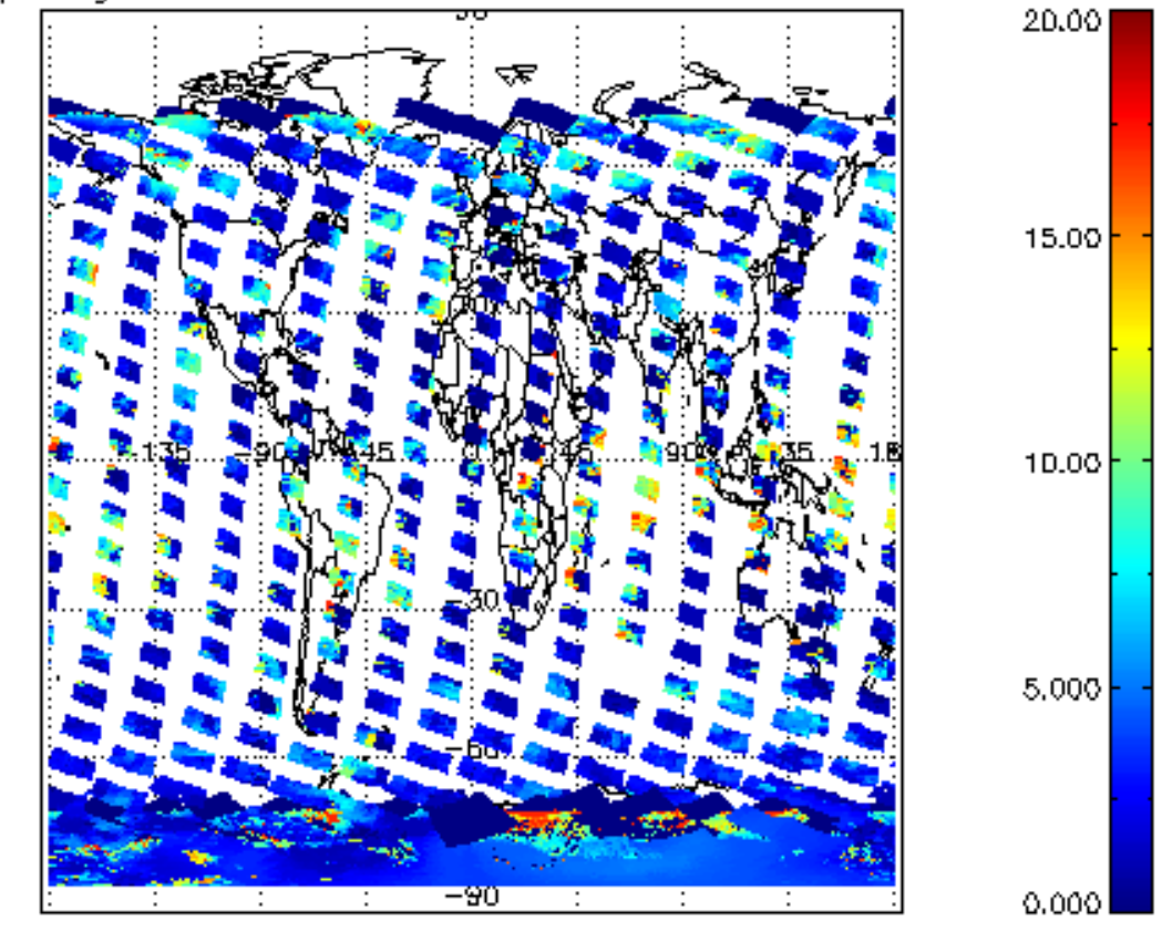
cL_top_height for 25JAN2008 00:00:00 to 26JAN2008 00:00:00
