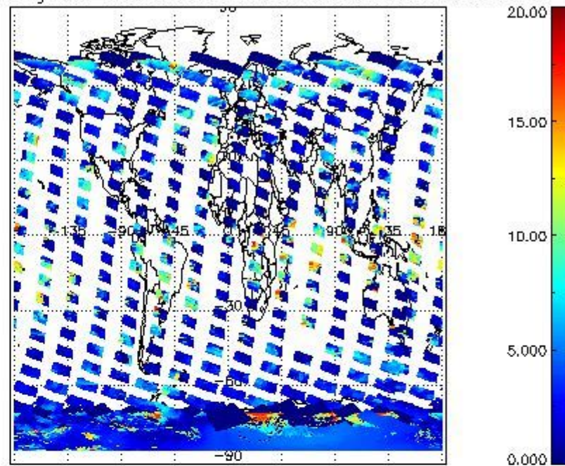
cL_top_height for 25JAN2008 00:00:00 to 26JAN2008 00:00:00
