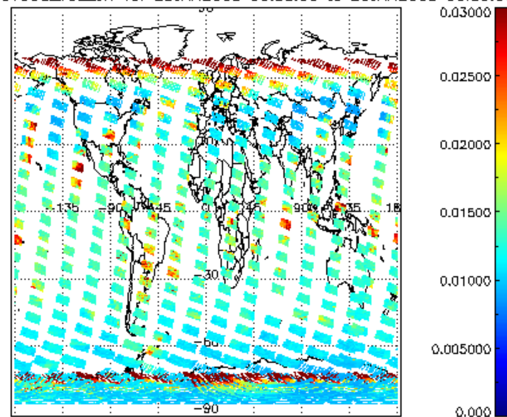
SCIOL2P_NADUV003_vcd_err for 25JAN2008 00:00:00 to 26JAN2008 00:00:00
