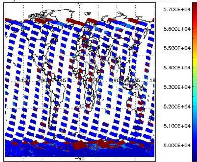
cloud_flags for 25JAN2008 00:00:00 to 26JAN2008 00:00:00
