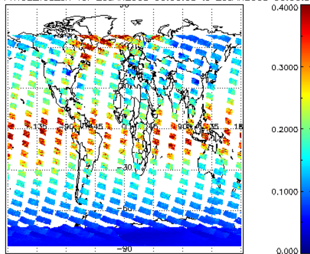
SCIOL2P_NADUV1NO2_vcd_err for 25JAN2008 00:00:00 to 26JAN2008 00:00:00
