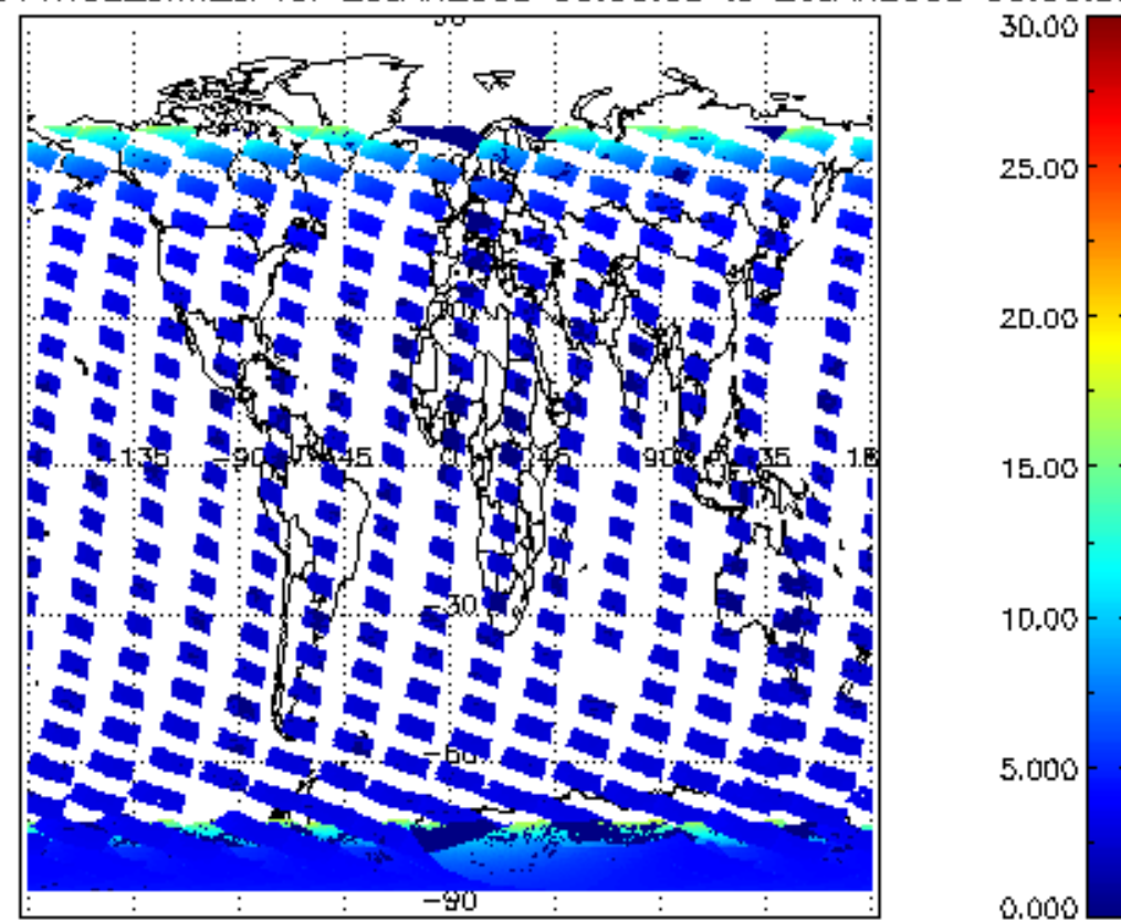
SCIOL2P_NADUV1NO2_amf_cl for 25JAN2008 00:00:00 to 26JAN2008 00:00:00
