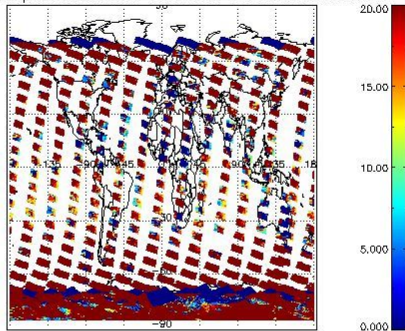
cLopt_depth for 25JAN2008 00:00:00 to 26JAN2008 00:00:00
