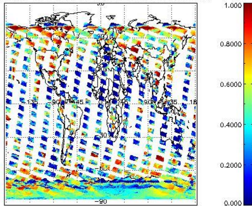
cL_frac for 25JAN2008 00:00:00 to 26JAN2008 00:00:00
