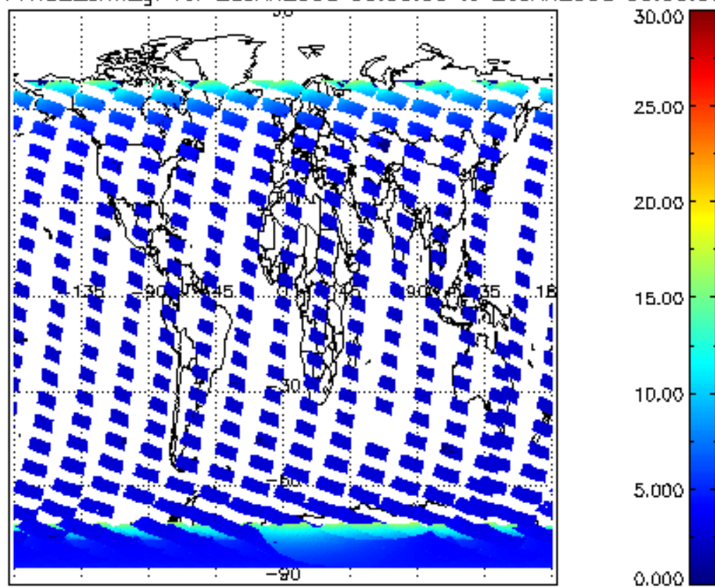
SCIOL2P_NADUV1NO2_amf_gr for 25JAN2008 00:00:00 to 26JAN2008 00:00:00
