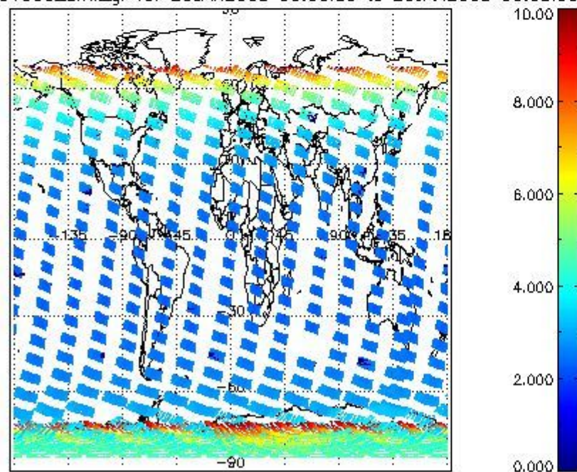
SCIOL2P_NADUV003_amf_gr for 25JAN2008 00:00:00 to 26JAN2008 00:00:00
