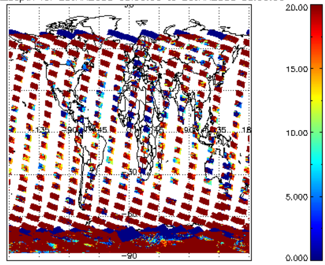
cLopt_depth for 25JAN2008 00:00:00 to 26JAN2008 00:00:00
