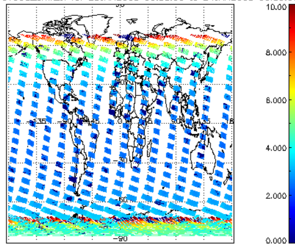
SCIOL2P_NADUV003_amf_cl for 23JAN2008 00:00:00 to 24JAN2008 00:00:00
