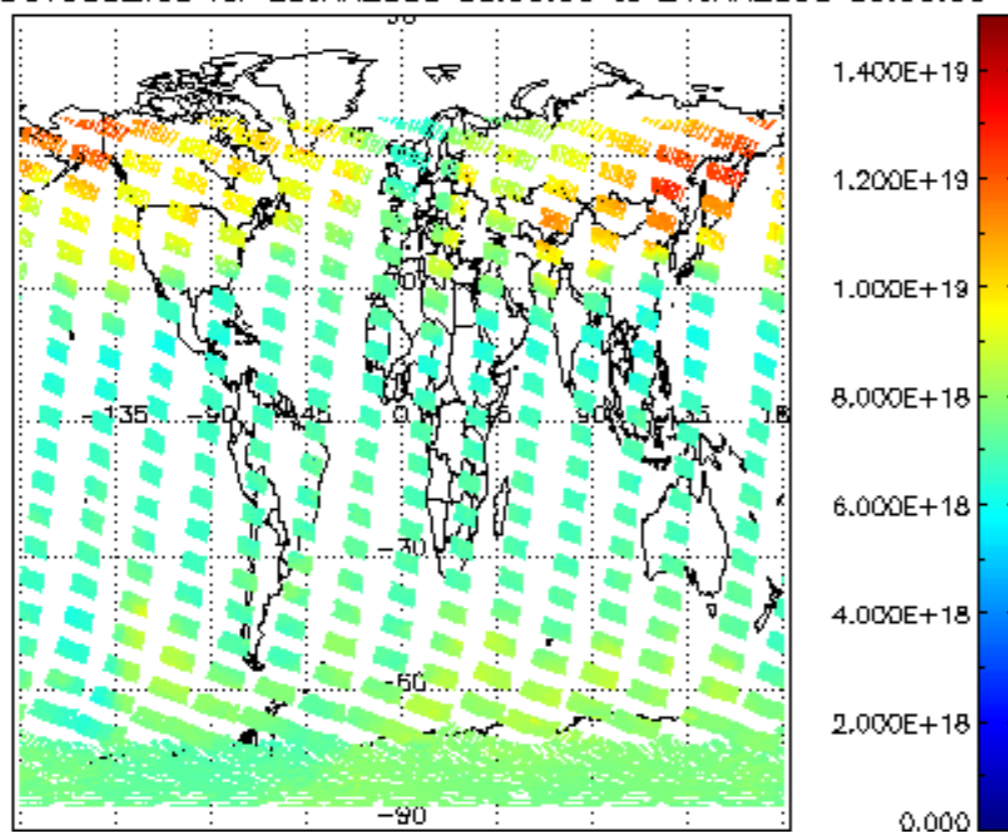
SCIOL2P_NADUV003_vcd for 23JAN2008 00:00:00 to 24JAN2008 00:00:00
