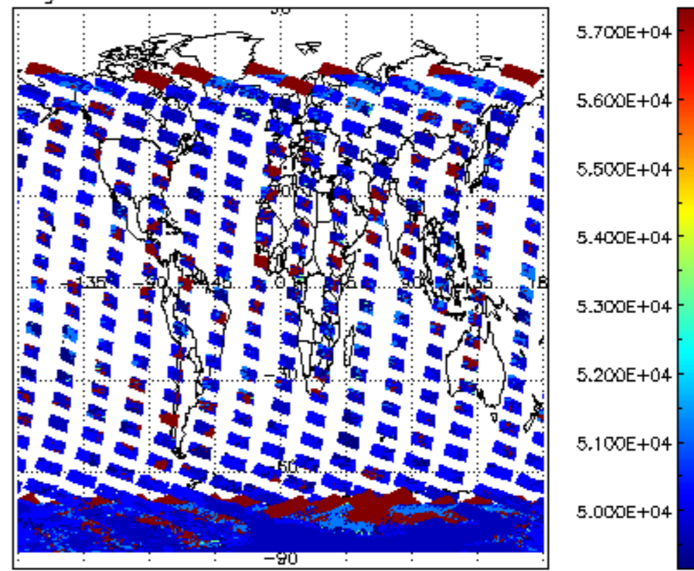
cloud_flags for 23JAN2008 00:00:00 to 24JAN2008 00:00:00
