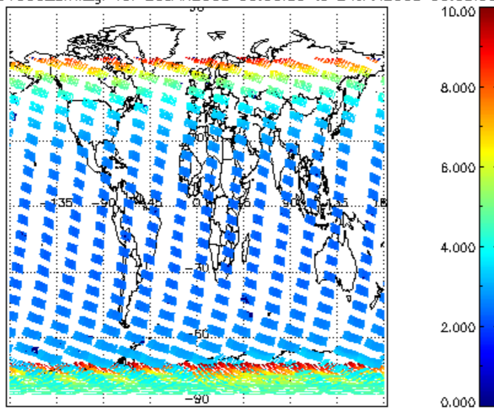
SCIOL2P_NADUV003_amf_gr for 23JAN2008 00:00:00 to 24JAN2008 00:00:00
