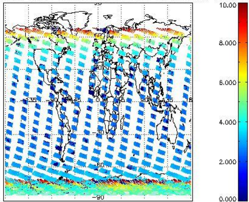
SCIOL2P_NADUV003_amf_cl for 23JAN2008 00:00:00 to 24JAN2008 00:00:00
