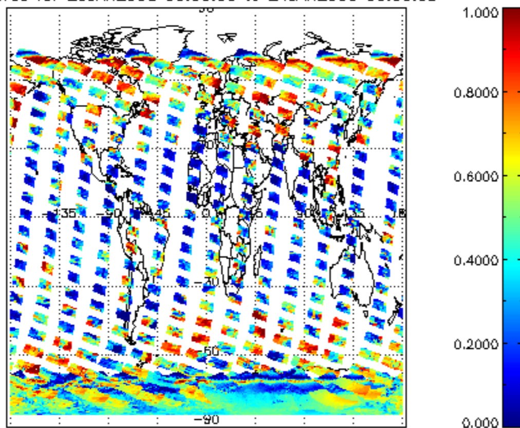
cL_frac for 23JAN2008 00:00:00 to 24JAN2008 00:00:00
