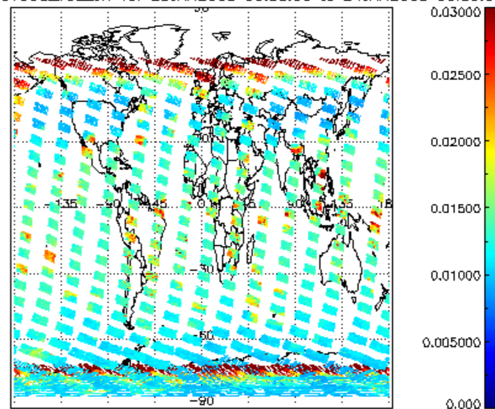
SCIOL2P_NADUV003_vcd_err for 23JAN2008 00:00:00 to 24JAN2008 00:00:00
