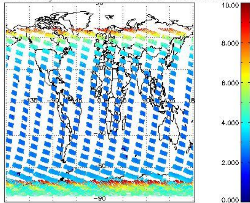
SCIOL2P_NADUV003_amf_gr for 23JAN2008 00:00:00 to 24JAN2008 00:00:00
