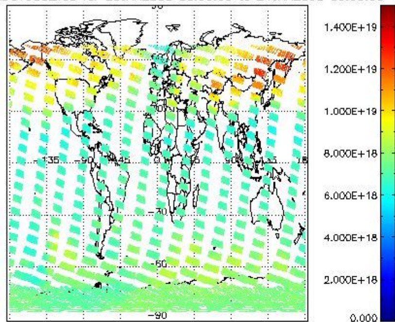
SCIOL2P_NADUV003_vcd for 23JAN2008 00:00:00 to 24JAN2008 00:00:00
