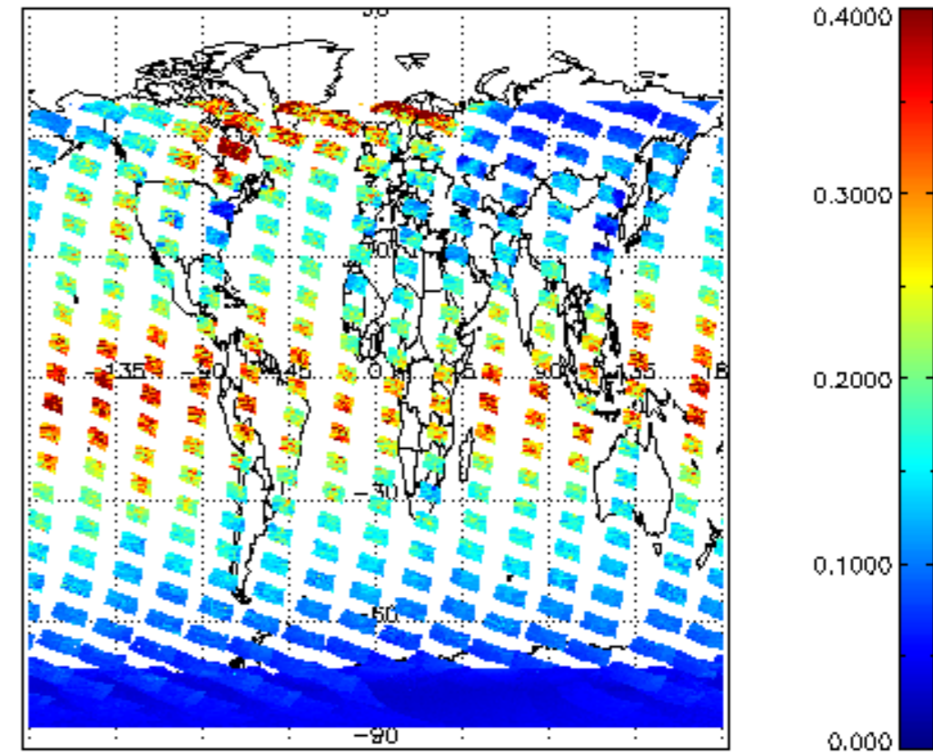
SCIOL2P_NADUV1NO2_vcd_err for 23JAN2008 00:00:00 to 24JAN2008 00:00:00
