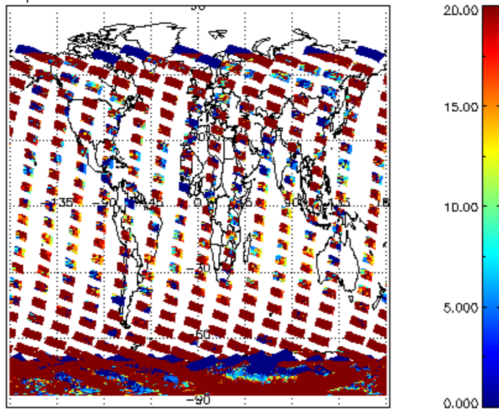
cLopt_depth for 23JAN2008 00:00:00 to 24JAN2008 00:00:00
