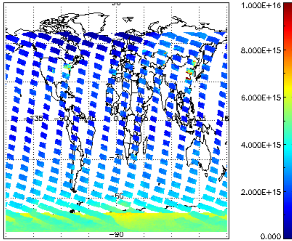
SCIOL2P_NADUV1NO2_vcd for 23JAN2008 00:00:00 to 24JAN2008 00:00:00
