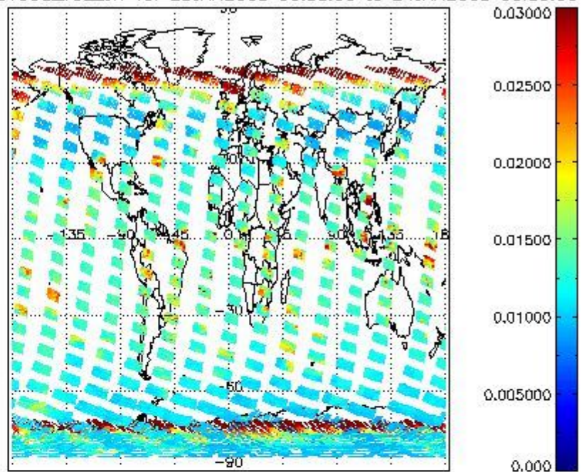
SCIOL2P_NADUV003_vcd_err for 23JAN2008 00:00:00 to 24JAN2008 00:00:00
