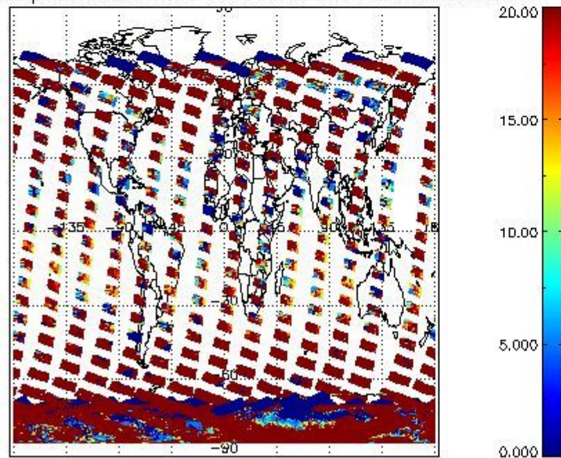
cLopt_depth for 23JAN2008 00:00:00 to 24JAN2008 00:00:00
