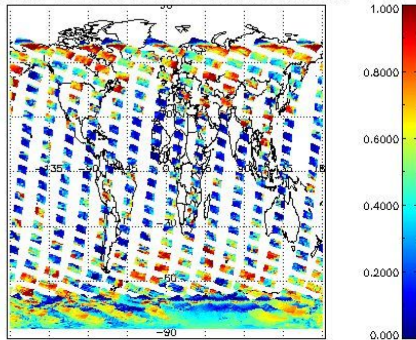
cL_frac for 23JAN2008 00:00:00 to 24JAN2008 00:00:00
