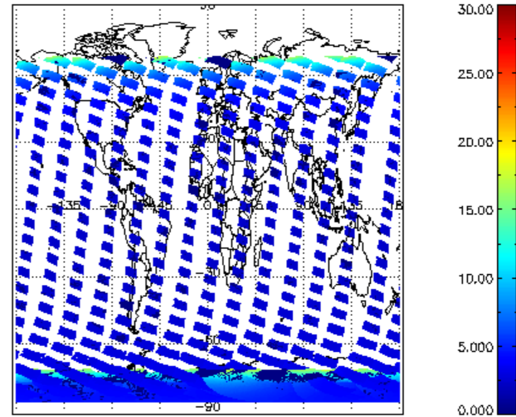
SCIOL2P_NADUV1NO2_amf_cl for 23JAN2008 00:00:00 to 24JAN2008 00:00:00
