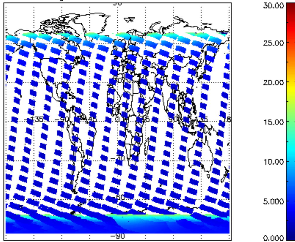
SCIOL2P_NADUV1NO2_amf_gr for 23JAN2008 00:00:00 to 24JAN2008 00:00:00
