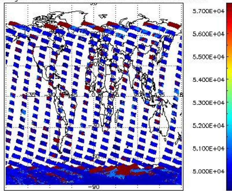
cloud_flags for 23JAN2008 00:00:00 to 24JAN2008 00:00:00
