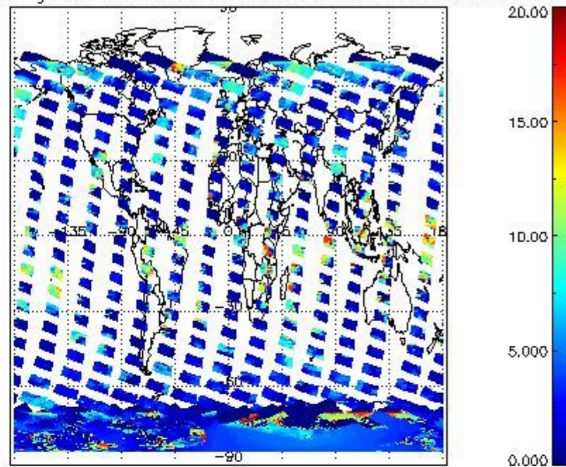
cL_top_height for 23JAN2008 00:00:00 to 24JAN2008 00:00:00
