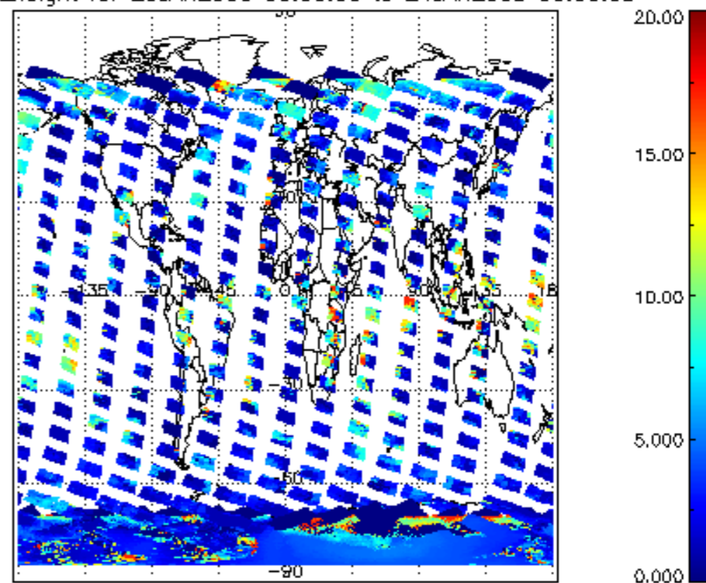
cL_top_height for 23JAN2008 00:00:00 to 24JAN2008 00:00:00
