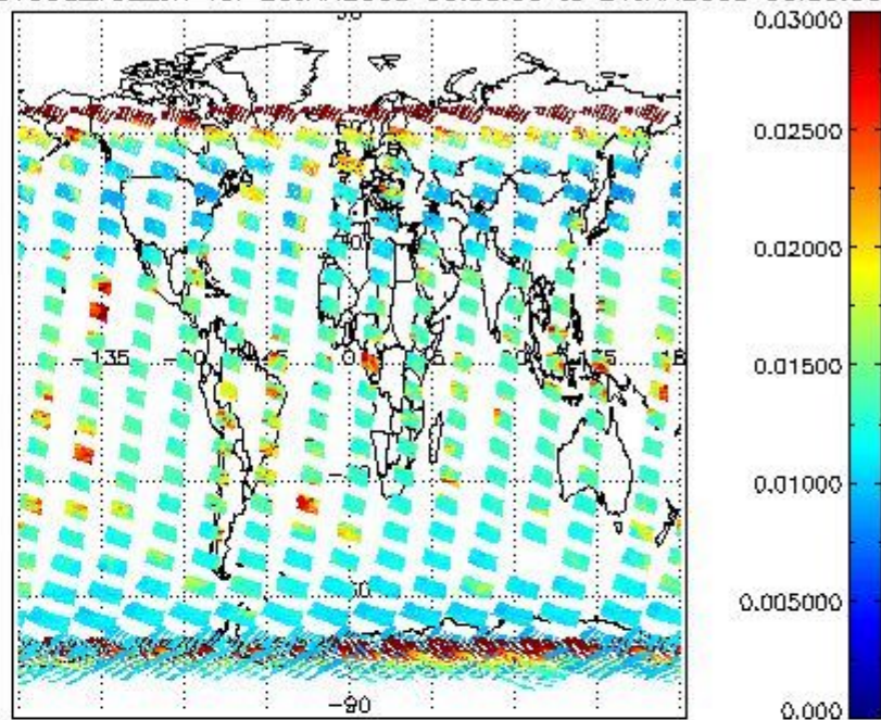
SCIOL2P_NADUV003_vcd_err for 20JAN2008 00:00:00 to 21JAN2008 00:00:00
