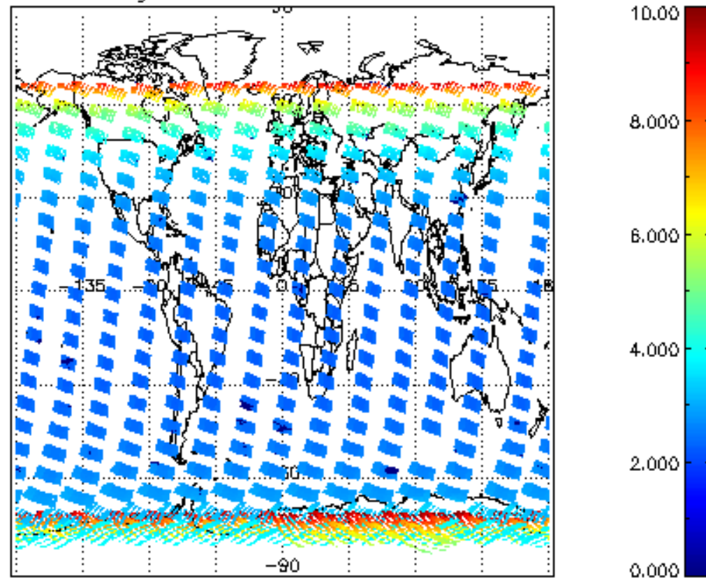
SCIOL2P_NADUV003_amf_gr for 20JAN2008 00:00:00 to 21JAN2008 00:00:00
