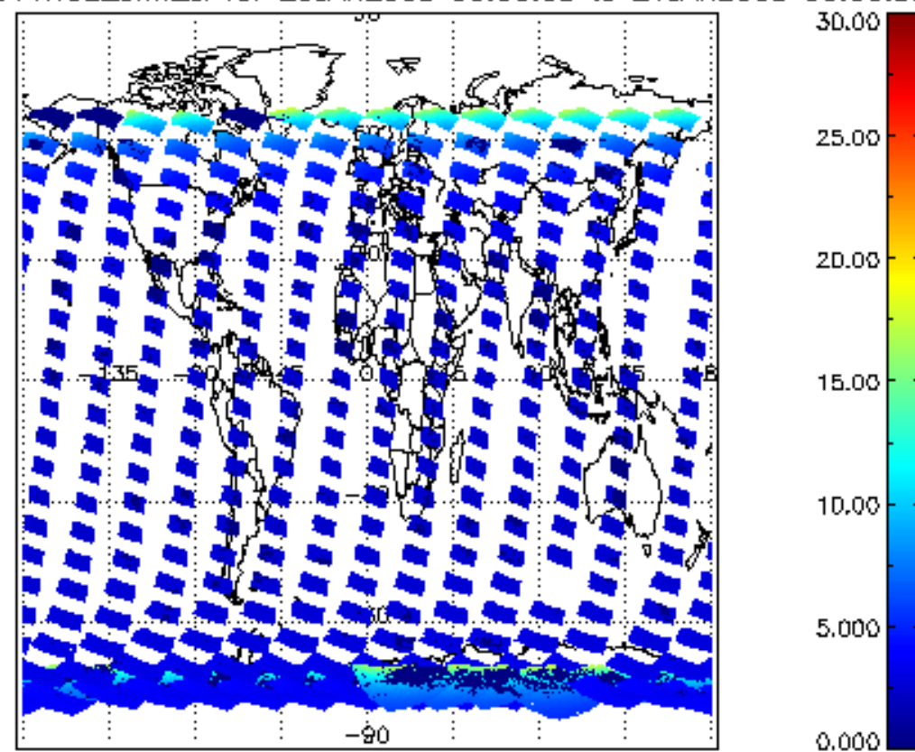
SCIOL2P_NADUV1NO2_amf_cl for 20JAN2008 00:00:00 to 21JAN2008 00:00:00
