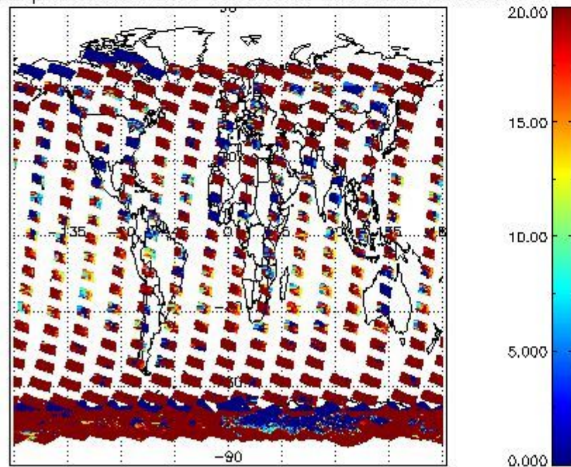
cLopt_depth for 20JAN2008 00:00:00 to 21JAN2008 00:00:00
