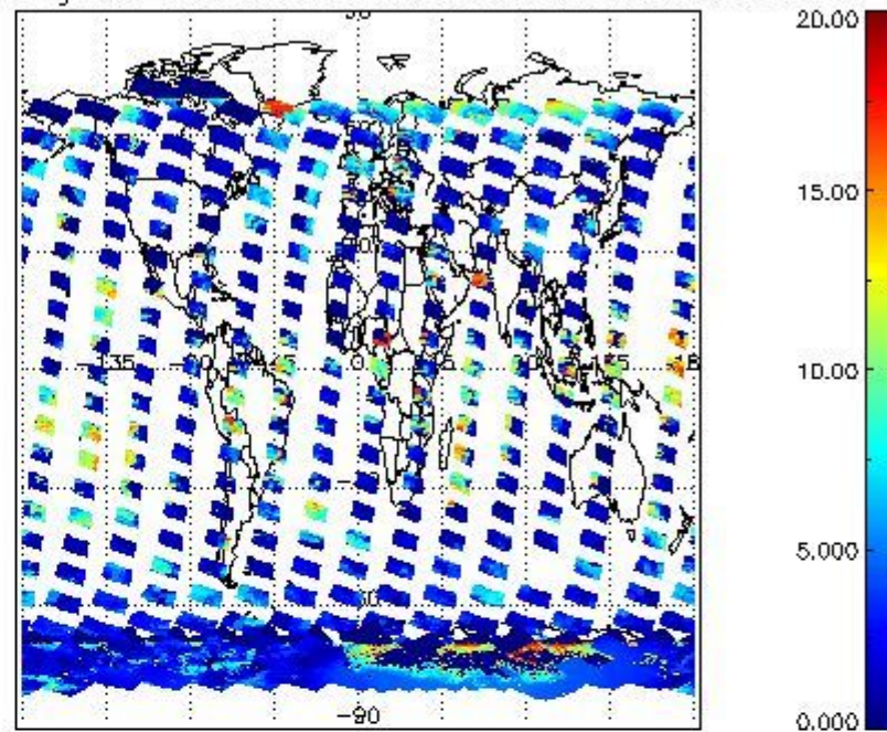
cL_top_height for 20JAN2008 00:00:00 to 21JAN2008 00:00:00
