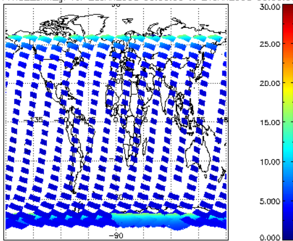
SCIOL2P_NADUV1NO2_amf_gr for 20JAN2008 00:00:00 to 21JAN2008 00:00:00
