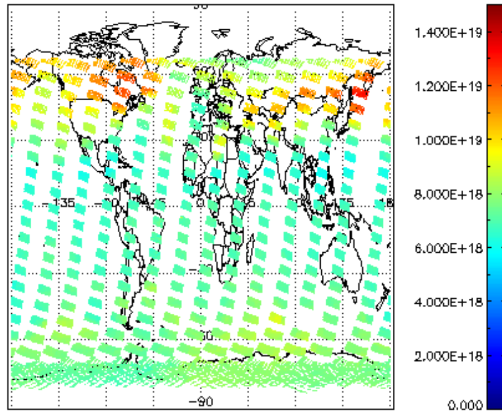
SCIOL2P_NADUV003_vcd for 20JAN2008 00:00:00 to 21JAN2008 00:00:00
