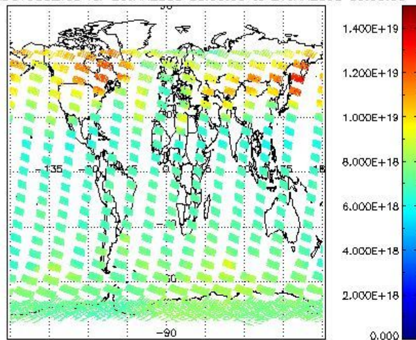
SCIOL2P_NADUV003_vcd for 20JAN2008 00:00:00 to 21JAN2008 00:00:00
