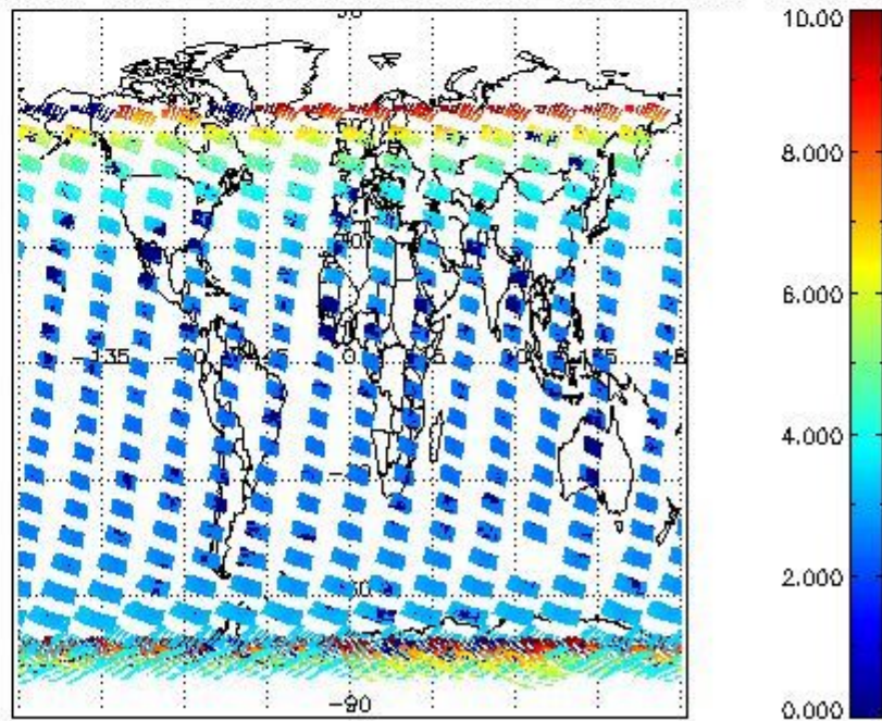
SCIOL2P_NADUV003_amf_cl for 20JAN2008 00:00:00 to 21JAN2008 00:00:00
