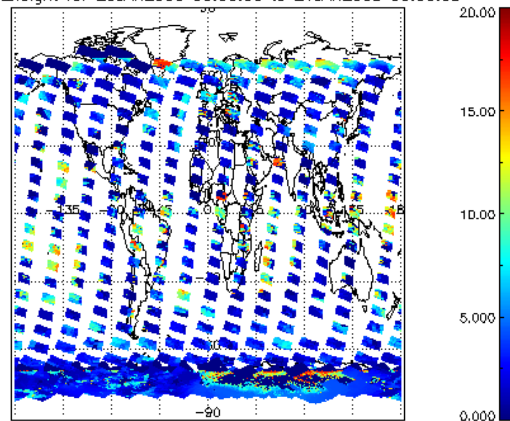
cL_top_height for 20JAN2008 00:00:00 to 21JAN2008 00:00:00
