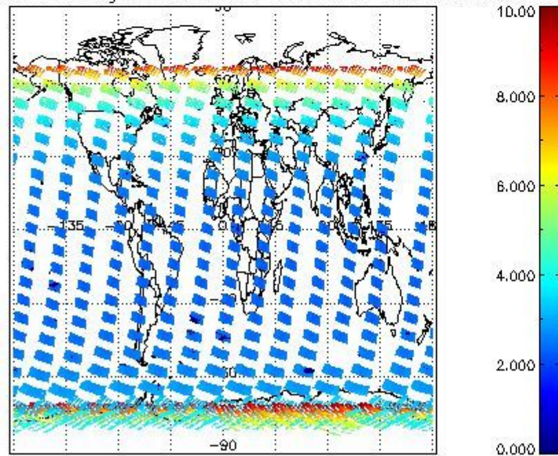
SCIOL2P_NADUV003_amf_gr for 20JAN2008 00:00:00 to 21JAN2008 00:00:00
