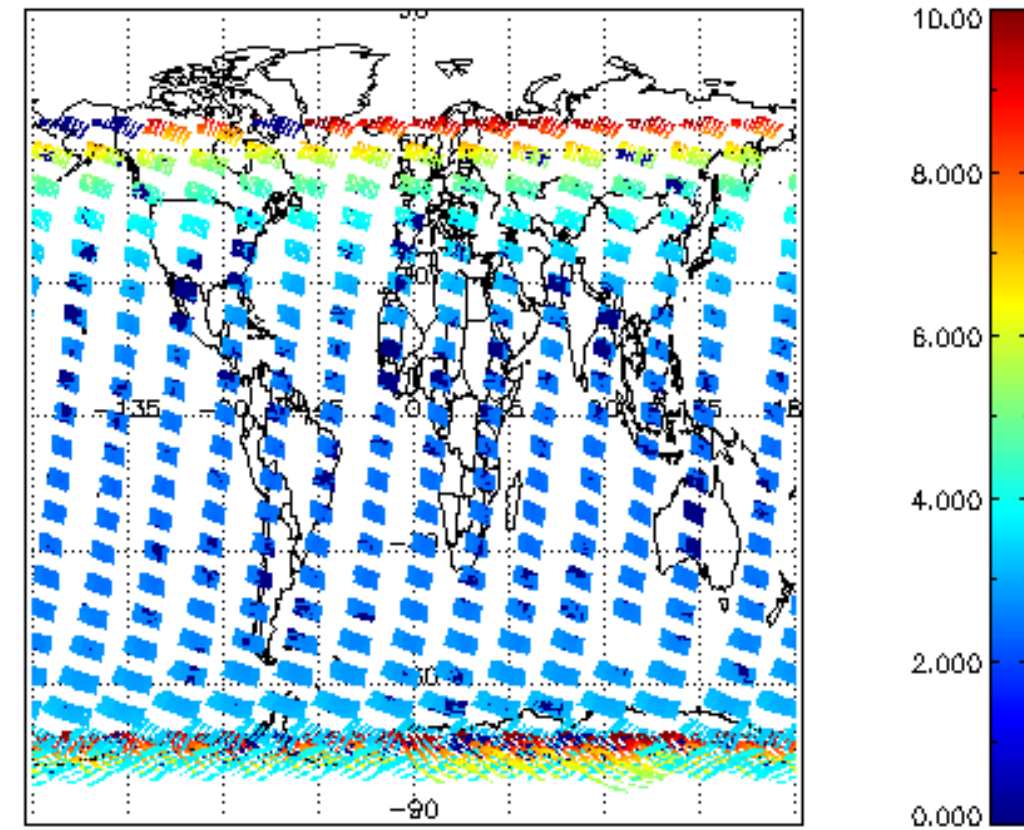
SCIOL2P_NADUV003_amf_cl for 20JAN2008 00:00:00 to 21JAN2008 00:00:00
