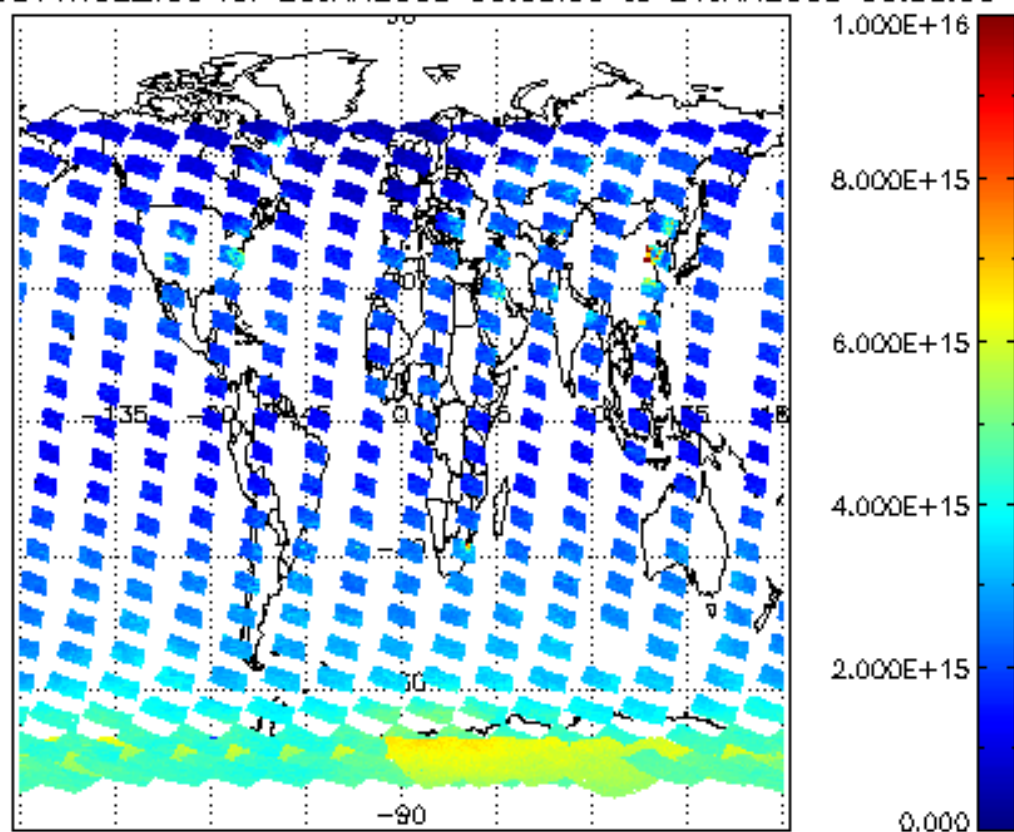
SCIOL2P_NADUV1NO2_vcd for 20JAN2008 00:00:00 to 21JAN2008 00:00:00
