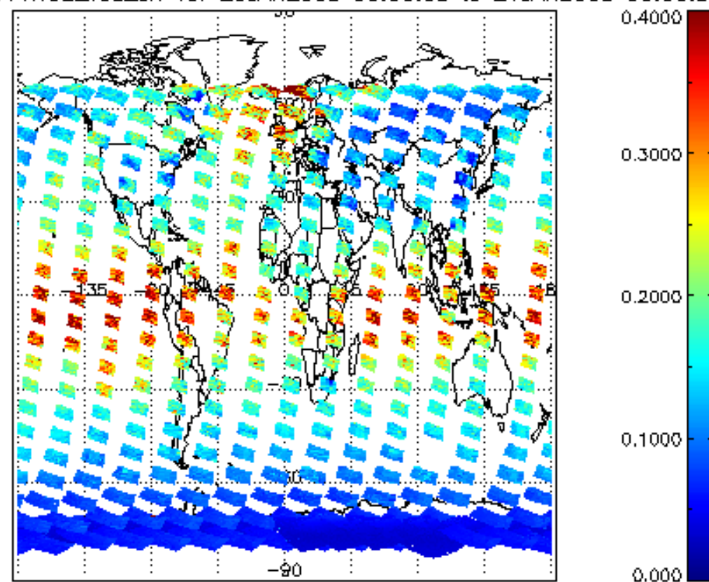
SCIOL2P_NADUV1NO2_vcd_err for 20JAN2008 00:00:00 to 21JAN2008 00:00:00
