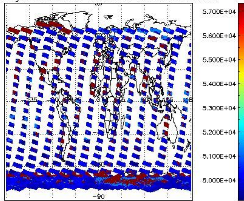
cloud_flags for 20JAN2008 00:00:00 to 21JAN2008 00:00:00
