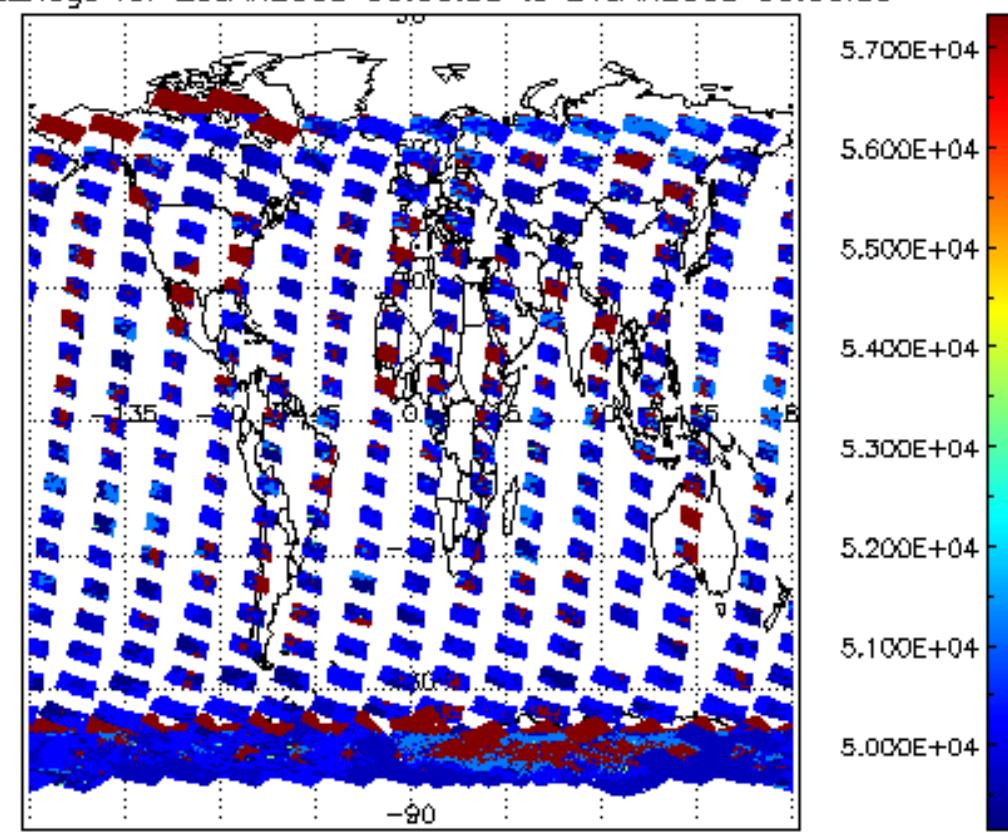
cloud_flags for 20JAN2008 00:00:00 to 21JAN2008 00:00:00
