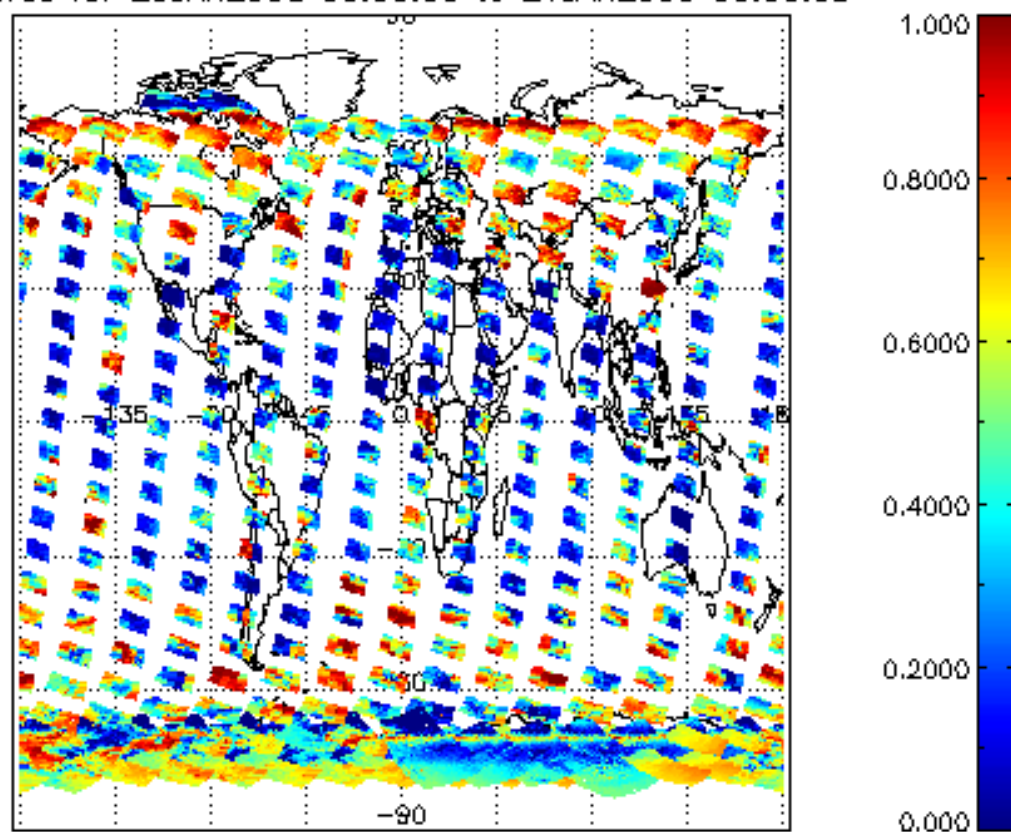
cL_frac for 20JAN2008 00:00:00 to 21JAN2008 00:00:00
