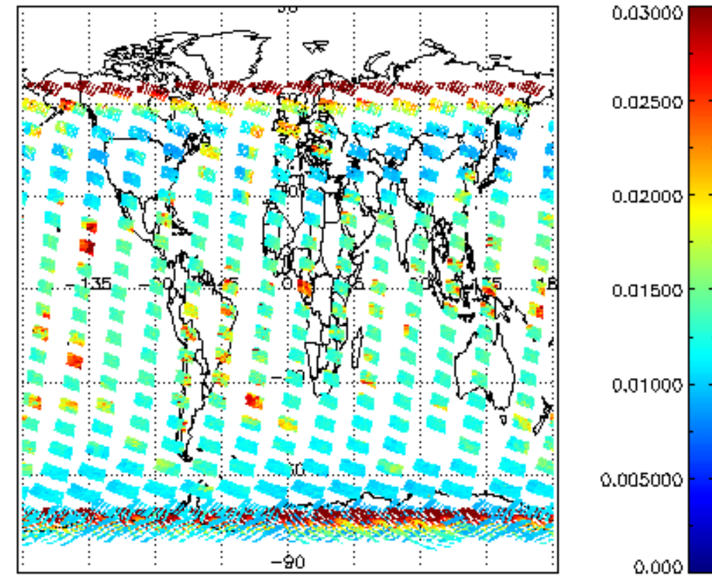
SCIOL2P_NADUV003_vcd_err for 20JAN2008 00:00:00 to 21JAN2008 00:00:00
