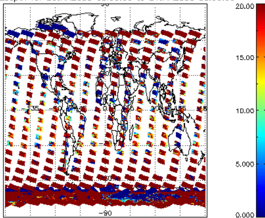
cLopt_depth for 20JAN2008 00:00:00 to 21JAN2008 00:00:00
