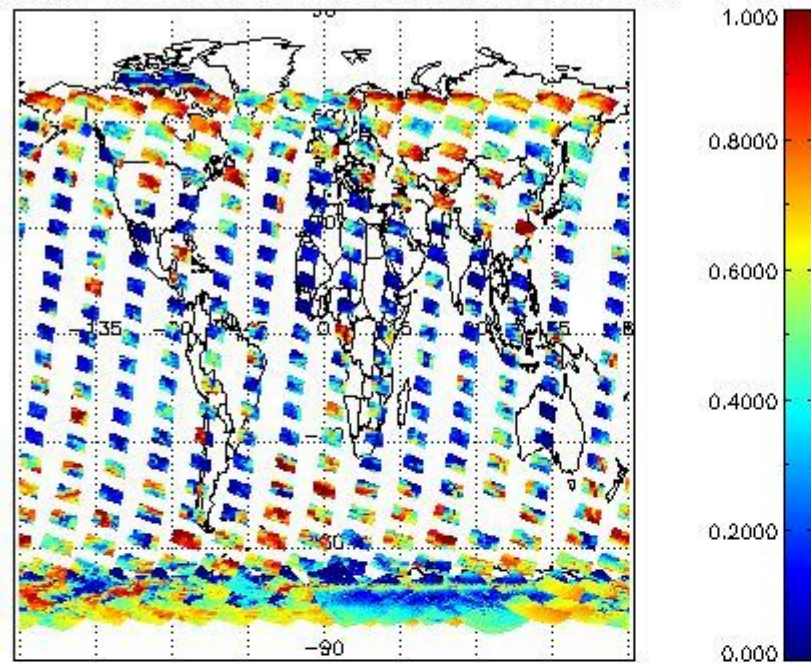
cL_frac for 20JAN2008 00:00:00 to 21JAN2008 00:00:00
