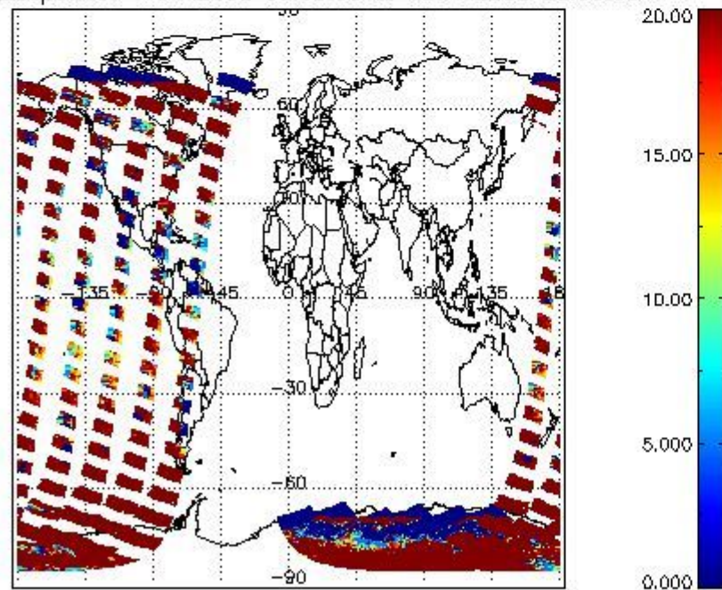
cLopt_depth for 17JAN2008 00:00:00 to 18JAN2008 00:00:00
