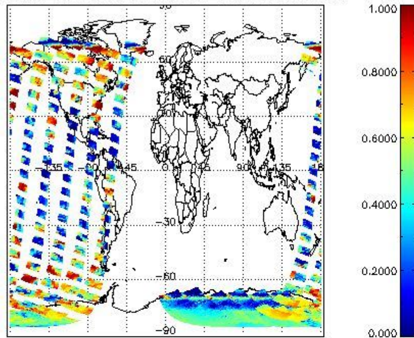
cL_frac for 17JAN2008 00:00:00 to 18JAN2008 00:00:00
