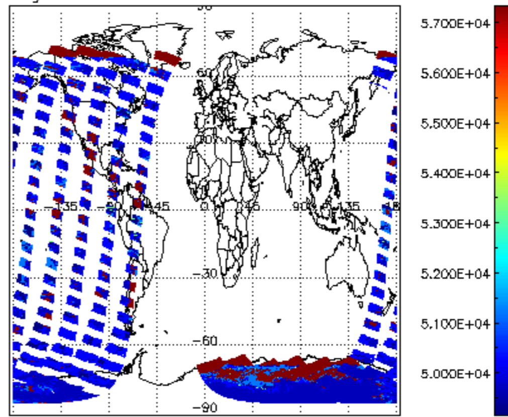
cloud_flags for 17JAN2008 00:00:00 to 18JAN2008 00:00:00
