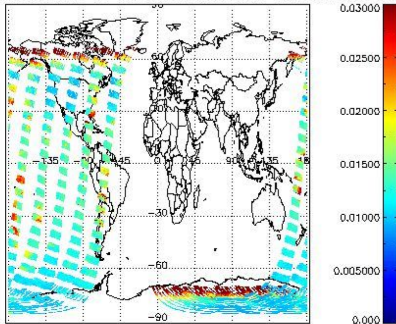
SCIOL2P_NADUV003_vcd_err for 17JAN2008 00:00:00 to 18JAN2008 00:00:00
