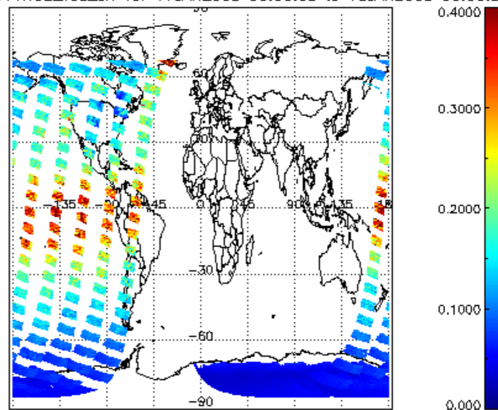
SCIOL2P_NADUV1NO2_vcd_err for 17JAN2008 00:00:00 to 18JAN2008 00:00:00
