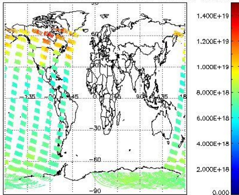
SCIOL2P_NADUV003_vcd for 17JAN2008 00:00:00 to 18JAN2008 00:00:00
