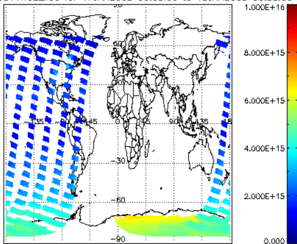
SCIOL2P_NADUV1NO2_vcd for 17JAN2008 00:00:00 to 18JAN2008 00:00:00
