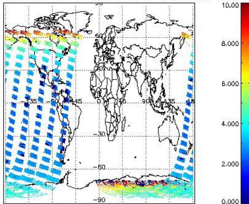
SCIOL2P_NADUV003_amf_cl for 17JAN2008 00:00:00 to 18JAN2008 00:00:00
