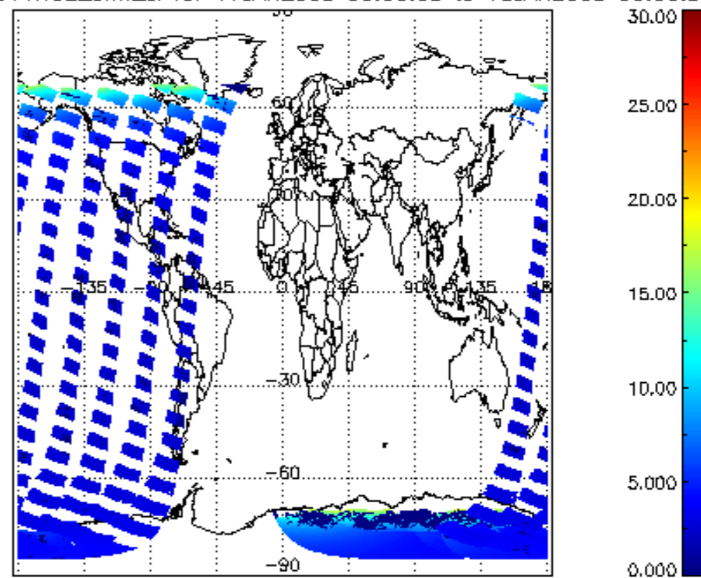
SCIOL2P_NADUV1NO2_amf_cl for 17JAN2008 00:00:00 to 18JAN2008 00:00:00
