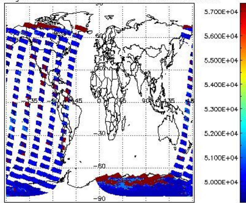
cloud_flags for 17JAN2008 00:00:00 to 18JAN2008 00:00:00
