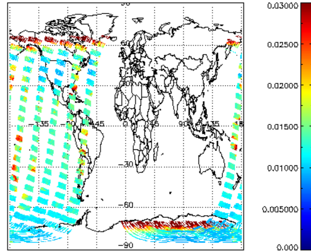
SCIOL2P_NADUV003_vcd_err for 17JAN2008 00:00:00 to 18JAN2008 00:00:00
