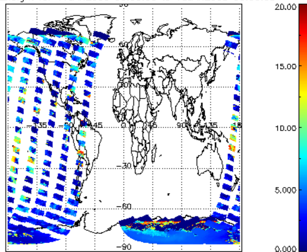
cL_top_height for 17JAN2008 00:00:00 to 18JAN2008 00:00:00
