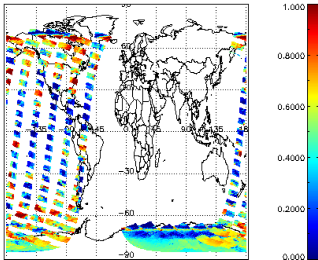
cL_frac for 17JAN2008 00:00:00 to 18JAN2008 00:00:00
