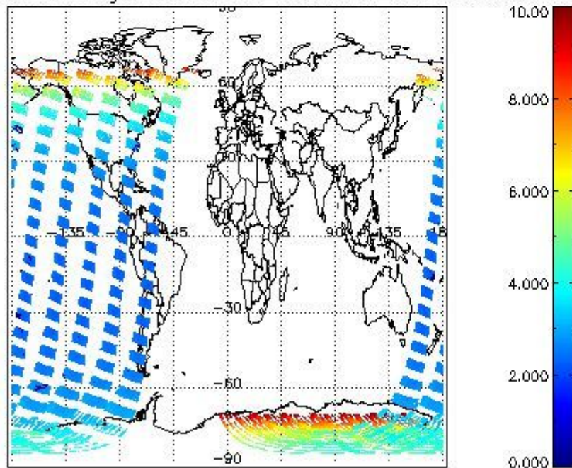
SCIOL2P_NADUV003_amf_gr for 17JAN2008 00:00:00 to 18JAN2008 00:00:00
