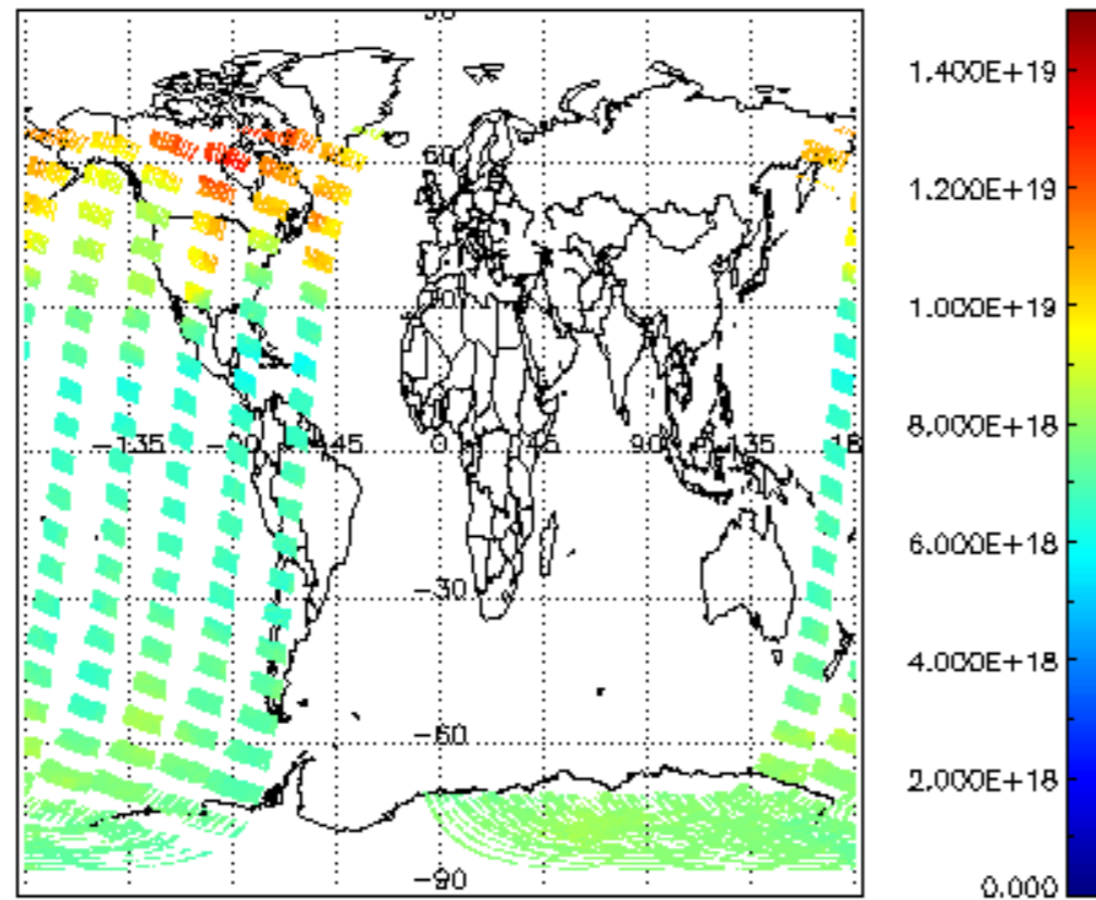
SCIOL2P_NADUV003_vcd for 17JAN2008 00:00:00 to 18JAN2008 00:00:00
