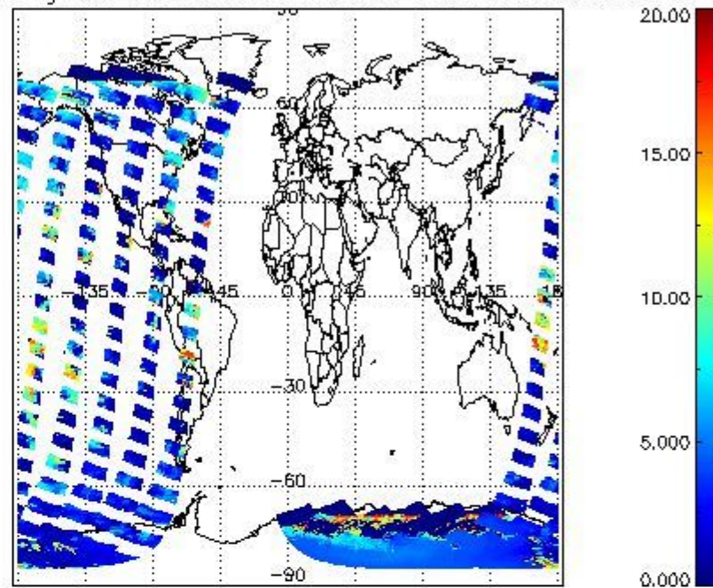
cL_top_height for 17JAN2008 00:00:00 to 18JAN2008 00:00:00
