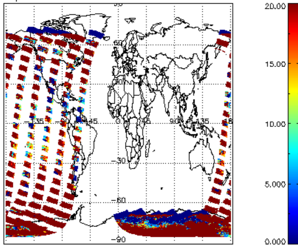
cLopt_depth for 17JAN2008 00:00:00 to 18JAN2008 00:00:00
