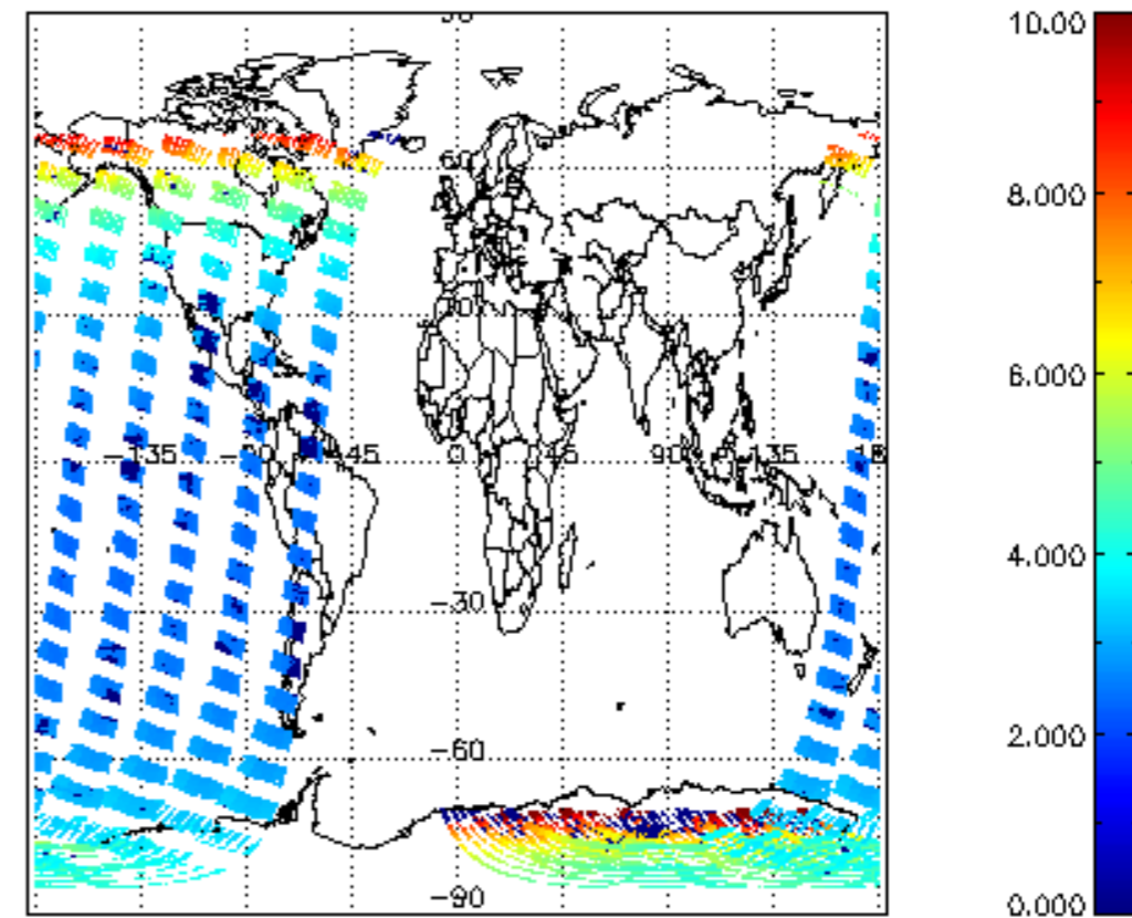
SCIOL2P_NADUV003_amf_cl for 17JAN2008 00:00:00 to 18JAN2008 00:00:00
