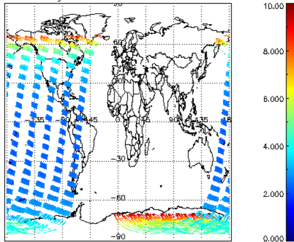
SCIOL2P_NADUV003_amf_gr for 17JAN2008 00:00:00 to 18JAN2008 00:00:00
