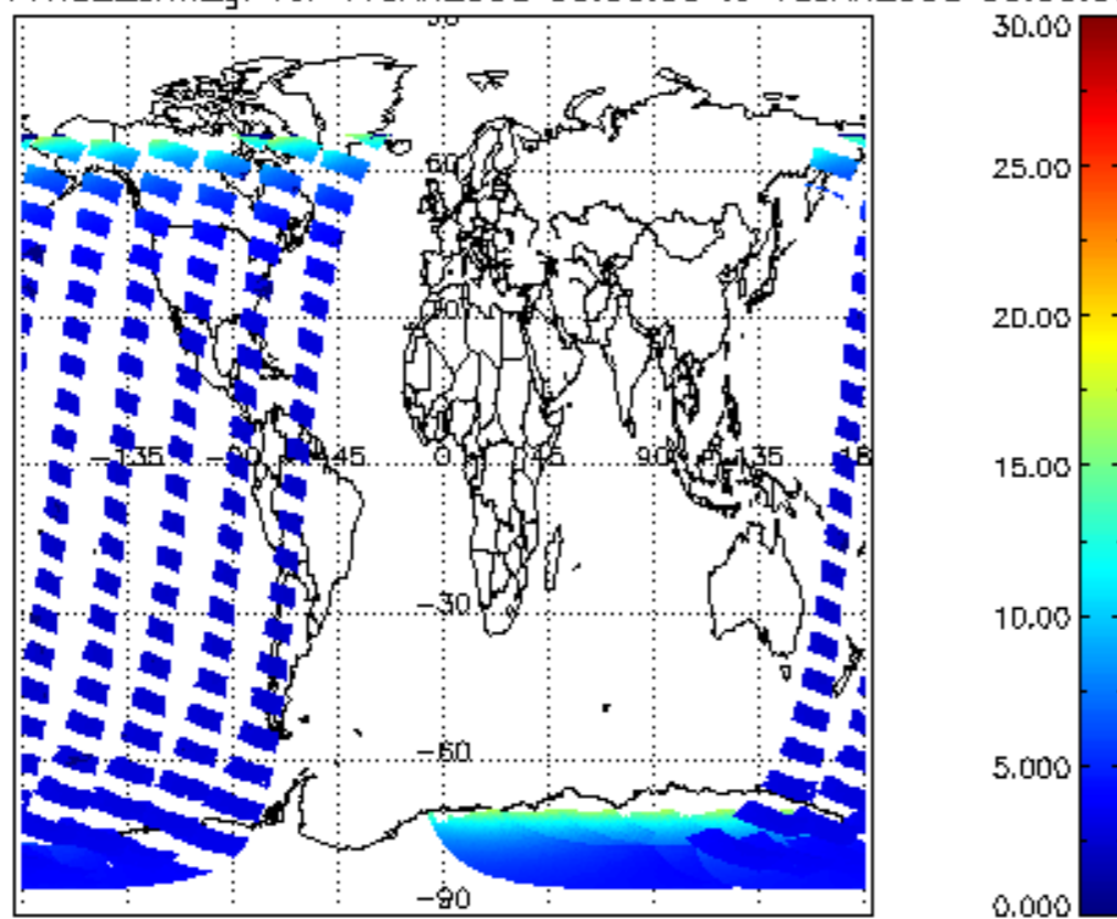
SCIOL2P_NADUV1NO2_amf_gr for 17JAN2008 00:00:00 to 18JAN2008 00:00:00
