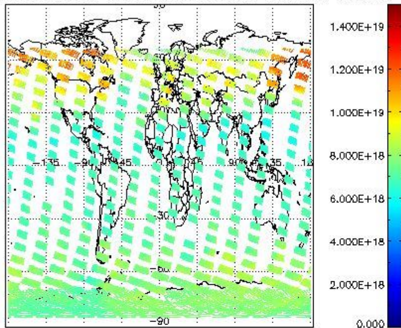
SCIOL2P_NADUV003_vcd for 15JAN2008 00:00:00 to 16JAN2008 00:00:00
