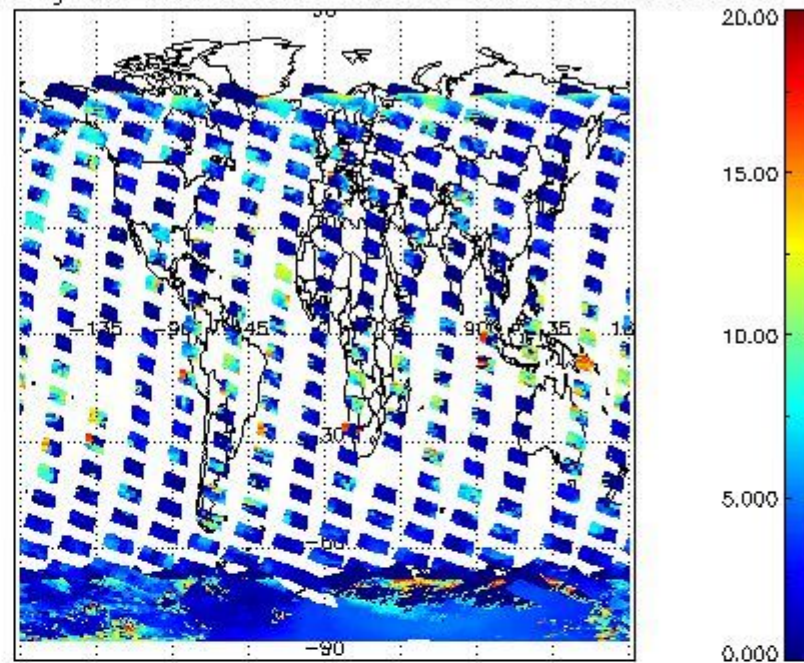
cL_top_height for 15JAN2008 00:00:00 to 16JAN2008 00:00:00
