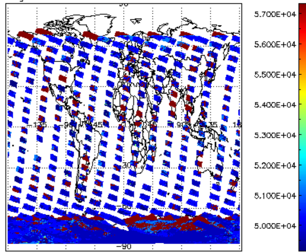
cloud_flags for 15JAN2008 00:00:00 to 16JAN2008 00:00:00
