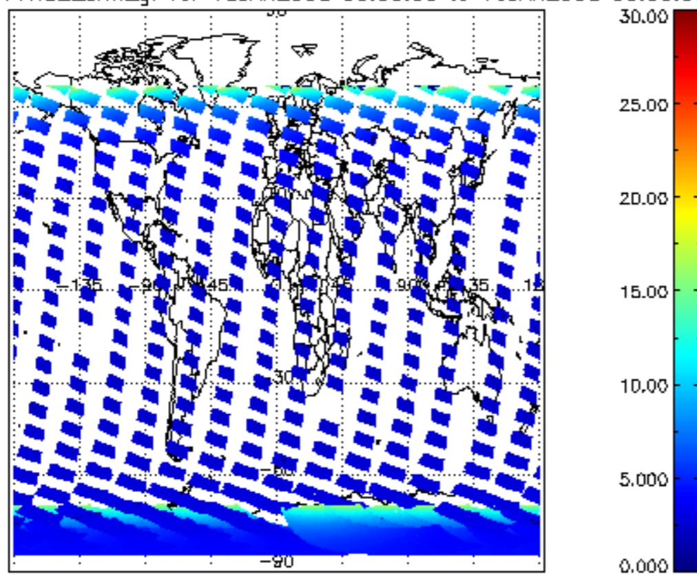
SCIOL2P_NADUV1NO2_amf_gr for 15JAN2008 00:00:00 to 16JAN2008 00:00:00
