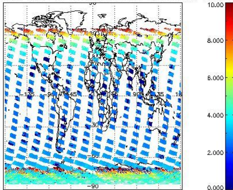
SCIOL2P_NADUV003_amf_cl for 15JAN2008 00:00:00 to 16JAN2008 00:00:00
