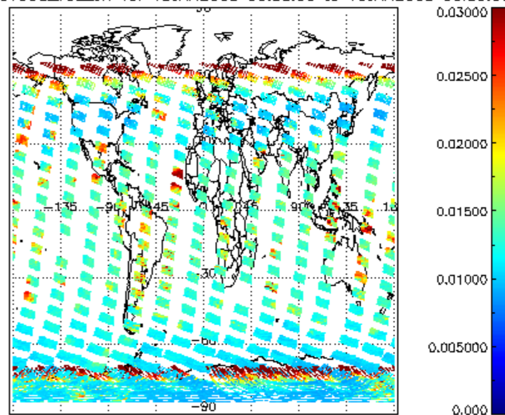
SCIOL2P_NADUV003_vcd_err for 15JAN2008 00:00:00 to 16JAN2008 00:00:00
