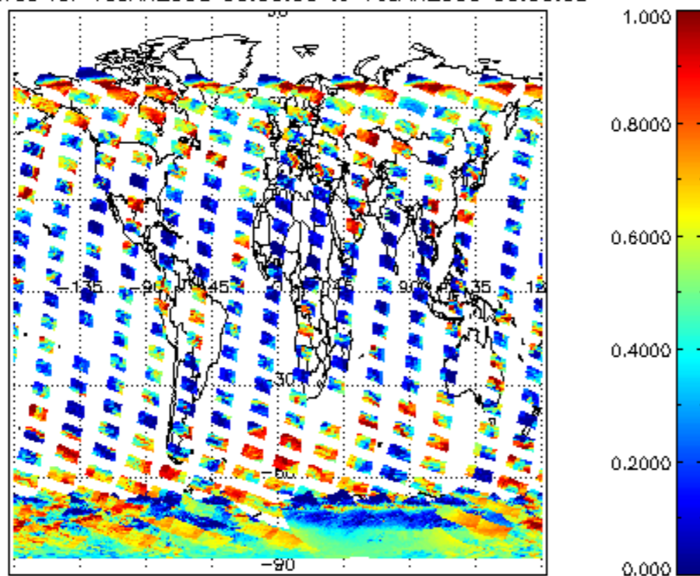
cL_frac for 15JAN2008 00:00:00 to 16JAN2008 00:00:00
