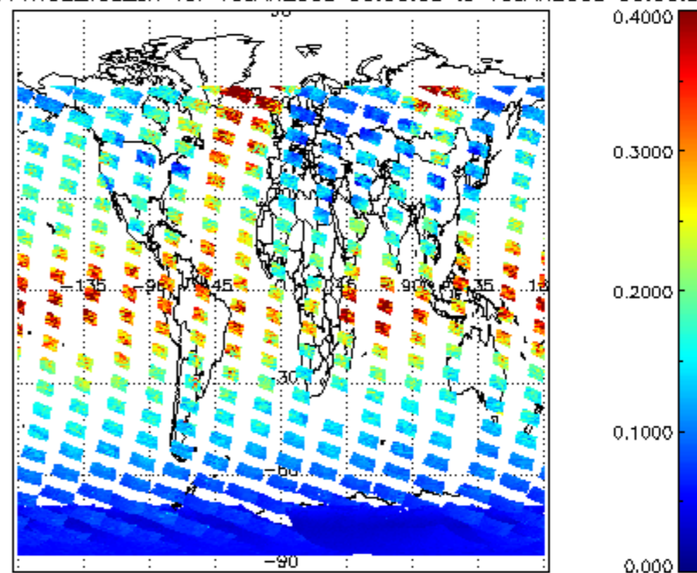
SCIOL2P_NADUV1NO2_vcd_err for 15JAN2008 00:00:00 to 16JAN2008 00:00:00
