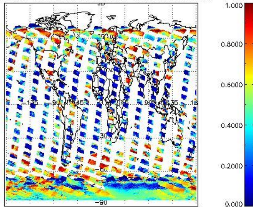
cL_frac for 15JAN2008 00:00:00 to 16JAN2008 00:00:00
