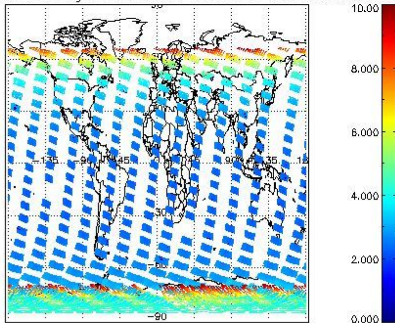
SCIOL2P_NADUV003_amf_gr for 15JAN2008 00:00:00 to 16JAN2008 00:00:00
