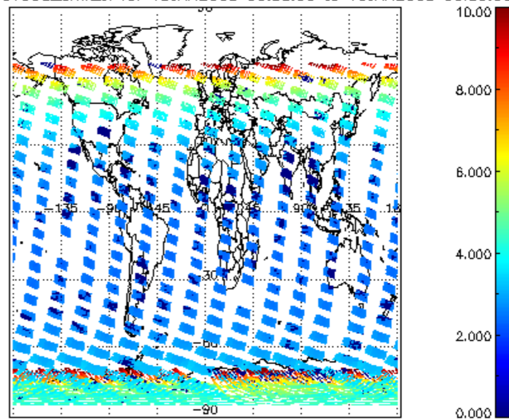
SCIOL2P_NADUV003_amf_cl for 15JAN2008 00:00:00 to 16JAN2008 00:00:00
