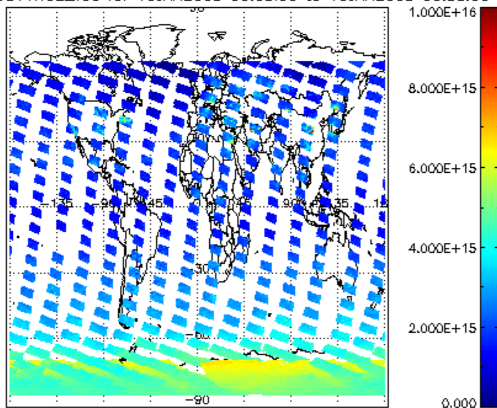
SCIOL2P_NADUV1NO2_vcd for 15JAN2008 00:00:00 to 16JAN2008 00:00:00
