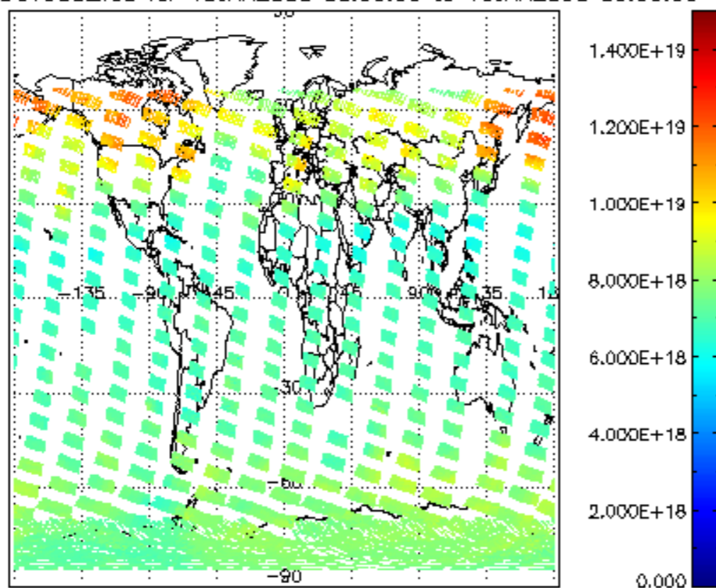
SCIOL2P_NADUV003_vcd for 15JAN2008 00:00:00 to 16JAN2008 00:00:00
