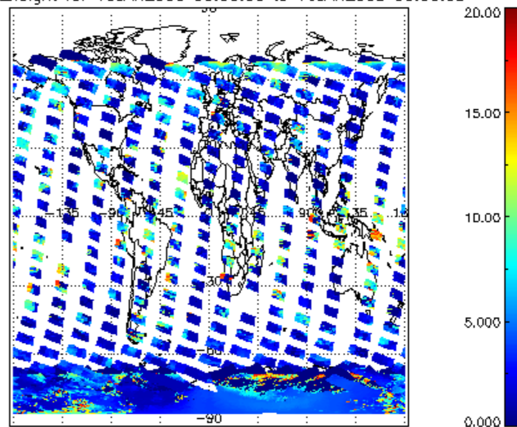
cL_top_height for 15JAN2008 00:00:00 to 16JAN2008 00:00:00
