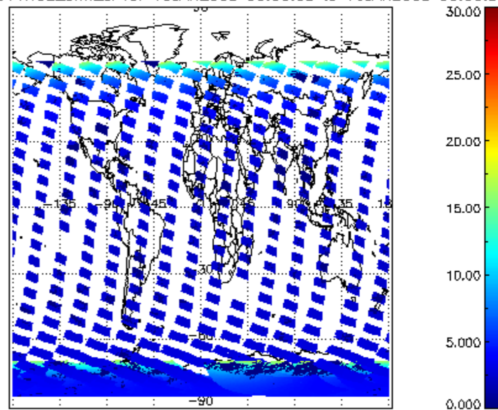
SCIOL2P_NADUV1NO2_amf_cl for 15JAN2008 00:00:00 to 16JAN2008 00:00:00
