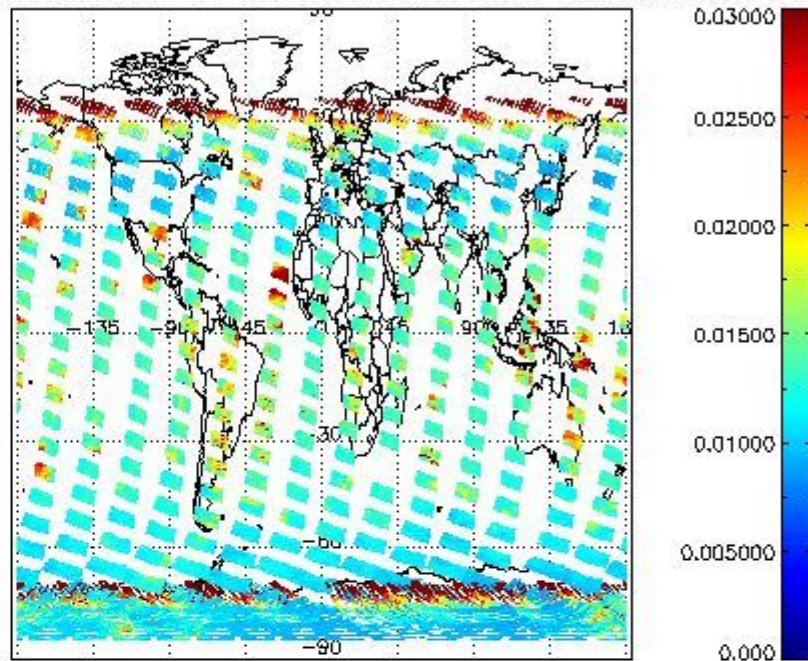
SCIOL2P_NADUV003_vcd_err for 15JAN2008 00:00:00 to 16JAN2008 00:00:00
