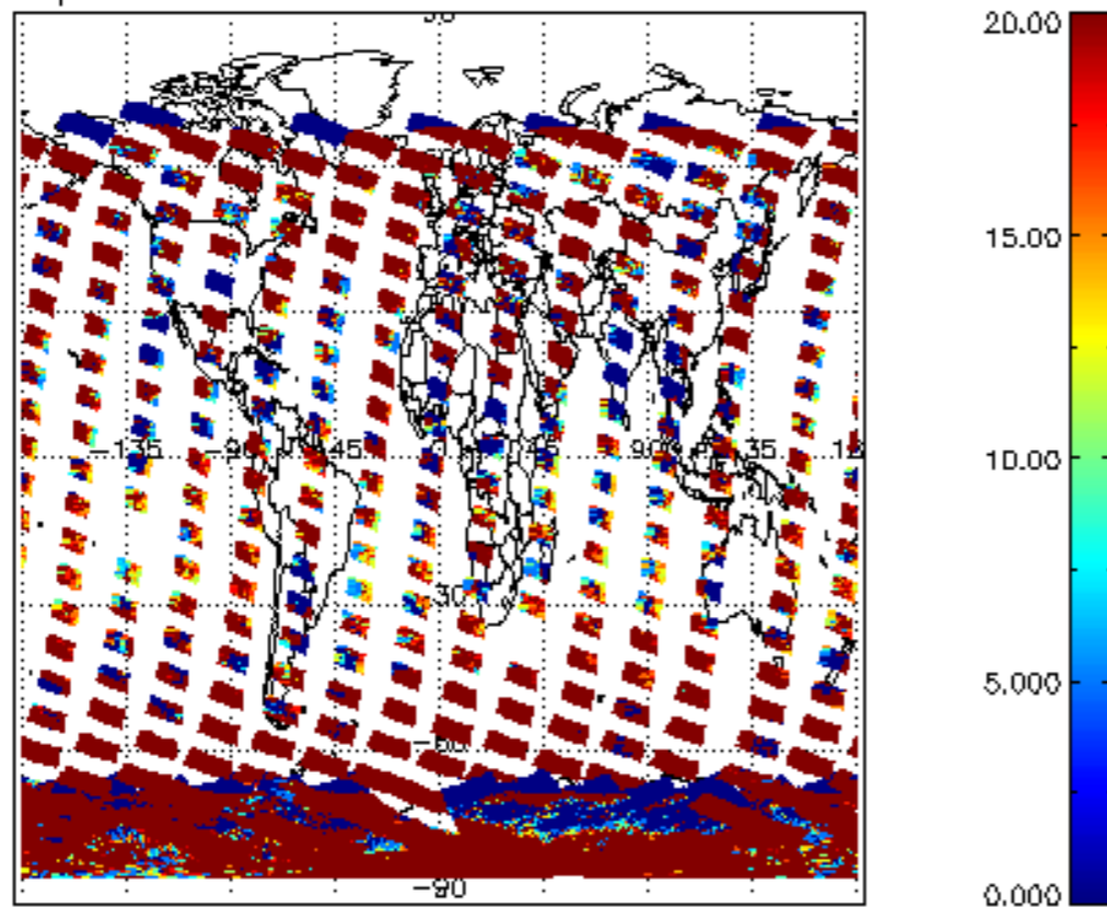
cLopt_depth for 15JAN2008 00:00:00 to 16JAN2008 00:00:00
