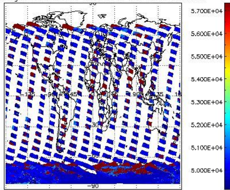
cloud_flags for 15JAN2008 00:00:00 to 16JAN2008 00:00:00
