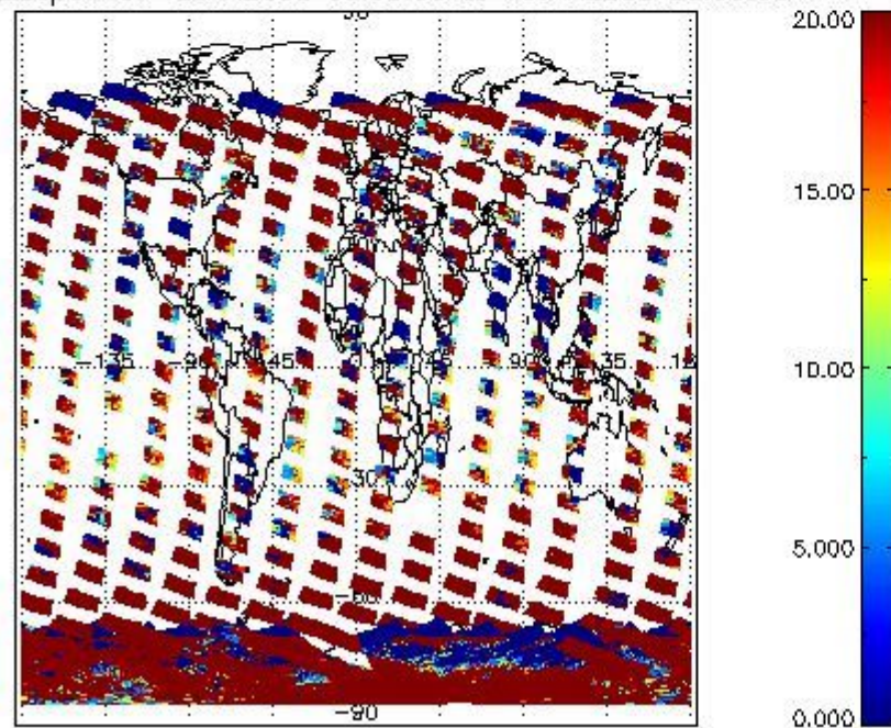
cLopt_depth for 15JAN2008 00:00:00 to 16JAN2008 00:00:00
