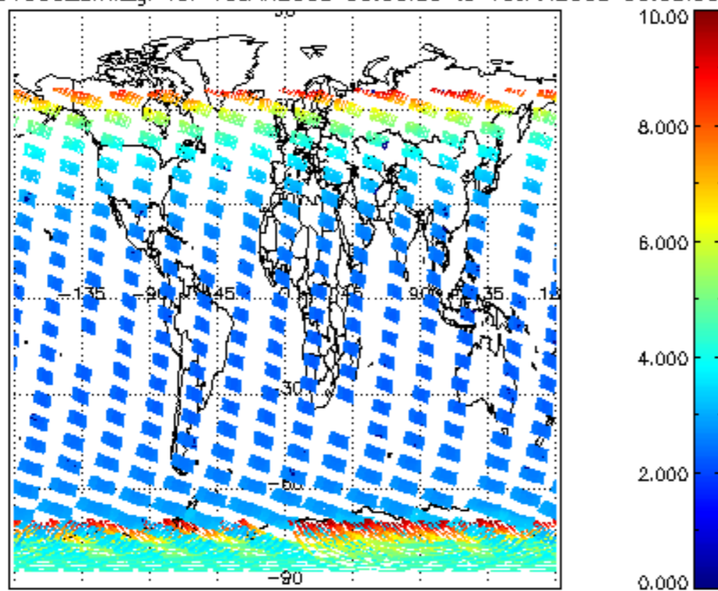
SCIOL2P_NADUV003_amf_gr for 15JAN2008 00:00:00 to 16JAN2008 00:00:00
