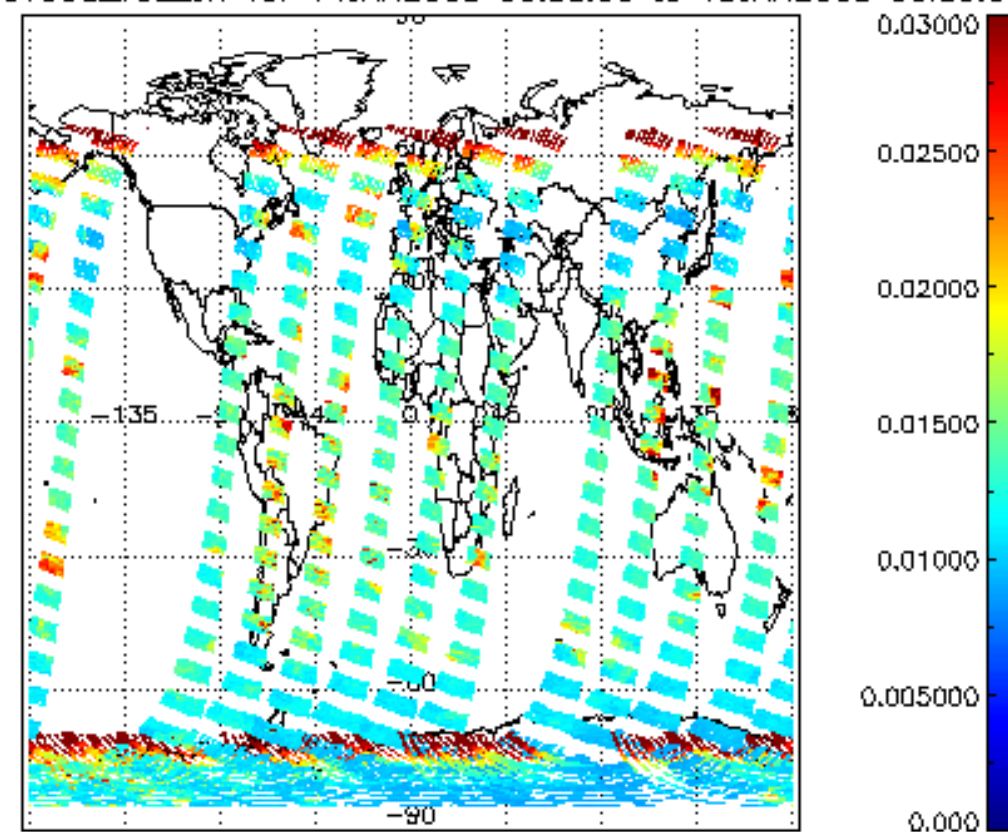
SCIOL2P_NADUV003_vcd_err for 14JAN2008 00:00:00 to 15JAN2008 00:00:00
