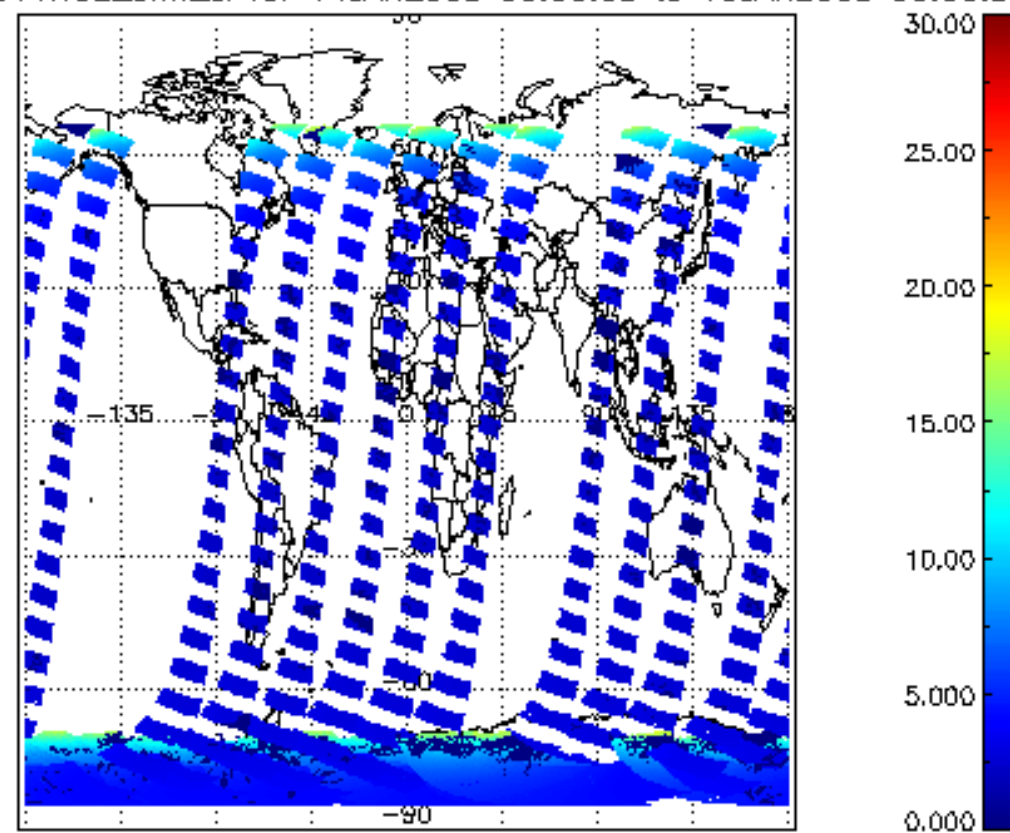
SCIOL2P_NADUV1NO2_amf_cl for 14JAN2008 00:00:00 to 15JAN2008 00:00:00
