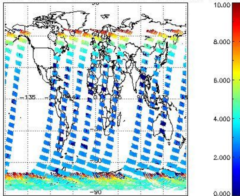
SCIOL2P_NADUV003_amf_cl for 14JAN2008 00:00:00 to 15JAN2008 00:00:00
