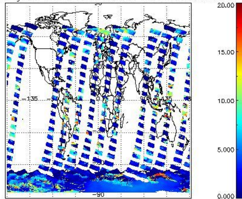
cL_top_height for 14JAN2008 00:00:00 to 15JAN2008 00:00:00
