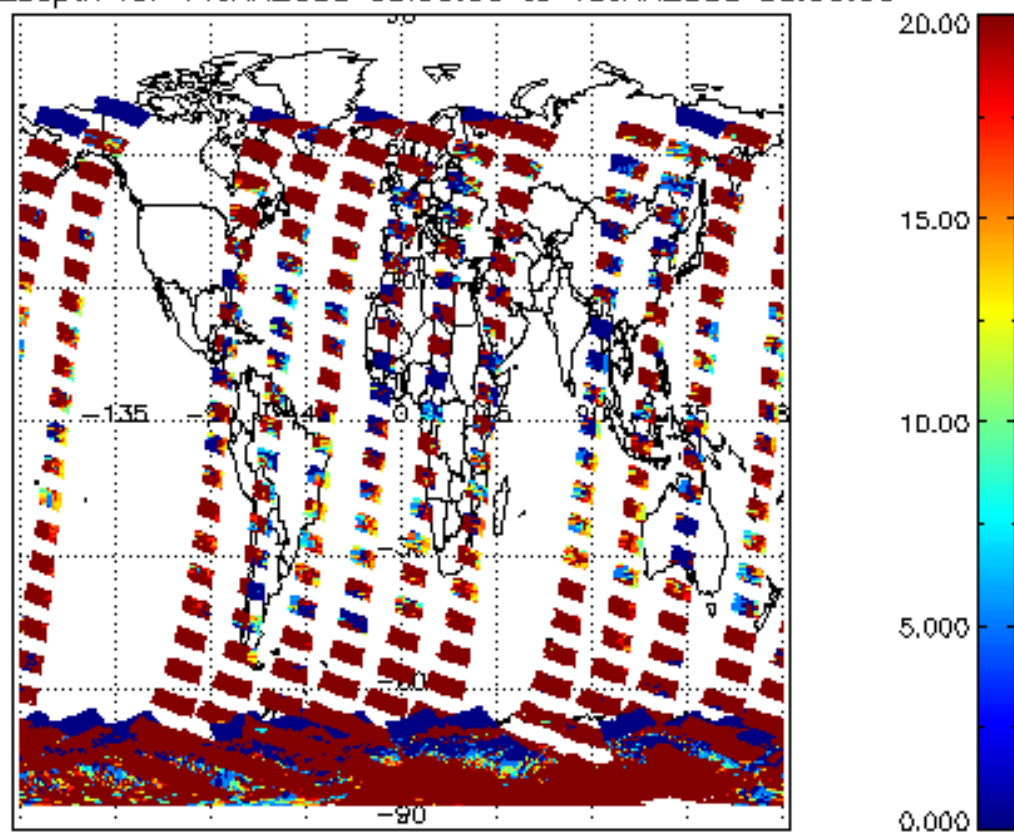
cL_opt_depth for 14JAN2008 00:00:00 to 15JAN2008 00:00:00
