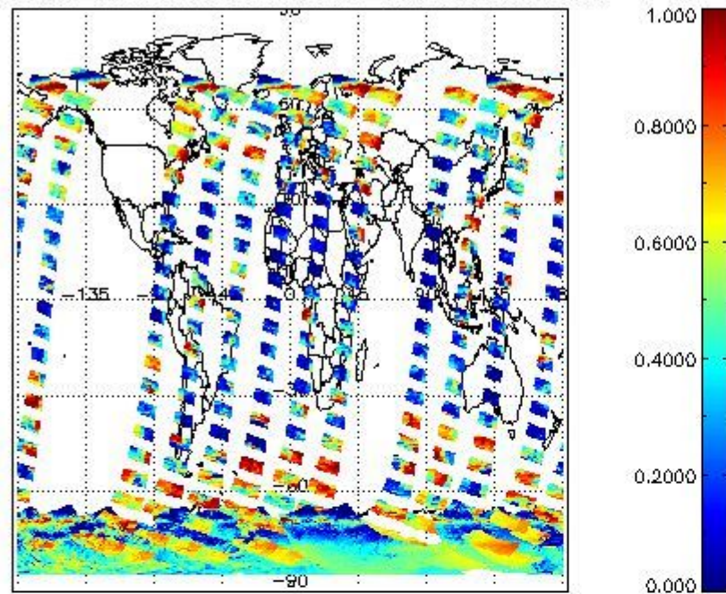
cL_frac for 14JAN2008 00:00:00 to 15JAN2008 00:00:00
