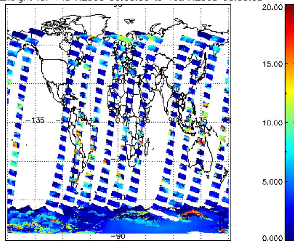
cL_top_height for 14JAN2008 00:00:00 to 15JAN2008 00:00:00
