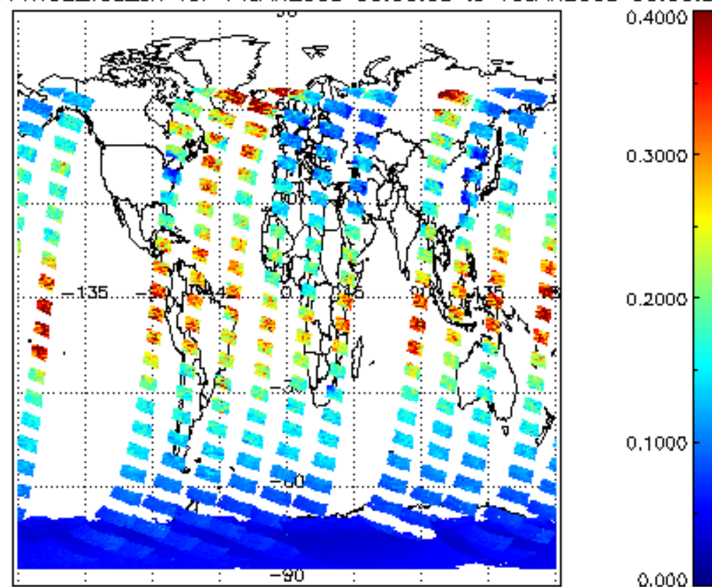
SCIOL2P_NADUV1NO2_vcd_err for 14JAN2008 00:00:00 to 15JAN2008 00:00:00
