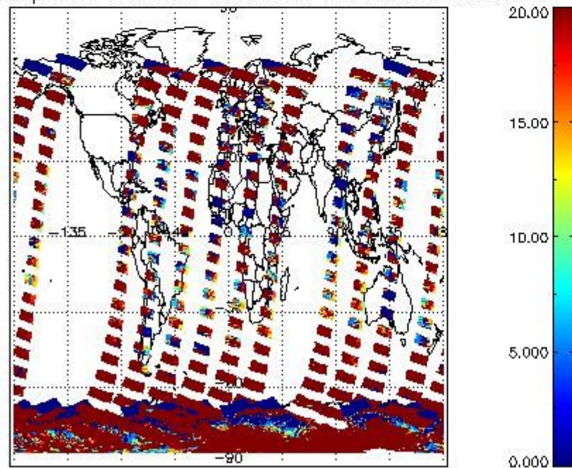
cLopt_depth for 14JAN2008 00:00:00 to 15JAN2008 00:00:00
