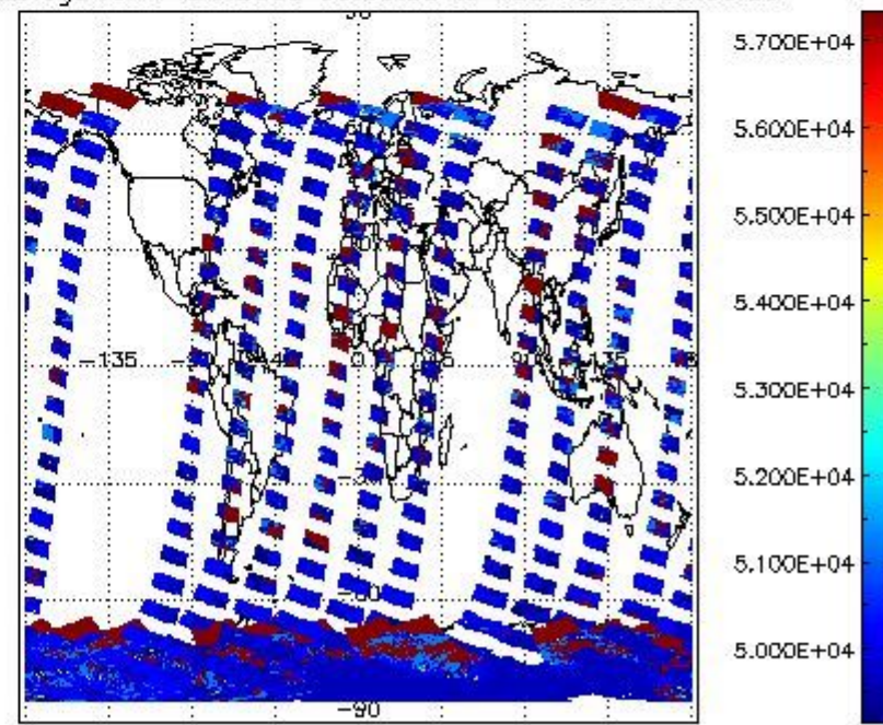
cloud_flags for 14JAN2008 00:00:00 to 15JAN2008 00:00:00
