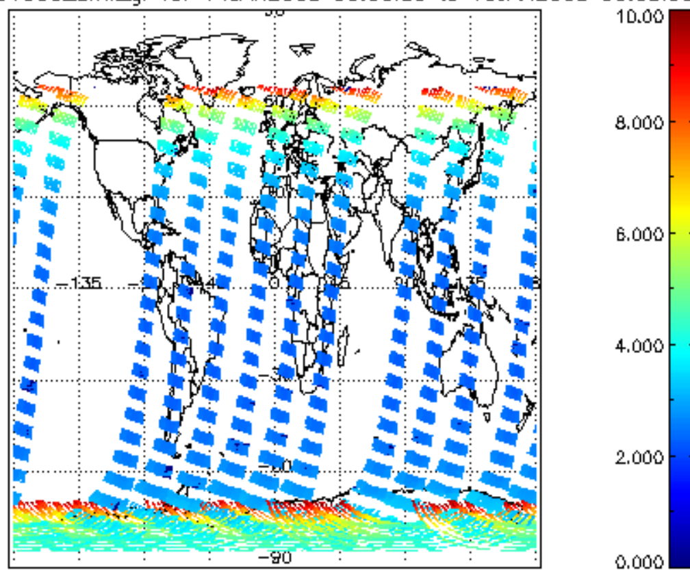
SCIOL2P_NADUV003_amf_gr for 14JAN2008 00:00:00 to 15JAN2008 00:00:00
