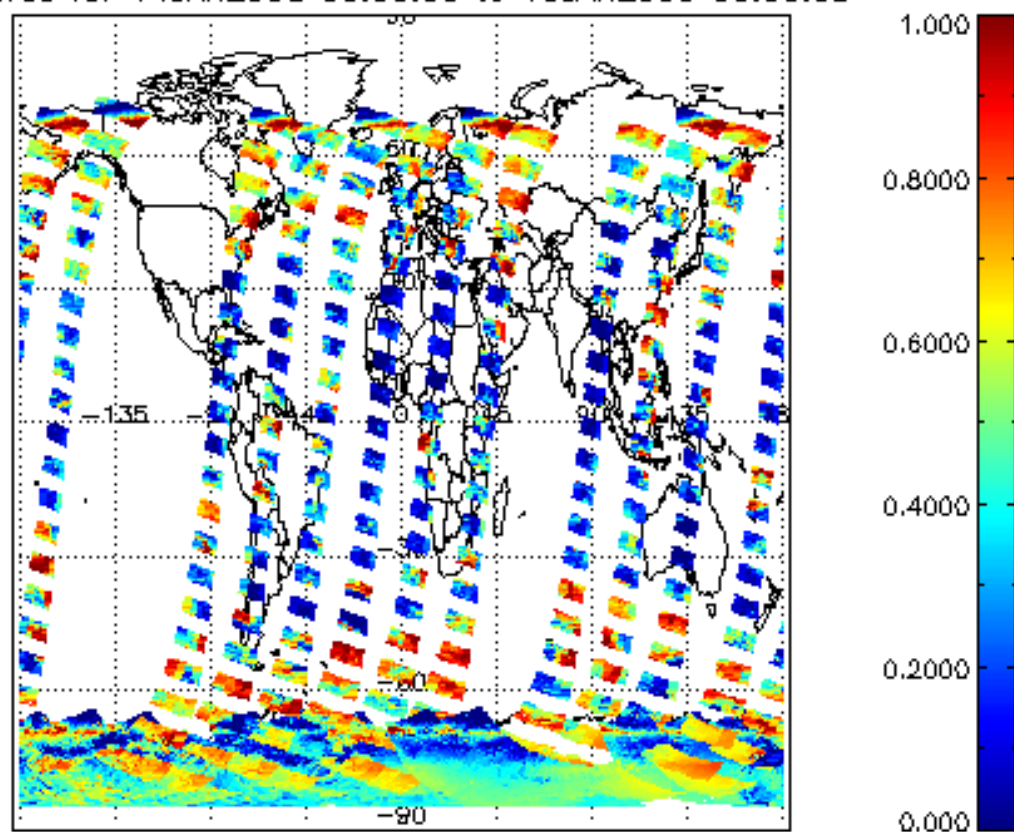
cL_frac for 14JAN2008 00:00:00 to 15JAN2008 00:00:00
