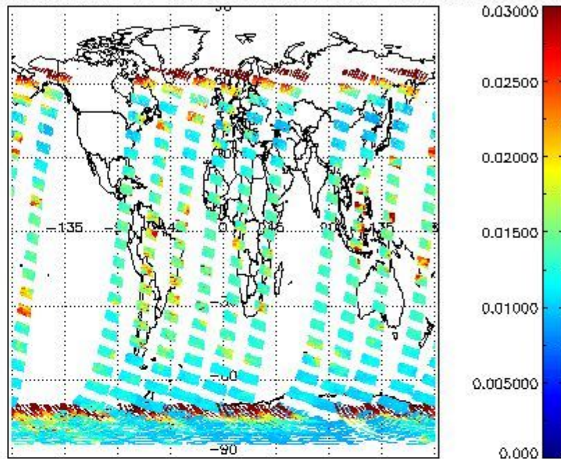
SCIOL2P_NADUV003_vcd_err for 14JAN2008 00:00:00 to 15JAN2008 00:00:00
