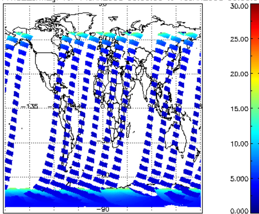
SCIOL2P_NADUV1NO2_amf_gr for 14JAN2008 00:00:00 to 15JAN2008 00:00:00
