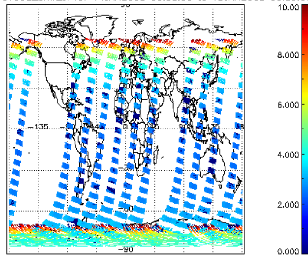
SCIOL2P_NADUV003_amf_cl for 14JAN2008 00:00:00 to 15JAN2008 00:00:00
