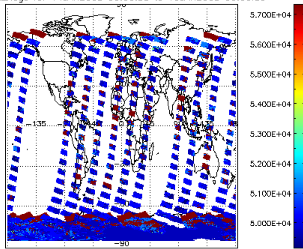
cloud_flags for 14JAN2008 00:00:00 to 15JAN2008 00:00:00
