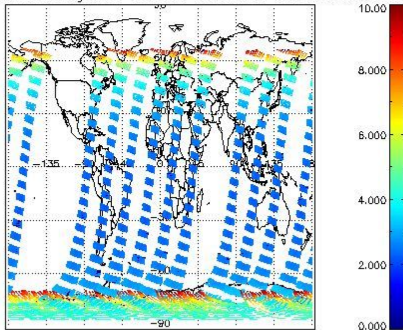
SCIOL2P_NADUV003_amf_gr for 14JAN2008 00:00:00 to 15JAN2008 00:00:00
