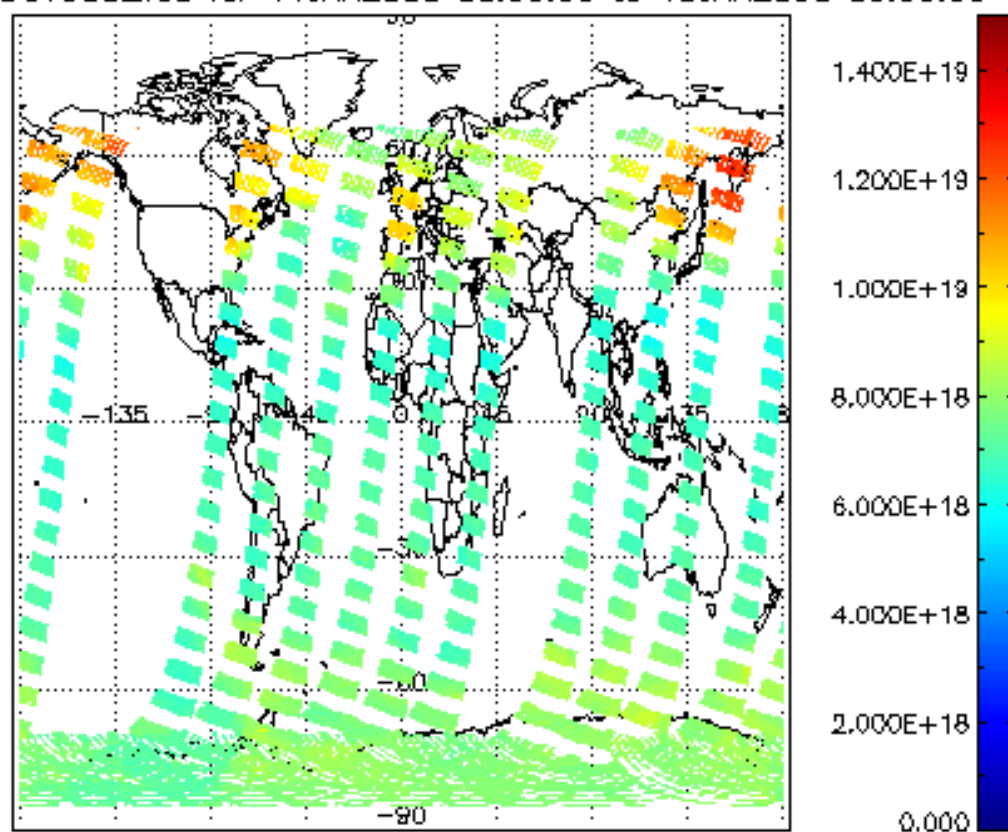
SCIOL2P_NADUV003_vcd for 14JAN2008 00:00:00 to 15JAN2008 00:00:00
