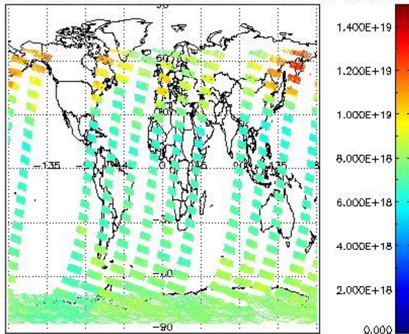
SCIOL2P_NADUV003_vcd for 14JAN2008 00:00:00 to 15JAN2008 00:00:00
