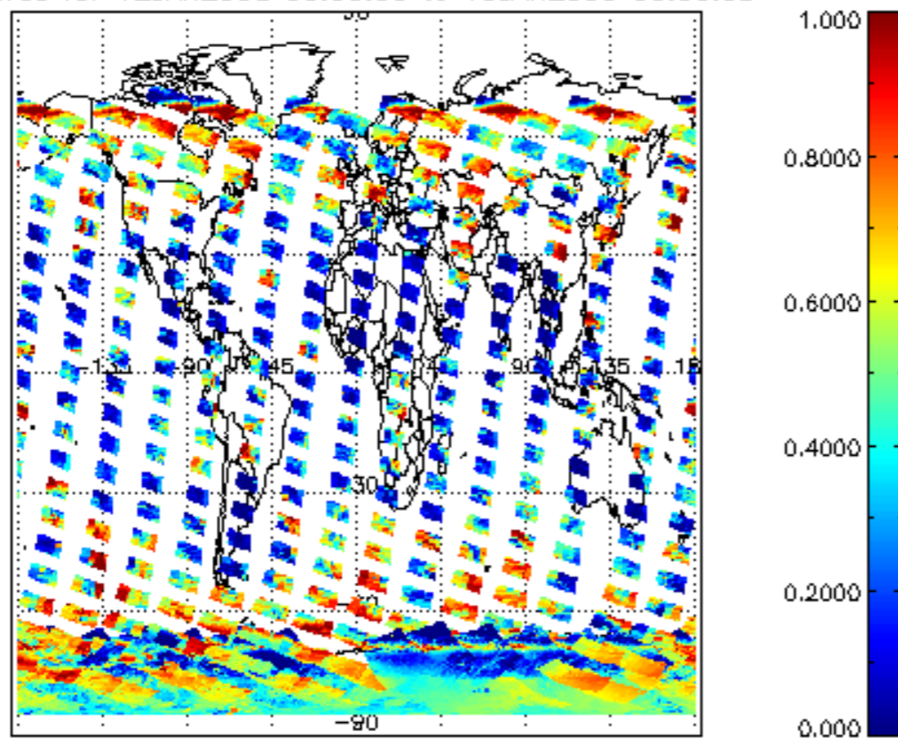
cL_frac for 12JAN2008 00:00:00 to 13JAN2008 00:00:00
