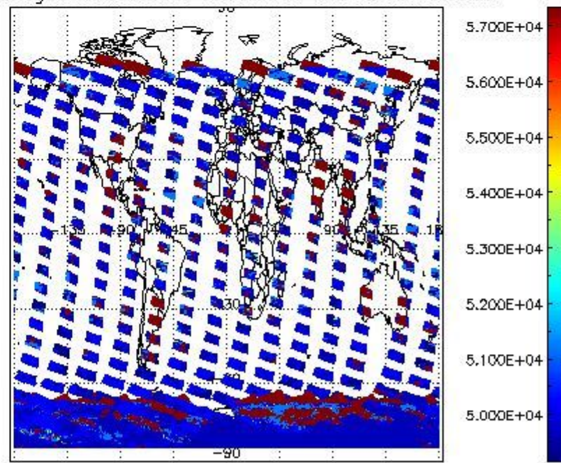
cloud_flags for 12JAN2008 00:00:00 to 13JAN2008 00:00:00
