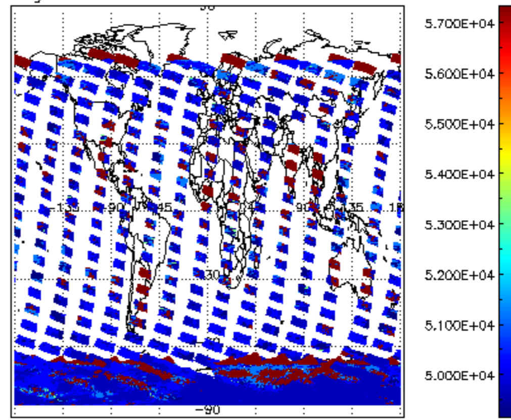
cloud_flags for 12JAN2008 00:00:00 to 13JAN2008 00:00:00
