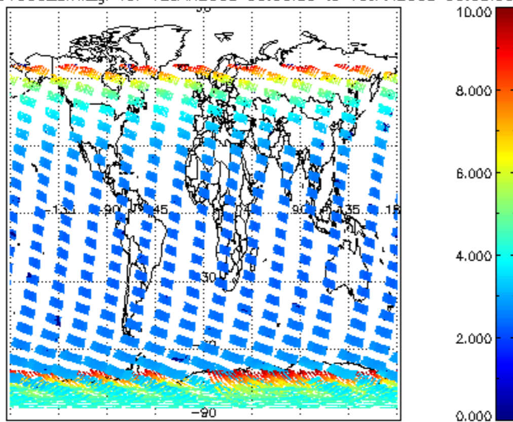
SCIOL2P_NADUV003_amf_gr for 12JAN2008 00:00:00 to 13JAN2008 00:00:00
