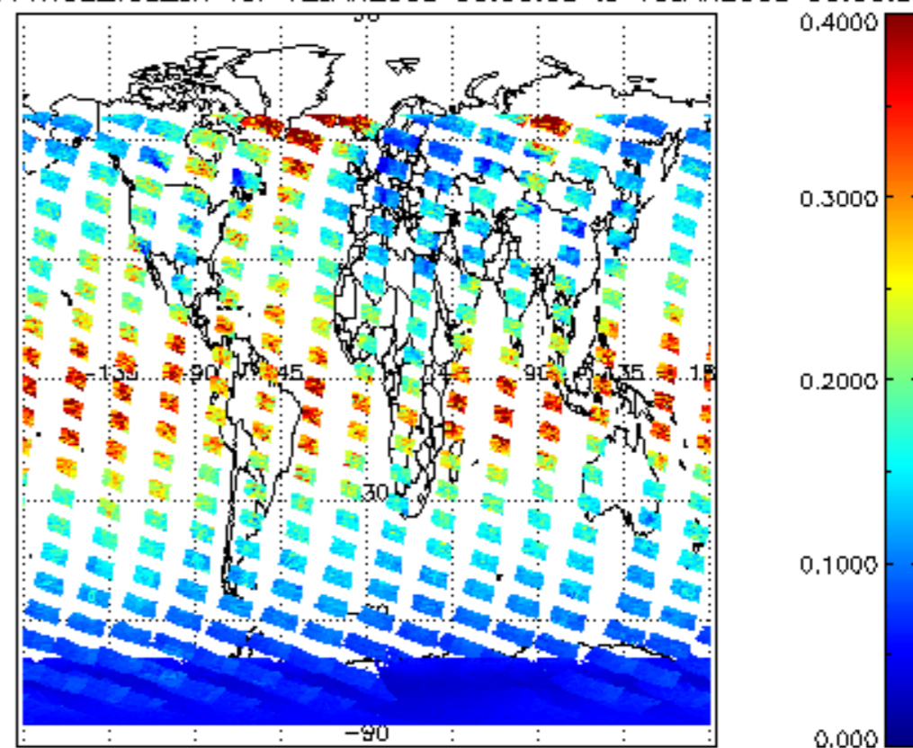
SCIOL2P_NADUV1NO2_vcd_err for 12JAN2008 00:00:00 to 13JAN2008 00:00:00
