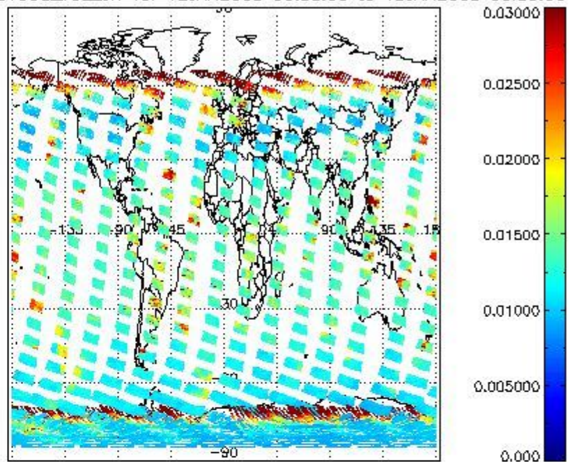
SCIOL2P_NADUV003_vcd_err for 12JAN2008 00:00:00 to 13JAN2008 00:00:00
