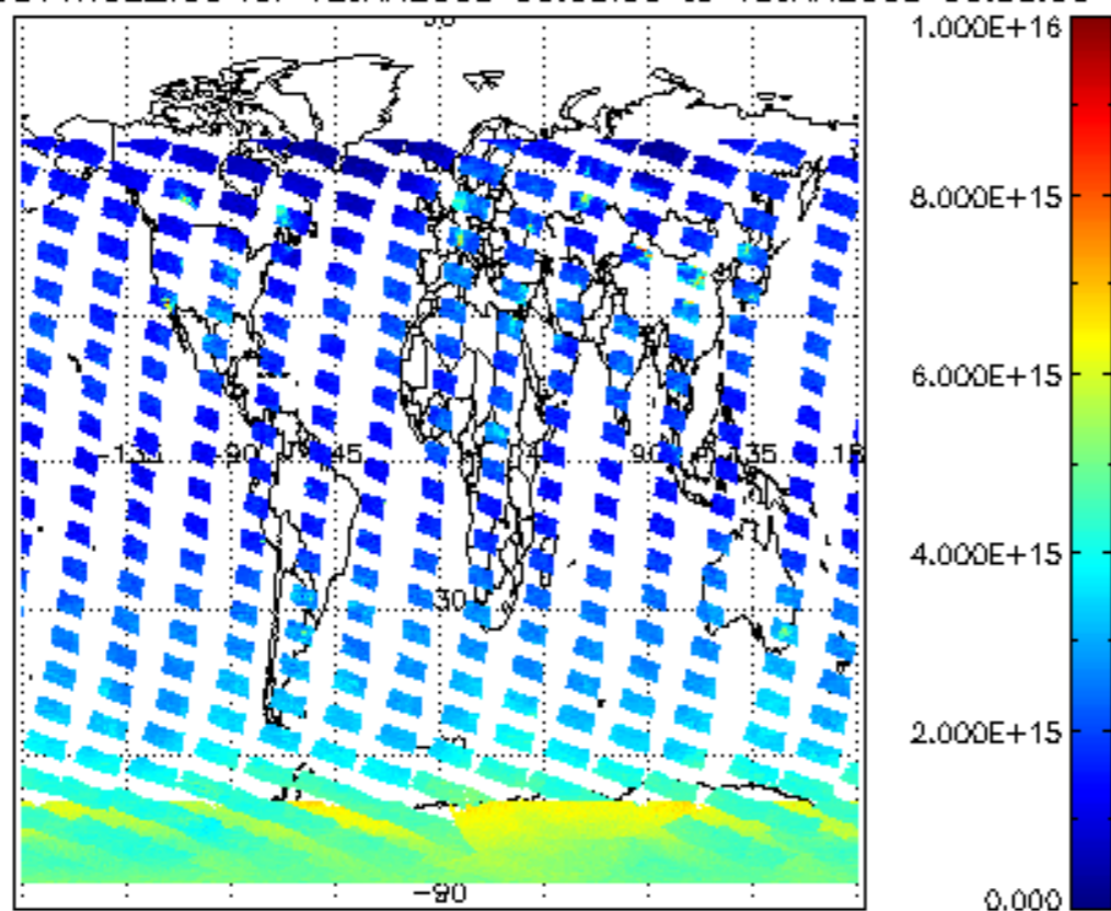
SCIOL2P_NADUV1NO2_vcd for 12JAN2008 00:00:00 to 13JAN2008 00:00:00
