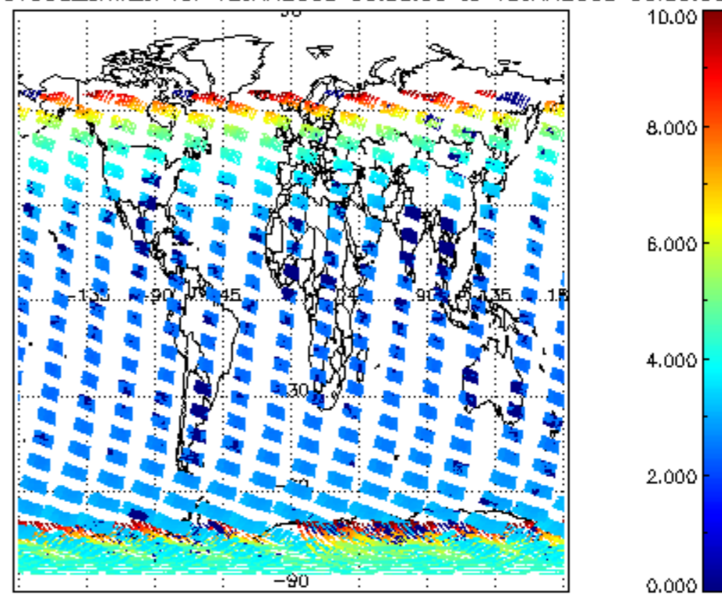
SCIOL2P_NADUV003_amf_cl for 12JAN2008 00:00:00 to 13JAN2008 00:00:00
