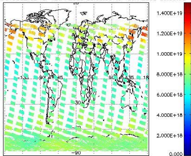
SCIOL2P_NADUV003_vcd for 12JAN2008 00:00:00 to 13JAN2008 00:00:00
