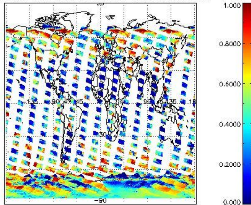
cL_frac for 12JAN2008 00:00:00 to 13JAN2008 00:00:00
