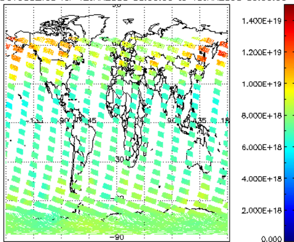
SCIOL2P_NADUV003_vcd for 12JAN2008 00:00:00 to 13JAN2008 00:00:00
