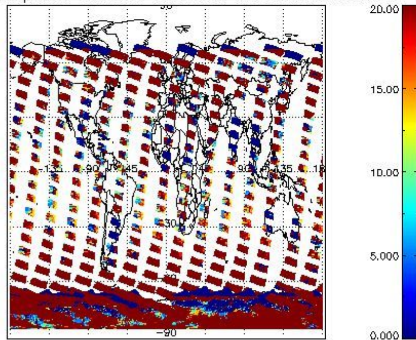
cLopt_depth for 12JAN2008 00:00:00 to 13JAN2008 00:00:00
