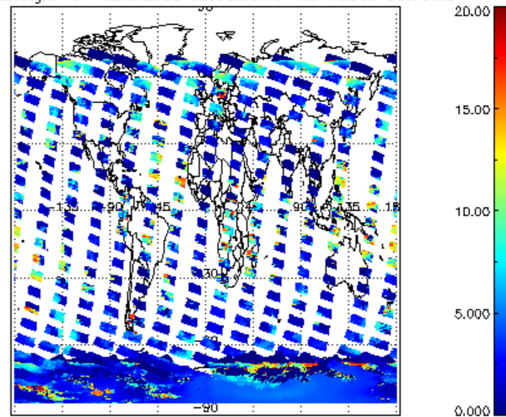
cL_top_height for 12JAN2008 00:00:00 to 13JAN2008 00:00:00
