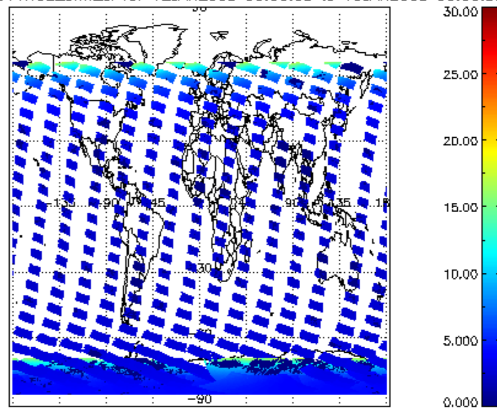
SCIOL2P_NADUV1NO2_amf_cl for 12JAN2008 00:00:00 to 13JAN2008 00:00:00
