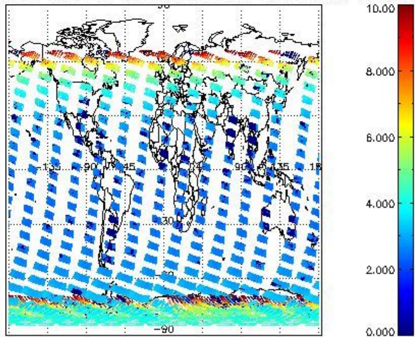
SCIOL2P_NADUV003_amf_cl for 12JAN2008 00:00:00 to 13JAN2008 00:00:00
