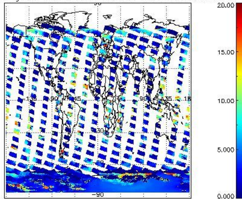
cL_top_height for 12JAN2008 00:00:00 to 13JAN2008 00:00:00
