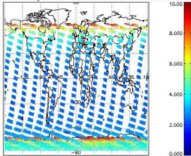
SCIOL2P_NADUV003_amf_gr for 12JAN2008 00:00:00 to 13JAN2008 00:00:00
