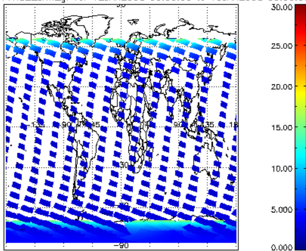
SCIOL2P_NADUV1NO2_amf_gr for 12JAN2008 00:00:00 to 13JAN2008 00:00:00
