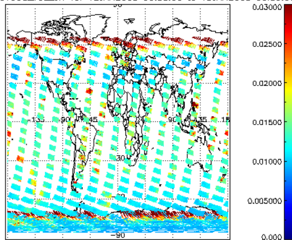
SCIOL2P_NADUV003_vcd_err for 12JAN2008 00:00:00 to 13JAN2008 00:00:00
