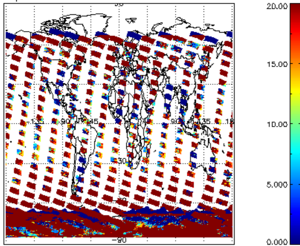
cLopt_depth for 12JAN2008 00:00:00 to 13JAN2008 00:00:00
