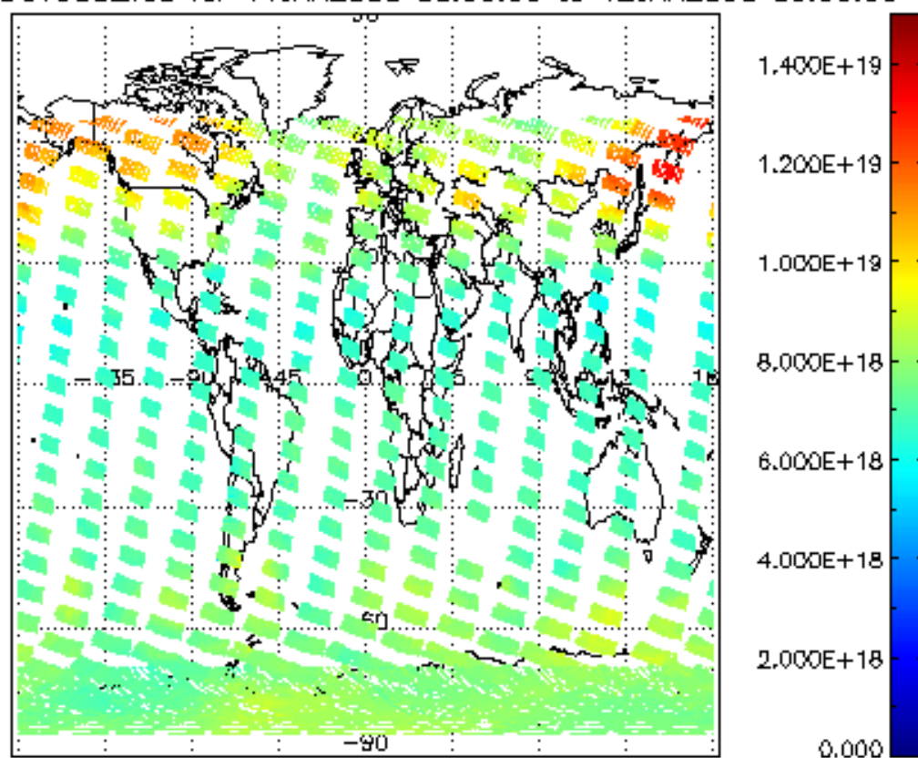
SCIOL2P_NADUV003_vcd for 11JAN2008 00:00:00 to 12JAN2008 00:00:00
