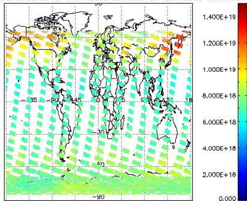
SCIOL2P_NADUV003_vcd for 11JAN2008 00:00:00 to 12JAN2008 00:00:00
