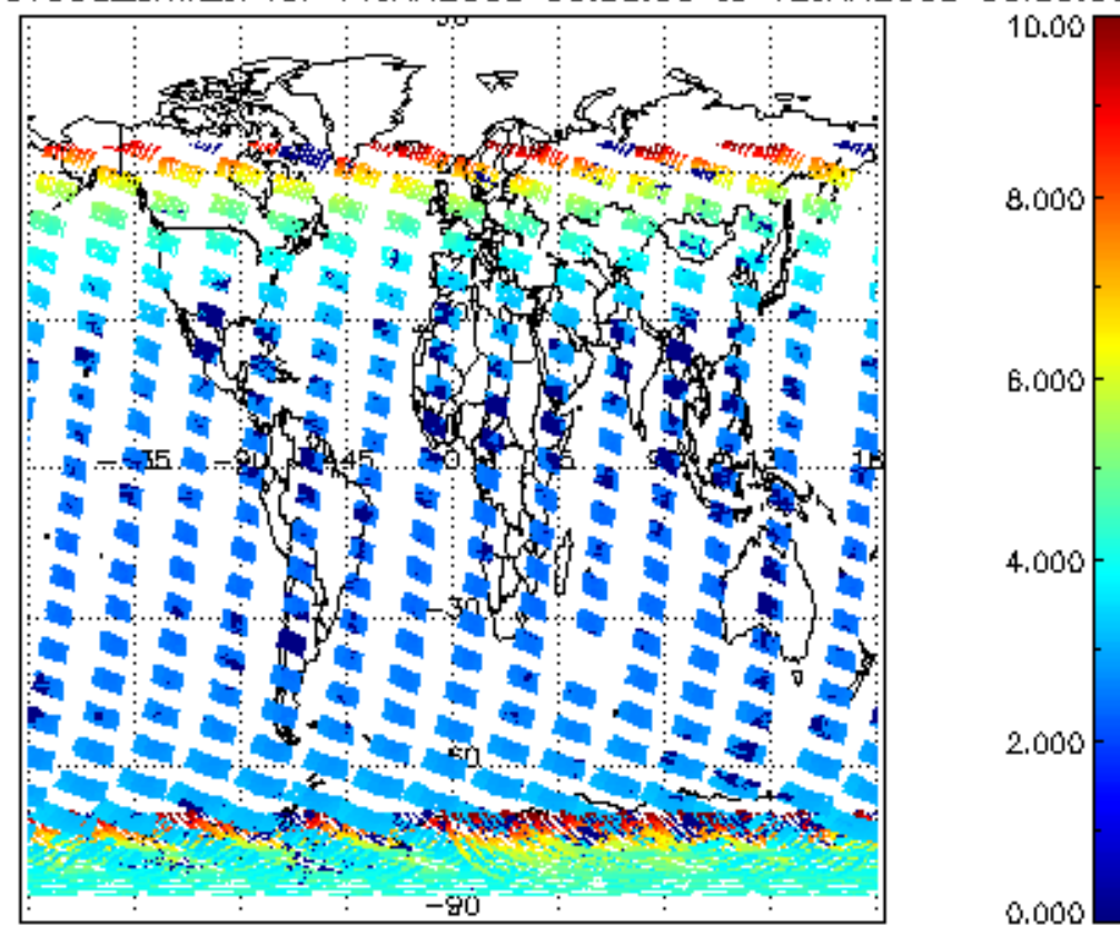
SCIOL2P_NADUV003_amf_cl for 11JAN2008 00:00:00 to 12JAN2008 00:00:00
