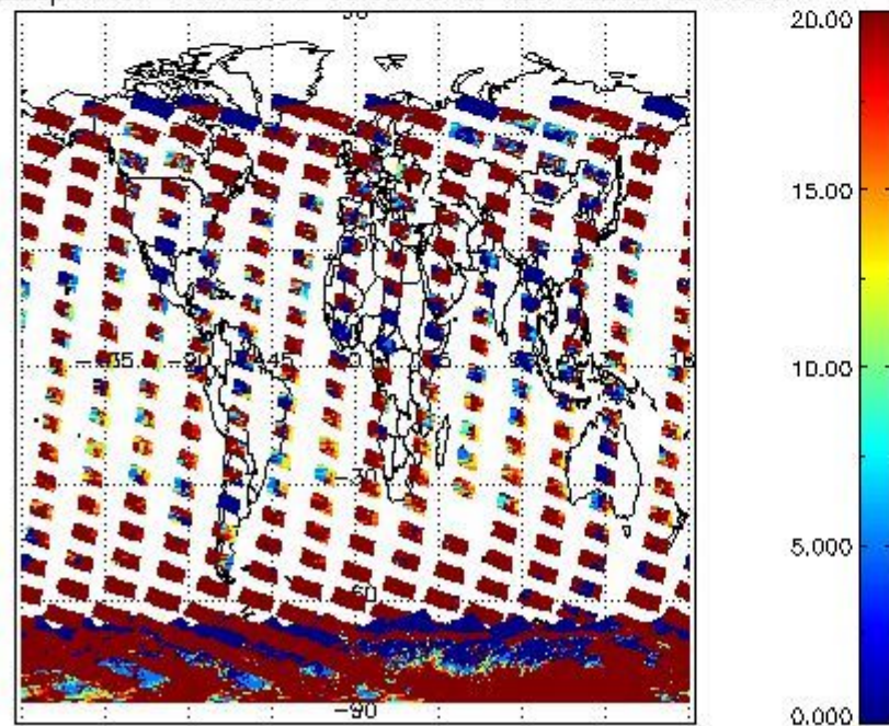
cLopt_depth for 11JAN2008 00:00:00 to 12JAN2008 00:00:00
