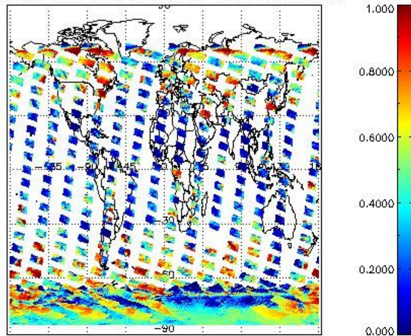
cL_frac for 11JAN2008 00:00:00 to 12JAN2008 00:00:00
