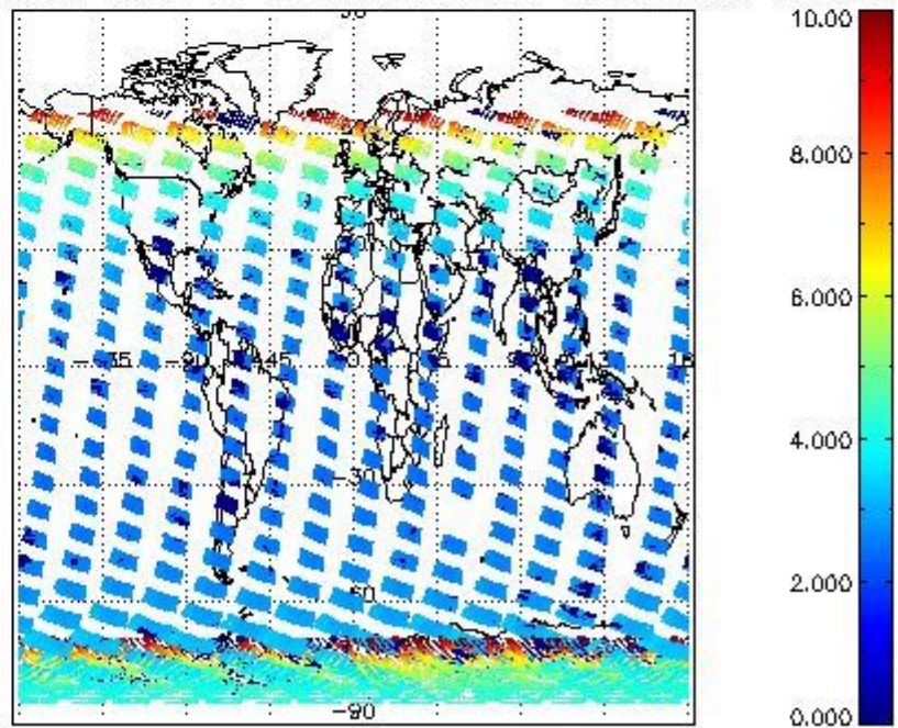
SCIOL2P_NADUV003_amf_cl for 11JAN2008 00:00:00 to 12JAN2008 00:00:00
