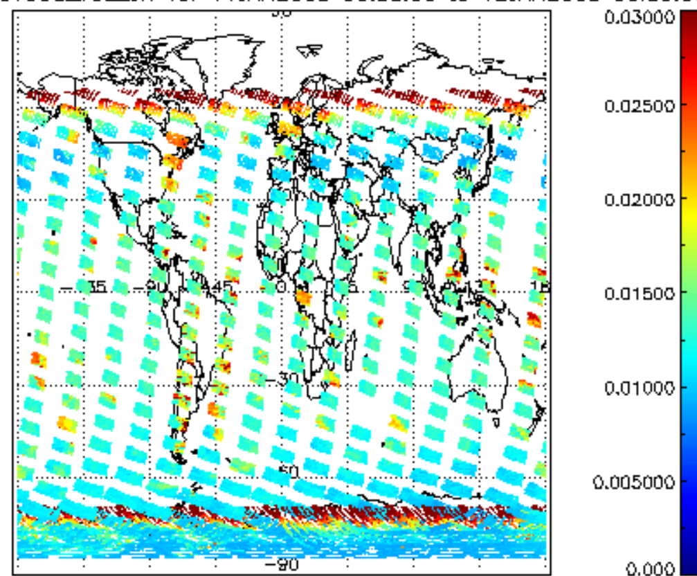
SCIOL2P_NADUV003_vcd_err for 11JAN2008 00:00:00 to 12JAN2008 00:00:00
