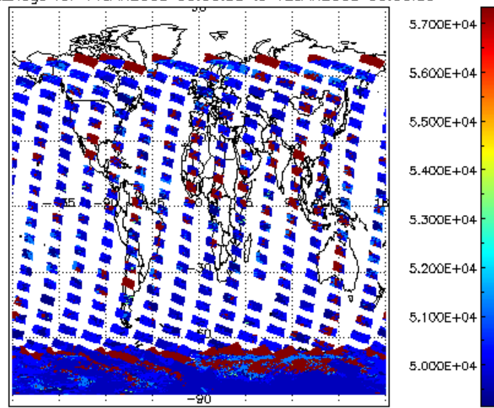
cloud_flags for 11JAN2008 00:00:00 to 12JAN2008 00:00:00
