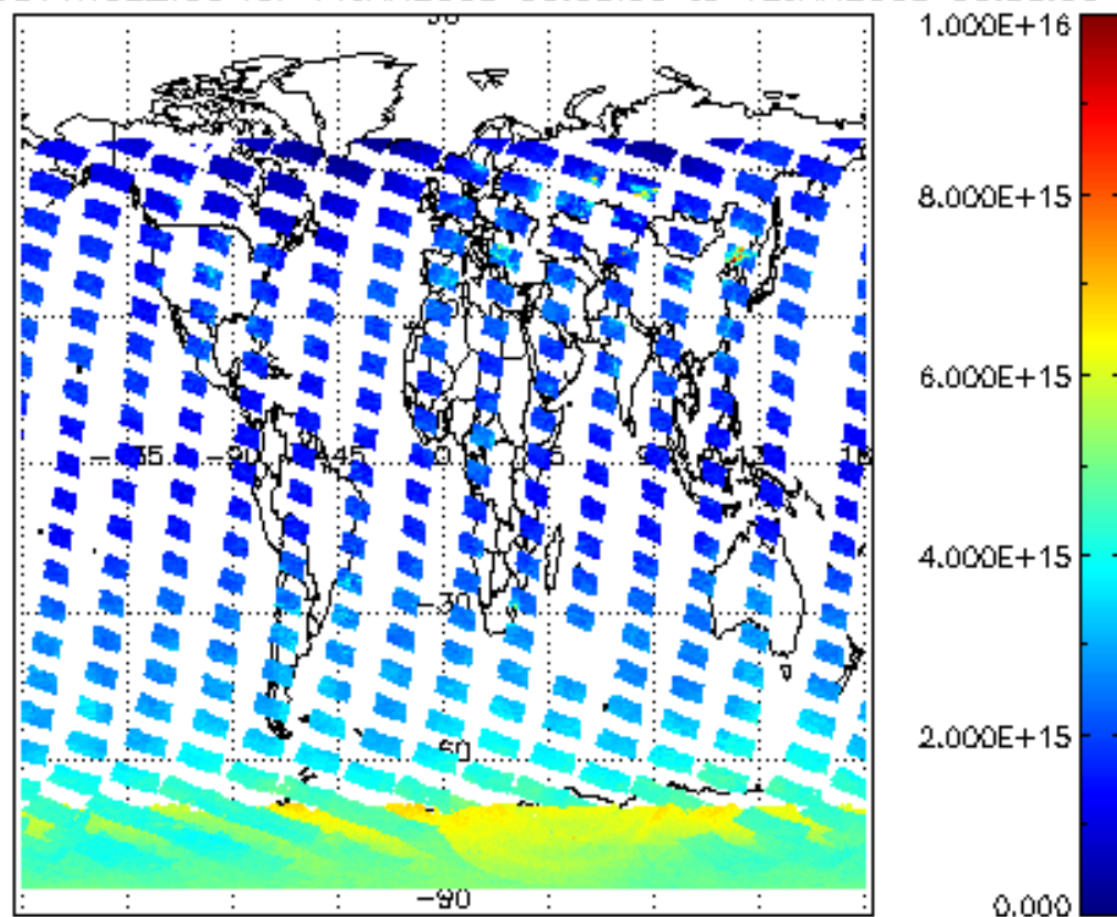
SCIOL2P_NADUV1NO2_vcd for 11JAN2008 00:00:00 to 12JAN2008 00:00:00
