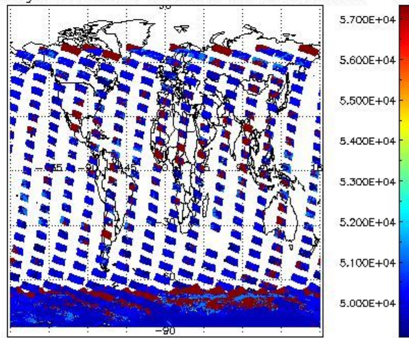
cloud_flags for 11JAN2008 00:00:00 to 12JAN2008 00:00:00
