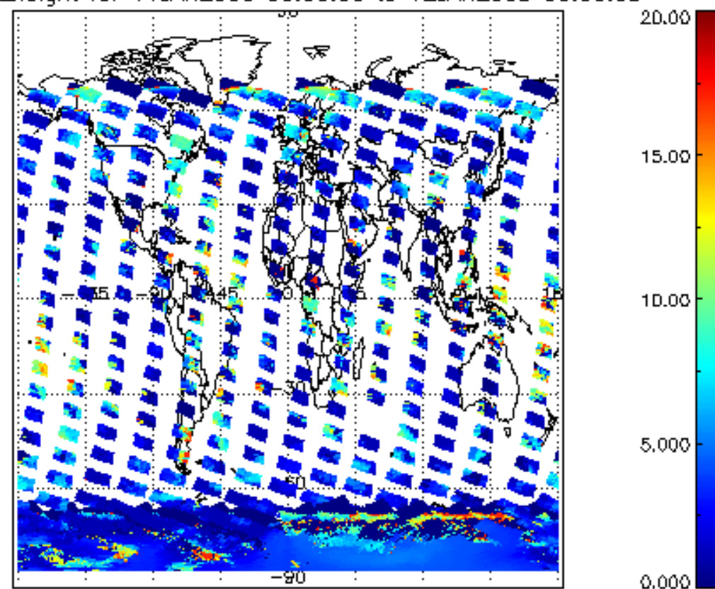
cL_top_height for 11JAN2008 00:00:00 to 12JAN2008 00:00:00
