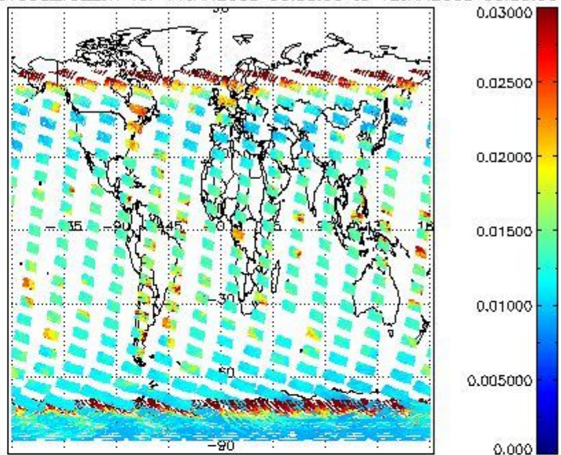
SCIOL2P_NADUV003_vcd_err for 11JAN2008 00:00:00 to 12JAN2008 00:00:00
