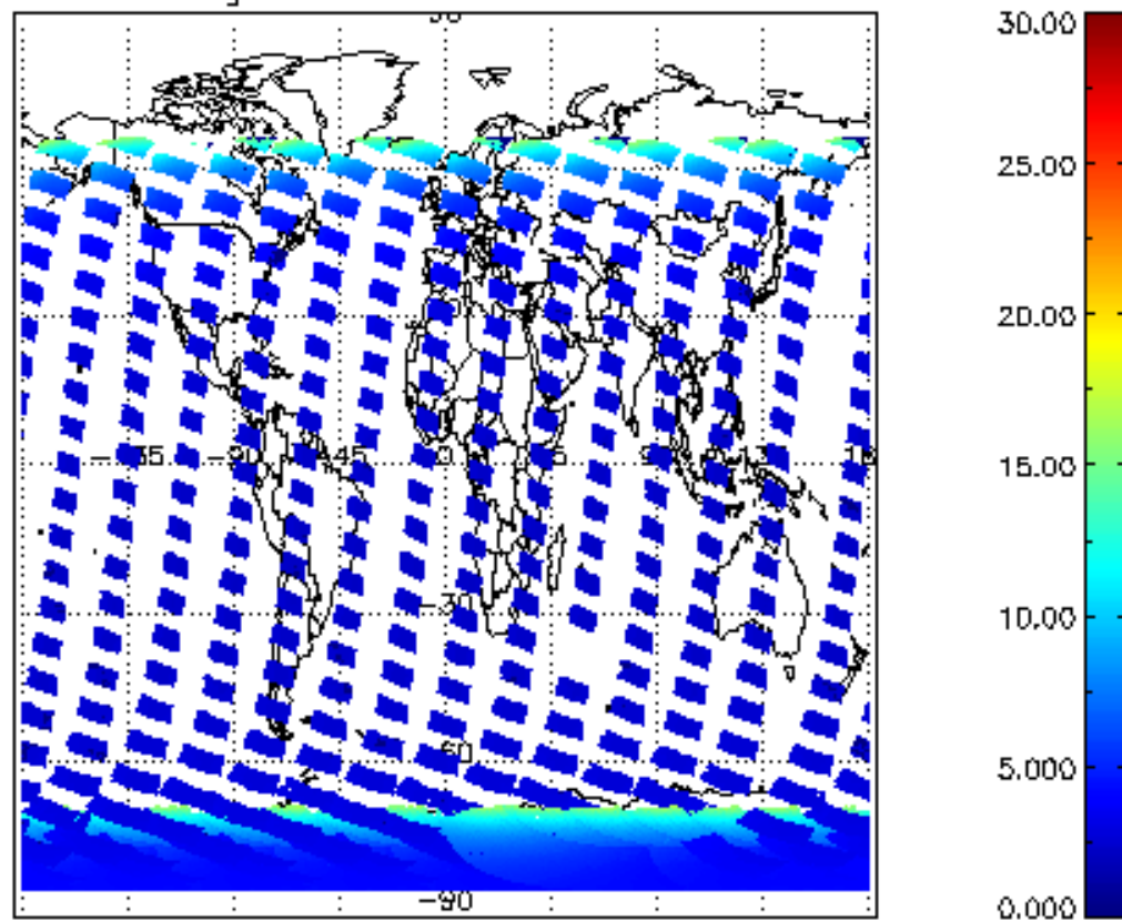
SCIOL2P_NADUV1NO2_amf_gr for 11JAN2008 00:00:00 to 12JAN2008 00:00:00
