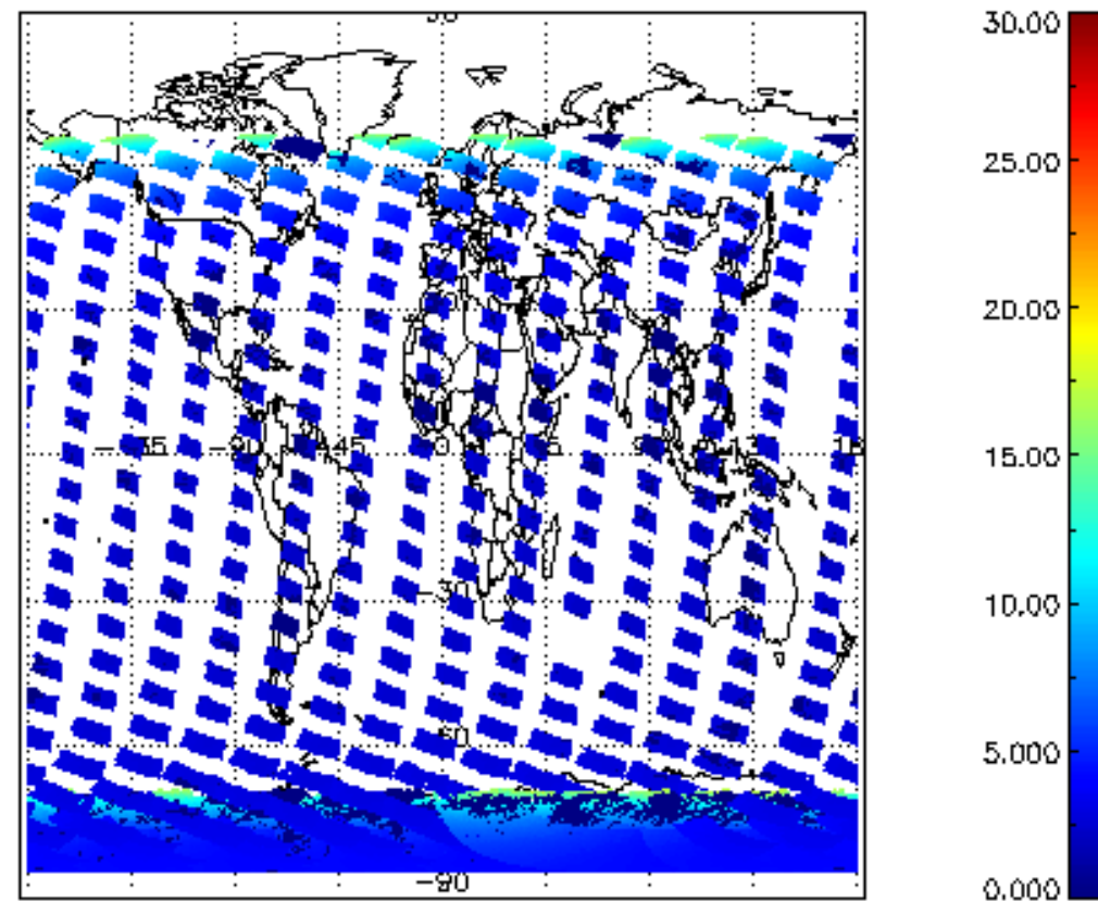
SCIOL2P_NADUV1NO2_amf_cl for 11JAN2008 00:00:00 to 12JAN2008 00:00:00
