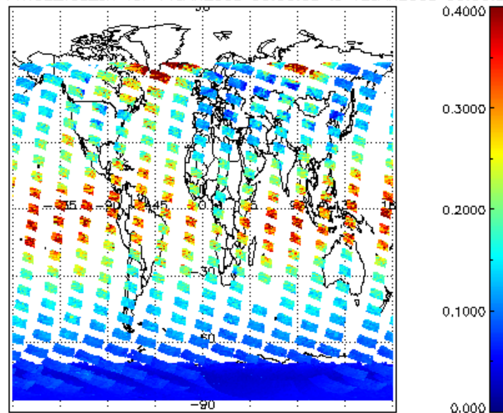
SCIOL2P_NADUV1NO2_vcd_err for 11JAN2008 00:00:00 to 12JAN2008 00:00:00
