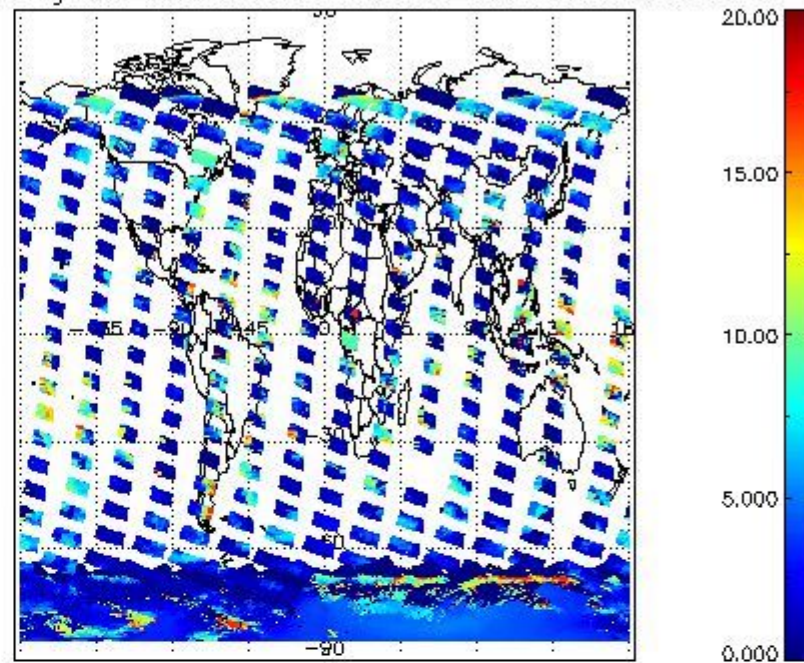
cL_top_height for 11JAN2008 00:00:00 to 12JAN2008 00:00:00
