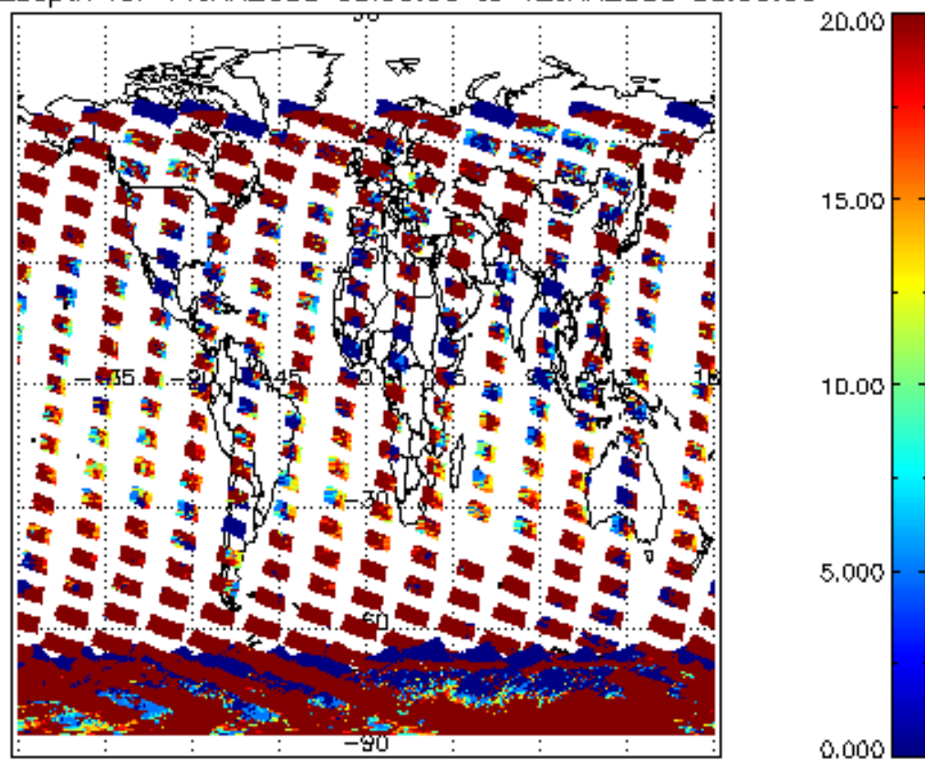
cLopt_depth for 11JAN2008 00:00:00 to 12JAN2008 00:00:00
