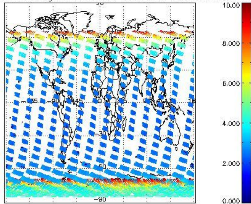
SCIOL2P_NADUV003_amf_gr for 11JAN2008 00:00:00 to 12JAN2008 00:00:00
