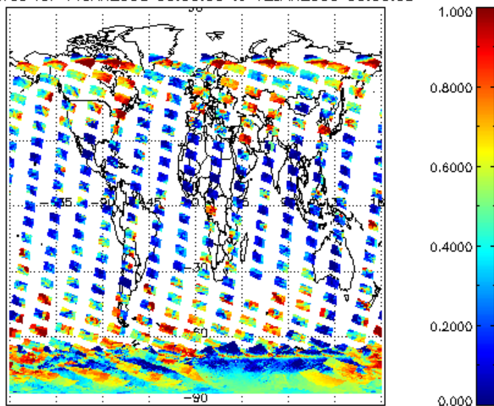
cL_frac for 11JAN2008 00:00:00 to 12JAN2008 00:00:00
