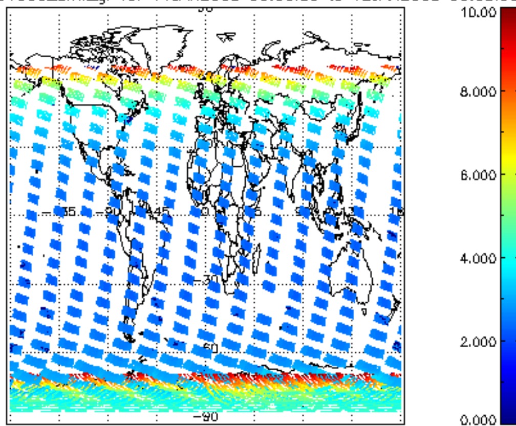
SCIOL2P_NADUV003_amf_gr for 11JAN2008 00:00:00 to 12JAN2008 00:00:00
