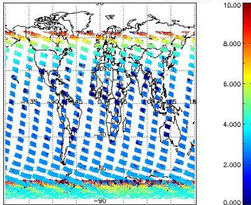
SCIOL2P_NADUV003_amf_cl for 10JAN2008 00:00:00 to 11JAN2008 00:00:00
