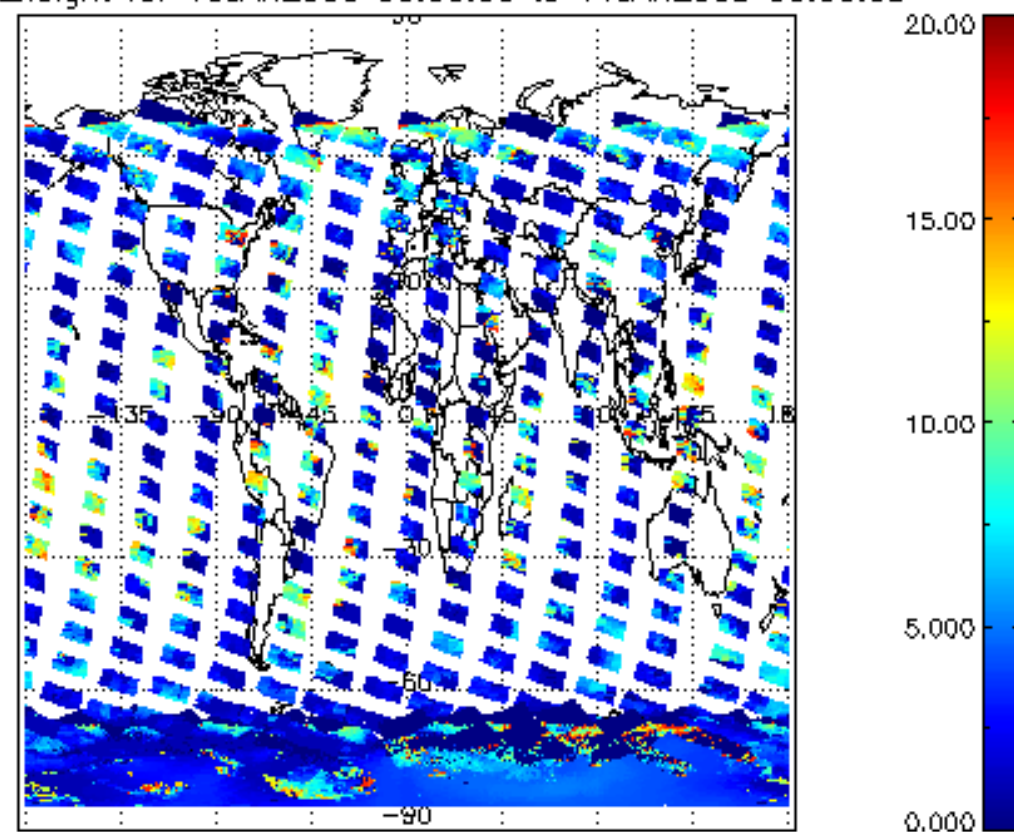
cL_top_height for 10JAN2008 00:00:00 to 11JAN2008 00:00:00
