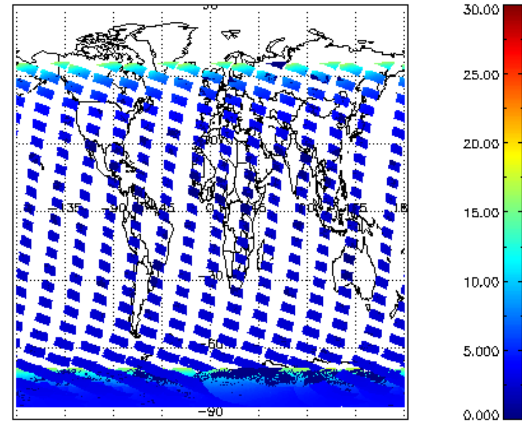
SCIOL2P_NADUV1NO2_amf_cl for 10JAN2008 00:00:00 to 11JAN2008 00:00:00
