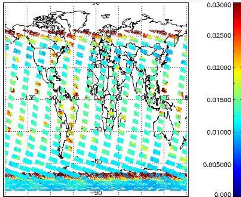
SCIOL2P_NADUV003_vcd_err for 10JAN2008 00:00:00 to 11JAN2008 00:00:00
