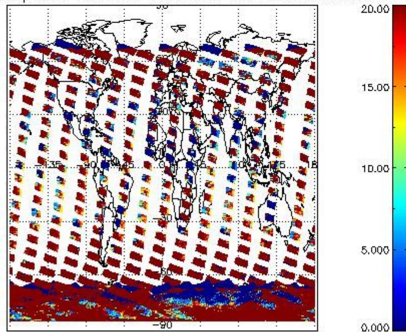
cLopt_depth for 10JAN2008 00:00:00 to 11JAN2008 00:00:00
