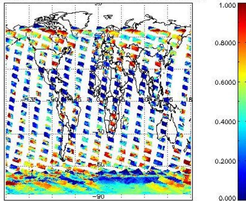
cL_frac for 10JAN2008 00:00:00 to 11JAN2008 00:00:00
