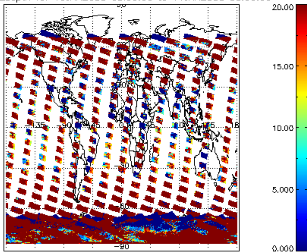
cLopt_depth for 10JAN2008 00:00:00 to 11JAN2008 00:00:00
