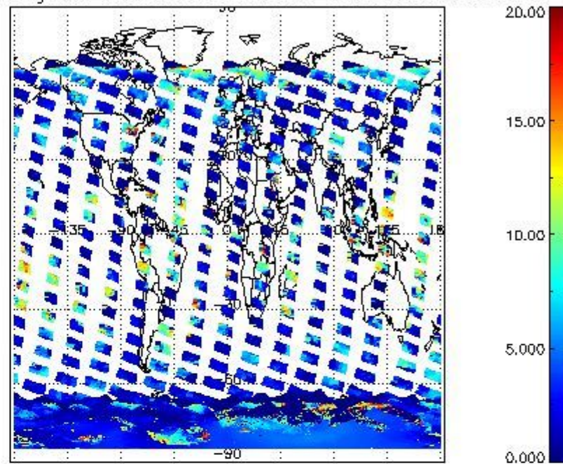
cL_top_height for 10JAN2008 00:00:00 to 11JAN2008 00:00:00
