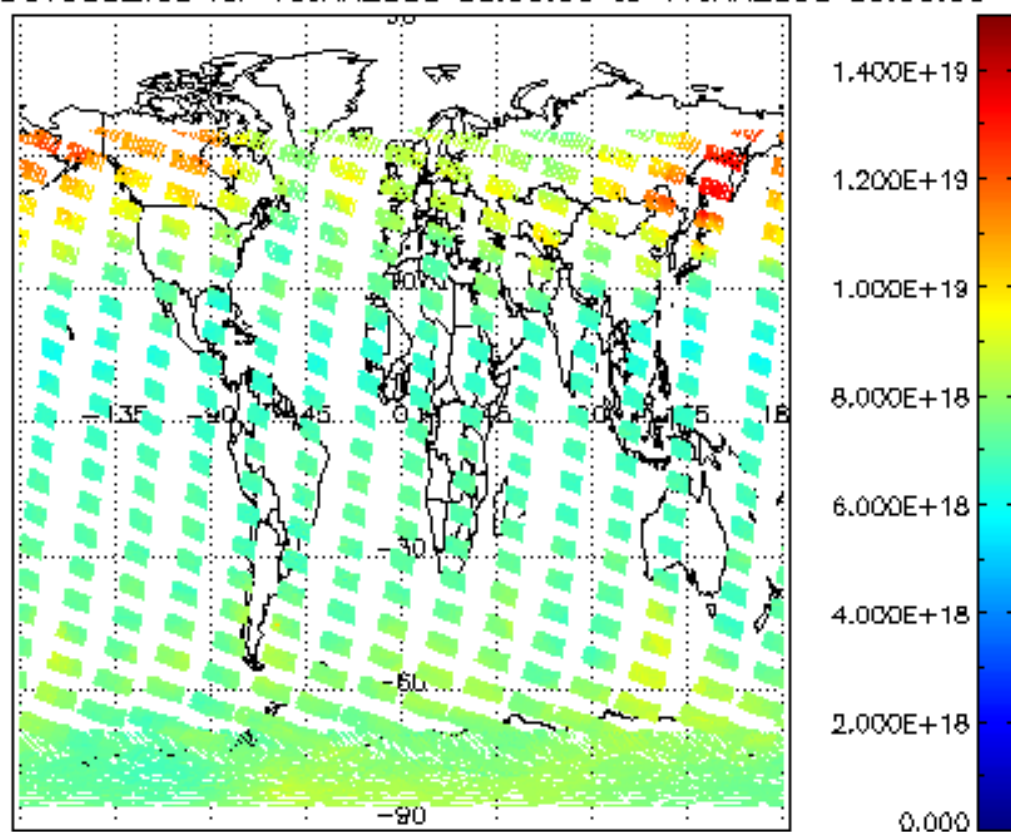
SCIOL2P_NADUV003_vcd for 10JAN2008 00:00:00 to 11JAN2008 00:00:00
