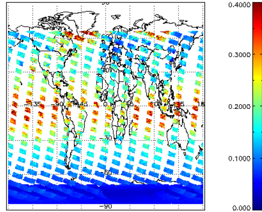
SCIOL2P_NADUV1NO2_vcd_err for 10JAN2008 00:00:00 to 11JAN2008 00:00:00
