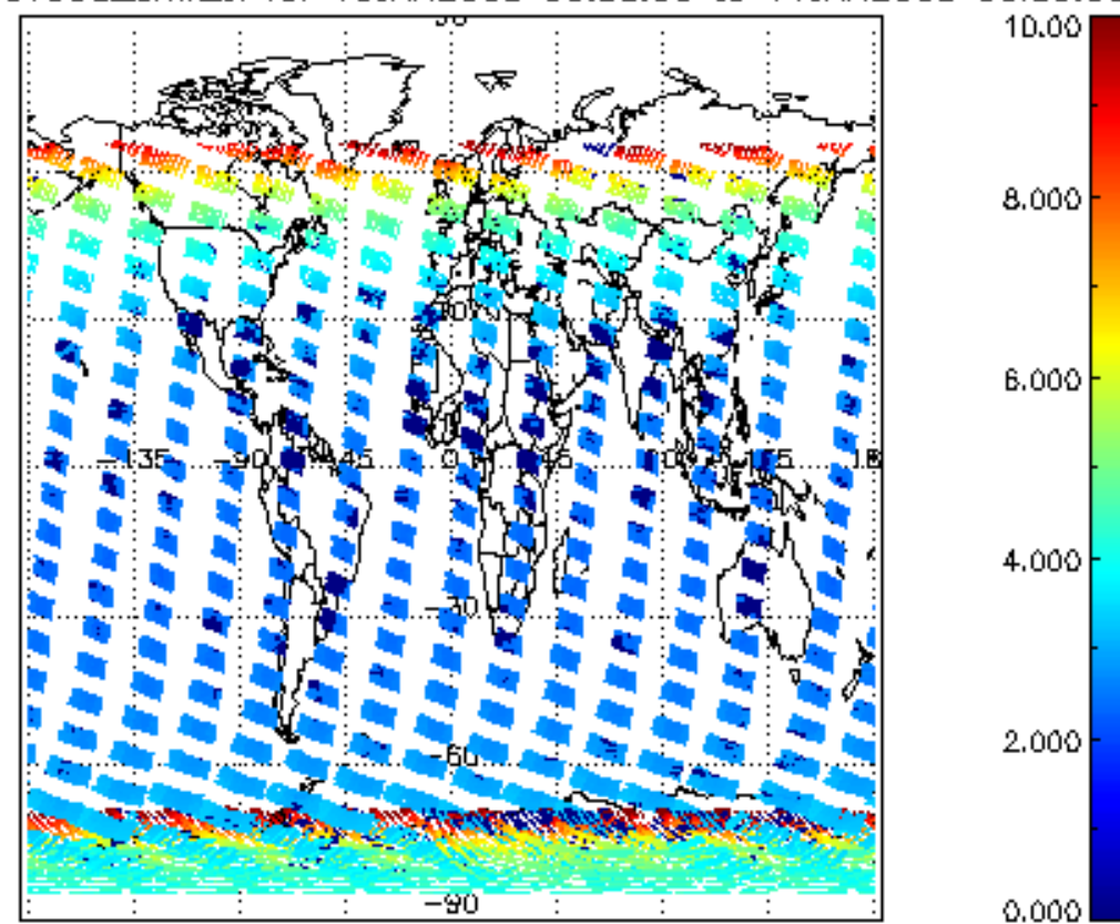
SCIOL2P_NADUV003_amf_cl for 10JAN2008 00:00:00 to 11JAN2008 00:00:00
