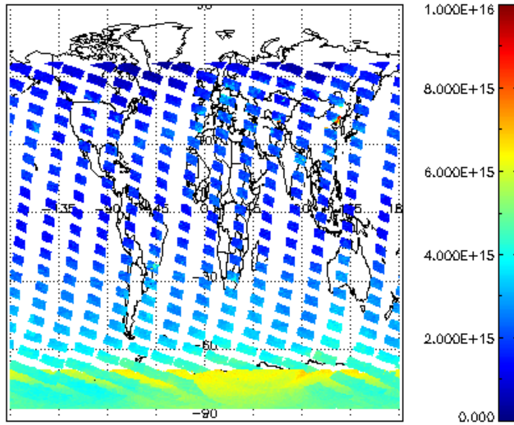
SCIOL2P_NADUV1NO2_vcd for 10JAN2008 00:00:00 to 11JAN2008 00:00:00
