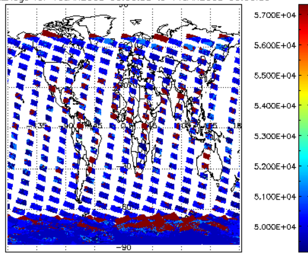
cloud_flags for 10JAN2008 00:00:00 to 11JAN2008 00:00:00
