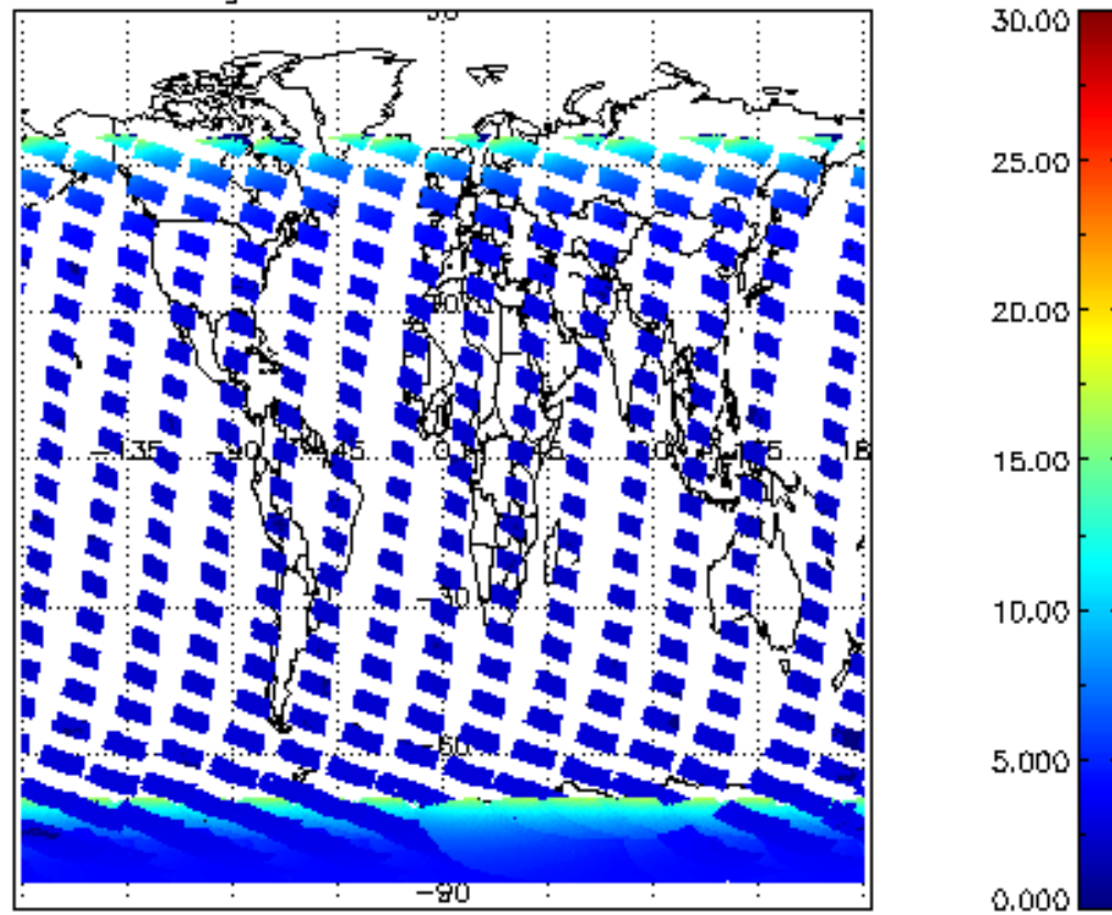
SCIOL2P_NADUV1NO2_amf_gr for 10JAN2008 00:00:00 to 11JAN2008 00:00:00
