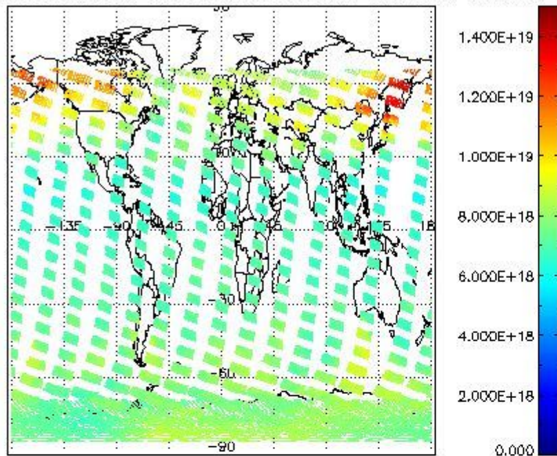
SCIOL2P_NADUV003_vcd for 10JAN2008 00:00:00 to 11JAN2008 00:00:00
