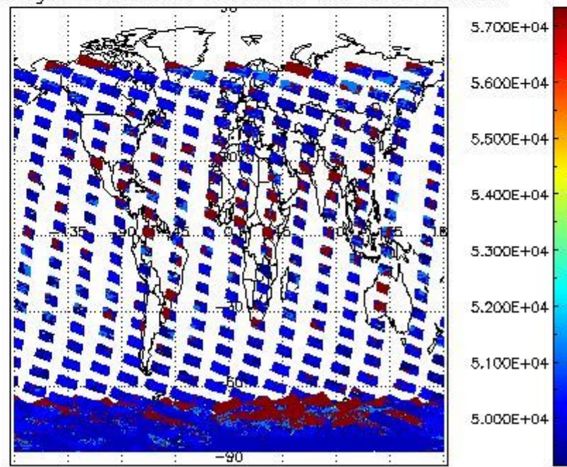
cloud_flags for 10JAN2008 00:00:00 to 11JAN2008 00:00:00
