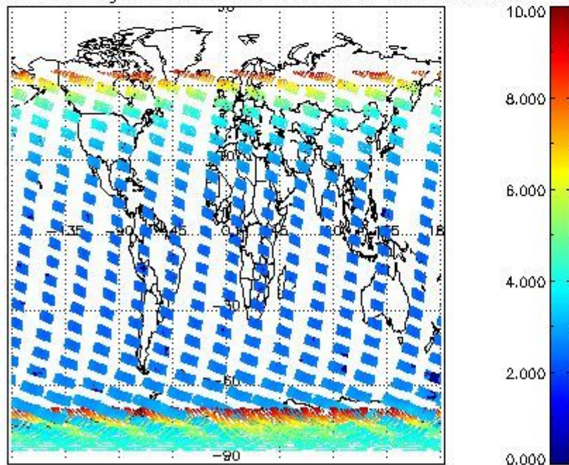
SCIOL2P_NADUV003_amf_gr for 10JAN2008 00:00:00 to 11JAN2008 00:00:00
