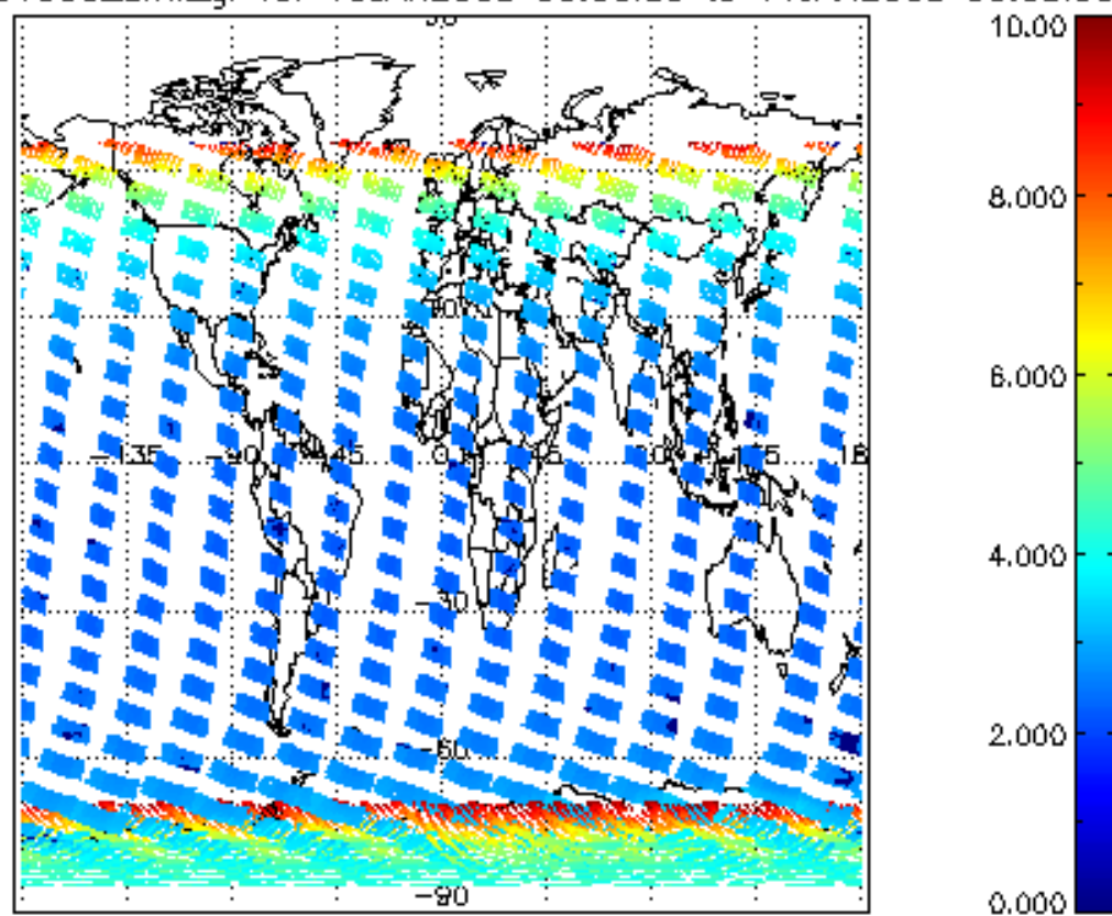
SCIOL2P_NADUV003_amf_gr for 10JAN2008 00:00:00 to 11JAN2008 00:00:00
