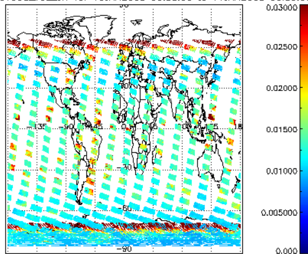
SCIOL2P_NADUV003_vcd_err for 10JAN2008 00:00:00 to 11JAN2008 00:00:00
