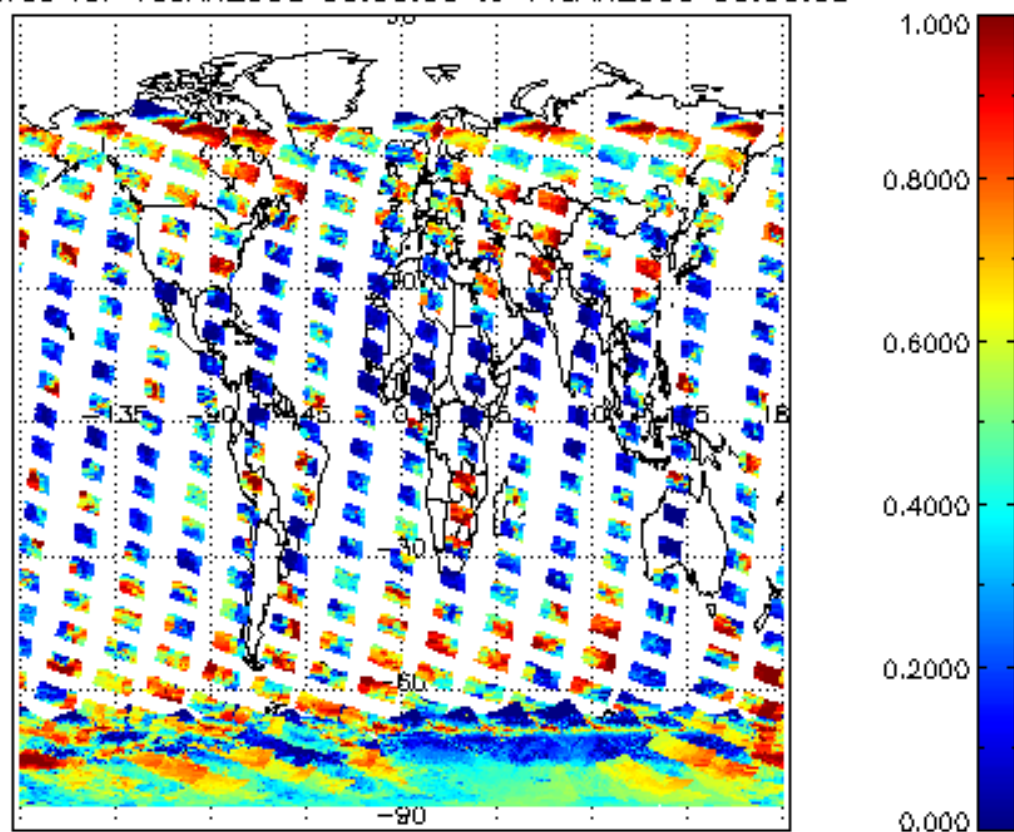
cL_frac for 10JAN2008 00:00:00 to 11JAN2008 00:00:00
