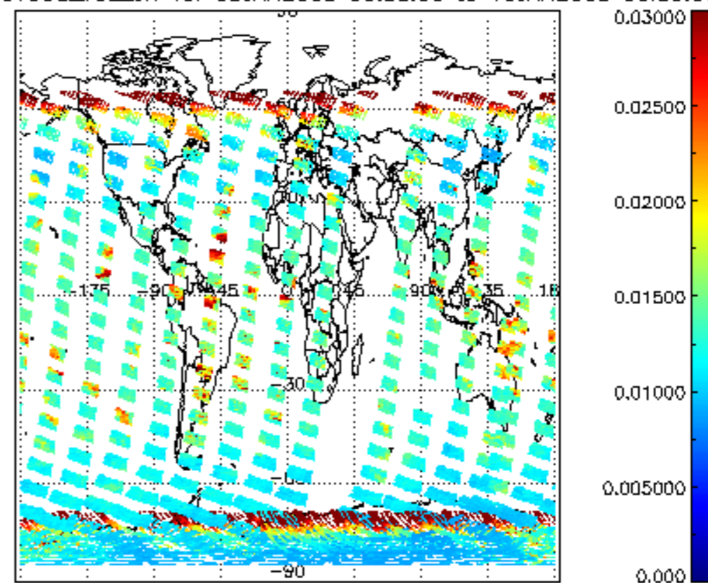
SCIOL2P_NADUV003_vcd_err for 09JAN2008 00:00:00 to 10JAN2008 00:00:00
