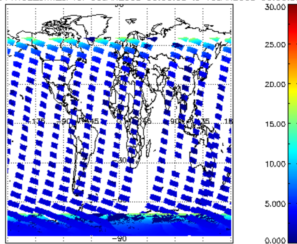
SCIOL2P_NADUV1NO2_amf_cl for 09JAN2008 00:00:00 to 10JAN2008 00:00:00
