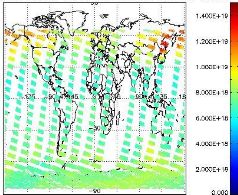
SCIOL2P_NADUV003_vcd for 09JAN2008 00:00:00 to 10JAN2008 00:00:00
