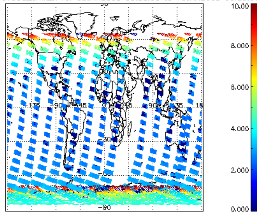
SCIOL2P_NADUV003_amf_cl for 09JAN2008 00:00:00 to 10JAN2008 00:00:00
