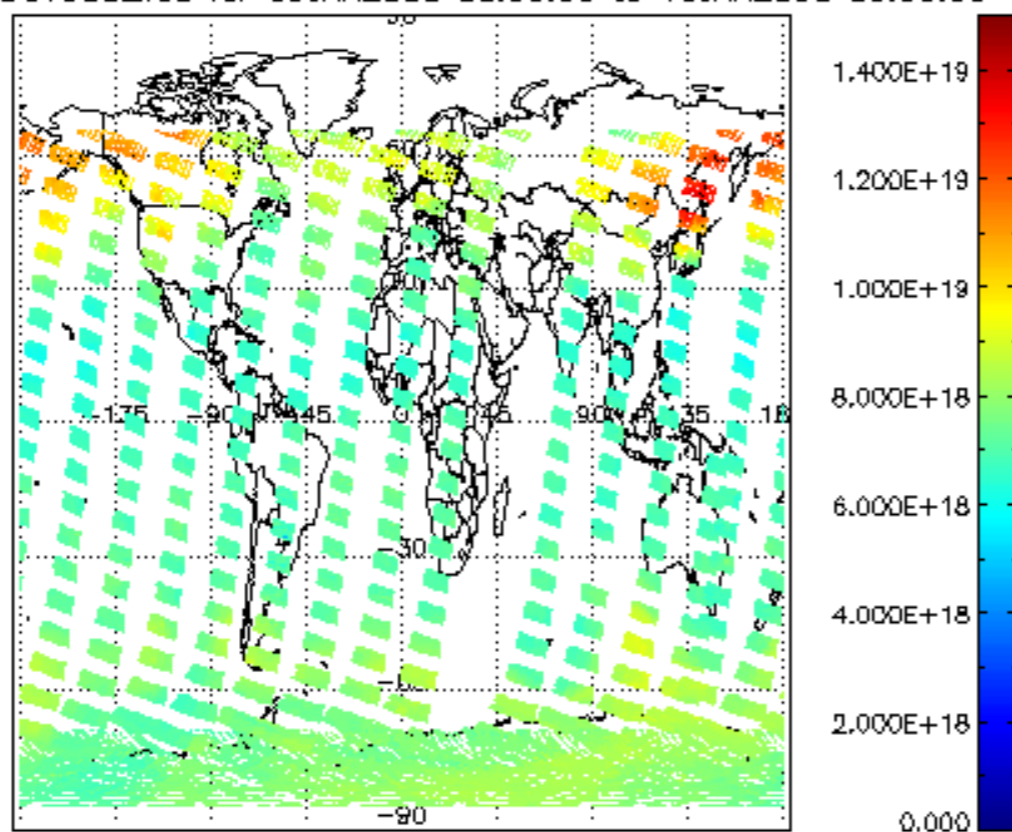
SCIOL2P_NADUV003_vcd for 09JAN2008 00:00:00 to 10JAN2008 00:00:00
