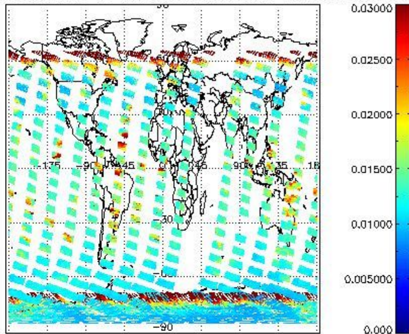
SCIOL2P_NADUV003_vcd_err for 09JAN2008 00:00:00 to 10JAN2008 00:00:00
