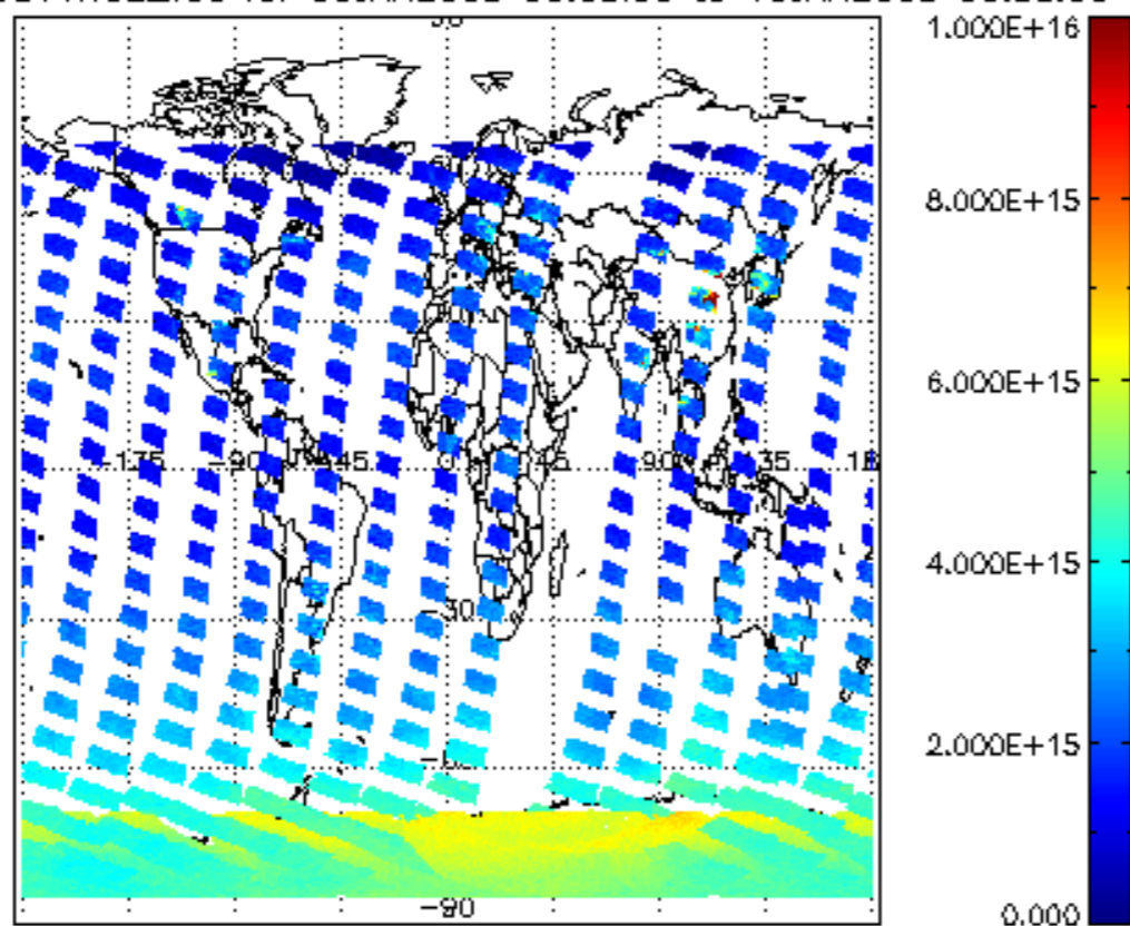
SCIOL2P_NADUV1NO2_vcd for 09JAN2008 00:00:00 to 10JAN2008 00:00:00
