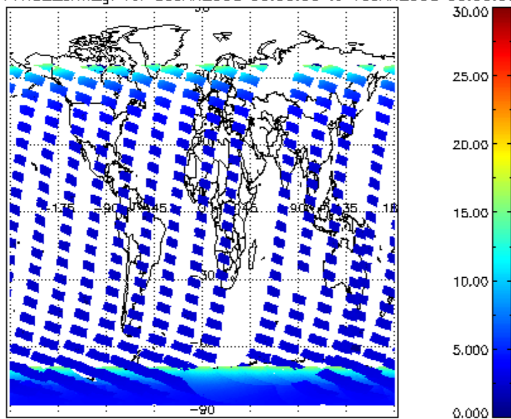
SCIOL2P_NADUV1NO2_amf_gr for 09JAN2008 00:00:00 to 10JAN2008 00:00:00
