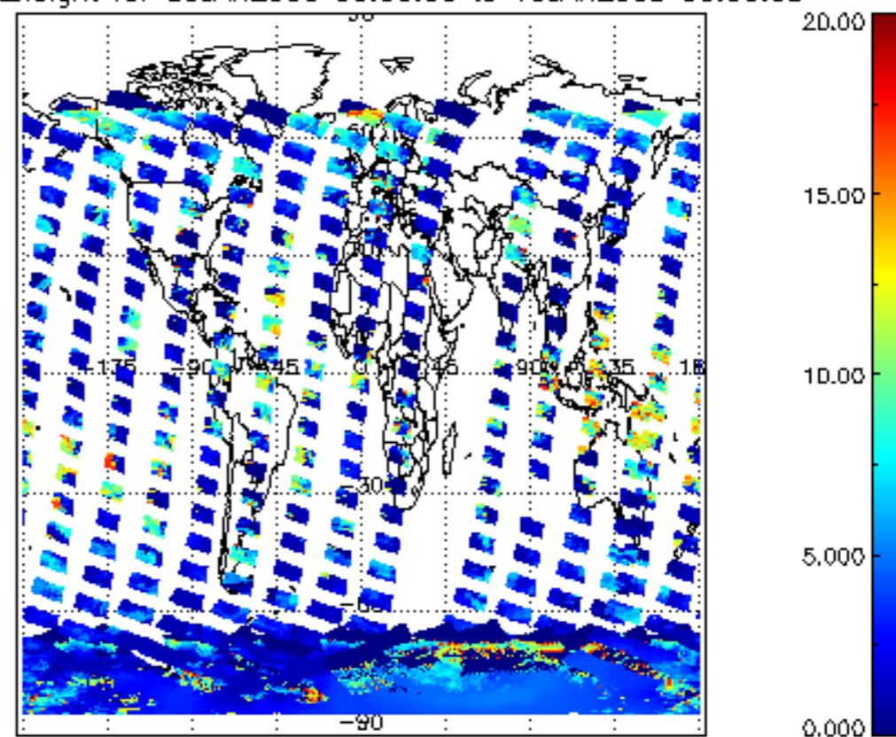
cL_top_height for 09JAN2008 00:00:00 to 10JAN2008 00:00:00
