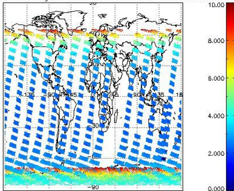
SCIOL2P_NADUV003_amf_gr for 09JAN2008 00:00:00 to 10JAN2008 00:00:00
