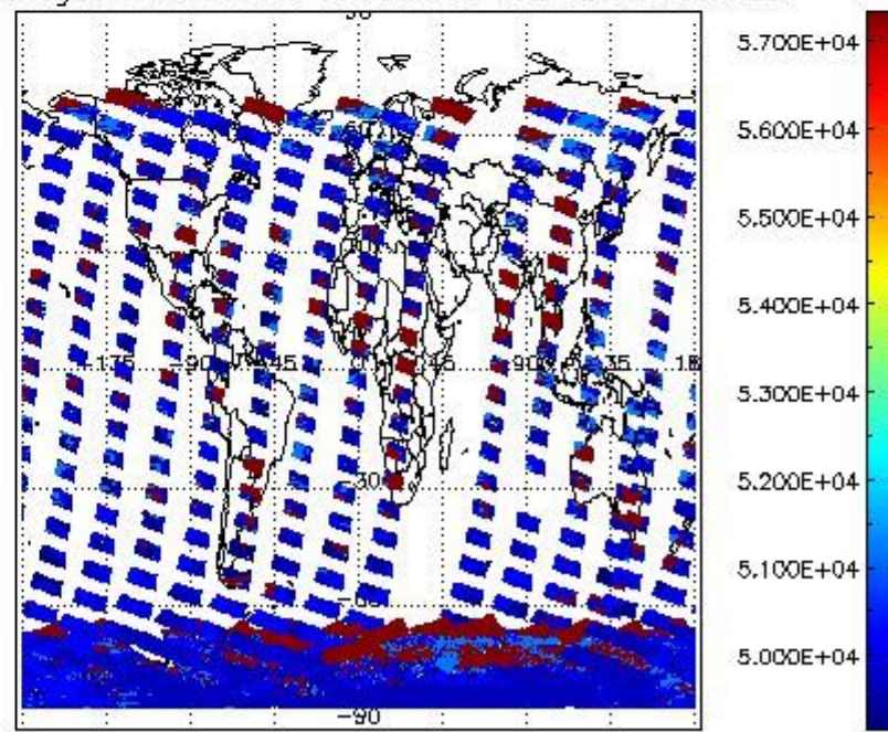
cloud_flags for 09JAN2008 00:00:00 to 10JAN2008 00:00:00
