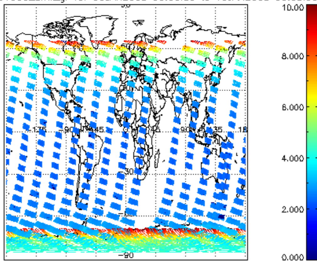
SCIOL2P_NADUV003_amf_gr for 09JAN2008 00:00:00 to 10JAN2008 00:00:00
