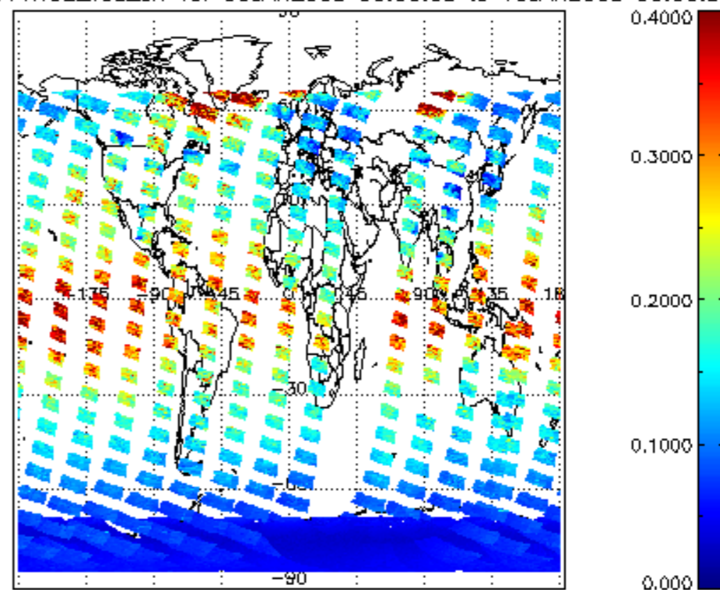
SCIOL2P_NADUV1NO2_vcd_err for 09JAN2008 00:00:00 to 10JAN2008 00:00:00
