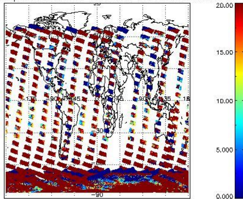
cLopt_depth for 09JAN2008 00:00:00 to 10JAN2008 00:00:00
