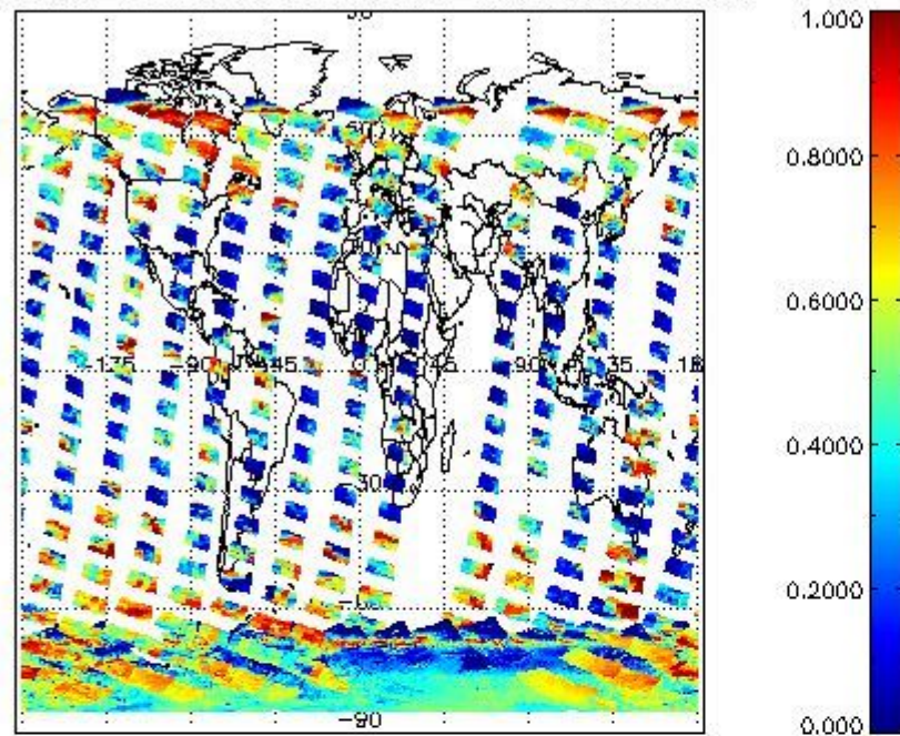
cL_frac for 09JAN2008 00:00:00 to 10JAN2008 00:00:00
