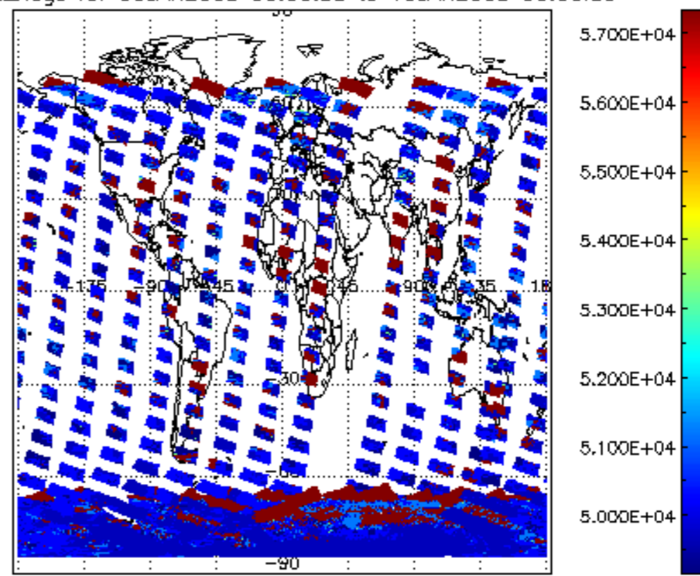
cloud_flags for 09JAN2008 00:00:00 to 10JAN2008 00:00:00
