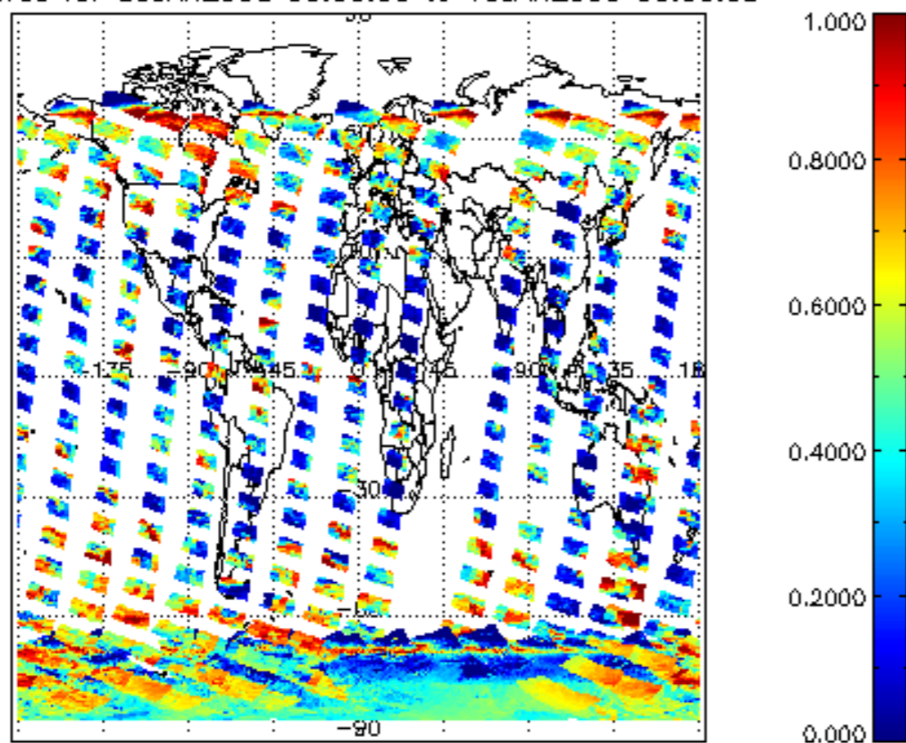
cL_frac for 09JAN2008 00:00:00 to 10JAN2008 00:00:00
