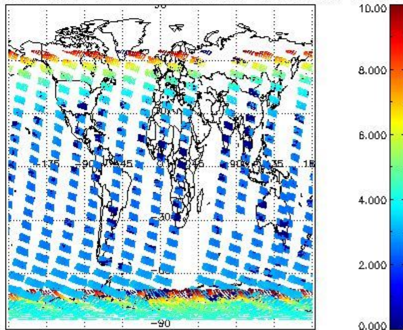
SCIOL2P_NADUV003_amf_cl for 09JAN2008 00:00:00 to 10JAN2008 00:00:00
