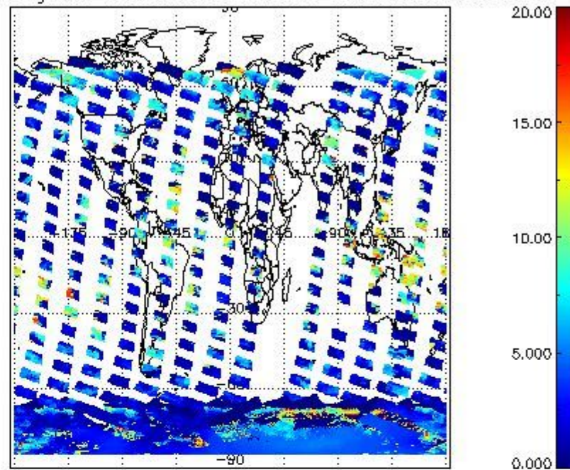
cL_top_height for 09JAN2008 00:00:00 to 10JAN2008 00:00:00
