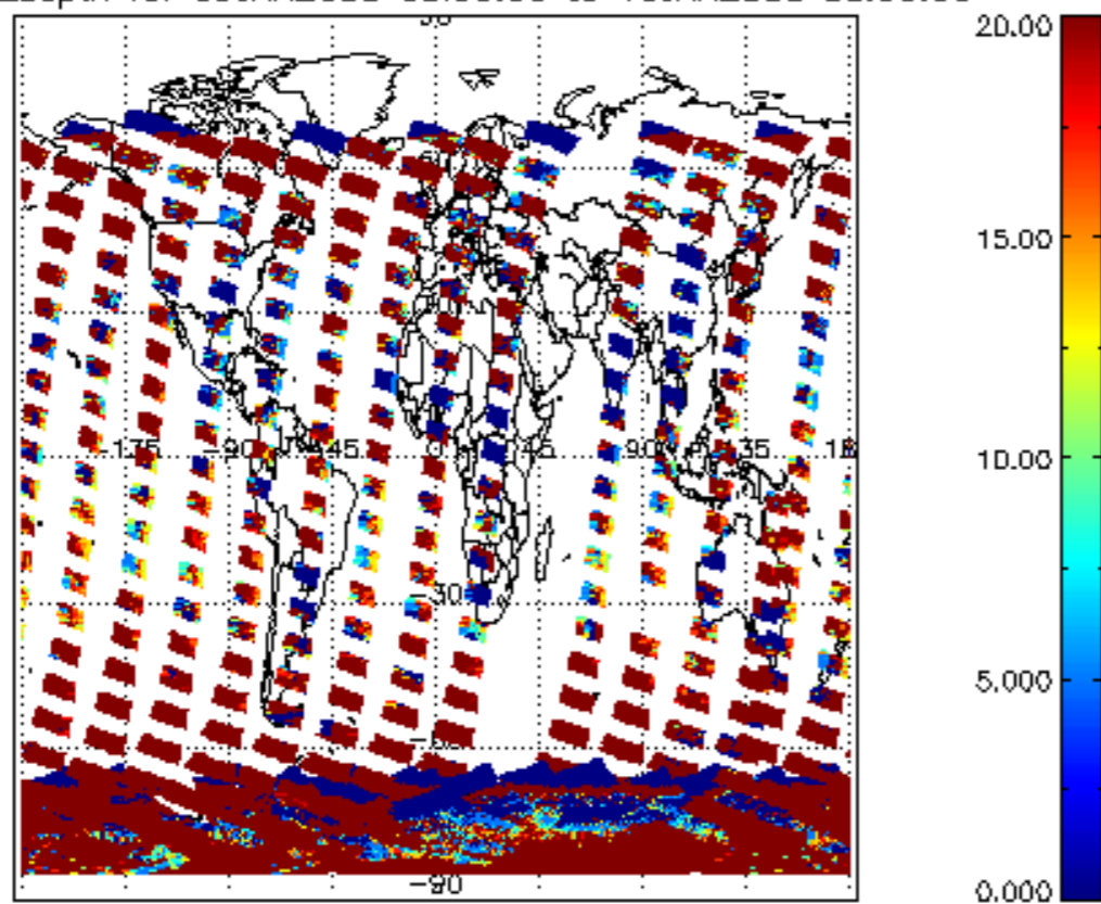
cLopt_depth for 09JAN2008 00:00:00 to 10JAN2008 00:00:00
