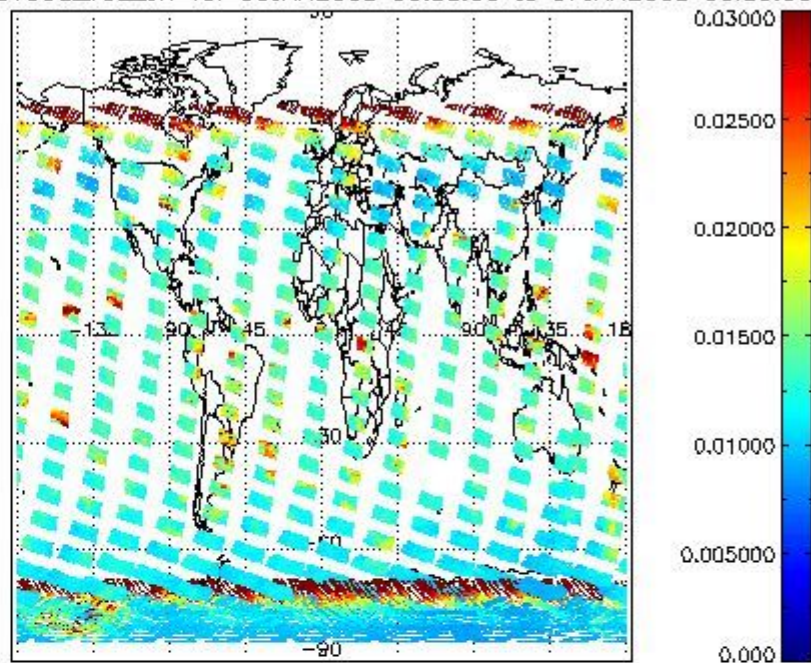
SCIOL2P_NADUV003_vcd_err for 06JAN2008 00:00:00 to 07JAN2008 00:00:00
