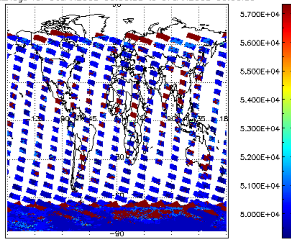
cloud_flags for 06JAN2008 00:00:00 to 07JAN2008 00:00:00
