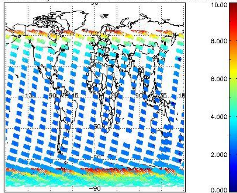
SCIOL2P_NADUV003_amf_gr for 06JAN2008 00:00:00 to 07JAN2008 00:00:00
