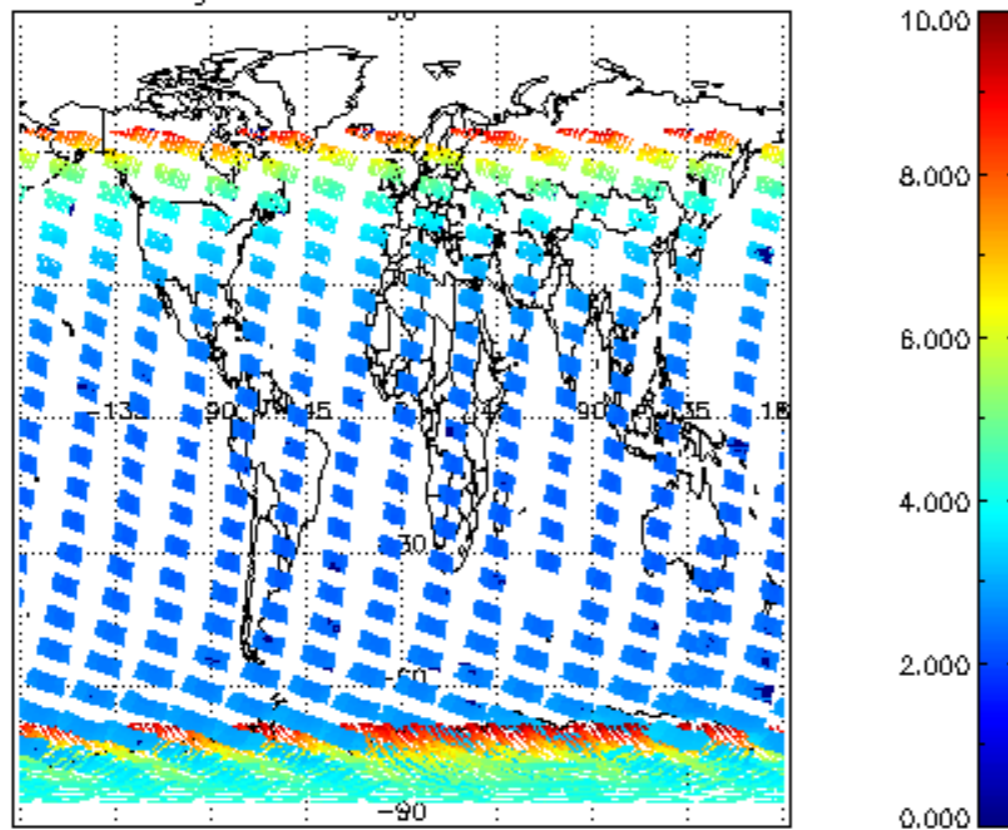
SCIOL2P_NADUV003_amf_gr for 06JAN2008 00:00:00 to 07JAN2008 00:00:00
