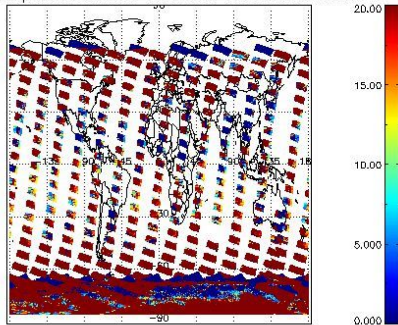
cLopt_depth for 06JAN2008 00:00:00 to 07JAN2008 00:00:00
