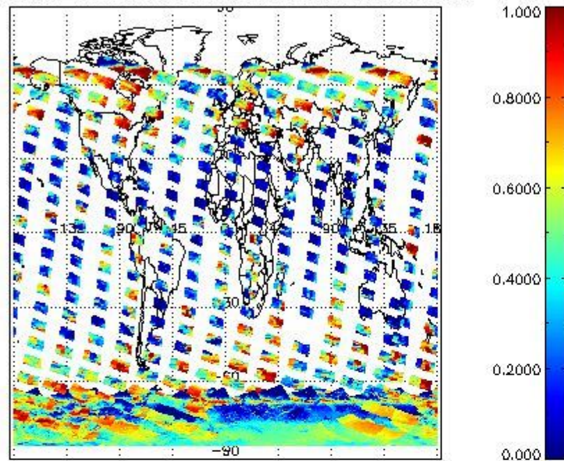
cL_frac for 06JAN2008 00:00:00 to 07JAN2008 00:00:00
