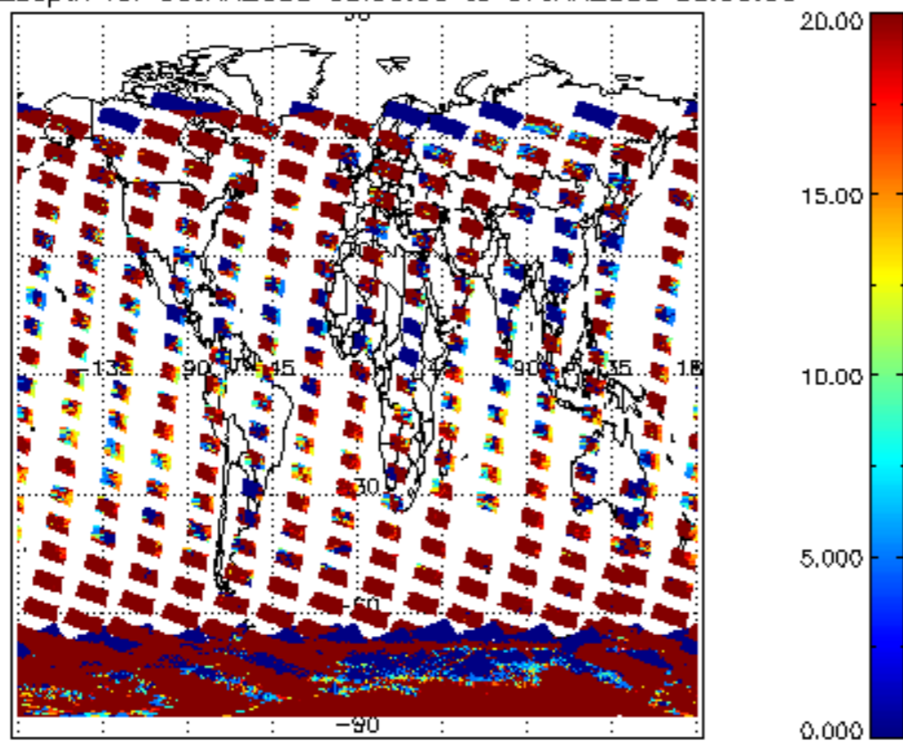
cLopt_depth for 06JAN2008 00:00:00 to 07JAN2008 00:00:00
