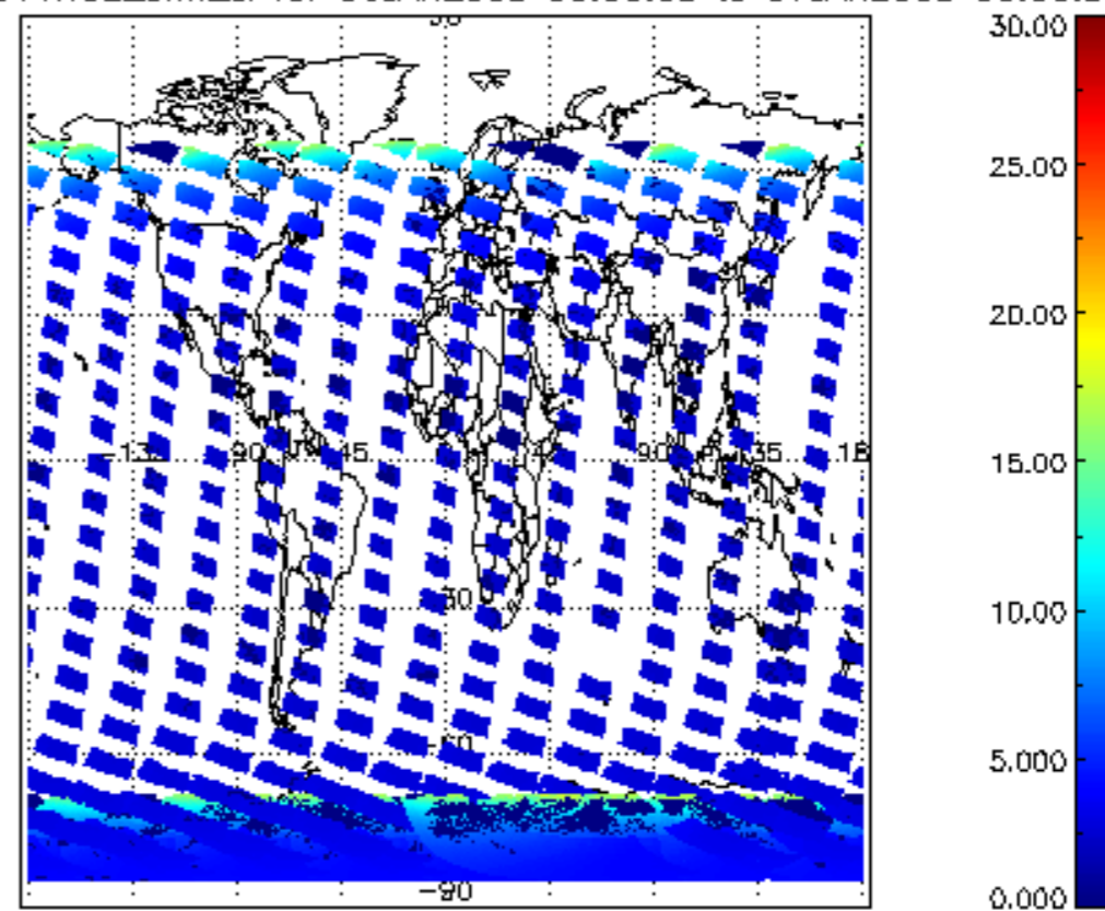
SCIOL2P_NADUV1NO2_amf_cl for 06JAN2008 00:00:00 to 07JAN2008 00:00:00
