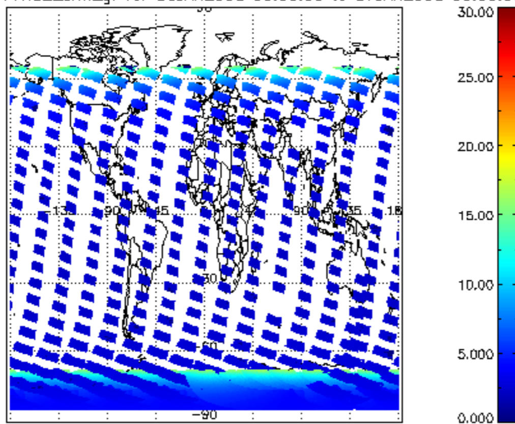
SCIOL2P_NADUV1NO2_amf_gr for 06JAN2008 00:00:00 to 07JAN2008 00:00:00
