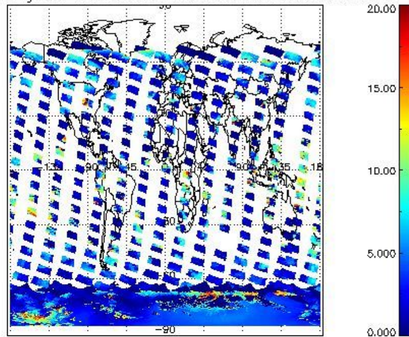
cL_top_height for 06JAN2008 00:00:00 to 07JAN2008 00:00:00
