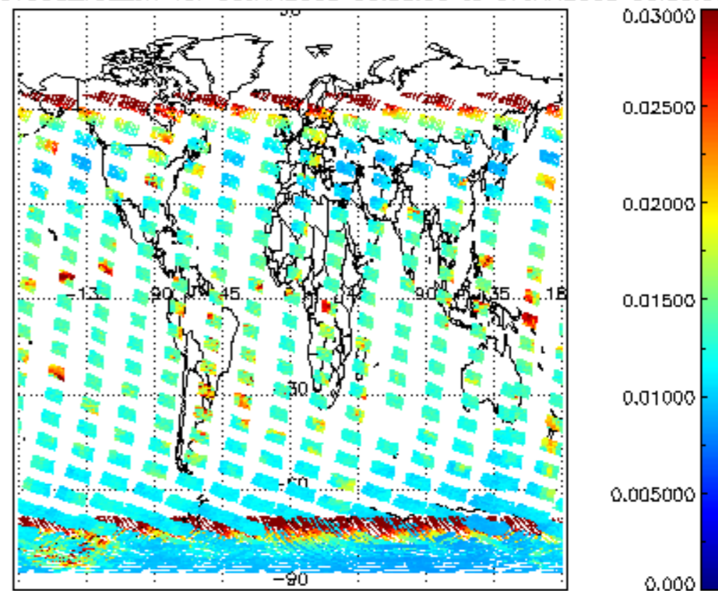
SCIOL2P_NADUV003_vcd_err for 06JAN2008 00:00:00 to 07JAN2008 00:00:00
