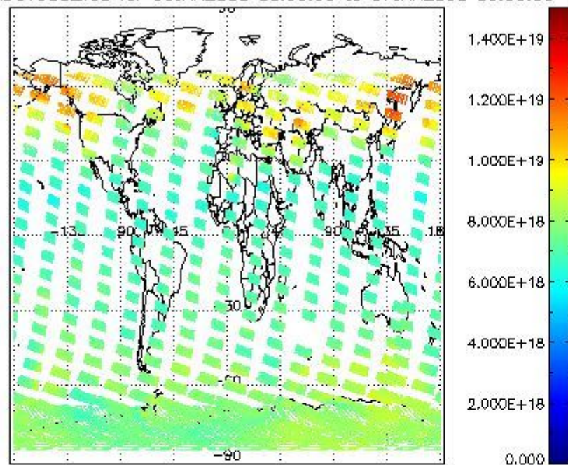
SCIOL2P_NADUV003_vcd for 06JAN2008 00:00:00 to 07JAN2008 00:00:00
