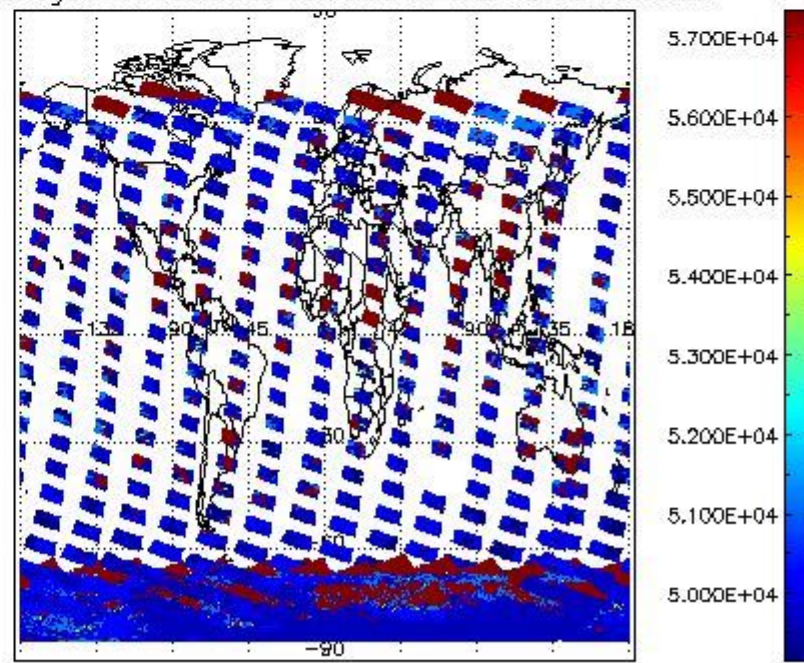
cloud_flags for 06JAN2008 00:00:00 to 07JAN2008 00:00:00
