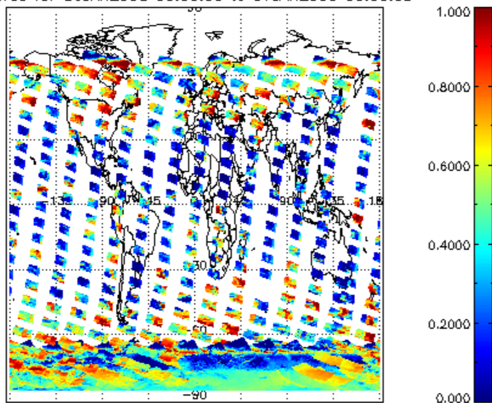
cL_frac for 06JAN2008 00:00:00 to 07JAN2008 00:00:00
