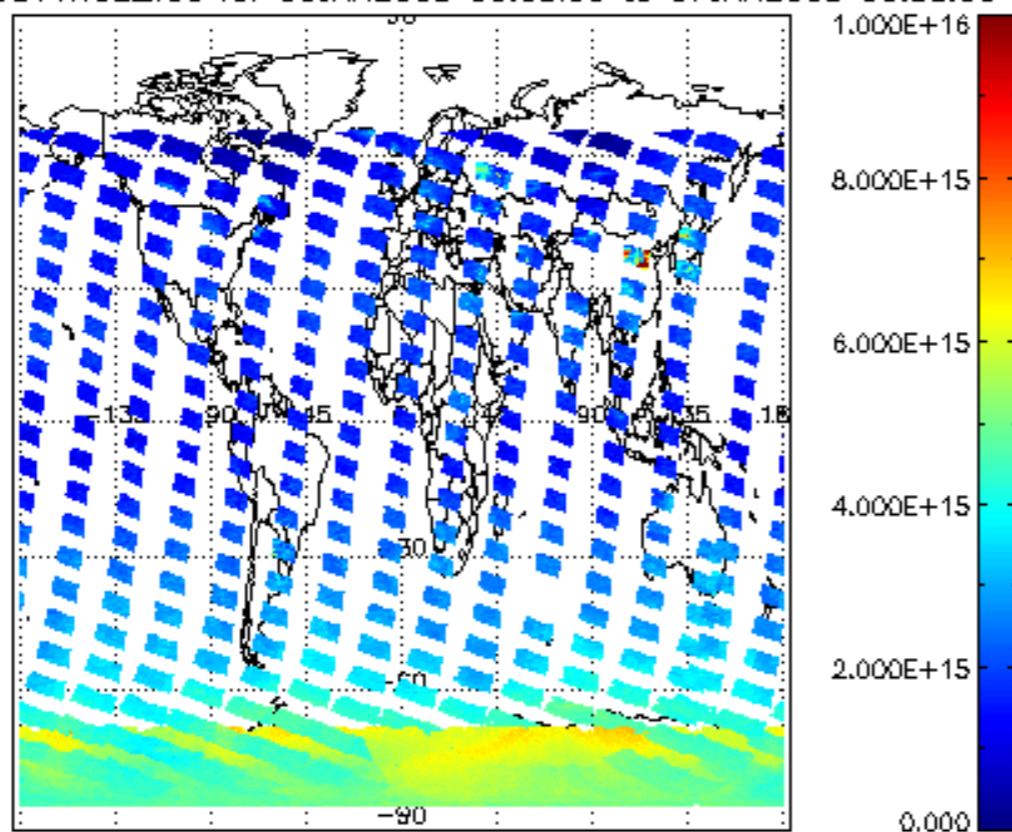
SCIOL2P_NADUV1NO2_vcd for 06JAN2008 00:00:00 to 07JAN2008 00:00:00
