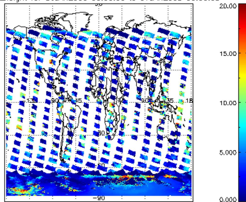
cL_top_height for 06JAN2008 00:00:00 to 07JAN2008 00:00:00
