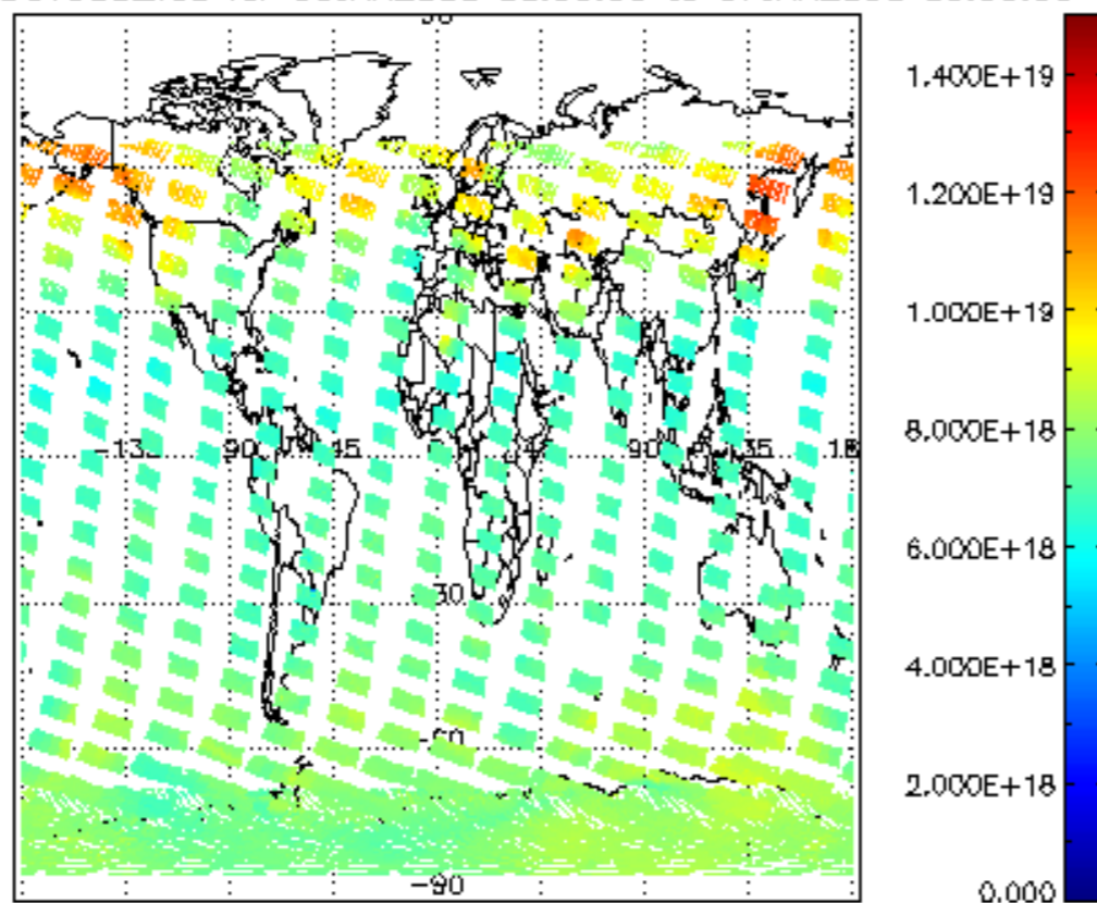
SCIOL2P_NADUV003_vcd for 06JAN2008 00:00:00 to 07JAN2008 00:00:00
