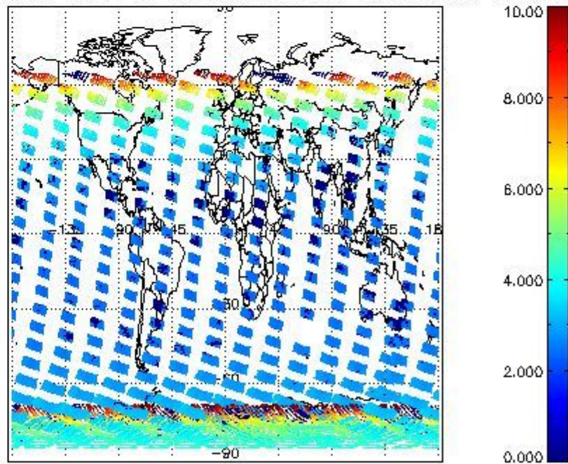
SCIOL2P_NADUV003_amf_cl for 06JAN2008 00:00:00 to 07JAN2008 00:00:00
