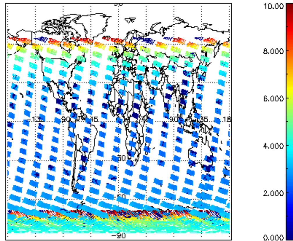
SCIOL2P_NADUV003_amf_cl for 06JAN2008 00:00:00 to 07JAN2008 00:00:00
