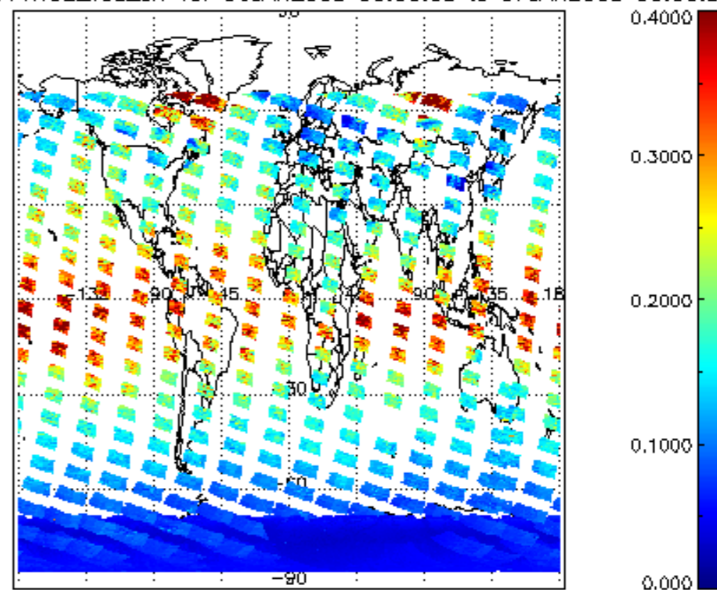
SCIOL2P_NADUV1NO2_vcd_err for 06JAN2008 00:00:00 to 07JAN2008 00:00:00
