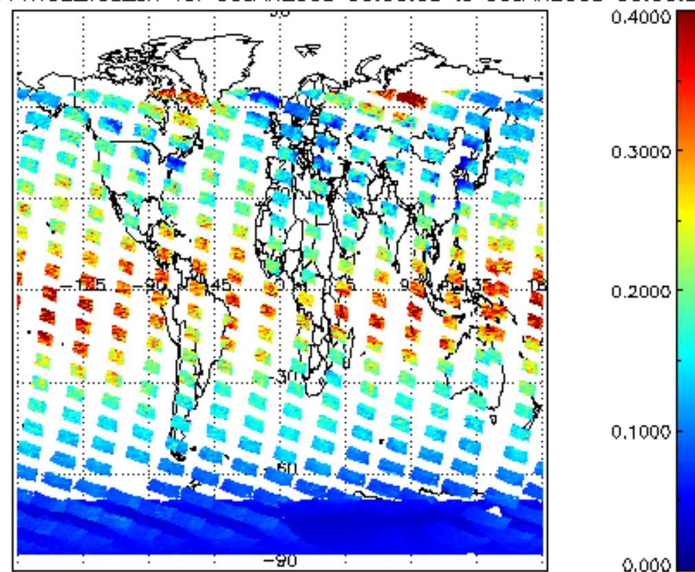
SCIOL2P_NADUV1NO2_vcd_err for 05JAN2008 00:00:00 to 06JAN2008 00:00:00
