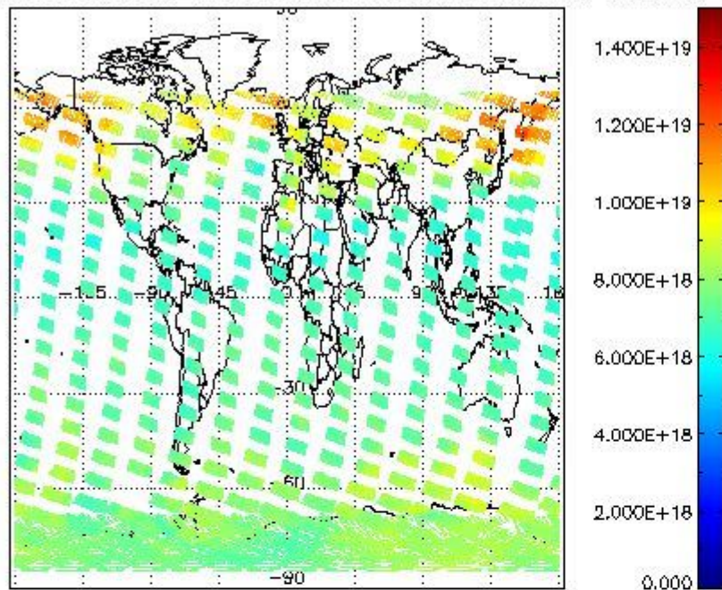
SCIOL2P_NADUV003_vcd for 05JAN2008 00:00:00 to 06JAN2008 00:00:00
