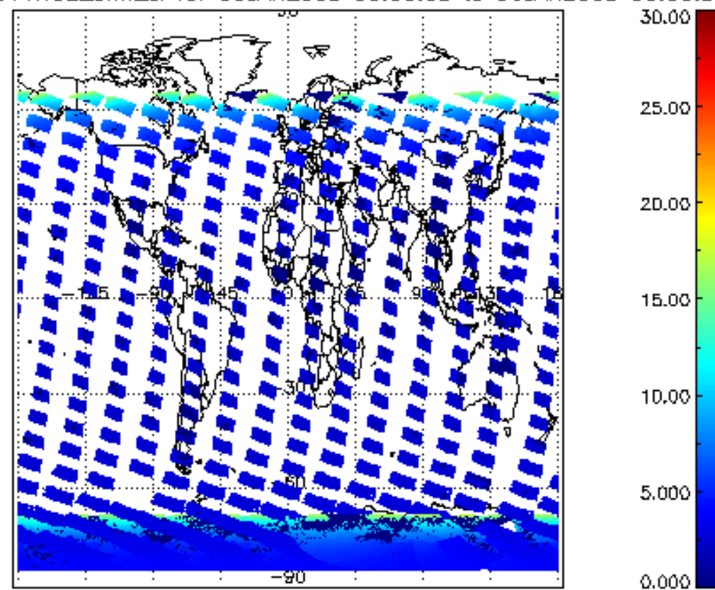
SCIOL2P_NADUV1NO2_amf_cl for 05JAN2008 00:00:00 to 06JAN2008 00:00:00
