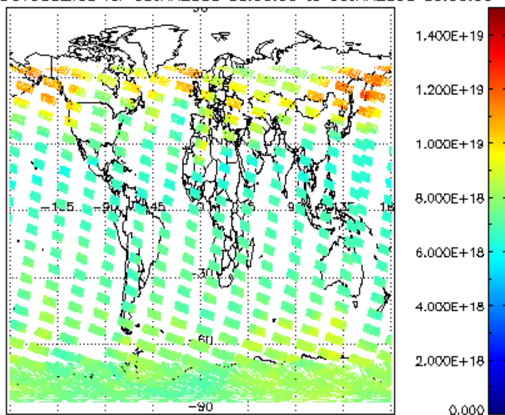
SCIOL2P_NADUV003_vcd for 05JAN2008 00:00:00 to 06JAN2008 00:00:00
