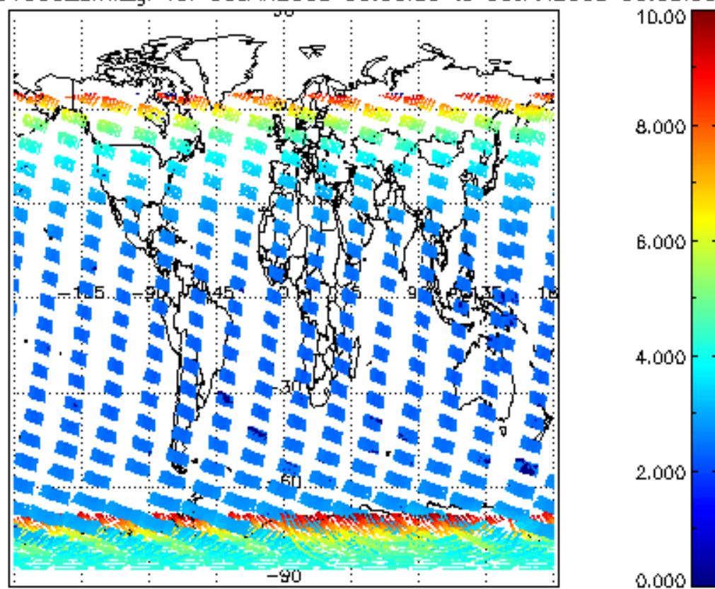
SCIOL2P_NADUV003_amf_gr for 05JAN2008 00:00:00 to 06JAN2008 00:00:00
