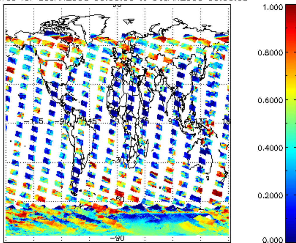
cL_frac for 05JAN2008 00:00:00 to 06JAN2008 00:00:00
