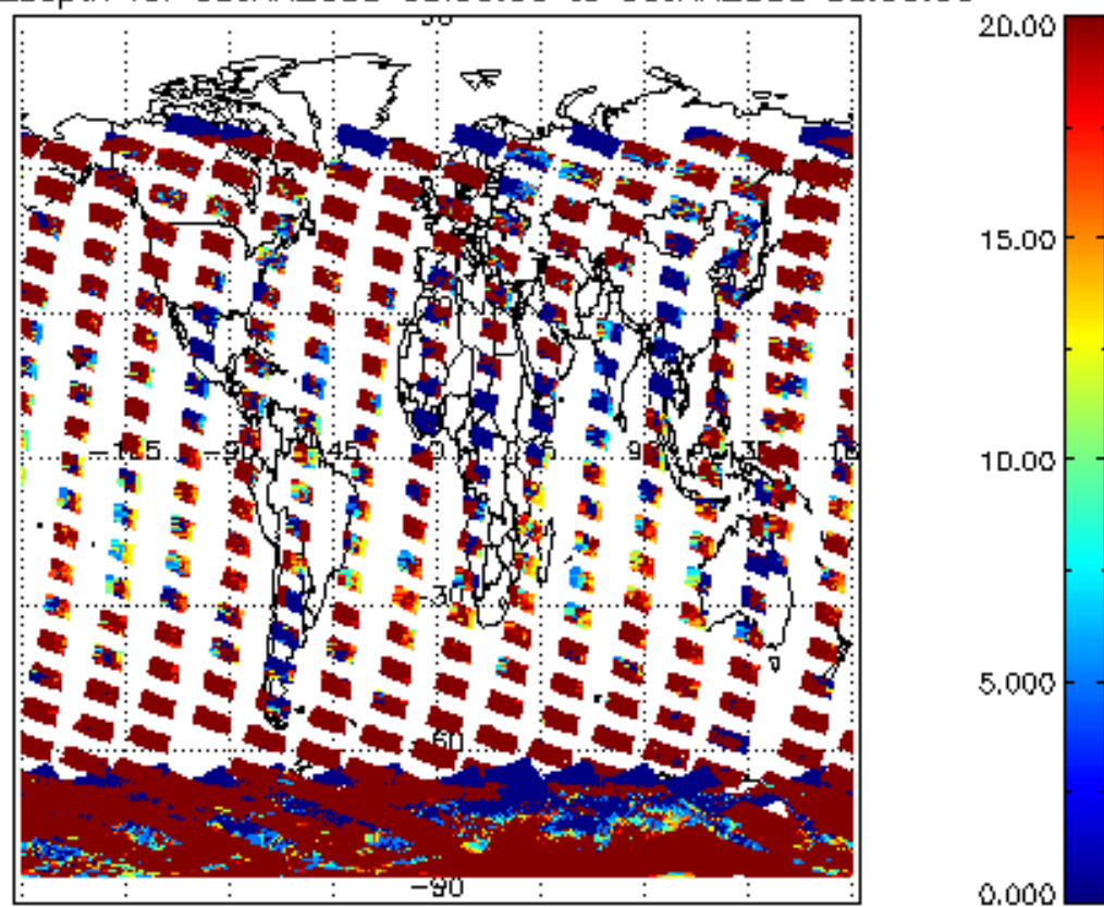
cLopt_depth for 05JAN2008 00:00:00 to 06JAN2008 00:00:00
