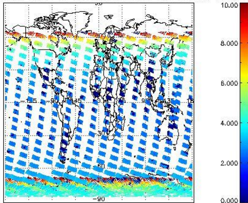
SCIOL2P_NADUV003_amf_cl for 05JAN2008 00:00:00 to 06JAN2008 00:00:00
