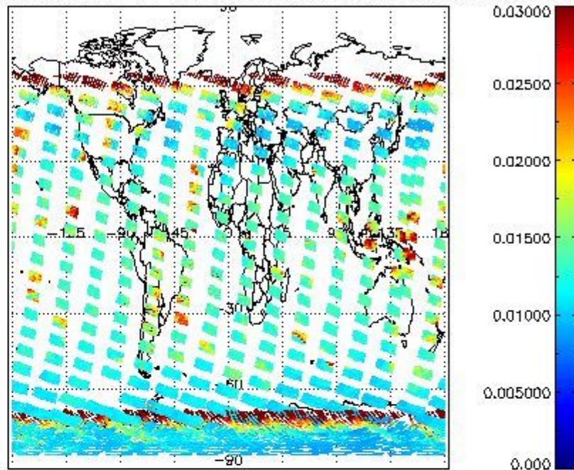
SCIOL2P_NADUV003_vcd_err for 05JAN2008 00:00:00 to 06JAN2008 00:00:00
