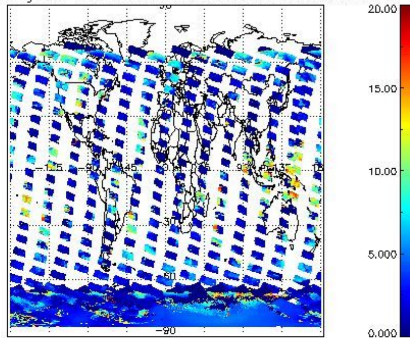
cL_top_height for 05JAN2008 00:00:00 to 06JAN2008 00:00:00
