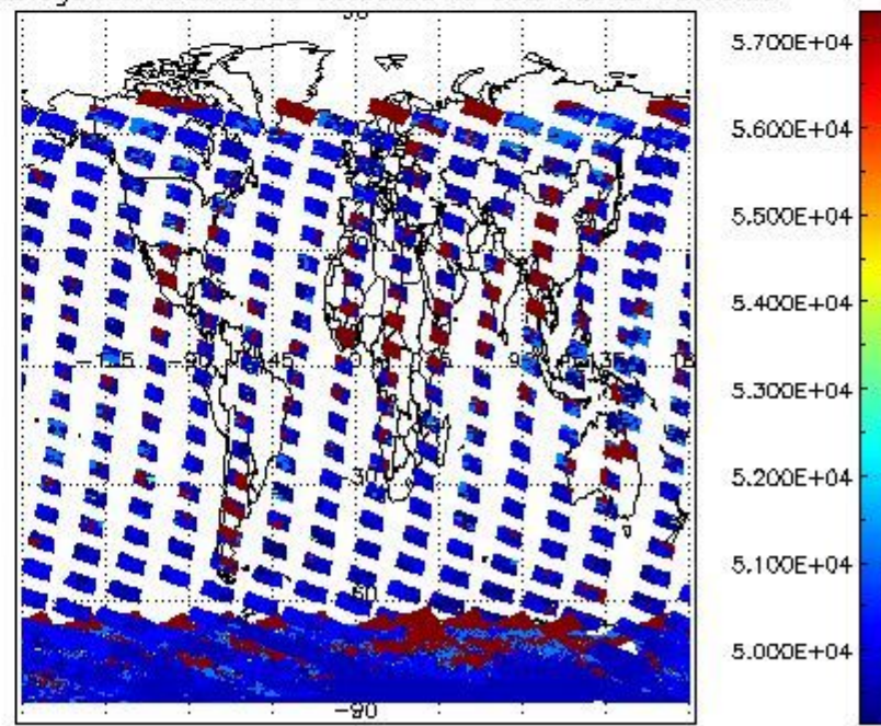
cloud_flags for 05JAN2008 00:00:00 to 06JAN2008 00:00:00
