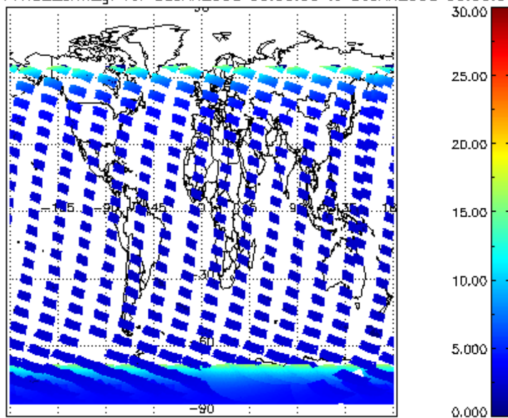
SCIOL2P_NADUV1NO2_amf_gr for 05JAN2008 00:00:00 to 06JAN2008 00:00:00
