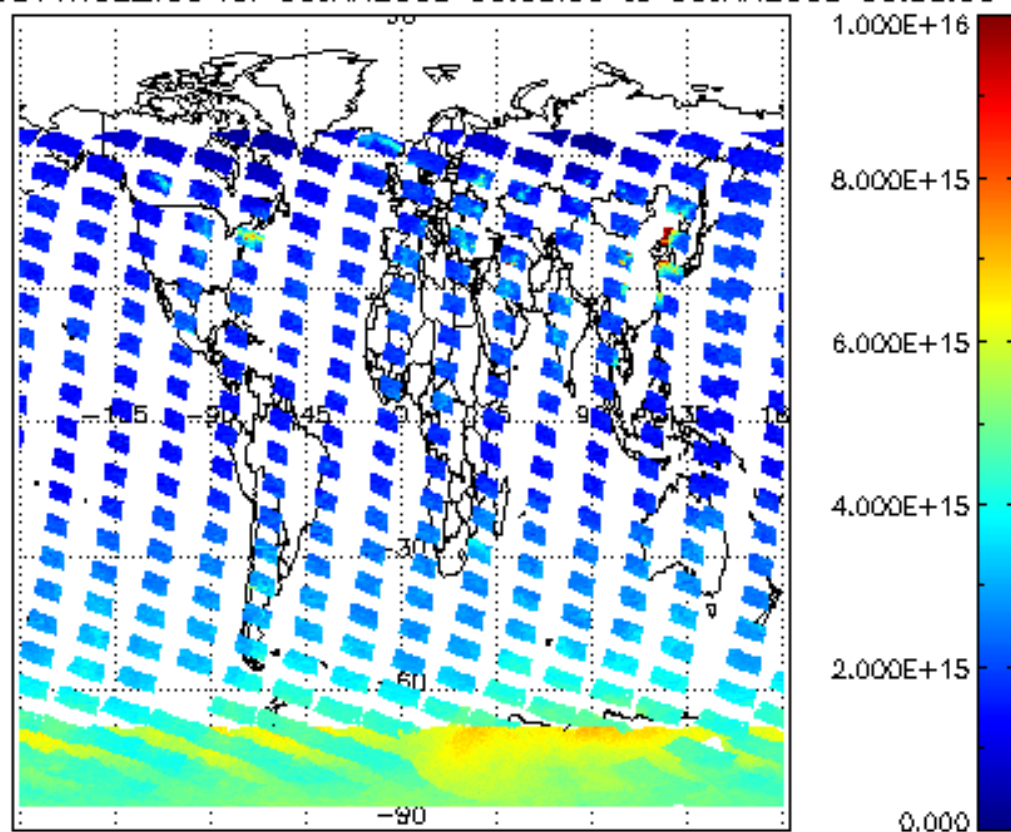
SCIOL2P_NADUV1NO2_vcd for 05JAN2008 00:00:00 to 06JAN2008 00:00:00
