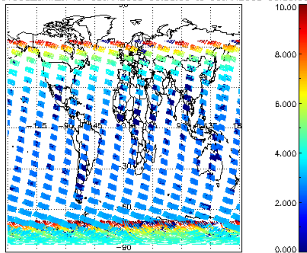
SCIOL2P_NADUV003_amf_cl for 05JAN2008 00:00:00 to 06JAN2008 00:00:00
