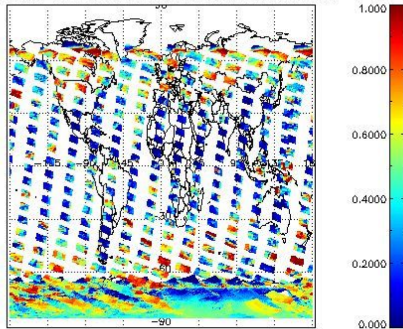
cL_frac for 05JAN2008 00:00:00 to 06JAN2008 00:00:00
