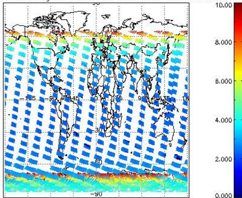
SCIOL2P_NADUV003_amf_gr for 05JAN2008 00:00:00 to 06JAN2008 00:00:00
