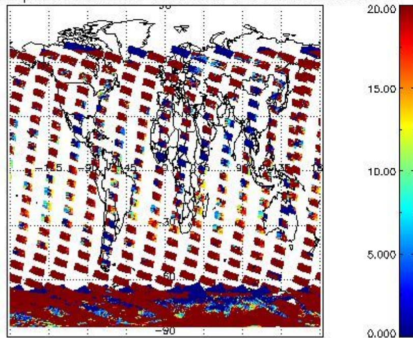
cLopt_depth for 05JAN2008 00:00:00 to 06JAN2008 00:00:00
