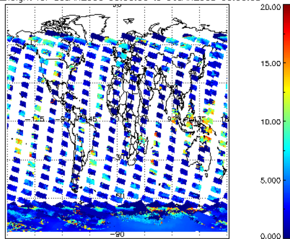
cL_top_height for 05JAN2008 00:00:00 to 06JAN2008 00:00:00
