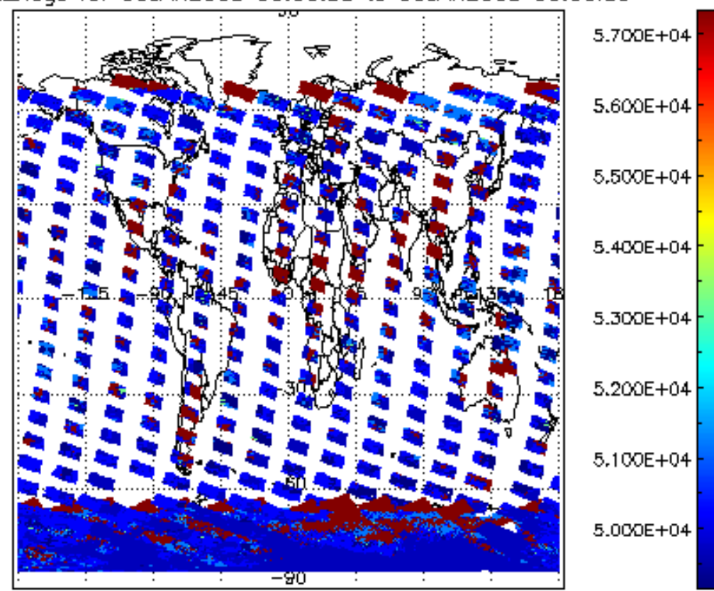
cloud_flags for 05JAN2008 00:00:00 to 06JAN2008 00:00:00
