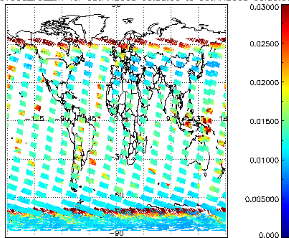
SCIOL2P_NADUV003_vcd_err for 05JAN2008 00:00:00 to 06JAN2008 00:00:00
