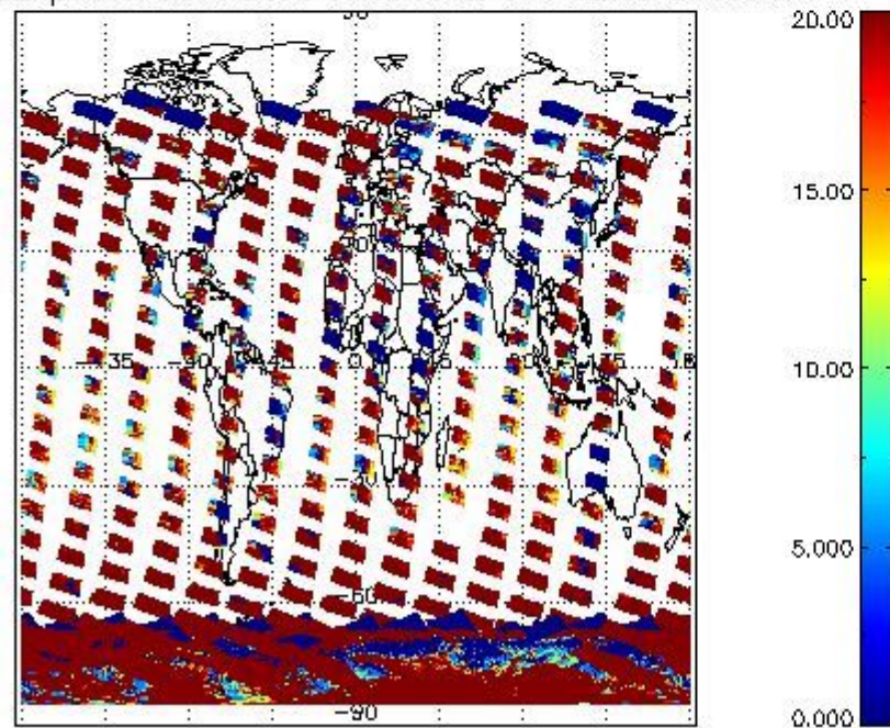
cLopt_depth for 04JAN2008 00:00:00 to 05JAN2008 00:00:00
