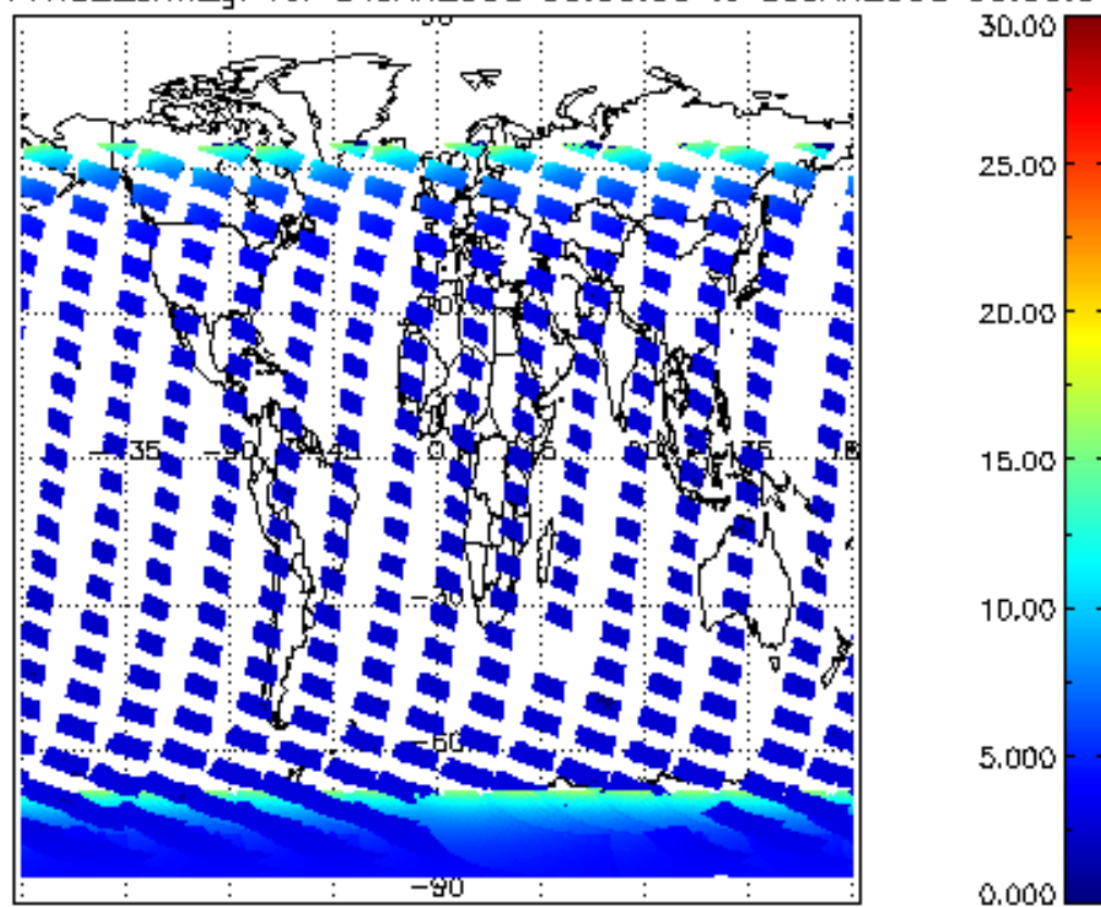
SCIOL2P_NADUV1NO2_amf_gr for 04JAN2008 00:00:00 to 05JAN2008 00:00:00
