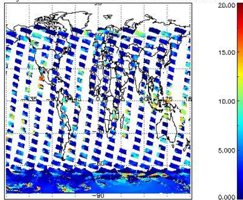
cL_top_height for 04JAN2008 00:00:00 to 05JAN2008 00:00:00
