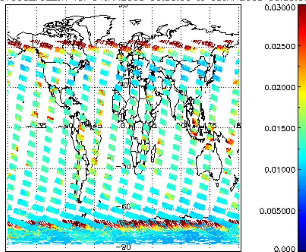
SCIOL2P_NADUV003_vcd_err for 04JAN2008 00:00:00 to 05JAN2008 00:00:00
