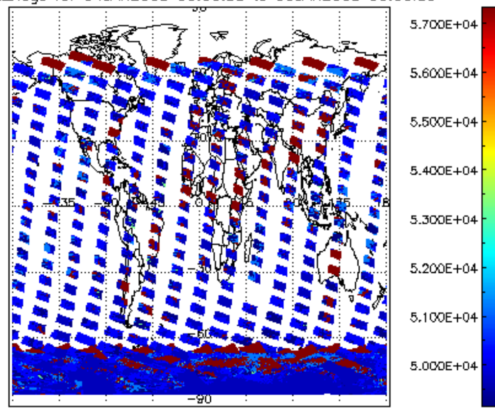
cloud_flags for 04JAN2008 00:00:00 to 05JAN2008 00:00:00
