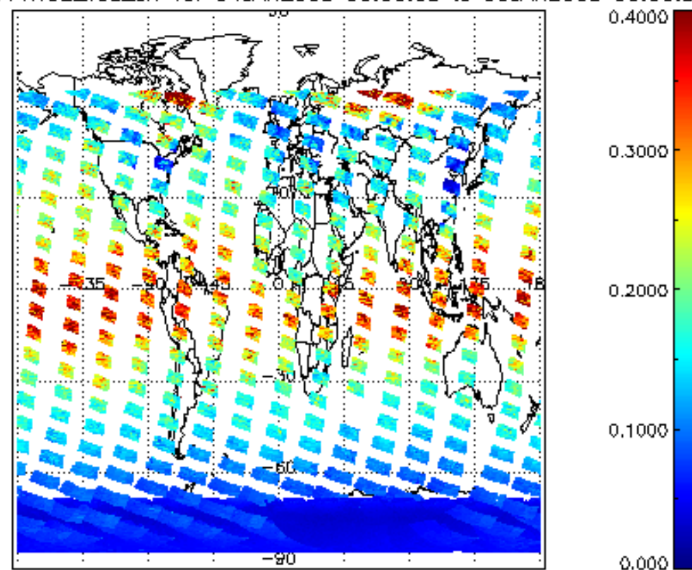
SCIOL2P_NADUV1NO2_vcd_err for 04JAN2008 00:00:00 to 05JAN2008 00:00:00
