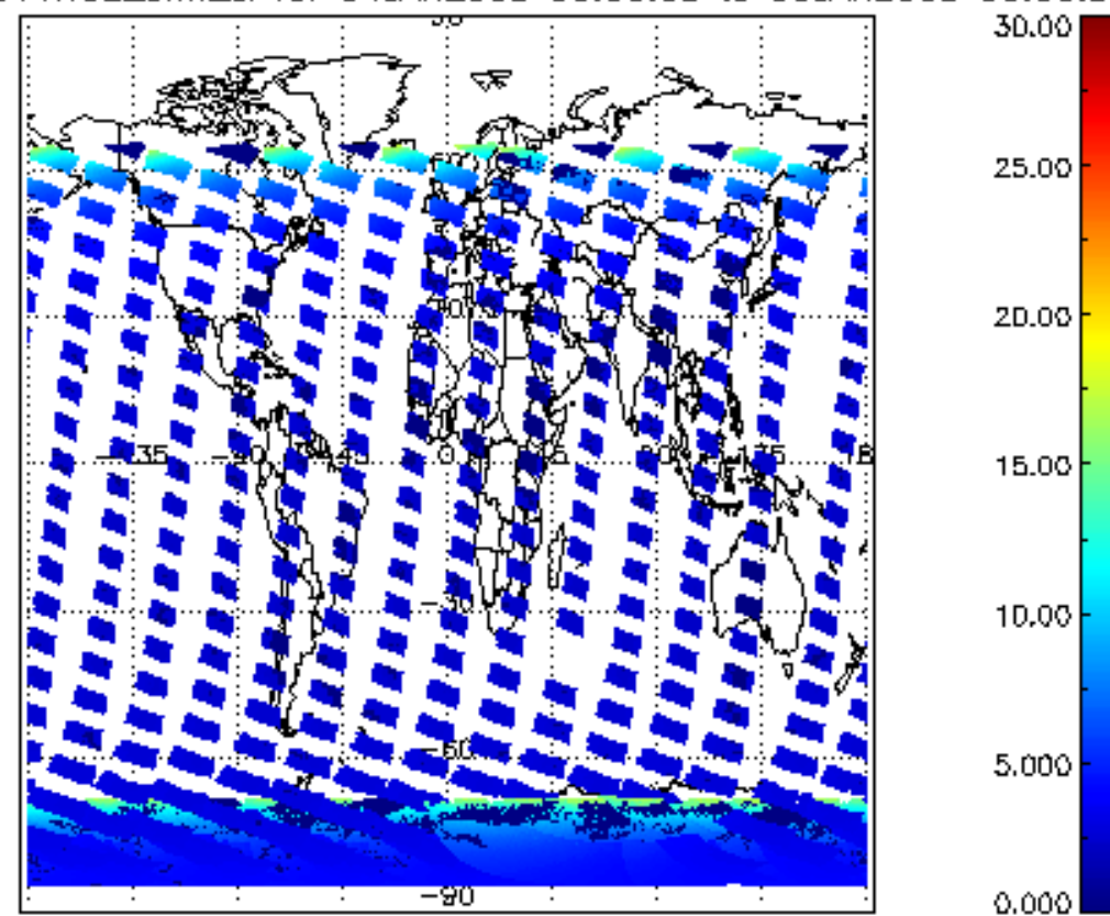
SCIOL2P_NADUV1NO2_amf_cl for 04JAN2008 00:00:00 to 05JAN2008 00:00:00
