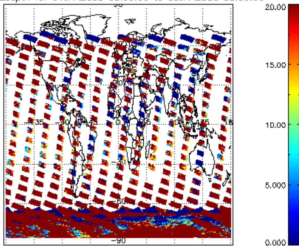
cLopt_depth for 04JAN2008 00:00:00 to 05JAN2008 00:00:00
