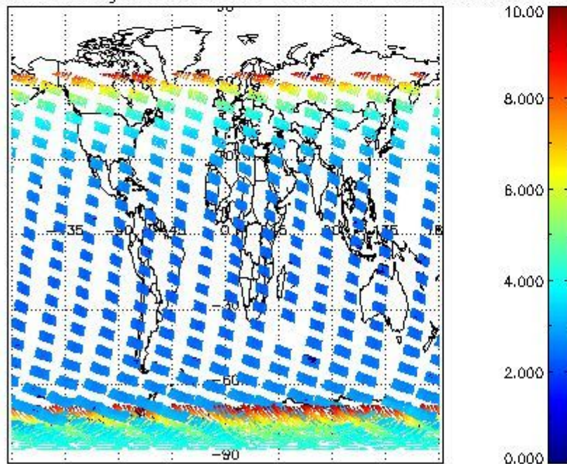
SCIOL2P_NADUV003_amf_gr for 04JAN2008 00:00:00 to 05JAN2008 00:00:00
