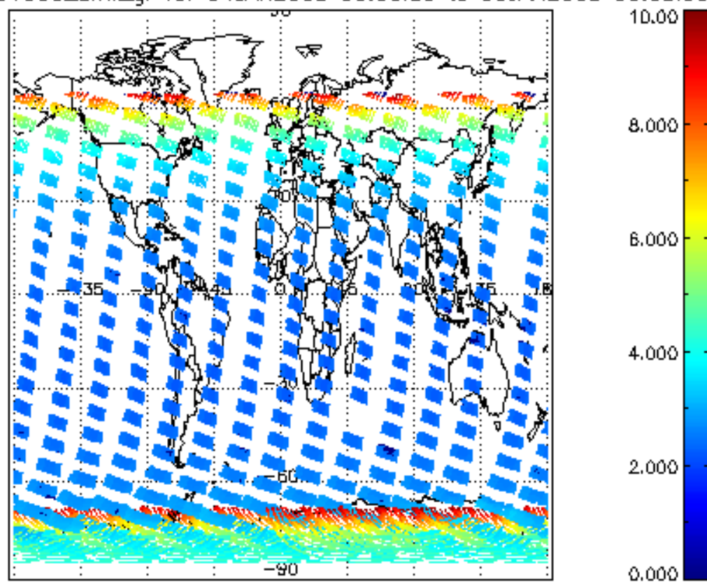
SCIOL2P_NADUV003_amf_gr for 04JAN2008 00:00:00 to 05JAN2008 00:00:00
