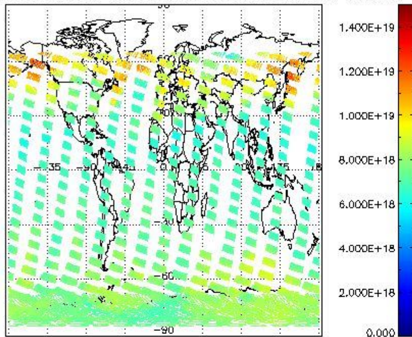
SCIOL2P_NADUV003_vcd for 04JAN2008 00:00:00 to 05JAN2008 00:00:00
