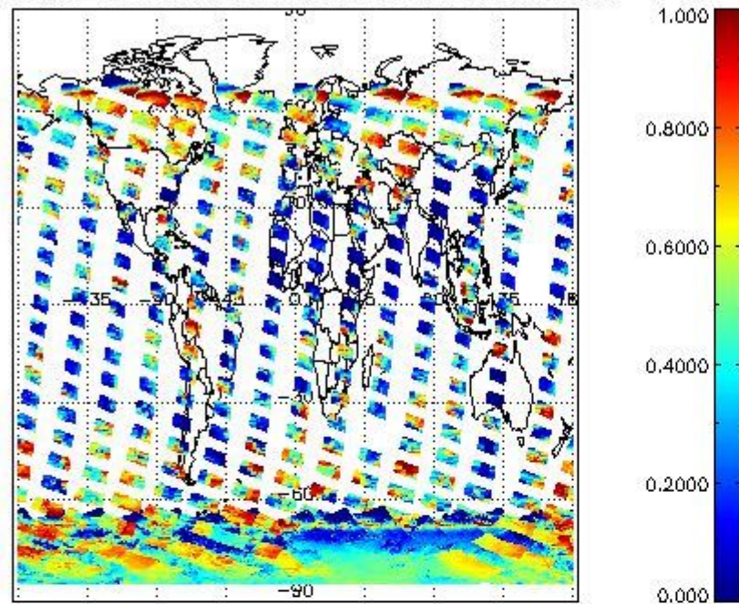
cL_frac for 04JAN2008 00:00:00 to 05JAN2008 00:00:00
