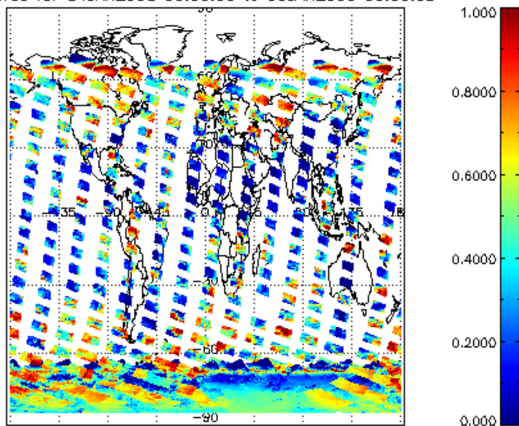
cL_frac for 04JAN2008 00:00:00 to 05JAN2008 00:00:00
