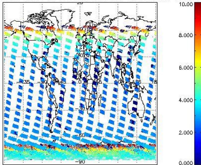
SCIOL2P_NADUV003_amf_cl for 04JAN2008 00:00:00 to 05JAN2008 00:00:00
