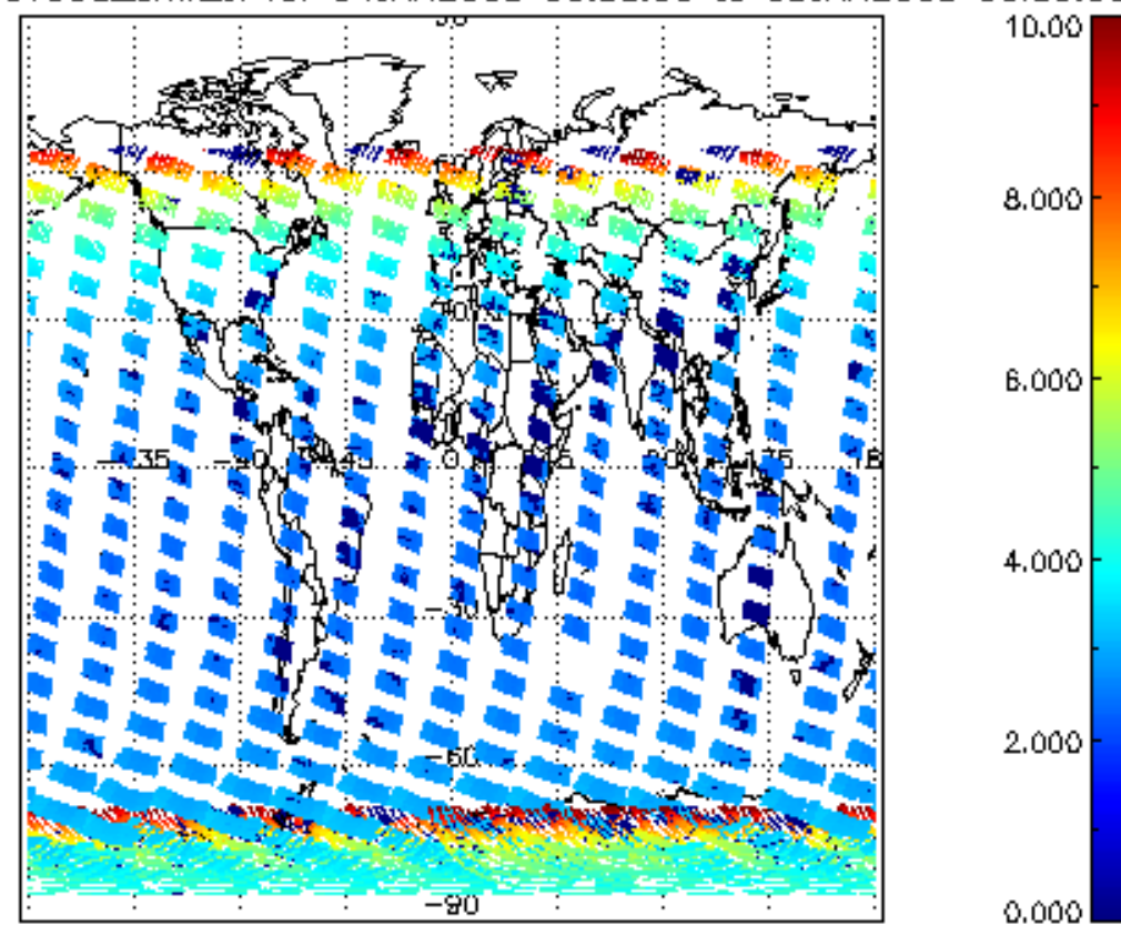
SCIOL2P_NADUV003_amf_cl for 04JAN2008 00:00:00 to 05JAN2008 00:00:00
