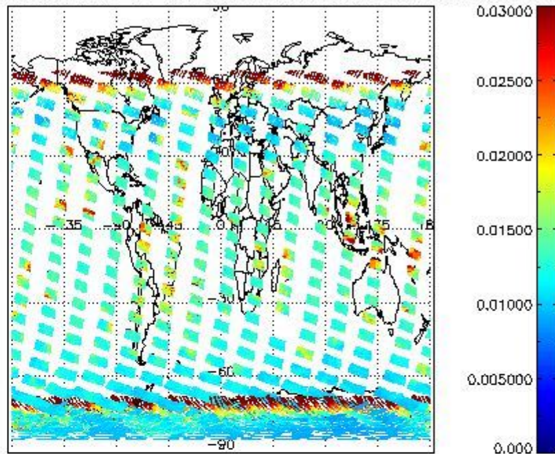
SCIOL2P_NADUV003_vcd_err for 04JAN2008 00:00:00 to 05JAN2008 00:00:00
