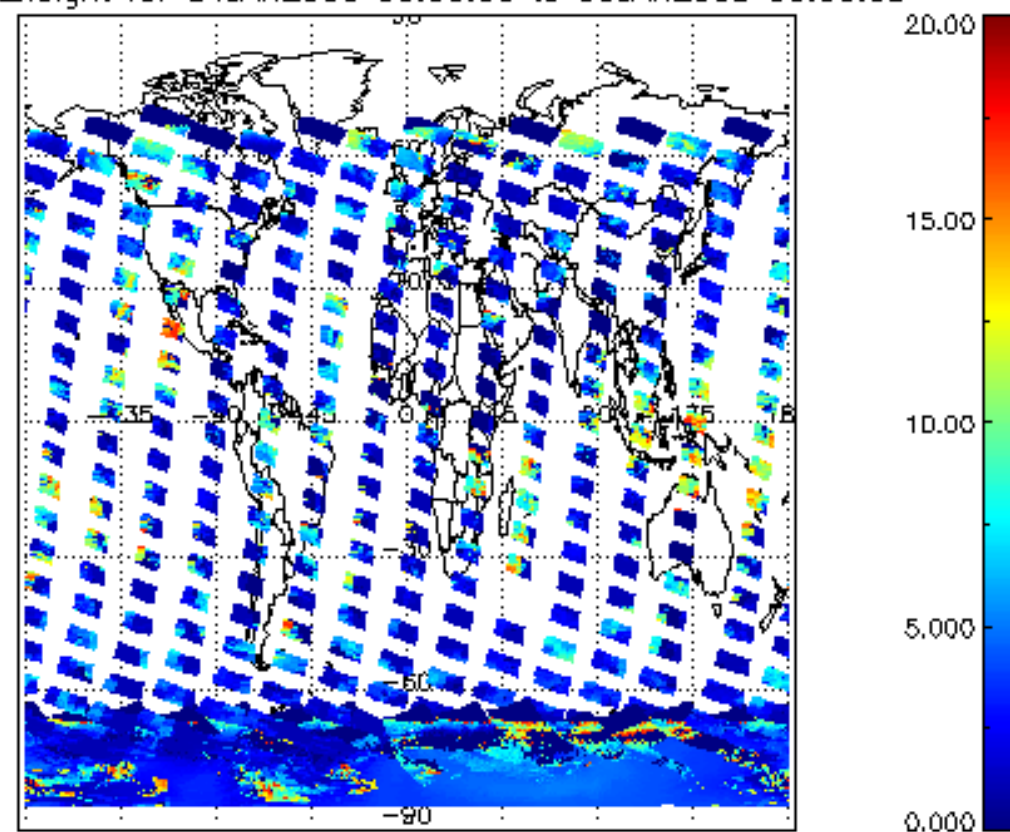
cL_top_height for 04JAN2008 00:00:00 to 05JAN2008 00:00:00
