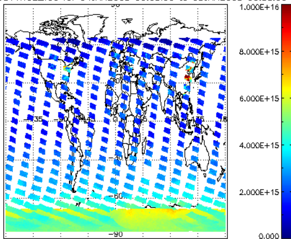
SCIOL2P_NADUV1NO2_vcd for 04JAN2008 00:00:00 to 05JAN2008 00:00:00
