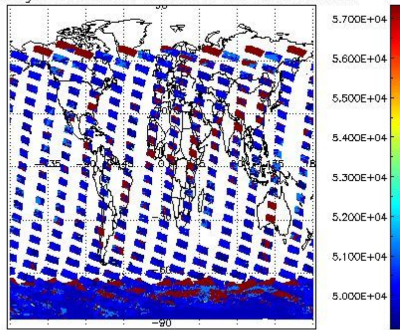
cloud_flags for 04JAN2008 00:00:00 to 05JAN2008 00:00:00
