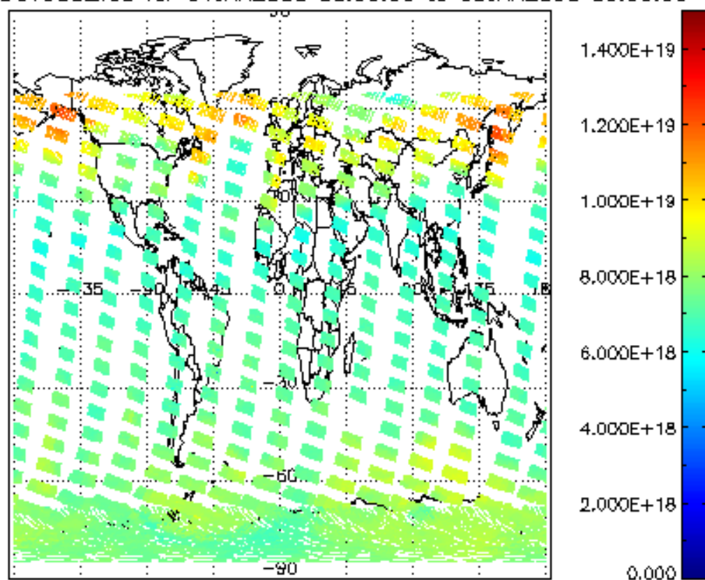
SCIOL2P_NADUV003_vcd for 04JAN2008 00:00:00 to 05JAN2008 00:00:00
